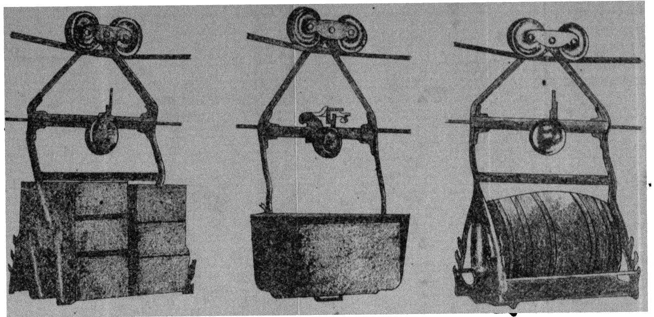
CARRIERS FOR THE "OTTO" AERIAL ROPEWAYS.
