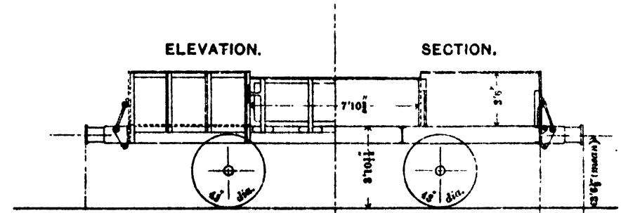
LOW SIDED GOODS WAGON.
