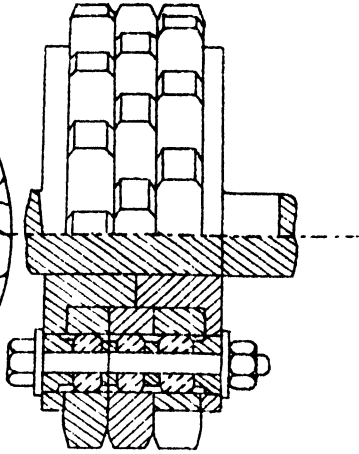
DETAILS OF THE RACK.
