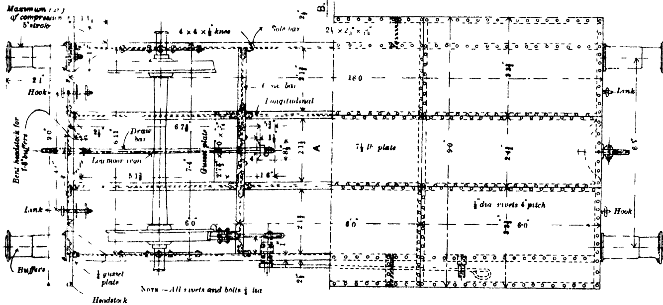
TOP PLAN
