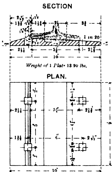
BEARING PLATE. For Dog spikes
