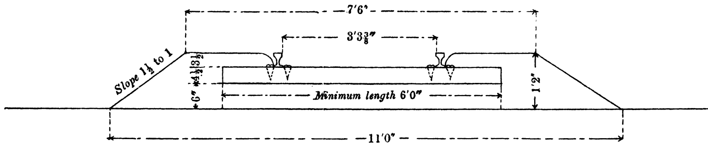
Type C. Metre Gauge—Flat-footed Rails on wooden sleepers, without bearing-plates.
