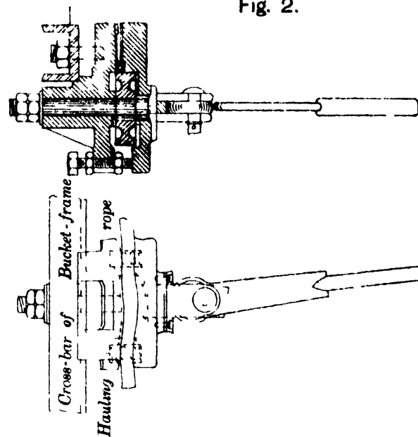
FRICTION GRIP WITH CORRUGATED JAWS
