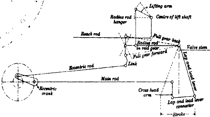
Diagram showing outline and names of parts of Walschaerts gear
