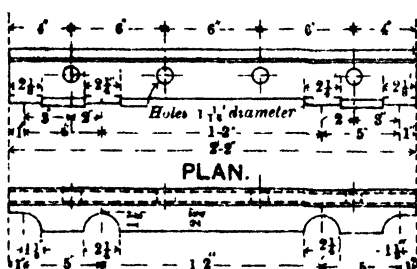
ELEVATION OF FISHPLATES. Notched for Coach screws.
