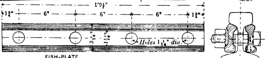
FISH-PLATE. Scale—2 Inches = 1 Foot.
