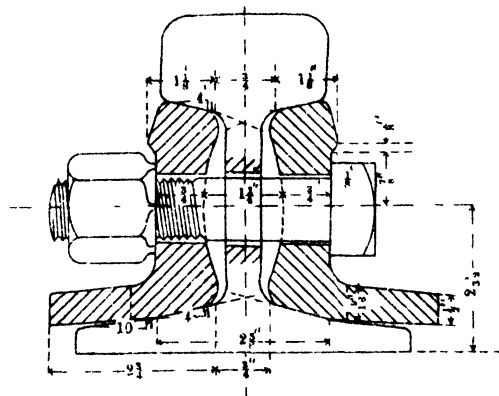
SECTION OF FISHPLATES
