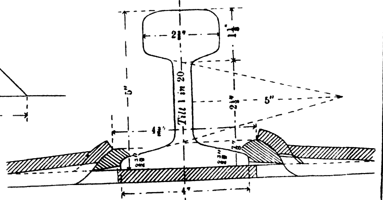
SECTION OF RAIL AND RAIL SEAT.
