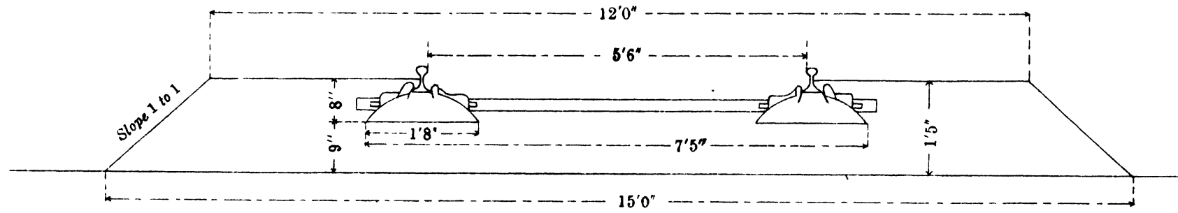
BALLAST SECTION. Scale— \frac{1}{4} Inch = 1 Foot.
