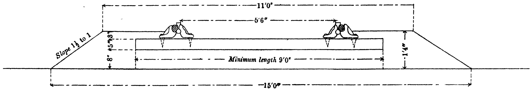
Type A. Standard Gauge—Bull-headed Rails in Chairs, with wooden sleepers.
