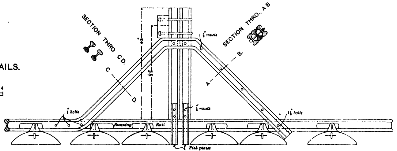
SIDE ELEVATION.
