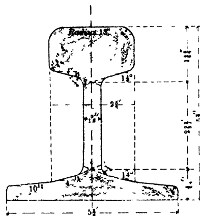
SECTION OF RAIL
