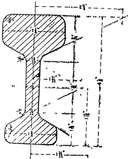
FIG. 9. SECTION OF 50 lbs BULL-HEADED RAIL
