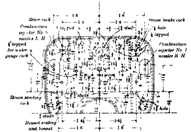
BACK ELEVATION OF FIRE BOX SHOWING POSITION OF MOUNTINGS.
