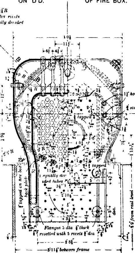
HALF SECTION ON D.D.
