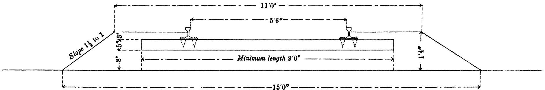
Type B. Standard Gauge—Flat-footed Rails on wooden sleepers, with bearing-plates.
