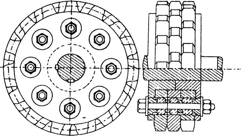
Fig. 5. DETAILS OF PINION.
