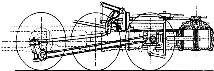
Development of Walschaerts gear completed
