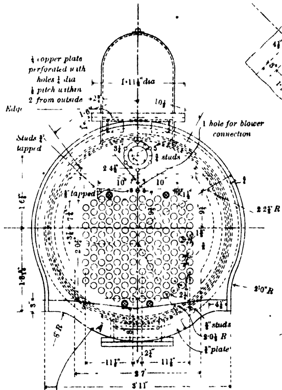
FRONT ELEVATION OF BOILER.
