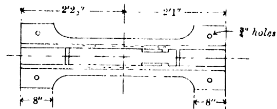
PLAN OF BOX.
