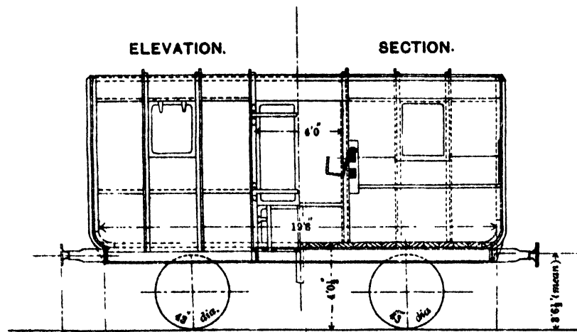
COVERED GOODS FOUR WHEELED WAGON.
