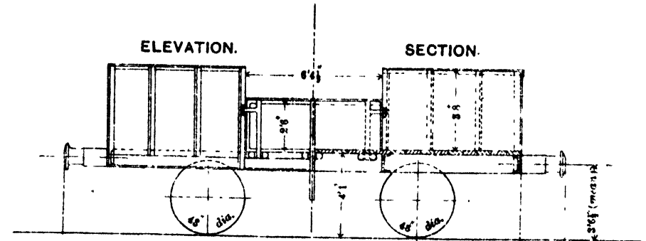
HIGH-SIDED GOODS WAGON
