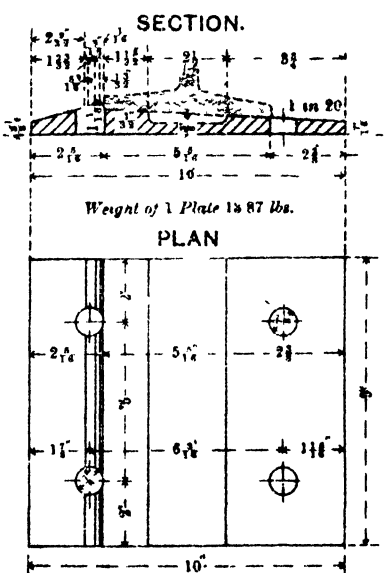
BEARING PLATE. For Coach screws.
