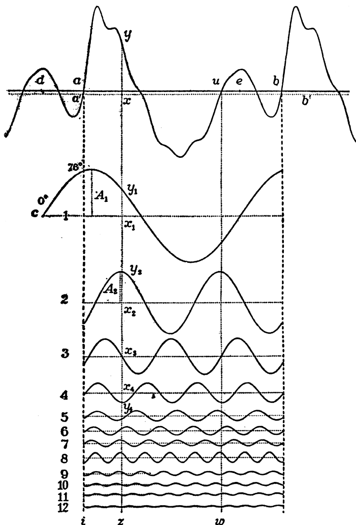
FIG. 25. AN ORGAN PIPE CURVE AND ITS HARMONIC COMPONENTS
