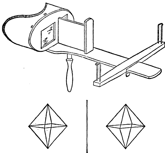
FIG. 28. THE BREWSTER STEREOSCOPE AND A SAMPLE SLIDE
