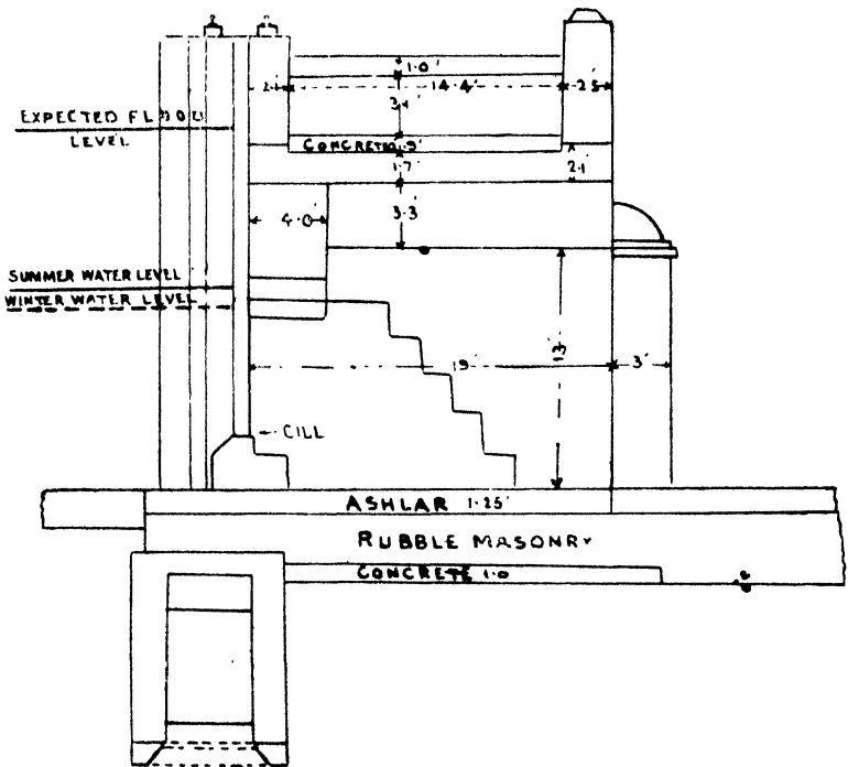
DIAGRAM OF A REGULATOR FOR A CANAL OLD ARRANGEMENT
