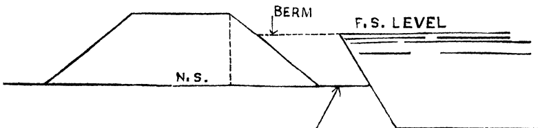
BERM LEFT AT NATURAL SURFACE
