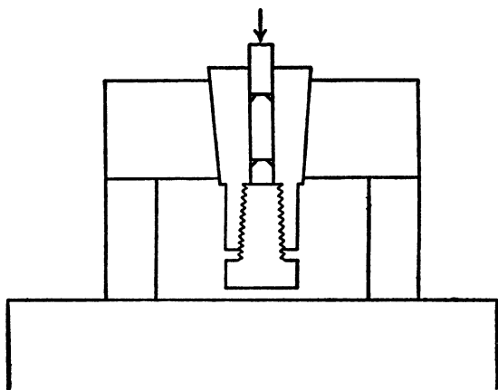
FIGURE 2.—Simple method of giving external support to a pressure vessel by using the thrust on the piston, which produces internal pressure to push the whole vessel into a supporting conical sleeve.
