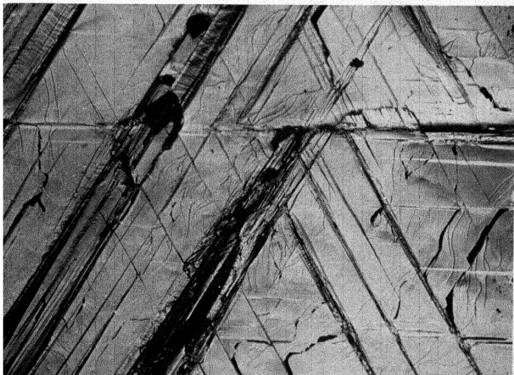
2. Fractograph—or photomicrograph of an unpolished and unetched fracture surface—for metallic bismuth, showing geometric markings which contain the story of deformation and fracture. Magnified 35 times.
