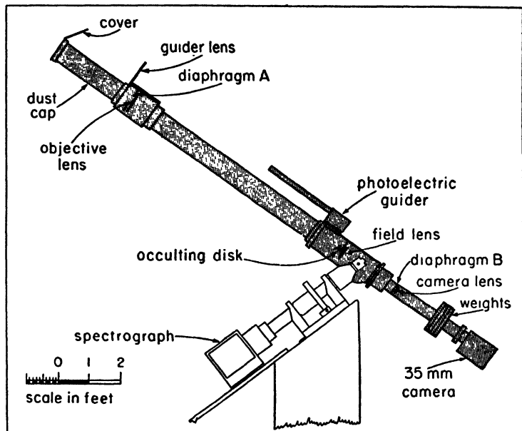
FIGURE 1.—The operating principles of the coronagraph are illustrated in this schematic diagram of the High Altitude Observatory coronagraph. Lyot, inventor of the coronagraph, found that sunlight scattered into the image of an ordinary telescope from the following sources rendered such telescopes useless for artificial eclipse photography:
