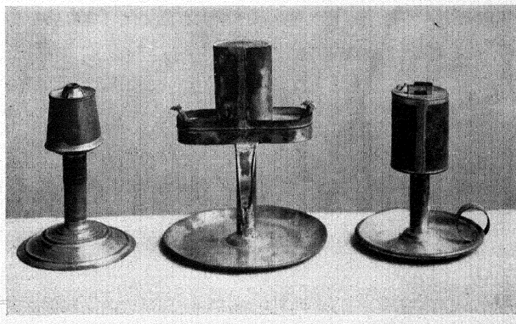
Three patent models of tin lard-burning lamps: Left , Harvey Temlinson's patent, Geneva N. Y., September 1, 1843, embodying an Argand burner with copper air tube. Middle , Zebulon Warroll's patent, Chester Hill, Ohio, February 7, 1842, depending upon gravity for flow of fuel, the heat from the flame warming the lard in the reservoir. Right , One of several patents by Robert Cornelius, of Philadelphia, this one dated April 6, 1843. A ribbon wick with copper conductor strip is the working principle.
