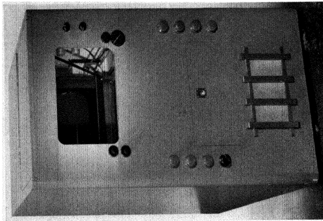
2. STEREOTELEVISION RECEIVER: POLAROID SCREENS IN FRONT OF THE TWO VIEWING TUBES AND IN FRONT OF THE EYES OF THE OBSERVER MAKE ONE IMAGE VISIBLE TO EACH EYE
