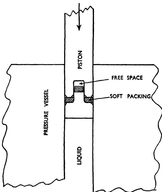
FIGURE 1.—Application to a piston of the principle by which the pressure in the packing is automatically maintained at a pressure greater by a fixed percentage than the pressure in the liquid. Leaks therefore cannot occur.
