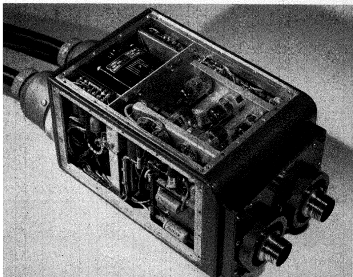
2. STEREOTELEVISION CAMERA FOR CONVEYING THREE-DIMENSIONAL IMAGES
