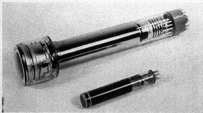
2. SIZE REDUCTION AND SIMPLIFICATION IN TELEVISION PICK-UP TUBES: THE IMAGE ORTHICON AND THE VIDICON
