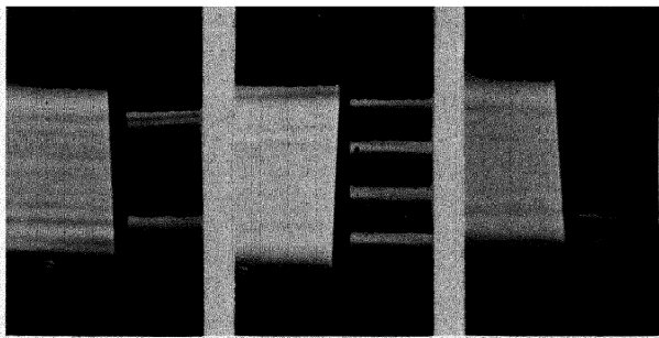
2. Transmission of a wide ultrasonic beam through aluminum wedges of increasing taper. Transmission occurs only where the wedge thickness is such as to give internal resonance. Courtesy Bell Laboratories Record .
