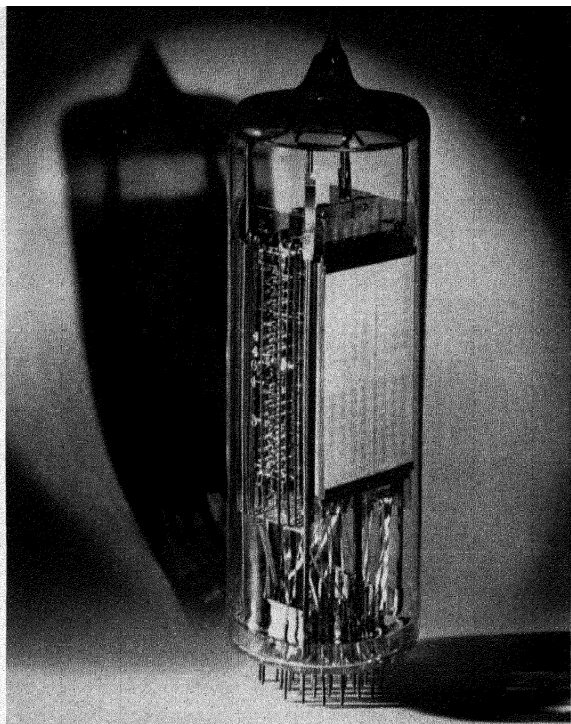
1. THE SB-256 TUBE, AN EFFICIENT ELECTRONIC MEMORY
