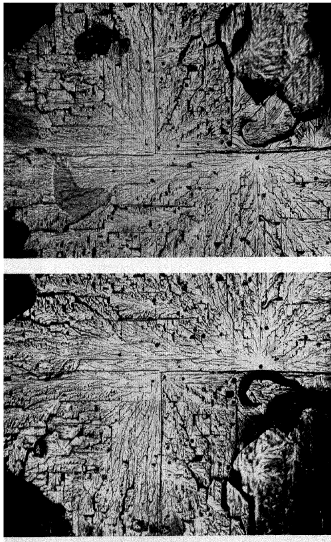
Obverse and reverse fractographs showing both matching faces of a fracture traverse through a single grain of iron. The sharp 90° angles prove this to be a cubic cleavage. The markings display an elaborate architecture within the grain, and their variations on the opposite surfaces are informative. Magnified 100 times.
