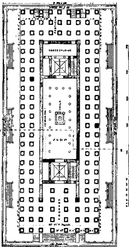
PLAN OF TEMPLE OF DIANA AT TPHLSUS (Rebuilt on this plan in the third century B.C.)
