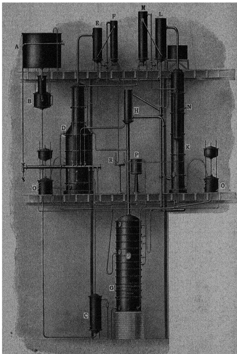
FIG. 29.—TRIPLE-COLUMN CONTINUOUS STILL.
