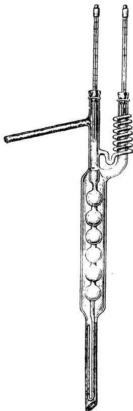
FIG. 39. FRACTIONATING COLUMN FOR FUSEL OIL ANALYSIS.
