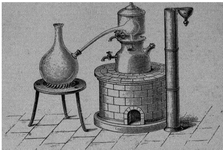
FIG. 9. DISTILLING APPARATUS.
