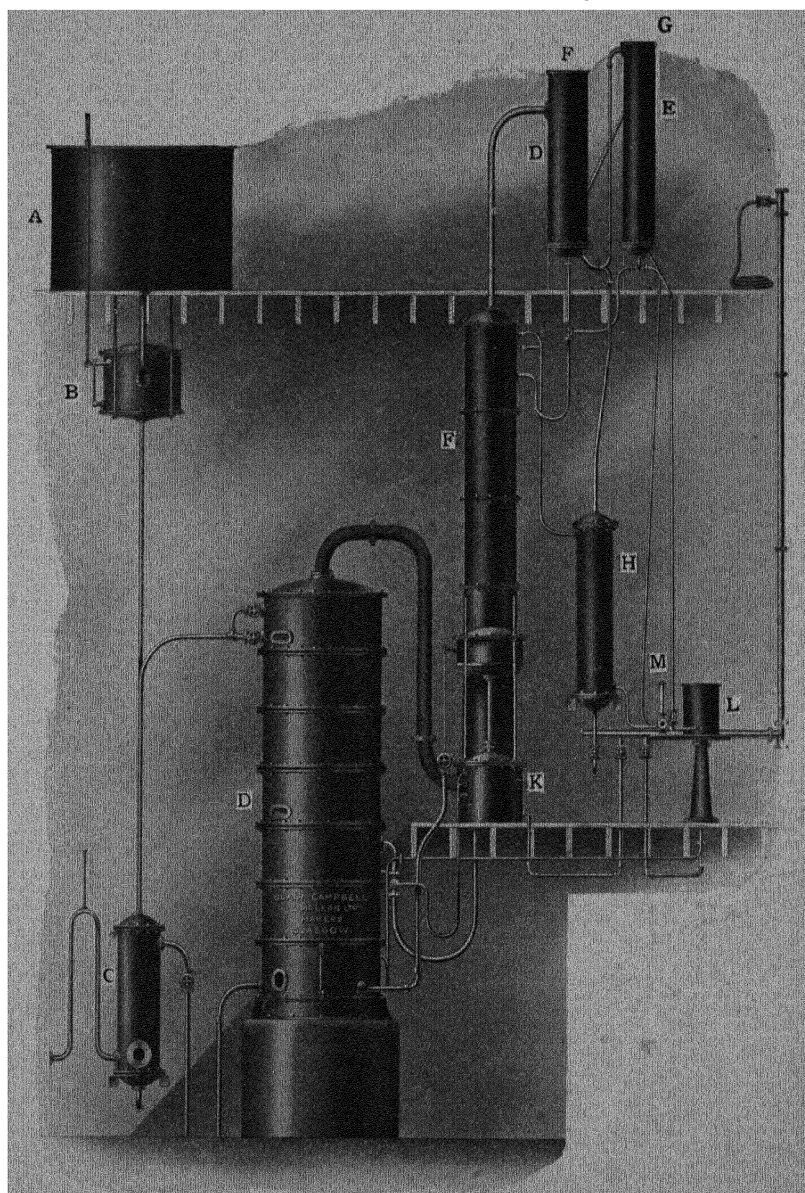
FIG. 26.—DOUBLE COLUMN CONTINUOUS STILL.
