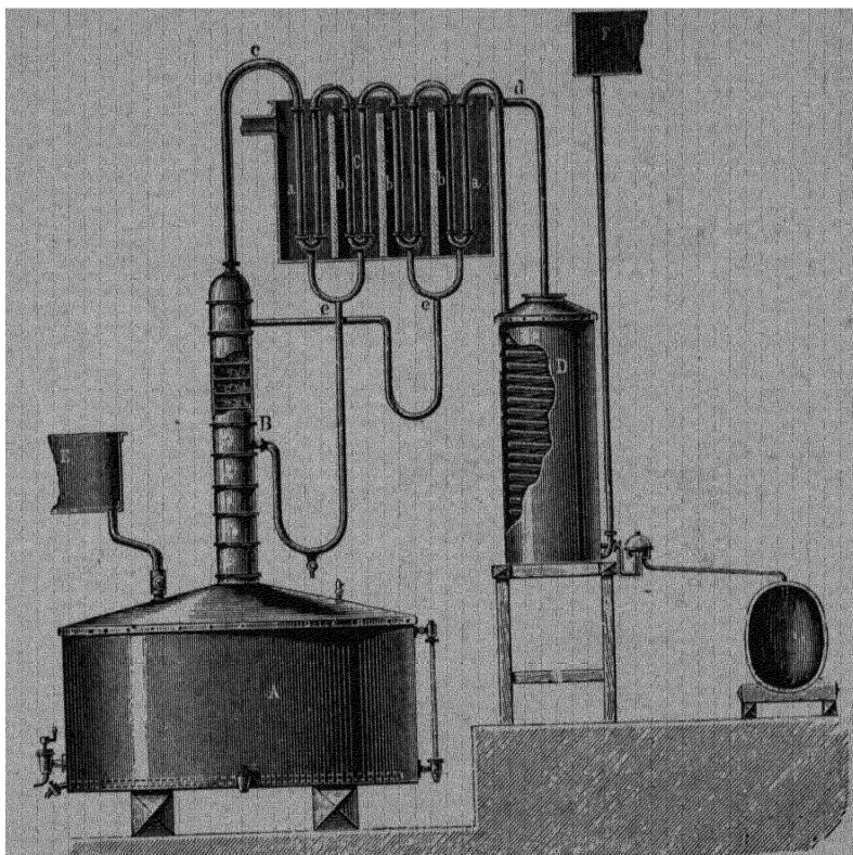
FIG. 27.—FRENCH COLUMN APPARATUS FOR RECTIFICATION OF ALCOHOL.
