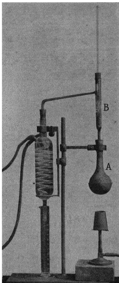
FIG. 38. DISTILLATION APPARATUS. Used in determining the boiling range of wood-naphtha and mineral oil. A, copper flask; B, distilling tube with glass beads.
