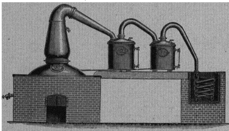
FIG. 41.—COPPER RUM STILL.
