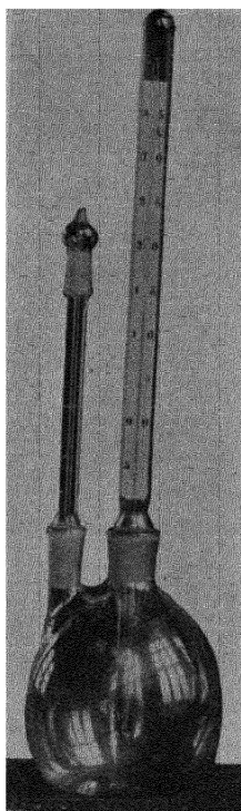
FIG. 33. — GEISLER'S FORM OF PYKNOMETER.
