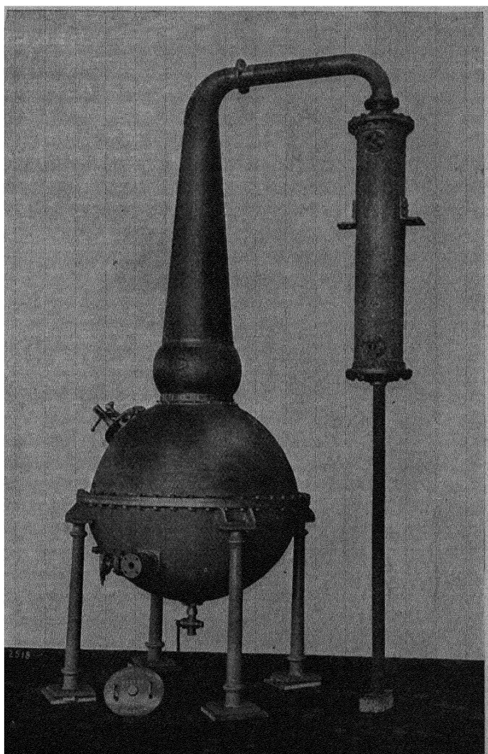
FIG. 40.— STEAM JACKETED STILL.
