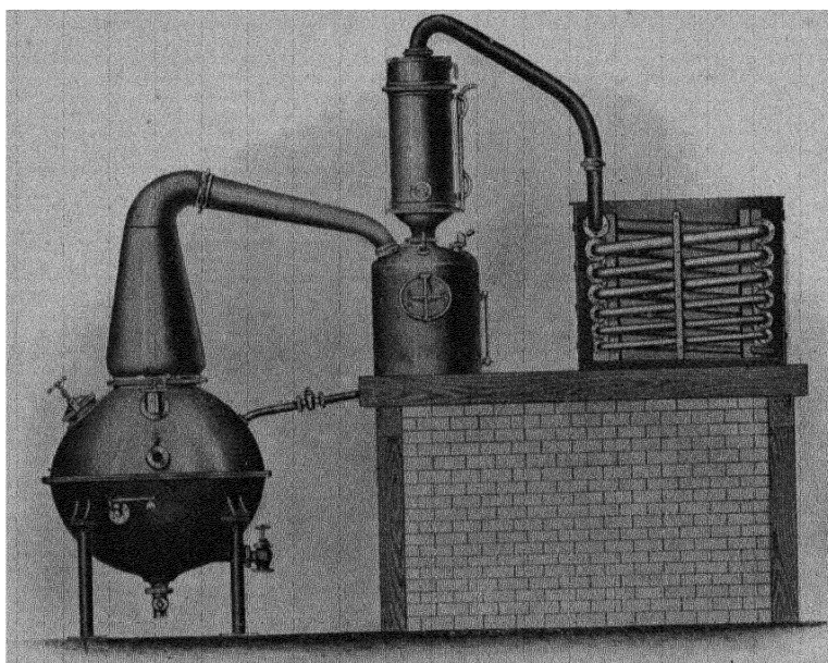
FIG. 43. —STEAM-JACKETED POT-STILL.
