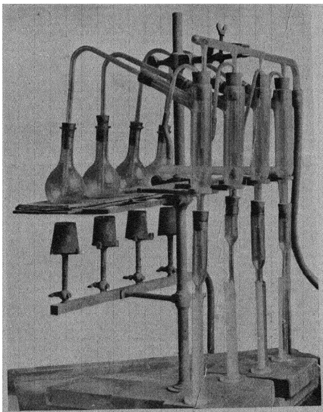
FIG. 35.—BATTERY OF DISTILLING APPARATUS.
