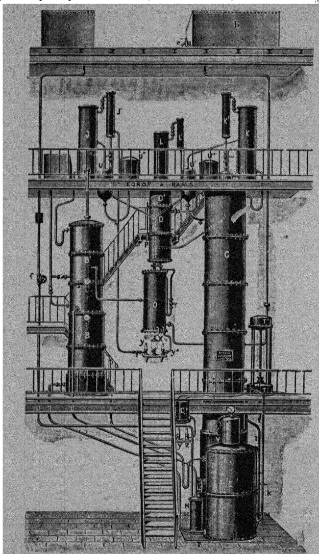
FIG. 28. MODERN STILL, FOR CONTINUOUS RECTIFICATION.
