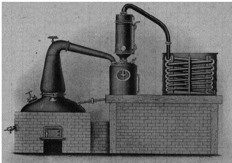
FIG. 42.—STILL FOR DIRECT FIRING.
