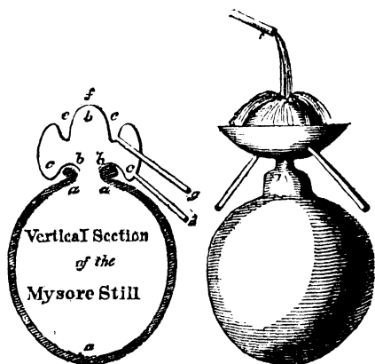
FIG. 8.—ANCIENT STILL USED IN SOUTHERN INDIA.
