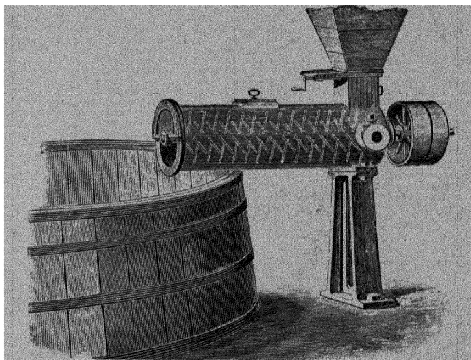
FIG. 18. MASH TUN, WITH STEEL'S MASHING MACHINE.
