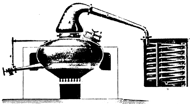
FIG. 22. SIMPLE POT-STALL, FIRE HEATED, WITH CONDENSER. (1) Boiling vessel; (2) still-head; (3) condenser worm (Ha-lam Foundry Co., Ltd., Derby).
