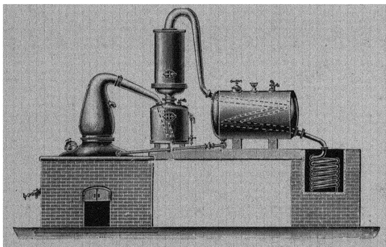
FIG. 44.—POT-STILL FOR DIRECT FIRING.
