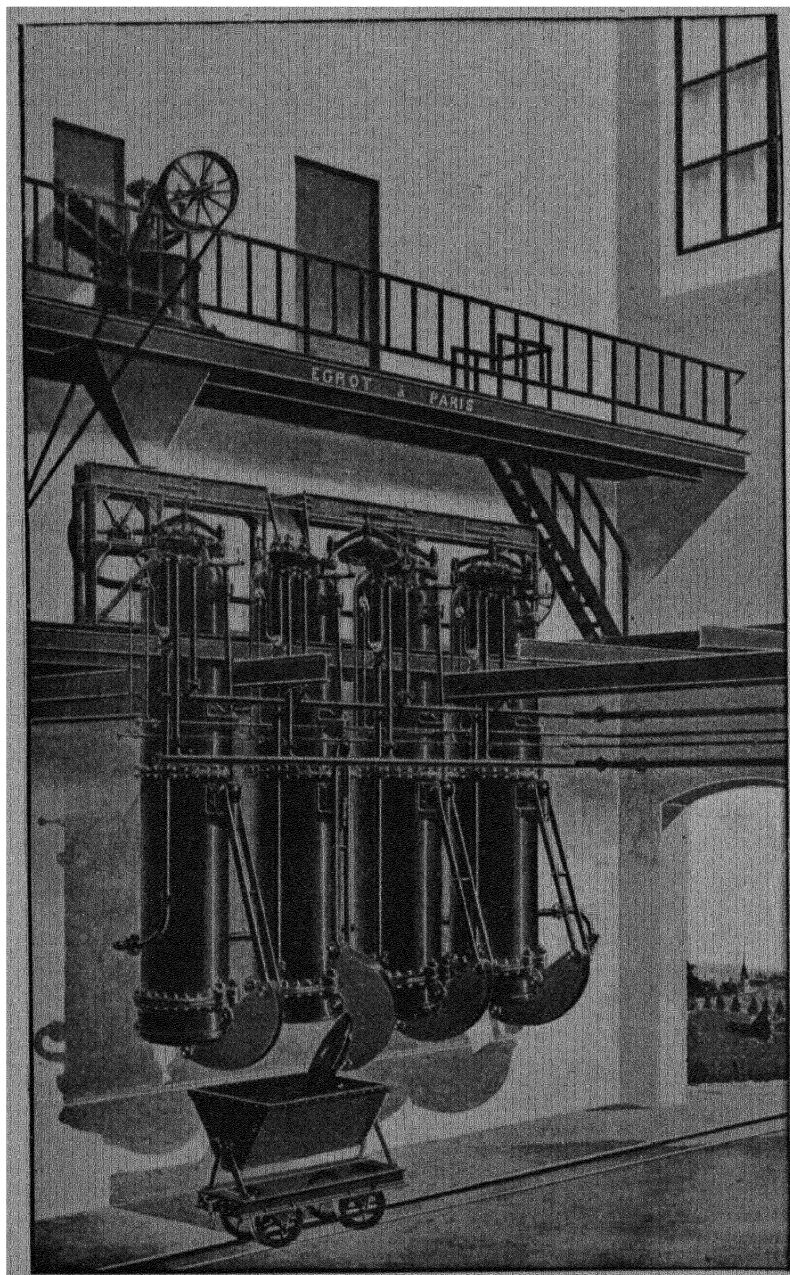
FIG. 21. BATTERY OF FOUR DIFFUSION VATS FOR EXTRACTION OF SUGAR. BEETS (Egrot and Grangé, Paris).
