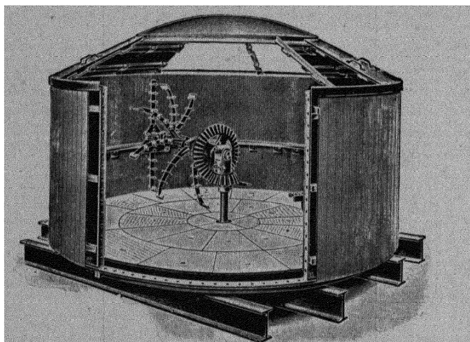
FIG. 19.--MASH TUN WITH RAKE STIRRING GEAR (Blair, Campbell, and McLean).
