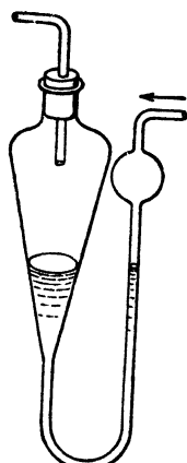
FIG. 3.—Chudiakow's vessel.
