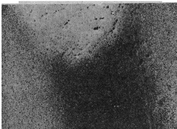
FIG. 11. Segregated Core in Mild Steel Bar \times 15 diam. (Reproduced half size—i.e., \times 7\frac{1}{2} diam.)
