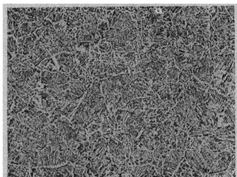
FIG. 10. Overheated Mild Steel, \times 15 diam. (Reproduced half size—i.e., \times 7\frac{1}{2} diam.)
