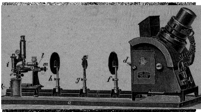
FIG. 5. "GENERAL ARRANGEMENT OF THE SLIT ULTRA MICROSCOPE."
