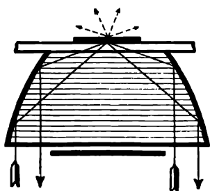
FIG. 5. SECTION OF PARABOLOID CONDENSER, SHOWING PATH OF RAYS.
