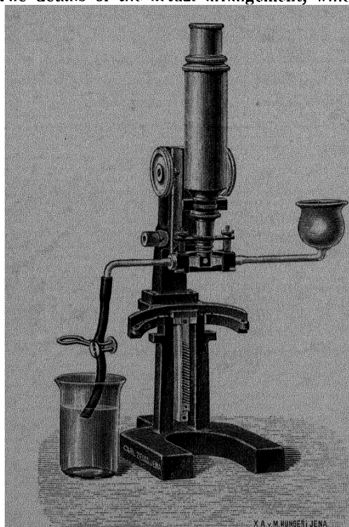
FIG. 4. MICROSCOPE WITH QUARTZ CHAMBER FOR ULTRA-MICROSCOPIC EXAMINATION OF LIQUIDS.
