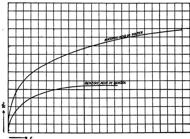
FIG. 13.—TYPICAL ADSORPTION ISOTHERMS.
