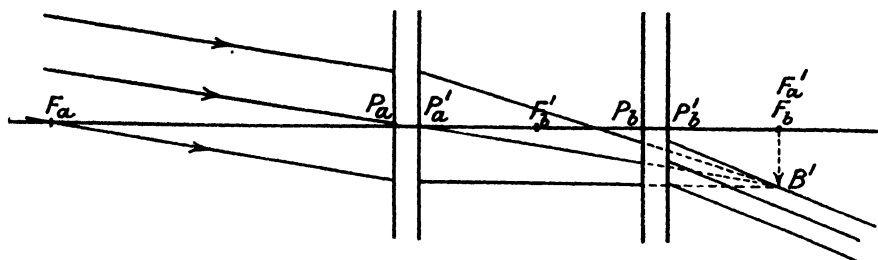
FIG. 12. GALILEAN TELESCOPE (Diagrammatic)
