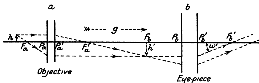
FIG. 57. A GAUSSIAN DIAGRAM OF THE MICROSCOPE
