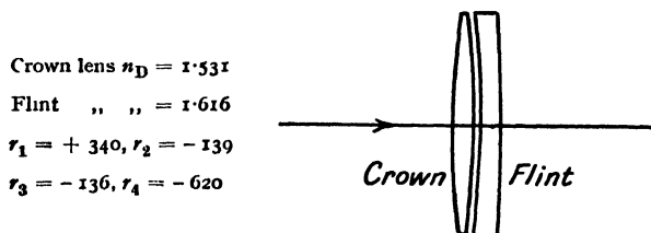
FIG. 14. FRAUNHOFER OBJECTIVE
