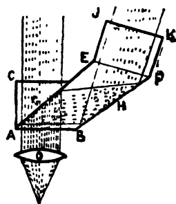
(R. & J. Beck, Ltd.) FIG. 125. BINOCULAR MICROSCOPE SYSTEM
