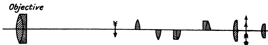
FIG. 30. VARIABLE POWER TELESCOPE (OTTWAY)
