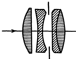
FIG. 152(a). THE ZEISS TESSAR ( f/4.5 )
