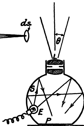
FIG. 177(b). SPHERE EPISCOPES
