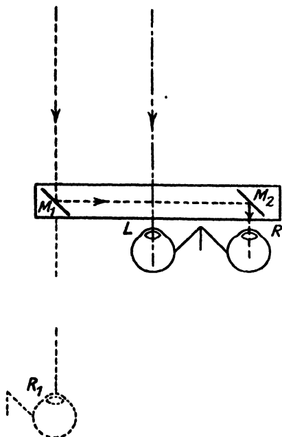
FIG. 114. STRATTON'S PSEUDOSCOPE
