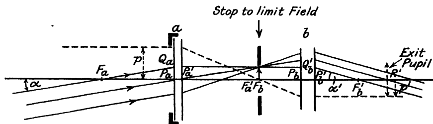
FIG. 11. ASTRONOMICAL TELESCOPE (Diagrammatic)
