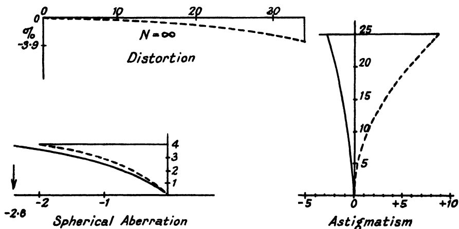
FIG. 154. FRENCH LANDSCAPE LENS ( f/15 )
