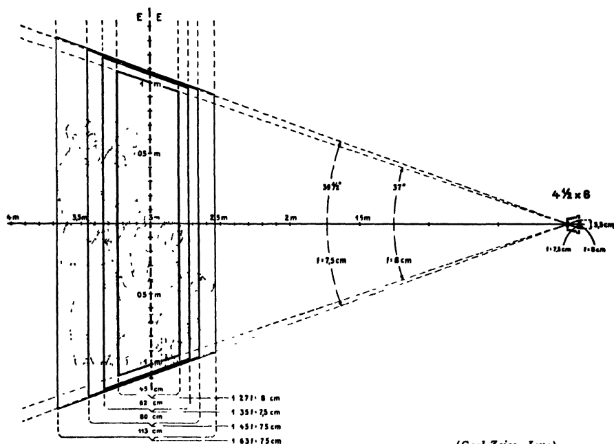
FIG. 161. FOCAL DEPTH FOR A 6 \times 4\frac{1}{2} CM. CAMERA USING VARIOUS LENSES
