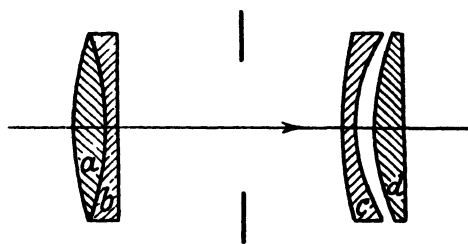
FIG. 150. THE PETZVAL PORTRAIT OBJECTIVE.
