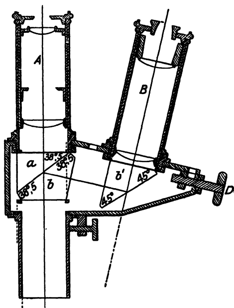
FIG. 127. ABBE STEREOGRAPHIC EYEPIECE SYSTEM
