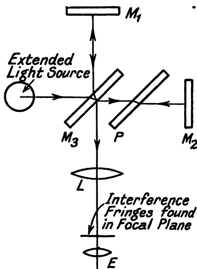
FIG. 199. MICHELSON INTERFEROMETER
