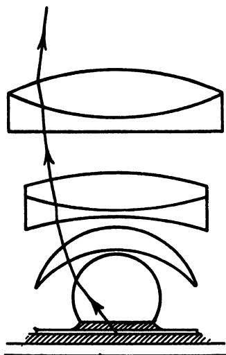
FIG. 60(a). SECTION OF IMMERSION ACHROMAT
