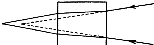
FIG. 126. ALTERATION OF FOCUS POSITION DUE TO BLOCK OF GLASS
