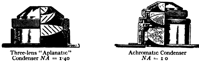
FIG. 64. TYPICAL CONDENSERS (Zeiss)
