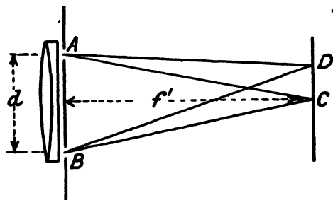
FIG. 192. FIZEAUS' EXPERIMENT
