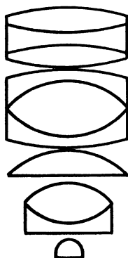
FIG. 60(b). SECTION OF TYPICAL APOCHROMATIC OBJECTIVE
