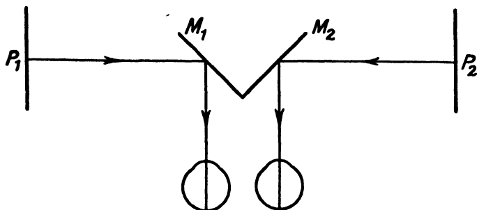
FIG. 107. WHEATSTONE STEREOSCOPE
