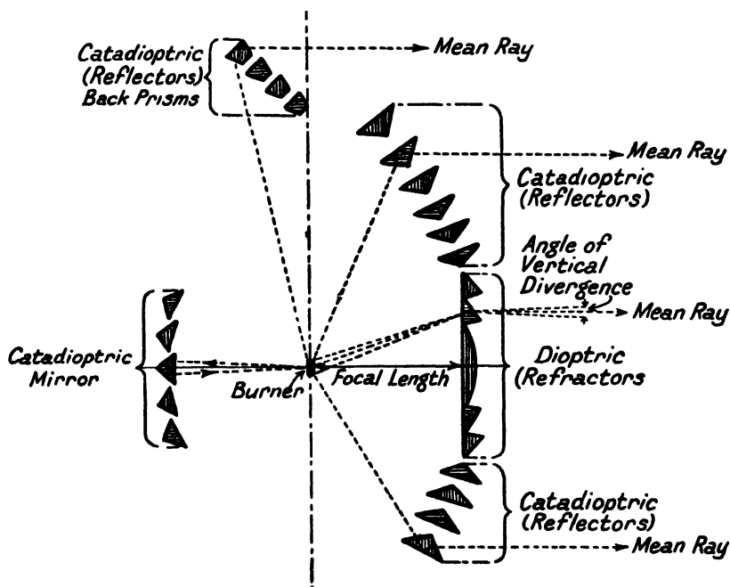
FIG. 184. LIGHTHOUSE PROJECTION SYSTEM
