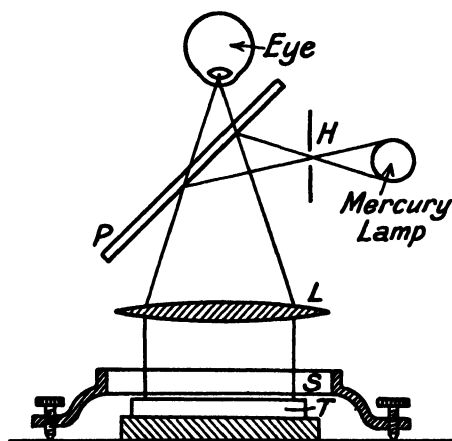
FIG. 198. FIZEAU TYPE INTERFEROSCOPE
