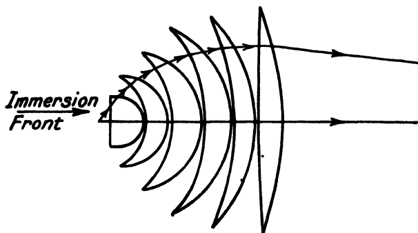
FIG. 96. MONOCHROMAT OBJECTIVE
