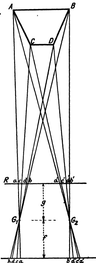
FIG. 110. PERSPECTIVE PROJECTION
