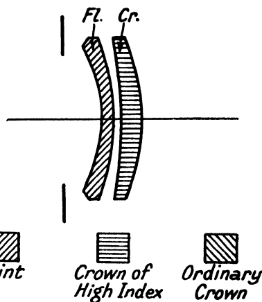
FIG. 145. ANASTIGMATICALLY CORRECTED, SEPARATED DOUBLET
