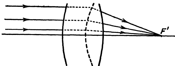
FIG. 157. THE "PRINCIPAL SURFACE" OF A COMA-FREE LENS
