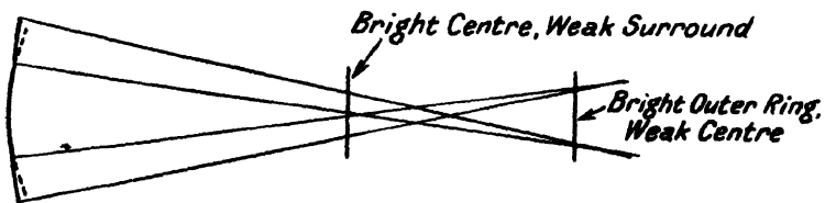
(3) Spherical Over-correction
