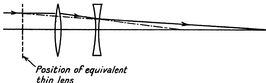
FIG. 162. TELEPHOTO COMBINATION
