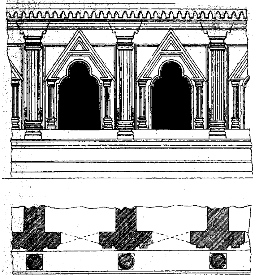
BUNIAR: PLAN AND ELEVATION OF TEMPLE PERISTYLE.
