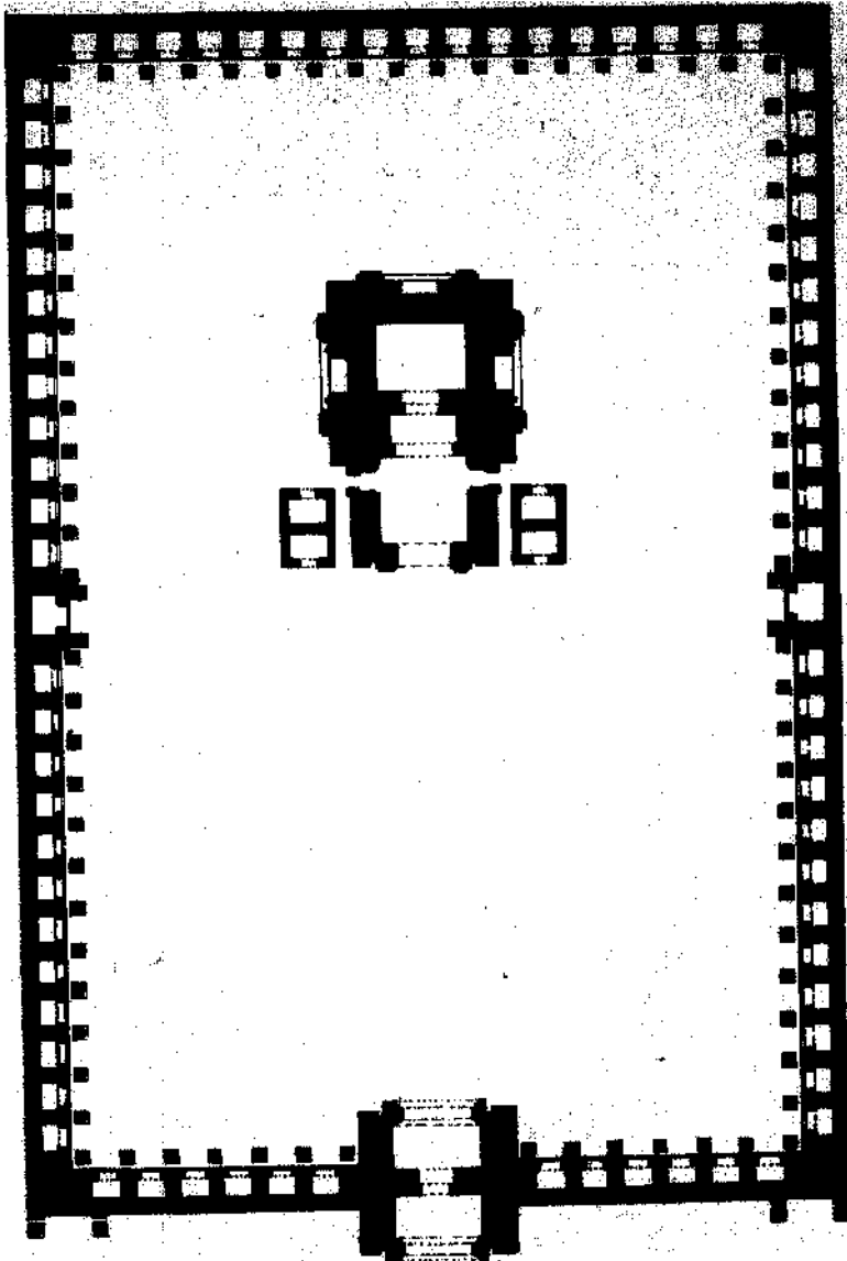
MARTAND: PLAN OF TEMPLE.
