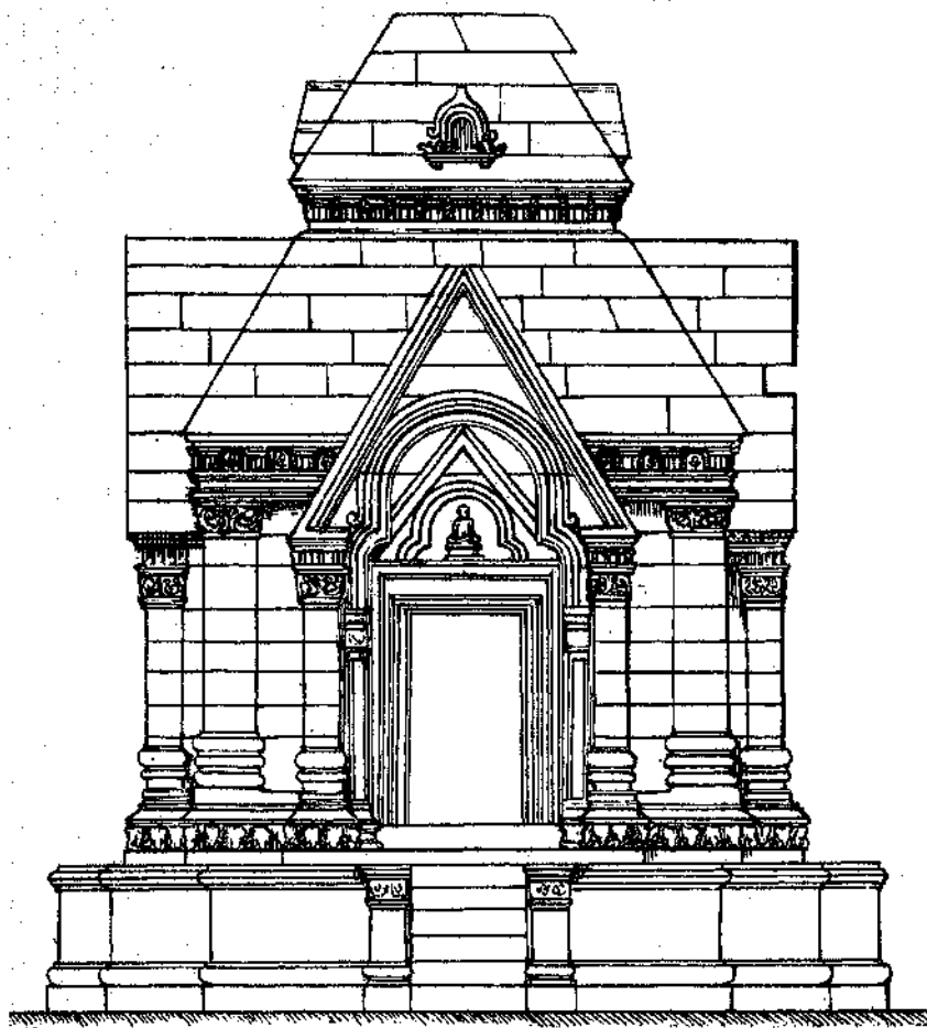
PANDRETHAN : ELEVATION OF TEMPLE.
