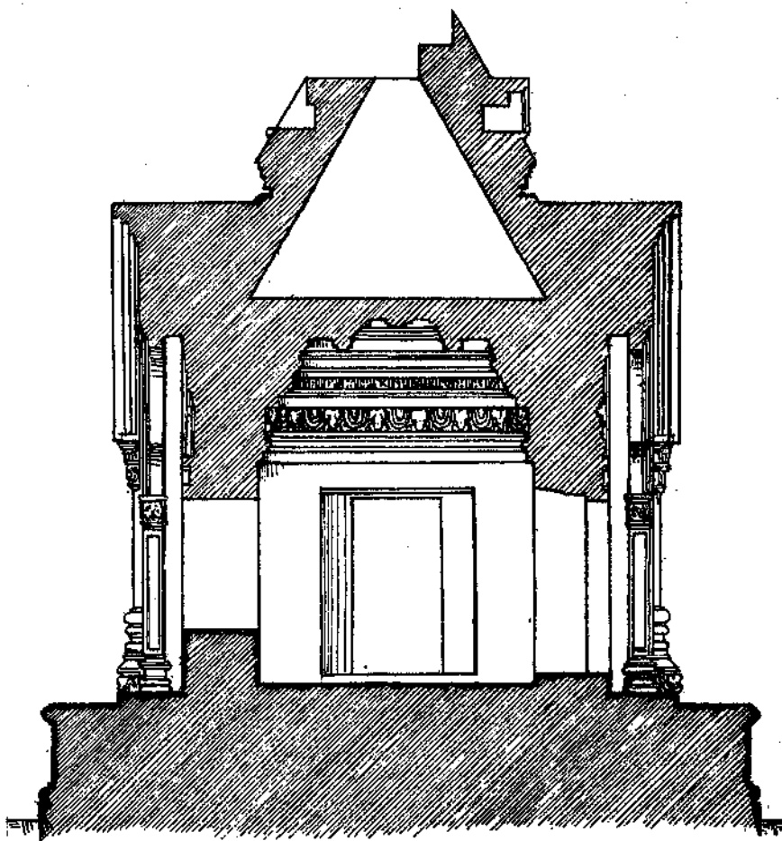
PANDRETHAN : SECTION THROUGH TEMPLE.
