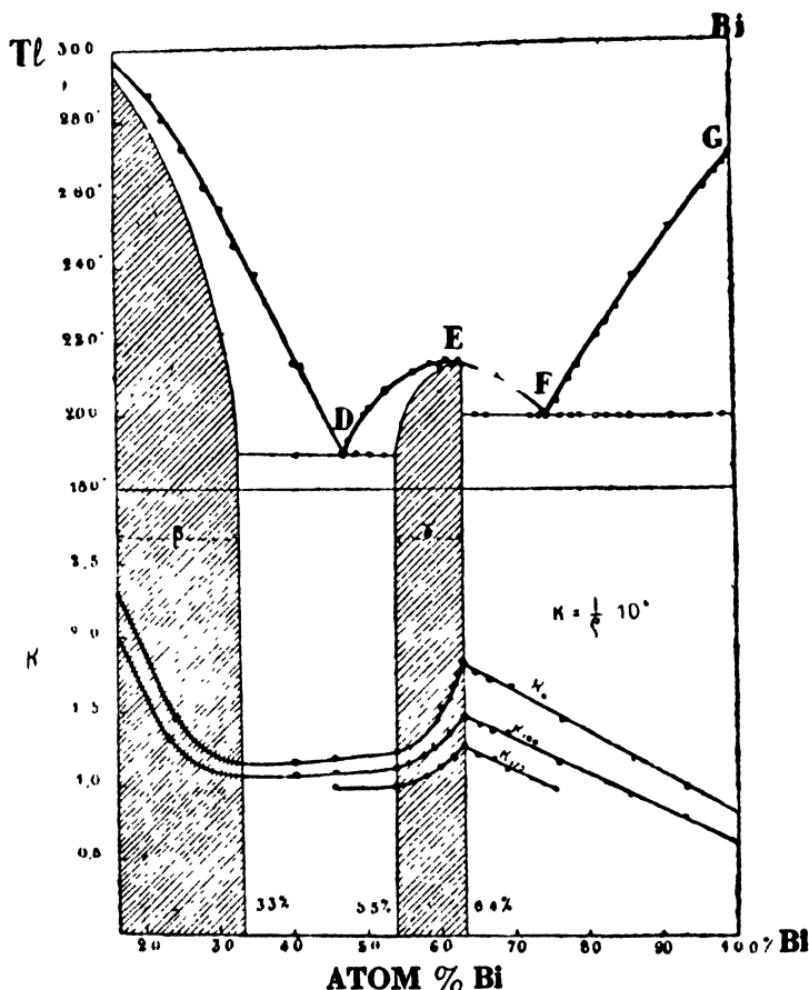
FIG. 7. Freezing-point curve for the system: Thallium plus Bismuth; and curves showing specific conductance of thallium-bismuth alloys at various temperatures.
