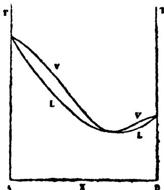
FIG. 11. Liquid-vapor equilibrium at constant temperature of a system forming a minimum-boiling azeotropic mixture.
