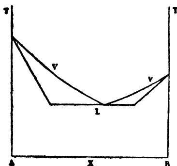
FIG. 12. Liquid-vapor equilibrium of a two liquid phase system at constant pressure.
