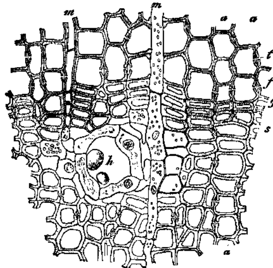
FIG. 53.—Part of a cross-section through the wood of the Scotch fir at the limits of a year's ring. /, Spring wood; s, late wood; „, bordered pit; a, a radial row of tracheides which doubles; h, resin passage; m, medullary rays (x 240).
