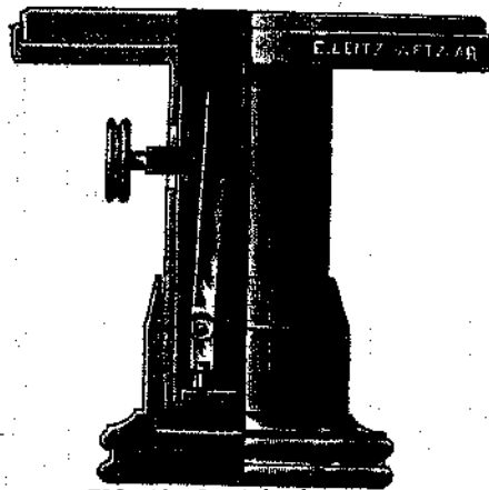
FIG. 29.—Leitz's band microtome.
