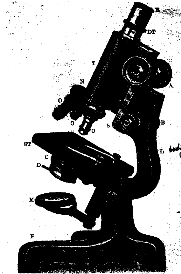
FIG. 3.—Watson's "Service" Microscope. For description see text.
