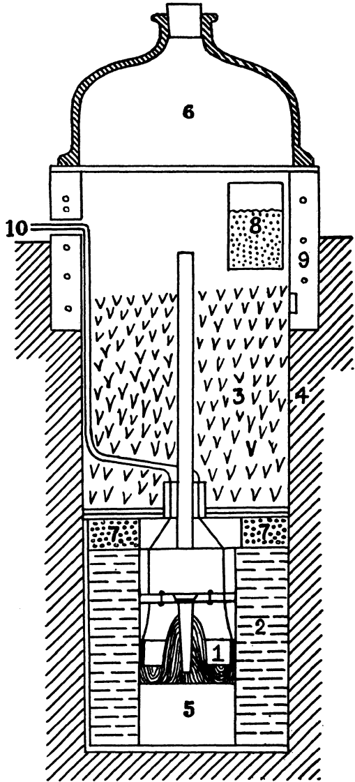
Figure 22. A. Tian's Microcalorimeter.
