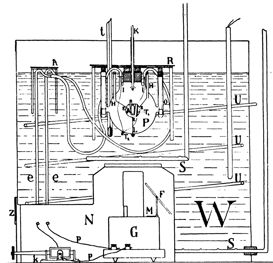
Figure 33. Swietoslowski's Improved Microcalorimeter.
