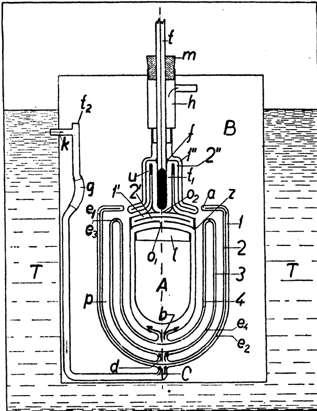
Figure 53. Swietoslowski's Labyrinth Flow Calorimeter.
