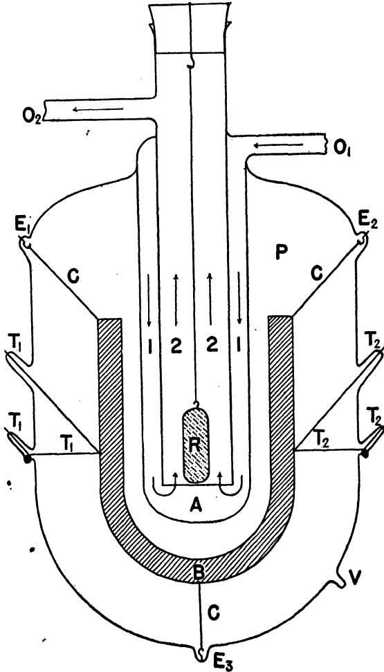
Figure 36. Swietoslowski and Zlotowski's Microcalorimeter for Measuring the Heat of Absorption of Gamma Rays.
