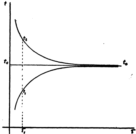
Figure 42. Cooling and Heating Curves of a Thermally Inert Block.
