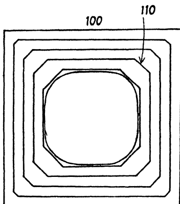
FIG. 9. A rounded crystal of sodium chlorate, on being put into supersaturated solution, develops 110 and 100 faces. The more rapidly growing 110 faces are subsequently eliminated.
