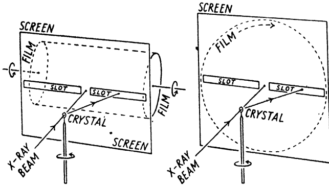
FIG. 108. Moving-film goniometers which record a limited angular range of reflections. Left: Robinson, Cox. Right: Schiebold, Sauter.
