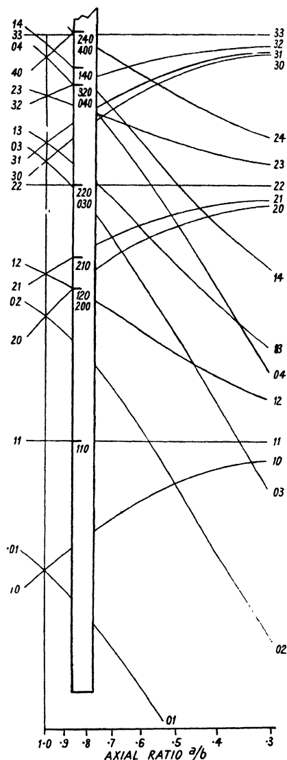
FIG. 79. Graphical method for indexing equatorial reflections on rotation photographs. The pattern shown is that of polychloroprene ( hk0 reflections).
