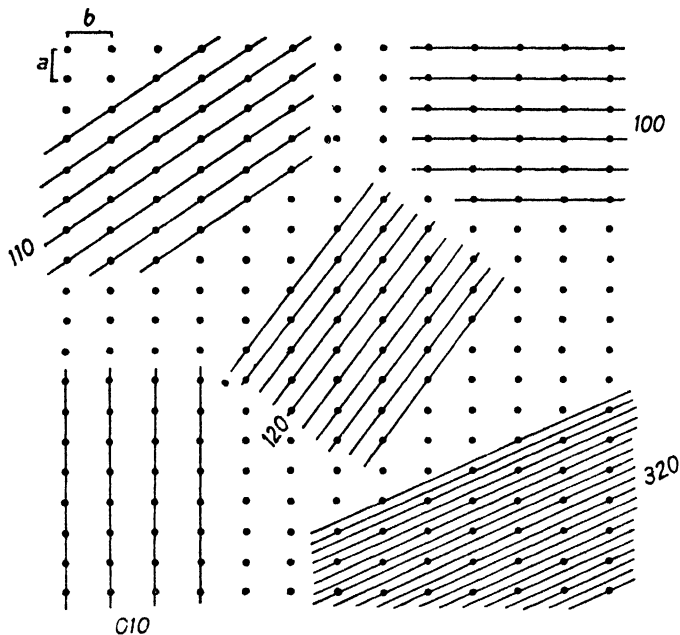
FIG. 10. Various sets of planes in a crystal.
