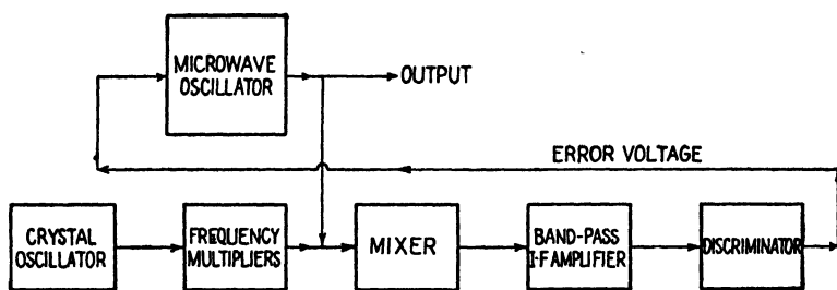
FIG. 6.—Block diagram of an automatic-frequency-control system.
