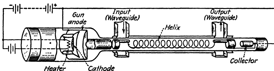
FIG. 27.—Traveling-wave tube.
