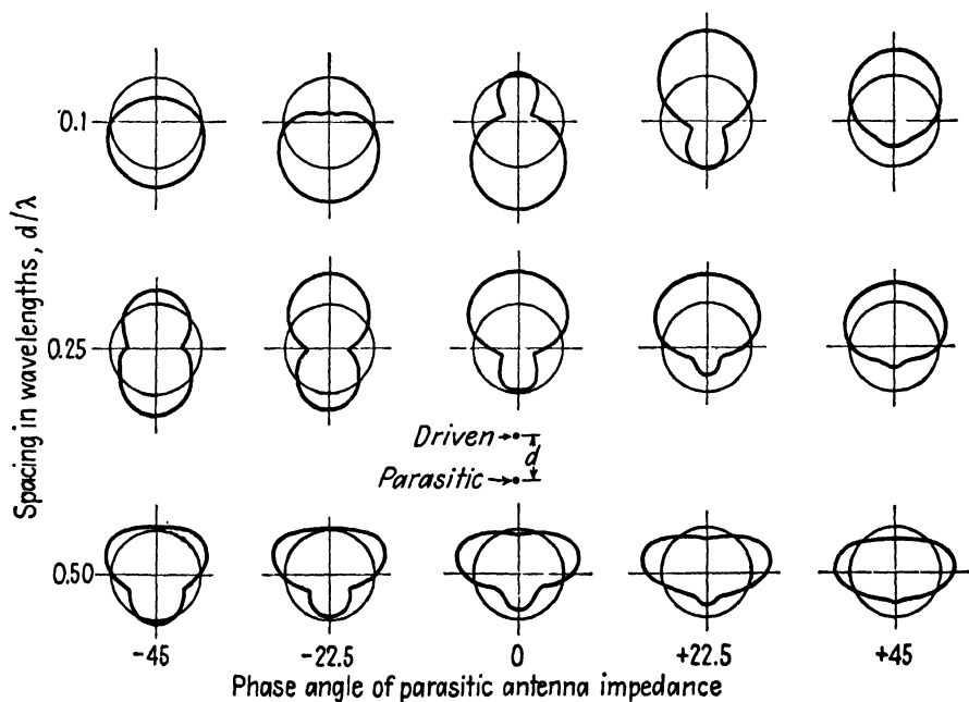
FIG. 15.—Field patterns in the horizontal plane for a driven antenna and a parasitic antenna.
