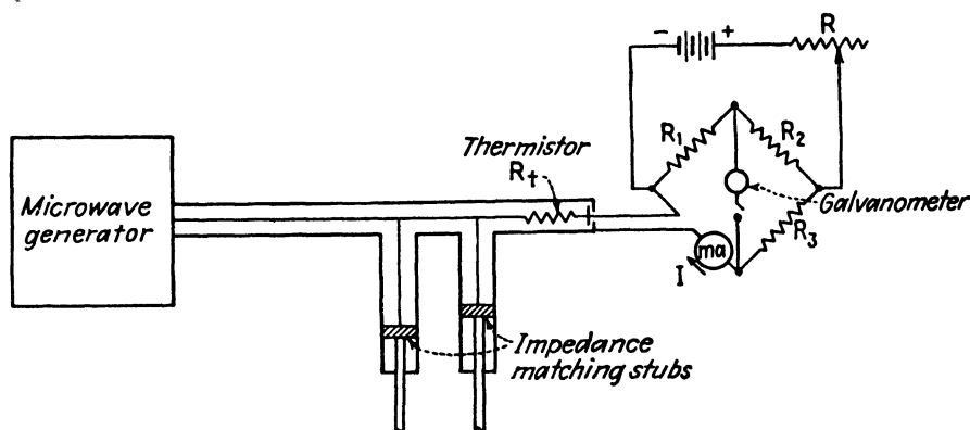
FIG. 6.—Thermistor bridge for power measurement.
