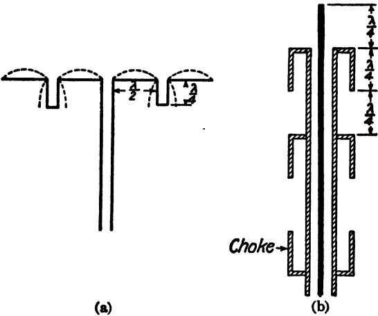
FIG. 12.—Colinear arrays.
