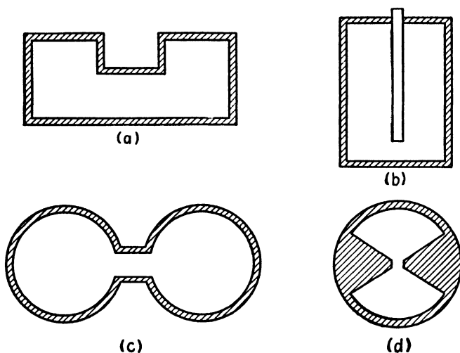
FIG. 8.—Reentrant resonators.
