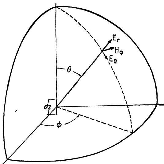
FIG. 1.—Coordinates for the incremental antenna.
