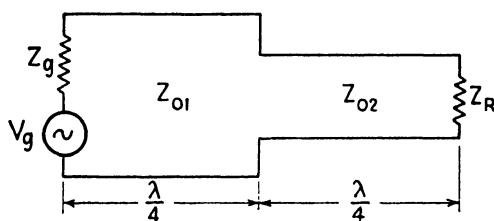
FIG. 11.—Impedance transformer consisting of two quarter-wavelength lines.
