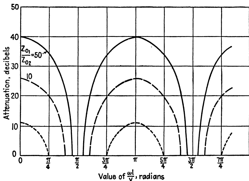
FIG. 22.—Attenuation characteristic of the filter shown in Fig. 18a.
