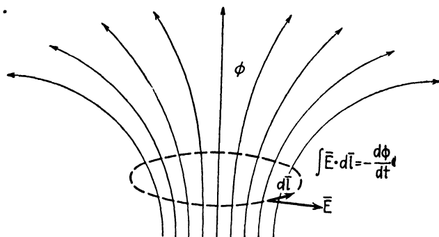
FIG. 1.—An illustration of Faraday's induced emf law.
