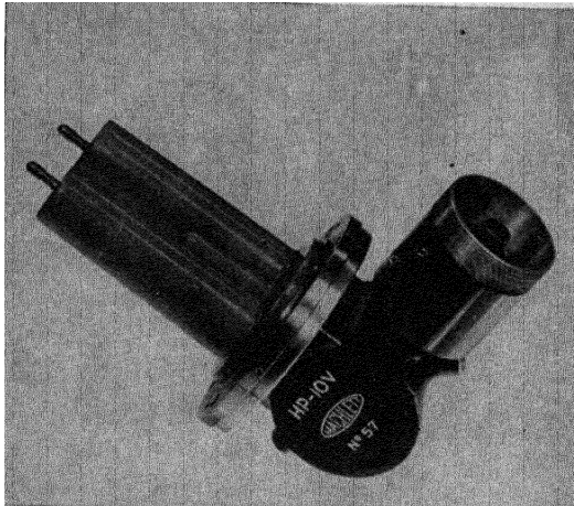
FIG. 3.—High-power cavity magnetron. (Courtesy of the M.I.T. Radiation Laboratory.)
