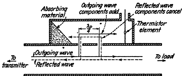
FIG. 8.—Directional coupler.
