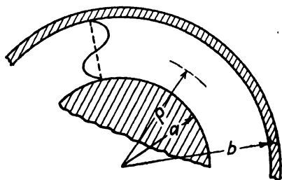
FIG. 9.—Coaxial line.
