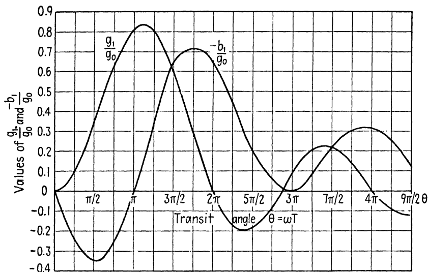
FIG. 6. \omega - c conductance and susceptance of the temperature-limited diode, as a function of transit angle. The susceptance is capacitive for small transit angles.
