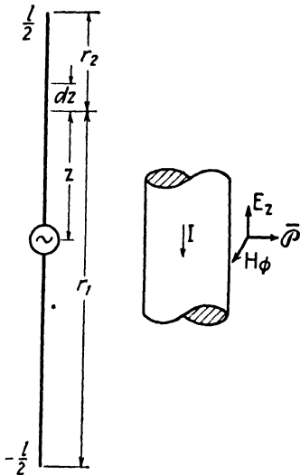
FIG. 3.—Illustration for induced-emf analysis.
