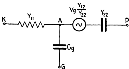
FIG. 10.—Equivalent circuit of the triode at microwave frequencies.
