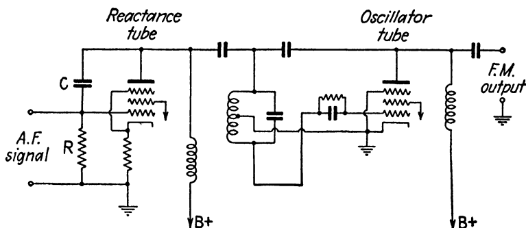
FIG. 5.—Reactance-tube modulator.
