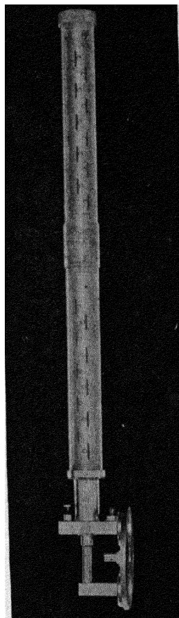
FIG. 15.—Slot antenna for \lambda = 3 centimeters. Beam width to half-power points is 10 degrees.
