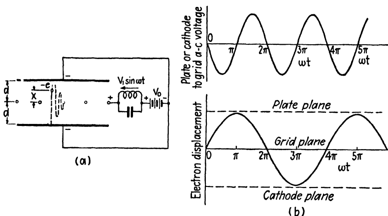
FIG. 1.—Positive-grid oscillator.
