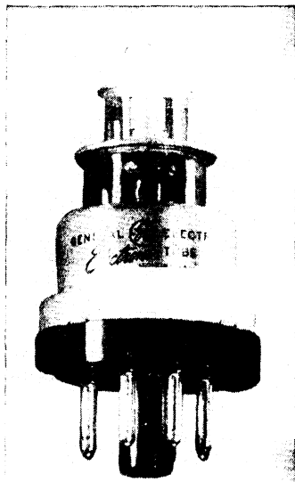
FIG. 2.—G.E. 2C40 lighthouse tube. (Courtesy of the General Electric Company.)
