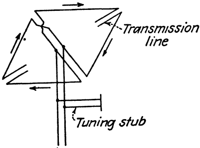
FIG. 17.—Alford loop.
