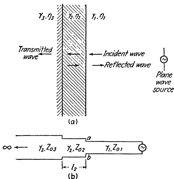
FIG. 4.—Multiple reflection and the transmission-line analogy.
