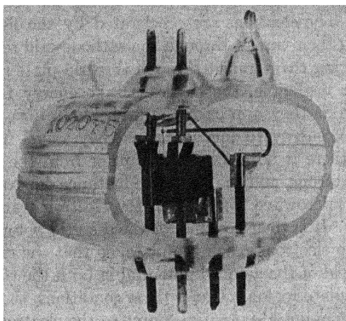
FIG. 1.—W.E. 368A triode. ( Courtesy of the Western Electric Company. )
