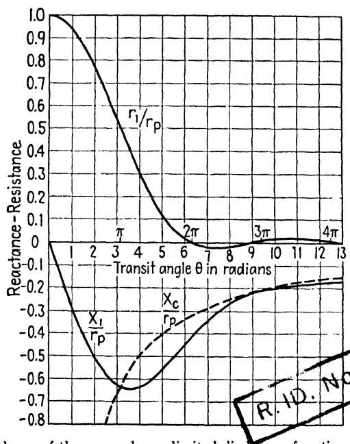
FIG. 8.—Impedance of the space-charge-limited diode as a function of transit angle.
