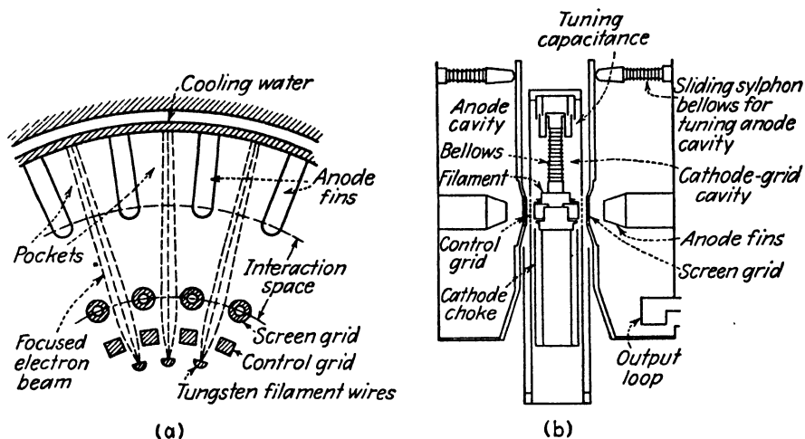
FIG. 26.—Sectional view of the resnatron.
