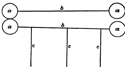
FIG. 48.—Method of cutting a channel in which standards are placed for transverse cuts. a , core drill holes; b , wire saw cuts to make channel; c , subsequent transverse wire saw cuts.
