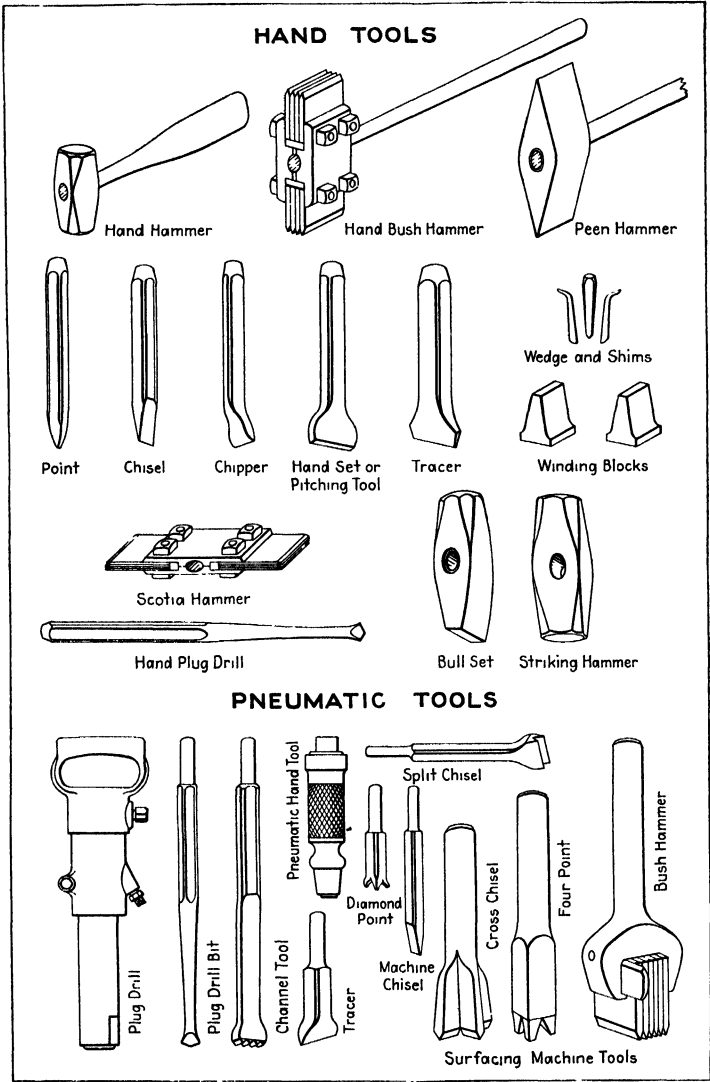
FIG. 28.—Granite cutting tools. (Courtesy of Federal Board for Vocational Education.)
