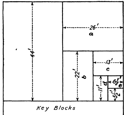
FIG. 17.—Method of subdividing blocks in an Ohio sandstone quarry. Breaks are made in the order of lettering, a , b , c , d , e .
