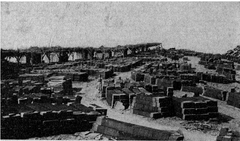
FIG. 52.—Typical roofing-slate piling yard with splitting shanties in background.
