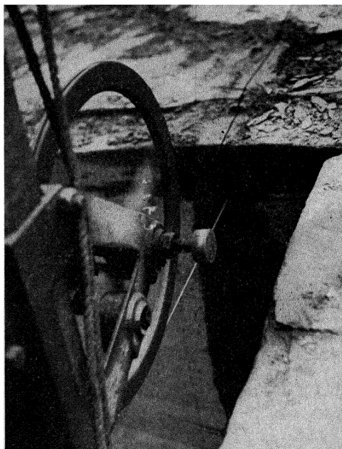
FIG. 46.—Wire saw at the point where it leaves the cut.
