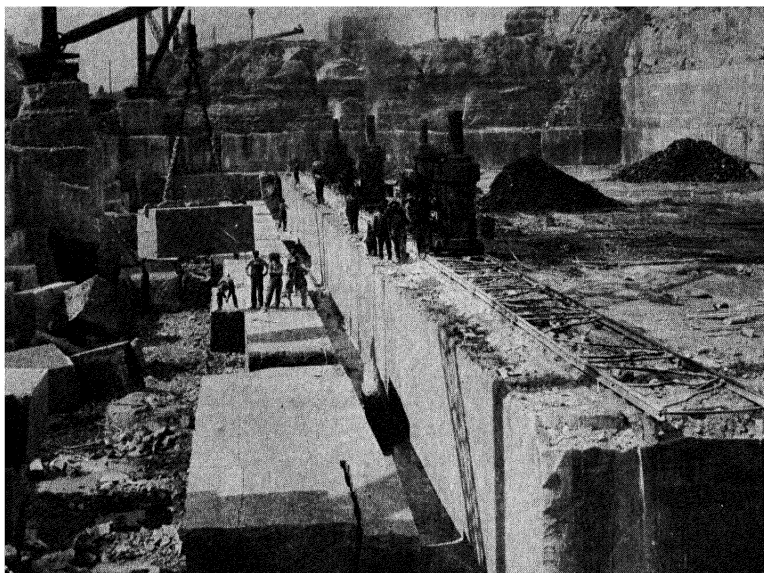
FIG. 10.—Method of subdividing and hoisting limestone blocks. ( Courtesy of Indiana Limestone Company. )
