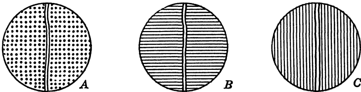
FIG. 67. Appearance of the markings of Pleurosigma angulatum with axial (A) and decentered illumination from two azimuths at 90° to each other. B results from oblique rays from the top or bottom; C is produced by rays coming from either side.
