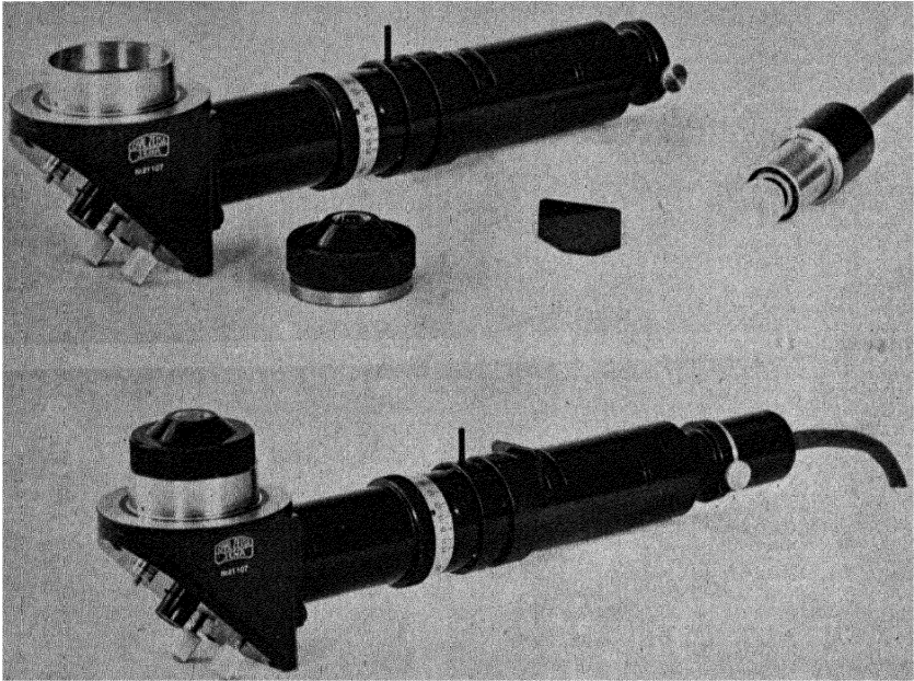
FIG. 54. ZEISS PANCRATIC CONDENSER
