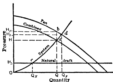
Fig 48. Natural Draft acting against Fan (9)
