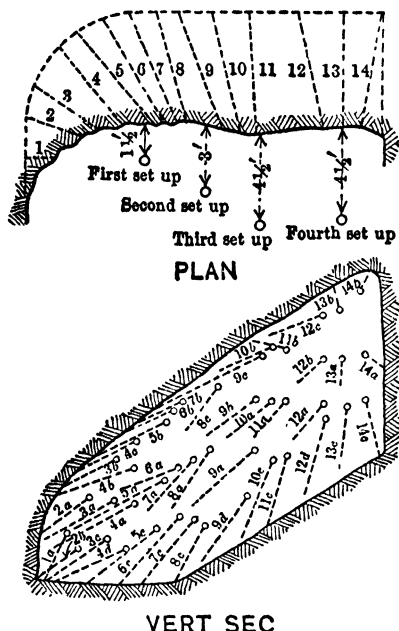
Fig 249. Drift-stope
