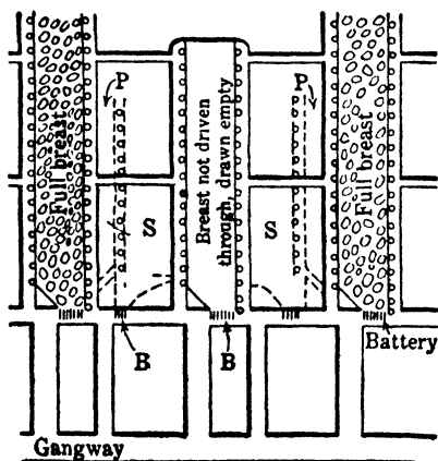
Fig 751. Robbing by Pillar-skipping Method (609)
