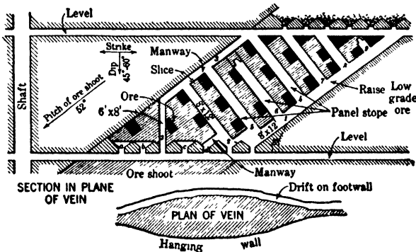
Fig 248. Panel System of the Herman Mine
