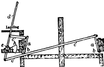
Fig 119. Chairs for Surface Landing
