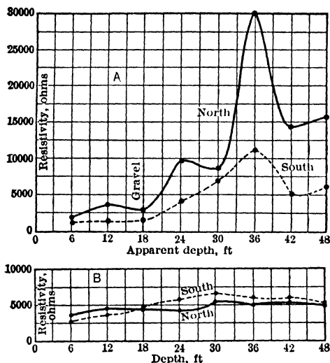
Fig 29. Typical Resistivity Curves in Humboldt Basin, Nev (10)
