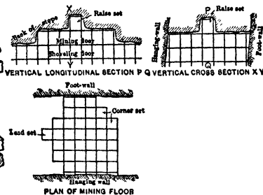
Fig 286. Diag of Square-set System
