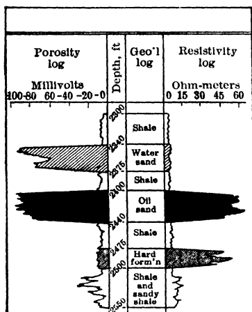
Fig 44. Typical Interpretation of Theoretical Porosity and Resistivity Measurements in Same Hole (18)
