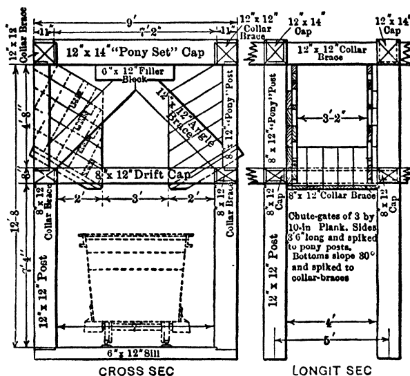
Fig 572. Ray Motor-haulage System, Drift Sets, Pony Sets, and Chute-gates
