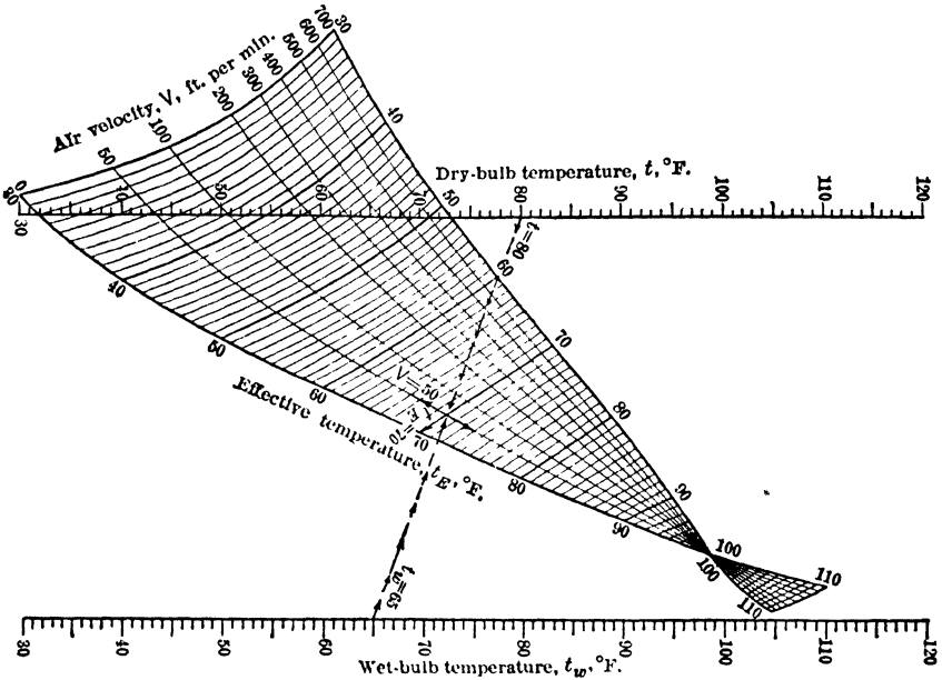
Fig 59. Effective-temp Chart for Men at Rest and Stripped to the Waist (9)
