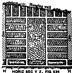
Fig 536. Extraction Drifts
