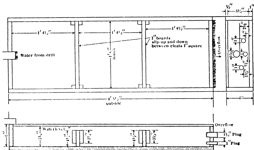
Fig 55 Wooden Sludge Box, Cleveland Cliffs Iron Co
