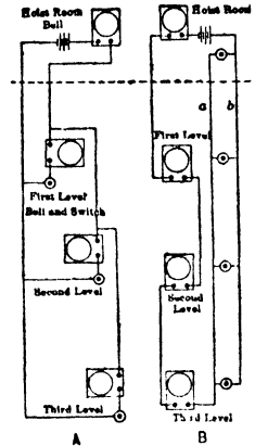
Fig 94. Low-voltage Electrical Signal Layouts
