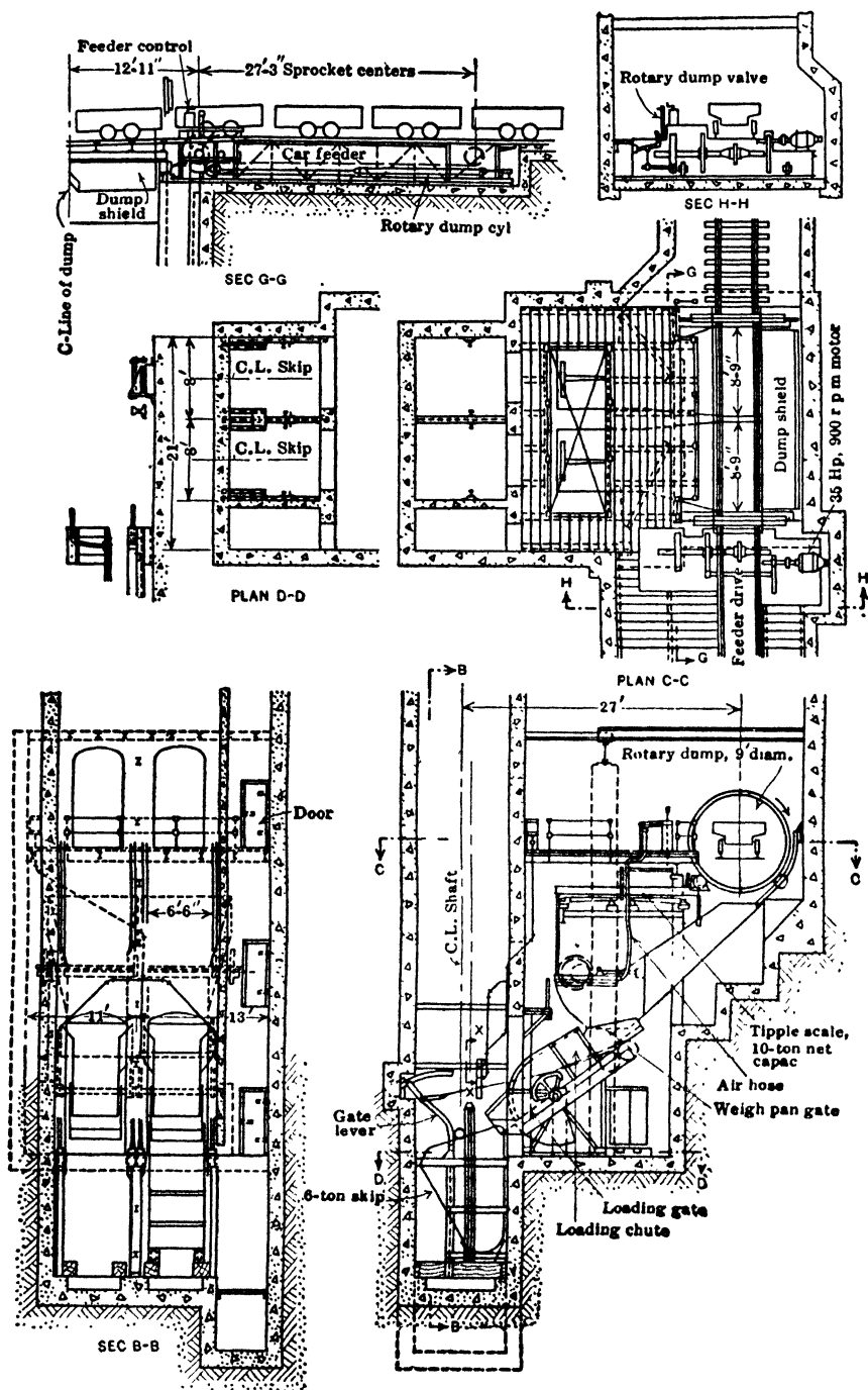
Fig 149. Shaft Bottom, Thermal Mine No 4, Ill. (Coal Age)
