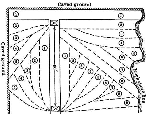
Fig 471. Radial Slicing, Mesabi Range, showing Variations in Plan
