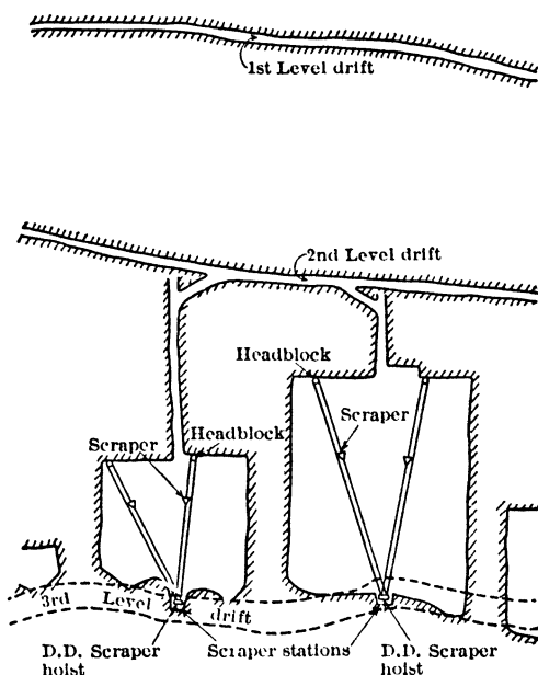
Fig 193. Breast Stopping in Flat-lying Section of Orebody, Sherritt Gordon Mine, Manitoba
