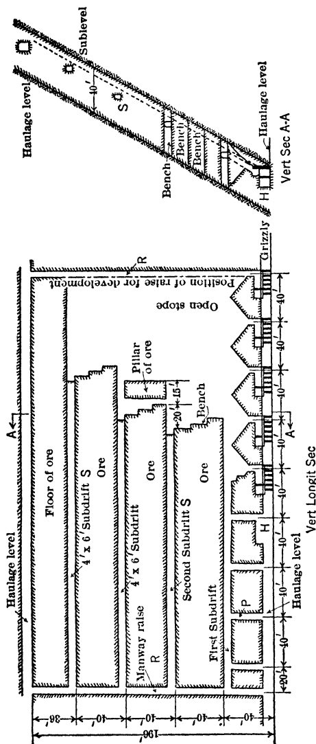
Fig 270. Sub-level Stopping in Narrower Orebodies, Ducktown, Tenn (180)
