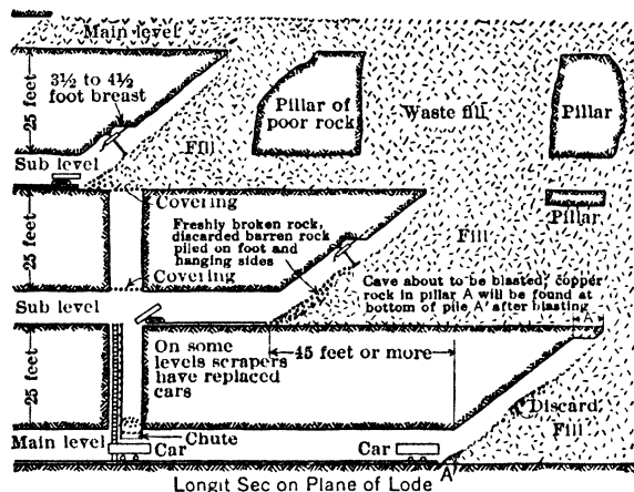
Fig 406 Sub-level, Inclined Cut-and-fill Method, Champion Mine, Painesdale, Mich (488)
