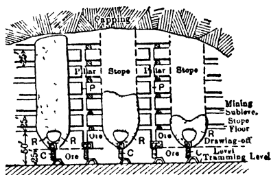
CROSS-SEC THRO STOPE AND PILLARS Fig 579 Miami Method
