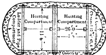
Fig 3. Modified Elliptical Shaft
