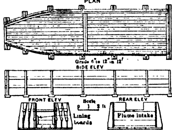
Fig 828. Mud Box or Dump Box (after Purington)
