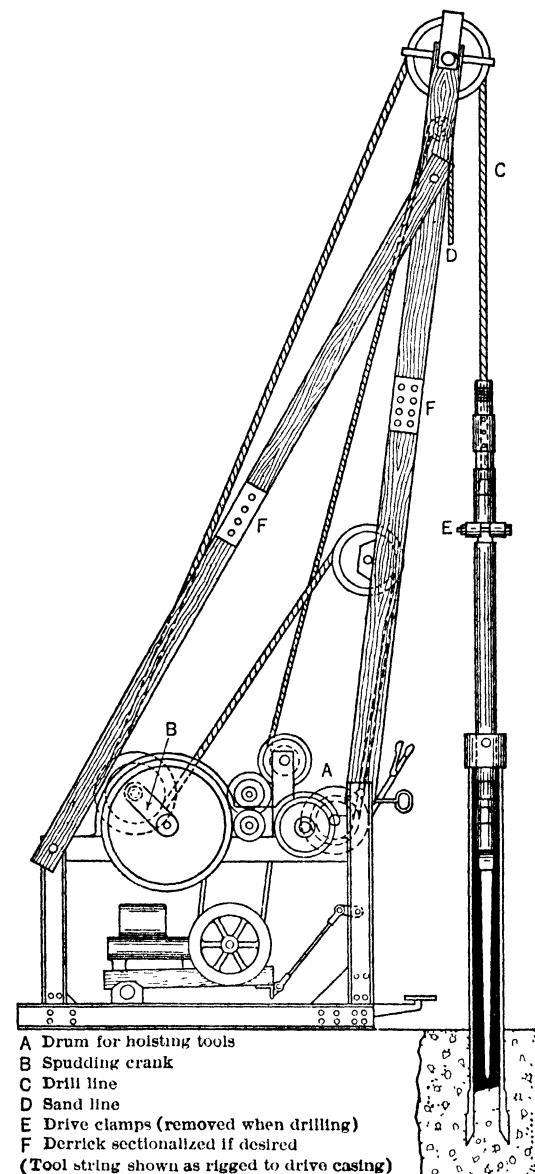
Fig 40. Light Placer Drill (C. K. Hillman Co)
