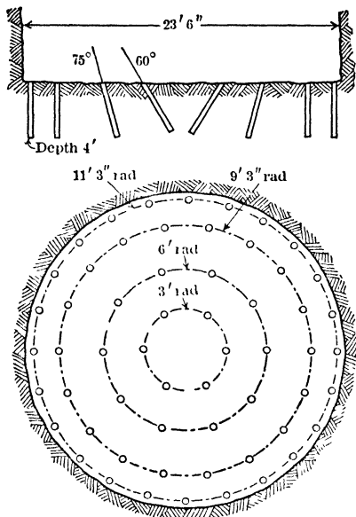
Fig 7. Pyramid Cut for Circular Shaft (Randfontein)
