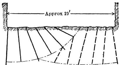
Fig 10. Bench Cut at McPherson Shaft
