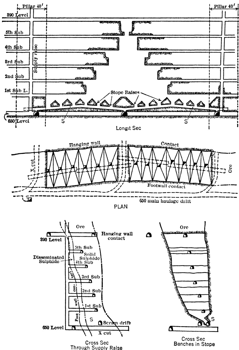
Fig 278. Typical Sub-level Stope, Flin Flon Mine, Manitoba
