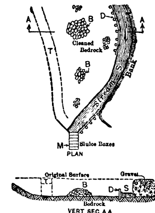
Fig 807 Ground-sluicing (diagrammatic)
