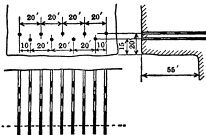
Fig 22. Staggered Holes to Increase Shattering Effect
