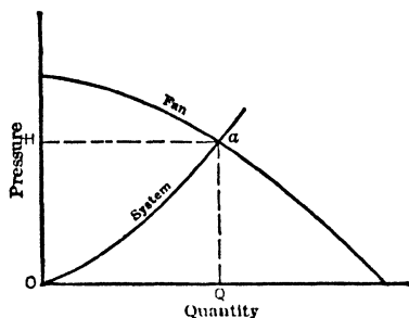
Fig 46. Fan as only Pressure Source (9)
