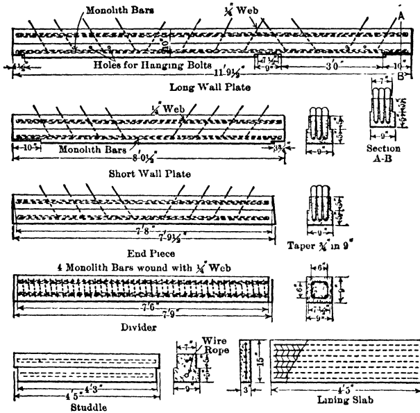
Fig 26. Reinforced-concrete Shaft Sets (34)
