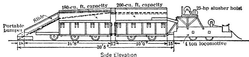
Fig 12. Scraper-loading Unit, Montreal Mine, Wis
