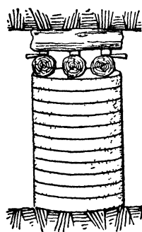
Fig 198. Concrete "Pancake" Column
