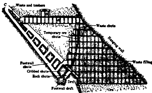
Fig 303. Vert-face Stope, Cross-sec
