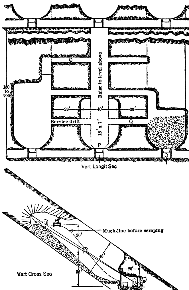
Fig 447. "Semi-shrinkage" Stoping, Walker Mine (ideal sections)
