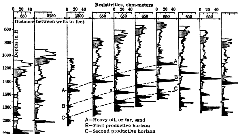
Fig 47. Example of Oil Structure disclosed by Resistivity Logs (17)
