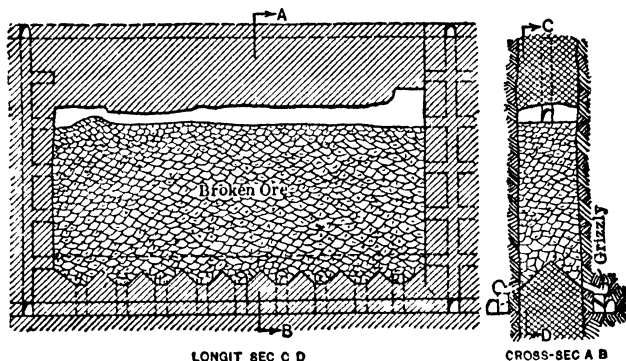
Fig 442. Shrinkage Stope, Coronado Mine, Metcalf, Ariz
