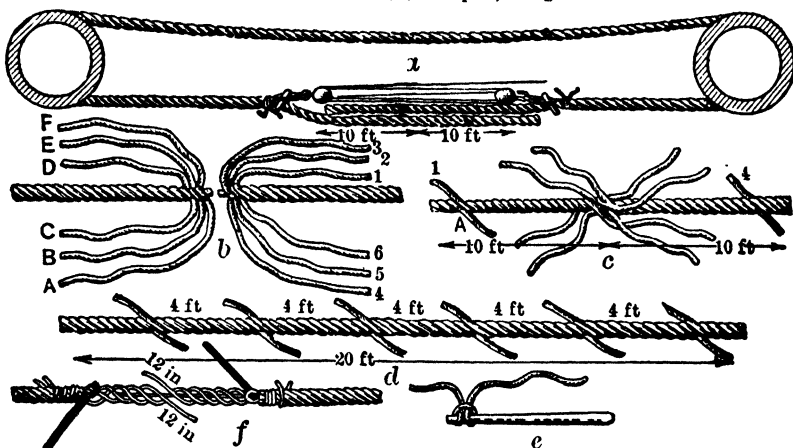
Fig 36. Splicing Wire Rope
