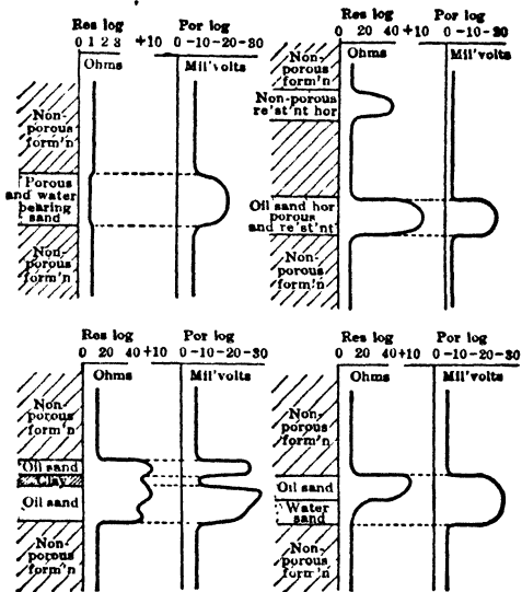
Fig. 43 Interpretation of Resistivity Measurements in Boreholes (16)
