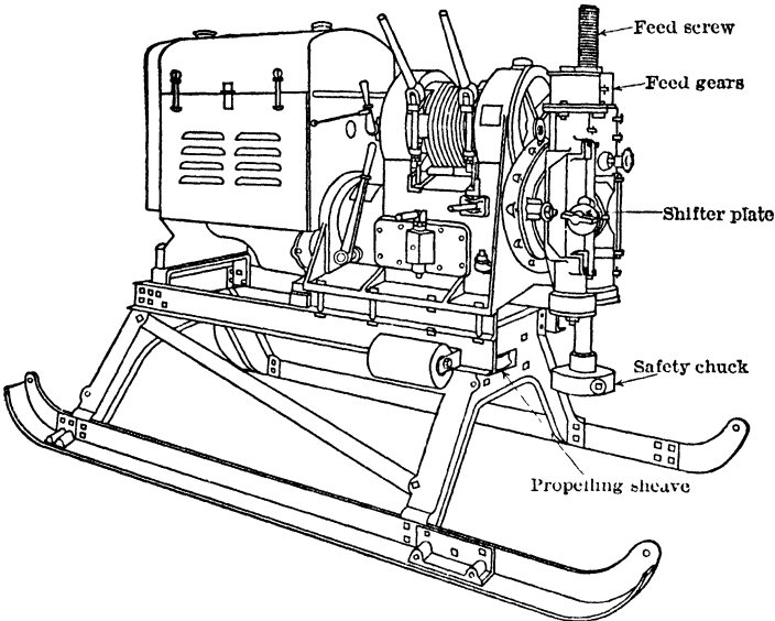
Fig 45. Gasolene-driven, Swivel-head, Screw-feed Diamond Drill (E. J. Longyear Co)
