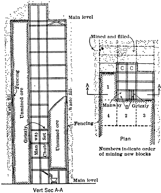
Fig 361. Mitchell Slicing applied to Mining of Vert Pillars, United Verde Ext Mine, Jerome, Ariz
