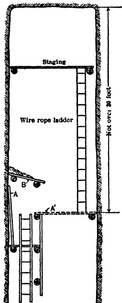
Fig 166. Top of 4 by 8-ft Raise, Champion Mine, Painesdale, Mich. (Planks A are laid across at A' when men ascend to start a new round. Sollar B is to protect main ladder-way)
