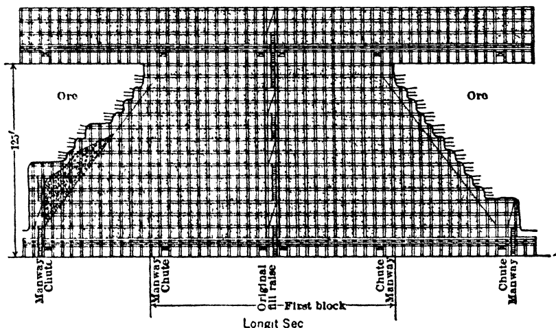
Fig 300 Square-set Rill Stope, Lake Shore Mine, Kirkland Lake, Ont
