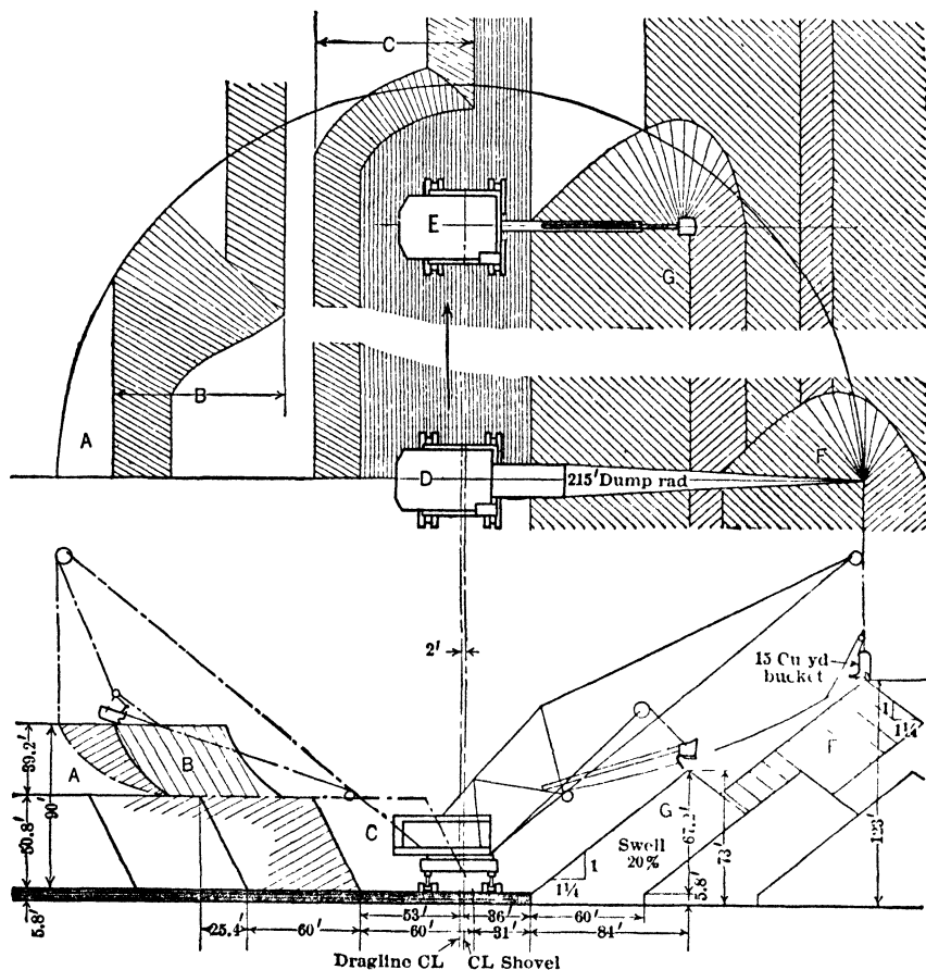
Fig 692. Stripping Coal Seam with Power Shovel and Dragline
