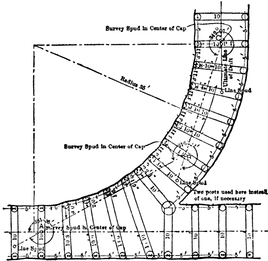
Fig 28. Curve Layout
