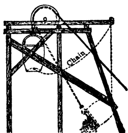
Fig 105. Bucket Dump
