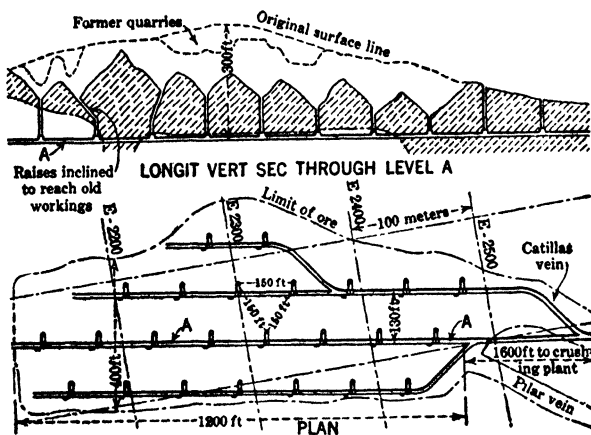
Fig 687. Glory-hole Work, Fresnillo, Mex (640)
