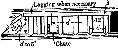
Fig 769. Face Timbering, Miller Mine
