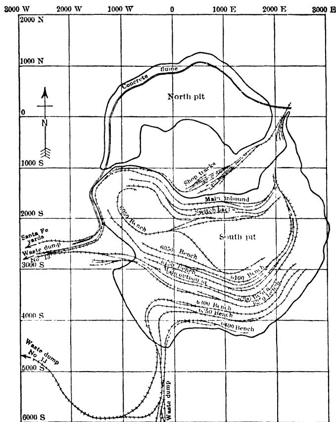
Fig 671. Pit Outline and Track Layout, Chino Mine, Santa Rita, N M, as of Jan, 1939
