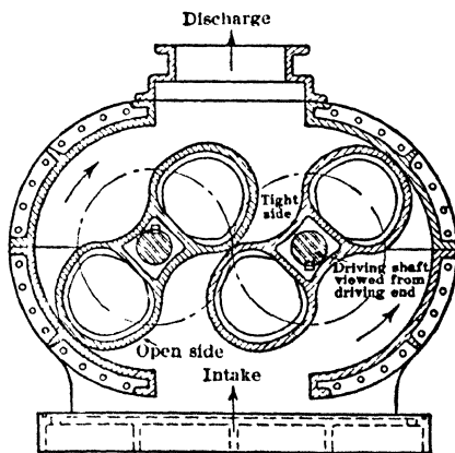
Fig 42 Root Blower (9)
