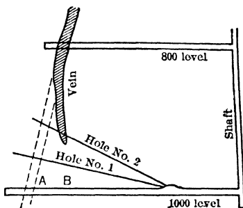
Fig 47. Locating Downward Extension of Vein
