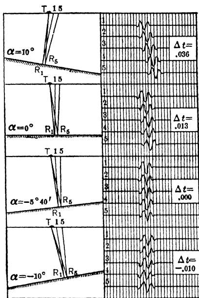
Fig 54. Theoretical Seismograms for varying Dips. Aver veloc, 6 000 ft per sec. Depth, 7 000 ft. Space between geophones 1 and 5, 1 000 ft (21)
