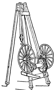
Fig 1. Derrick for Wash Boring
