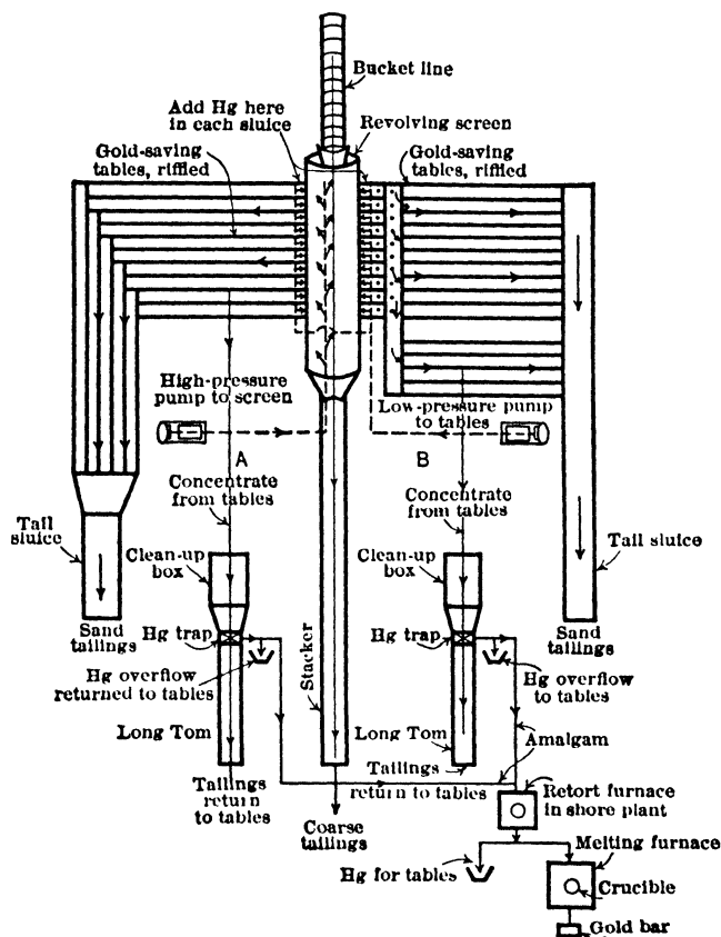
Fig 850. Flowsheets of Gold Dredge equipped with Tables. A—Conventional type. B—Improved Arrangement
