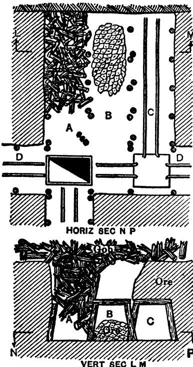
Fig 511. Slicing and Stripping Details
