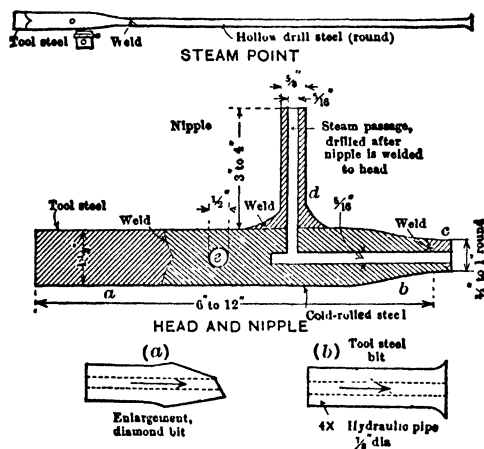
Fig 870. Steam Points (after Ellis)
