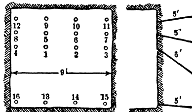
Fig 121. Bottom-draw Cut in Quartzite, Sullivan Mine, Kimberley, B C
