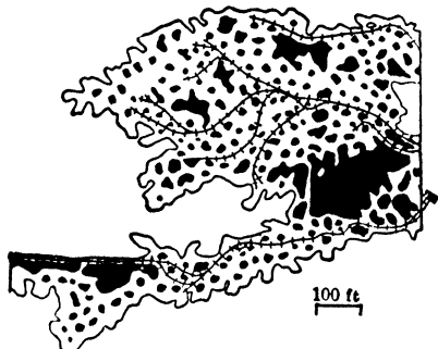
Fig 177 Plan of Part of a Mine in S E Missouri, worked by Breast Stopping
