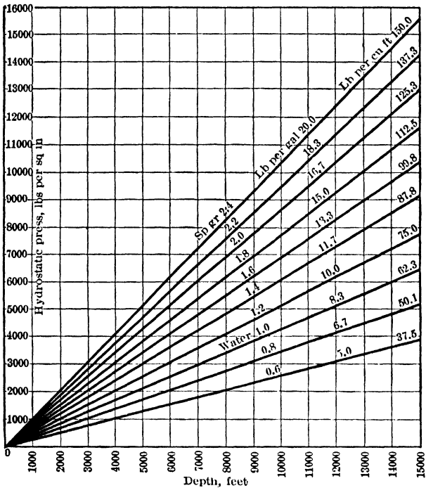
Fig 22. Pressures of Mud Fluids
