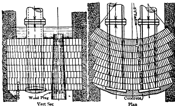
Fig 3. Details of Underground Dam, Hazleton Shaft Colliery
