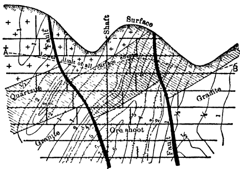
Fig 34 Assay Sec on Plane of Vein, Showing Lines of Equal Widths of Vein Filling. High Values (Shaded Areas) Correspond to Relatively Great Widths, and Show that the Two are in Some Way Related
