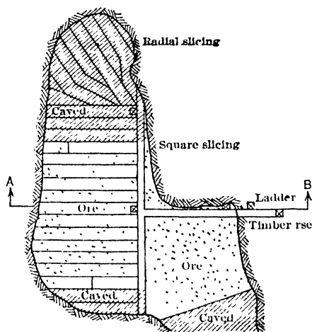
Plan of 7th Sub Level
