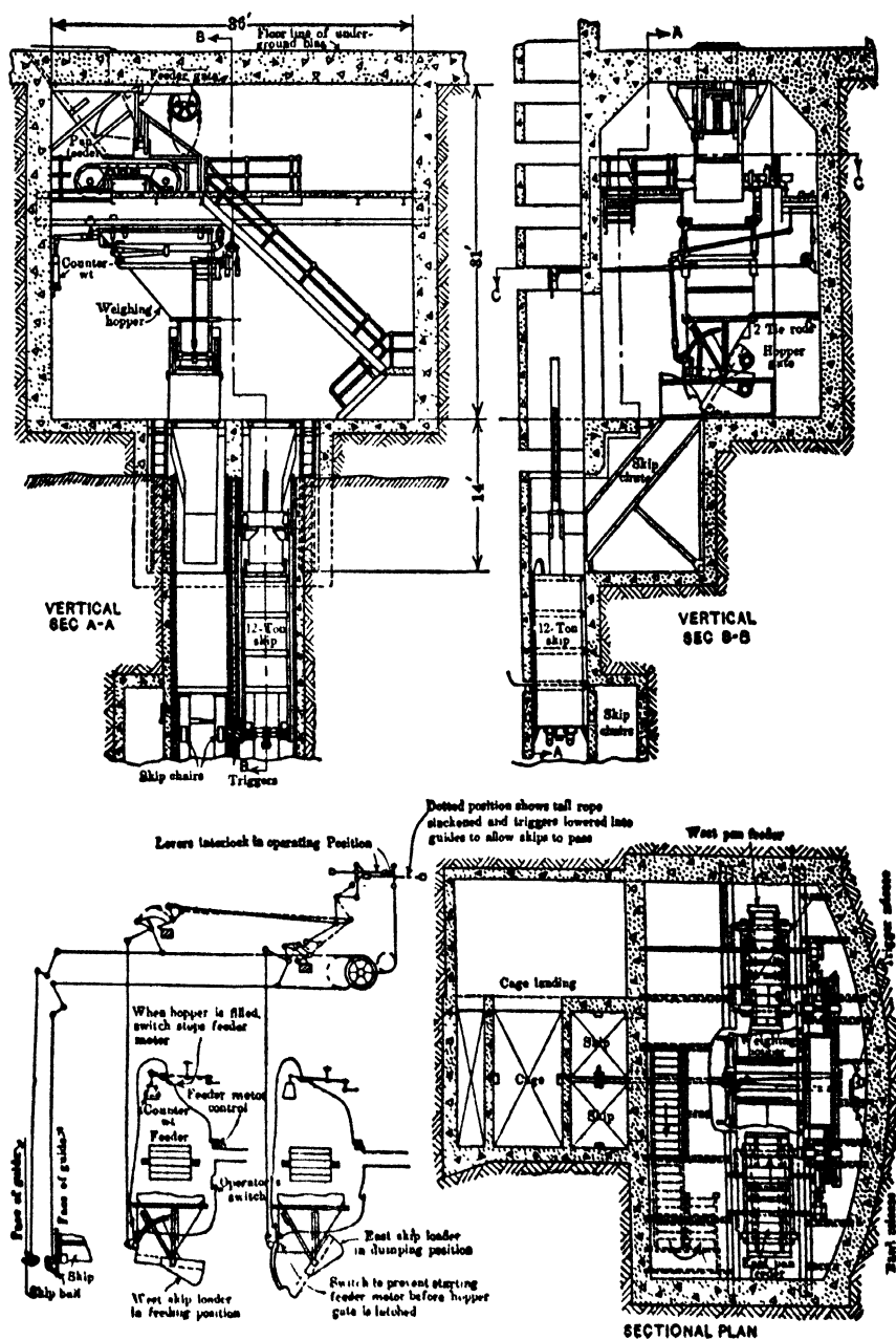
Fig 150. Skip Loading Arrangement, Porphyry Shaft, Inspiration Mine, Ariz (E & M J)
