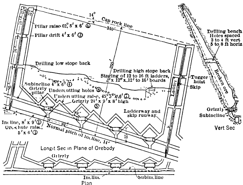
Fig 445 Shrinkage Stope Development and Mining, Mt Hope Mine, Mt Hope, N J (529) Numbers in circles indicate successive development steps
