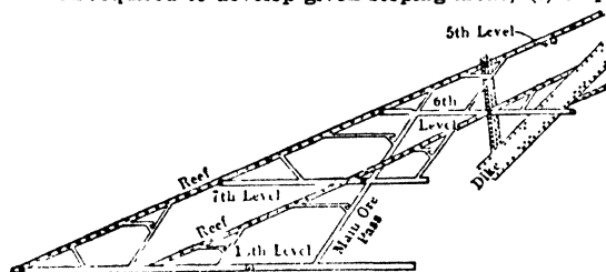
Fig 646. Development at Crown Mines, Transvaal ( E & M J )
