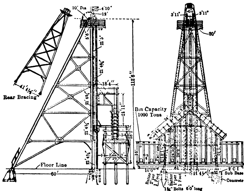
Fig 73 Steel Headframe, Orig Mine, Butte, Mont. ( E & M Jour )
