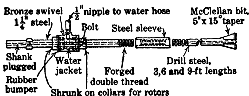
Fig 90. Swivel and Steel Assembly for Deep-hole Hammer Drilling
