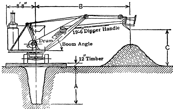
Fig 6. Trenching with Power Shovel
