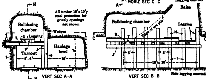
Fig 636. Chinaman Chute with Bulldozing Chamber, Tenn Copper Co
