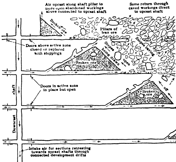
Fig 12. Method of Ventilating Retreating Shrinkage Stopes (9)
