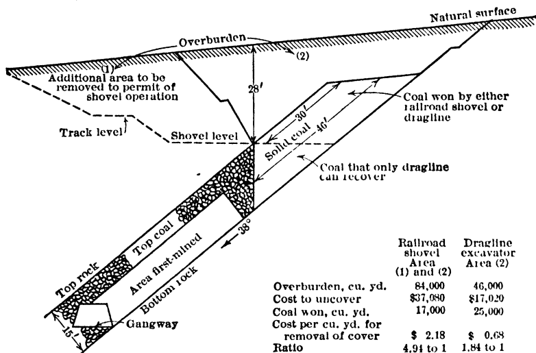
Fig 694. Railroad Shovel vs Dragline Excavator, both removing 28 ft of Cover
