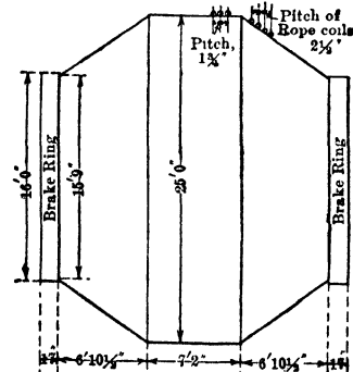
Fig 12. Cylindro-conical Drum, Tamarack No 5 Shaft
