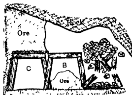
Fig 518 Newport Mine, Slicing and Stripping under Capping
