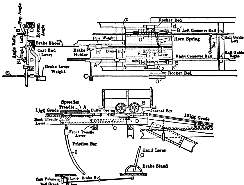
Fig 52d. Phillips Cross-over Dump
