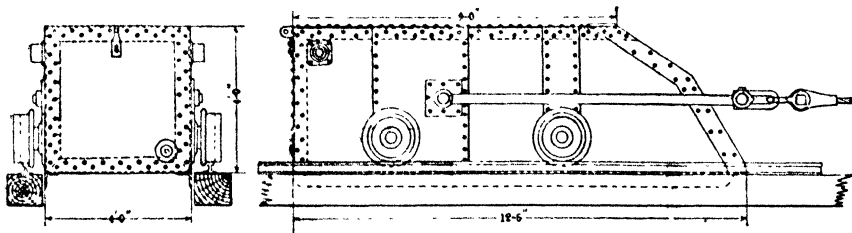
Fig 126. 8-ton Skip, Hancock No 2 Shaft, Quincy Copper Mine, Mich; Weight, 4\frac{3}{4} Tons
