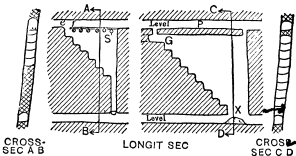
Fig 209. Simple Underhand Stopes
