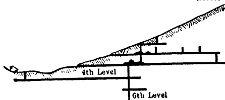
Fig 105. Section in Plane of Vein
