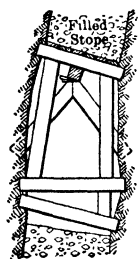
Fig 377. Support for Stull and Post Sets while mining Level-pillars, Nevada Wonder Mine (Fig 379)
