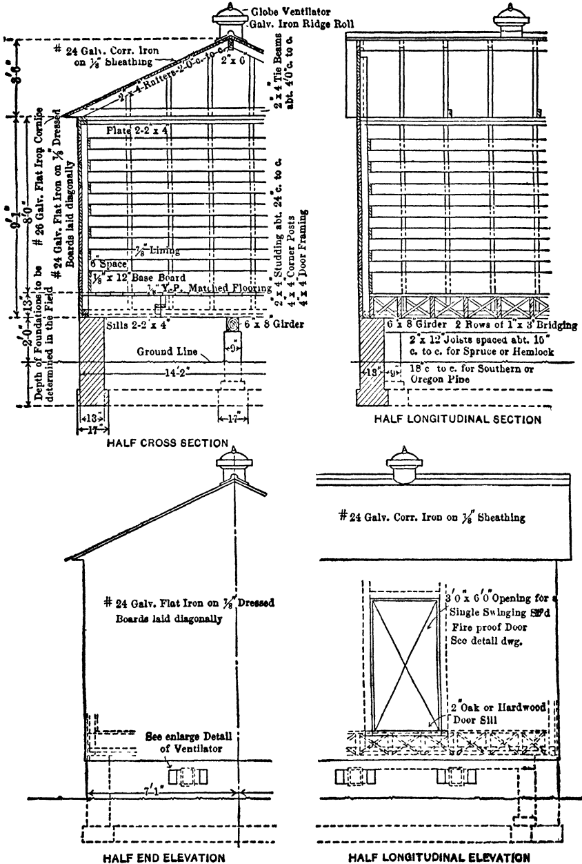
Fig 6. Black Powder Magazine
