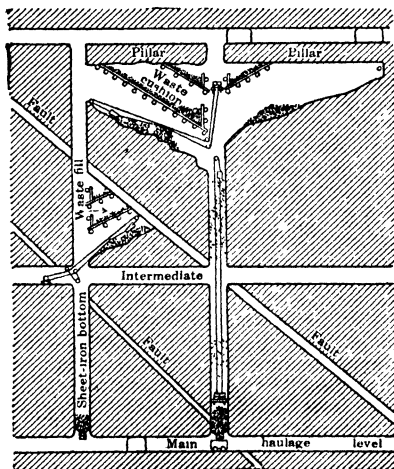
Fig 213. Underhand Stoping, Golden Messenger Mine, York, Mont. (Longit sec in plane of vein)
