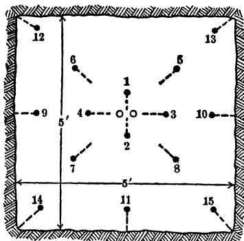
Fig 155. Pyramid Cut with Blank Center, Burra Burra Mine, Ducktown, Tenn. Holes 6.5 ft deep
