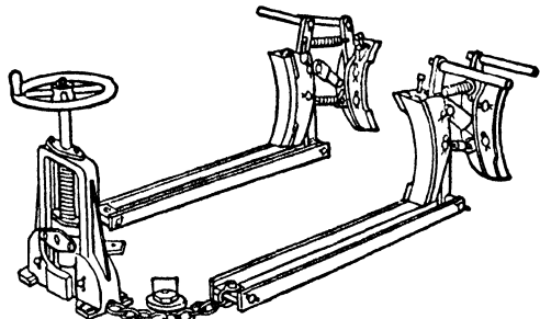
Fig 20 Vertical Screw Brake
