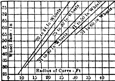
Fig 30 Minimum-radius Curve
