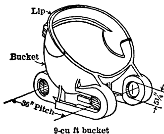
Fig 849. Manganese-steel Bucket with Rivetless Lip
