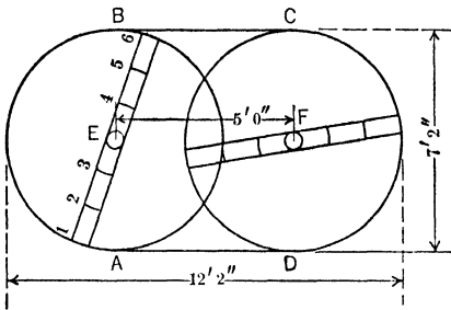
Fig 11 Diagram of McKinlay Entry Borer
