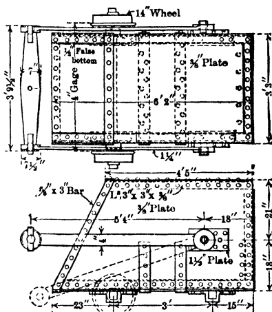
Fig 124. 3 5-ton Skip, Mineville, N Y (E & M J)
