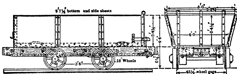
Fig 16. Steel and Wood Colliery Car (Shamokin, Pa)
