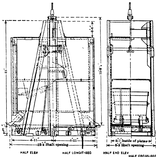
Fig 122. Man and Material Cage, Inspiration Mine, Aris (E & M J)
