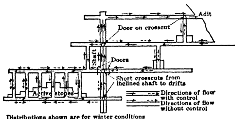
Fig 34. Controlled Natural-draft Distribution (9)
