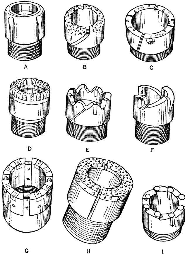
Fig 44. Diamond-drill Bits
