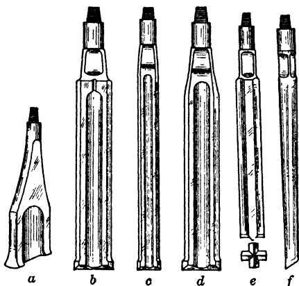
Fig 15. Churn Drill Bits (Star Drilling Mach Co)
