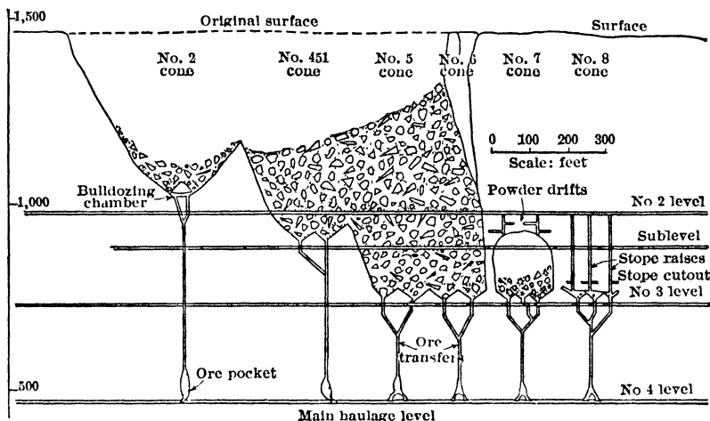
Fig 462. Development, Alaska Juneau Mine
