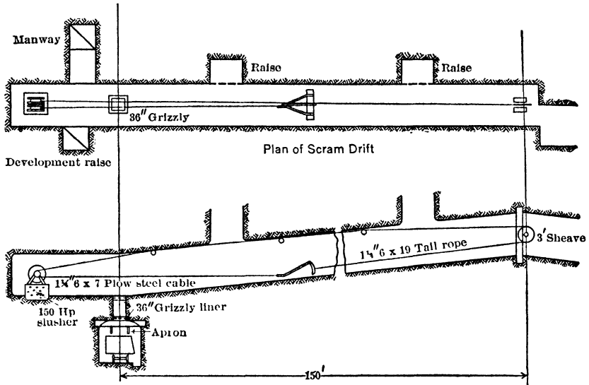
Fig 279. Layout of Scram Drift, Flin Flon Mine, Manitoba
