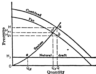
Fig 47. Natural Draft acting with Fan (9)
