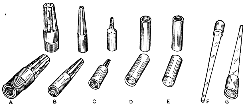
Fig 48. Diamond-drill Fishing Tools (Sullivan Machy Co)
