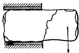
Fig 792. Rock Layer acting as a Fixed Beam, showing how doming effect may start in horiz strata at edge of excavated ground (465)
