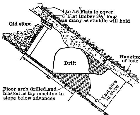
Fig 242 Section showing Removal of Floor Arch, Conglomerate Lode, Calumet, Mich. (489)
