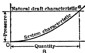
Fig 28 Pressure-quantity Characteristic for Natural-draft Flow (9)
