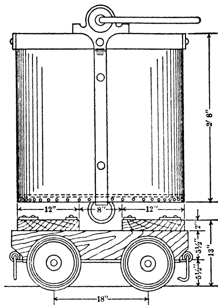
Fig 103 Ore Bucket on Truck Hartley Mine, Interstate Zinc & Lead Co, Baxter Springs, Kan, (63, 37)
