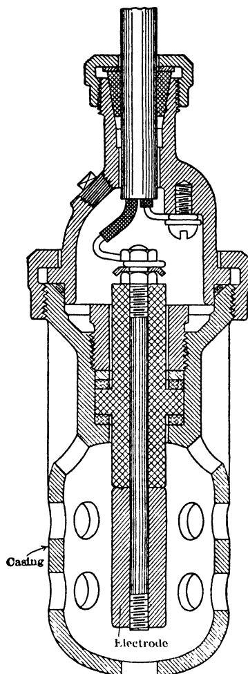
Fig 19. Electrode for Starting Hazleton Pump
