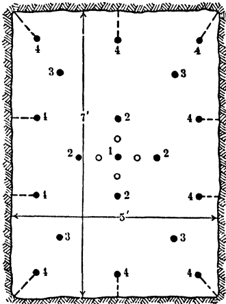
Fig 153. Burned Cut, Homestake Mine, Lead, S D. Holes 7 ft-4 in deep
