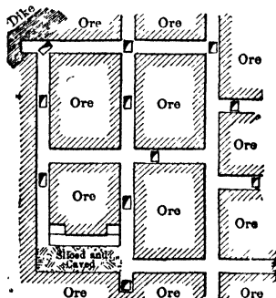
Fig 517. Newport Mine, Plan of Part of a Sub-level
