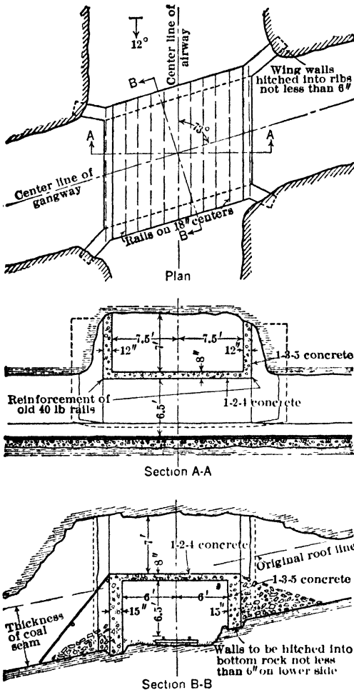
Fig 6. Overcast of Reinforced Concrete (27)
