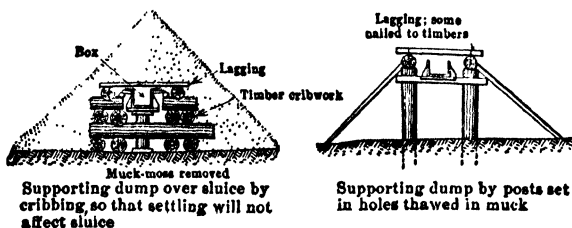
Fig 862. Methods of Protecting Sluice under Winter Dumps (after Ellis)
