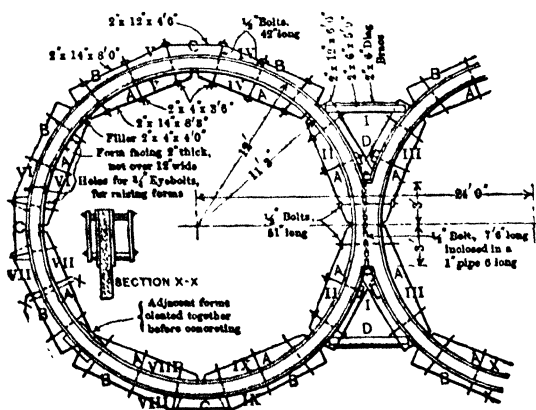
Fig 158. Concrete Forms for Bins in Fig 157
