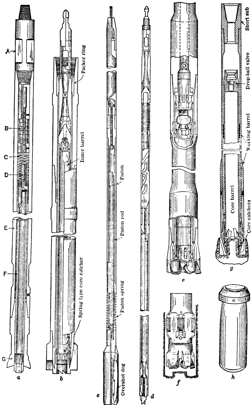
Fig 33. Core Drills for Oil Wells
