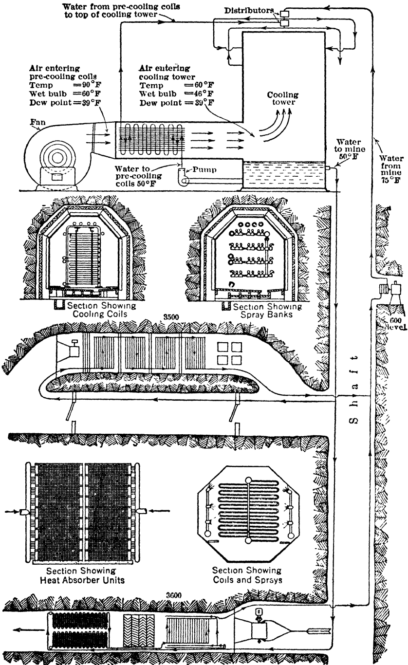
Fig 63. Evaporative Cooling System devised for Butte Mines (98)
