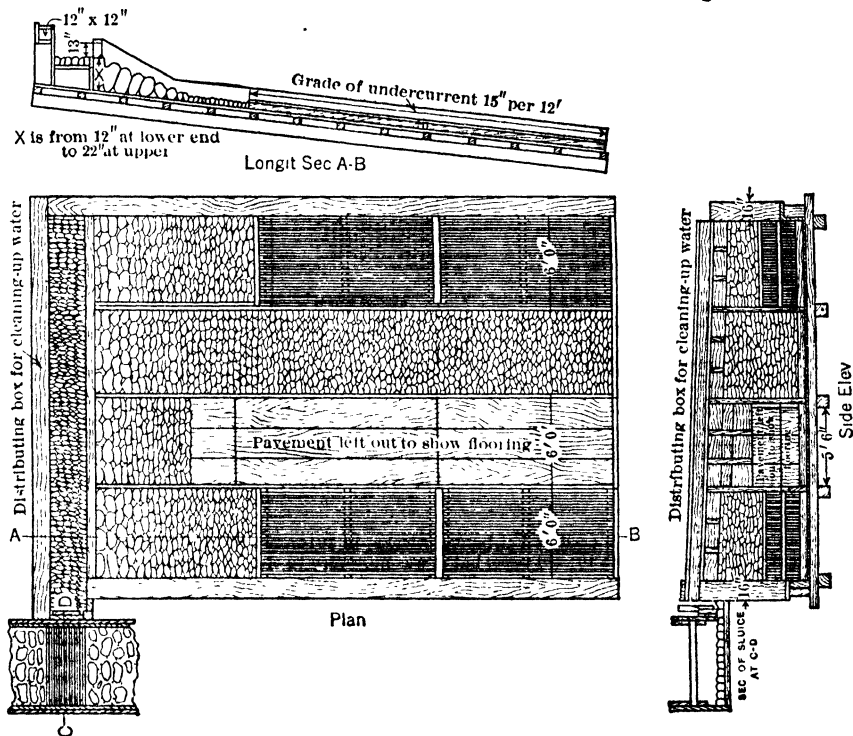
Fig 840. North Bloomfield Undercurrent (after Bowie)
