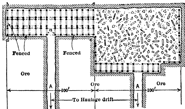
Fig 473. Parallel Slicing, Hibbing-Chisholm Distr, Minn. If b-c is a shore line, the 2 caps a and all posts except those along b-d and d-e are blasted; if b-c is a face of minable ore, this side also is wire-fenced and its posts are not blasted
