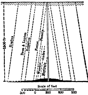
Fig 797. Sizes of Shaft Pillars, according to Different Formulas (Knox)
