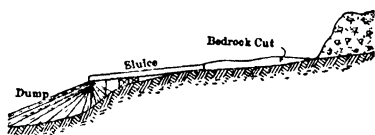
Fig 814. Simple Layout for Hydraulicking (after Young)
