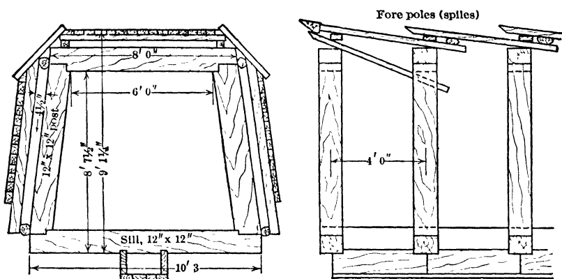
Fig 25 Forepoling with Regular and Bridging Sets
