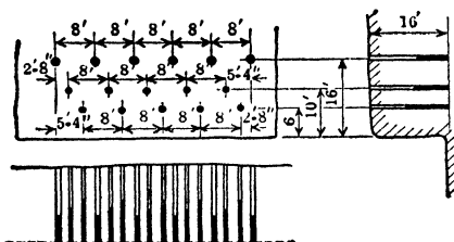
Fig 24. Arrangement of Holes to Reduce Secondary Blasting
