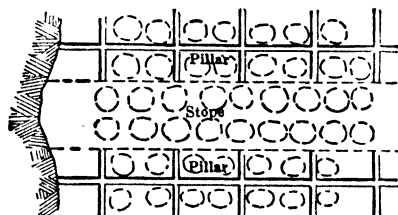
Fig 583. Miami Method, Plan of Stope Floor
