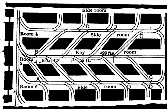
Fig 730. Room System, Peabody Coal Co Mines No 8, Ill (491)
