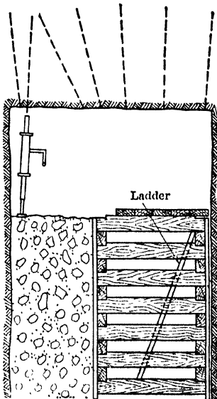
Fig 162. Use of Cribbing in Two-compt Raise
