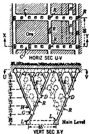
Fig 525. Sub-level Caving. Branched Raises (diagrammatic)
