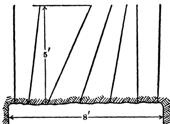
Fig 155. Pyramid Cut with Blank Center, Burra Burra Mine, Ducktown, Tenn. Holes 6.5 ft deep
