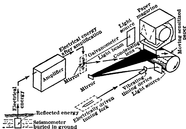
Fig 48. Diagram showing Reflection Seismograph System (21)
