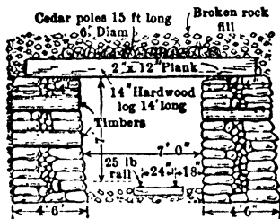
Fig 396. Dry-wall Gangway, Baltic Method
