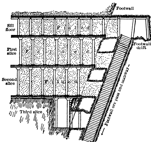
Fig 410 Sec through Ore Pass, Tiro General Mine, Charcoas, Mex (241)
