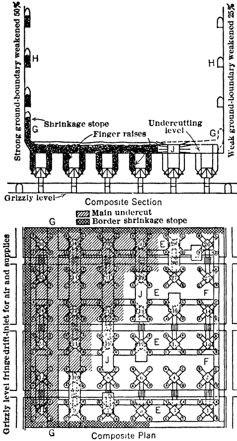
Fig 548. Undercutting and Grizzly Levels, Miami Copper Co
