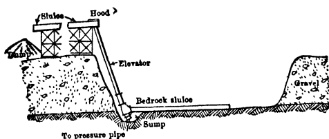
Fig 843. Elevator Pit (diagrammatic vert sec)
