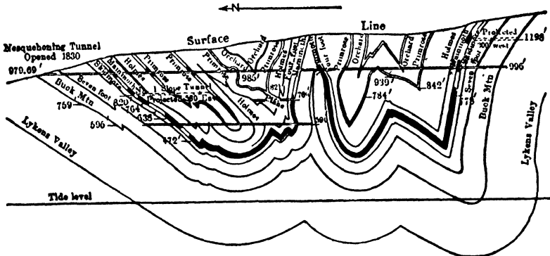
Fig 740. Workings from Nesquehoning Tunnel, Southern Anthracite Field (Whildin)
