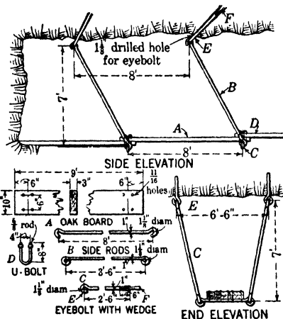
Fig 180. Hanging Scaffold or Staging
