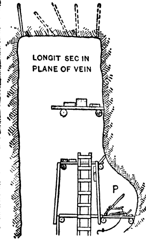
Fig 161. Draw-cut for Small Vert Raise
