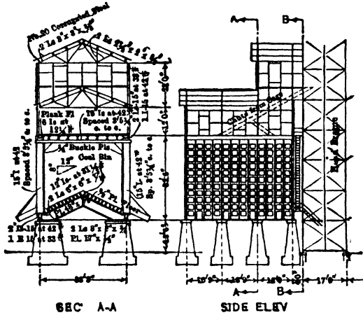
Fig 151. Coal Storage Bin, H. C. Frick C & C Co
