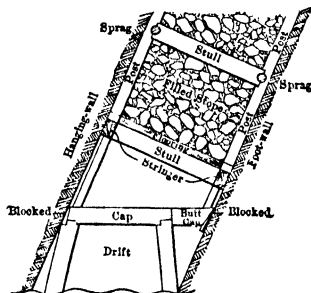
Fig 366. Leaning Stope-set, Cal
