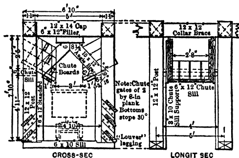
Fig 576. Ray-Hand-tramming System, Drift-sets and Chute-gates
