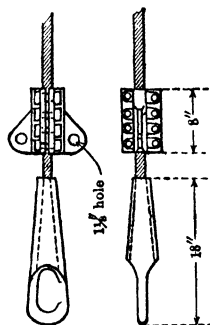
Fig 40 Rope Clamps for Bridle Chains
