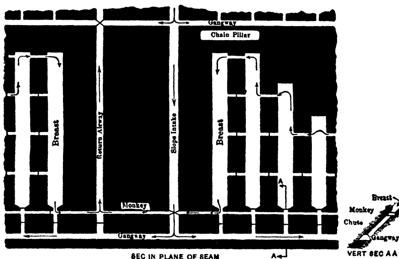
Fig 709. Typical Development of a Pitching Anthracite Seam, Penna
