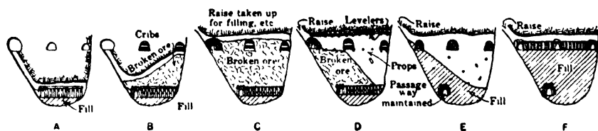
A Bottom filled, sets placed, raise carried up B Stope in progress C Stope finished D Drawing down stope, back timbered E Stope emptied, fill started F Fill finished, with sets ready for another lift.
