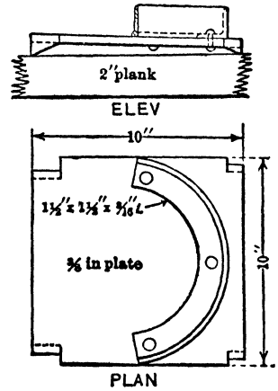
Fig 139. Foot-plate for Slope Drill in Drifting
