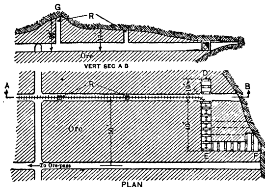
Fig 474. Starting Slices at Edge of Deposit, Mesabi
