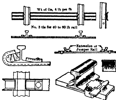
Fig 26. Steel Ties and Rail-fastenings
