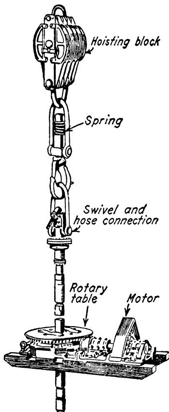
Fig 21. Rotary Drive (Union Tool Co)
