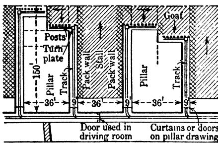
Fig 757. Robbing Pillars, Pillar-and-stall Method, Wales (611)
