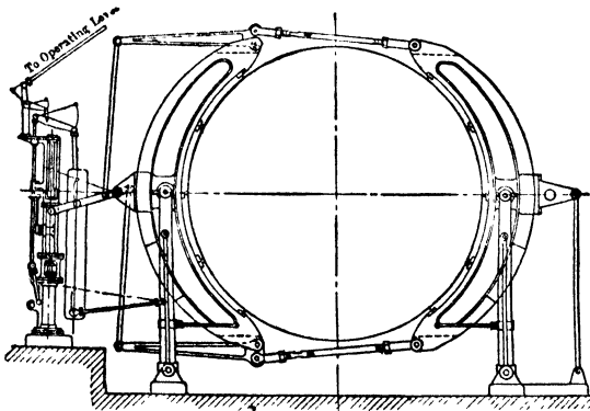
Fig 18. Parallel-motion Post Brake, Operated by Comp-air Cylinder (Nordberg)
