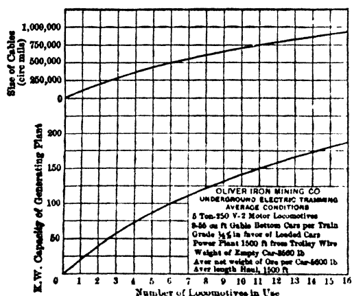
Fig 53. Power and Transmission Line for Trolley Haulage
