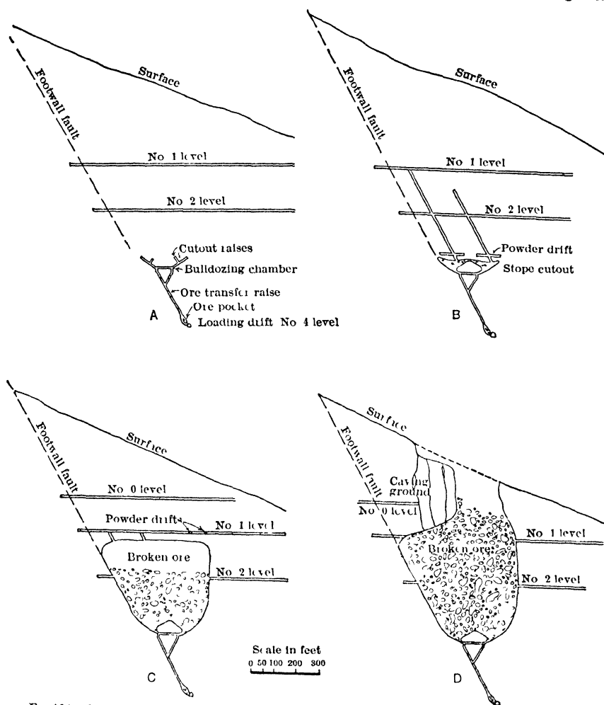
Fig 464 Stages in Development of a Shrinkage Stope, Alaska Juneau Mine, Juneau, Alaska
