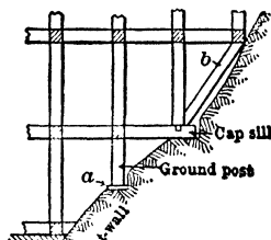
Fig 345. Timbering against Sloping Footwall
