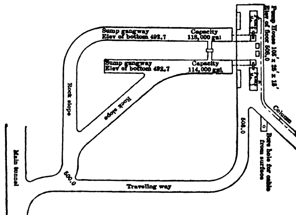
Fig 2. Plan of Sumps and Pump Room, No 6 Mine, Lehigh Nav Coal Co, Lansford, Pa
