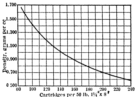
Fig 1 Stick Count of Cartridges vs Density
