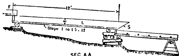
SEC A A
