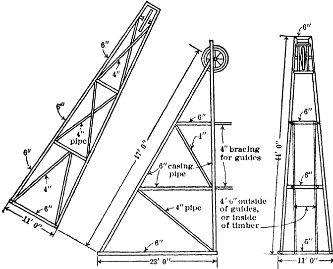
Made entirely from used 6" churn drill casing and second hand 4" pipe. All joints welded. Total length of 6" casing = 325 ft. Total length of 4" pipe = 175 ft. Approx wt = 6 ton
