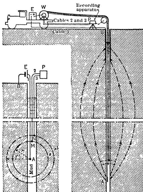
Fig 58. Diagram of Electrical Coring
