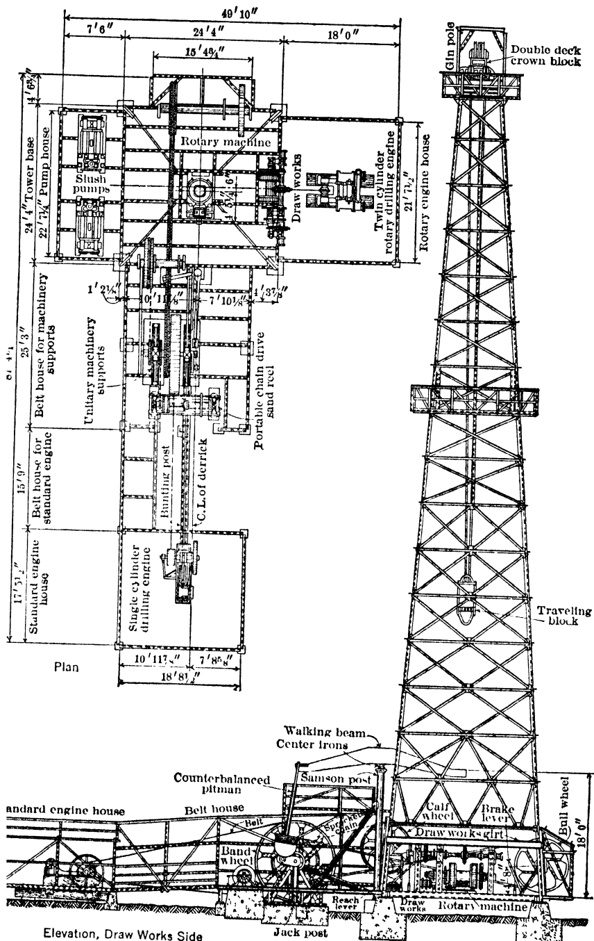
Fig 19. Combination Rig (Cable-tool and Rotary). (Emsco Derrick and Equipment Co)
