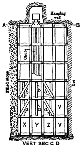
Fig 357. Recovering Timber from Square-set Stope
