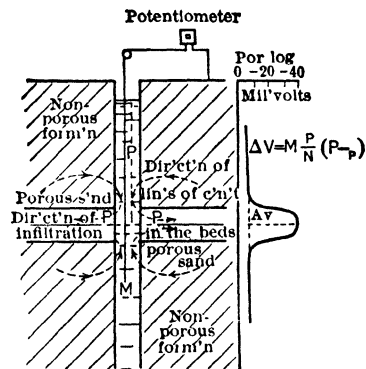
Fig. 41 Recognition of Porous Beds by Resistivity Measurements (16)
