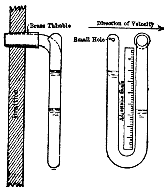
Fig 18. Water Gage
