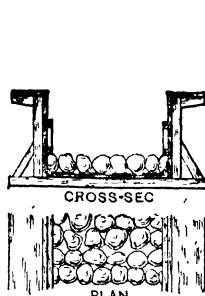
Fig 830. Cobble Riffles
