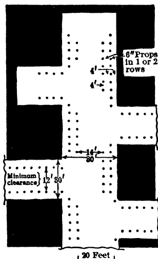
Fig 734. Timbering Diagram, Moffat Mine, Ill (634)
