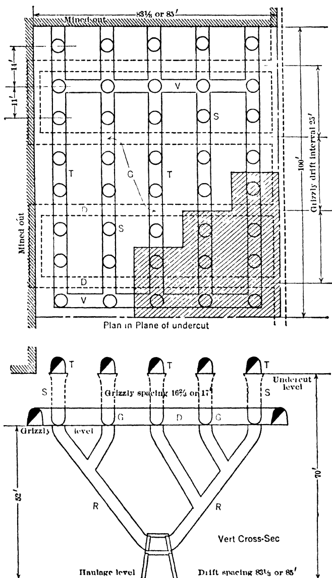
Fig. 549. Block Caving, Inspiration Mine, Ariz. Max haulage-drift spacing for highest ore horizon
