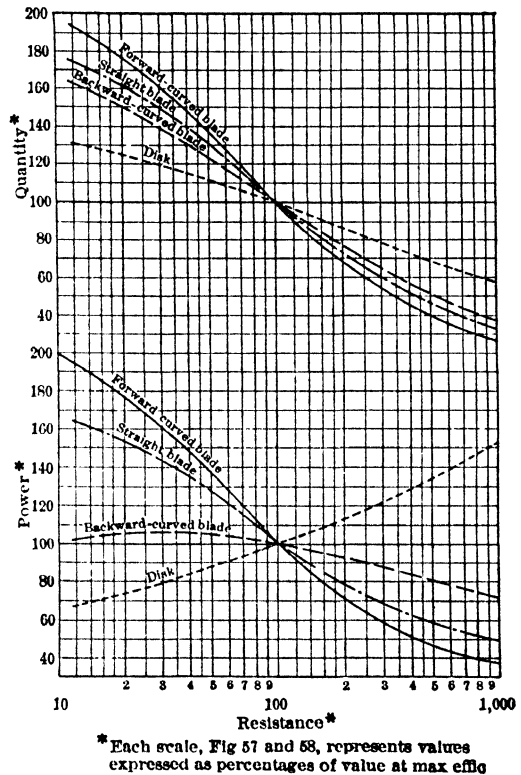
Fig 57. Comparative Quantity and Power Characteristics of Mine Fans (9)
