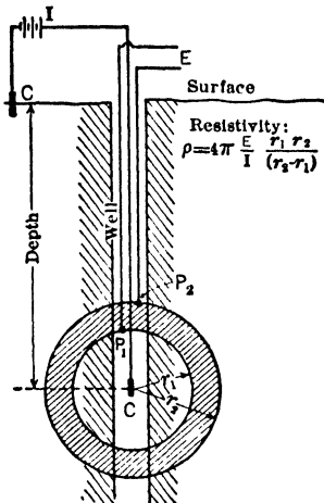
Fig. 40 Resistivity about a Single Electrode Adapted from E. R. Shepard (12)
