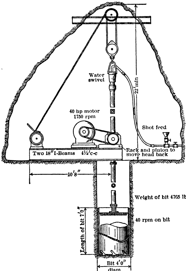
Fig 168. Set-up of Calyx Drill, United Verde Mine, Jerome, Ariz
