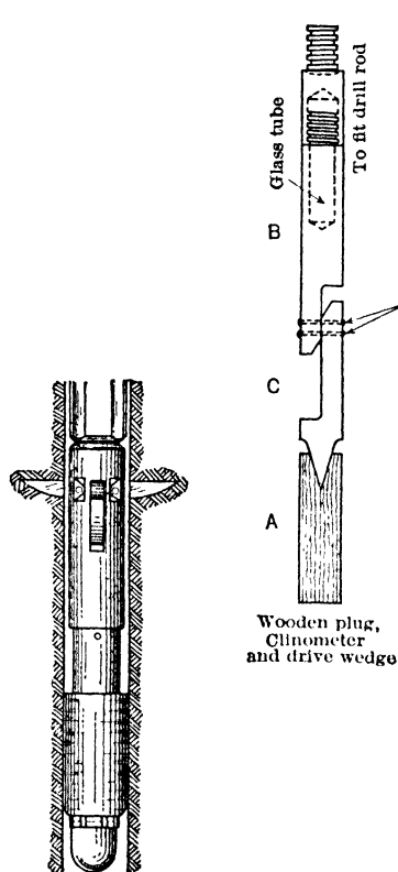
Fig. 37. Eastman Hydraulic Bridger
