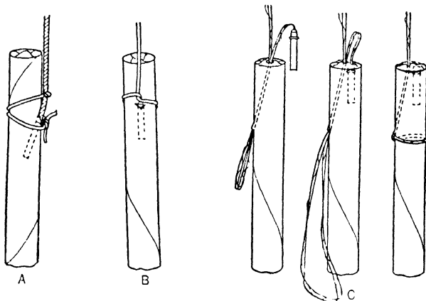
Fig 7. Methods for Priming Dynamite. A and C are recommended; B, often used
