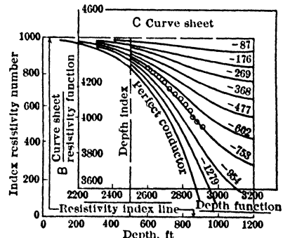
Fig 35 Resistivity Curve plotted from Conversion Table. Low-resistance Bed
