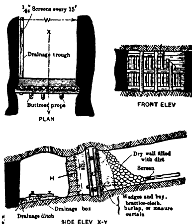
Fig 782 Bulkheads for Dips of 10° to 25°
