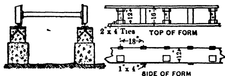
Fig 90. Skip-track Concrete Stringer and Form ( E & M Jour )
