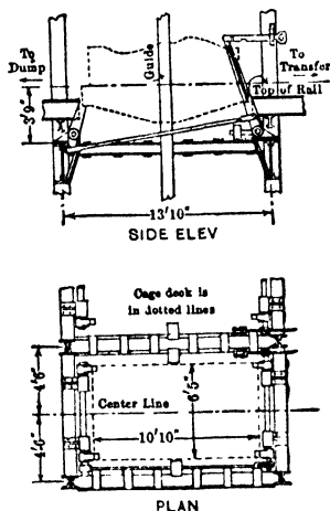
Fig 120 Surface Chairs, Anna-belle Shaft, Four States Coal and Coke Co
