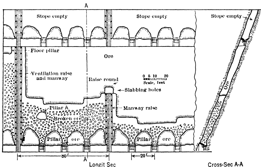
Fig 438. Shrinkage Stope in Nevada-Massachusetts Mine, Mill City, Nev
