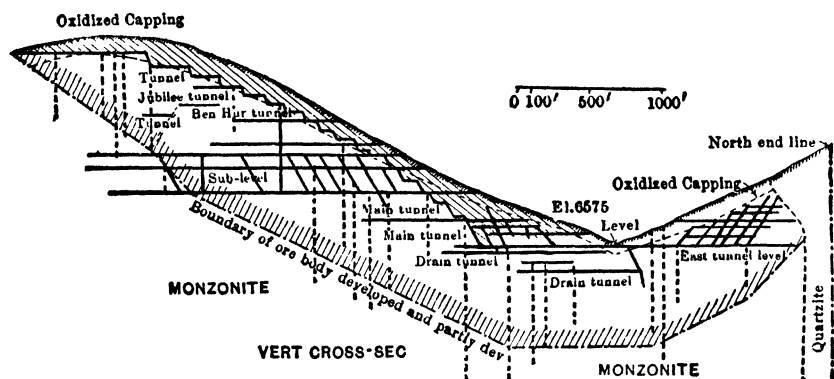
Fig 672. Open-cut Mining, Utah Copper Mine
