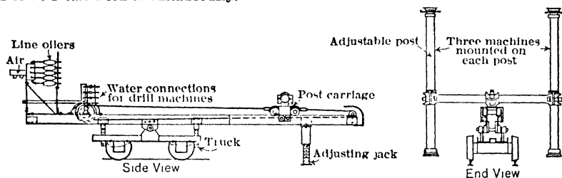
Fig 1 Drill Carriage, Montreal Mine
