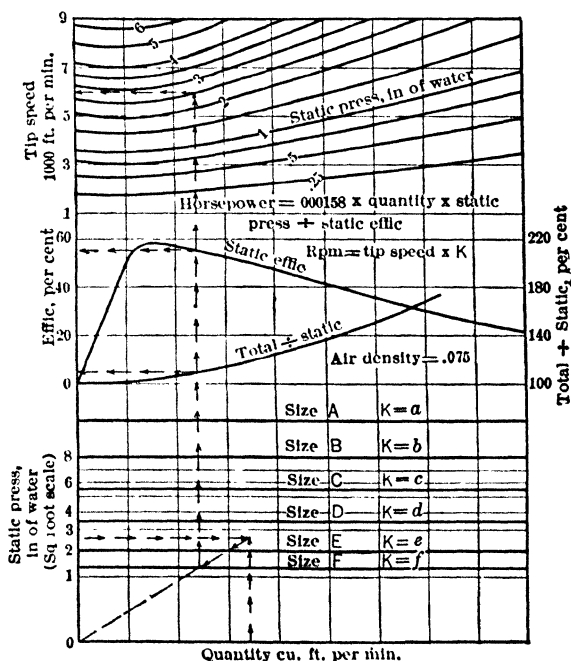
Fig 55. Performance Chart, B. F. Sturtevant Co (9)
