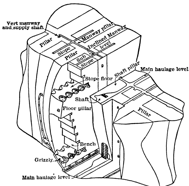
Fig 274. Sub-level Stoping, "Lower H" Orebody, Horne Mine, Noranda, Quebec
