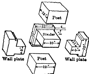
Fig. 22. Framing for Spliced Wall Plate (16)
