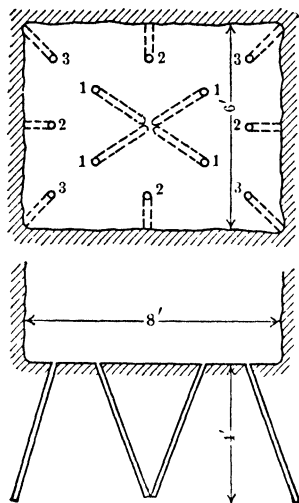
Fig 8. Pyramid Cut for Rectangular Shaft
