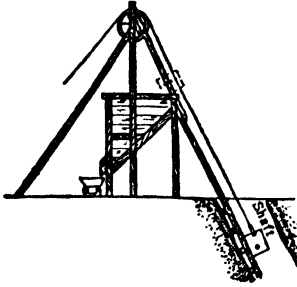
Fig 65 Frame for Inclined Shaft, Porcupine, Ont
