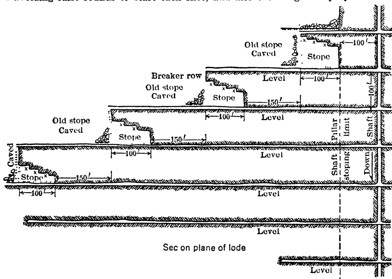
Fig 243. Retreating Stopping System, Conglomerate Lode, Calumet, Mich. (x indicates position of drills)
