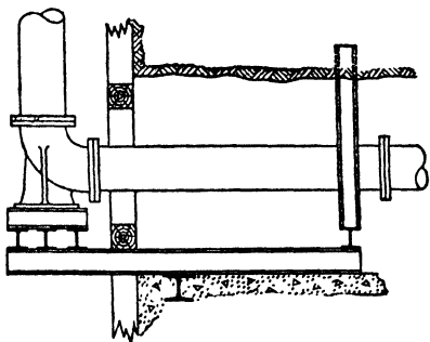
Fig 10. Mode of Supporting Column Pipe in Shaft
