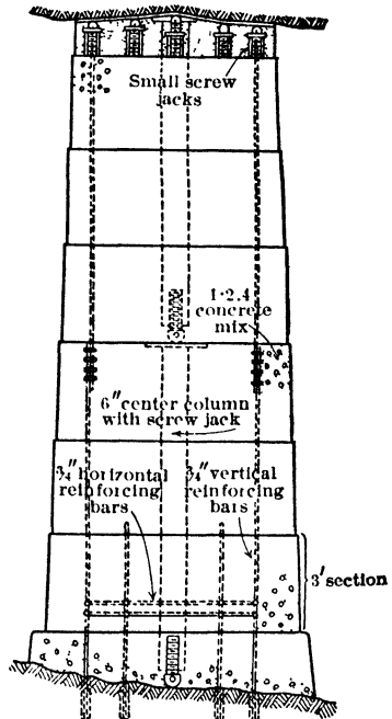
Fig 181. Concrete Column replacing Ore Pillar, S E Mo
