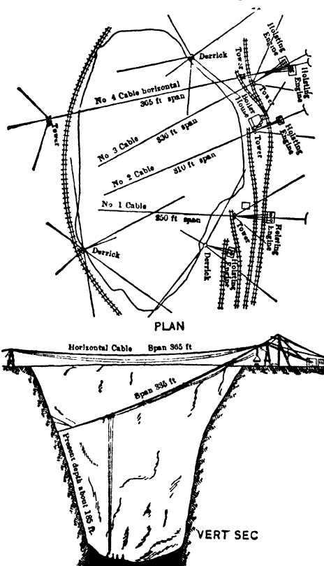
Fig 666. Open Pit, Tilly Foster Iron Mine, N Y
