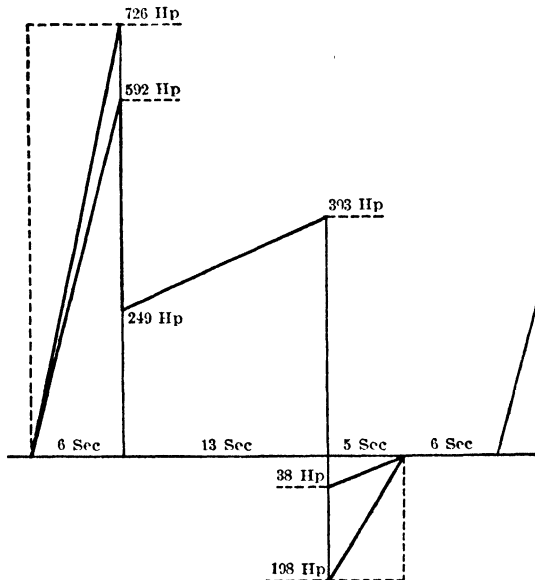
Fig 44. Power Diagram for Conical Drum (Gen Elec Co)
