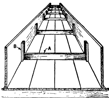
Fig 876. Typical Palong (supports omitted)
