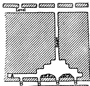
Fig 230 Level-pillars, Overhand Stope (Sec in plane of vein)
