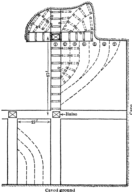
Fig 470. Radial Slicing, Mesabi Range, showing Successive Stages of Removal
