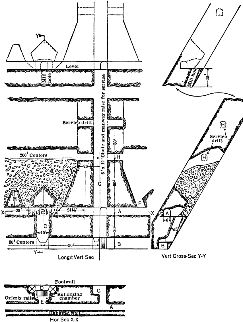
Fig 446. Shrinkage Stopping, Walker Mine (ideal sections)
