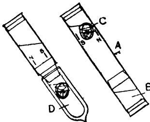
Fig 62. Maas Borehole Compass
