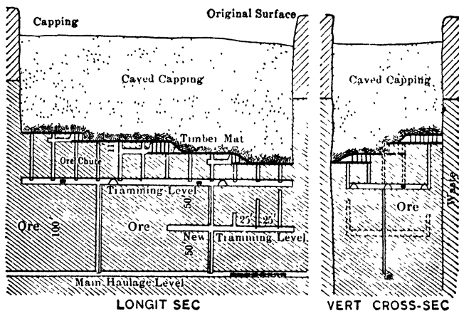
Fig 491. Top-slicing, Arizona Copper Co, Morenci, Ariz
