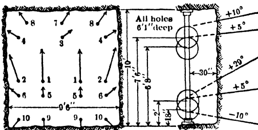
Fig 124. Top-draw Cut in Blocky Sulphide Ore, Mountain Con Mine, Butte, Mont
