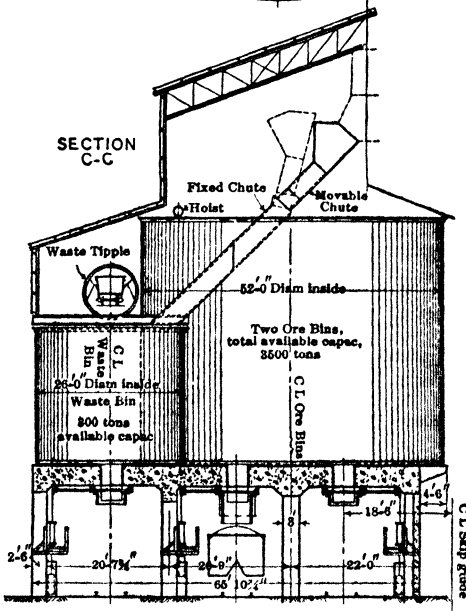
Fig 155. Ore Bins, Porphyry Shaft, Inspiration Mine, Ariz
