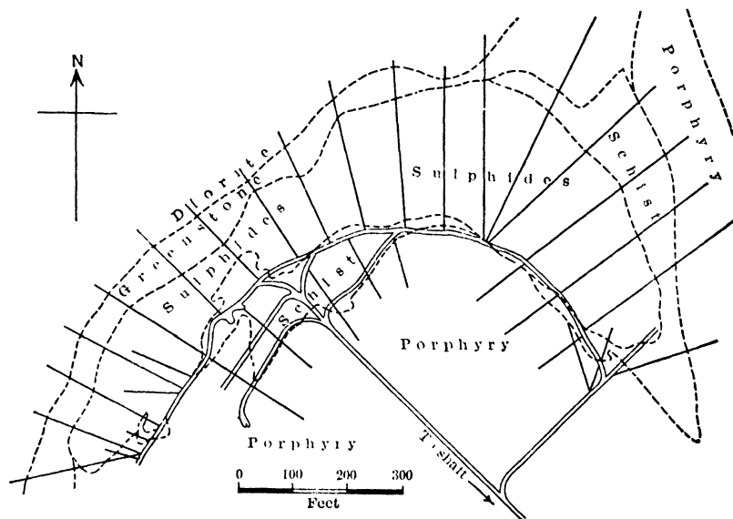
Fig 48 Diamond Drilling on One Level of United Verde Mine, Jerome, Ariz (97)
