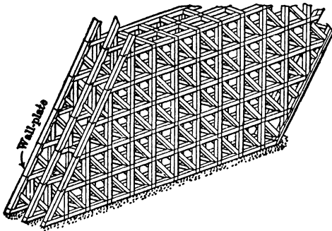
Fig 349. Complete Reinforcement, Deidesheimer System
