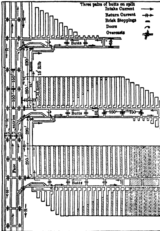
Fig 721. Systematic Mining, Pittsburgh Region
