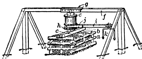
Fig 53. Whim for Sinking Shaft at Mineville, N Y
