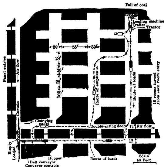
Fig 733. Tractor-trailer Cycle, Moffat Mine, Ill (634)
