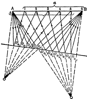
Fig 53. Seismic Paths in Continuous Profiling (25)
