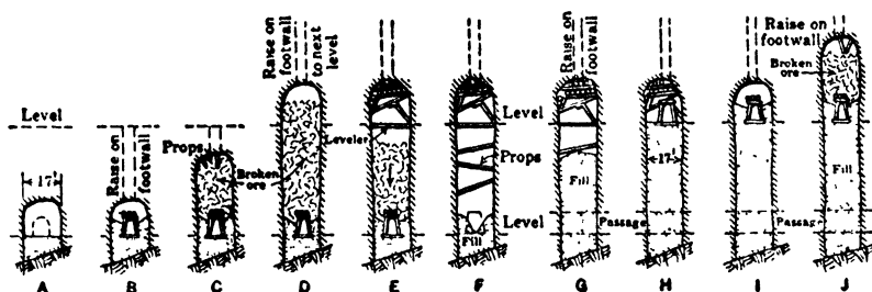
A Drift widened, bottom filled B Sets on fill, footwall raises C Stope being carried up D Stope finished, 15 ft or more above level E Pulling stope, back taken up, levels placed F Stope finished, with props to hold sides G Stope being filled, with passage on lower level H Stope filled, sets erected, ready to take out timber I Fill behind sets, ready for mining J Stope going up to repeat cycle.
