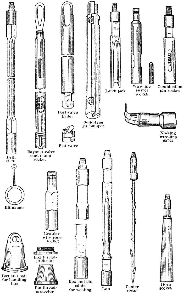
Fig 41 Drilling and Fishing Tools for Churn Drilling (Bucyrus-Armstrong)
