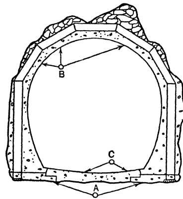
Fig 24. Order of Concreting, Colorado River Aqueduct
