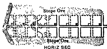
Fig 588. Miami Method, Drill Holes in Pillars
