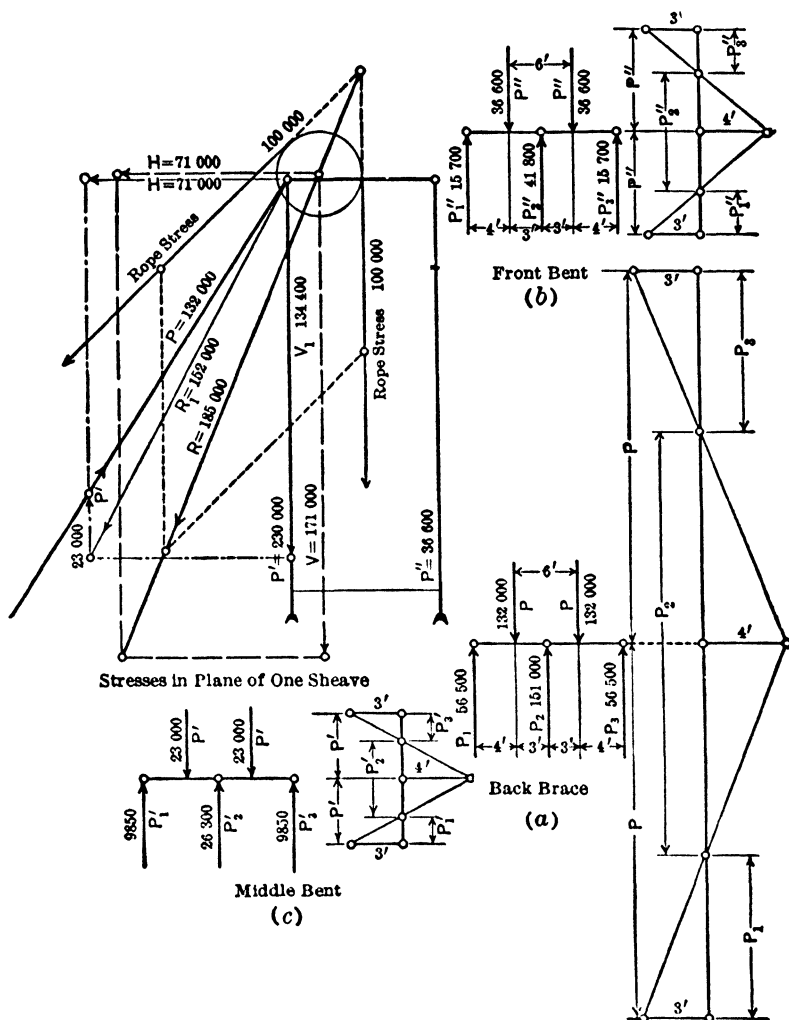
Fig 60. Resolution of Stresses in Plane of One Rope and Sheave
