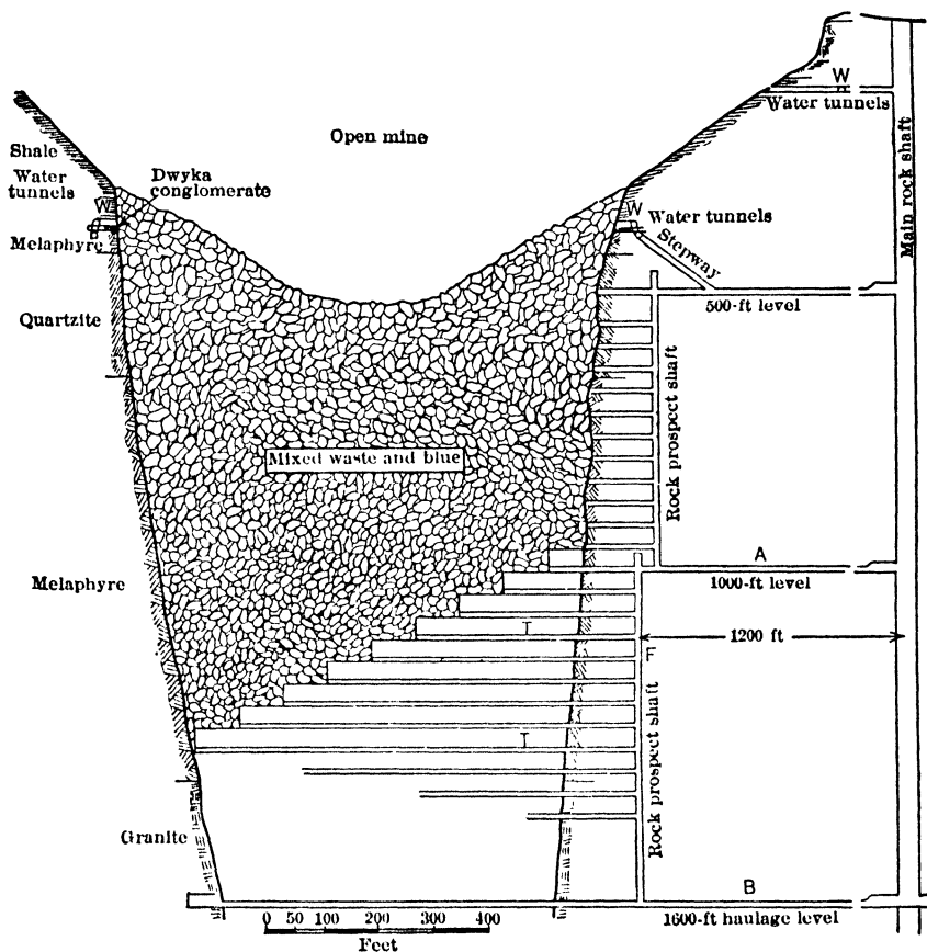
Fig 607 Vert Cross-sec showing General Development, De Beers Diamond Mine, Kimberley, So Africa
