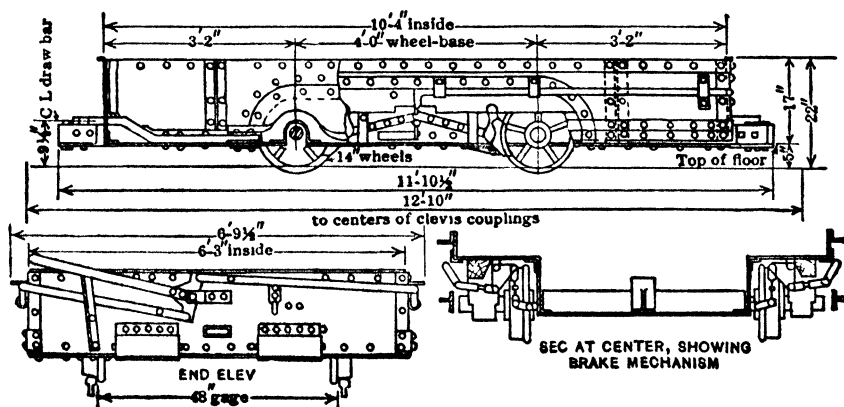
Fig 1 All-steel, "Low-vein" Car
