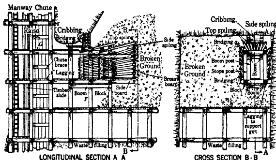
Fig 369. Recovering Square-set Stope, Butte, Mont (534)
