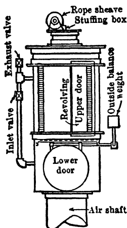
Fig 12 Mattsen Lock
