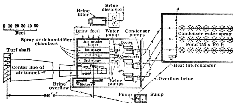
Fig 61. Sketch-plan of Robinson Deep Refrigeration Plant (79)
