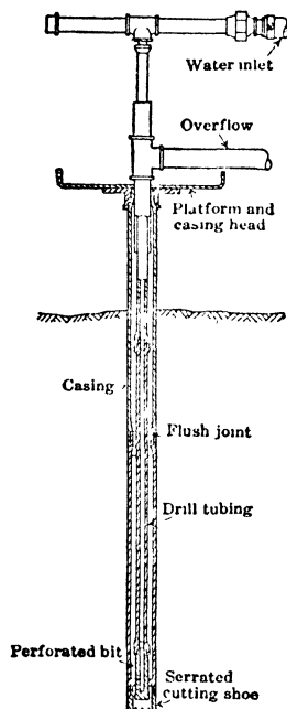
Fig 9. Empire Hydraulic Jetting Drill
