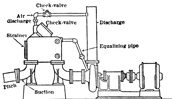
Fig 25. Centrifugal Pump with Suction-line Primer
