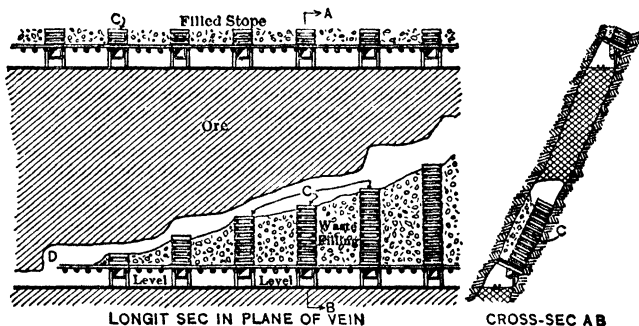
Fig 374. Filled Stope, Narrow Vein
