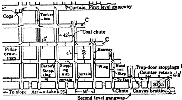
Fig 748. Development by Chute-and-pillar, with Ventilation Details, Pierce County, Wash (610)
