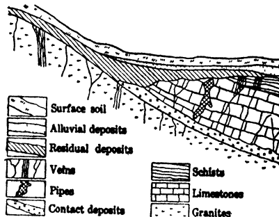
Fig 873. Types of Malayan Tin Deposits. Ideal Sec
