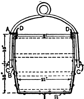
a. Oil-barrel Bucket (E & M J)
