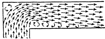
Fig 21. Air Flow at Bend (9)
