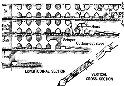
Fig 254 Stoping Method, Quincy Mine, Showing Use of Light Scraper and Portable Hoist
