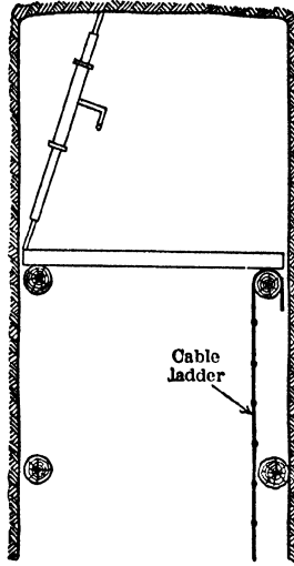
Fig 160. Use of Stulls in Single-compt Raise
