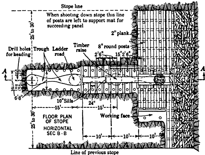
Fig 503 Humboldt Mine, Ariz, Inclined Top-slicing
