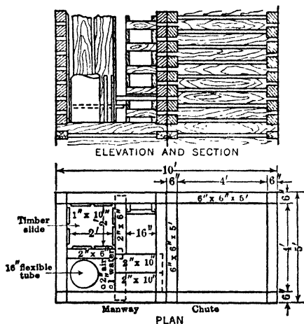
Fig 14. Two-compartment Cribbed Raise (9)
