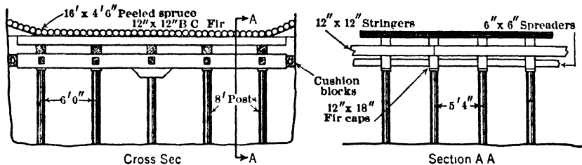
Fig 299 Sill-floor Timbering, Lake Shore Mine, Kirkland Lake, Ont
