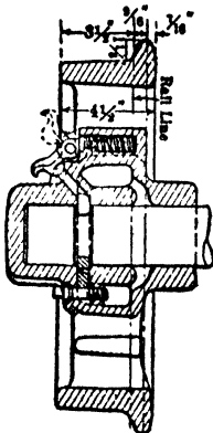
Fig 18. Faught Self-oiling Wheel
