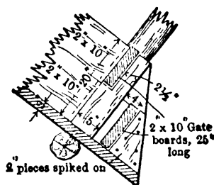
Fig 630. Chute-gate, Dives Pelican Mine, Colo
