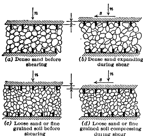
Fig 1. Effect of Shear on Volume of Sand, Shown by Grain Rearrangement
