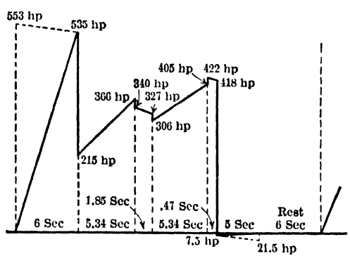
Fig 46. Power Diagram, Cylindro-conical Drum, Plotted to Time
