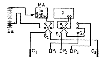
Fig 30. Circuit Diagram for Earth Resistivity Measurements (12)
