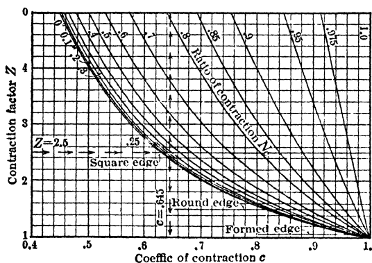
Fig 26. Relation of Coefficient of Contraction c to Contraction Factor Z (19)
