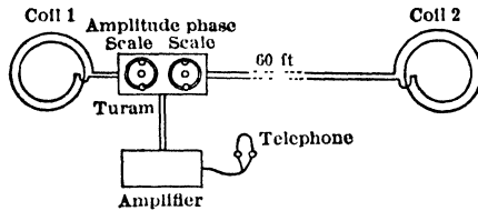
Fig 36. Apparatus used in Turam Method (14)
