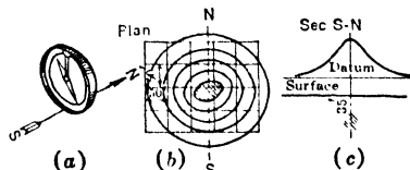
Fig 12. Dip Needle perpendicular to Magnetic Meridian (6)
