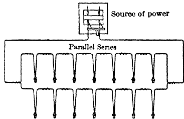
Fig 11 Parallel-series Wiring
