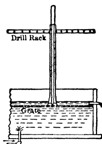
Fig 3 Drill-tempering Tank
