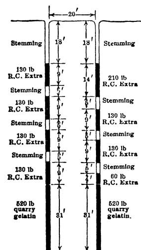
Fig 12. Alternate Methods of Charging a 6-in Hole
