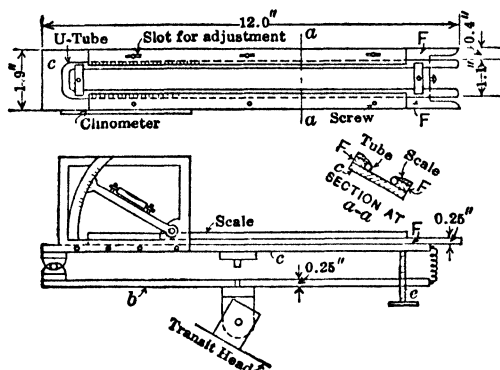
Fig 19. Weeks Manometer (Min &amp; Met, Jan, 1923)
