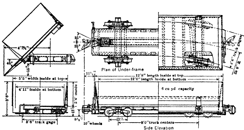
Fig 17a. Double-truck Car, Hanna Coal Co, St. Clairsville, Ohio
