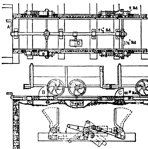
Fig 116 Automatic Cager
