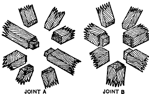
Fig 364. Details of Joints, Moore System
