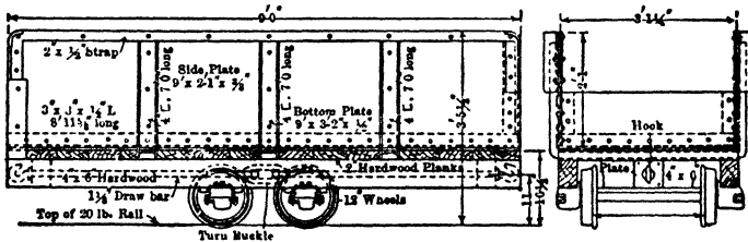
Fig 4. Trimountain Copper-mine Car
