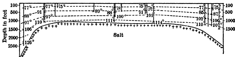
Fig 58. Isothermal Profile W-E across Humble Salt Dome, Texas (26)
