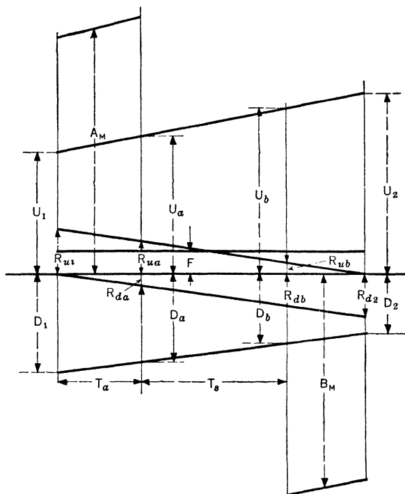
Fig 41 Component Moments, Load Diagram for Conical Drums and Reels, plotted to Revolutions
