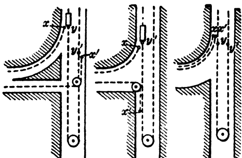
Fig 57. Modes of Attaching Branch Ropes x, x' to Main Rope y, y'
