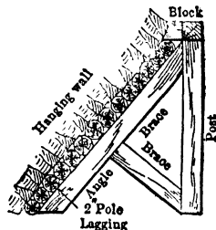
Fig 347. Angle Set (E & M Jour)
