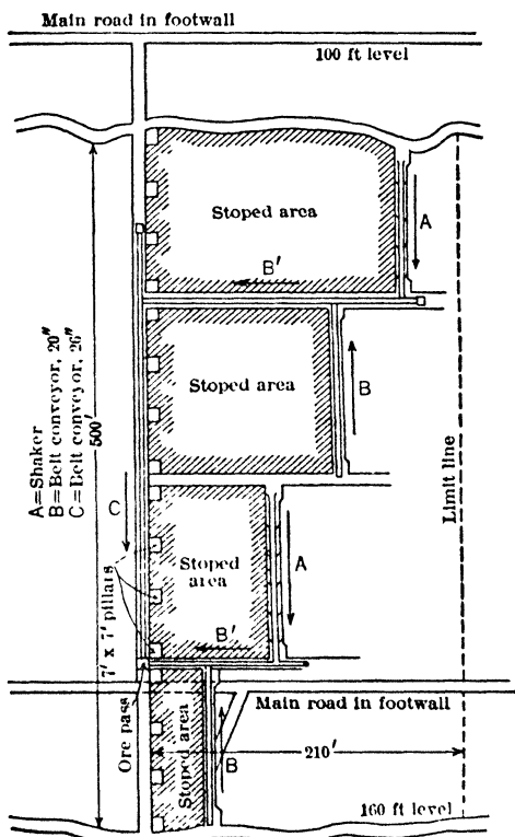
Fig 654. Stopping with 'Shaking Chutes and Belt Conveyers, Boleo Mines
