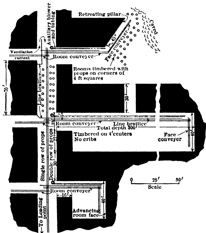
Fig 728. Typical Room Diagram, MacAlpin Coal Co (490)
