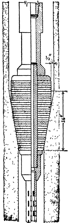
Fig 32. Johnston Formation Tester
