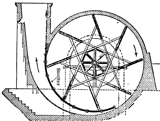
Fig 36. Early Type of Guibal Fan (12)
