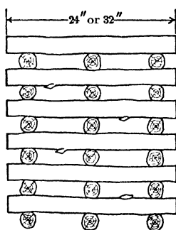
Duplex Pack. Three 3" sticks in each row. Also made of 4" sq sticks, 48" long
