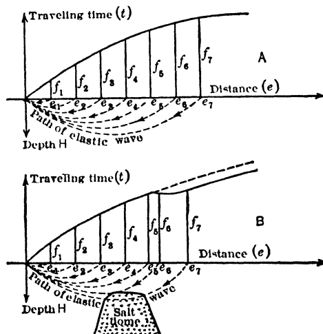
Fig 51. Mintrop Geological Testing Method. Adapted from Mintrop (23)
