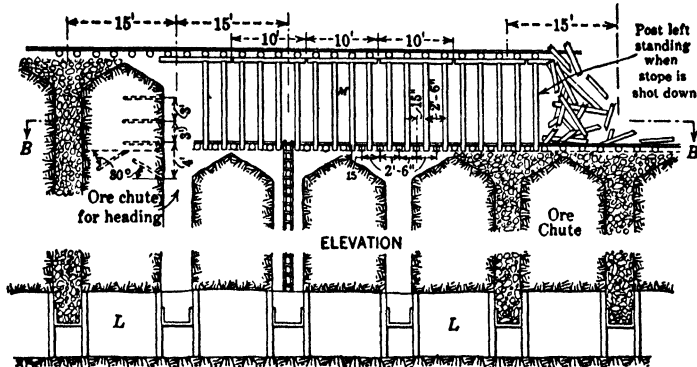
Fig 502. Humboldt Mine, Ariz, Inclined Top-slicing. Sec A-A, Fig 503
