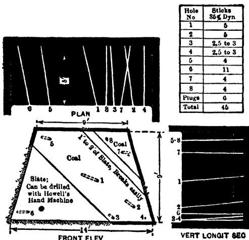
Fig 773. Driving Gangway, Buck Mtn Seam
