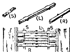
Fig 836. Bouery Manganese-steel Riffle
