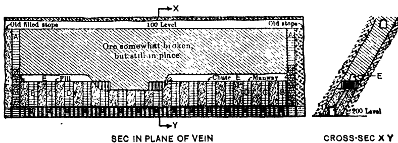
Fig 384. Filled Flat-back Stope in Weak Ore
