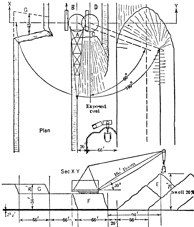
Fig 693 Stripping Coal Seam with Dragline Alone
