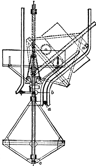
Fig 113. Self-dumping Cage
