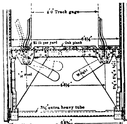
Fig 117. Car Stops for Self-dumping Cages, Jed Coal and Coke Co
