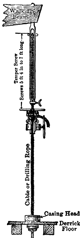
Fig 14. Method of Suspending Drilling Rope
