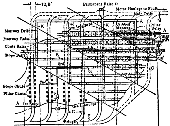
PLAN, 1ST SUB AND MOTOR LEVEL
