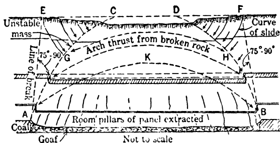
Fig 791. Suggested Mechanics of Room-and-pillar Caving (623)
