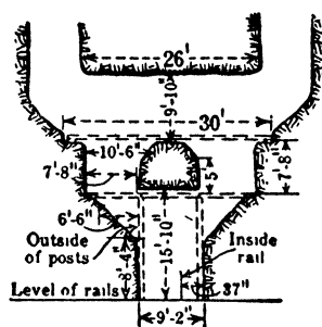
Fig 599. Silver Dyke Mine. Rock Limits of Double-pocket Chute and Bulldozing Chamber
