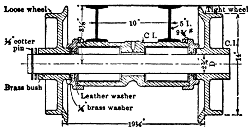
Fig 19. McCaskell Wheel and Axle
