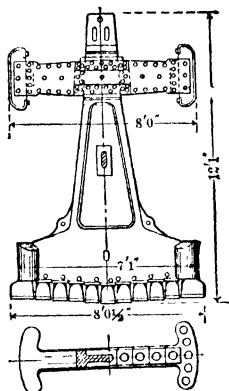
Fig 30 Small Trepan
