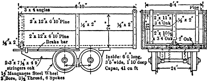
Fig 3. Sub-level Car, Mesabi Iron Range
