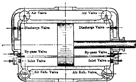
Fig 49. Anaconda Air-hoist Cylinder, B. V. Nordberg (47)
