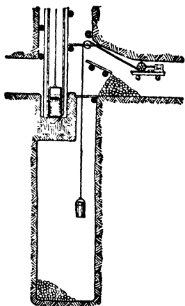
Fig 14. Sinking Under Rock Pentice
