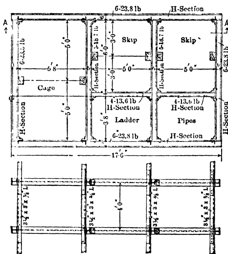
Fig 25. Steel Timbering for 5-compartment Shaft
