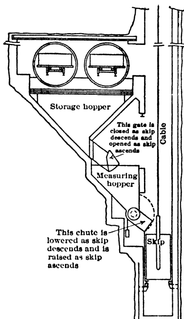
Fig 146. Shaft Bottom Dumping Arrangement, Standard No 2 Mine, Schoper, Ill (37, 69)
