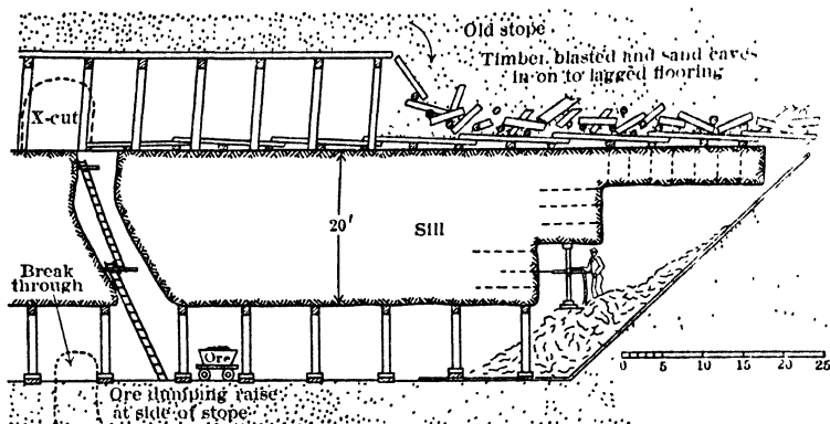
Fig 304. Mining Level-pillar, Hollinger Mine, Ontario
