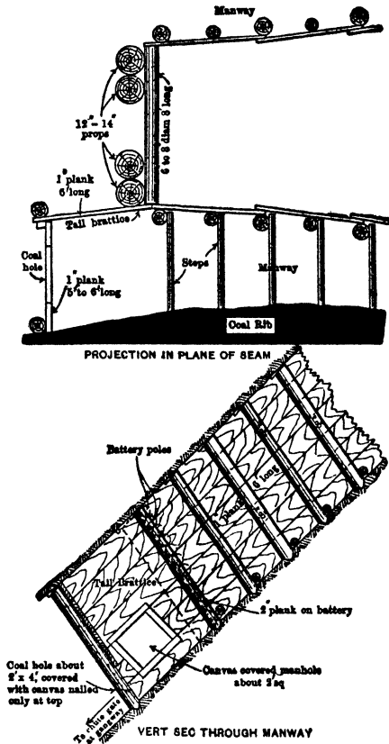
Fig 714. Battery Construction
