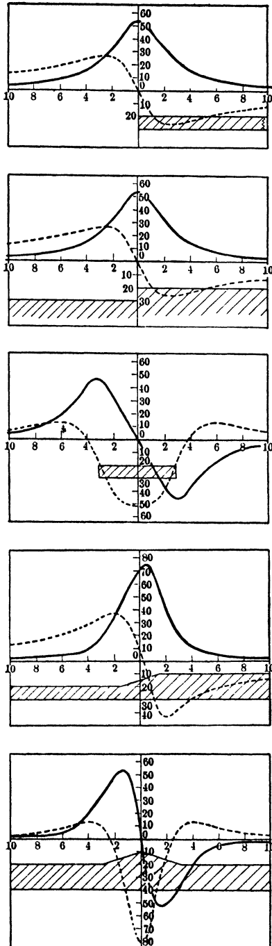
Fig 1. Theoretical Gradient and Curvature Anomalies caused by Geologic Conditions (1)
