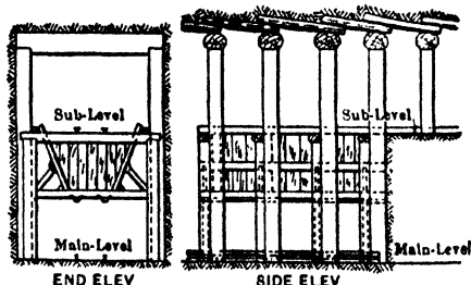
Fig 645. Hanging Chute-gate, Mesabi Range, Minn
