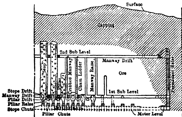
Fig 571. Ray Motor-haulage System
