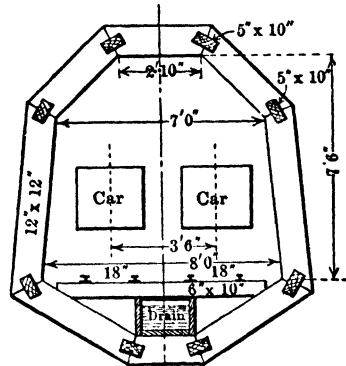
Fig 21. Inverted Arch Set for Swelling Ground
