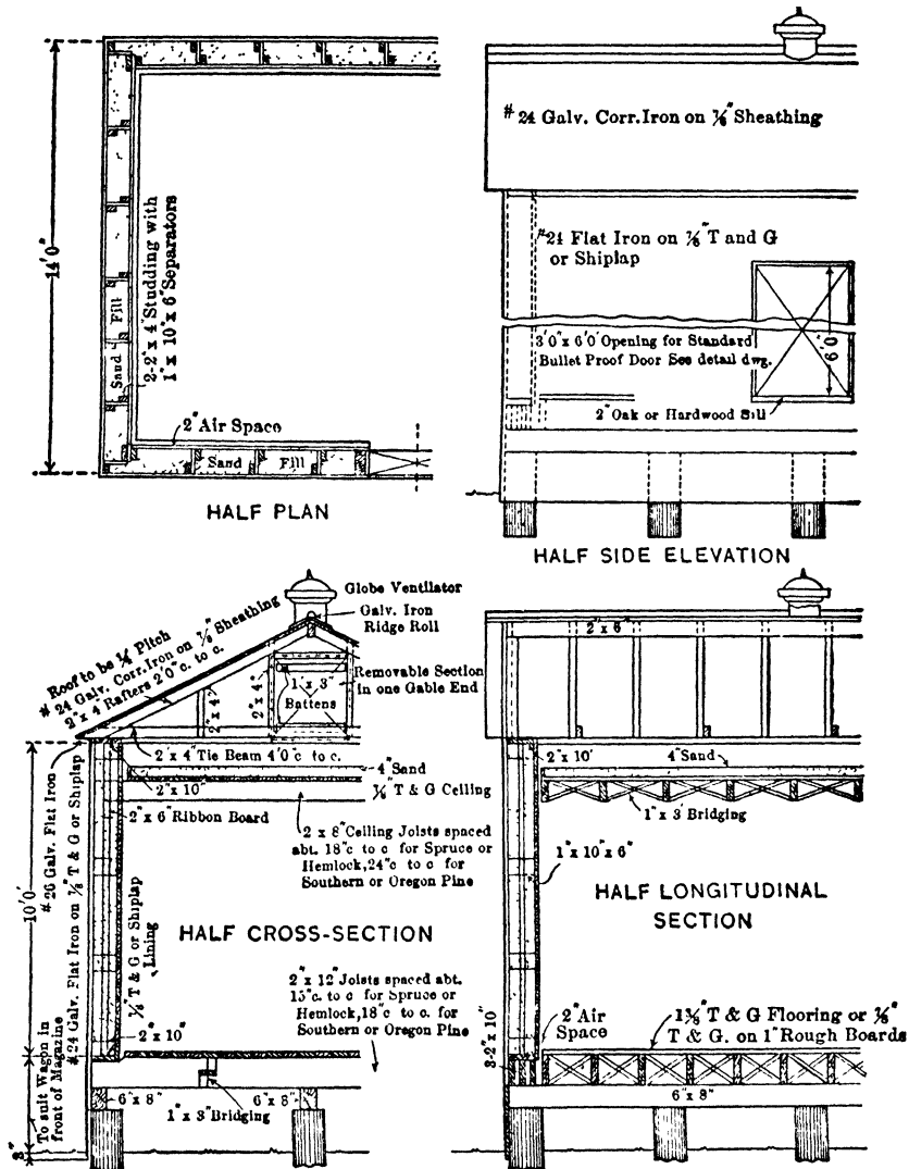
Fig 5. Wooden Dynamite Magazine
