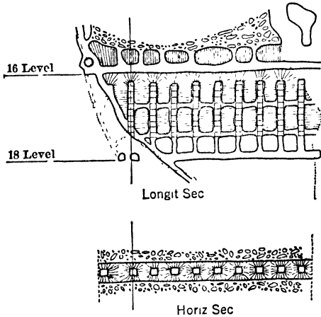
Fig 456. Sec through Pillar, showing Raizes and Drill Holes, Creighton Mine, Ont
