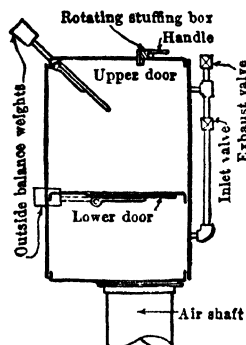
Fig 13 Moran Lock
