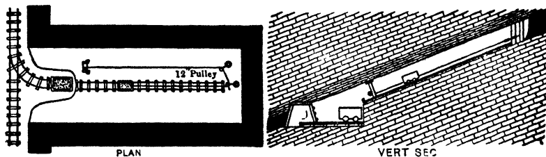
Fig 711. Buggy Breast (Coal Miners' Pocketbook. Pitch exaggerated)
