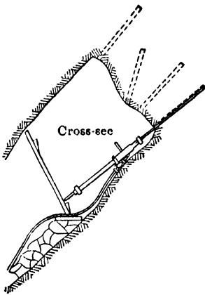
Fig 159. Draw-cut for Small Inclined Raise
