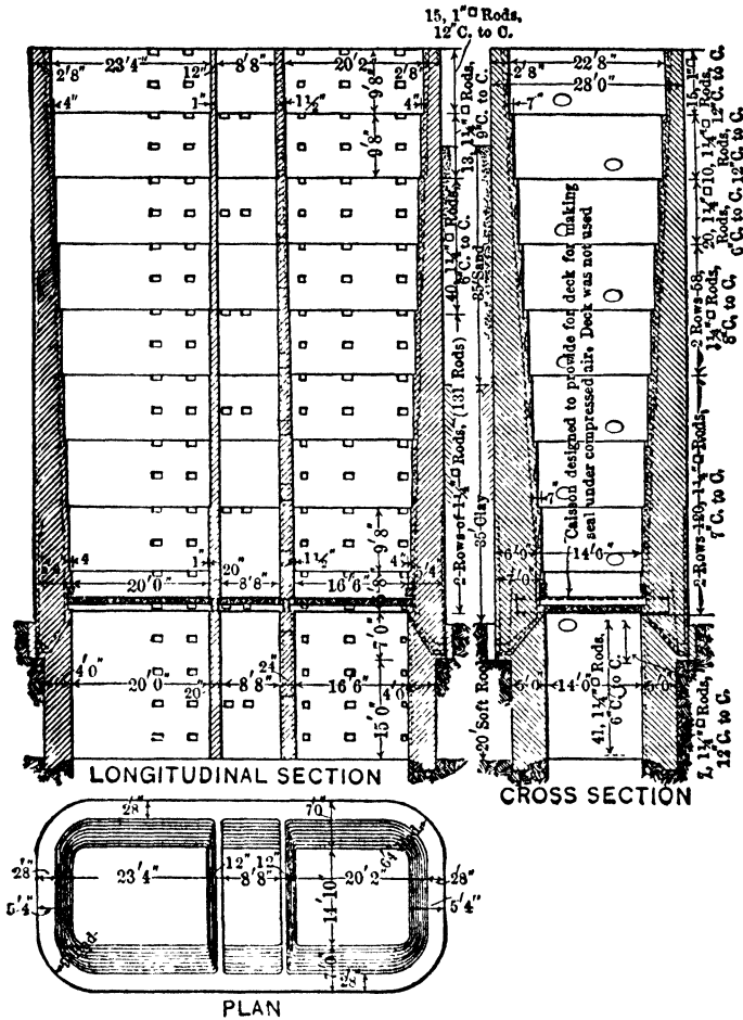
Fig 11 Del, Lack & Western Colliery Caisson ( Eng News )
