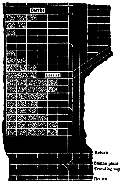
Fig 739. British Practice, Bord-and-pillar or Panel System (Hughes)
