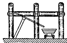
Fig 479. Chute for Square-set Slicing, Mesabi
