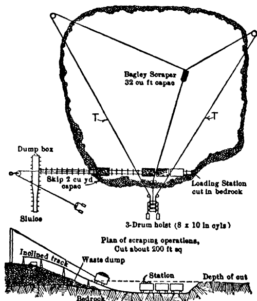
Fig 811. Bagley Scraper with Incline and Auxiliary Hoist
