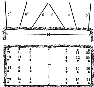
Fig 149. Simple V-cut, Sullivan Mine, Kimberley, B C
