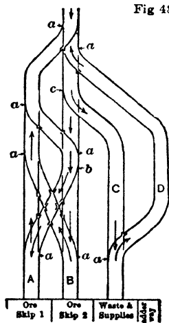
Fig 49. Shaft Station Layout
