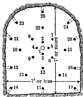
Fig 135 Burned Cut, Franklin Mine, Franklin, N J. Central holes, 8.5 ft deep, others, 8 ft. Center hole, unloaded, has 3-in diam. Holes fired in sequence, as numbered, using fuses all of same length. Loaded and fired in 4 rounds. Nos 2-5, Nos 6-9, Nos 10-14, Nos 15-25
