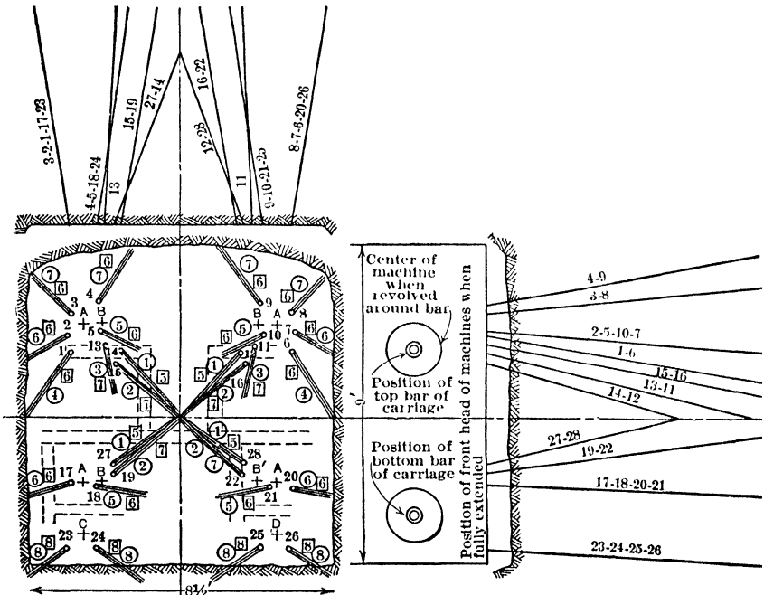
Fig 8. Double Pyramid-cut Round (Ojuela Tunnel)
