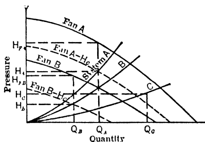
Fig 53. Solution by Trial and Error for Fans acting in Parallel on Separate Airways (9)
