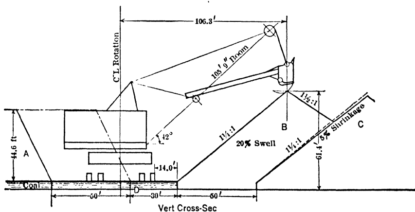
Fig 691. Stripping Coal Seam with Power Shovel Alone
