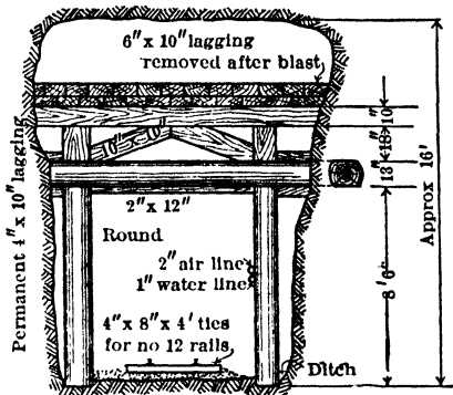
Fig 418. Typical Sill Timbering, Victoria Mine, Britannia Beach, B C
