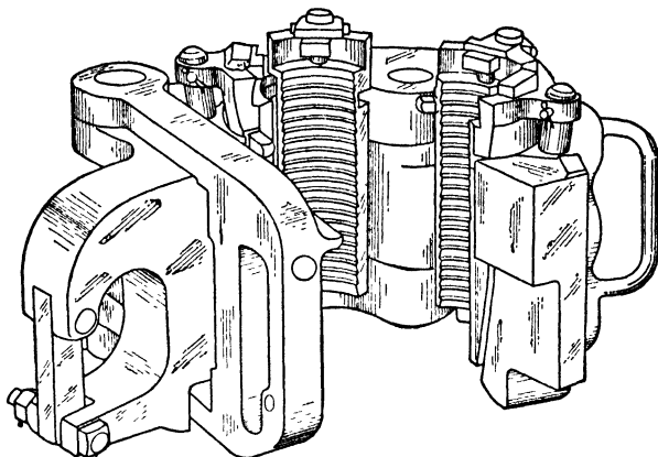
Fig 29. Ideal Door Grip Tubing Elevator
