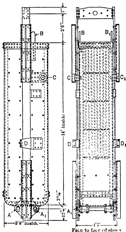
Fig 129 145-Cu ft (10-ton) Skip, Belmont, Badger State, and Mountain Con Mines, Anaconda C M Co, Butte, Mont (79)
