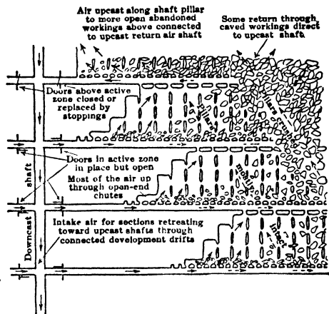
Fig 11. Method of Ventilating Retreating Open Stopes (9)
