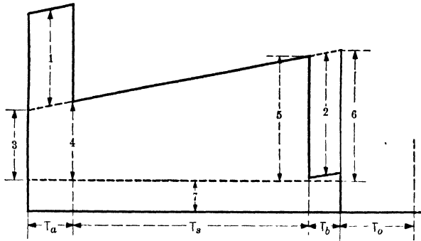
Fig 42 Resultant Moments, Load Diagram for Conical Drums and Reels, Balanced Operation plotted to Revolutions
