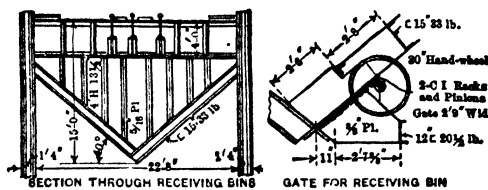
Fig 160. V-bottom Bins, Ariz Copper Co (89)
