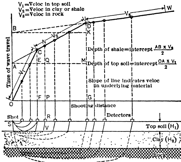
Fig 50. Time-distance Curves for First Arrival of Waves. Adapted from E. R. Shepard (12)
