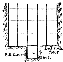
Fig 343. Leonard Mine; Vert Cross-sec through Slope
