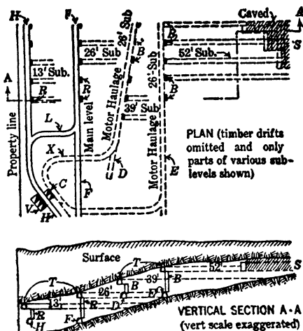
Fig 483. Top-slicing, Utica Mine, Minn (diagrammatic)
