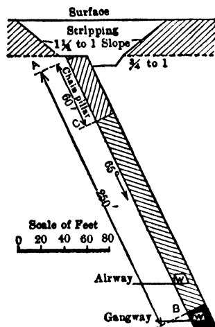
Fig 697. Pennsylvania Anthracite Stripping
