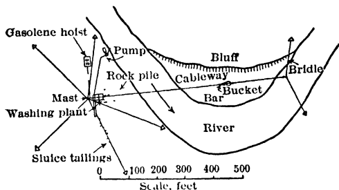
Fig 810 Placer Mining with Power Scraper, Auburn, Calif
