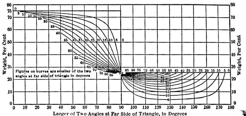
Fig 95. Weighting Factor for Any One of Three Adjacent Boreholes
