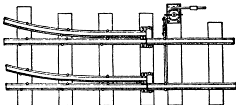
Fig 37. Stub Switch
