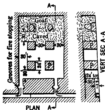
Fig 758. Square-chamber Method, South Staffordshire
