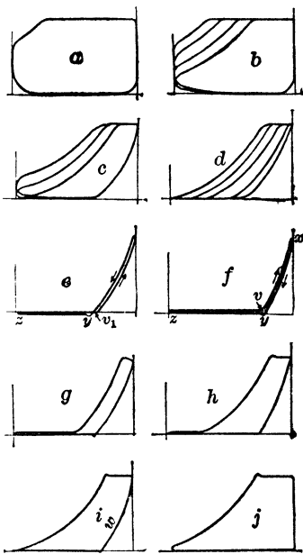
Fig 48 Air-hoist Cards, B. V. Nordberg (47)
