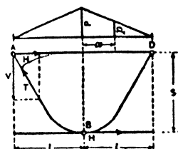
Fig 161 Diagram of Suspension Bunker
