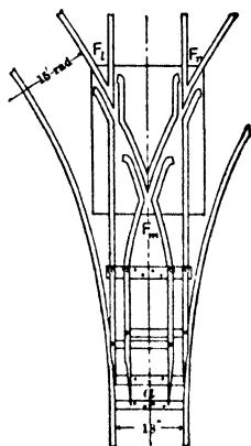
Fig 36 Double Turnout
