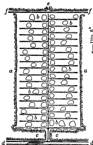
Longit Sec in Plane of Reef
