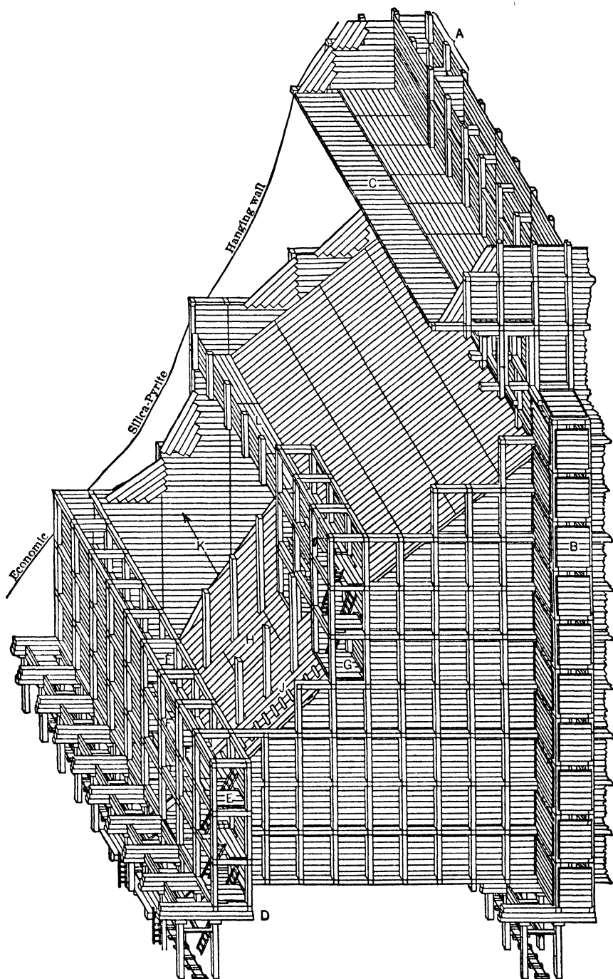
Fig 426. Mining a 48-ft Section under a Filled Stope by Inclined Cut-and-fill, Campbell Mine, Warren, Ariz
