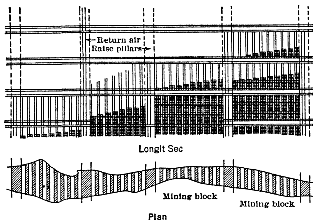
Fig 291. Diagrammatic Plan and Sec of Stopping Blocks, Frood Mine, Sudbury, Ont
