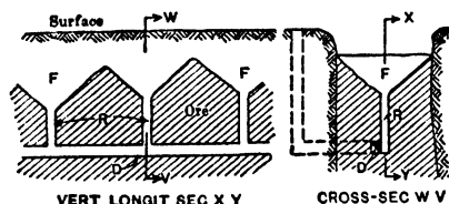
Fig 684. Glory-hole Method (Diagrammatic)
