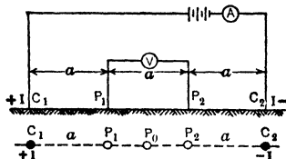
Fig 25. Spacing of Electrodes for Ground Resistivity Measurements
