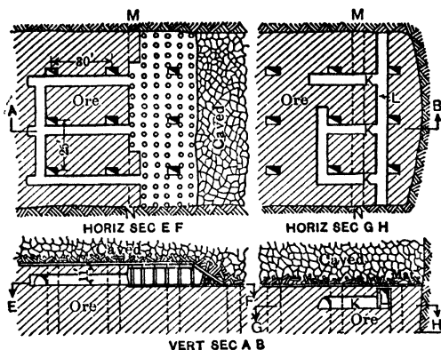
Fig 489. Top-slicing, Morenci-Metcalf Distr, Ariz (diagrammatic)
