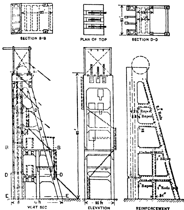
Fig 80 Concrete Headframe, Curry Shaft, Penn Iron Mining Co, Vulcan, Mich ( E & M Jour )
