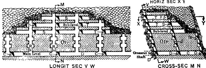
Fig 506. Sub-level Caving in Wide Vein (diagrammatic)
