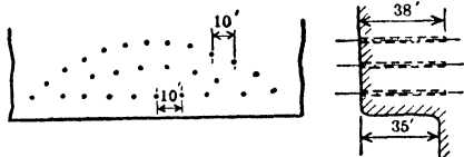
Fig 23. Arrangement of Holes for Breaking Hard Bottom
