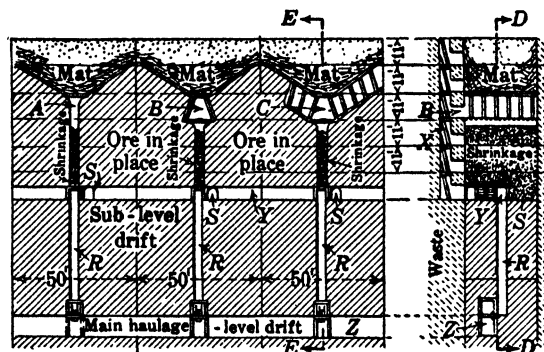
VERTICAL LONGITUDINAL SECTION D-D
