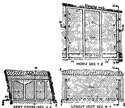
Fig 534. Development for Block-caving, Pewabic Mine
