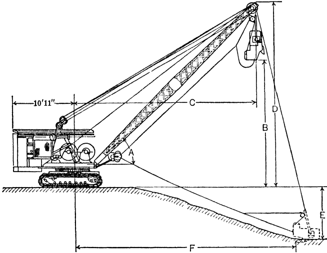
Fig 4 Erie Dragline Scraper
