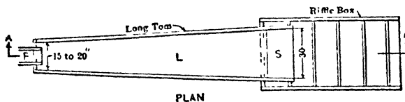
Fig 806 Long Tom (after Bowie)
