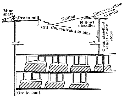
Fig 395. Matahambre System of Filling Stopes (Diagrammatic)
