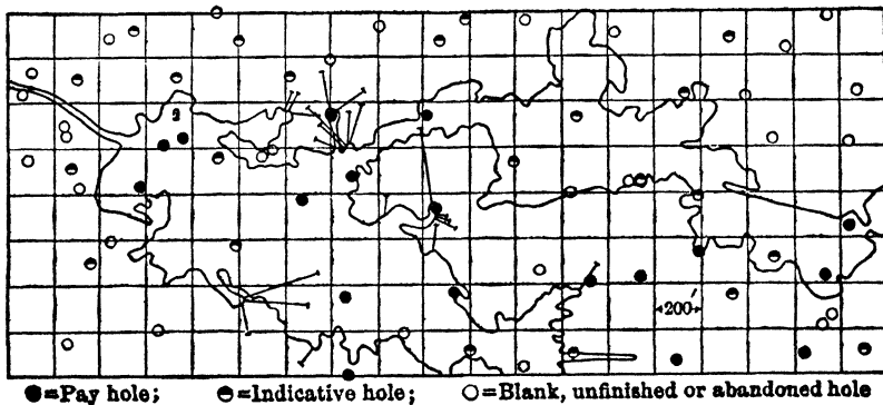
Fig 89. Boring near Flat River, Mo (H. A. Guess)
