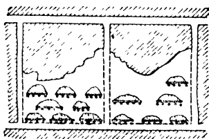
Fig 232 Artificial Pillars (After Hoover)
