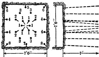
Fig 132. Deep Pyramid Cut in Hard Schist and Quartz. McIntyre Mine, Schumacher, Ont
