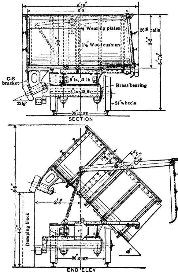
Fig 8. Side-dump Car, 130 cu ft, Granby Mining Co, Anyox, B C
