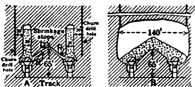
Fig 600. Silver Dyke Mine, Diagrammatic Vert Secs
