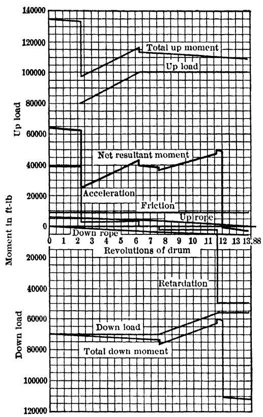
Fig 45. Component and Resultant Moments, Cylindro-conical Drum, Plotted to Revolutions (Gen Elec Co)
