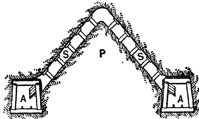
Fig 373. Caving for Waste. Diagrammatic Cross-sec
