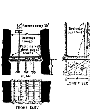
Fig 781 Bulkhead for Dips under 10°
