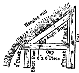
Fig 348. Half-angle Set (E & M Jour)
