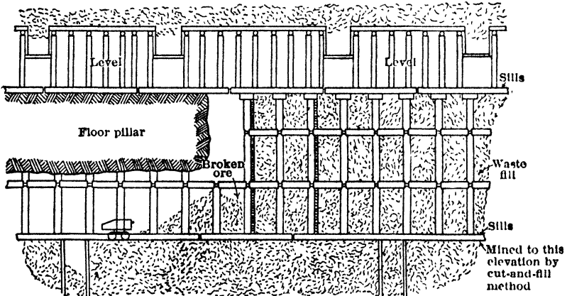
Fig 381. Longit Sec showing Method of Extracting Floor Stills, McIntyre Mine, Schumacher, Ont
