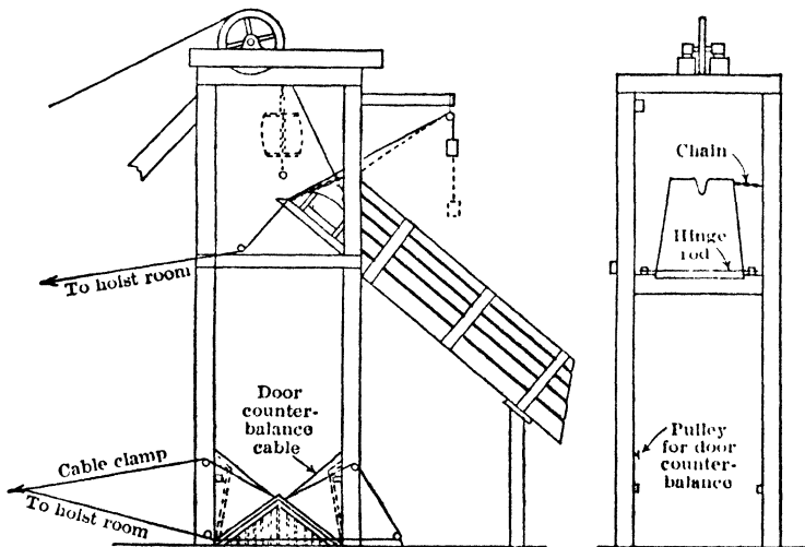
Fig 108. Bucket Dump (37)
