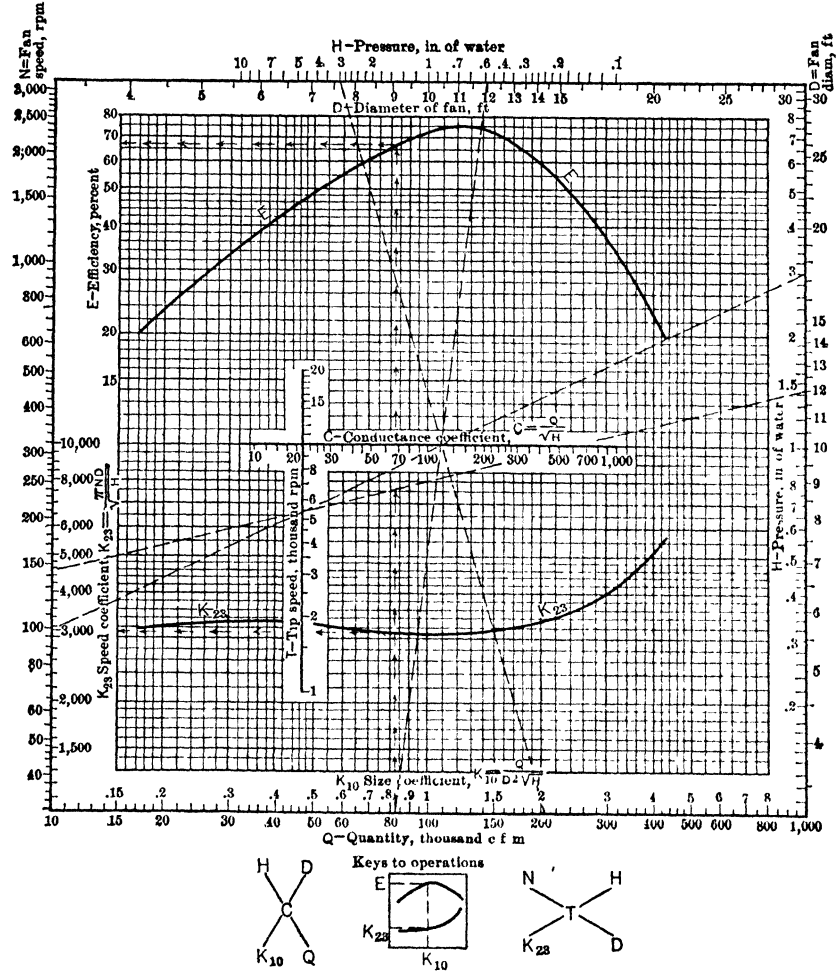
Fig 56. Nomogram Chart for Fan Selection (76)
