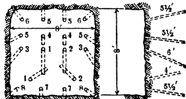
Fig 123 Wedged Draw Cut in Hard Diabase, Pecos Mine, N Mex
