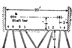
Fig 5. "V," Center or Wedge Cut for Shaft Sinking
