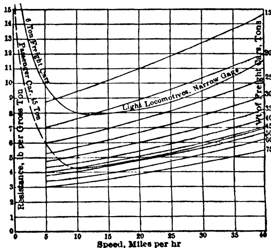
Fig 52. Tractive Resistance of R R Equipment (Baldwin Locomotive Works)
