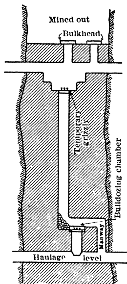
Fig 219 Glory-hole Stope in Chimney Deposit, El Potosí Mine Chihuahua, Mex (Vert sec)
