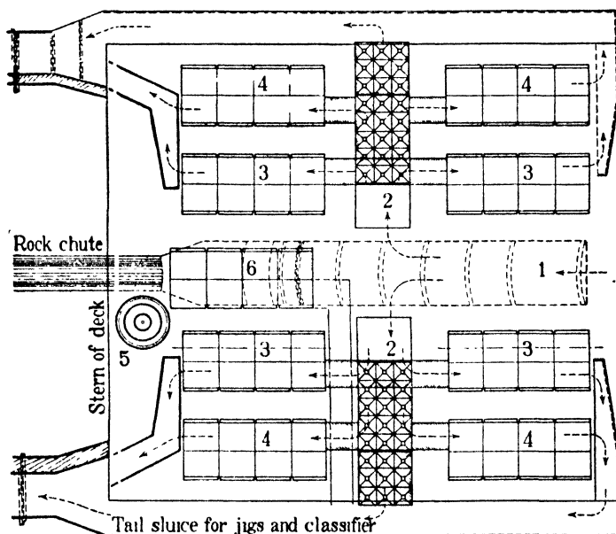
Fig 882 Rantau Classifier-jig Tin Dredge; Outline Deck Plan, showing Arrangement of Equipment. 1, trommel; 2, classifiers; 3, coarse jigs; 4, fine jigs. 5, settling cone to remove water from hutch products; 6, cleaner jig. Classifiers are high enough to feed jigs by gravity. Arrows show direction of flow.
