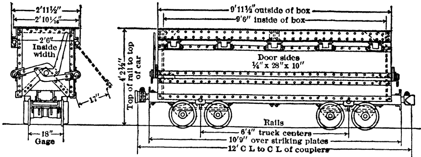
Fig 17c. 57-cu ft, Gable-bottom Car, Park-Utah Consol Mines Co, Park City, Utah
