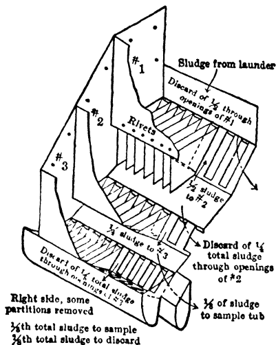
Fig 65. Riffles of Ray Consol Sludge Splitter
