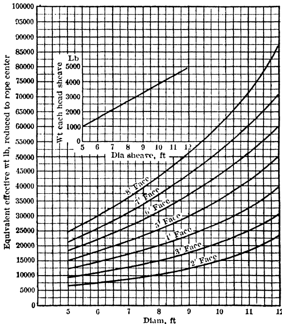
Fig 15. Effective Weight of Drums (Single-cylinder) and Head Sheaves, for Estimating Purposes Only (Gen Elec Co) For gears, add 10%, for double drums, add 100%
