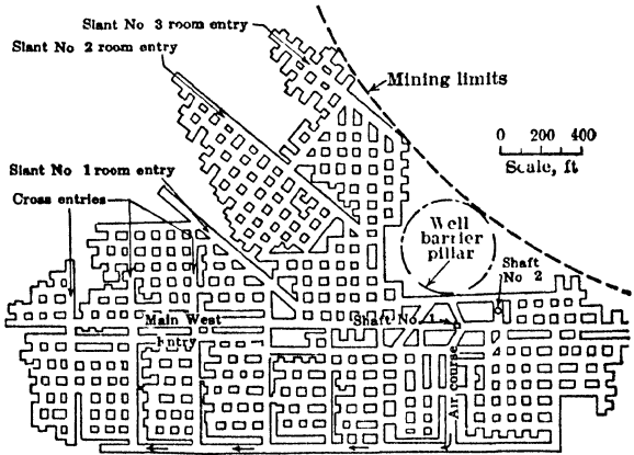
Fig 200 Plan of Workings, Detroit Rock Salt Co, Detroit, Mich
