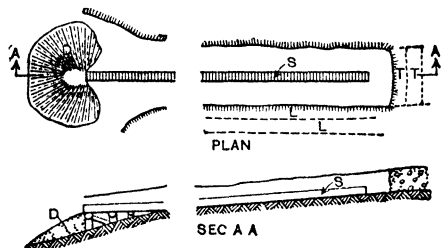
Fig 808 Simple Shoveling-in
