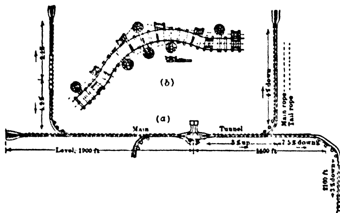
Fig 56. Tail-rope System, Sherrard Mine, Ill (part)
