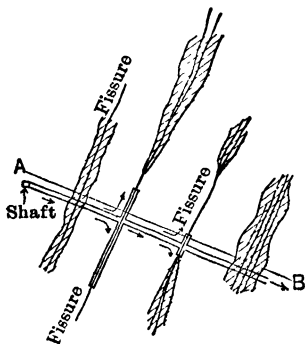
Fig 7 Plan of Flat Shoots in Thin Sedimentary Layers (Arrows show Direction for Crosscuts and Drifts)
