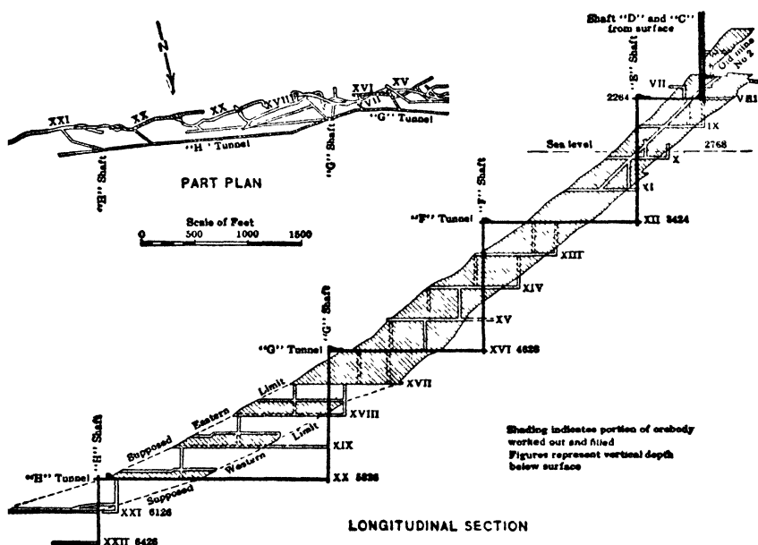
Fig 113. Development at Medium Depth, Morro Velho Mine, Brazil
