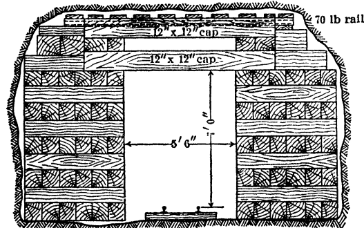
Fig 147. Timber Bulkhead, United Verde Ext Mine
