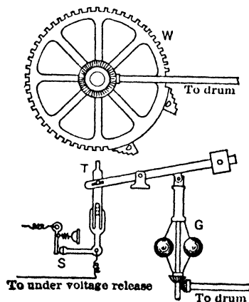
Fig 142. Diagram of Mechanical Overwind Device for Mine Hoists (3)
