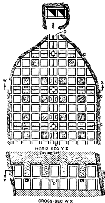
Fig 537. Block-caving into Chutes, Mowry Mine (1933)
