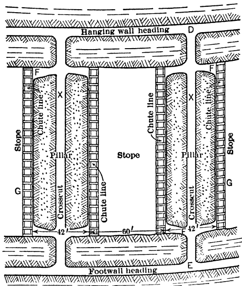
Fig 451. Plan of Sill-floor Operations in Wide Ore, Homestake Mine, Lead, So Dak
