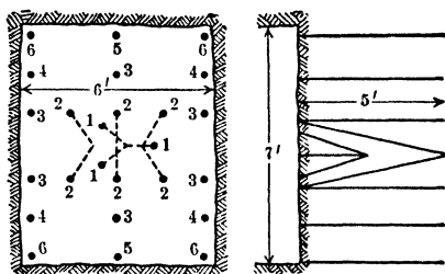
Fig 129. Double Pyramid Cut in Hard Shale and Massive Sulphide Frisco Mine, S F del Oro, Chih, Mex
