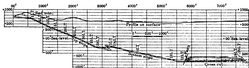
Fig 246. See through Slope of No 3 Mine, Woodward Iron Co, Bessemer, Ala
