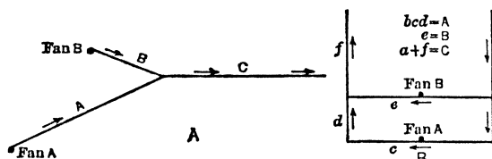
Fig 52 A, Analysis of Flow Conditions for Fans acting in Parallel on Separate Airways, B, Sketch Diagram (9)
