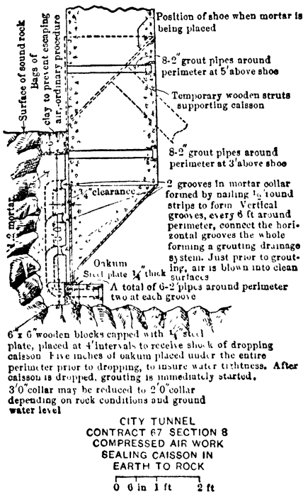
Fig 15 Sealing Details for Drop-shafts
