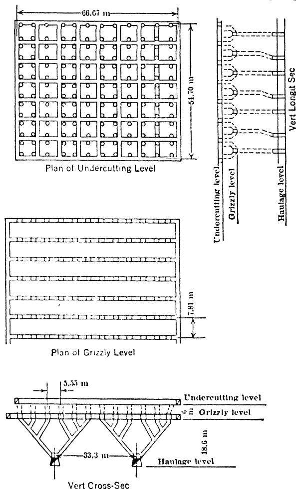
Fig 560. Plans and Secs of Typical Block, Andes Copper Mining Co
