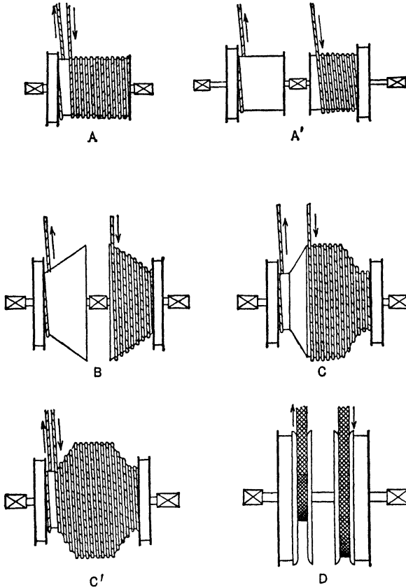
Fig 8. Common Forms of Hoist Drums
