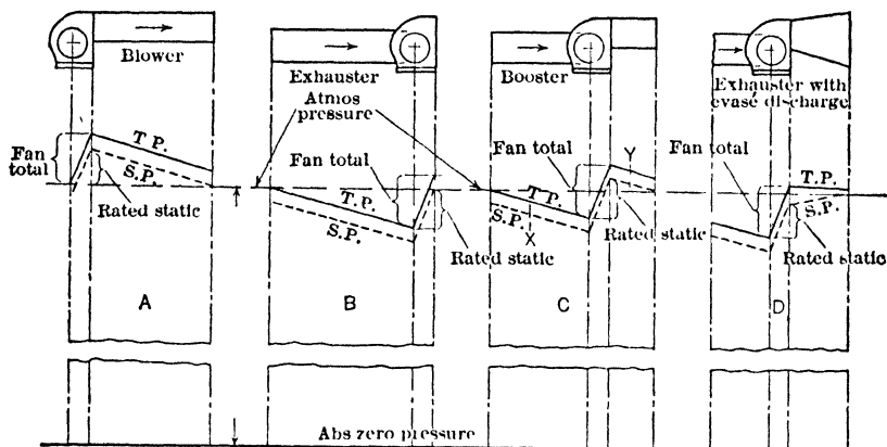
Fig 45. Pressure Changes in Ventilating Systems (71)
