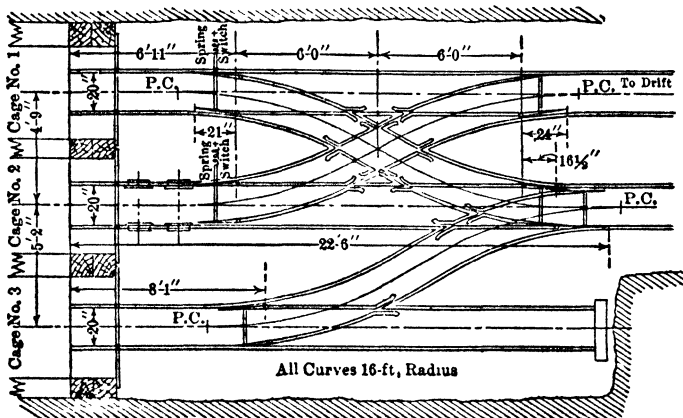
Fig 45. Double Crossover or Diamond Switch
