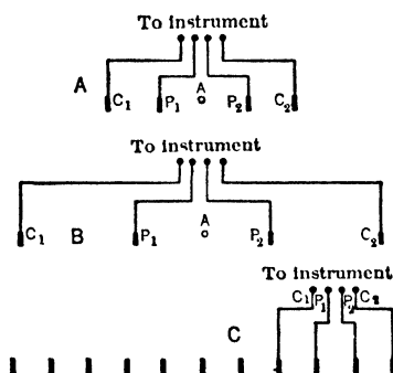
Fig 27 Stake Layout for Measuring Resistivity A and B, for increasing depths at one point C, for constant depth along a line (11)
