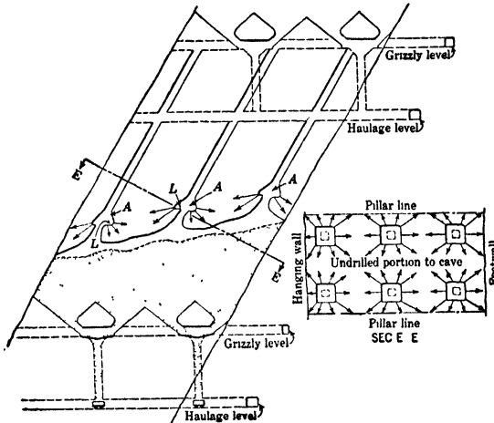
Fig 461. Beatson Mine, Alaska. (Vert sec A-A, Fig 457, later stage)
