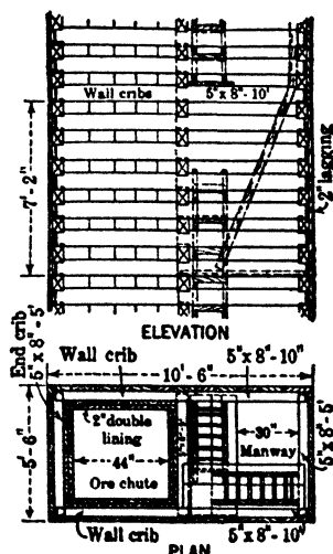
Fig 391. Cribbed Chute and Manway, United Verde Mine
