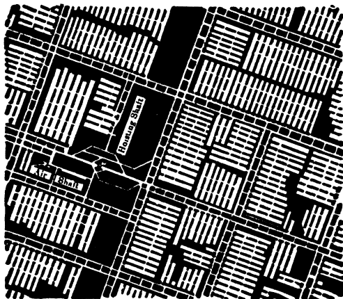
Fig 729. Block Room-and-pillar System, Ill
