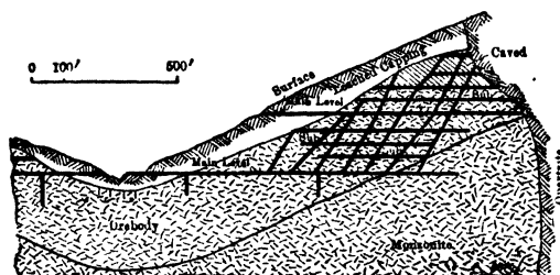
Fig 565. Utah Copper Co Cross-sec through Part of Orebody
