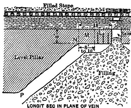
Fig 403. Mining Level-pillars, Baltic Method
