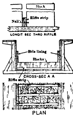
Fig 831. Block Riffles
