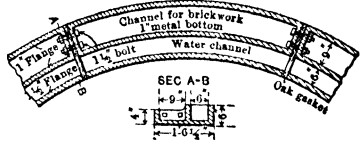
Fig 27. Walling Crib and Water Ring Combined
