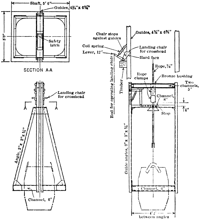
Fig 109. Crosshead for Bucket Sinking, Macassa Mines, Kirkland Lake, Ont (37, 65)
