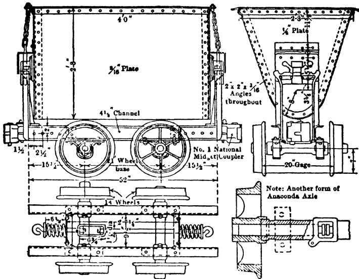
Fig 9. V-body Mine Car, with Anaconda Truck (Copper Queen Mine)
