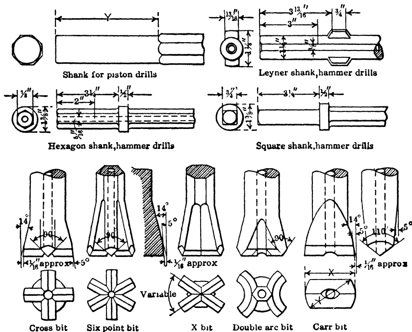
Fig 1. Types of Drill Bits and Shanks
