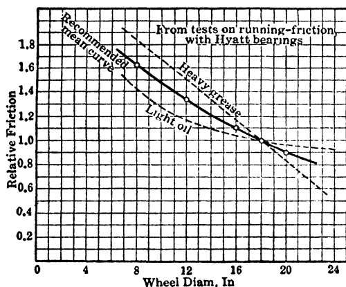
Fig 51a. Relative Friction for Different Wheel Diam, Compared with 18-in Diam (6)
