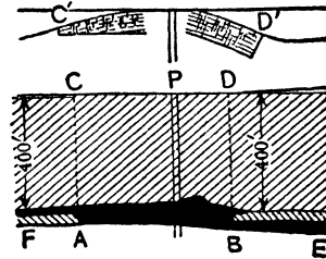
Fig 798. Effect of Shaft Pillar on Surface Subsidence (Fayol)
