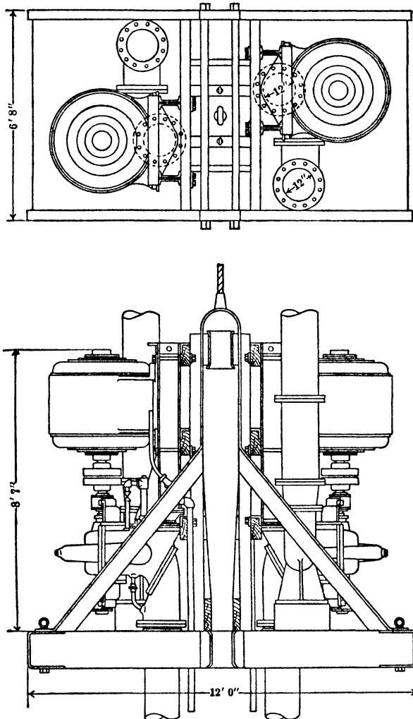
Fig 16. Two 400-hp Hasleton Sinking Pumps, on Cage. (Barrett, Haentjens & Co, Hasleton, Pa)
