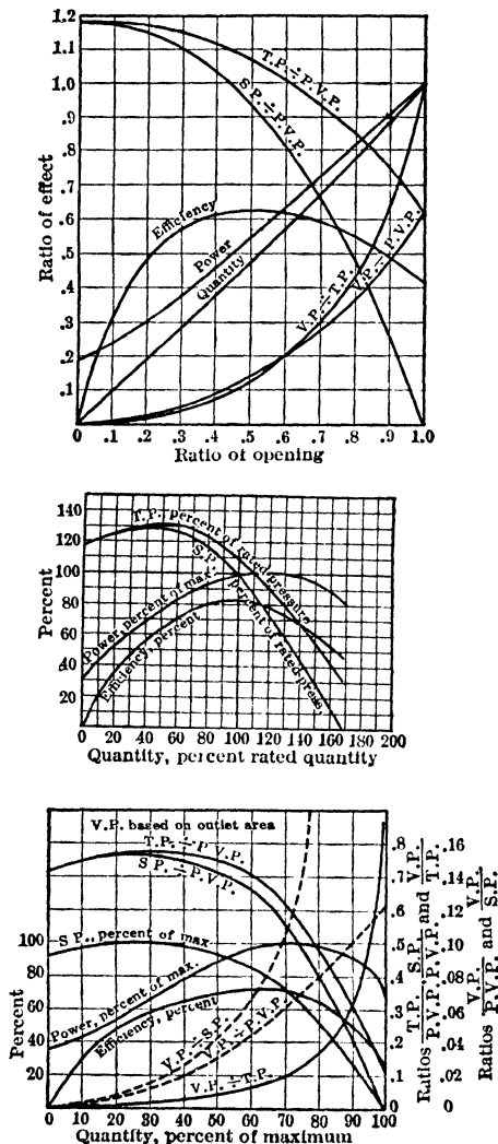
Fig 54. Three Types of Characteristic-ratio Charts
