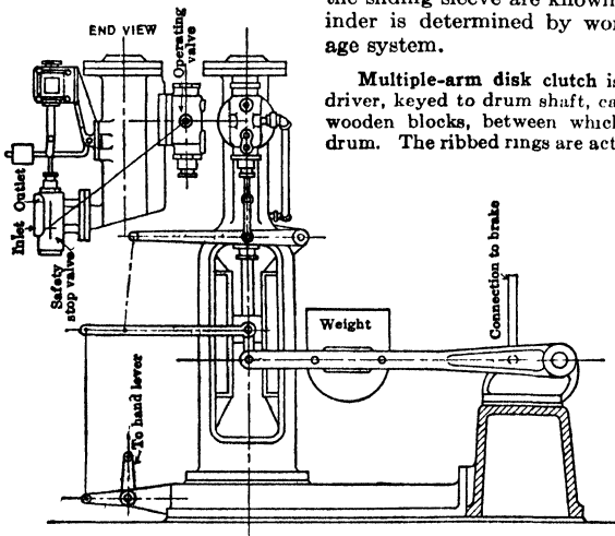
Fig 21. Oil-operated Brake Engine, with Automatic Stop, for Electric Hoist
