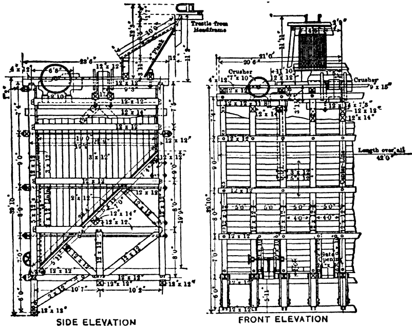
Fig 153. Bin with Grizzly and Crusher
