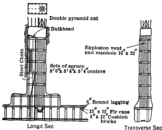
Fig 165. Two-compt Square-set Raise, Lake Shore Mine, Kirkland Lake, Ont
