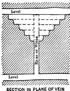
Fig 206. Underhand Stope, Cornish Method
