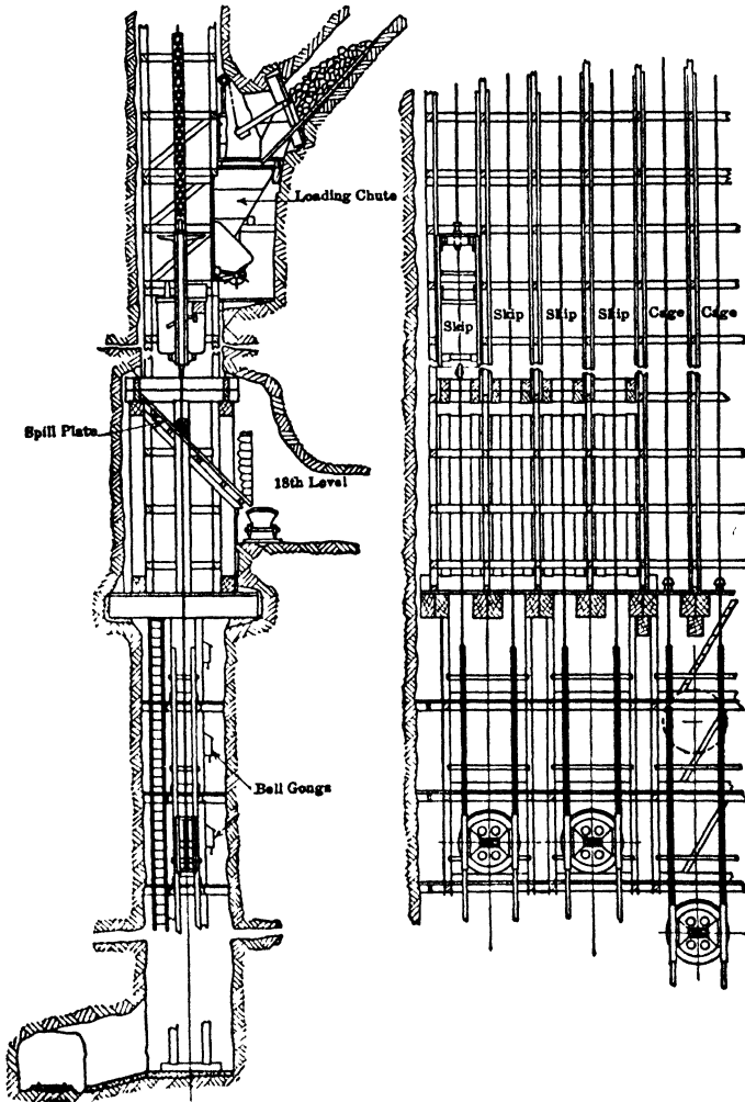
Fig 148. Loading Station, No 3 Shaft, Village Deep Mine, Rand
