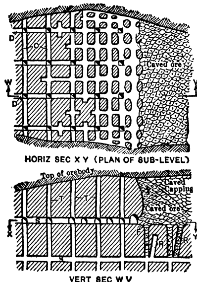
Fig 539. Block-caving, Morenci
