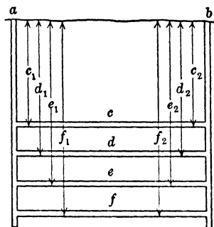
Fig 33. Multi-level Type of Split-flow Circuits
