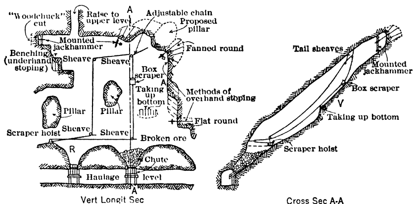
Fig 244 Breaking and Handling Ore in Open Stopes, Edwards Mine, St Lawrence Co, N Y (253)
