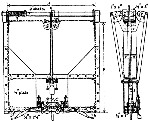
Fig 110 Safety Crosshead for Sinking Buckets (U S Bur Mines, Tech Pap 276)
