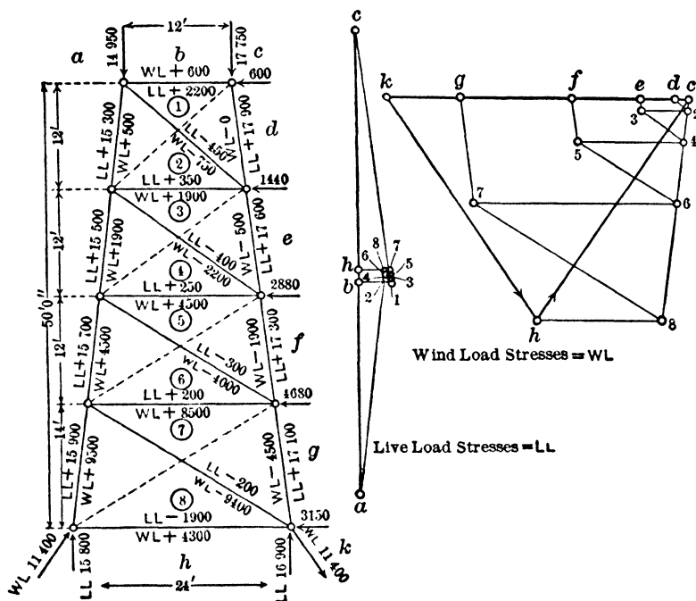
Fig 58 Headframe Stress Sheet, Front Elev
