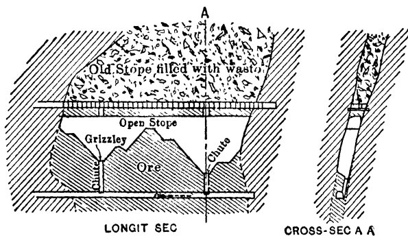
Fig 208. Underhand Stopping, Morenci, Ariz
