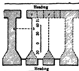
Fig 203. Stope Layout for Scraper Loading
