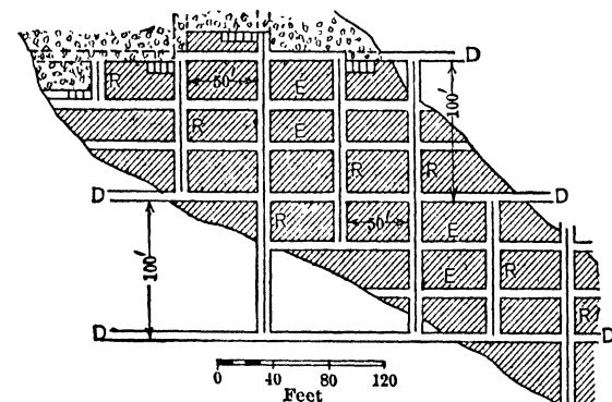
Ideal Longit Sec Projected on Vert Plane Fig 497 Top-slicing in Judge Mine, Park City, Utah
