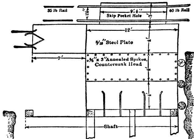
Fig 47. Turnsheets or Tarantulas
