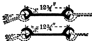
Fig 6. Lackawanna Steel Sheet Pile
