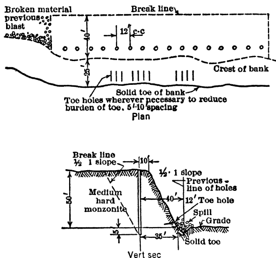
Fig 679 Bench Blasting, New Cornelia Mine, Ajo, Ariz
