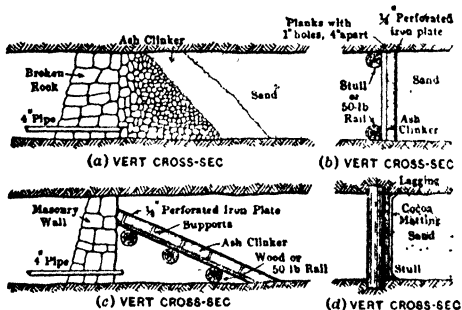
Fig 658. Types of Barricade for Sand Filling on the Rand
