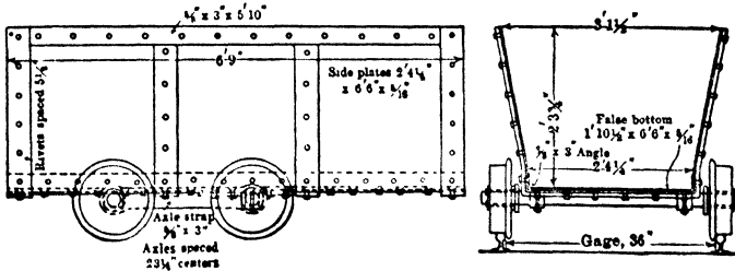
Fig 7. Open-end Dumping Car (Mich Copper District)
