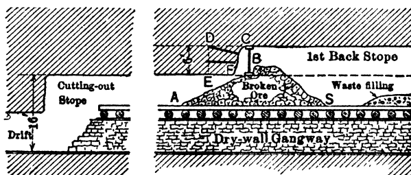
Fig 400. Starting Stopes, Baltic Method; Longit Sec
