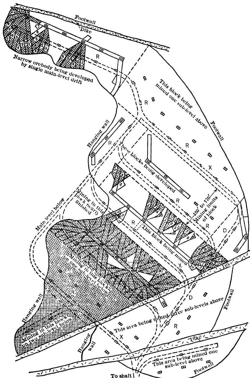
Fig 486. Top-slicing in Negaunee Distr, Marquette Range, Mich. Typical Plan. Small numbers indicate sequence of slices. Hatched areas are caved
