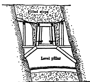
Fig 376. Mining Level-pillars, Waihi Mine
