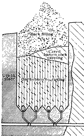
Fig 555. Use of Back-filling in Block-caving, King Mine, Quebec
