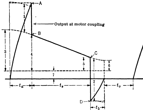
Fig 40a Load Diagram for Cylindrical Drums and Balanced Hoisting Horiz broken line at A shows aver motor torque required during acceleration and retardation (Gen Elec Co)
