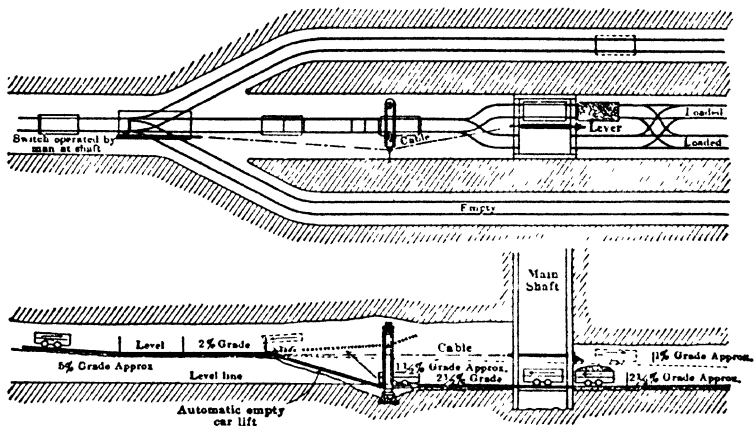
Fig 48. Shaft Bottom Layout, Pa and Ill
