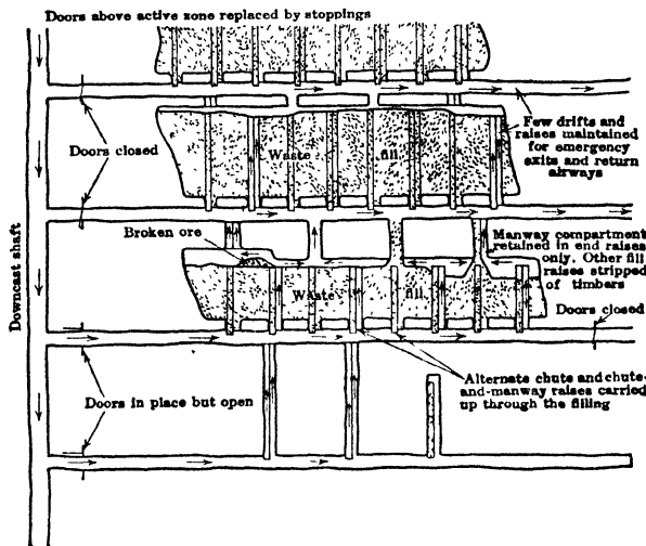
Fig 13. Method of Ventilating Horiz Cut-and-fill Stopes (9)
