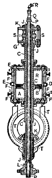
Fig 47. Hydraulic Feed
