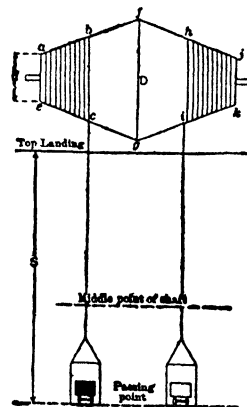
Fig 11. Passing Point of Cages
