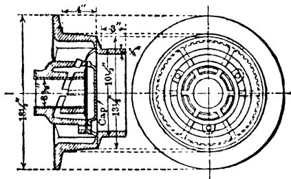
Fig 125. Rear Wheel, Mineville Skip
