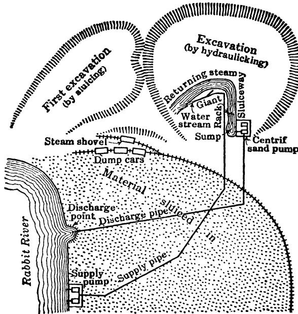
Fig 7. Layout for Hydraulic Stripping (35)
