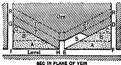
Fig 428. Rill Stope in Weak Ore, Calamon Mine, Spain
