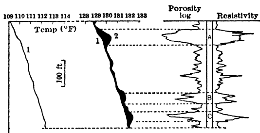
Fig 65. Study of Formations through Casing and "Old" Cement (30)
