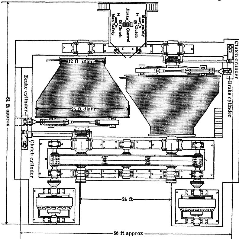
Fig 9 Motor-driven Double-drum Geared Hoist (Gen Elec Co)
