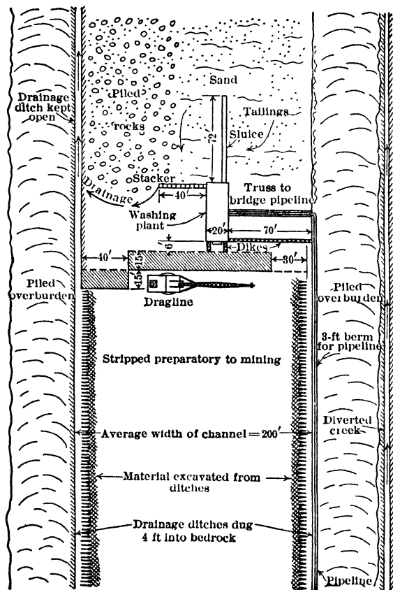
Fig 813. Dragline and Movable Washer, Atlantic City, Wyo (118)
