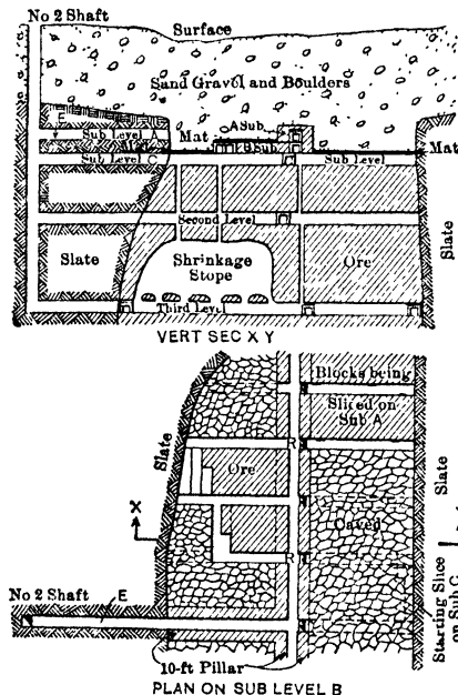
Fig 485. Top-slicing, Caspian Mine, Mich
