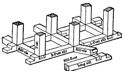
Fig 338. Sill-floor Timbering
