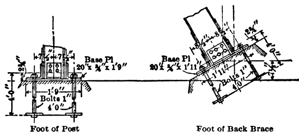
Fig 79 Anchorage for Headframe
