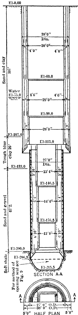
Fig 9 Drop-shaft in Two Sections St Albert Colliery, Canada
