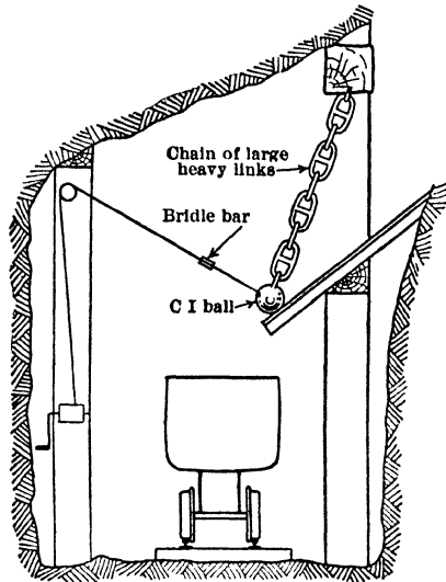
Fig 642. Cramp Chain Gate
