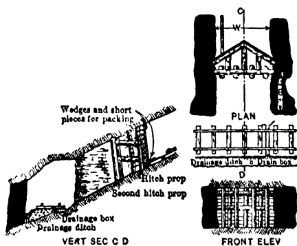
Fig 783 Bulkhead for Dips of 25° or More
