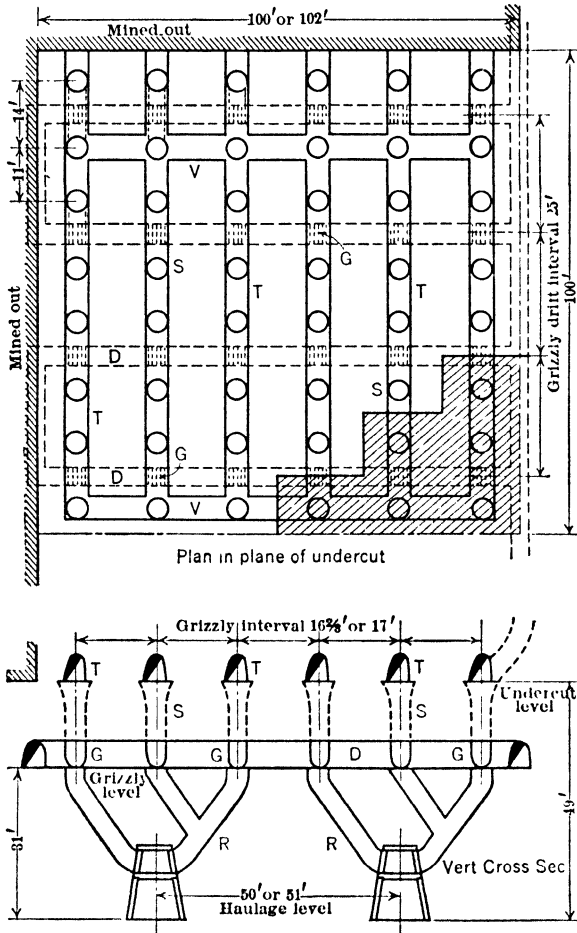
Fig 550. Block Caving, Inspiration Mine, Ariz. Min haulage-drift spacing for lowest ore horizon
