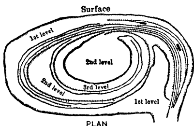
Fig 667. Spiral Track Layout, Mesabi Range
