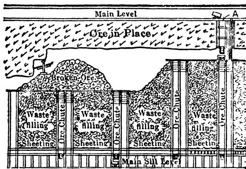
Fig 383. Back-filling at Butte, Mont
