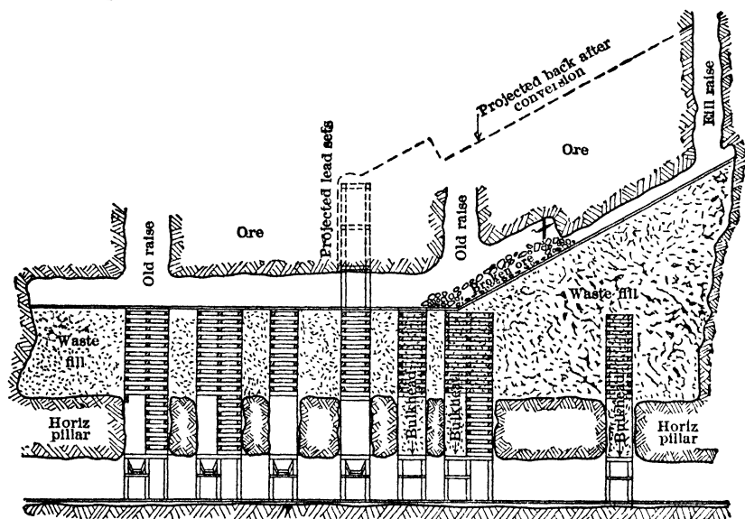
Fig 427. Typical Sec showing Conversion from Horiz to Inclined Cut-and-fill, United Verde Mine, Jerome, Ariz
