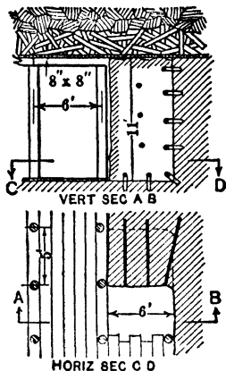
Fig 490. Breaking Ground in Slices, Detroit Copper Co, Morenci, Ariz
