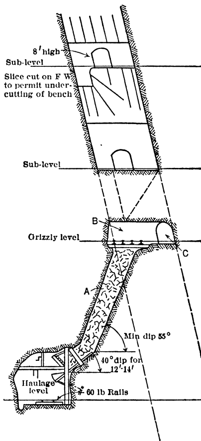
Fig 269a. Typical Sec through Chute Raise A-A of Fig 269
