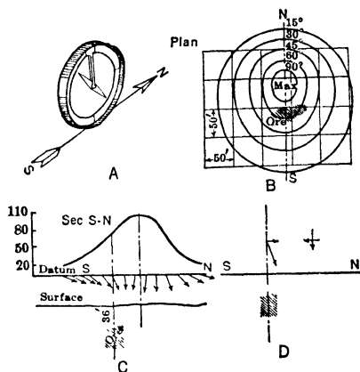
Fig 11. Dip Needle parallel with Magnetic Meridian (6)
