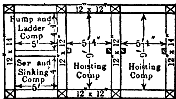
Fig 4. Shaft with Service or Sinking Compartment
