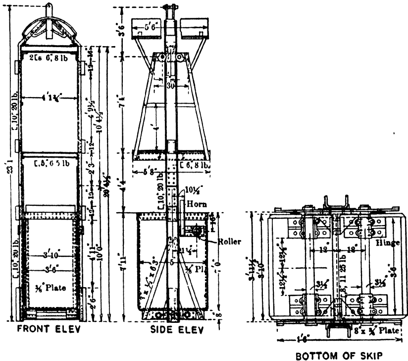
Fig 132 Combined skip and Cage
