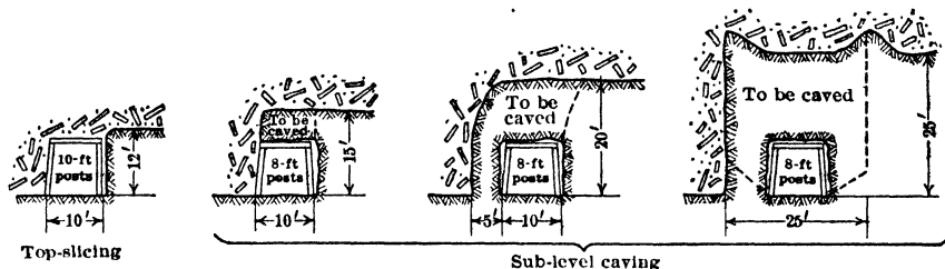
Fig 505. Diagrammatic Vert Cross-secs through Slice-drifts, comparing Top-slicing with Various Methods of Sub-level Caving
