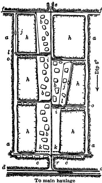
Fig 196. "Scatter-pile" Stope, Modder B Mine. a , Stope faces. b , Waste packs. c , Safety pillars. d , Haulage level. e , Winch. f , Drift. h , Piles of broken ore. i , Transportable scraper hoists. j , Scrapers. k , Brattice. l , Loading chutes. r , Raise entry to stope.
