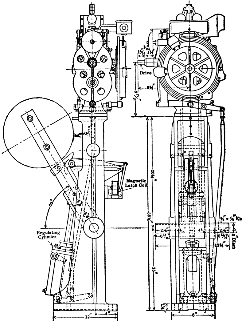
Fig 140 Lilly Controller for Small Electric Hoists
