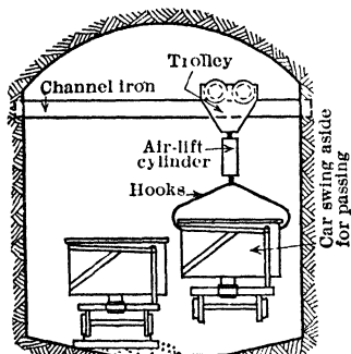
Fig 15. "Cherry Picker"
