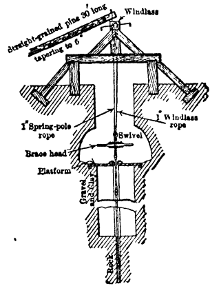
Fig 6. Spring-pole Rig Operated in Pit
