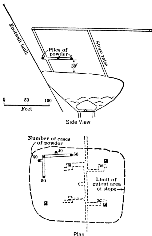
Fig 465. Typical "Powder Drift" Shot, Alaska Juneau Mine
