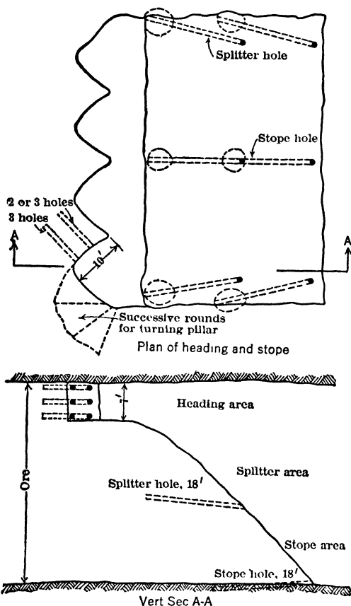
Fig 183. Stope and Heading Rounds, Breast Stopping, Tri-State Distr
