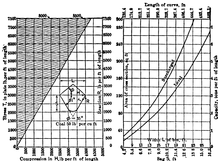
Fig 162. Diagram for Suspension Bunkers (R. W. Dull)
