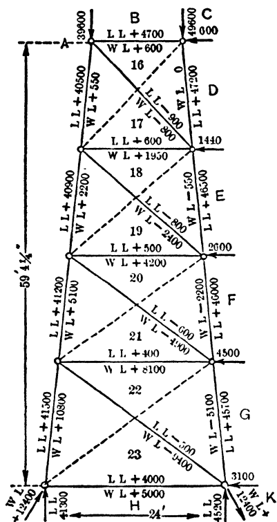
Fig 57. Headframe Stress Sheet, Projection on Plane of Back Stay
