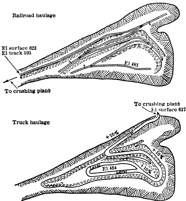
Fig 669. Two Haulage Systems, Louise Pit, Cuyuna Range
