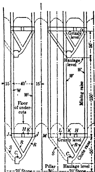
Fig 459. Beatson Mine, Alaska. (Vert sec XX, Fig 457)
