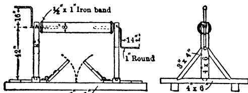
Fig 51. Hand Windlass
