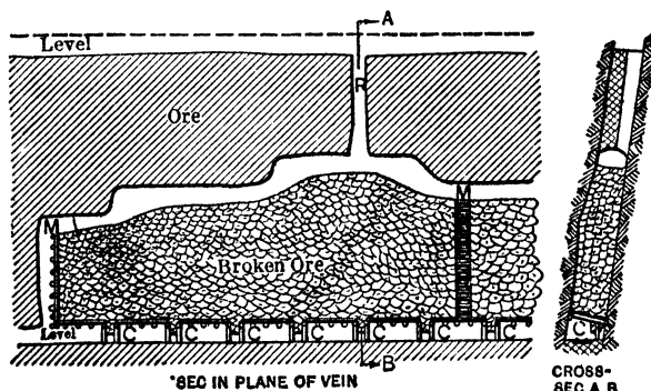
Fig 429. Shrinkage Stope, Narrow Vein
