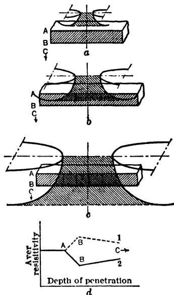
Fig 28 Effect of Increasing Depths on Resistivity Curves (11)
