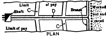
Fig 859. Layout of a Drift Mine in a Narrow Paystreak
