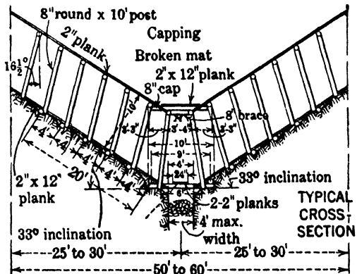
Fig 504. Humboldt Mine, Cross-section through Wings of Stope
