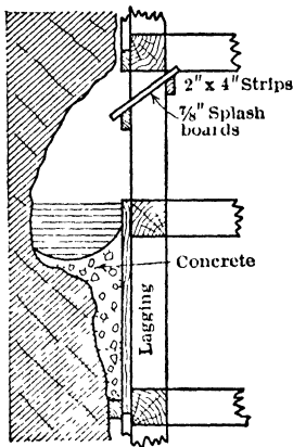
Fig 15 Water Ring for Timbered Shaft
