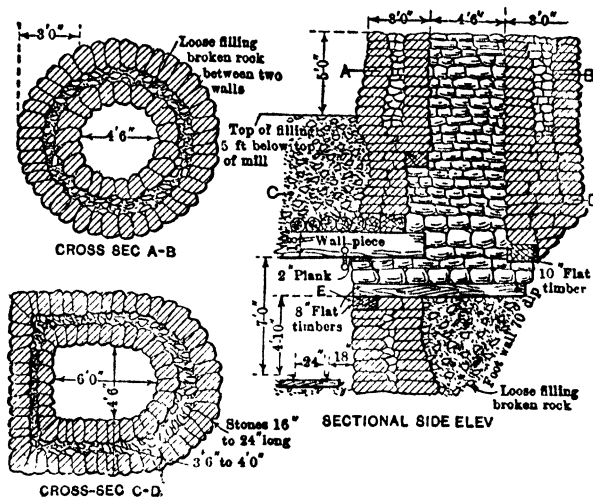
Fig 399. Dry-wall Mill Hole. After C. T. Rice (141)
