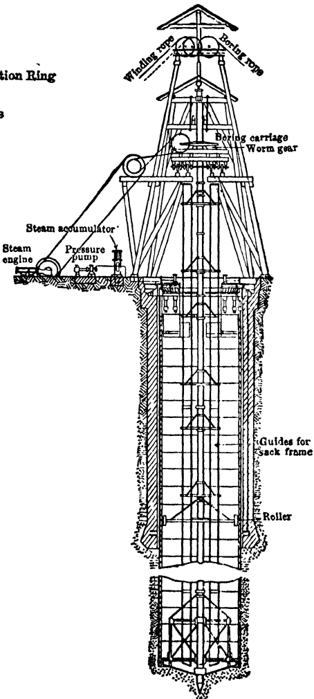
Fig 18. Sack Borer Adolf Shaft, Eschweiler Mining Co, Germany (Riemer)
