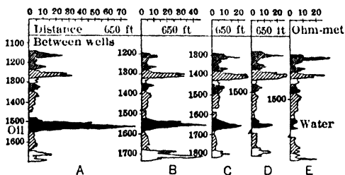
Fig 46. Transition from Oil- into Water-sand, Venezuela (20)
