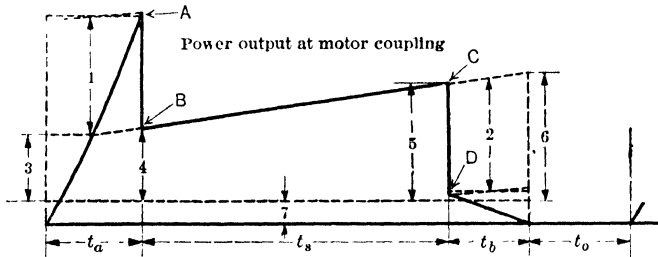
Fig 43. Power Diagram for Conical Drums and Reels; Balanced Operation plotted to Tim
