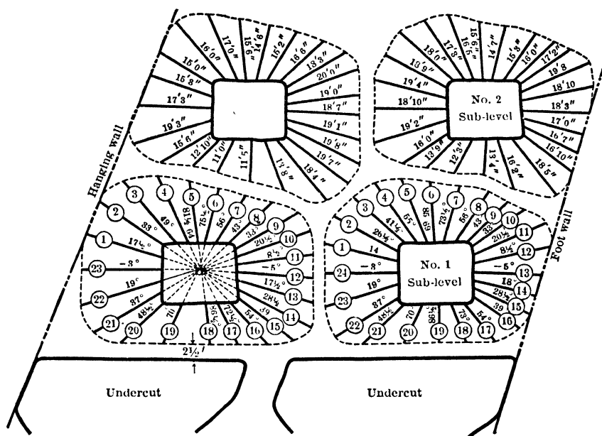
Fig 282. Ring-drilling Diagram for Longit Sub-level Stope, Mt Isa Mines, Queensland
