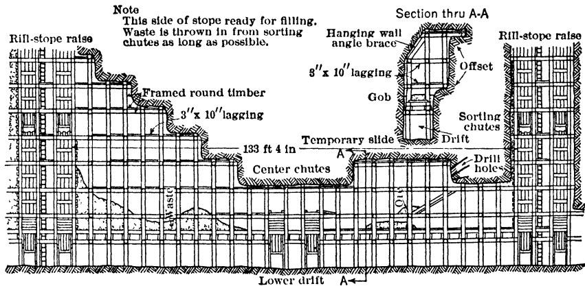
Fig 297. Preliminary Development of a Timbered Rill Stope
