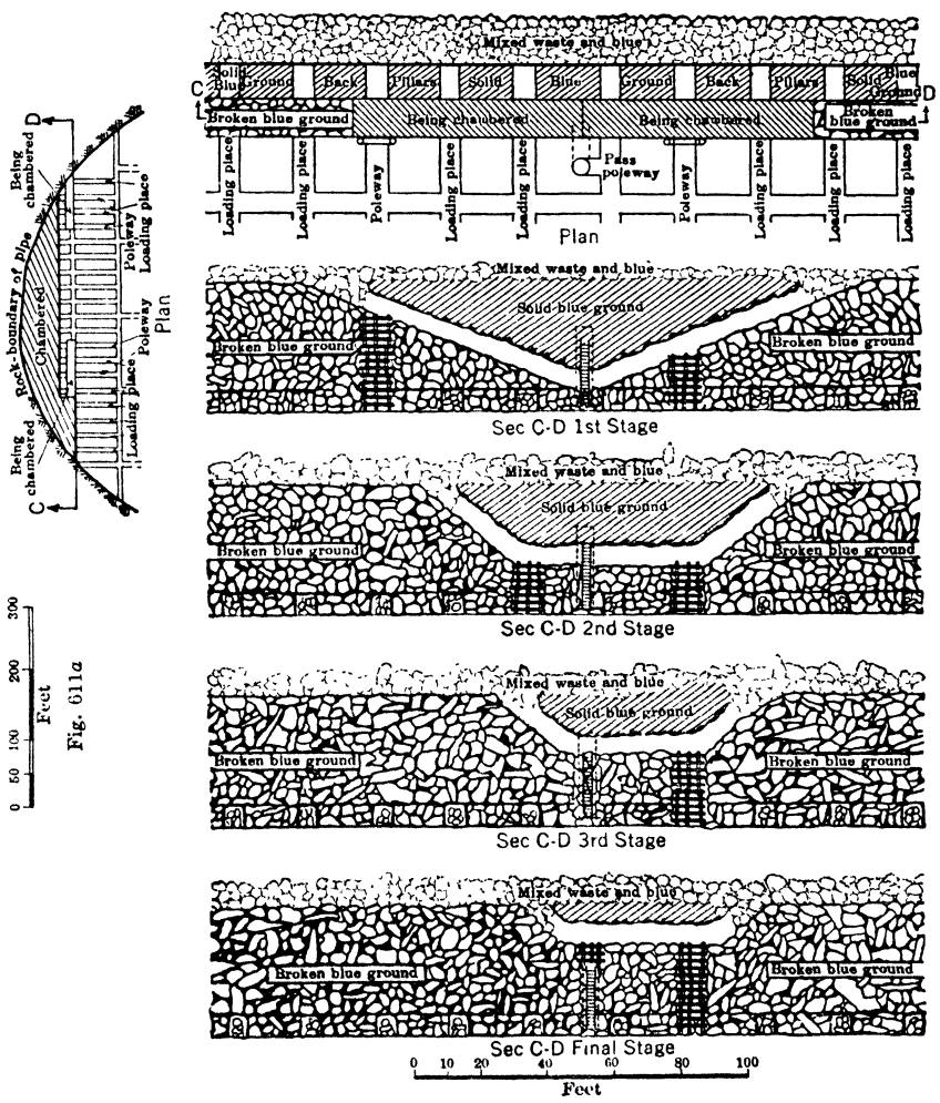
Fig 612. Method of Completing Chamber, De Beers Diamond Mine, Kimberley, So Africa
