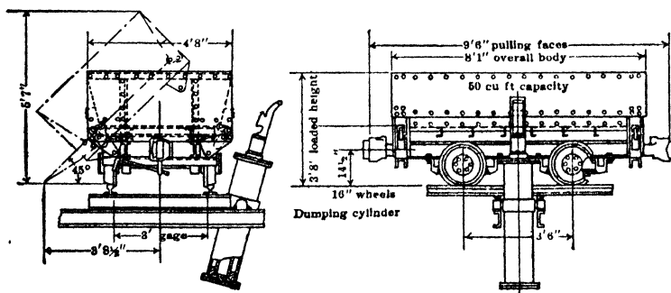
Fig 17b. Single-truck Car, Marting Ore Co, Caspian, Mich
