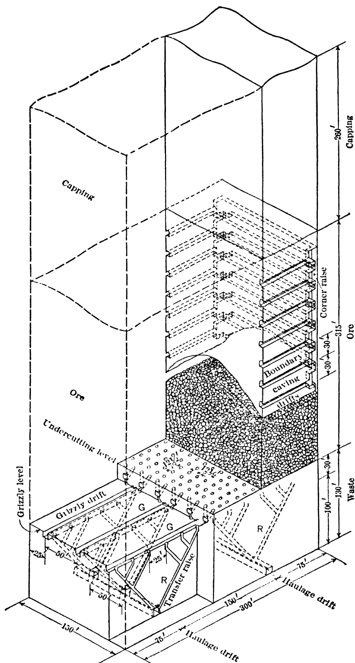
Fig 545. Isometric Drawing of Stope 150 by 300 Ft, Miami Copper Co
