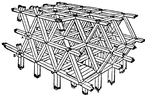
Fig 363. Moore System at Tonopah Belmont Mine
