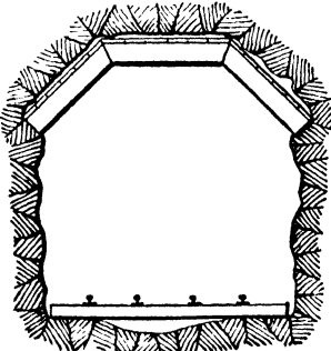
Fig 20 Arch Set without Posts
