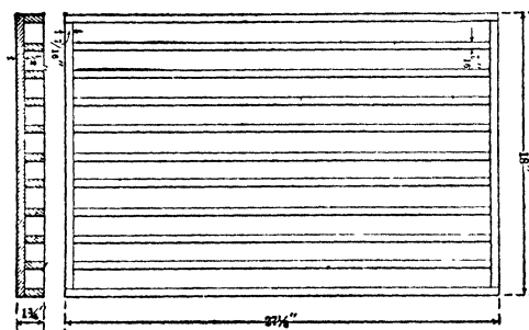
Fig 78. Wooden Core Box
