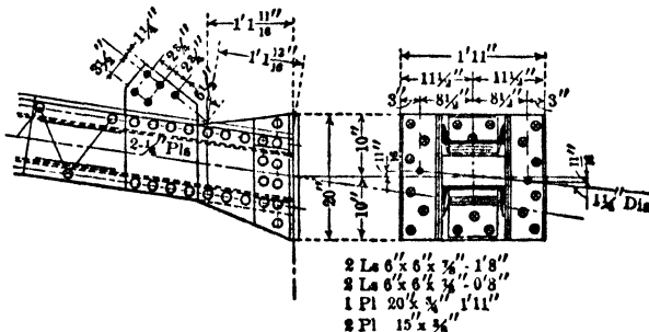
Fig 78. Base of Headframe Post
