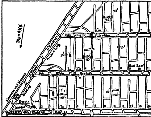
Fig 717. Systematic Mining, Georges Creek, Md
