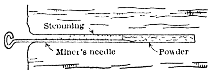
Fig 18. Miner's Needle, for Squib
