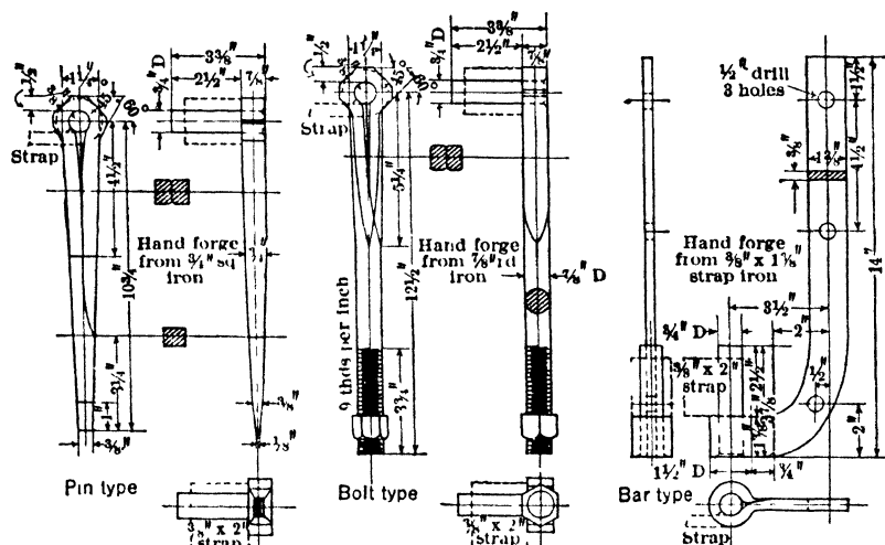
Fig 4 Door Hooks, or Studs, of Strap-type Hinges (27)
