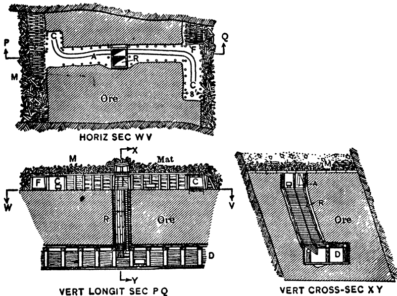
Fig 467. Top-slicing, Lake Angeline Mine, Mich
