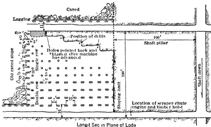
Fig 241 Open Stope, Conglomerate Lode, Calumet, Mich (489)
