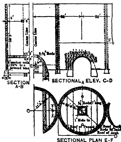
Fig 157 Reinforced Concrete Bins, Croton Iron Mines (88)
