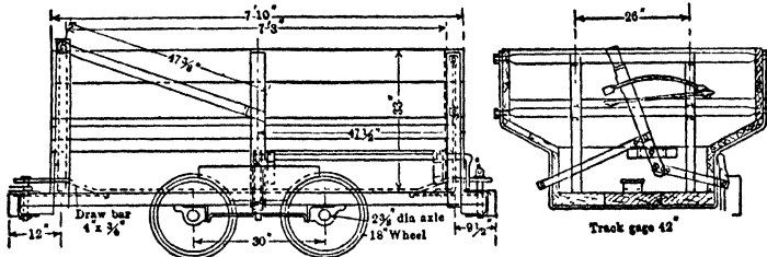
Fig 2. Hockensmith Standard Wooden Car
