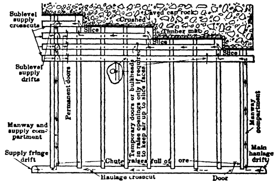
Fig 15. Hurdling Method of Ventilating Top-slice Stopes (9)
