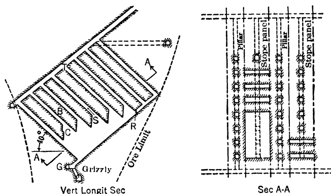
Fig 272. Diagrammatic Sketch showing Modified Form of Sub-level Stopping, Horne Mine, Noranda, Quebec
