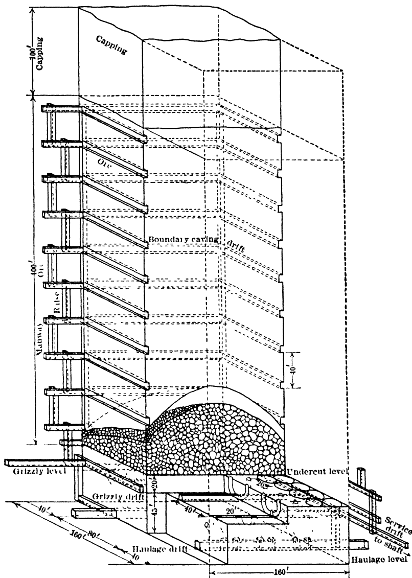
Fig 556 Isometric Drawing of Stope Block, King Mine, Quebec
