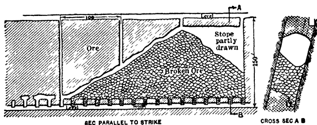
Fig 444 Shrinkage Stopping, Morris Lloyd Mine, Marquette Range, Mich
