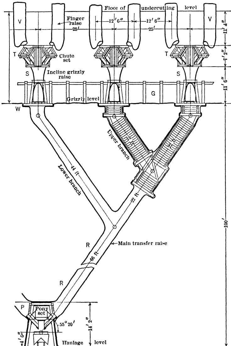
Fig 546. Vert Projection of Ore-transfer Raise System, Miami Copper Co (283)
