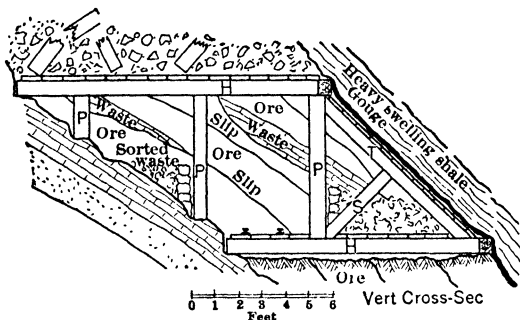
Fig 496. Top-slice Stope, Judge Mine, Park City, Utah (Looking at face of stope)
