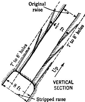
Fig 148 Enlarging a Raise by Stripping from Bottom
