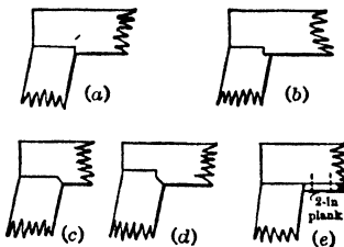
Fig 143. Joints between Cap and Post
