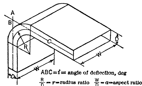
Fig 22. Bend Characteristics
