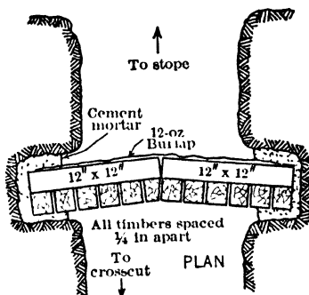
Bulkhead at Bottom of Shrinkage Stope Fig 662a. Details of Sand Filling, Home-stake Mine
