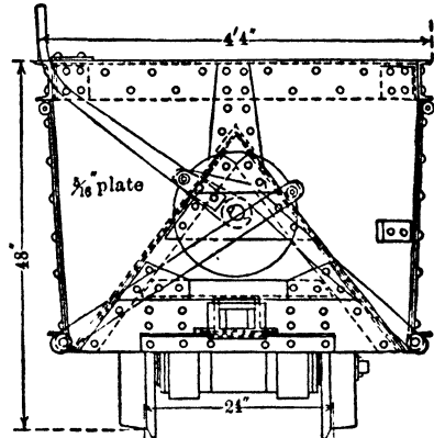
Fig 14. Saddle-back Car, Rear Elev (Miami Mine, Ariz)
