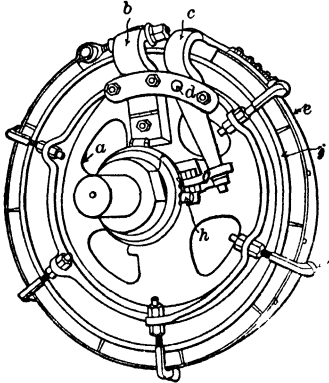
Fig 19. Lane Band Friction Clutch
