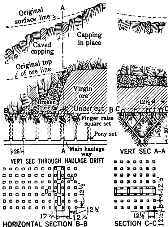
Fig 552. Block-caving, Ruth Mine, Ely, Nev (diagrammatic)
