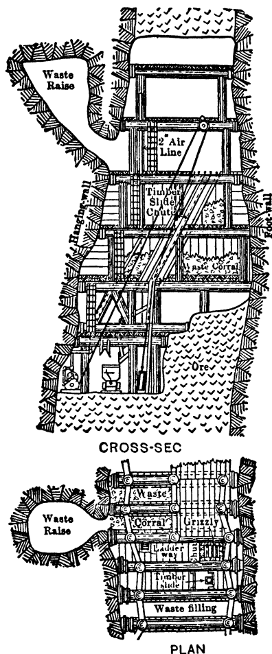
Fig 367. Stope Timbering, Morning Mine, Idaho
