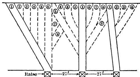
Fig 472. Radial Slicing, Mesabi Range, showing Variations in Plan
