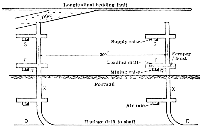
Fig 520 Montreal Mine, Generalized Plan of Haulage Level
