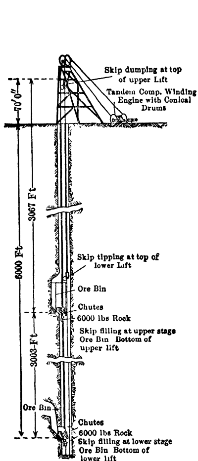
Fig 5 Hoisting in Tandem
