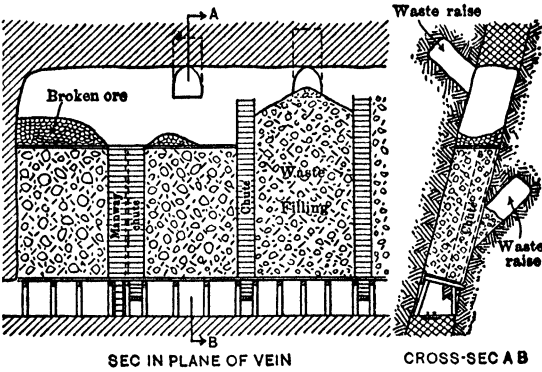
Fig 379. Filled Flat-back Stope, Nevada Wonder Mine
