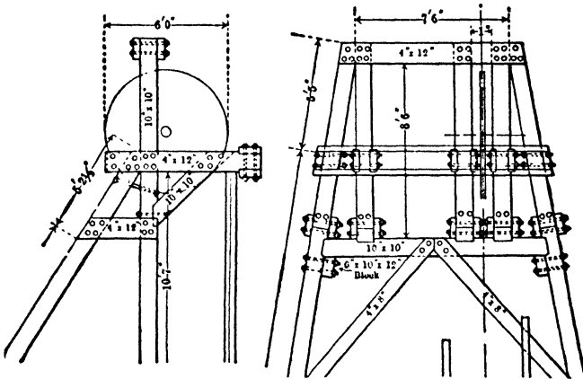
Fig 67. Two-post Headframe
