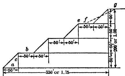
Fig 698 Ideal Layout of Power-shovel Benches, Nevada Consol Copper Co
