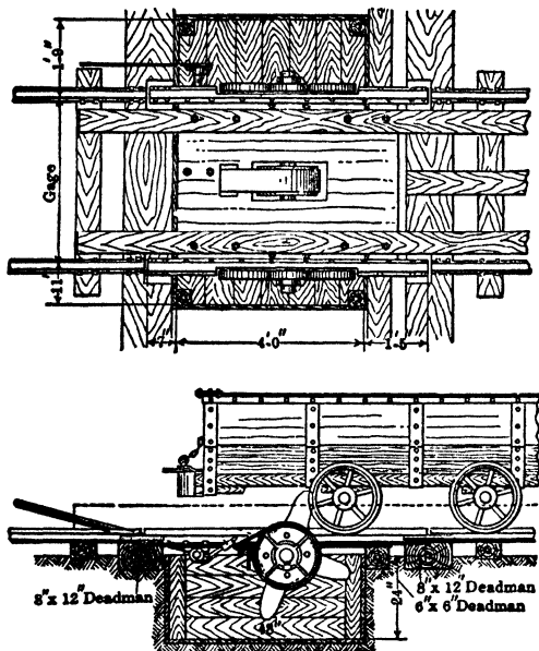
Fig 52a. Car Spragger
