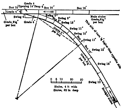
Fig 827. Turn-in Sluice at Head of Tunnel, Delaney Claim, Patrickville, Cal (after Bowie)
