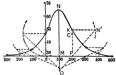
Fig 18. Approximation of Depth of Dike from Vert Magnetic Profile (8)
