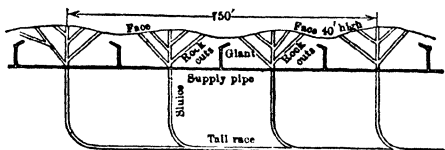
Fig 815. Layout for Hydraulicking Bench Gravel, Klondike (after Purington)
