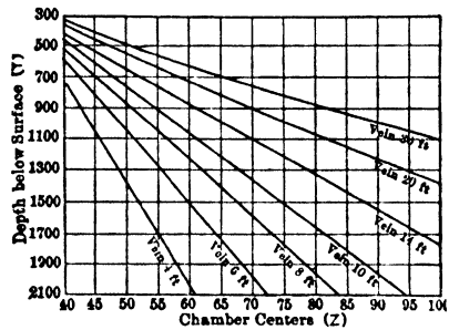
Fig 705a. Relation between Depths and Room Centers for Different Thicknesses of Seam for 24-ft Rooms
