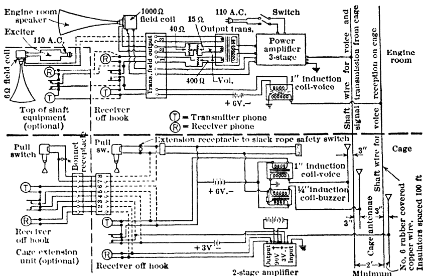
Fig 99. Wiring Diagram of Radio Cage-signalling System, Oglebay, Norton & Co. Ironwood, Mich (37, 61)
