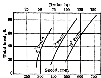
Fig 845. Recommended Speeds and Powers for Gravel Pumps under varying Heads, Nigerian Tin Fields
