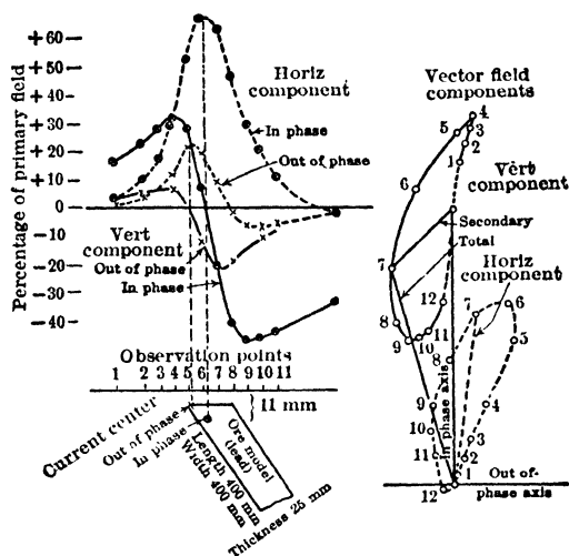
Fig 38. Electromagnetic Secondary Field Components over Ore Model (14)
