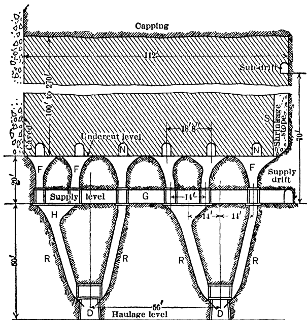
Fig 542. Block-caving into Branched Chutes, Morenci, Ariz (vert sec)
