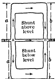
Fig 32. Shunt Type of Split-flow Circuits
