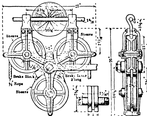
Fig 650 "Go-devil" Sheaves
