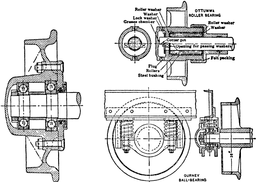
Fig 19b SKF Ball-bearing
