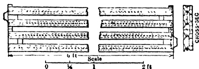
Fig 832. Longitudinal 'Rail Riffles (after Purington)
