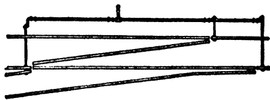
Fig 39. Stub Switch Without Frog
