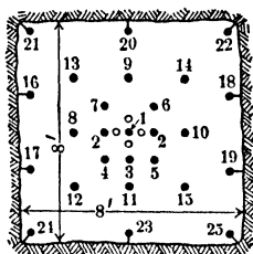
Fig 134 Burned Cut in Tough Limestone, Balmat Mine, Balmat, N Y. Holes average 6.5 ft deep
