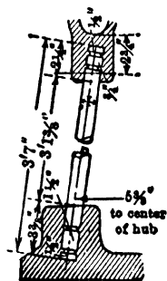
Fig 23 Wrought-iron Spoke Sheave Hub and Rim Ends of Spoke
