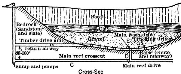
Fig 866. General Scheme of Development, Victoria Deep Leads
