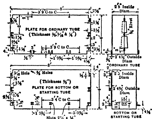
Fig 626. Cylindrical Steel Chute
