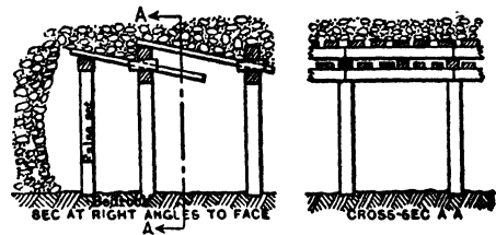
Fig 858. Breast Timbering, Hidden Treasure Mine
