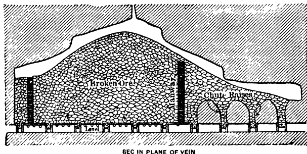
Fig 430. Shrinkage Stope, Lake View Consols Mine, Kalgoorlie, Australia
