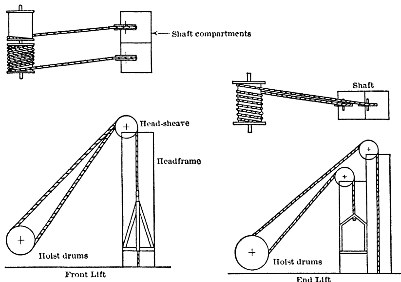
Fig 13. Diagram of Two Arrangements of Hoist with Reference to Headframe
