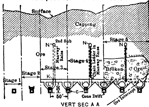
Fig 570 Ray Motor-haulage System (showing 5 stages of work)
