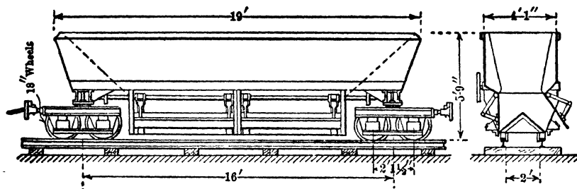
Fig 17. Double-truck Car (Crown Mines, Transvaal)
