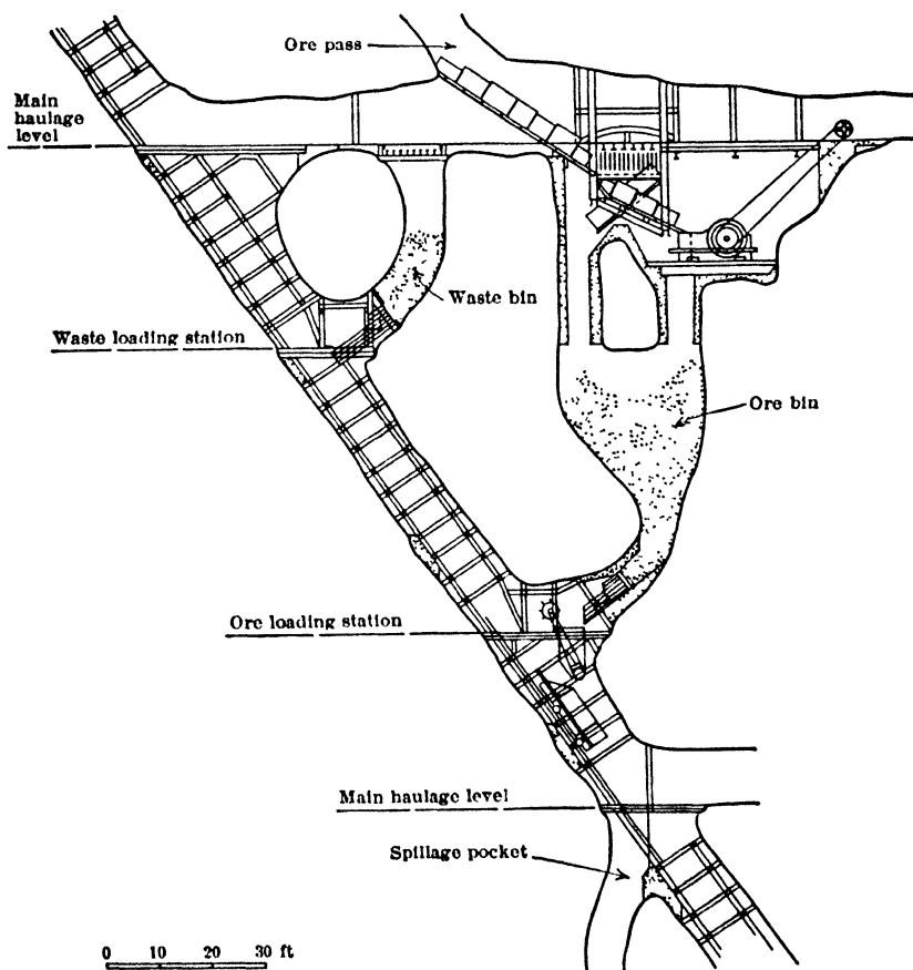
Fig 143. Loading 9-ton Skips, No 3 Shaft, Creighton Mine, Int Nickel Co, Canada (37, 68)
