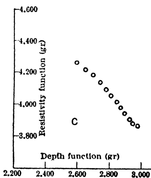
Fig 32. Resistivity Curve Plotted from Conversion Table (13)
