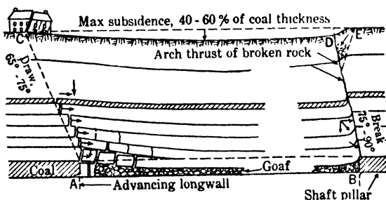
Fig 795 Suggested Mechanics of Longwall Subsidence
