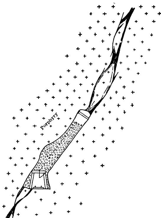
Fig 386. Vert Cross-sec through Typical Stope, Molybdenum Corp of America, Questa, N M
