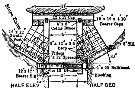
Fig 582. Miami Method, Chute-sets on Drawing-off Level
