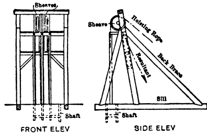
Fig 63. Timber Headframe; Montana Type (Ketchum)
