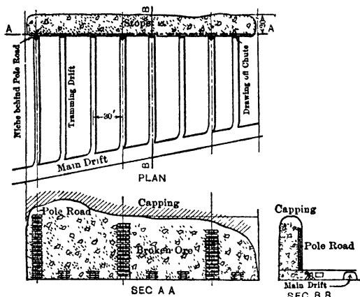
Fig 566. Boston Mine, Hand-tramming System, Chutes at One Side of Stope
