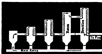
Fig 700. Single-entry System in Flat Seam
