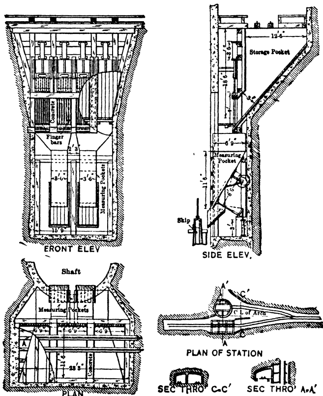
Fig 147. Stations and Storage Pockets, Negaunee No 3 Shaft (83)
