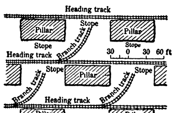
Fig 202. Branch Tracks for Working Wide Stopes
