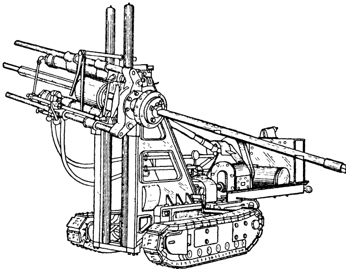
Fig 10. Stripborer Drill
