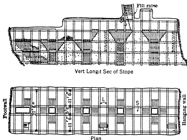
Fig 292. Plan and Sec of Stope, Frood Mine, Sudbury, Ont
