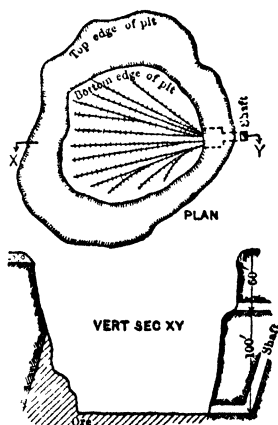
Fig 665. Open-cut, Creighton Mine, Ont
