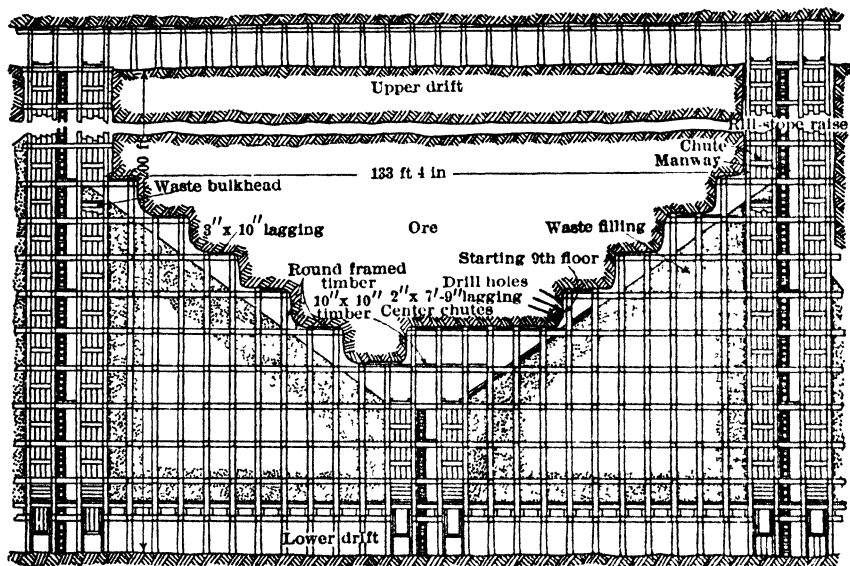
Fig 298. Timbered Rill Stopes after Development, as carried toward Upper Level
