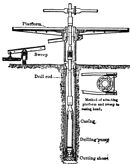
Fig 8. Empire Drill in Operation
