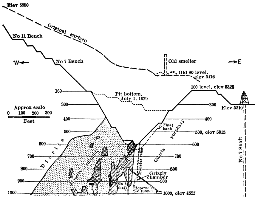
Fig 674. Typical Section of United Verde Pit, Jerome, Ariz, as of Jan 1, 1939 (looking north)
