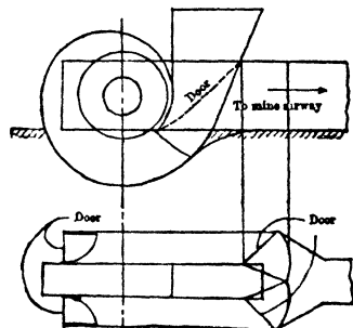
Fig 39. Setting for Reversible Fan
