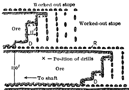
Fig 255 Open Overhand Stopes with Rib Pillars, Kearsarge Lode (Projection on plane of lode dipping 38^\circ )
