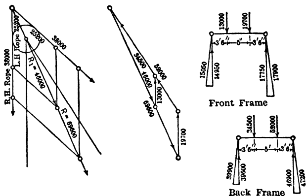
Fig 55. Rope Load Resolution
