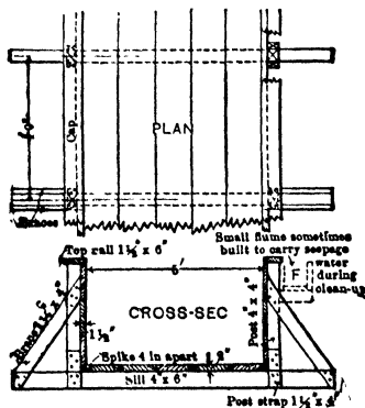
Fig 825. Sluice (riffles and side lining omitted)
