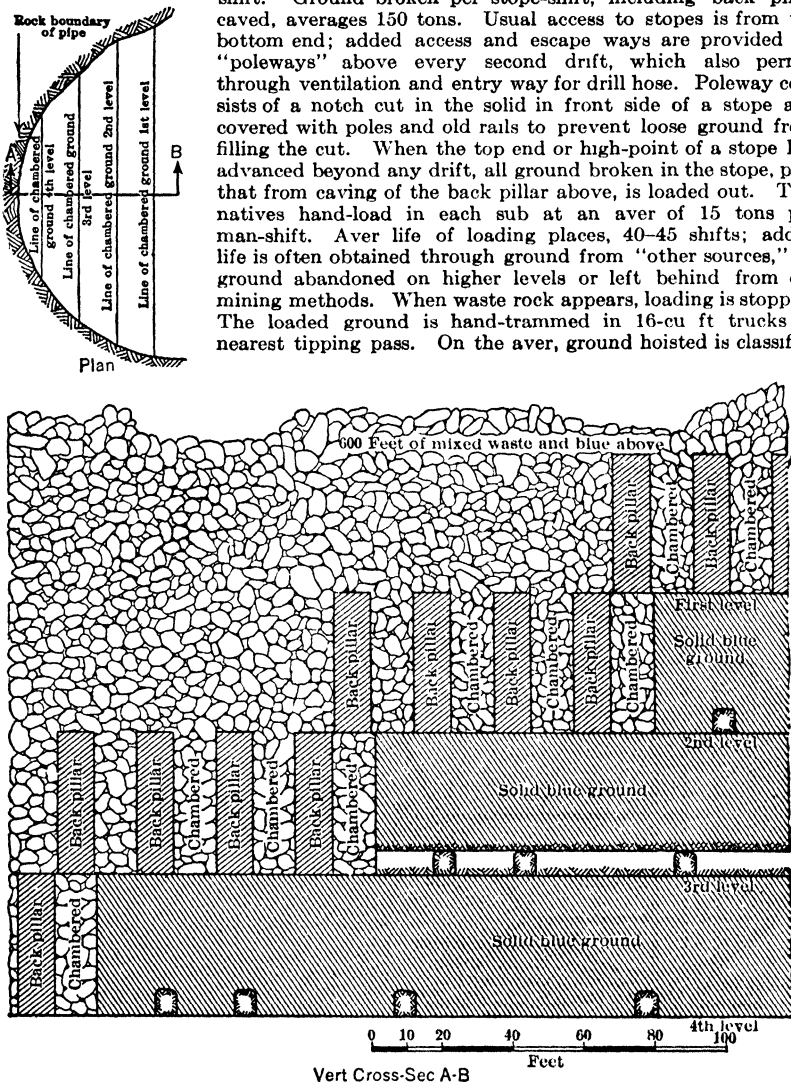
Fig 610. Stopping in De Beers Diamond Mine, Kimberley, So Africa. Showing back pillars left in place, and method of undercutting them from next level below
