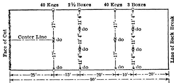
Fig 11. Arrangement of Charges for a Large Blast
