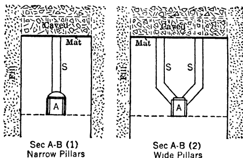
Fig 603. Top-slicing Pillars, N J Zinc Co
