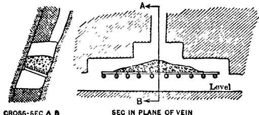
Fig 225. Overhand Stope, Stull Timbering
