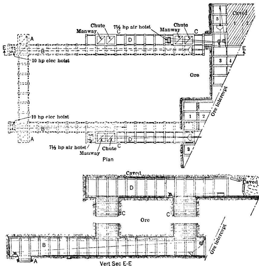
Fig 494. Top-slicing, Bisbee, Ariz
