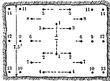
Fig 150. Reinforced Center V-cut in Tough Sulphides Victoria Mine, Britannia Beach, B C
