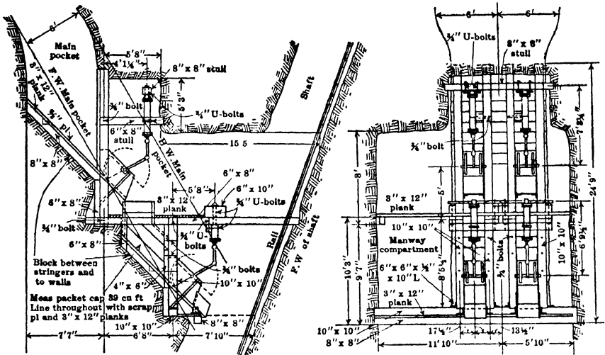
Fig 144. Skip Pocket for Inclined Shaft, Cerro de Pasco Copper Corp, Peru (37, 71)
