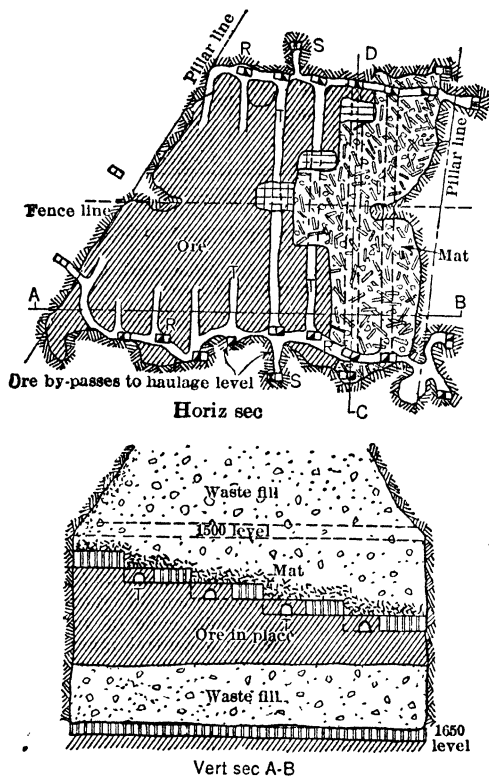
Fig 498. Top-slicing at United Verde Mine, Jerome, Ariz (227)
