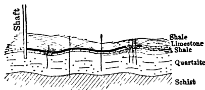
Fig 12 Section on AB (Fig 7), showing Position of Favorable Bed, and Occurrence of Ore in it along Fissures, also Position of Drift beneath Cap Rock
