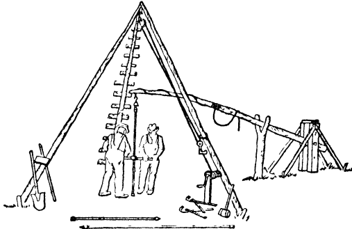
Fig 5. Spring-pole Drill
