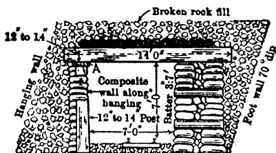
Fig 397. Gangway with One Composite Wall
