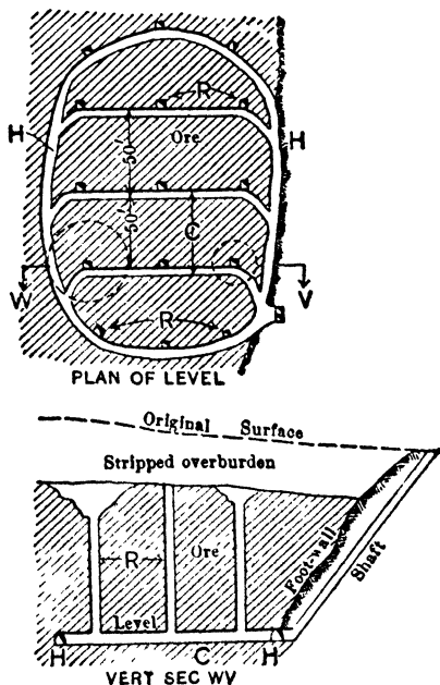
Fig 686. Milling System, Mesabi Range (Diagrammatic)
