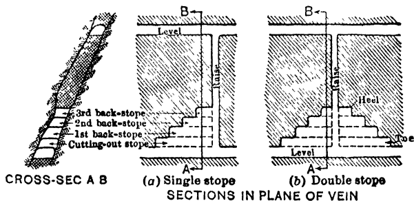
Fig 222 Open Overhand Stopes
