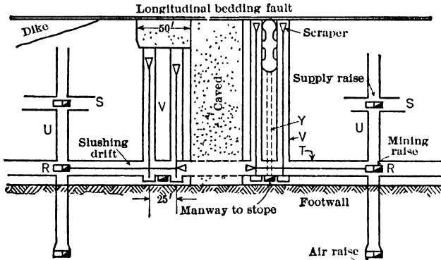
Fig 521. Montreal Mine, Generalized Plan of Sub-level
