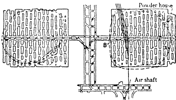
Fig 793. Effects of Subsidence in Panels of a Penna Coal Mine: dotted lines show cracks, 8-10 in wide at A, and 2 smaller ones at B (623)
