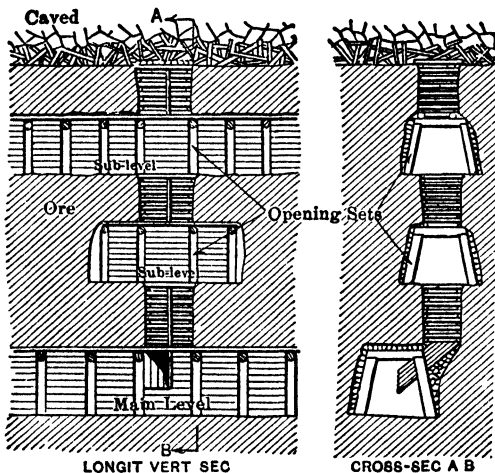
Fig 507. Timbering for Raises, Sub-level Caving
