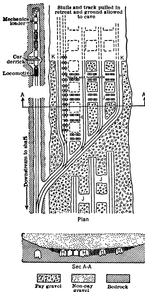
Fig 864. Room-and-pillar Drift Mining, Calaveras Central Mine.
