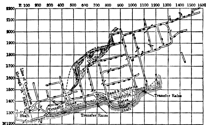
Fig 516 Newport Mine, Plan of 17th Level
