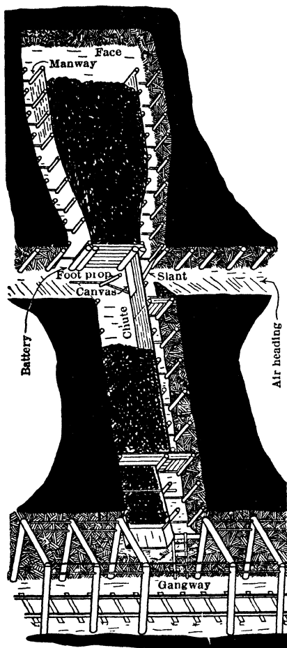
Fig 9. Start of "Full" Breast in Steep-pitch Breast-and-pillar Mining (P & R C & I Co)
