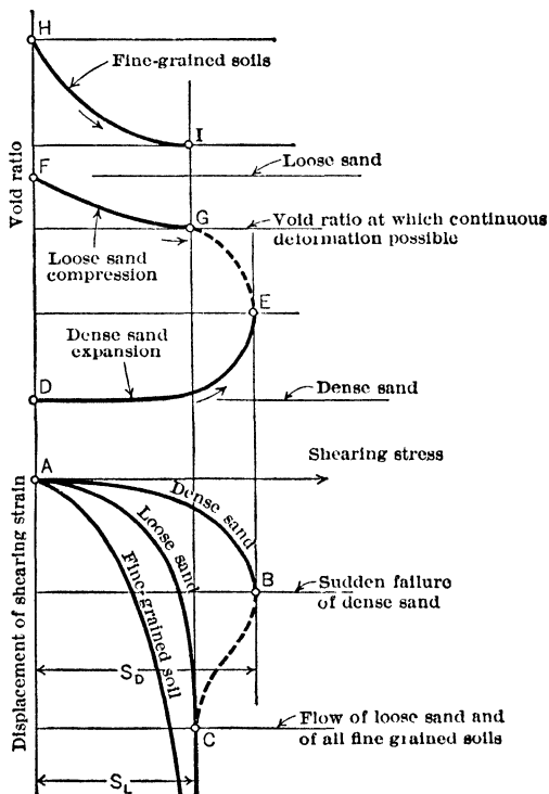
Fig 2. Displacement and Volume Change, as Functions of Shearing Stress of Sands
