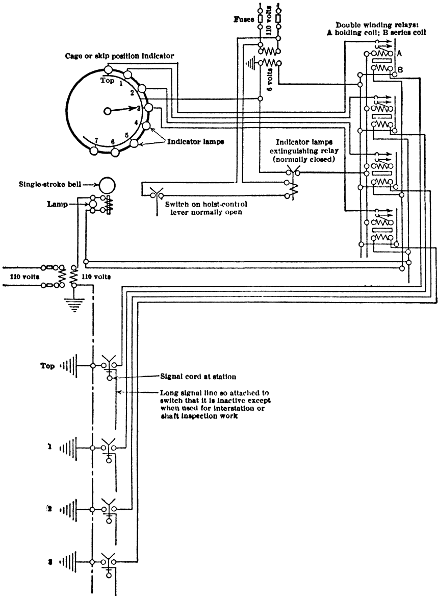
Fig 100. Electric Signalling System, One-compartment Ross Ore Hoist
