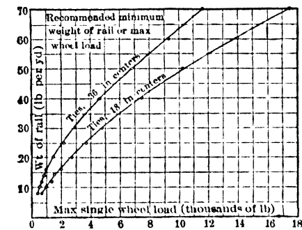
Fig 24. Weight of Rail for 1 1/2 and 3 ft Tie Spacing
