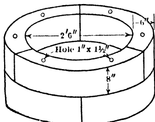
Fig 625. Concrete Chute Wall, Ashanti Goldfields
