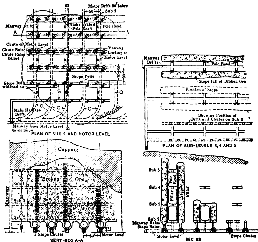
Fig 569. Boston Mine, Motor-haulage System
