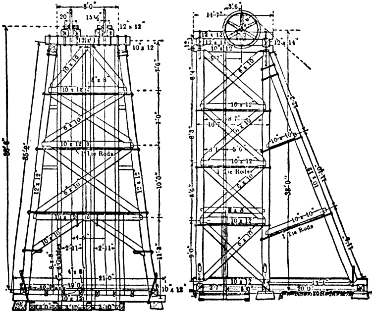
Fig 64. Four-post Frame, with Back Brace
