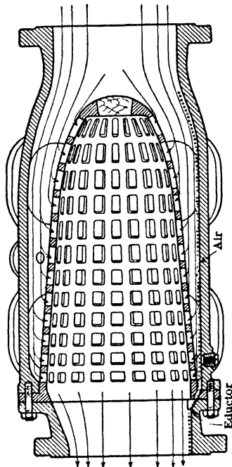
Fig 22. Large-capac Streamlined Strainer
