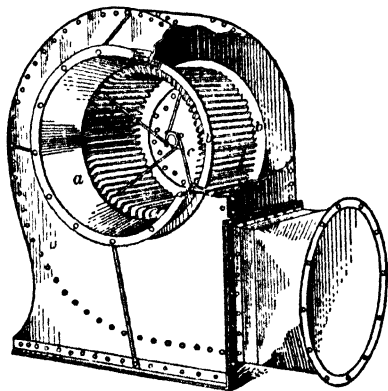
Fig 37. "Troy" Sirocco Fan (6)
