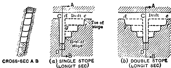
Fig 205. Simple Underhand Stopes
