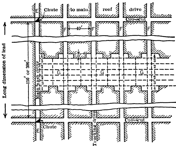
Fig 867. Development and Mining of Victoria Deep Leads by Block System
