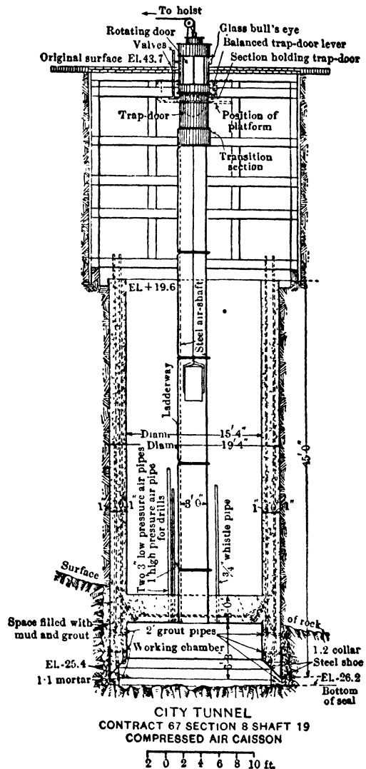
Fig 14. Drop-shaft equipped for Pneumatic Method
