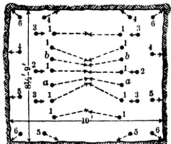
Fig 125 Vert V-cut in Dolomite, Bonne Terre Mine, Bonne Terre, Mo. Holes a, a and b, b, sometimes omitted; 8 side holes are 7.5 ft deep; all others, 9 ft
