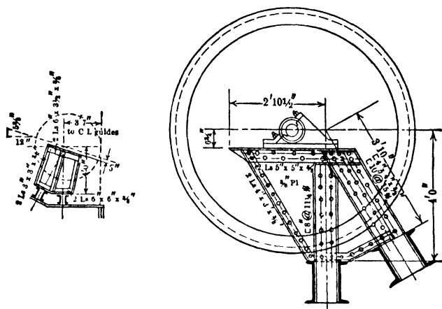
Figures 71 and 72. Sheaves Supported by Diaphragms
