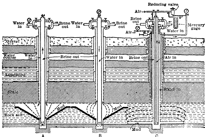
Fig 615. Three Types of Brine Wells. A. N Y Method for thin salt beds. B. Mich method for thick beds. C. Trump system
