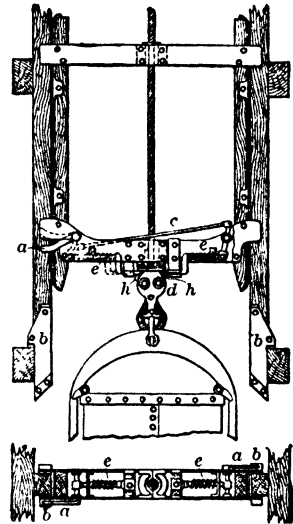
Fig 110a. Berry Safety Crosshead
