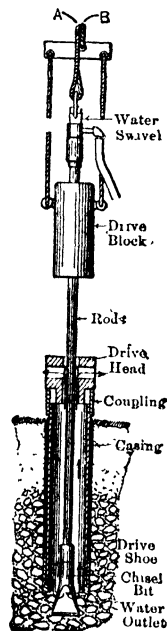
Fig 2. Chopping Bit in Combination with Drive Pipe
