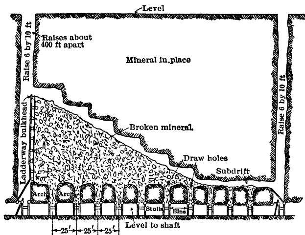
Fig 439. Shrinkage Stope in Wider Veins, Rosiclare, Ill (197)
