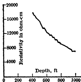
Fig 31. Resistivity Curve as Measured (13)
