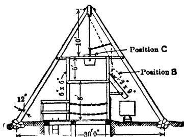
Fig 106. Bucket Dump
