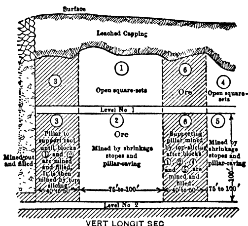
Fig 595. Duluth Mine, Diagram of Sequence of Operations
