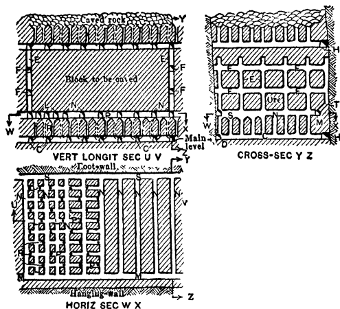
Fig 538. Block-caving into Chutes, Tobin Mine
