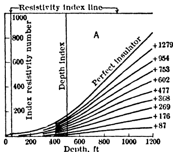
Fig 33. High-resistance Bed (13)
