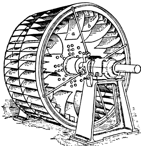
Fig 38. Rotor of Jeffrey Mine Fan (6)
