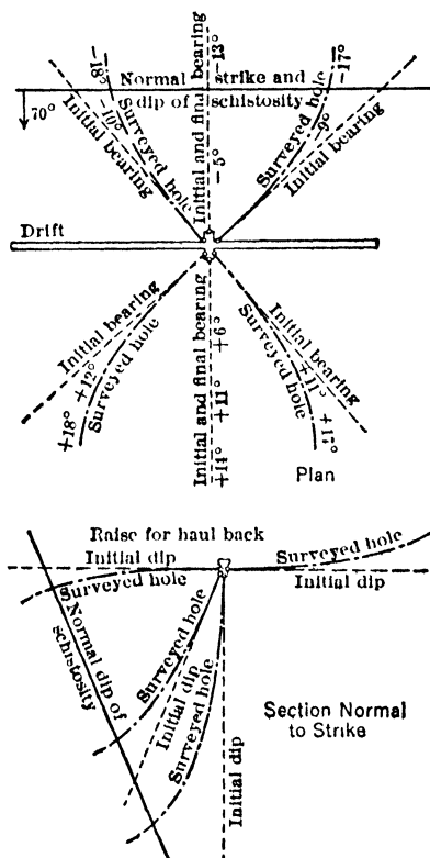
Fig 53. Deflection of Horizontal Diamond-drill Holes in Shear Zone (E & M Jour)
