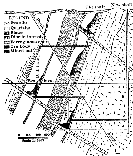
Fig 513. Typical Cross-section of a Gogebic Range Mine, showing Scheme of Development
