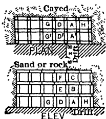
Fig 476. Square-set Slicing, Mesabi
