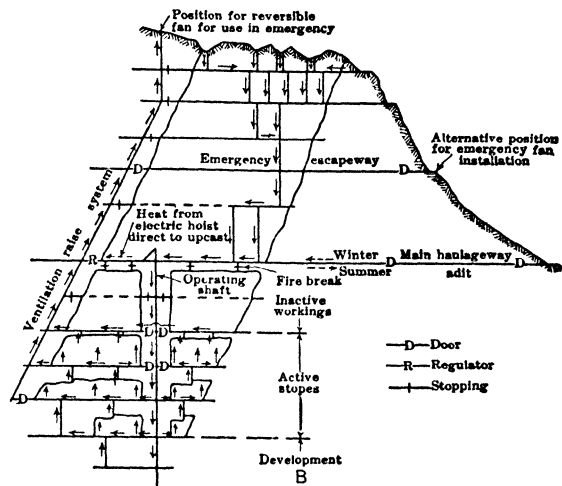
Fig 35. Natural-draft Distribution Controlled to Prevent Seasonal Reversal (9)
