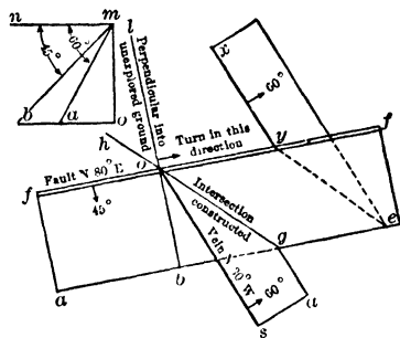
Fig 10 Zimmermann's Solution of a Fault. Construction as in Fig 9, but Vein Dips East, whence Exploratory Drift Turns East
