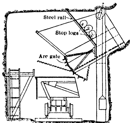
Fig 637. Underswung Arc Gate, Northern Ontario
