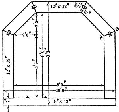
Fig 19. Arch Tunnel Set
