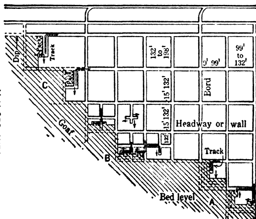
Fig 759. Robbing Pillars, Bord-and-pillar Method (611)
