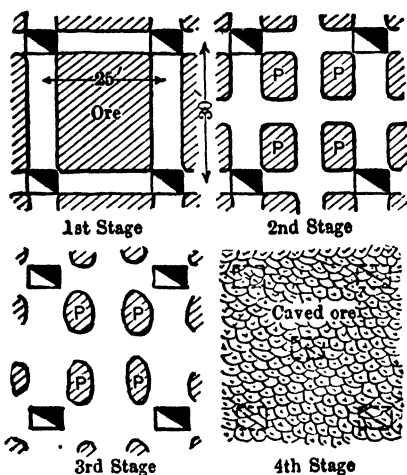
Fig 540. Stages of Work in Undercutting Sub-level Pillars, Morenci
