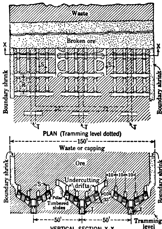
Fig 541. Block-caving, Humboldt Mine, Morenci, Ariz
