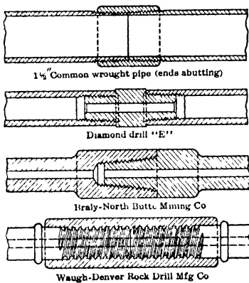
Fig 4 Evolution of Sectional Drill Rods (7)
