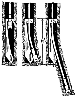
Fig 34. Eastman Removable Whipstock
