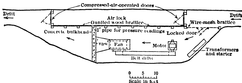
Fig 41 Booster Fan Installation (9)
