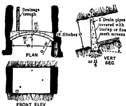
Fig 784 Masonry Bulkhead
