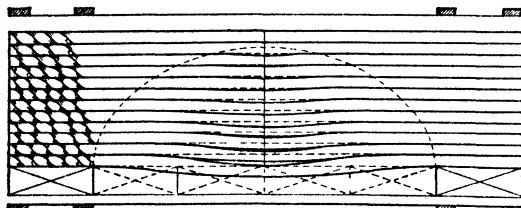
Fig 787. Fayol's Experimental Subsidence of Horiz Strata
