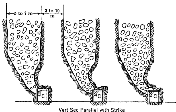
Fig 589. Original Development by Crosscuts, Braden Mine, Sewell, Chile
