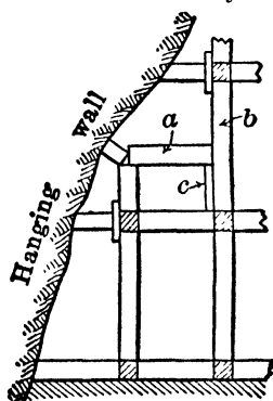
Fig 346. Timbering against Inclined Hanging Wall
