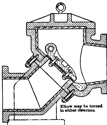
Fig 21. Check Valve, Wood-lined
