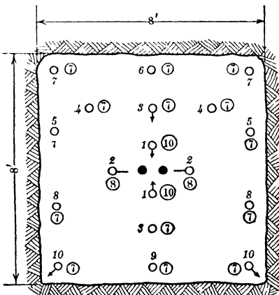
Fig 5 Michigan or "Burnt"-cut Round (For explanation of numerals at each hole, see note under Fig 4)
