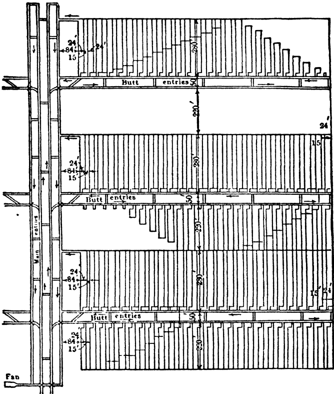
Fig 720. Systematic Mining, Pittsburgh Seam
