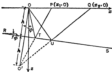
Fig 52. Determining Dip by McCollum-McGhee Method (24)
