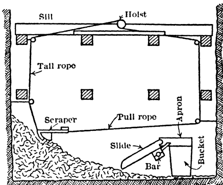
Fig 13 Scraper in Shaft Bottom, Champion Mine, Mich
