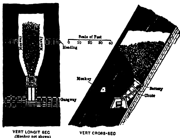
Fig 713. Battery Breast, Mammoth Seam, Hazleton, Penna (after Chance)
