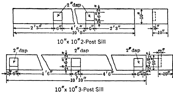
Fig 340. Details of Stope Sills, Bisbee, Ariz
