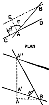
VERTICAL SECTION ON A-B Fig 75 To determine Thickness of Bed
