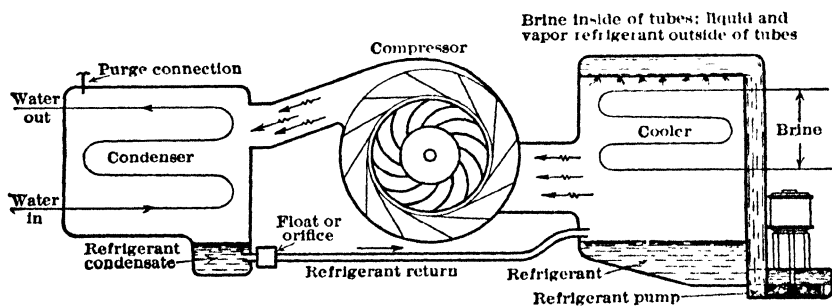
Fig 62. Arrangement of Centrifugal Refrigeration System (79)
