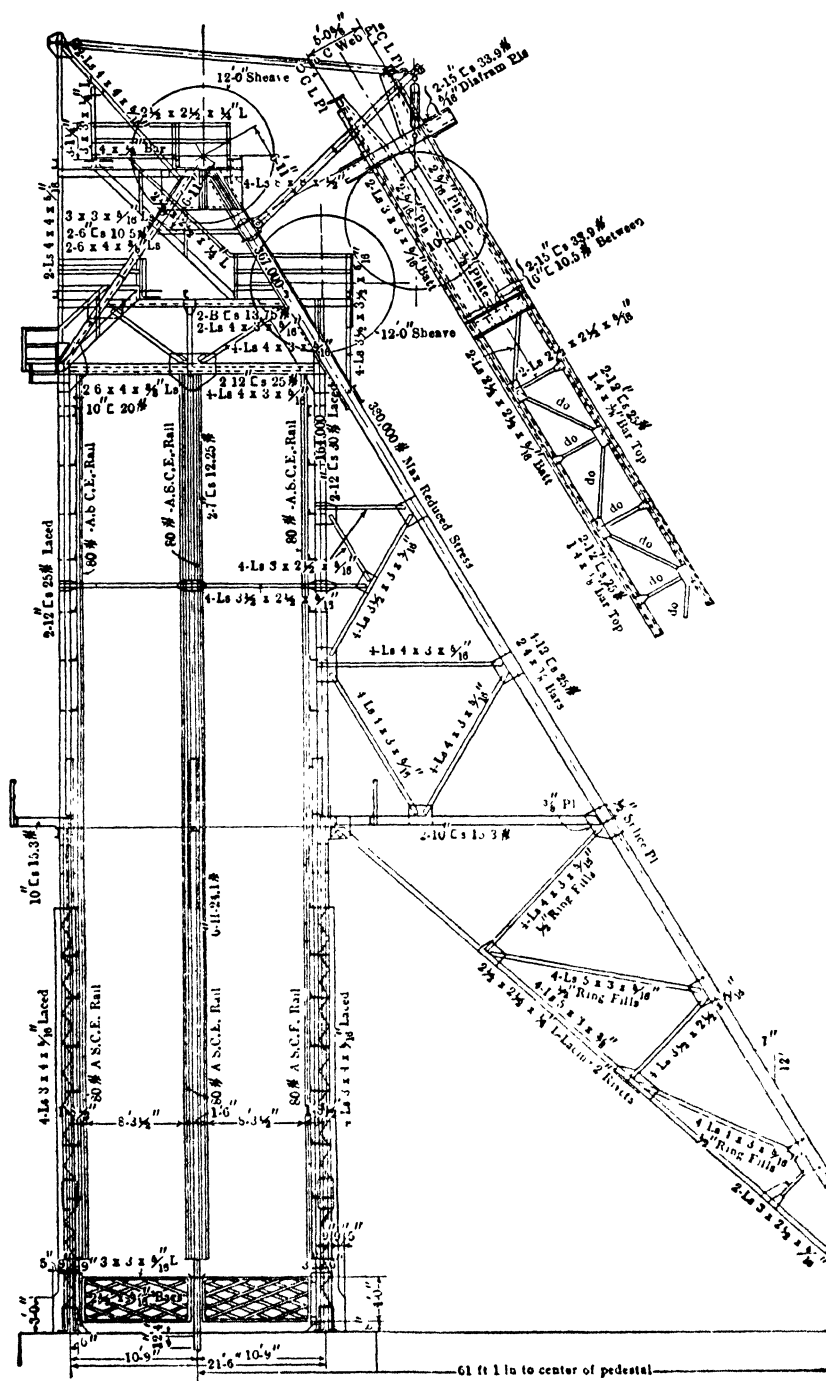
Fig 74. Steel Headframe, Consol Coal Co, Carretta, W Va
