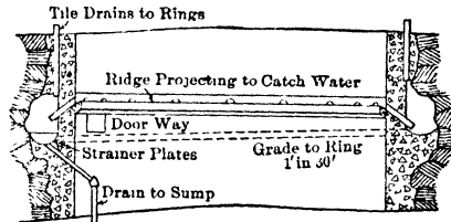
Fig 16 Water Ring for Concrete-lined Shaft (Mines & Min)
