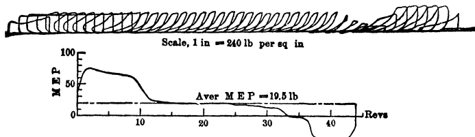
Fig 50. Hoisting Card (Leonard Shaft, Butte) from Head End of 34 x 72-in Air Hoist, 12-ft Drum; Running Balanced. Hoisting Speed, 1 800 ft in 45 sec (B V Nordberg, 47)
