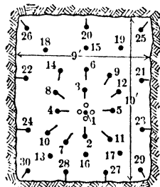
Fig 136 Burned-pyramid Cut, Crieghton Mine, Ont
