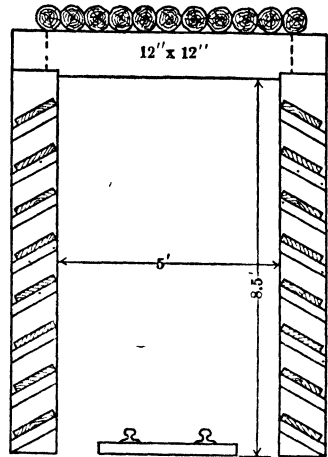
Fig 146. Shelf Lagging for Loose Ground
