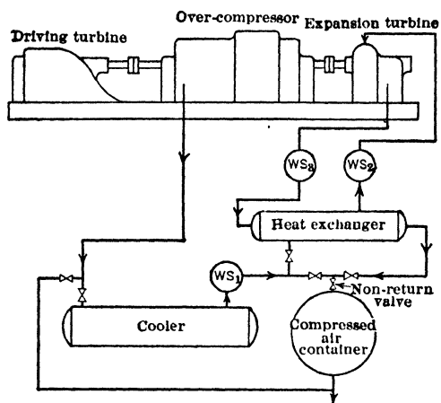
Fig 64. Devaporization Method for Comp Air (77)
