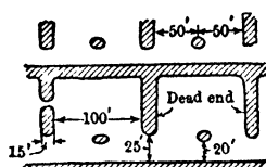
Fig 253 Stoping, Mohawk Mine (Sec in plane of lode)
