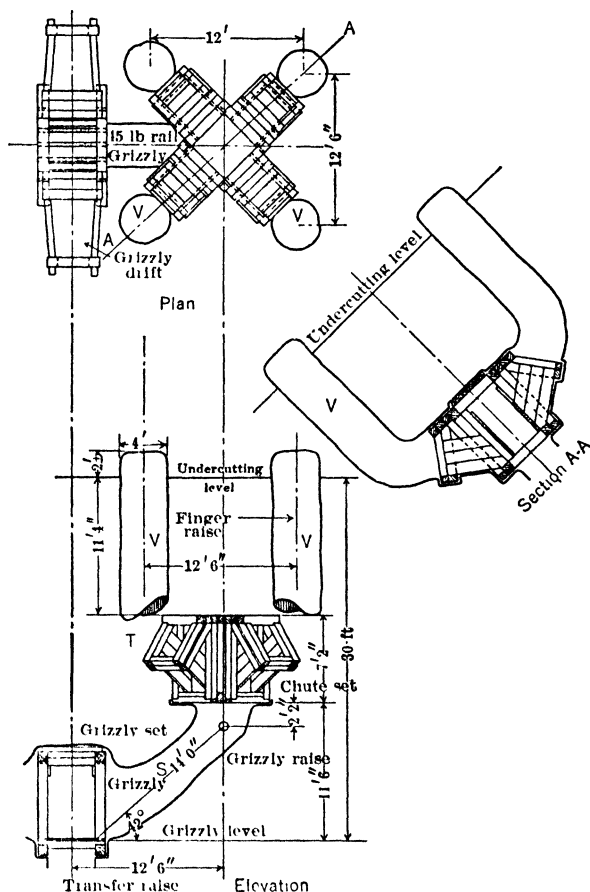
Fig 547. Location and Orientation of Chute Set, Miami Copper Co
