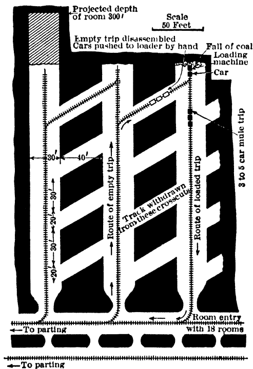
Fig 732. Mine-car Gathering Cycle, Moffat Mine, Ill (634)
