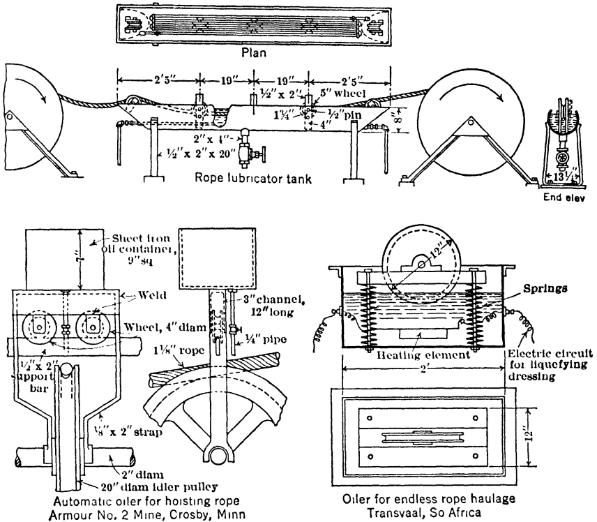
Fig 35a. Lubricating Devices for Wire Rope (37)
