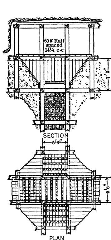
Fig 294. Wing-chute and Stope Grizzly, Frood Mine, Sudbury, Ont
