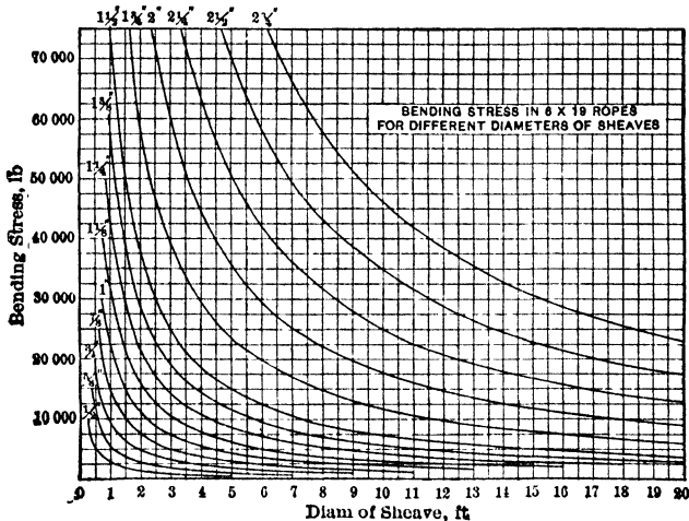
Fig 35. Bending Stresses in Hoisting Ropes
