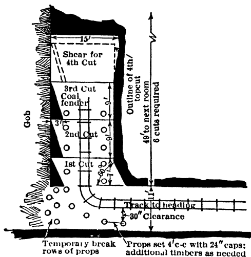
Fig 723. Mining of Room Pillars, Mona Mine
