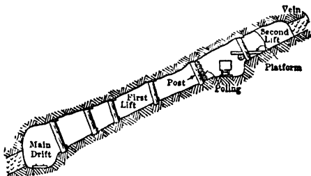
Fig 649. North Star Mine (Sec through stope, showing 1st track)
