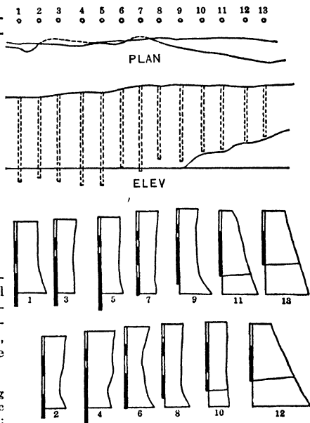
Fig 13. Different Loadings for Varying Conditions of Quarry Face
