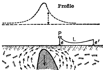
Fig 22. Ideal Profile of Potentials over Orebody (9)
