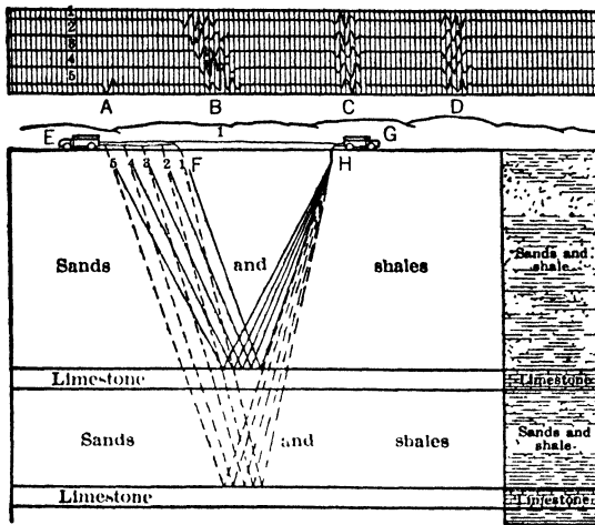
Fig 55. Observation Points, and Theoretical Seismograms for Two Limestone Horizons (21)
