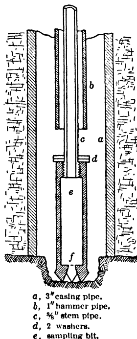
Fig 80. Chip-sampling Bit
