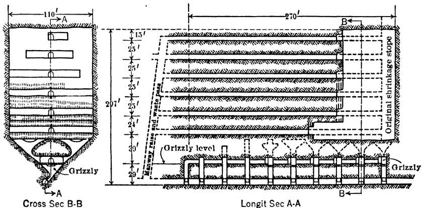
Fig 280. Mining Waste Rock for Filling, McIntyre Mine, Schumacher, Ont.
