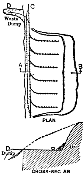
Fig 663 Open-cut on Hillside, Hand-loading
