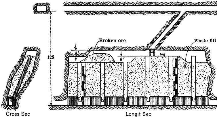
Fig 380. Horiz Cut-and-fill Stope, McIntyre Mine, Schumacher, Ont
