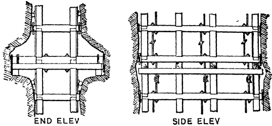
Fig 23 Bearing Timbers (16)
