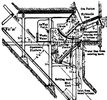
Fig 145. Shaft Pockets, Franklin Furnace, N J ( E & M Jour )
