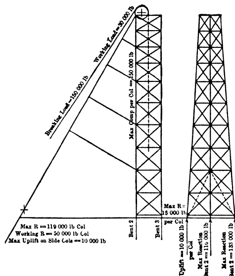
Fig 59. Main Stresses in a 6-post Frame
