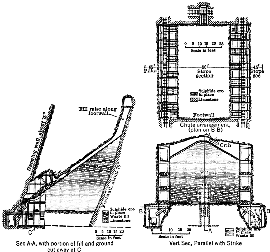
Fig 423 Inclined Cut-and-fill Stope, showing former use of double-lead sets running parallel with Section Lines, Campbell Orebody, Warren, Ariz (91)
