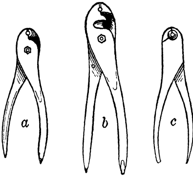
Fig 25 Cap Crimpers
