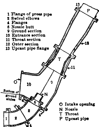
Fig 844. Hendy Hydraulic Elevator
