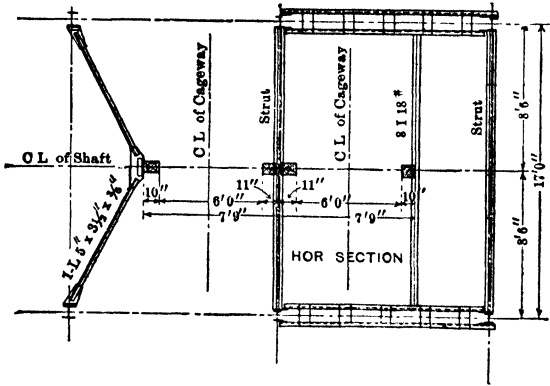
Fig 76. Guide Supports
