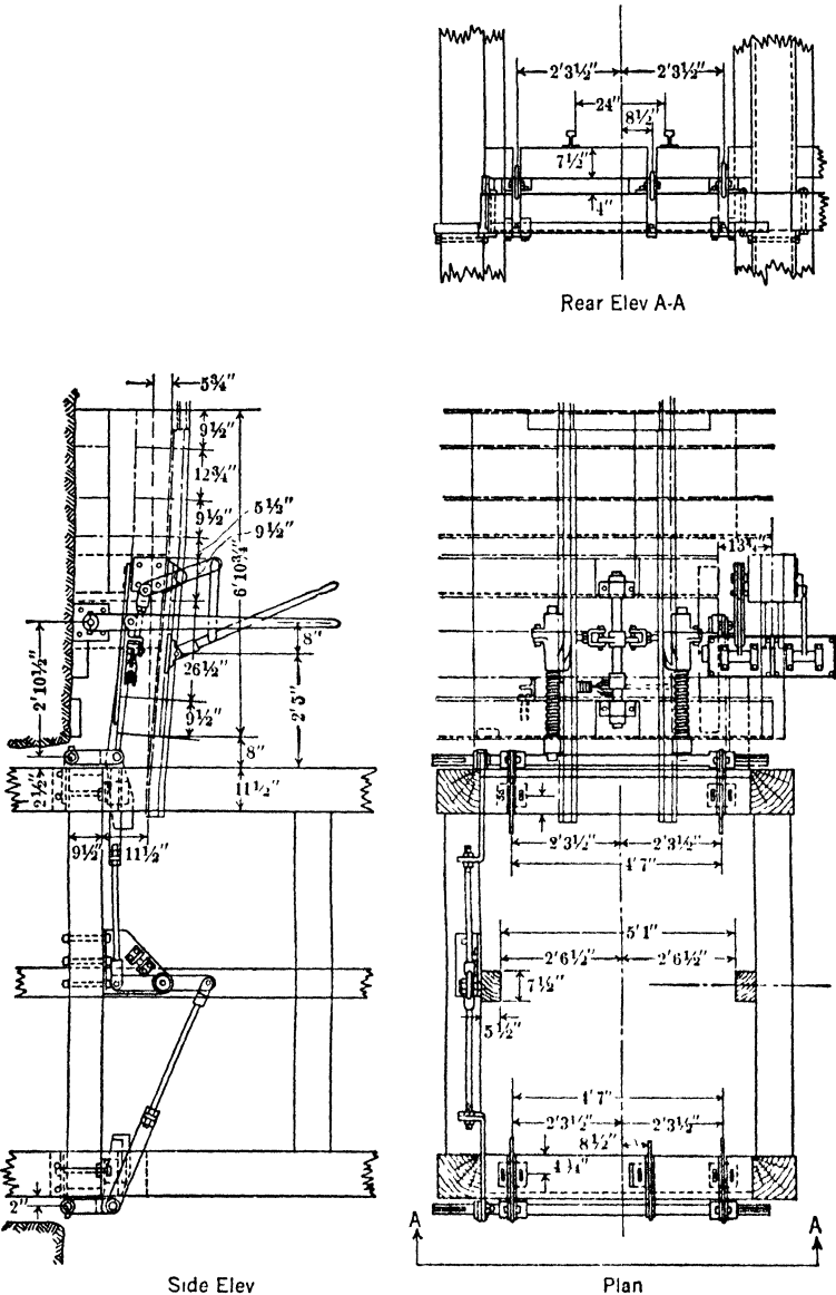
Fig 123. Underground Chairs and Caging Equipment, No 3 Shaft, Horne Copper Mine, Noranda, Quebec (37)
