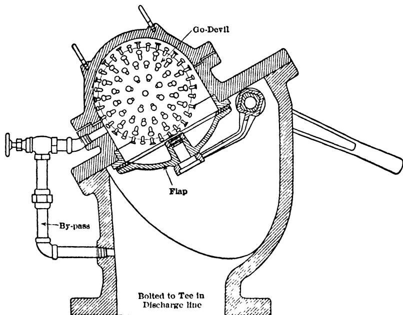
Fig 11. "Go-Devil" and Housing, for Cleaning Column Pipes
