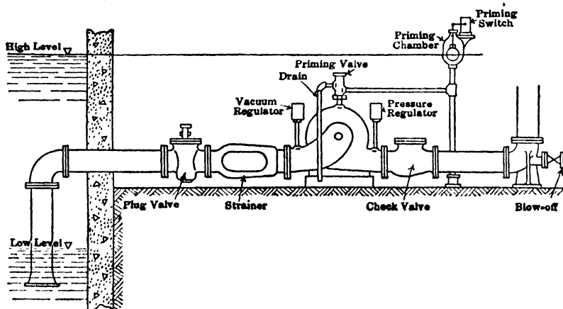
Fig 27. Automatic Control of a Centrifugal Pump Taking Water from a Dam
