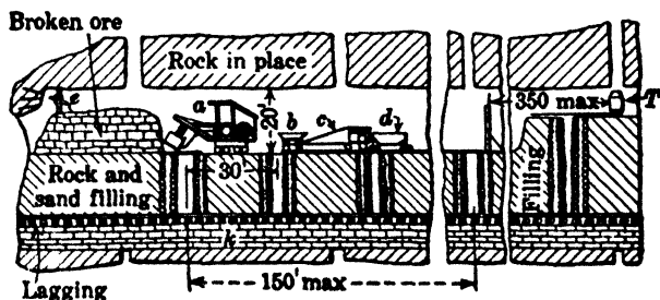
Fig 402. Mechanical Loading, Champion Mine
