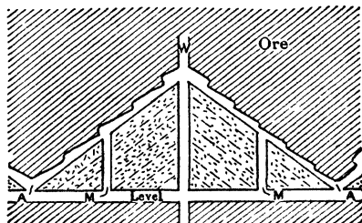
Fig 412. Starting Rill Stopes, Kalgoorlie
