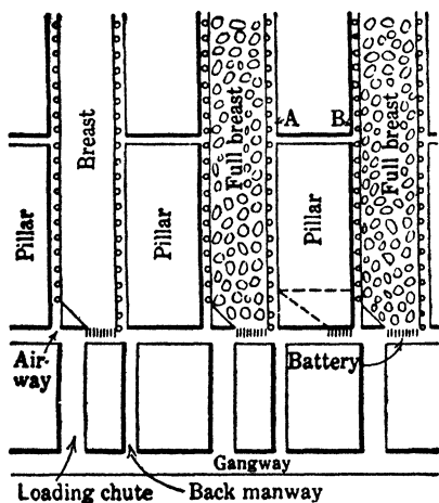
Fig 750. Robbing by Pillar-breast Method (609)
