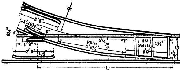
Fig 32. Point or Split Switch
