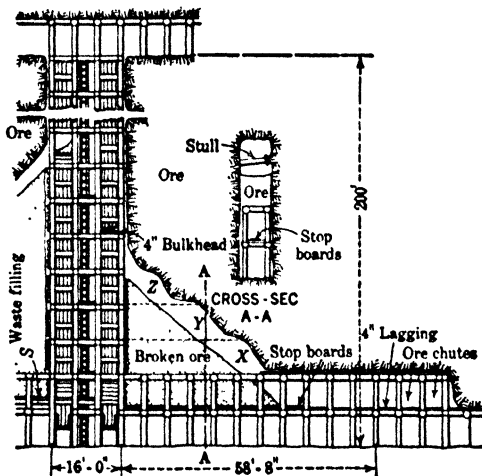
Fig 419. Opening a Rill Stope, Butte Distr, Mont (534)
