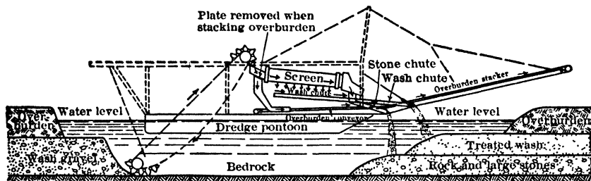
Fig 854. Dredge Equipped for Resoiling, Newstead, Victoria
