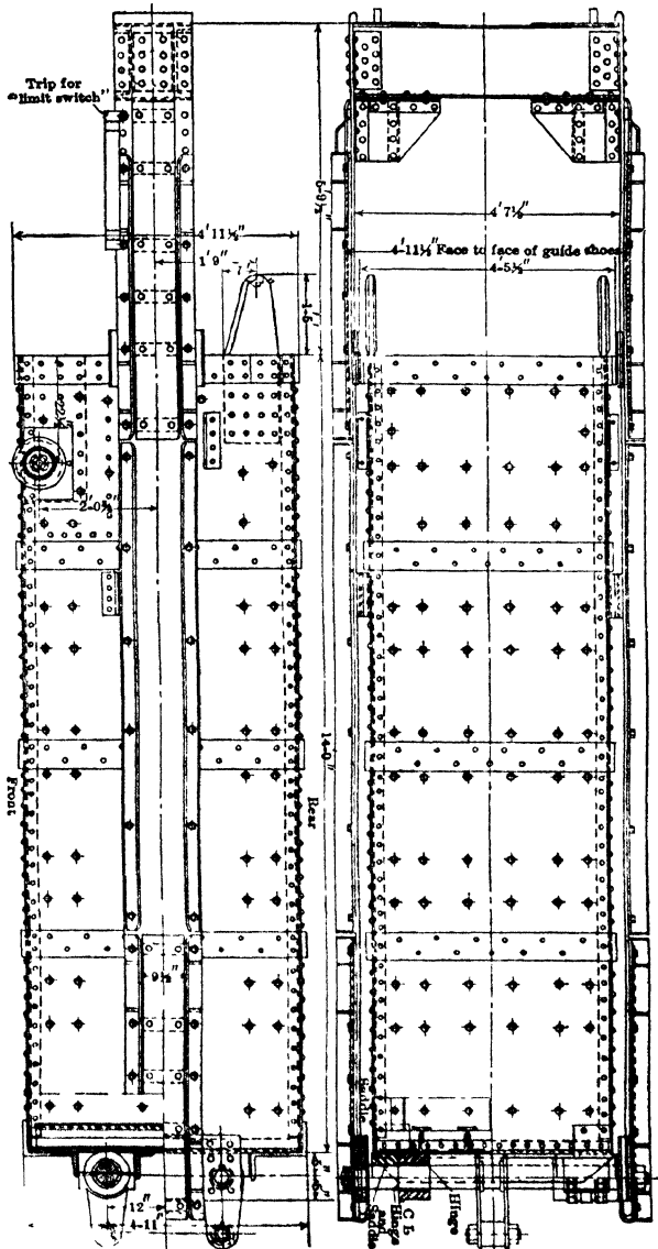
Fig 128 12-ton Skip, Inspiration Mine, Ariz (77)
