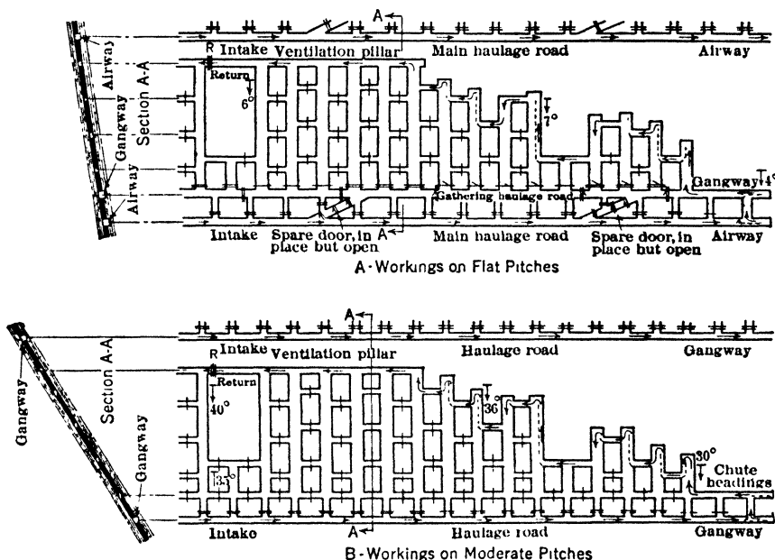
Fig 8. Methods of Ventilating Gassy Room-and-pillar Workings (27). (Legend as for Fig 2)
