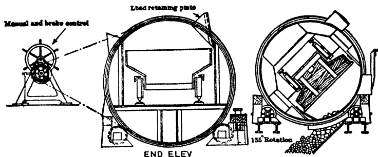
Fig 52e. Gravity Rotary Dumper, Hand-operated Car (Car Dumper and Equipment Co)
