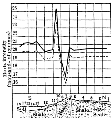
Fig 13. Survey of Horiz Magnetic Intensity, Valmont Dike Extension (7)
