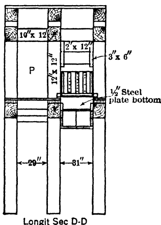
Fig 554. Details of Raise Timbering, Ruth Mine, Nev
