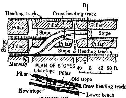
Fig 204. Working Lower Bench of Big Seam by Cross-heading
