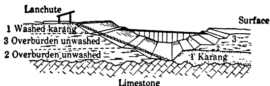
Fig 879. Open-cut worked by Benches Diagrammatic Cross-section (trestles to lower benches omitted)
