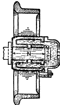
Fig 18a. Whitney Self-oiling Wheel
