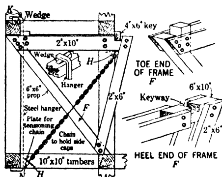
Fig 308. Mode of Support for Underhand Square-sets, Briggs Mine
