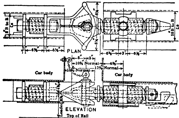
Fig 17d. Semi-automatic Spring Coupling (Allen & Garcia)
