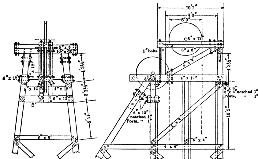
Fig 68. Headframe with Tandem Sheaves
