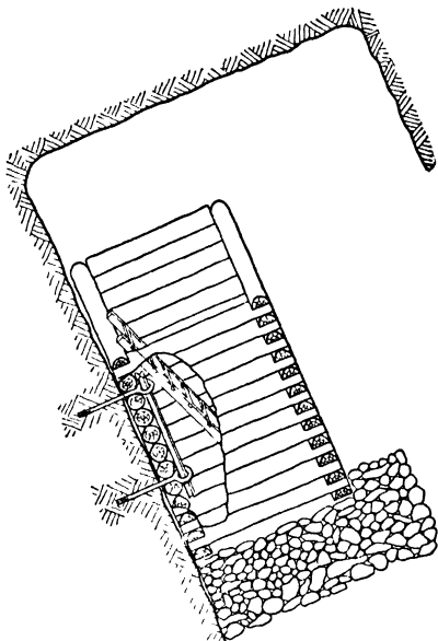
Fig 437. Cribbed Manway pinned to Wall by Eye-bolt and Rail, Wright-Hargreaves Mine, Kirkland Lake, Ont
