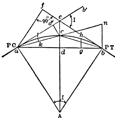
Fig 27. Laying Out Curve by Offsets
