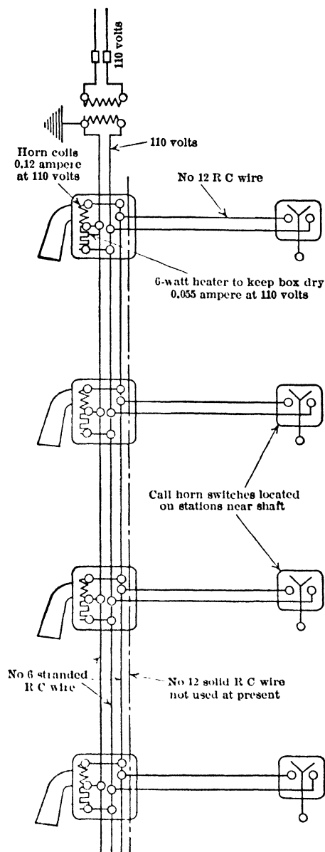
Fig 101. Call-horn System for the Ross Shaft
