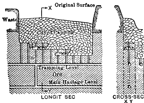
Fig 532. Arizona Copper Co. Sub-level Caving
