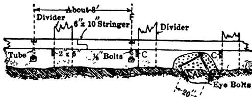
Fig 91. Copper Range Skip Track (Longit Sec)
