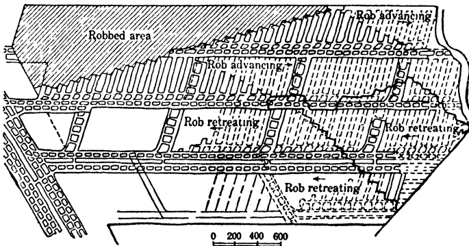
Fig 726. Room and Pillar, Mine No 6, U S Coal & Coke Co (607)
