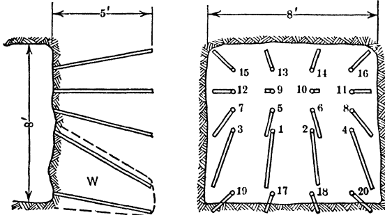
Rotation of firing holes designated by numbers shown at collar of holes
