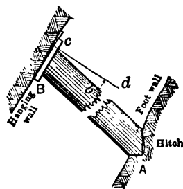
Fig 226. Stull Timbering
