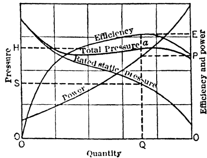
Fig 44. Characteristic Curves of Fan Performance (9)
