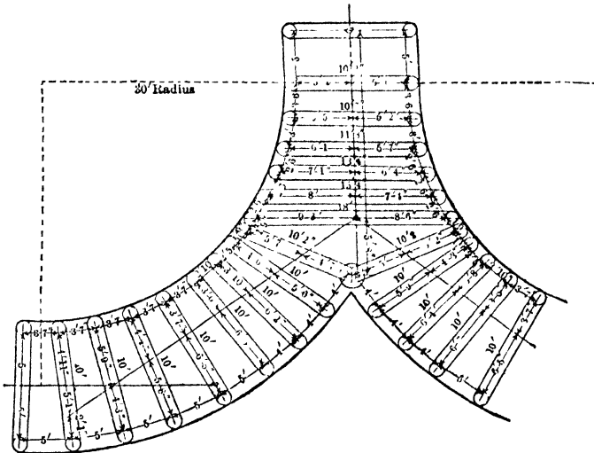
Fig 29. Layout for Double Turnout
