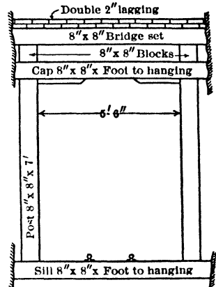
Fig 414 Gangway Timbering, Park City Consol Mine, Park City, Utah
