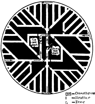
Fig 10. Ventilating System for Longwall Mining
