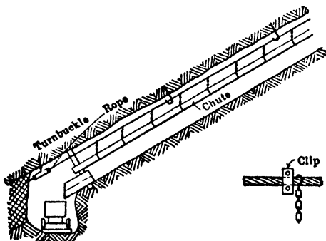
Fig 651. Mode of Support for Shaking Chutes
