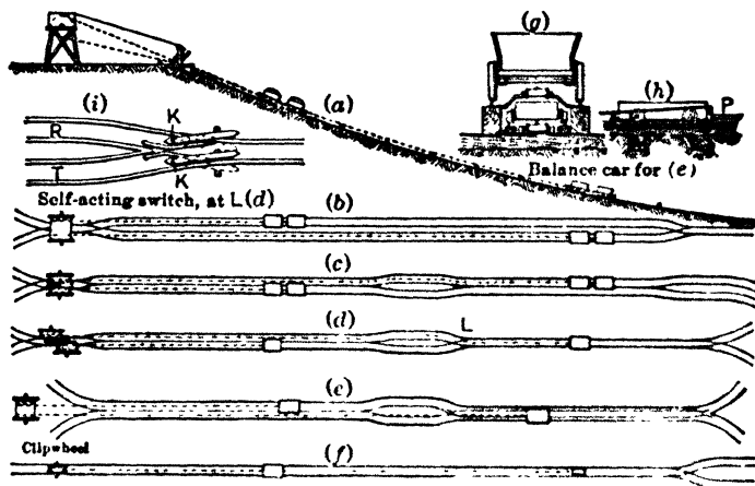
Fig 54. Track System for Self-acting Planes - Hildenbrand, except (e)
