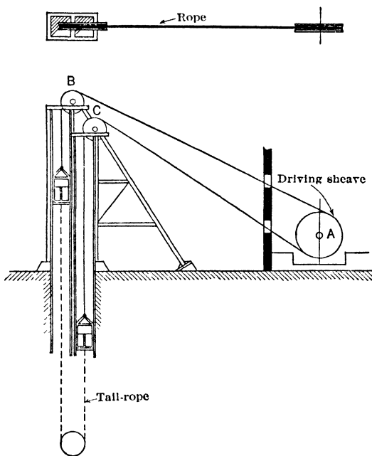
Fig 1. Diagram of Koepe Hoist
