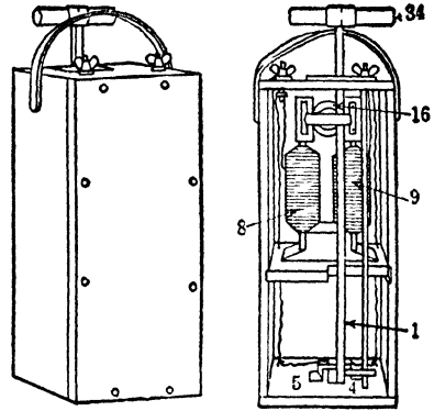
Fig 26 Blasting Machine
