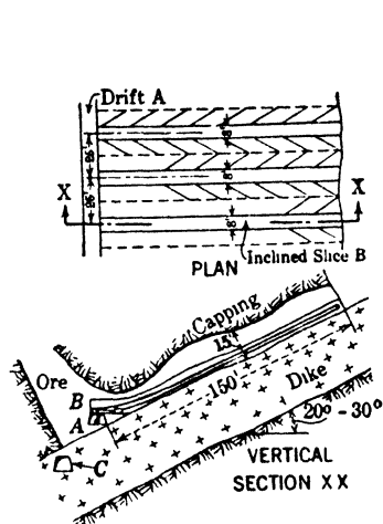
Fig 528. Scaper Loading in Trough-shaped Deposit
