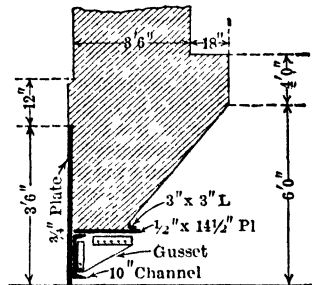
Fig 11a. Cutting Edge of Shoe, Colorado River Caisson (Rivets on outside countersunk)
