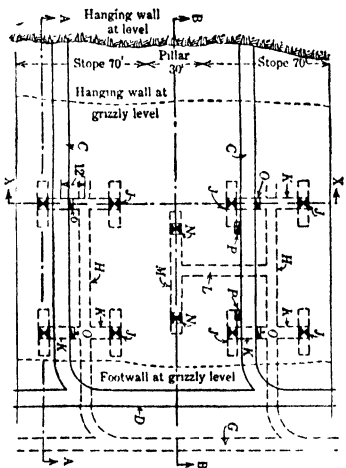
Fig 457 Beatson Mine, Alaska. (Diagram of main and grizzly levels; latter shown by dotted lines)
