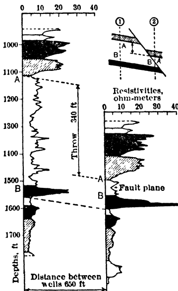
Fig. 42 Solution of a Fault by Resistivity Measurements in Boreholes (17)
