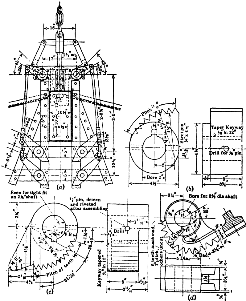
Fig 115. Types of Safety Catches
