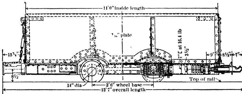
Fig 15. Colliery Car, Pittsburgh Coal Co, 1936.
