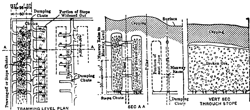
Fig 568. Boston Mine, Hand-tramming System, Chutes in Middle of Stope
