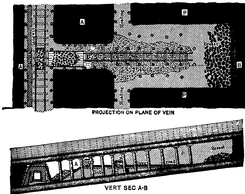
Fig 710. Buggy Breast (after Chance, Vol AC, 2nd Geol Surv Penna)
