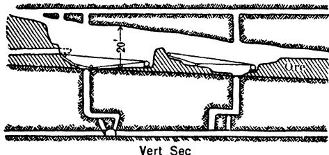
Fig 220. Glory-hole Stopping in a Thick Manto, El Potosí Mine, Chihuahua, Mex
