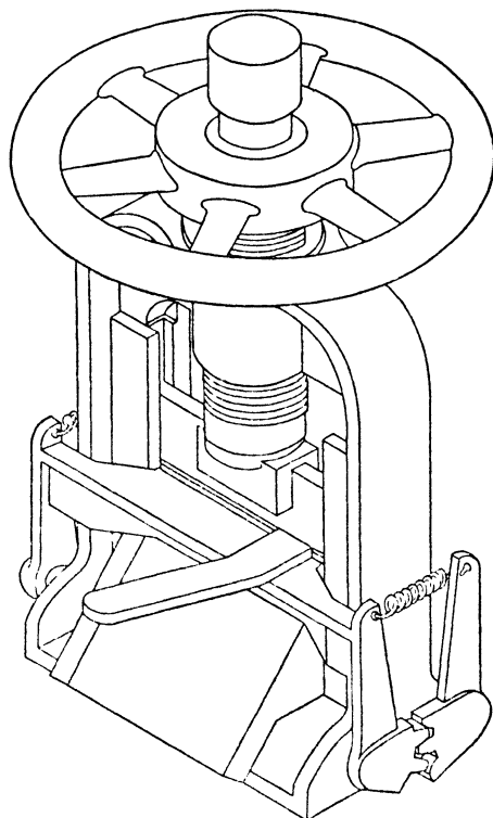
Fig 79 Core Splitter
