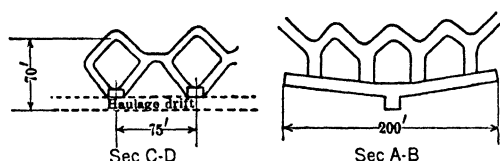
Fig 563. Slusher System Development, Climax, Colo
