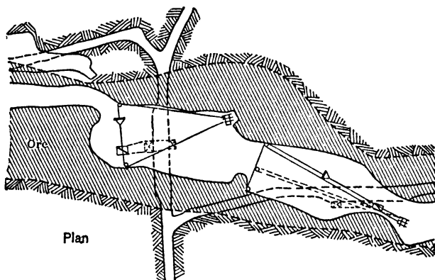
Fig 656. Scraping in El Potosí Mine, Mex
