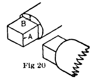
Fig 17, 18, 19, 20 Cribbing Joints
