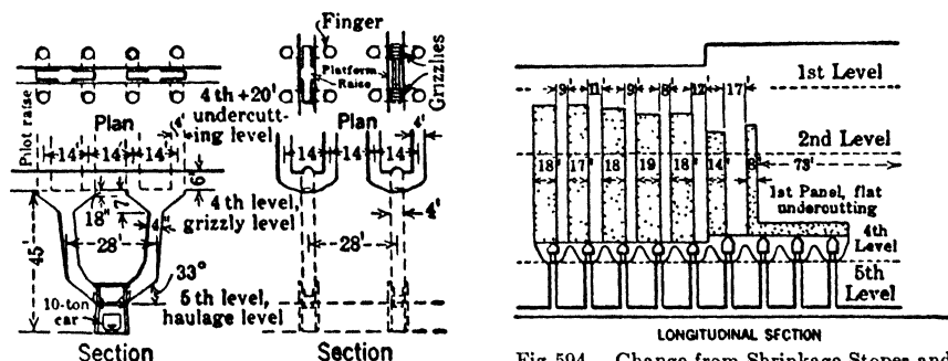
Fig 593. Haulage-level Raises, showing Fingers and Grizzly Stations, Humboldt Mine
