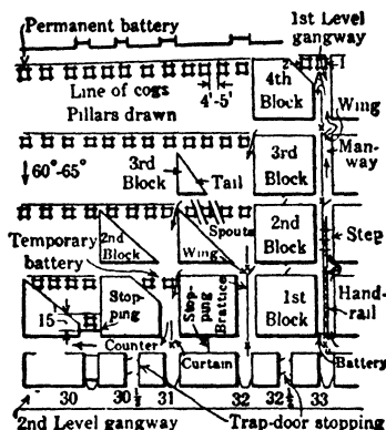
Fig 753. Pillar Drawing in Chute-and-pillar System, Pierce County, Wash (610)
