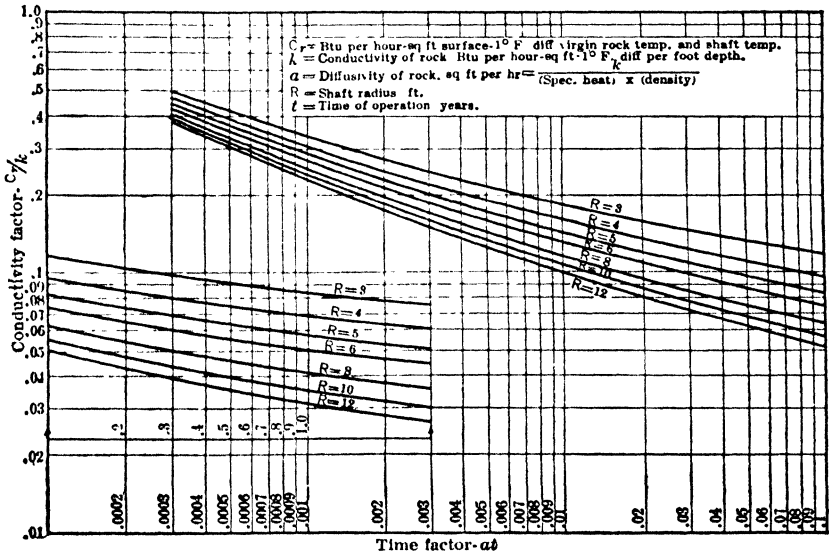
Fig 60. Chart of Heat Flow in Mines (79)
