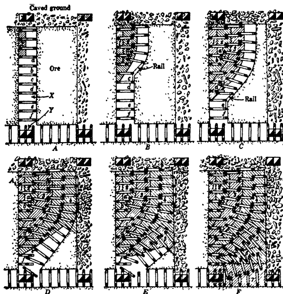
Fig 526. Radial Slicing (diagrammatic)
