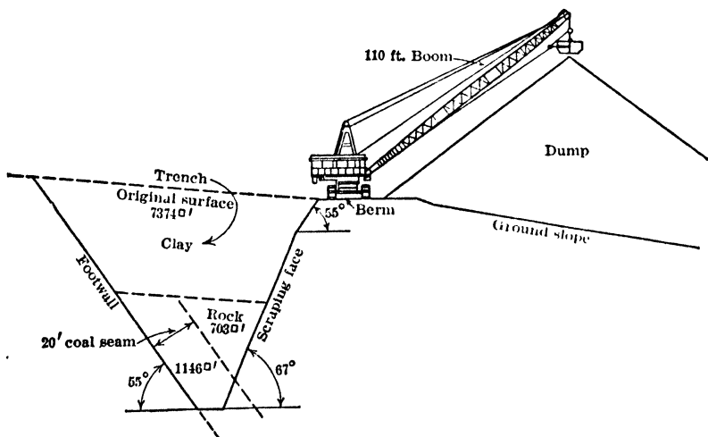
Fig 695. Dragline Excavation at Merriam Stripping
