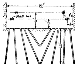
Fig 6. Double "V" or Wedge Cut
