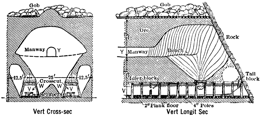
Fig 522. Stopping Procedure, Montreal Mine
