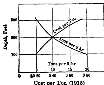
Fig 54 Capacity and Cost of Whim Hoisting
