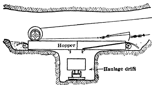
Fig 564. Vert Cross-sec through Haulage Drift, showing Slusher Platform, Climax, Colo
