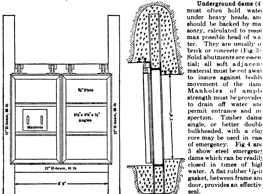
Fig 5. Emergency Flood Dam, 35-ft Head
