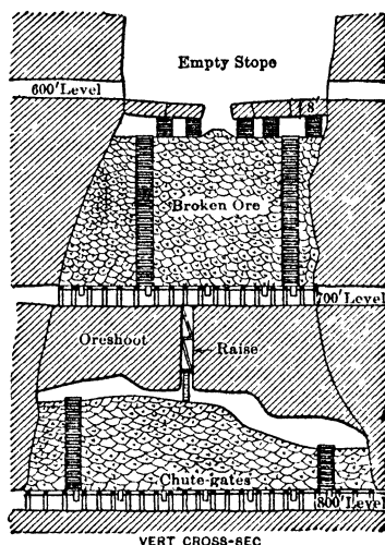
Fig 449. Shrinkage Stopes, Cresson Mine
