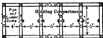
Fig 1. Rectangular Shaft
