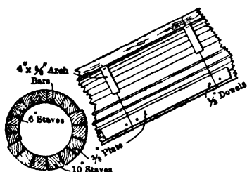
Fig 623. Inclined Cylindrical Chute
