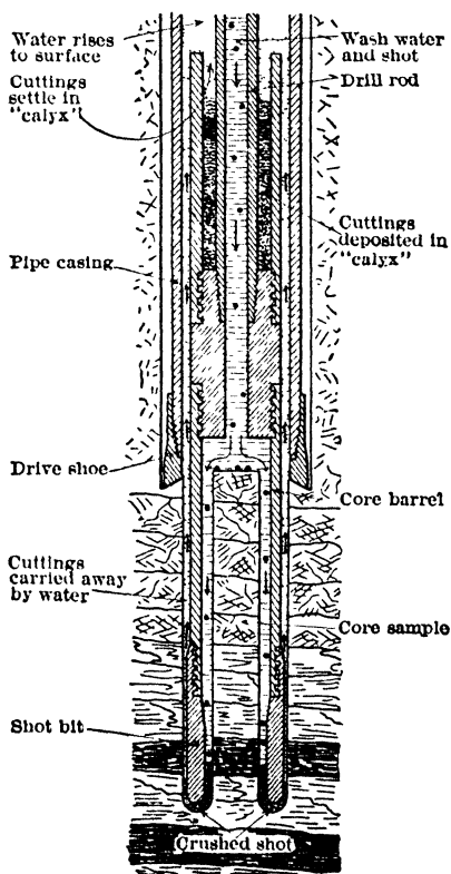
Fig 50. Calyx Drill
