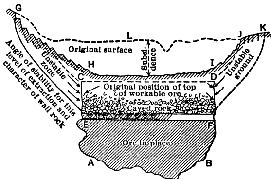
Fig 796. Suggested Mechanics of Subsidence in Block-caving of a Large Orebody
