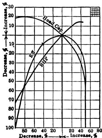
Fig 14. Performance of Volute Pumps
