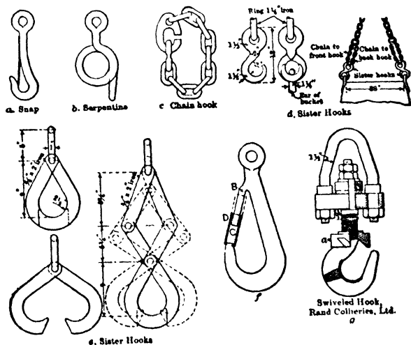
Fig 104. Bucket Hooks
