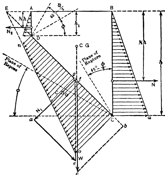
Fig 163. Graphic Solution for Shallow Bins
