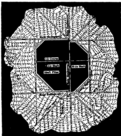
Fig 760 Longwall Advancing (after Swift)
