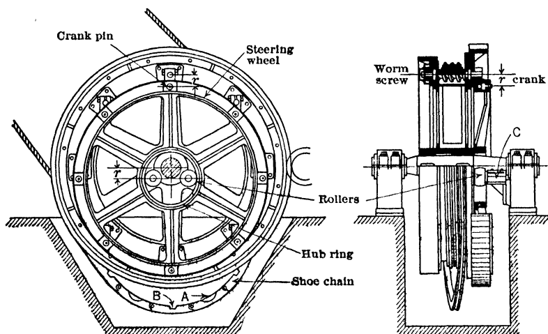
Fig 3. Ohnesorge Driving Sheave with Endless Shoe Chain. (E & M Jour)
