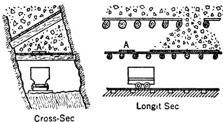
Fig 635. Simple Form of Chinaman Chute
