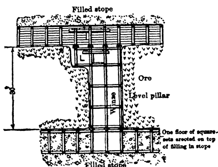
Fig 305. Square-setting for Underhand Stope
