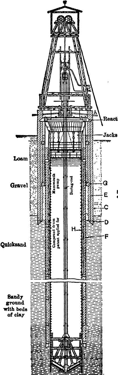
Fig 17. Honigmann Method, Mammoth Pump and Borer. Shafts IV and V, Rheinpreussen Colliery, Germany. A, Suction Pipe and Overflow; B, Compressed Air; C, Caisson; D, Shoe; E, Anchor Rods; F, Compound Lining; H, Cast-iron Lining (Riemer)
