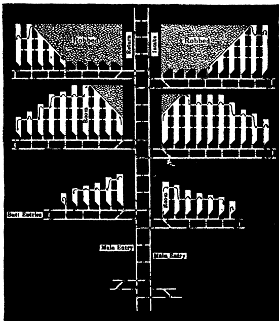
Fig 701. Double-entry System in Flat Seam (U S)
