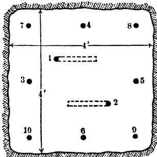
Fig 154. X-cut in Soft Hematite, Pioneer Mine, Ely, Minn. Holes 4.5 ft deep
