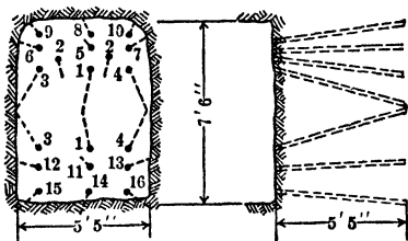
Fig 126. Horiz V-cut in Hard Limestone, Presidio Mine, Shafter, Tex
