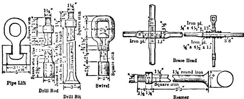
Fig 7. Parts of Spring-pole Drill
