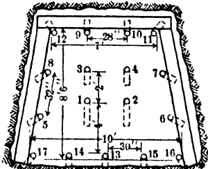
Fig 122 Bottom-draw, Jackhammer Cut in Schist, Inspiration Mine, Inspiration, Ariz
