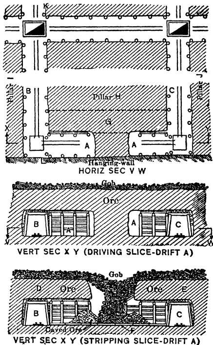
Fig 508 Slicing and Stripping Details
