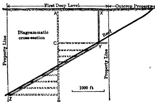
Fig 114. Outcrop and Deep-level Mines, Witwatersrand
