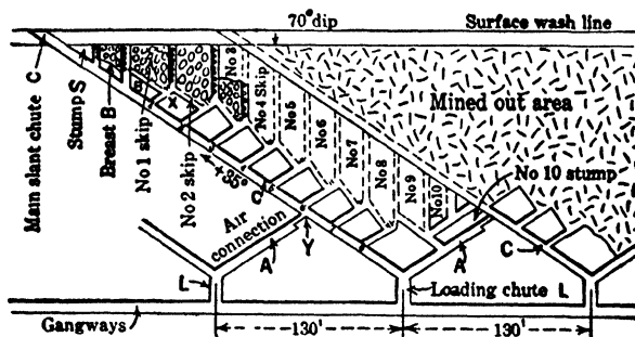
Fig 745. Orchard Seam, Lehigh Nav Coal Co, Penna (609)
