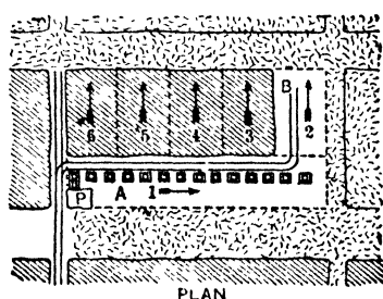
Fig 754. Robbing Pillars, Northumberland
