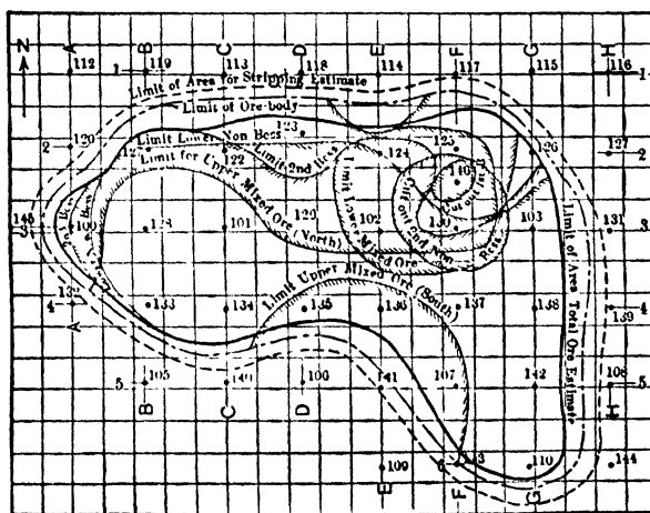
Fig 96. Typical Mesabi Orebody
