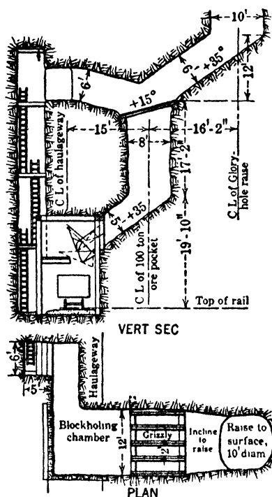
Fig 688. Bulldozing Chamber, Pocket, and Chute, Fresnillo, Mex (640)
