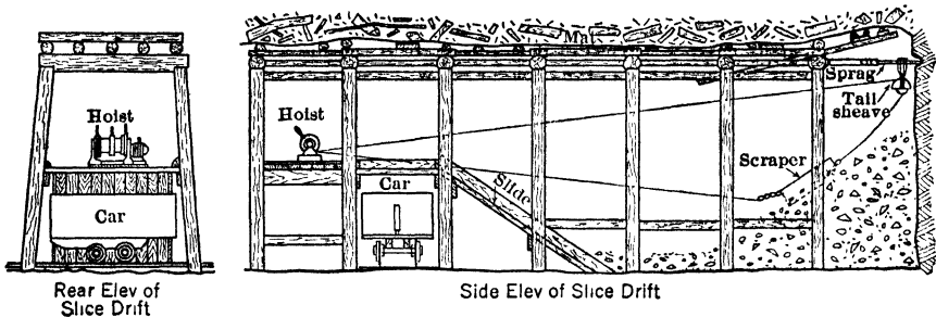
Fig 469. Slice-drift, Scraper-loading to Car
