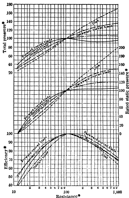
Fig 58. Comparative Pressure and Efficiency Characteristics of Mine Fans (9)
