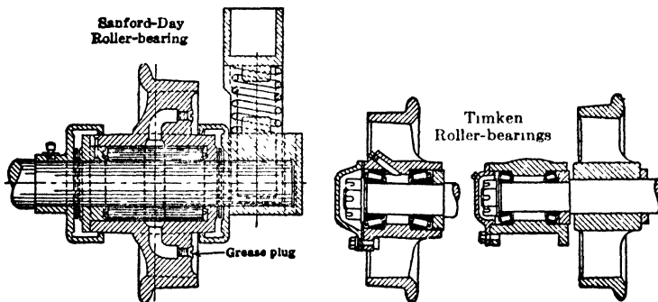
Fig 19a. Sanford-Day and Timken Roller-bearings
