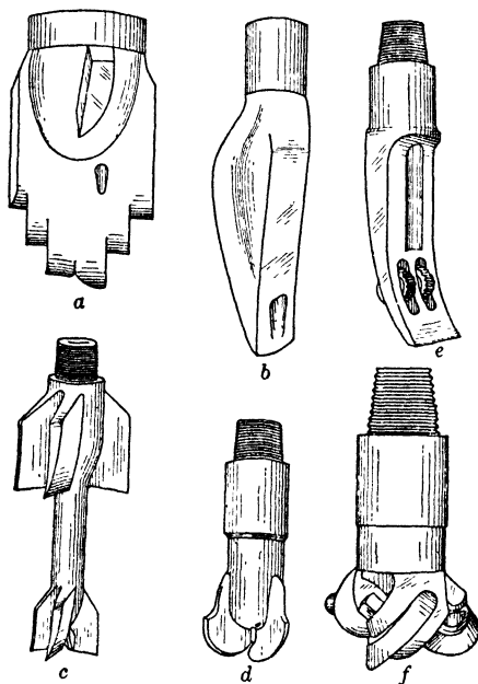
Fig 39. Special Bits for Directional Drilling
