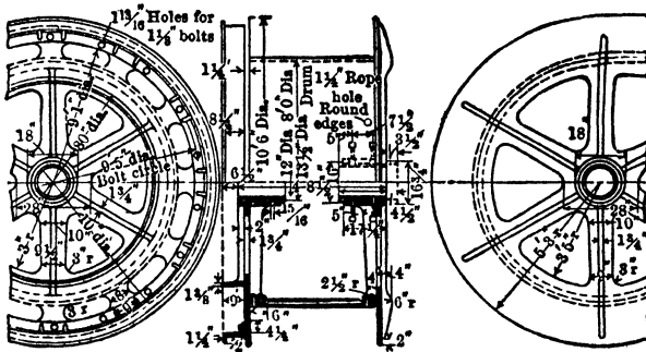
Fig 14a. Drum, 8 ft Diam X 4 ft Face
