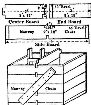
Fig 618 Two-compt Chute, Nevada Wonder Mine
