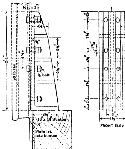
Fig 88 Bracket Support for Steel Rail Guides, Rand (Vaughan)
