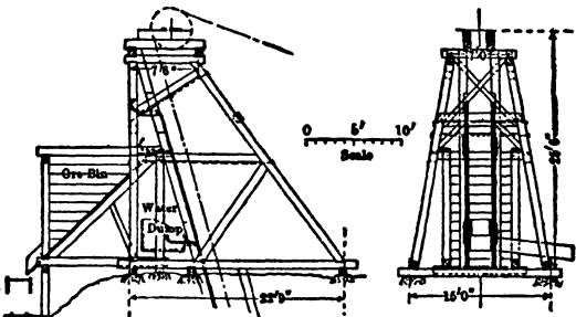
Fig 66. Headframe and Orebin for Development (Mines & Min)
