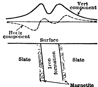
Fig 19. Typical Magnetic Anomalies for Conditions as shown (5)
