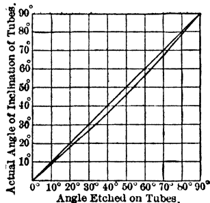
Fig 60. Curve of Capillarity Correction
