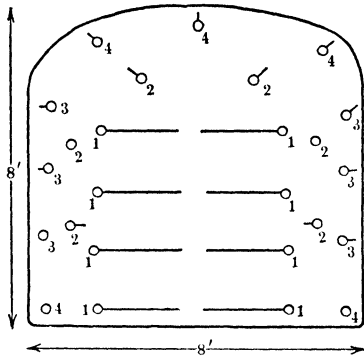
Fig 3 V-cut Round In trap rock, this round proved effective with 12-14 cartridges of 60% gelatin dynamite in each cut hole. From 10 to 12 cartridges of 60% special dynamite in other holes completes the charge. Advance by each round averaged 11-13 ft, using 13-ft holes. Figures in diagram indicate order of firing electric blasting caps. In easier ground, as sandstone, 2 easers and 2 side holes are not used, the 60% special dynamite also is replaced by 40% special dynamite
