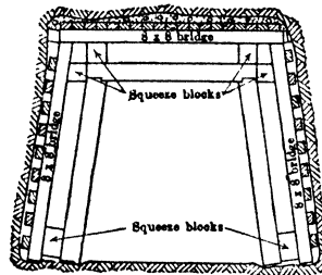
Fig 144. Timber Set for Heavy Ground
