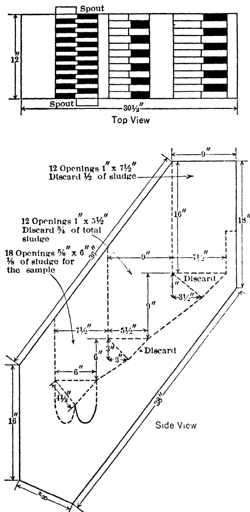
Fig 66. Splitting Device for Churn-drill Samples, Utah Copper Co
