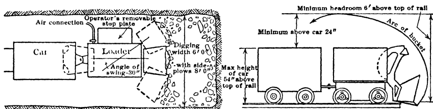
Fig 13. Shovel-type Loader Close-coupled to Mine Car for Small Headings
