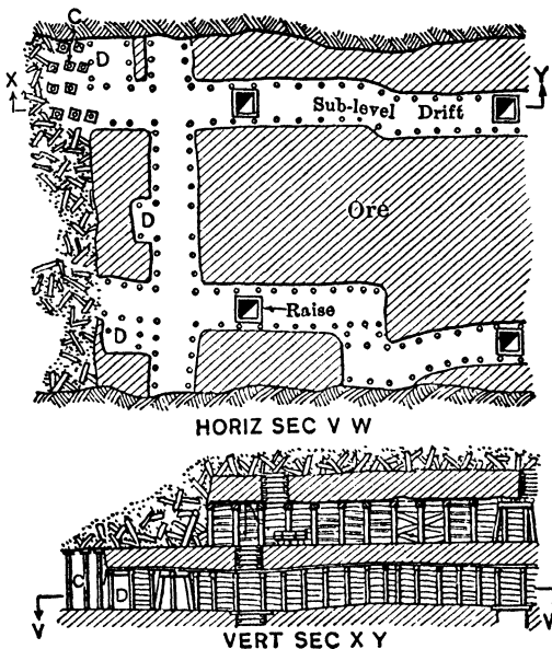
Fig 512. Slicing and Stripping Details
