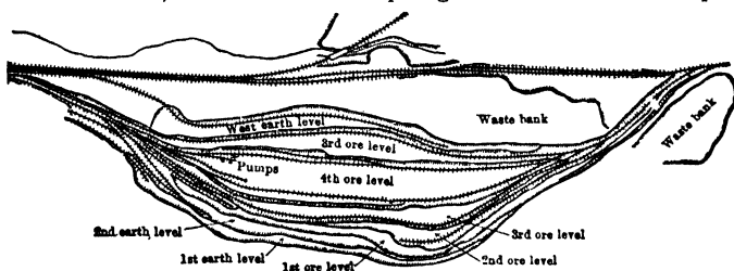
Fig 668. Track Layout, Mountain Iron Mine, Mesabi Range
