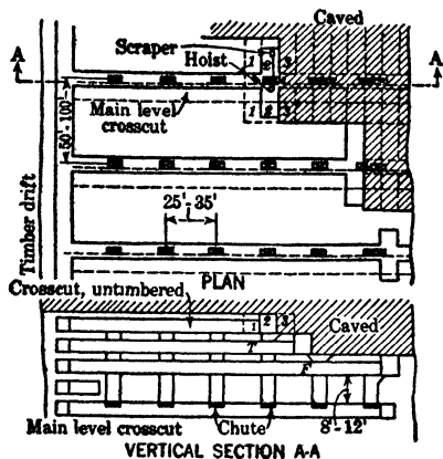
Fig 481. Drift Slicing, Scraper Loading (diagrammatic)
