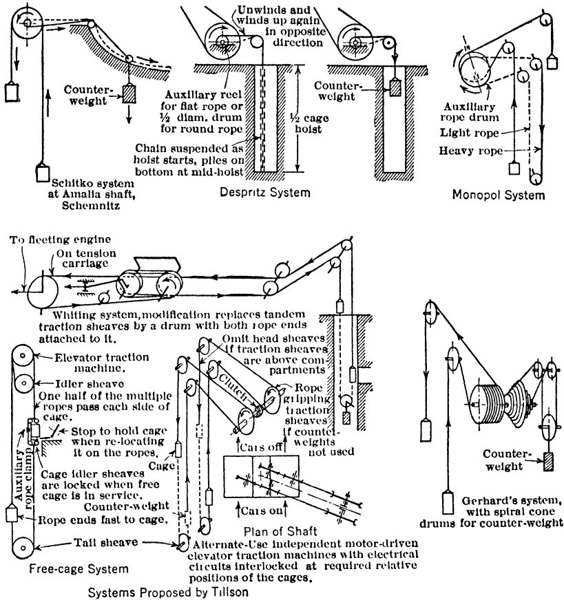
Fig 7. Miscellaneous Hoisting Systems (37)
