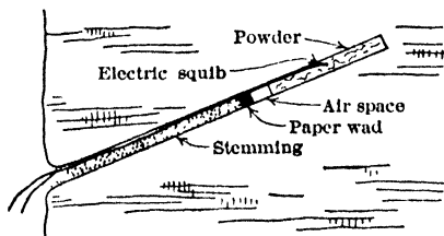
Fig 19. Blasting in Coal Air Space between Charge and Stemming
