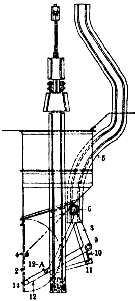
Fig 135. Lepley Bottom-discharge Coal Skip. Diagram of Mode of Dumping
