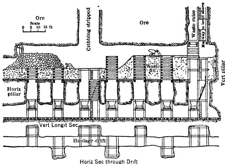
Fig 392. Typical Cut-and-fill Stope, United Verde Mine, Jerome, Ariz (227)
