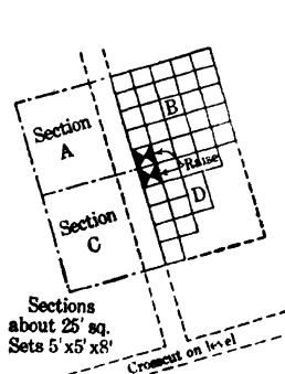
Fig 307. Plan of 5th Floor of Underhand Square-set Stope, Briggs Mine
