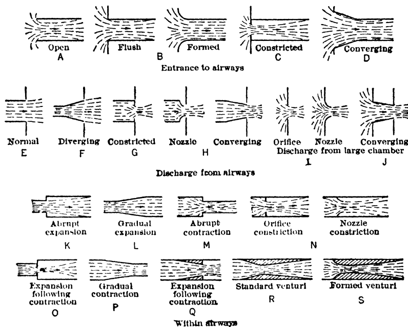
Fig 25. Common Types of Area Changes in Airways (9)
