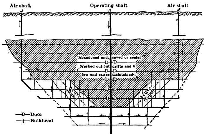
Fig 1. Ideal Layout of Mechanical-ventilation System, Metal Mines (9)
