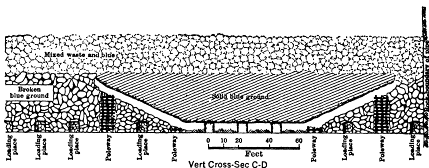
Fig 611. System of Chambering, De Beers Diamond Mine, Kimberley, So Africa
