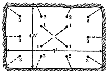
Fig 156. Pyramid Cut, Ruth Mine, Ruth, Nev. Holes average 6 ft deep
