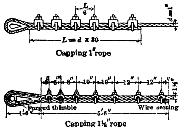
Fig 37. Correct Method of Capping Wire Ropes (Trans A I M E)
