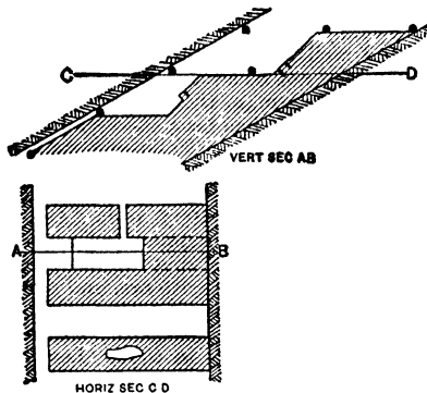
Fig 259. Underground Slate Quarry, Wales
