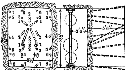
Fig 130. Pyramid-cut Round in Hard Sulphide or Porphyry. United Verde Mine, Jerome, Ariz
