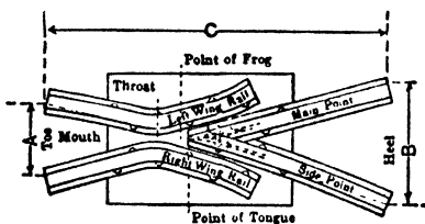
Fig 34. Fixed-rail Frog
