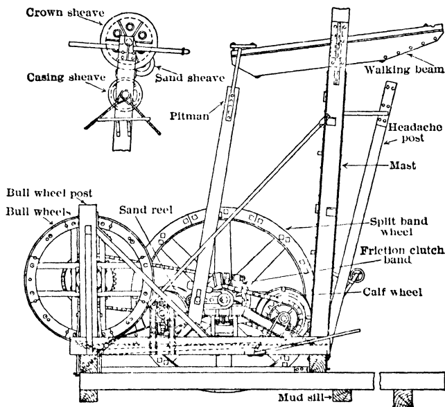
Fig 20 No 3 National Portable Drilling Rig
