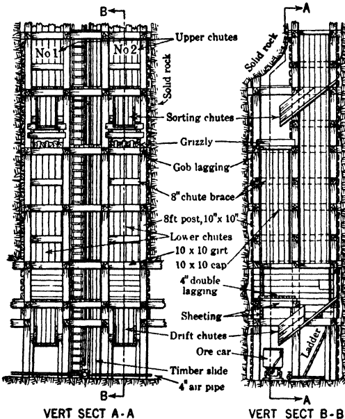
Fig 621. Square-set Chute with Sorting Grizzlies, Butte, Mont
