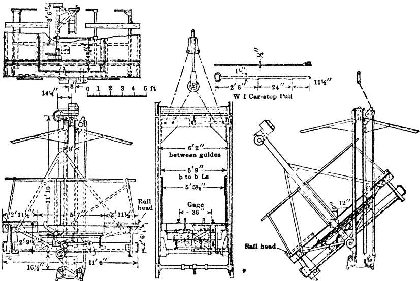
Fig 114. Drop-bottom, Self-dumping Car Cage, Lehigh Valley Coal Co, Wilkes-Barre, Pa (37)
