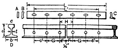
Fig 23. Rail Section and Splice Bars
