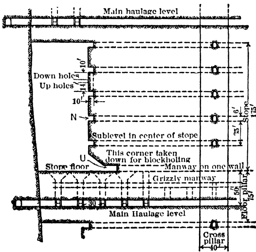
Fig 275. Side Elev, Horiz Sub-level Stope, "Lower H" Orebody, Horne Mine, Noranda, Quebec
