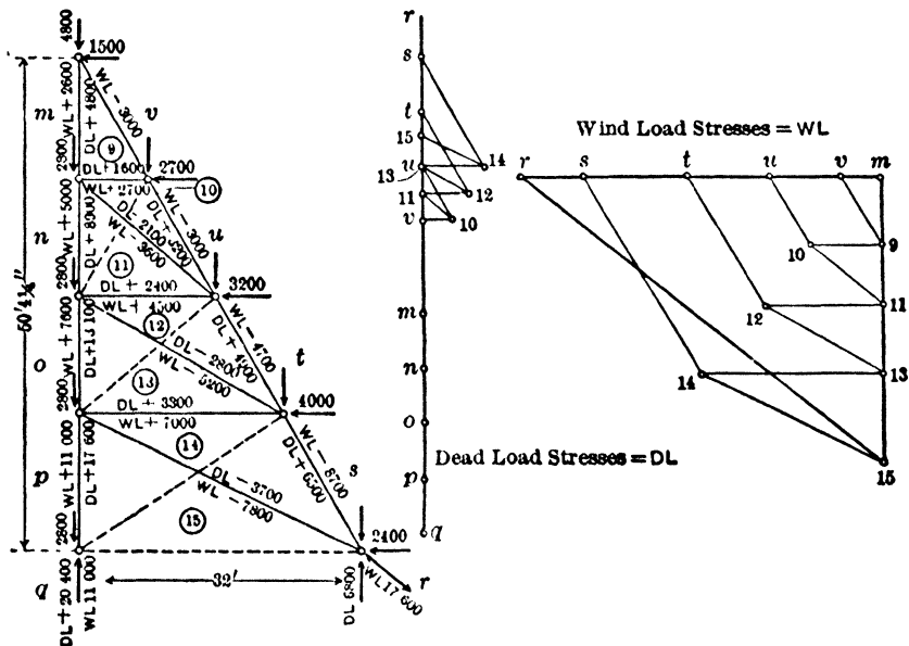
Fig 56. Headframe Stress Sheet, Side Elev
