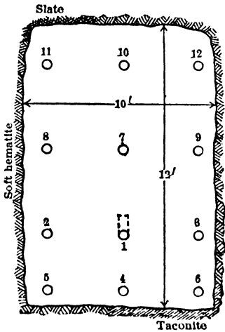
Fig 120 Jackhammer Round in Soft Iron Ore, Godfrey Mine, Hibbing, Minn, holes 6 ft deep, and all (ex No 1) drilled straight into face
