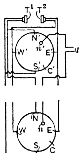
Fig 65 Diagram of Electrodes in Surface Receiver of Briggs' Clinophone
