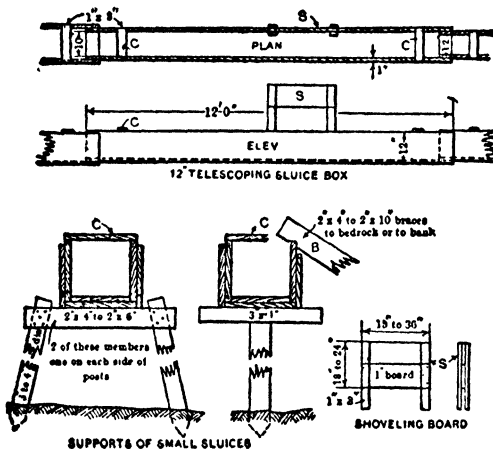
Fig 823. Small Sluices
