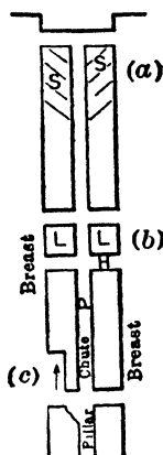
Fig 752 Robbing Pillars, Thick Steeply Pitching Seams
