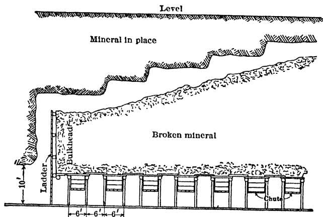
Fig 440. Shrinkage Stope, Narrow Veins, Rosiclare, Ill (197)
