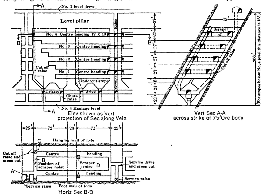
Fig 281. Longit Sub-level Stope, Mt Isa Mines, Queensland (500)
