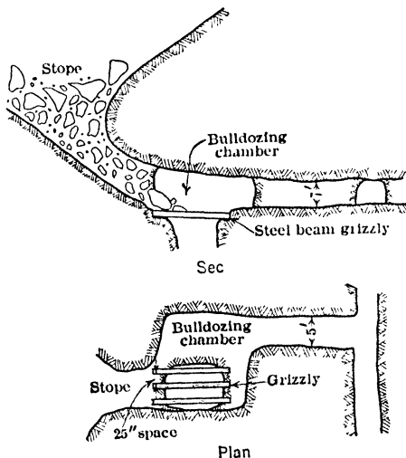
Fig 463. Bulldozing Chamber and Grizzly, Alaska Juneau Mine
