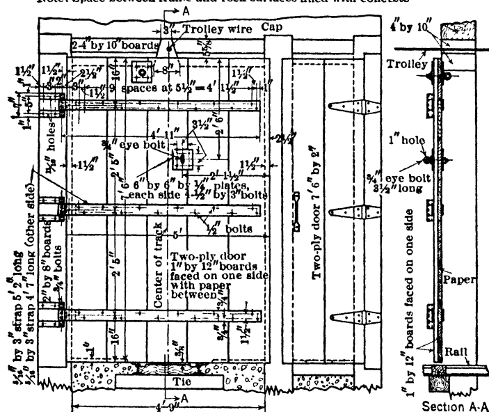
Fig 3. Ventilation Door used on Motor Haulageway in Metal Mine (31)
