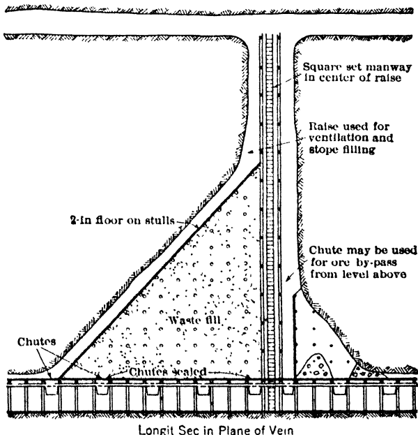
Fig 415. Rill Stope, Park City Consol Mines Co, Park City, Utah (244)
