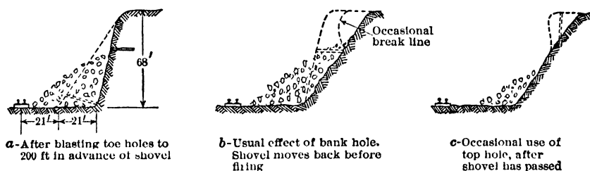
Fig 673 Blasting at Utah Copper Mine
