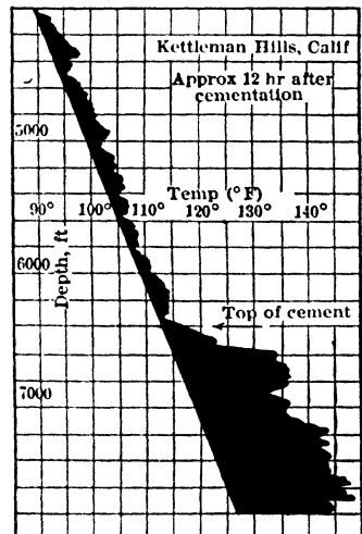
Fig 63. Temperature Survey 12 Hr after finishing Cementation around Casing in a Calif Well (29)
