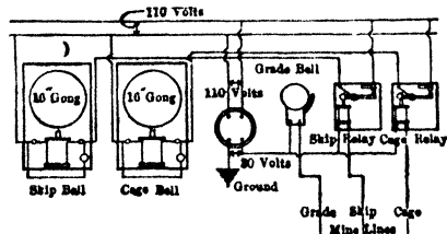
Fig 96. Signal System, Penn & Republic Mines, Mich
