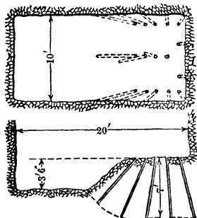
Fig 9. Bench or Slope Cut
