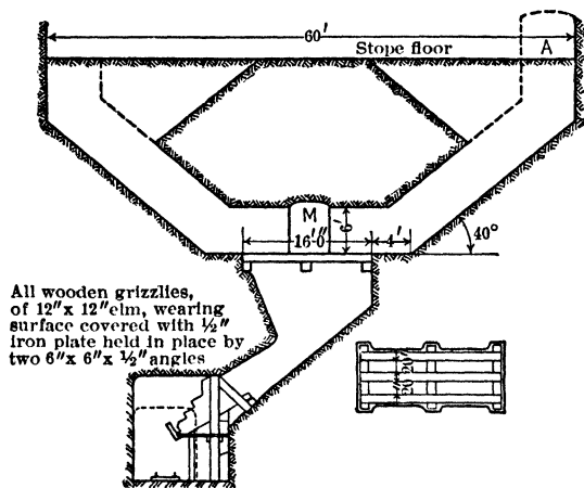
Fig 276. Chute Raise and Grizzly, Horne Mine, Noranda, Quebec
