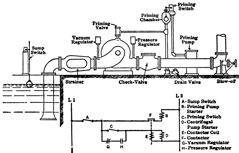
Fig 24 Arrangement of Primer and Accessories for Automatic Control of Centrifugal Pump, with Diagram of Wiring
