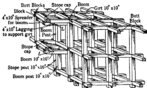
Fig 368. Recovering Square-set Stope, Butte, Mont (534)
