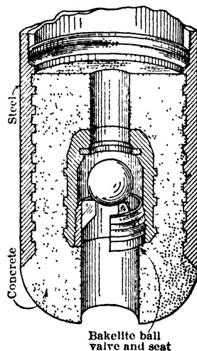
Fig 30. Baker Cement Float Shoe
