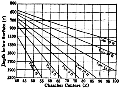
Fig 705. Relation between Depths and Room Centers for Different Thicknesses of Seam for 20-ft Rooms
