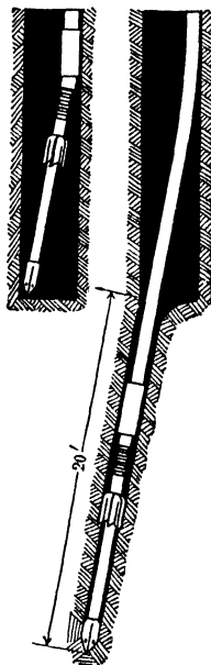
Fig 35. Lane Wells Knuckle Joint
