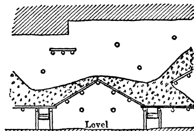
Fig 234 Wing Stulls (Sec in plane of vein)
