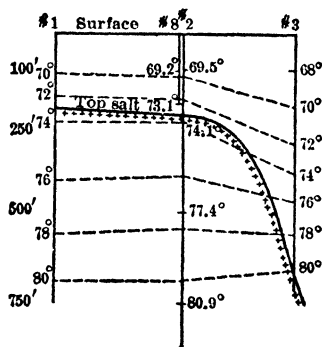
Fig 59. Isothermal Profile across South Edge of Grand Saline Salt Dome, Texas (26)
