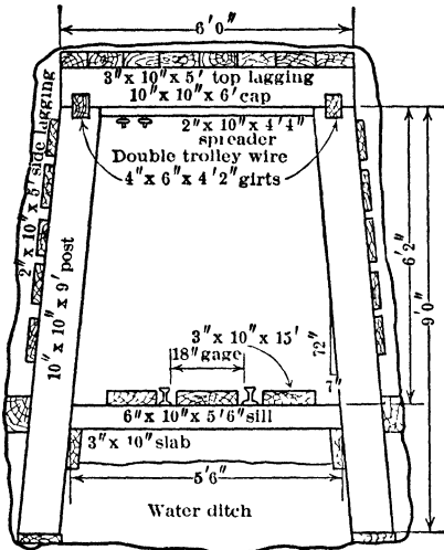
Fig 17 Drainage Tunnel Set with Ditch under Track
