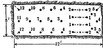
Fig 151. End V-cut, Wright-Hargreaves Mine, Kirkland Lake, Ont Holes average 4.5 ft deep
