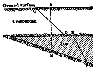
Fig 699 Limits of Power-shovel Pits, Mesabi (G. J. Young)
