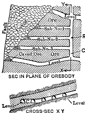
Fig 530. Mercur, Utah. Sub-level Caving
