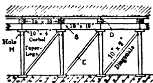
Fig 408. Crosscut Timbering, Broken Hill, N S W
