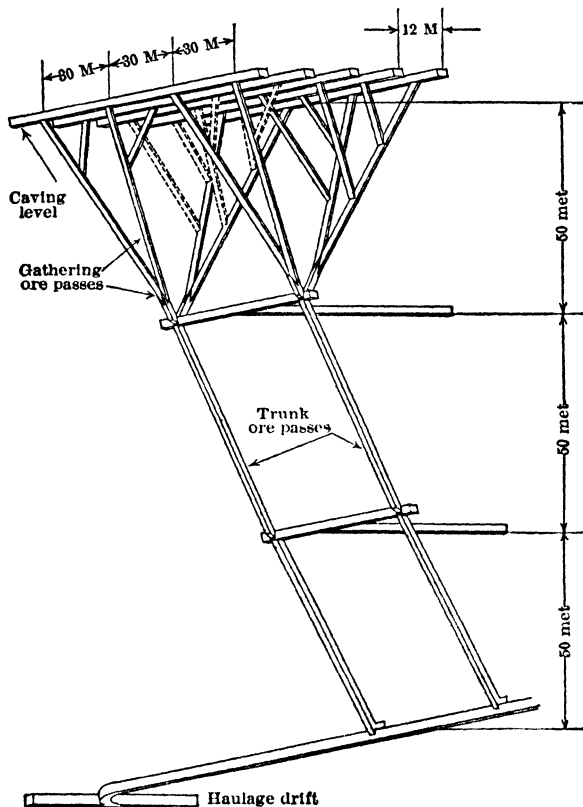
Fig 557. Ore-pass System, Braden Mine, Sewell, Chile (289)
