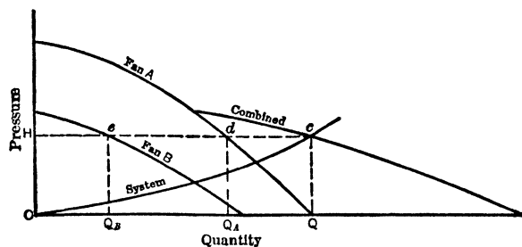
Fig 51. Two Fans acting together in Parallel (9)
