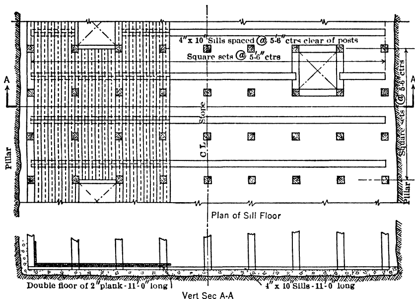
Fig 341 Sill Flooring, Frood Mine, Sudbury, Ont
