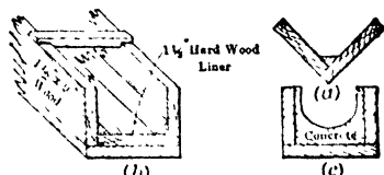
Fig 660. Launders for Handling Sand Underground (Rand)
