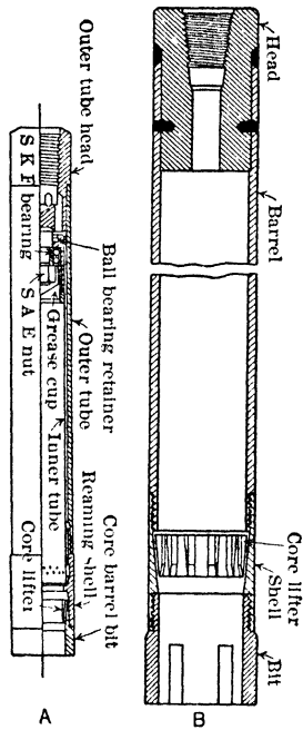
Fig 43 Core Barrels
