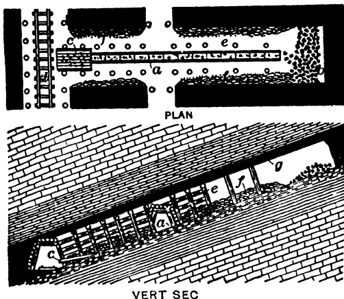
Fig 712. Chute Breast (Coal Miners' Pocketbook). a , Sheet-iron chute c , Loading platform. e , Props f , Gob g , Top coal
