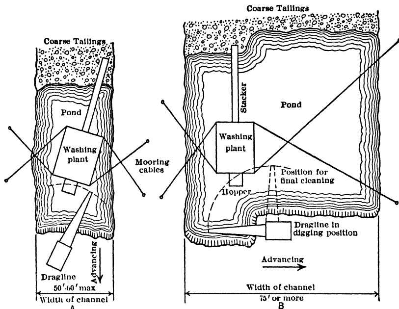
Fig 856 Two Procedures in Dragline Dredging
