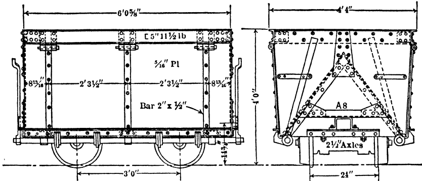
Fig 13. Gable-bottom Car, 47 cu ft Capac (Oliver Iron Mining Co)
