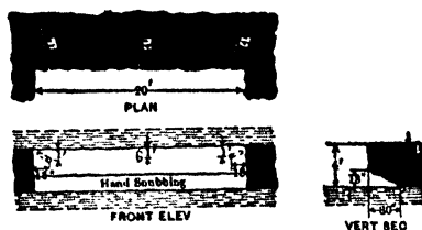
Fig 778. Mode of Placing Shots after Hand Snubbing
