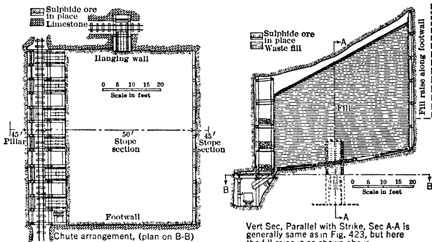
Fig 424. Inclined Cut-and-fill Stope, showing former use of Single Lead running parallel with Section Lines, Campbell Orebody, Warren, Ariz (91)
