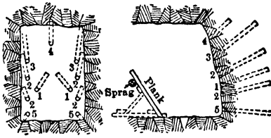
Fig 138. Inverted Draw-cut
