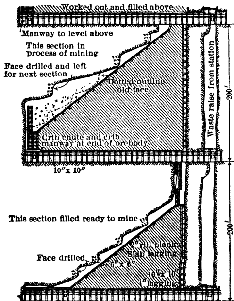
Fig 417. Ideal Longit Sec of Rill Stopes, Victoria Mine, Britannia Beach, B C (498)
