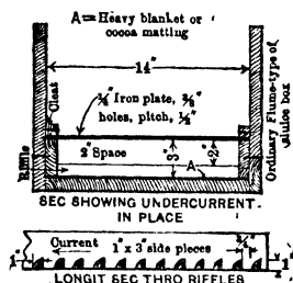
Fig 841 Undercurrent (after Ellis)
