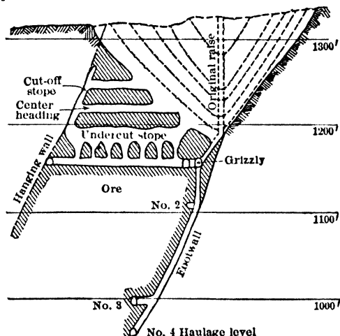
Fig 689. Vert Cross-sec through Glory-hole, Mt Isa, Queensland (500)
