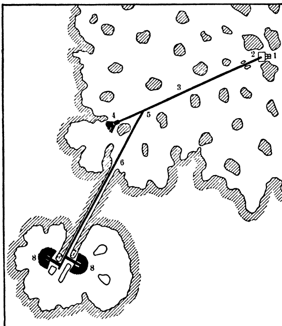
Fig 186. Part of D. C. & E. Mine, Oronogo, Mo, showing conveyer system and location of scrapers
