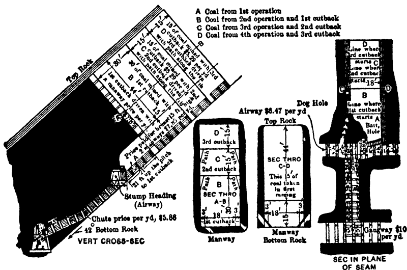
Fig 743. Cut-back in Breast 62, E Mammoth Seam, No 10 Shaft, L N C Co
