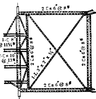
Fig 75. Horiz Sec of Frame, showing Guide Supports
