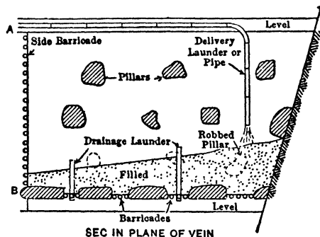
Fig 657. Sand Filling, Transvaal Gold Mines
