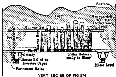
Fig 575. Ray Hand-trampling System
