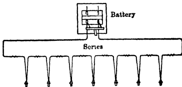
Fig 9 Series Wiring
