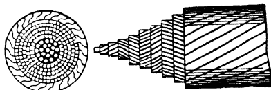
Fig 34. Locked Coil Hoisting Rope
