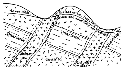
Fig 35. Sec of Veins Showing Geology Plotted on Walls (Solid Lines = Far Wall, Dotted = Near Wall. Shading Shows how Ore Shoots Occur only between Diabase Walls)
