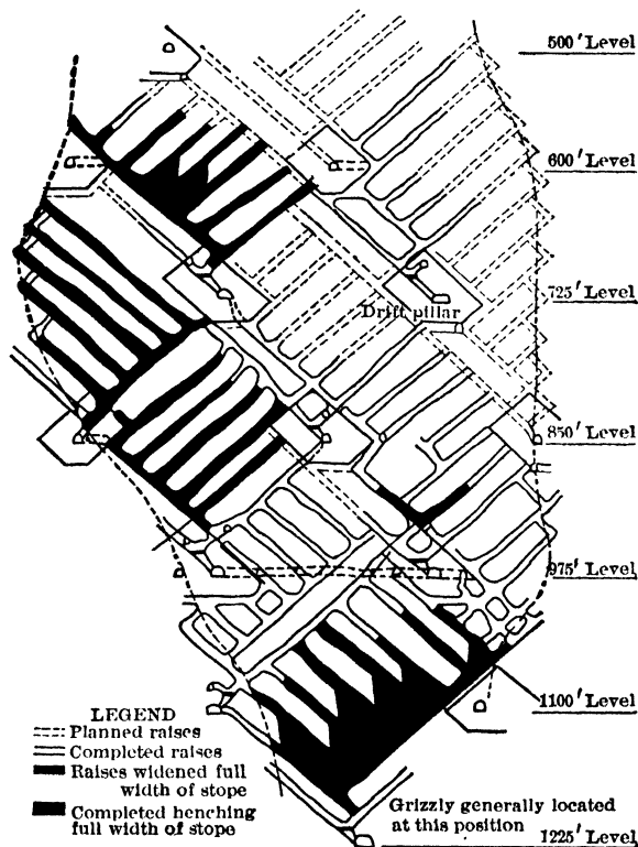
Fig 273. Longit Sec through a Stope Panel, "Upper H" Orebody, Horne Mine, Noranda, Quebec
