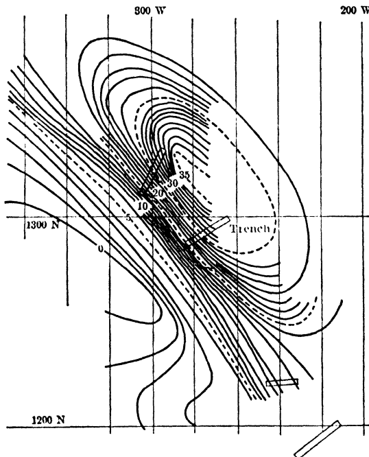
Fig 37. Equiphaser Curves in Electromagnetic Field over Orebody discovered Electrically (14)
