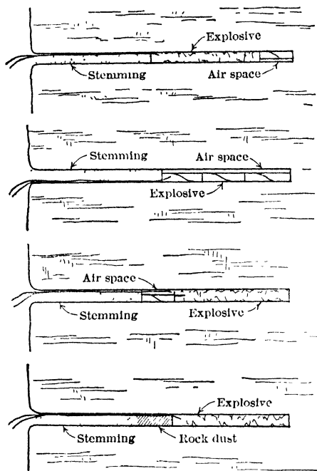
Fig 8. Modes of Charging for "Cushion" Blasting
