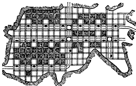
Fig 448. Cresson Mine, Plan of 600-ft Level (Fig 449)
