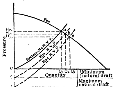
Fig 49. Fan Characteristic used as Combined Characteristic for Fan and Natural Draft (9)
