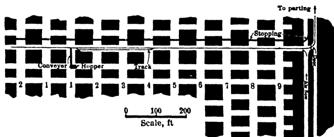
Fig 735. Mining System, Moffat Mine, Ill (634)
