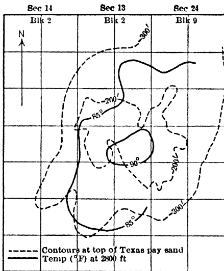
Fig 60. Stratigraphic and Isothermal Contours of Part of Big Lake Oil Field, Texas. Adapted from E. M. Hawtof (26)
