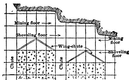
Fig 311. Wing-chutes, or Slides
