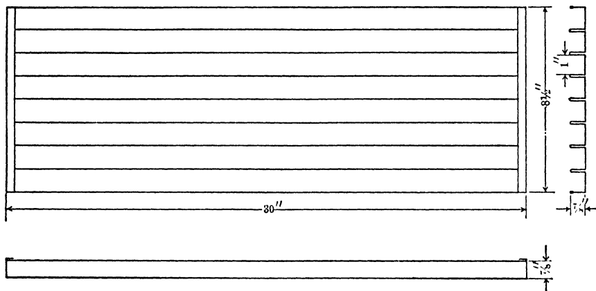
Fig 77. Galvanized-iron Core Box
