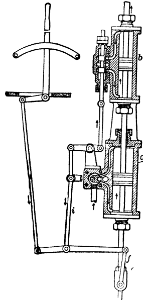
Fig 20. Auxiliary for Hoisting Engine Control
