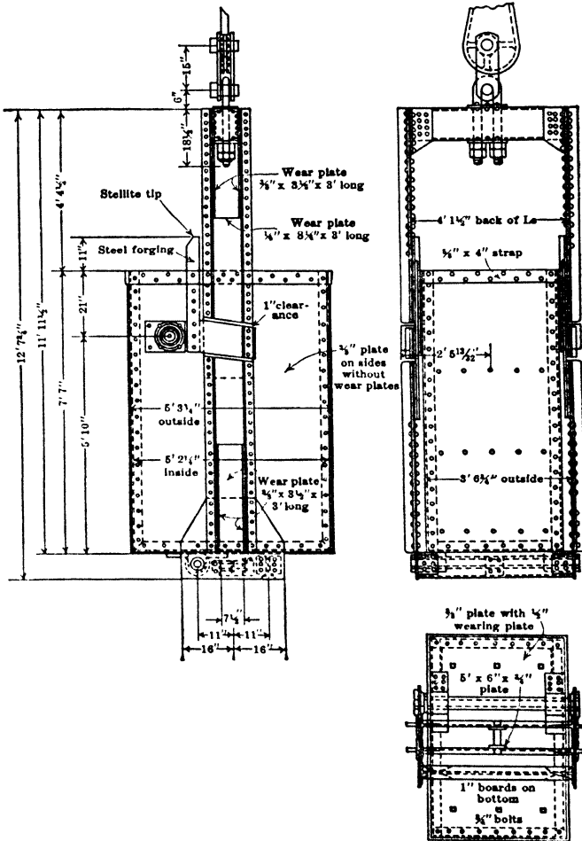
Fig 130 9-ton Kimberley-type Skip, Montreal Mining Co, Wis (80)
