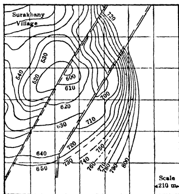
Fig 45. Example of Stratigraphic Contouring by Resistivity Logs (19)
