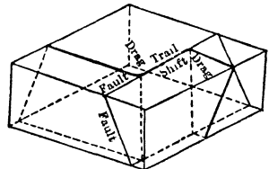
Fig 8 Shift Fault in Vein Dipping 50°. Same Effect would be Produced by Normal Fault, with Diagonal Displacement Involving Shift Component Away from Observer, or by a Large Throw, Straight Down the Dip
