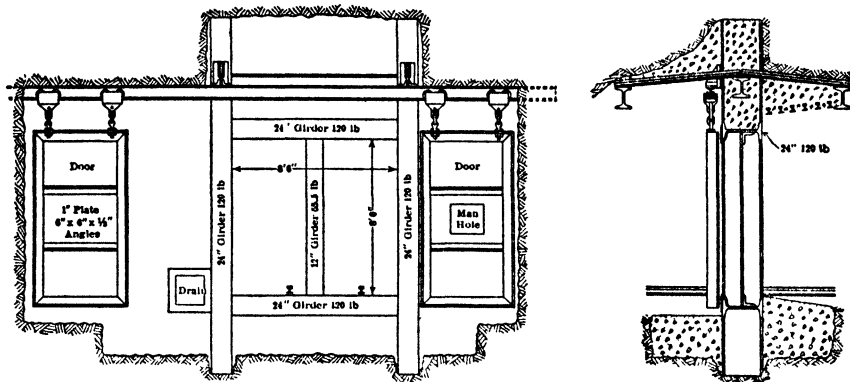
Fig 4. Emergency Flood Dam (for 45-ft Head), Lehigh Nav Coal Co, Tamaqua, Pa
