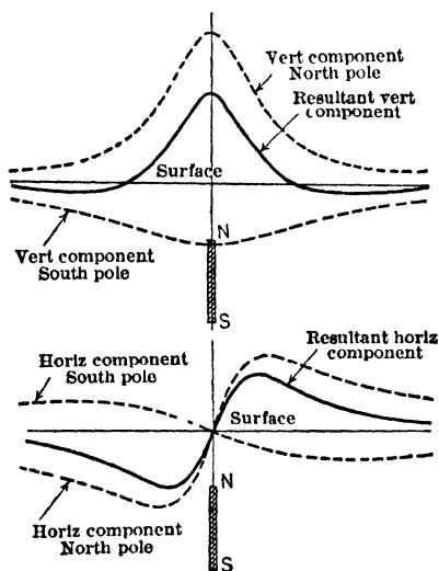
Fig 14 Theoretical Anomalies for Vert Dike of Finite Length (5)
