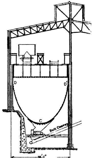
Fig 156 Suspension Mill Bin, Inspiration Copper Co
