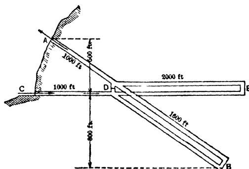
Fig 31 Simple Coal-mine Type of Split-flow Circuits
