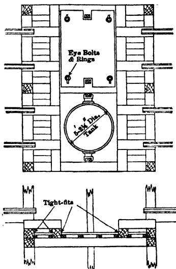
Fig 13. Platform at Bottom Level, No 4 Shaft, Lansford Mine (L Nav C Co)
