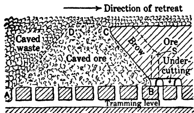
Fig 533. Humboldt Mine, Longit Vert Sec through Blocks (diagrammatic)
