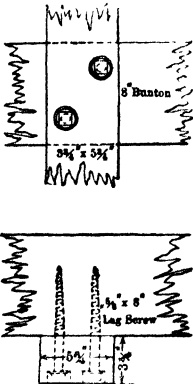
Fig 84. Fastening of Wood Guides
