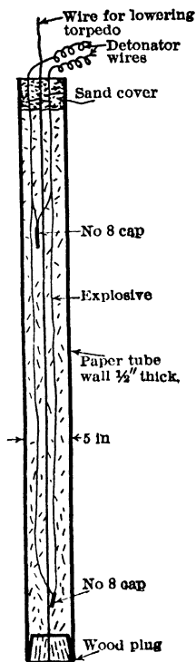
Fig 677. Sec of Torpedo for Blasting Hot Holes, United Verde Open-pit
