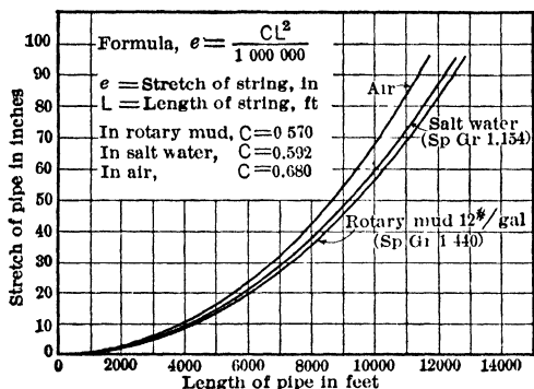
Fig 31. Stretch of Casing, Tubing, or Drill Pipe in Uniform Strings, freely Suspended in Various Fluids, without Float Plug ( Oil Weekly )
