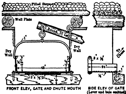
Fig 644. Chute-gate, Baltic Mine, Mich
