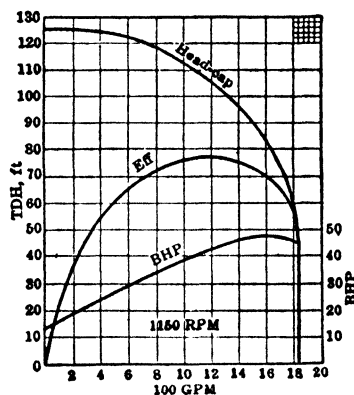
Fig 15. Characteristic Curves of a Centrifugal Pump
