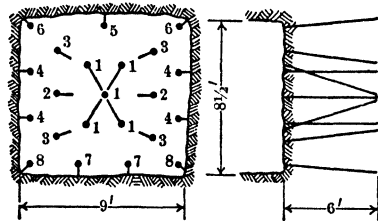
Fig 127. Pyramid Cut with Concentric Relievers, in Gneiss Mt Hope Mine, Mt Hope, N J
