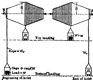
Fig 10 Design of Conical Drum
