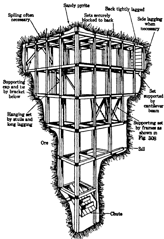
Fig 309. Briggs Method of Underhand Square-setting
