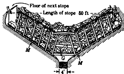
Fig 501. Coronado Mine, Ariz, Longit Sec through Slice
