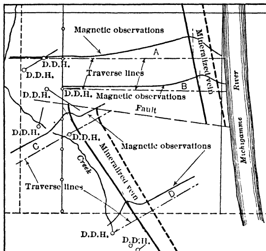
Fig 20. Detection of Horiz Faulting by Magnetic Anomalies (5)
