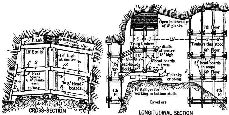
Fig 371. Recovering a Caved Stope Timbered by Stull Sets, Hecla Mine, Idaho (581)
