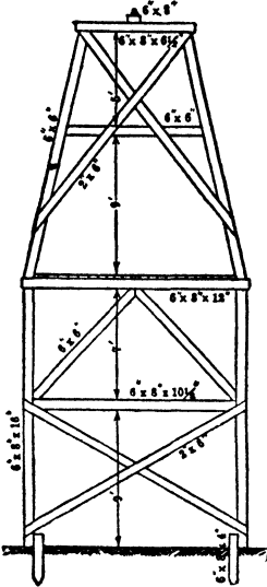
Fig 62. Small Joplin Type Headframe
