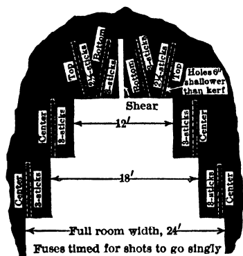
Fig 731. Breaking Coal in Peabody Coal Co Mine No 57, Ill (491)
