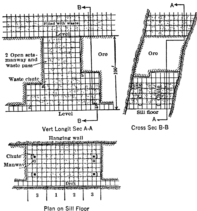
Fig 287. Block System (diagrammatic); numbers show order of mining blocks
