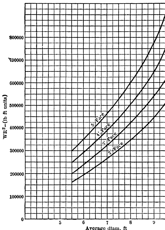
Fig 16. WR^2 of Conical Drums (double faced). For estimating purposes only. For gears, add 10%. (Gen Elec Co)
