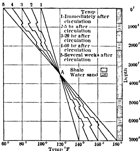
Fig 62. Probable Variation of Temp with Time Elapsed from Moment Circulation Ceased. Deep Wells (28)
