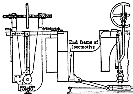
Fig 21. Locomotive Third-rail Brake
