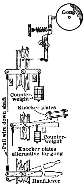
Fig 92. Bell Wire and Gong (37)
