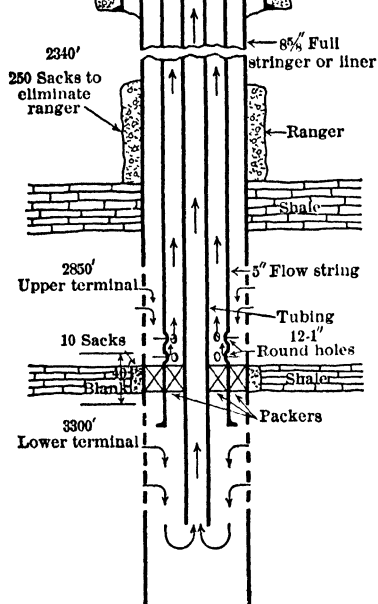
Fig 25. Multiple Zone Production ( Oil Weekly )
