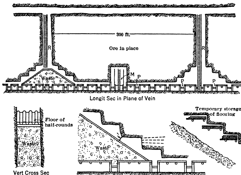
Fig 416. Filled Rill Stope, Wright-Hargreaves Mine, Kirkland Lake, Ontario
