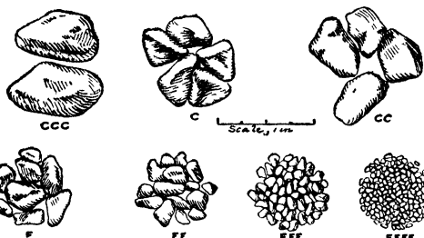
Fig 2 Standard Sizes of Black Powder Grains
