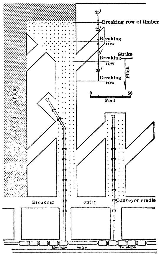
Fig 738. Room Work, D. O. Clark Mine, Wyo(636)
