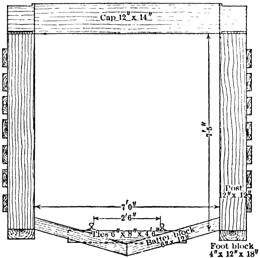
Fig 18. Set with Batter-blocks in Swelling Ground
