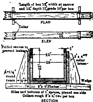
Fig 824. 14-in Telescoping Sluice Box, Fairbanks, Alaska (after Ellis)
