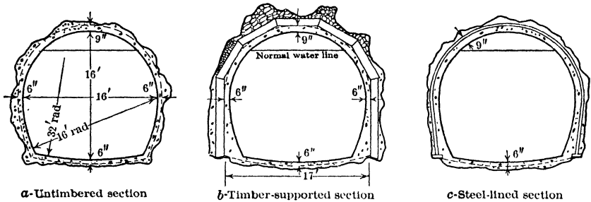
Fig 23. Typical Sections of Concrete Tunnel Lining, Colorado River Aqueduct
