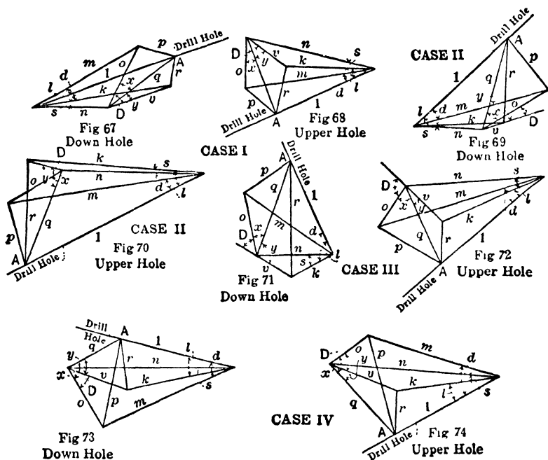
Fig 67-74. Various Combinations of Drill Hole and Bed ( E & M Jour )
