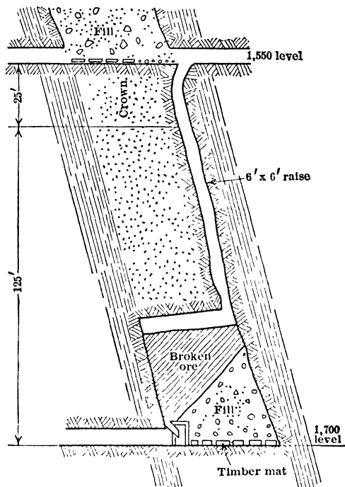
Fig 453. Cross-sec through Stope in Narrow Ledge, Homestake Mine, Lead, So Dak
