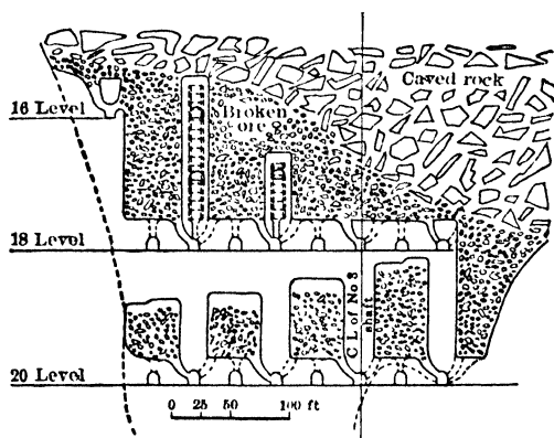
Fig 454. Longit Sec showing Crosscut and Chute-raise Arrangement, Creighton Mine, Ont
