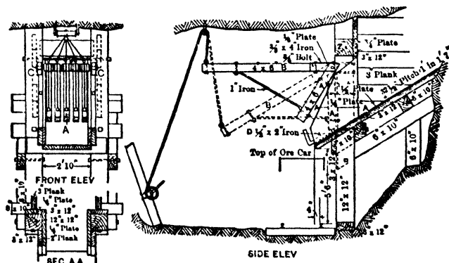
Fig 641. Finger Chute, Alaska Treadwell Mine
