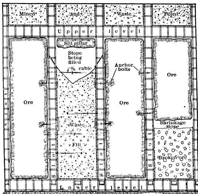
Fig 605 Method of Mining Pillars between Slots, and Tying Slot Timbers, Golden Queen Mine (310)
