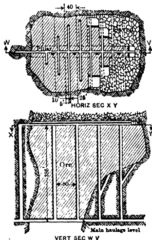
Fig 492 Panel Slicing, Arizona Copper Co (faces under attack shown thus —)
