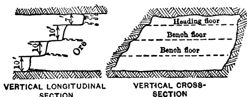
Fig 188. Breast Stoping, Wis Zinc Dist
