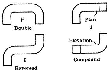
Fig 23. Types of Right-angle Bends (9)
