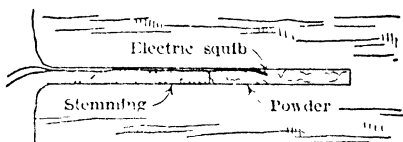
Fig 17. Blasting in Coal with Black Powder; Middle Cartridge Primed with Electric Squib
