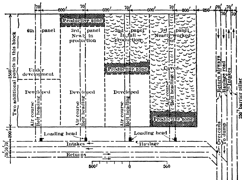
Fig 727. Mining System, MacAlpin Coal Co (490)
