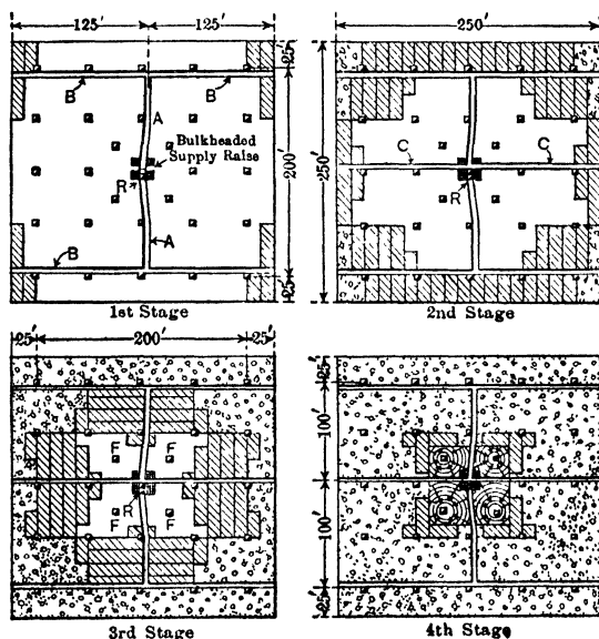
PLAN OF WORK ON 1 FLOOR AT DIFFERENT STAGES
