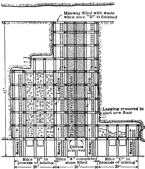
Fig 606. Square-set Shrinkage Stopes with subsequent Filling, Carson Hill Mine, Melones, Calif (297)
