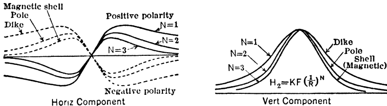
Fig 16. Variation in Magnetic Components for Dikes, Poles, and Shells (8)
