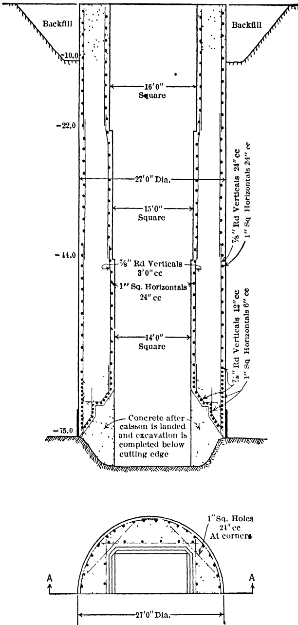
HALF PLAN Fig 8. Drop-shaft
