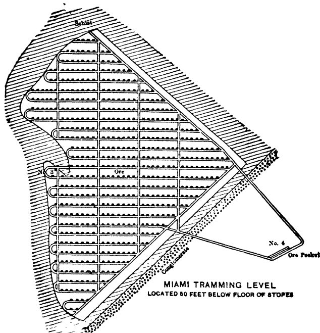
Fig 50a. Traming Level, Miami Copper Mine, Ariz (see Sec 10)
