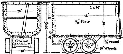
Fig 5. All-steel, Sub-level Car (Lake Shore Engine Works)
