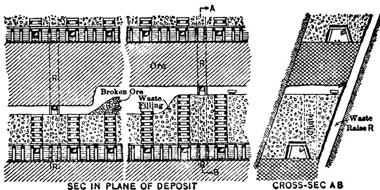
Fig 387. Filled Flat-back Stope, Minnesota Iron Co, Soudan, Minn
