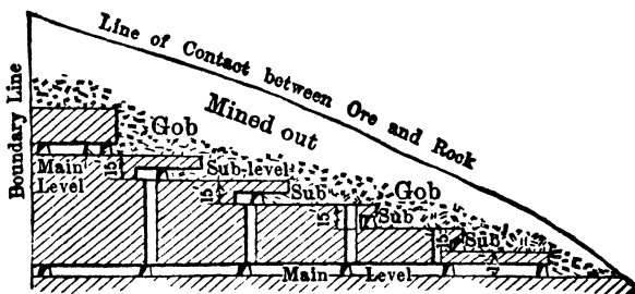
Fig 519 Newport Mine, Relation between Work on Sub-levels. (Vert longest sec, vert scale exaggerated)
