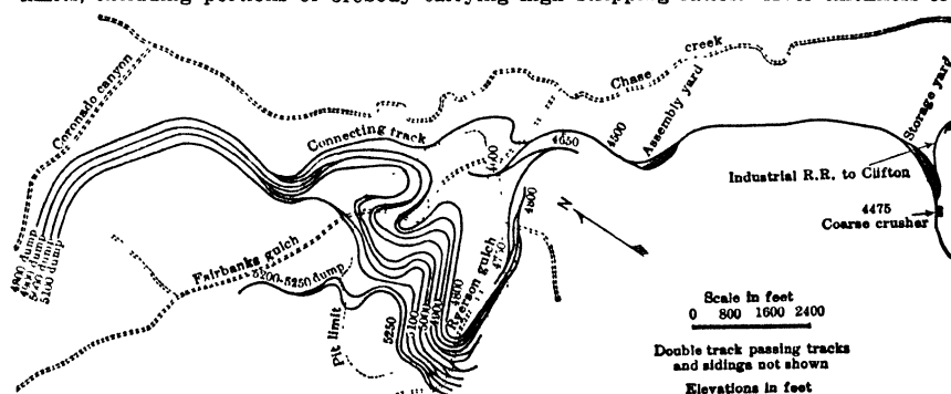
Fig 680. Layout of Pit, Morenci, Ariz
