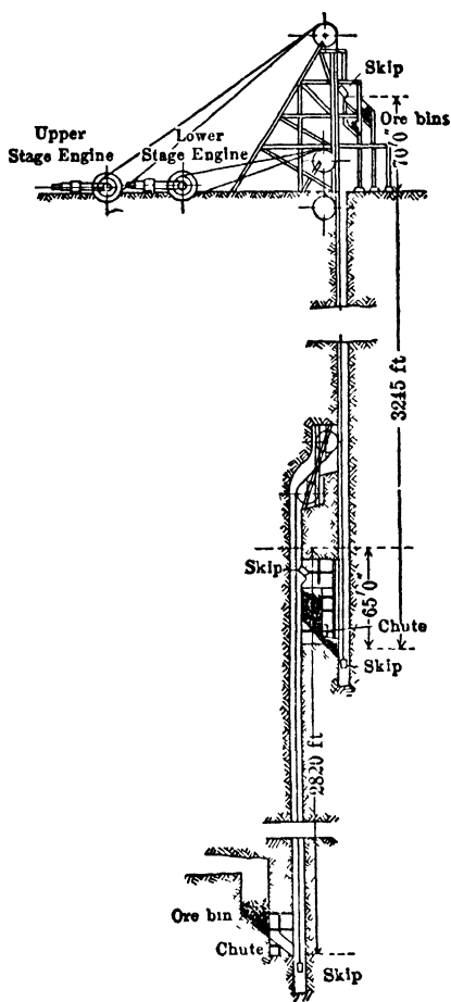
Fig 6 Two-stage Hoisting
