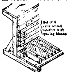
Fig 835. Rail Side Lining, La Grange, Cal
