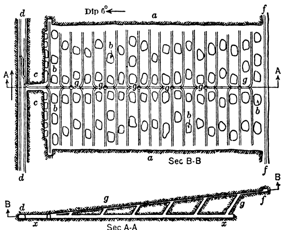
Fig 195 "Crosseut and Boxhole" Stope, East Rand. a , Stope faces. b , Waste packs. c , Safety pillars. d , Haulage level. f , Drift. g , Raises or "boxholes".
