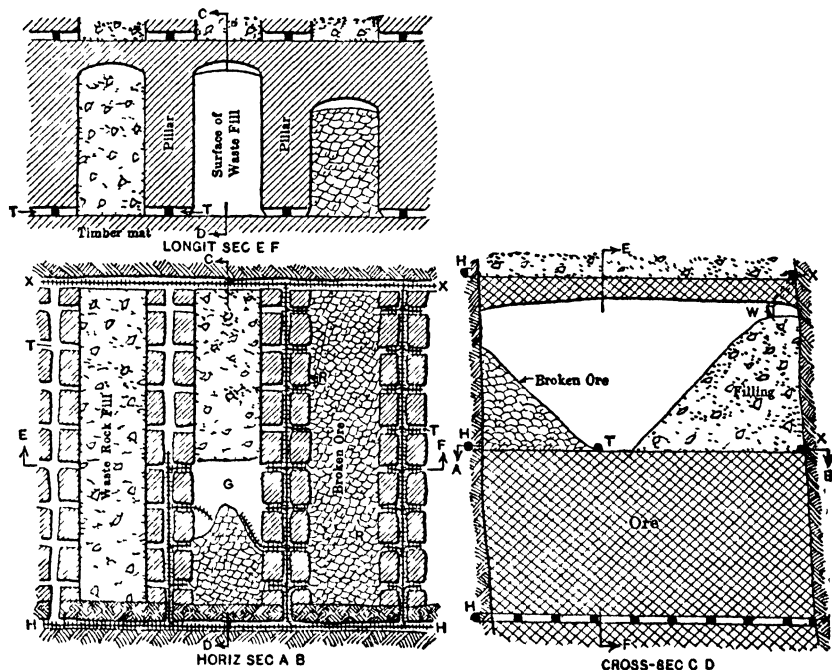
Fig 450 Shrinkage Stope, Homestake Mine, So Dak (former method)
