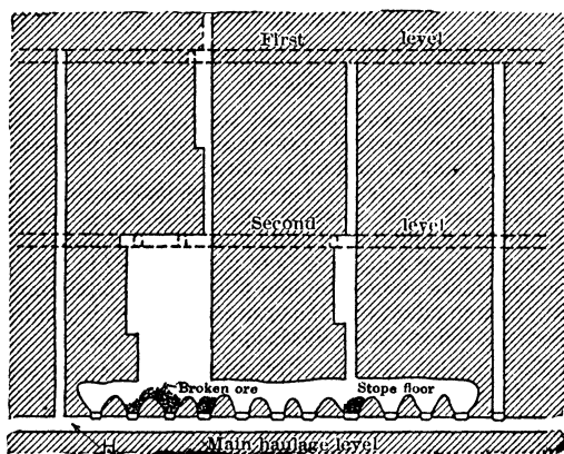
Fig 216. Underhand Stopping, Sherritt Gordon Mine, Manitoba. (Longit sec in plane of orebody)
