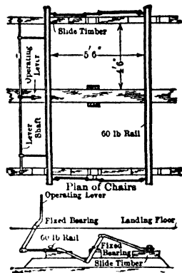
Fig 121 Desloge Landing Chairs (E & M Join)
