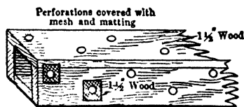
Fig 661. Drainage Launder for Sand Filling (Rand)
