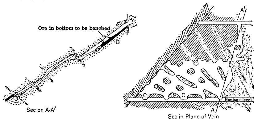
Fig 245. Overhand Stopping Method, Golden Messenger Mine, York, Mont (69)
