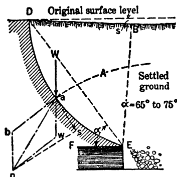
FED, Angle of "draw," as usually defined. EaD, "Plane of stability" EBD, Moving ground tending to slide Aa, Thrust of arch from caved ground Wa, Weight of strata an, Resultant thrust ns, Rubbing pressure on solid ground as, Slide component s, Subsidence
