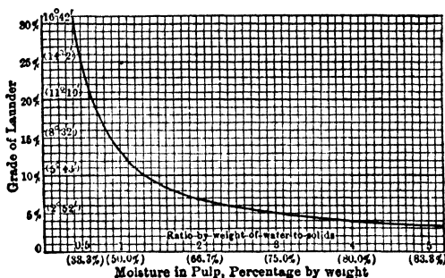
Fig 659. Launder Grades for Sand Pulp (Rand)
