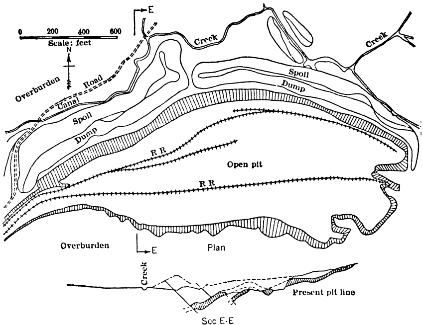
Fig 683. Open-pit Mining with Dragline, Cristo, Cuba
