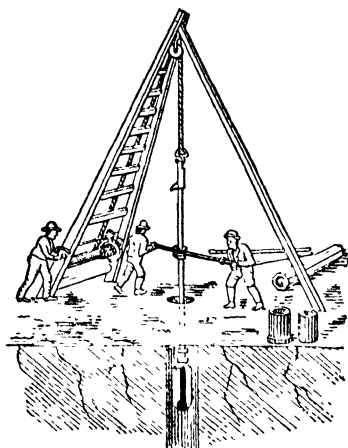
Fig 3. Well Borer Operated by 3 Men
