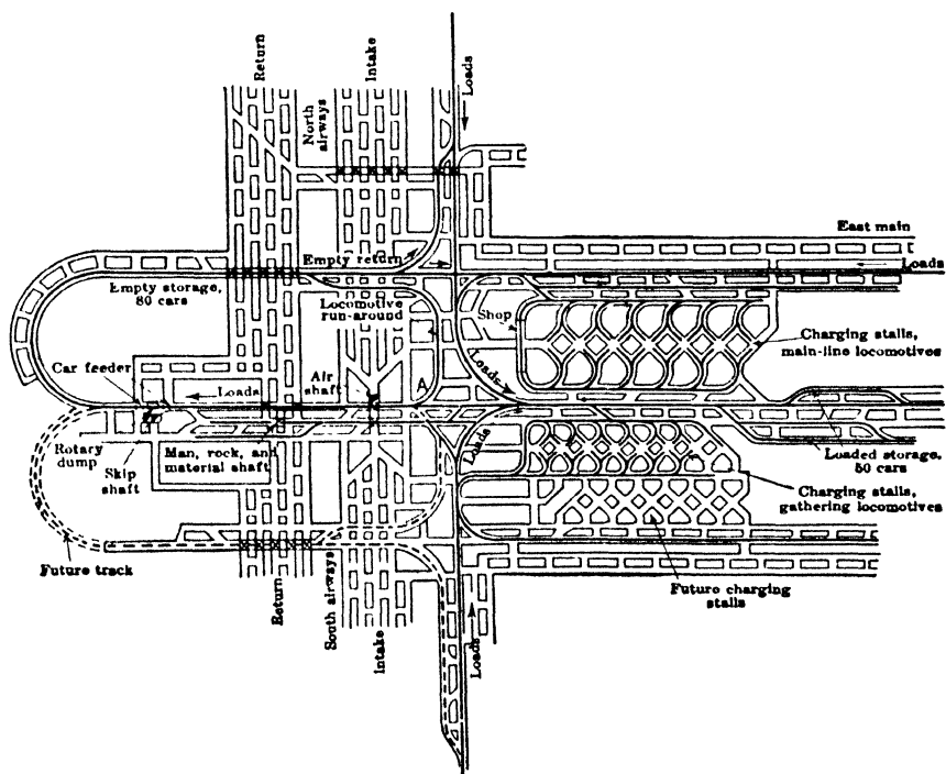
Fig 51. Shaft-bottom Layout, W Va Coal Mines (24a)
