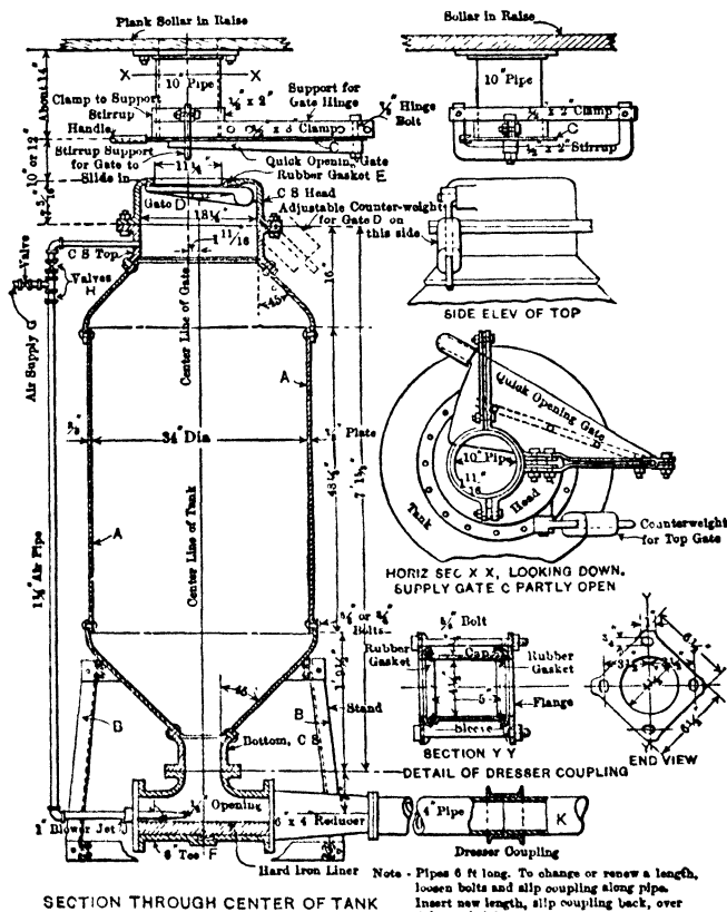
Fig 405. Sand-blowing Tank, Champion Mine, Mich (F. W. Denton)
