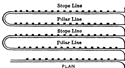
Fig 580 Miami Method, Part of Trimming Level
