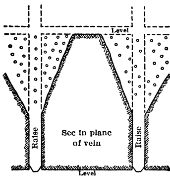
Fig 212. Underhand Stoping, Pilgrim Mine, Chloride, Ariz
