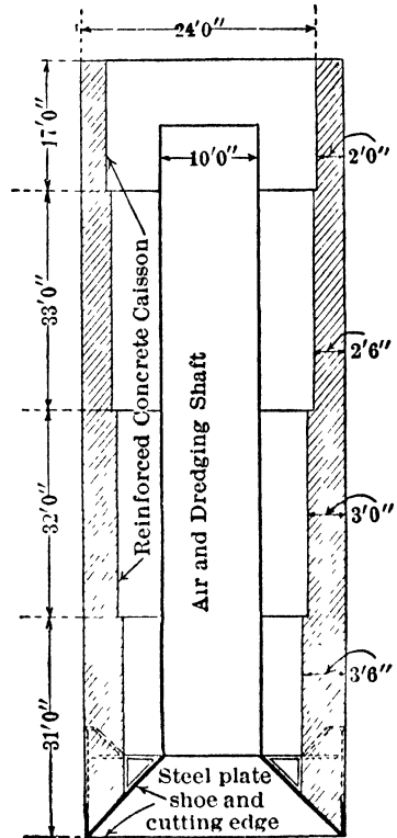
Fig 16 Caisson for Kidder Shaft, Cleveland-Cliffs Iron Co
