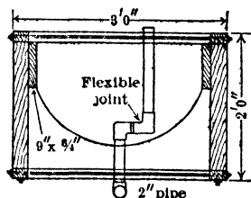
Fig 83. End Elevation of Sludge Box
