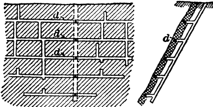
LONGIT SEC IN PLANE OF VEIN
