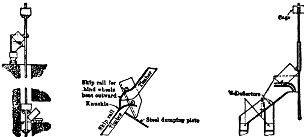
Fig 134. Arrangements for Loading and Dumping Skips
