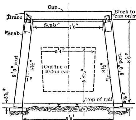
Fig 16. Three-piece Tunnel Set
