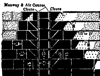
Fig 746. Mining Method, Tesla, Calif (Coal Miners' Pocketbook)
