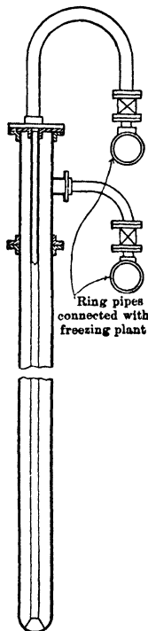
Fig 19 Freezing Pipes, Dawdon Colliery, England
