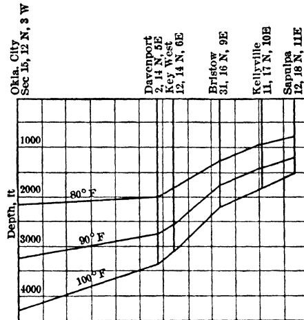
Fig 61. Temperature Profile, Oklahoma City to Sapulpa (27)
