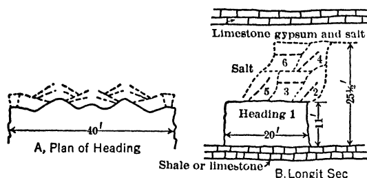
Fig 201. Breaking Ground in Detroit Rock Salt Mine
