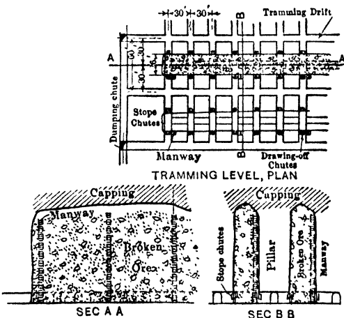
Fig 567. Boston Mine, Hand-tramming System; Chutes on Both Sides of Stope
