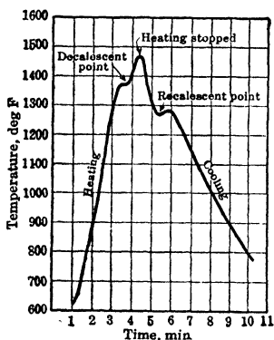
Fig 2. Critical Temperatures for High-carbon Steel (Steel and its Treatment, E F Houghton & Co)
