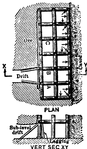
Fig 480. Boarding-up Rooms and Blasting Timbers, Mesabi Square-set Slicing
