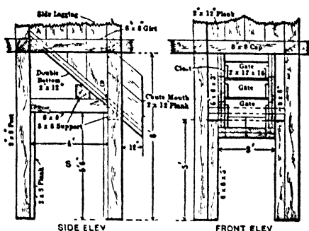
Fig 631. Chute-gate in Square-sets, Bingham, Utah
