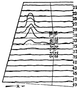
Fig 23. Layout of Traverse Lines for Survey by Potential Method (9)
