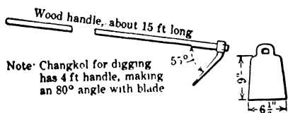
Fig 875. Changkol used in Lanchutes and Palongs
