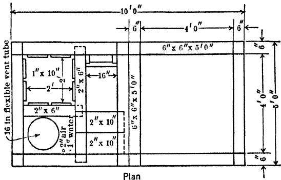
Fig 163. Cribbed Raise, Magma Mine, Superior, Ariz
