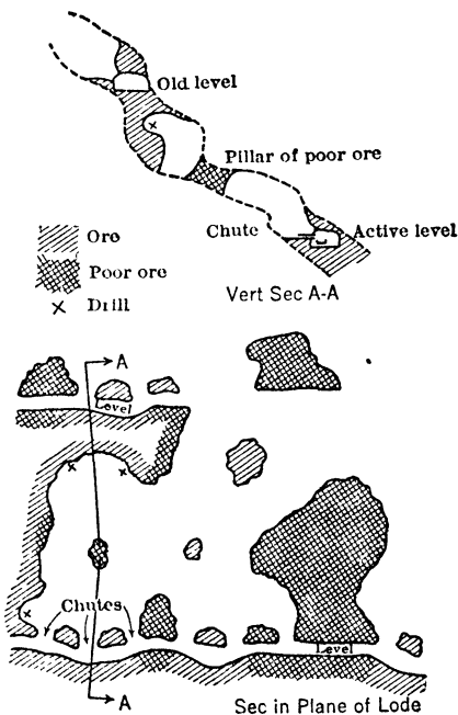
[ Fig 251. Open Stope, Osceola Lode
