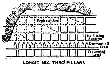
Fig 587. Miami Method, Mining Pillars
