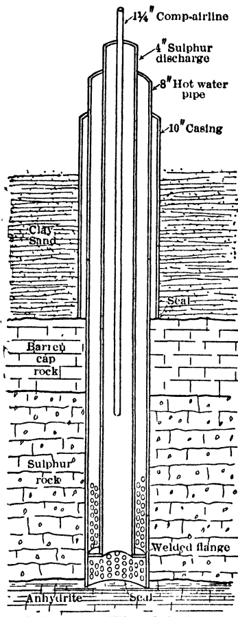
Fig 617. Arrangement at Bottom of Frasch Sulphur Well. (Diagrammatic sec, not to scale)
