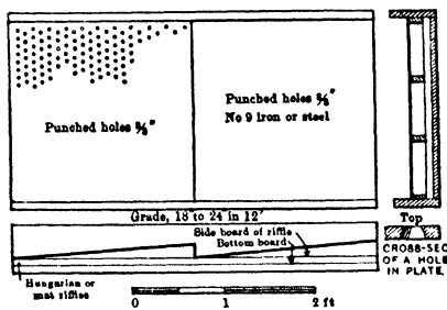
Fig 842 Caribou Undercurrent (after Purington)
