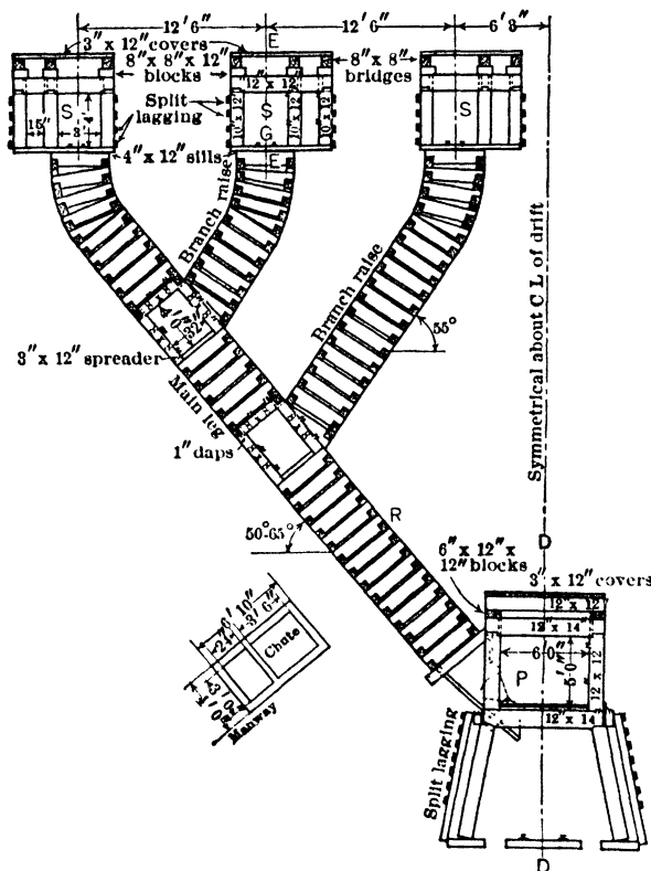
Fig 553. Raise-chute System, Ruth Mine, Nev
