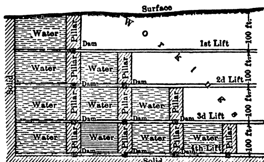
Fig 7. Series of Dams, with Counterbalanced Pressures
