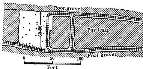
Fig 863. Development for Breasting, Vallecito Western Mine (18)
