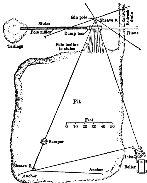
Fig 812. Slip Scraper dragged up Incline
