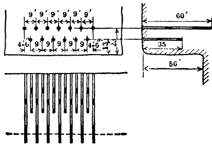
Fig 25. Arrangement of Holes on High Face to Reduce Secondary Blasting
