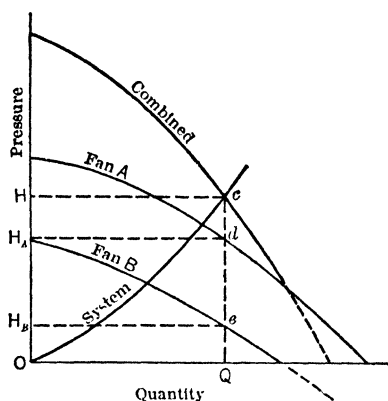
Fig 50. Two Fans acting in Series (9)
