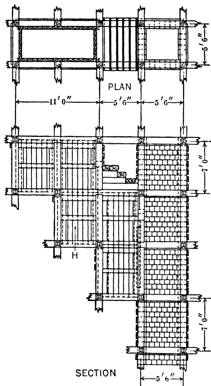
Fig 295. Method of Offsetting Chutes, and Use of "Bricking" as Lining, Frood Mine, Ont
