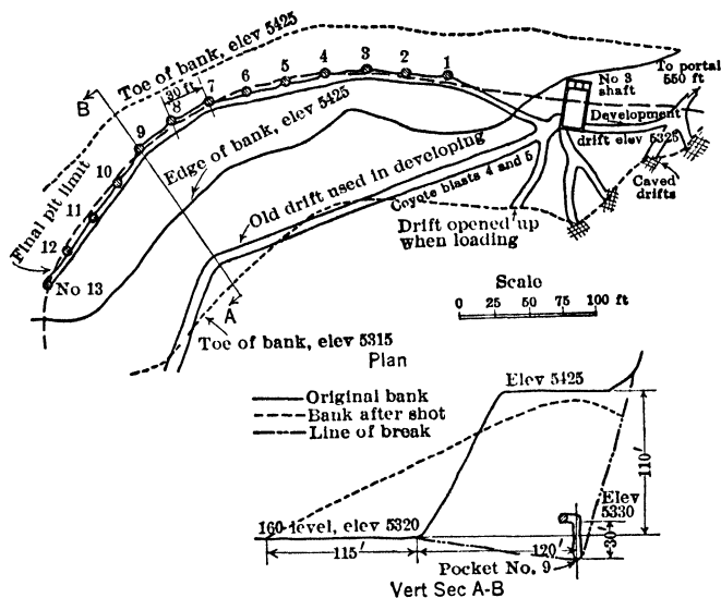
Fig 676. Development for Coyote Blast No 6, United Verde Open-pit
