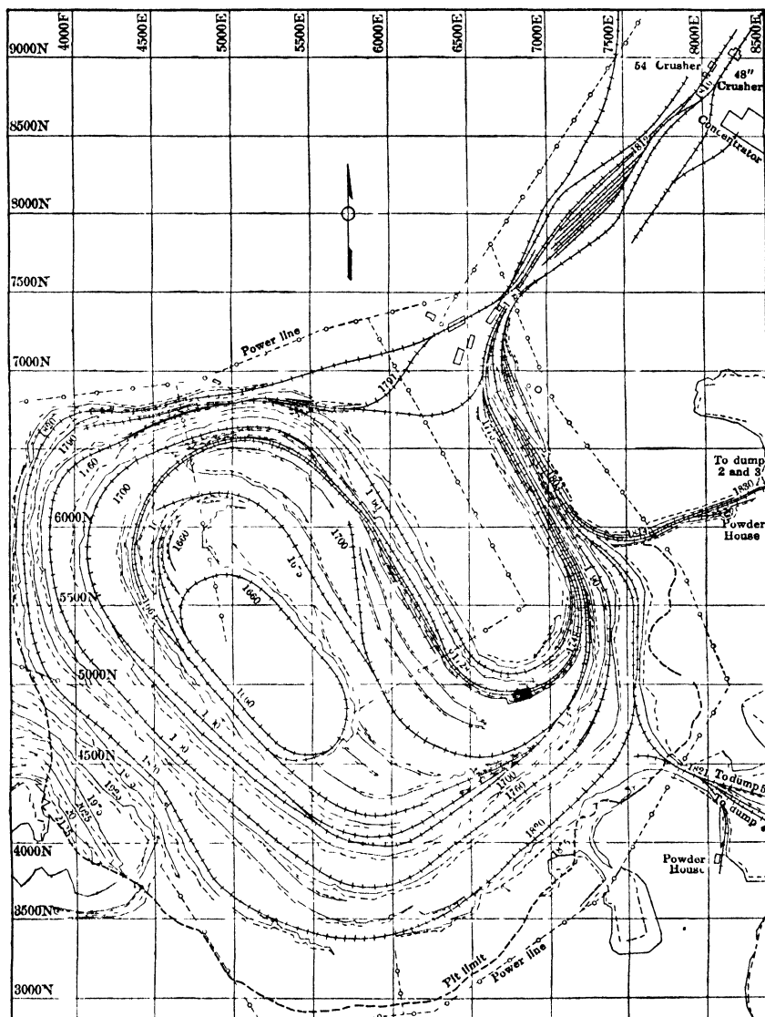
Fig 678 New Cornelia Open-pit, Ajo, Ariz, as of Jan 1, 1939
