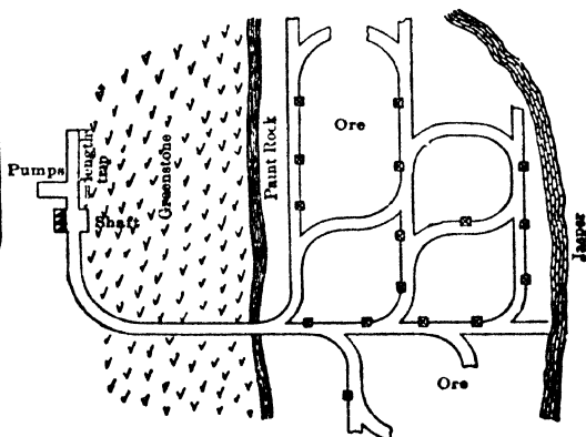
Fig 50. Locomotive Haulage Level, Ely, Minn
