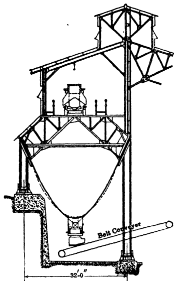
Fig 159. Suspension Bin, New Cornelia Copper Co, Ajo, Ariz (E & M J)
