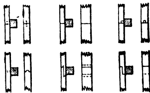
Fig 89. Joints for Wooden Guides
