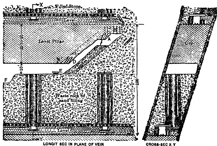
Fig 404. Mining Level-pillars, Baltic Method (Diagrammatic Sections)
