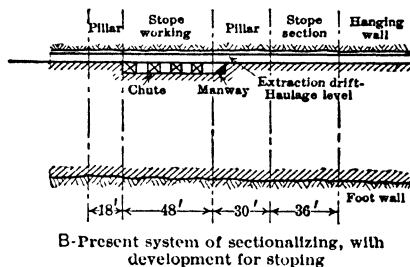
Fig 422 Systems of Dividing Orebody into Stope and Pillar Sections, Campbell Orebody, Warren, Ariz
