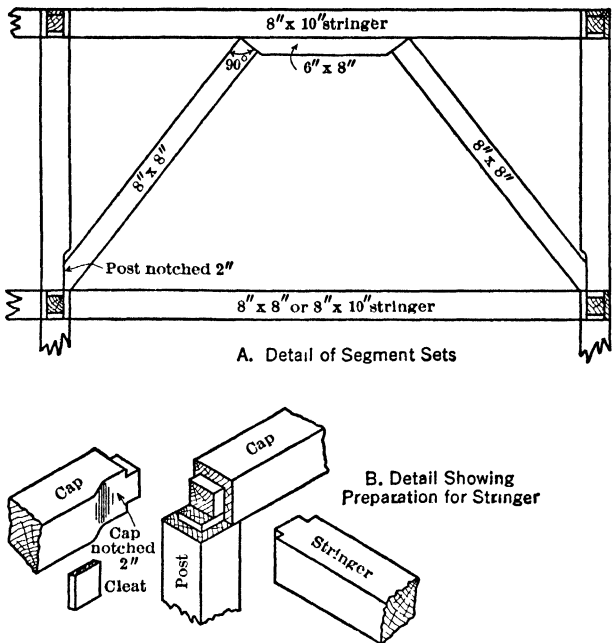
Fig 360. Details of Timber Framing for Mitchell Slicing System
