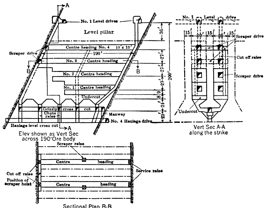
Fig 283. Transverse Sub-level Stope, Mt Isa Mines, Queensland (500)
