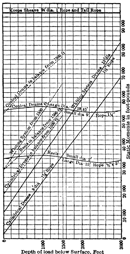
Fig 14. Static Hoisting Moments
