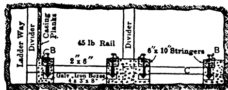
Fig 91a. Copper Range Skip Track (Cross-sec on E-F, Fig 91)
