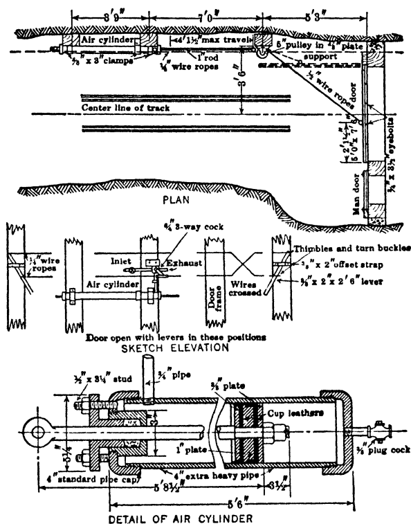
Fig 5. Device for Operating Ventilation Door by Comp Air, Metal Mines (31)
