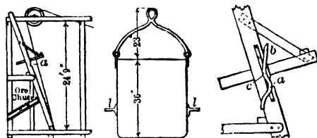
Fig 107. Automatic Dump for Inclines
