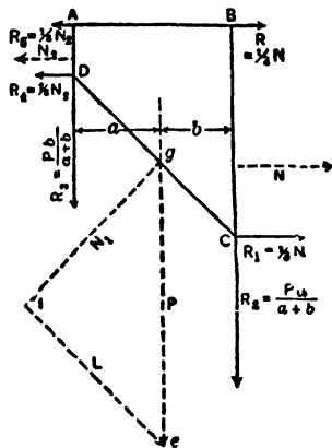
Fig 164 Stresses in Bin Framing
