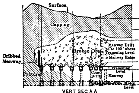
Fig 574. Ray Hand-trampling System
