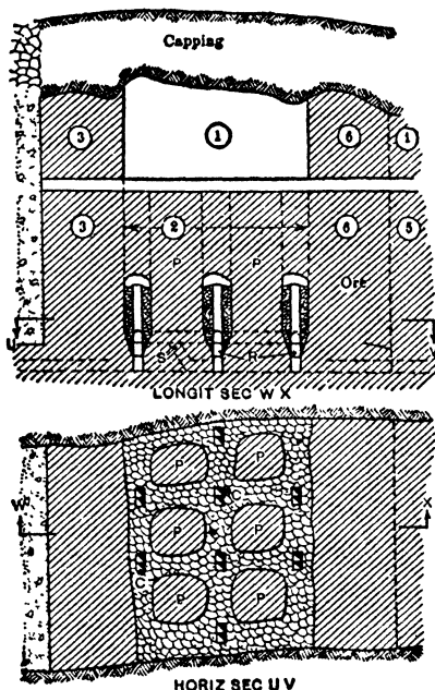
Fig 596. Duluth Mine, Pillar-caving in Block No 2, Fig 595
