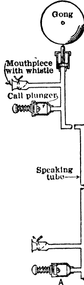
Fig 93. Pneumatic Bell and Speaking Tube Systems (37)
