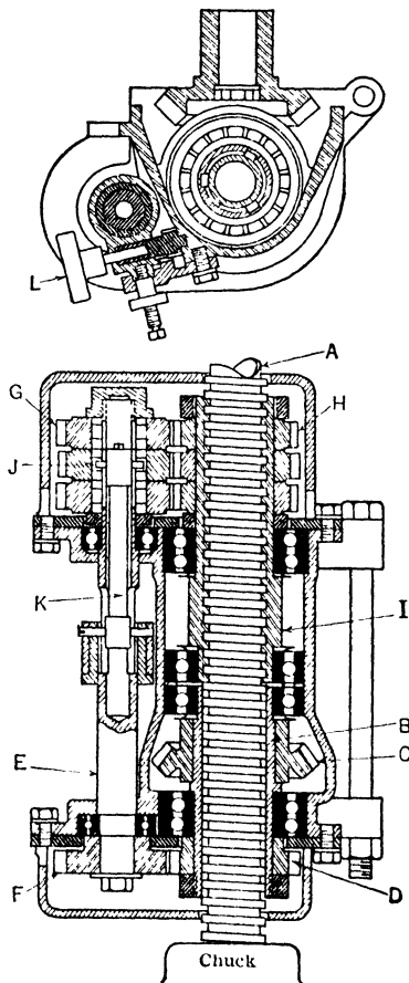
Fig 46 Differential-gear Screw Feed (Sulphur Machy Co)
