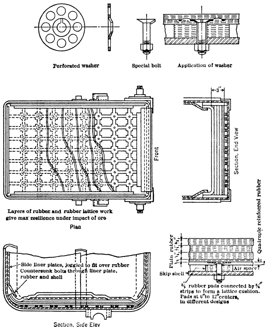
Fig 131. Rubber Skip Lining (37)
