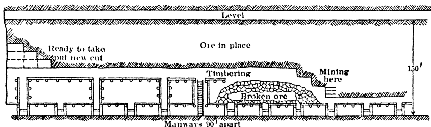
Fig 238. Open Overhand Stope, Wright-Hargreaves Mine, Ont. (Longit sec in plane of vein)
