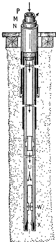
Fig 42 Boring Column of Diamond Drill
