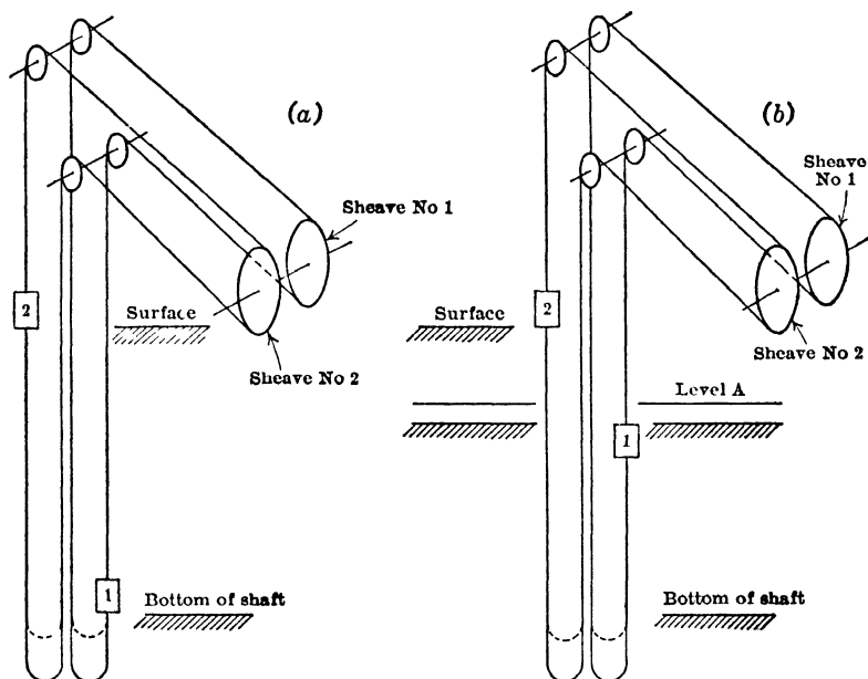
Fig 4 Diagram of Ohnesorge System for Hoisting from Different Levels ( E & M Jour )
