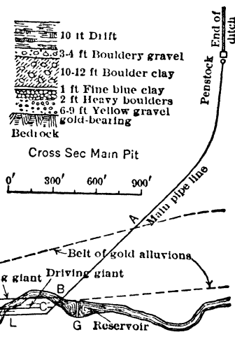
Fig 816. Hydraulic Mine near Beauceville, Quebec
