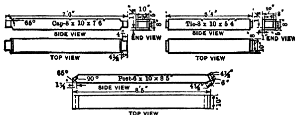
Fig 365. Details of Timbers, Moore System
