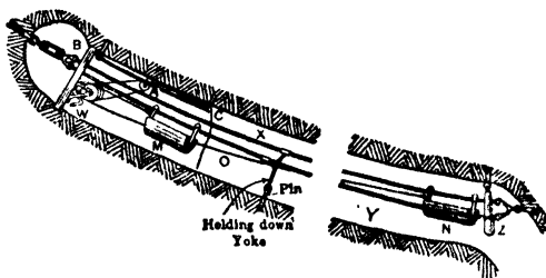
Fig 653. Aerial Ropeway for Stope Transport
