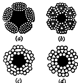
Fig 32. Flattened-strand Wire Ropes
