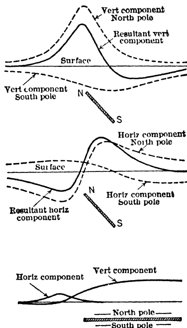
Fig 15 Theoretical Anomalies for Dikes of Finite Length (5)
