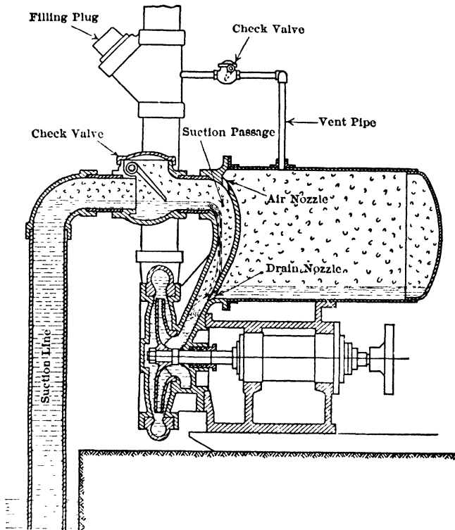
Fig 18. Hazleton Auto Station Pump
