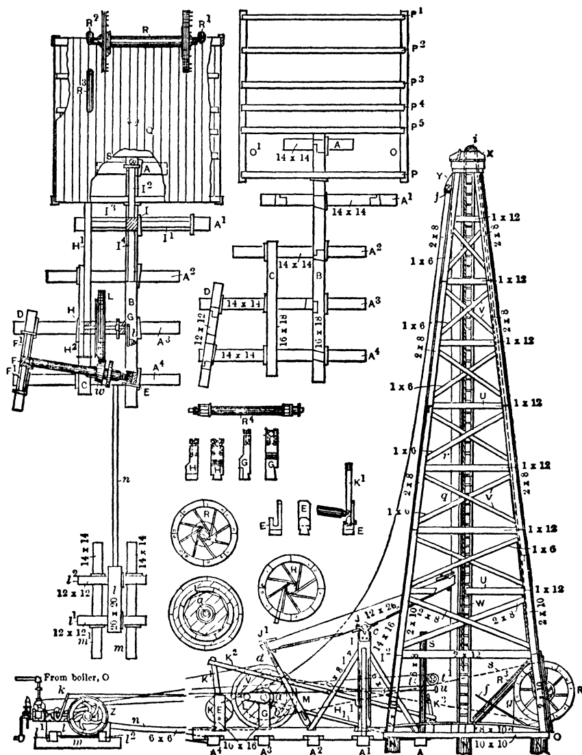
Fig 12. Standard Oil-well Rig
