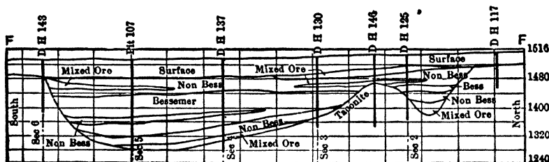
Fig 97. Section FF on Fig 96
