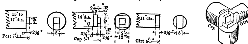
Fig 331. Sill-floor Set, Clark Mines, Butte, Mont
