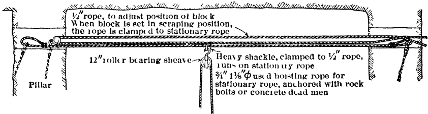
Fig 268 "Aerial Rig" for Scraper Sheave, Roan Antelope Mine, Nor Rhodesia
