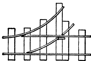
Fig 35. Grade Frog with Latch
