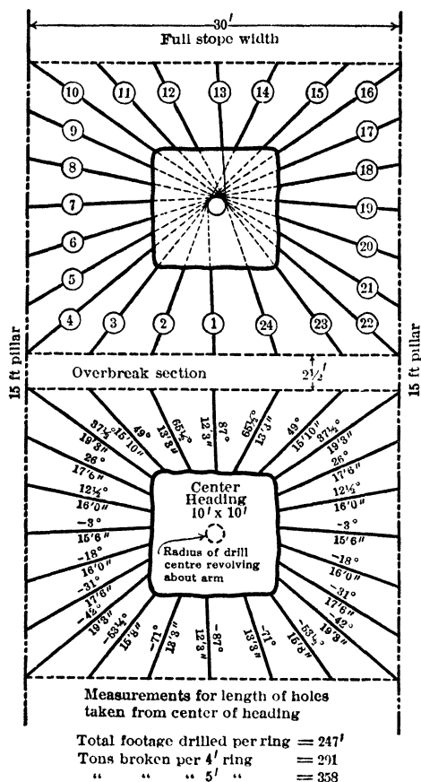
Fig 284. Ring-drilling Diagram for Transverse Stope, Mt Isa Mines, Queensland
