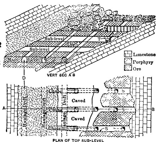
Fig 531. Mercur, Utah. Sub-level Caving
