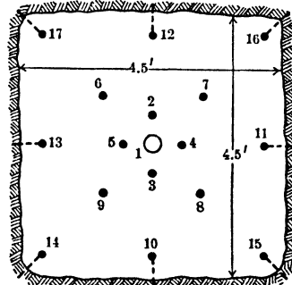
Fig 152. Burned Cut, Franklin Mine, Franklin, N J. Holes 8.5 ft deep. Center hole not loaded, others fired in sequence, as numbered, using fuses all of same length. Two rounds loaded and fired separately, Nos 2-9, Nos 10-17
