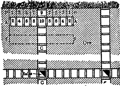
Fig 509. Slicing and Stripping Details
