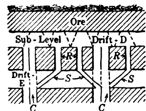
Fig 524. Vert Sec through Sub-level Drift (diagrammatic)
