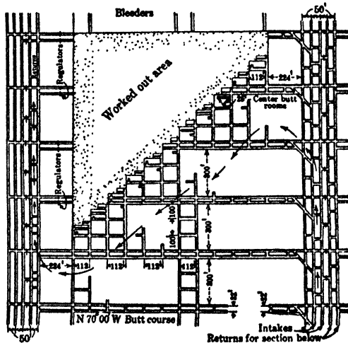
Fig 718. Standard Mining Method of Advancing and Retracting, Pittsburgh Seam, Connellsville Region, Penna (606)
