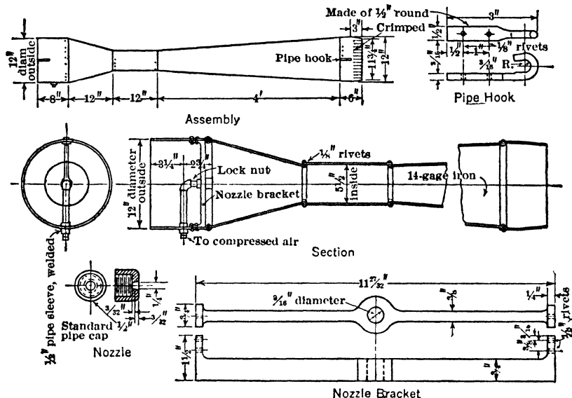
Fig 43. Modder Deep Type of Comp-air Injector (9)
