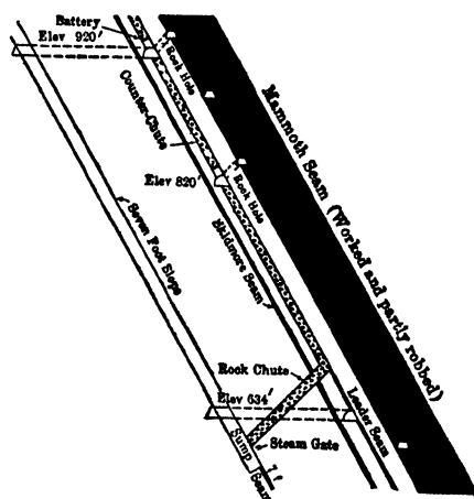
Fig 742 Counter-chute Method (Lawrence Colliery)
