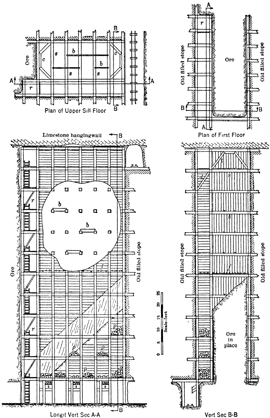
Fig 359. Mitchell Slicing System, Campbell Mine, Bisbee, Ariz
