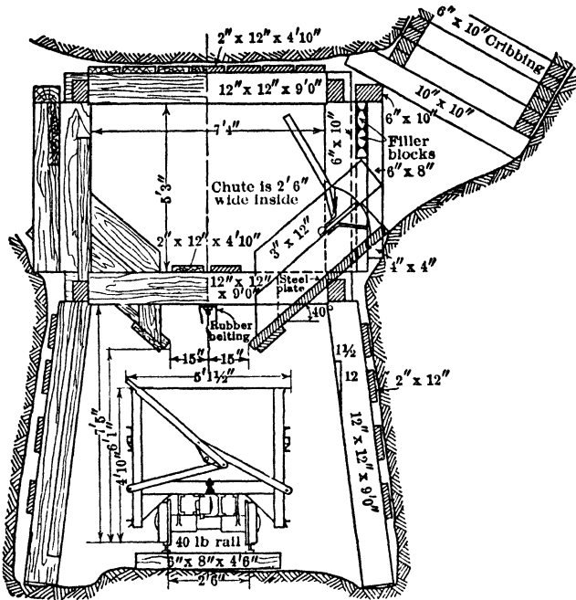
Fig 638. Overhung Arc Gate, Inspiration Mine
