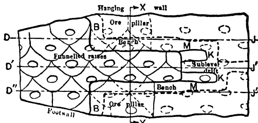
Fig 263. Plan of Sub-level Stope in Wide Orebody
