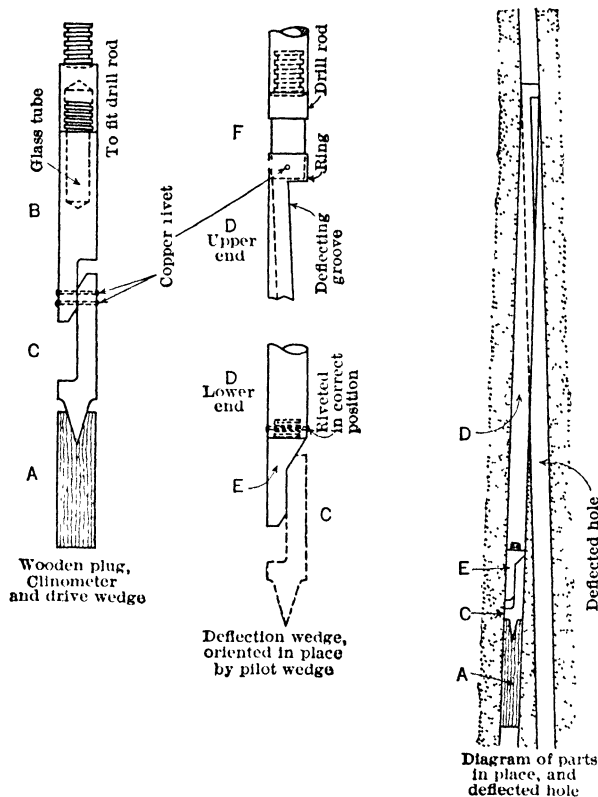
Fig. 38. Hall-Rowe Wedging Device (Canadian Inst Min & Metallurgy)
