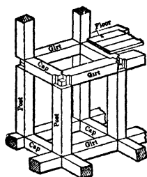
Fig 285. Square-set Timbering
