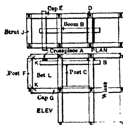
Fig 306. Details of Under-hand Square-setting
