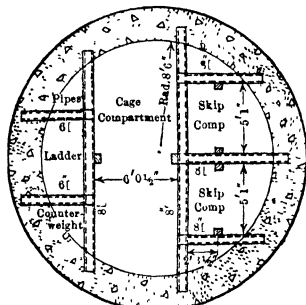
Fig 2. Circular Shaft
