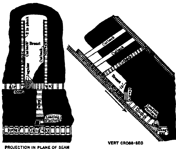
Fig 744. Cut-back System, Mammoth Seam, Penna
