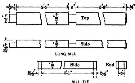
Fig 339. Sill Timbering, Homestake Mine
