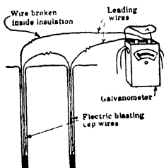
Fig 12 Testing Circuit with Galvanometer
