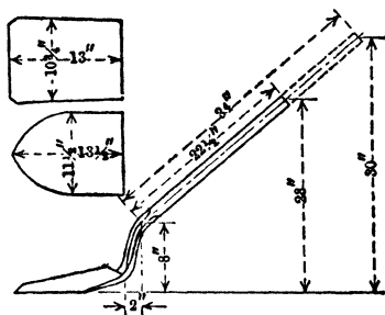
Fig 140. A Mining Shovel
