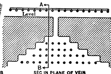
Fig 231. Stulled Stope
