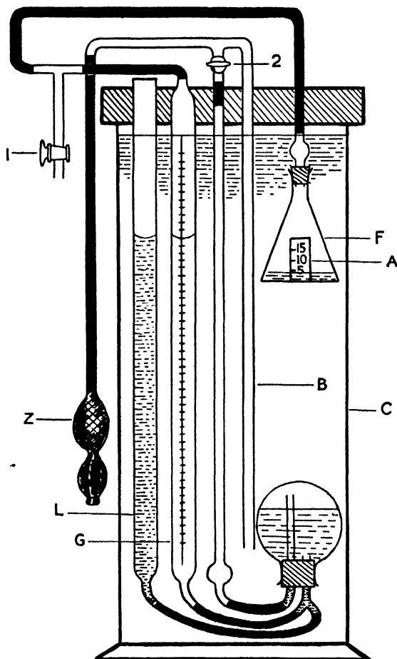
FIG. 2.—Collins' calcimeter.
