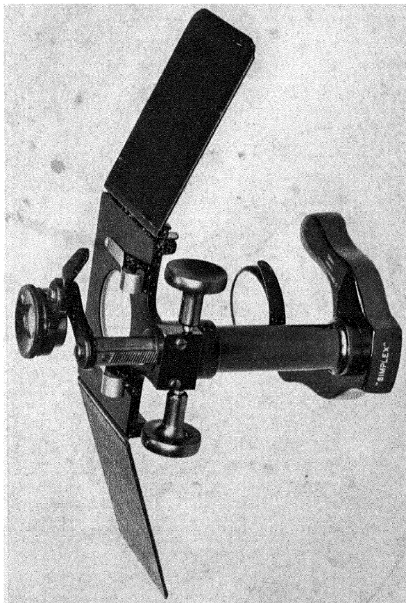
Fig. 4.—SIMPLE FORM OF DISSECTING MICROSCOPE (By Watson)
