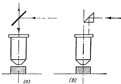
Fig. 60.—Vertical Illuminators
