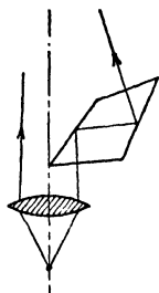
Fig. 74.—Wenham's Prism for Binocular Microscopes.
