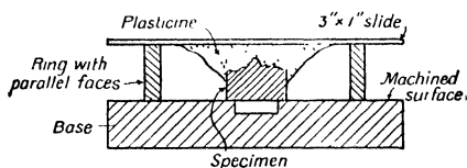
Fig. 68.—Method of Mounting a Metal Specimen for Examination
