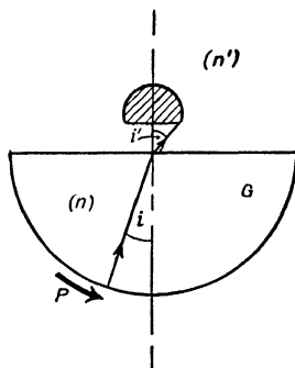
Fig. 34.—Principle of Abbe Apertometer
