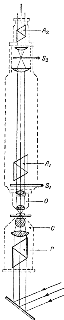
Fig. 81.—Optical System of a Polarization Microscope.
