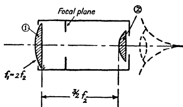
Fig. 24.—Huygenian Type Eyepiece
