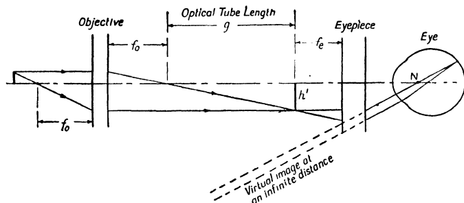
Fig. 8.—Ray Diagram showing Formation of Image in the Compound Microscope
