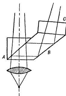
Fig. 76.—Arrangement of Prisms by Beck.
