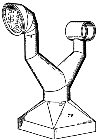
FIG. 154. — A paper model. A close examination of the opening in the cowl will show the method used to make the joints.
