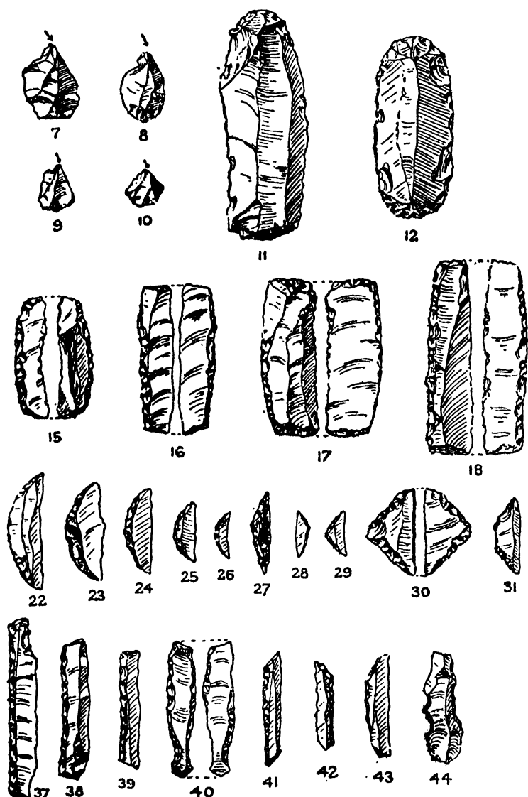
FIG. 8. Natufian microliths, \frac{1}{3} , after JRAI . 7-10 microburins; 22-6 lunates; 27-30 triangles, 30 showing Helwan retouch; 31 trapeze.
