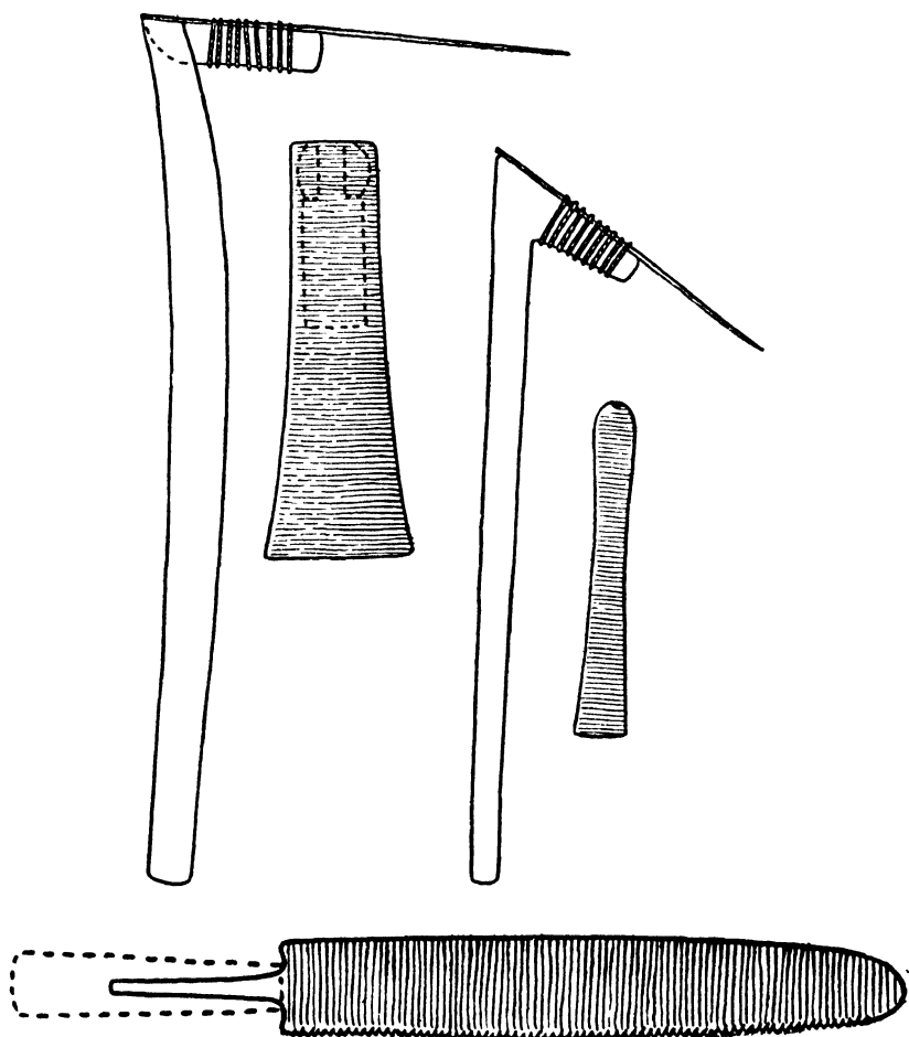
FIG. 46. Copper adzes with wooden handles and saw, Tomb of Hemaka, after Emery, l.
