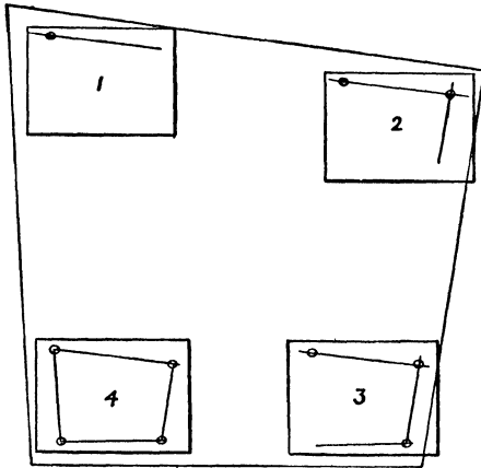
Fig. 52 —Traverse Method
