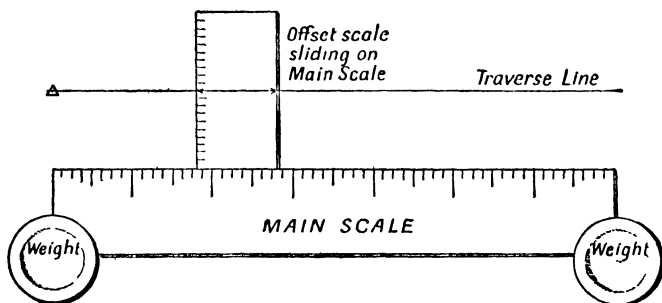
Fig. 27.—Cardboard Scales for plotting offsets
