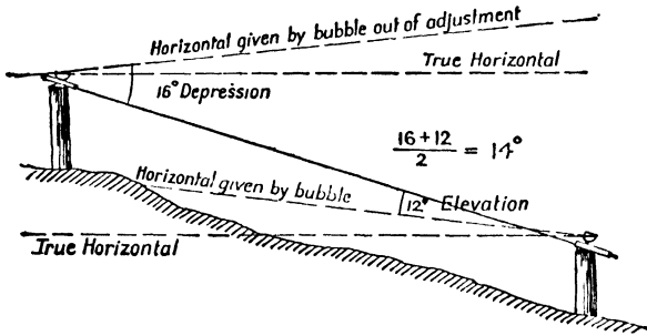
Fig. 39.—Testing for index error
