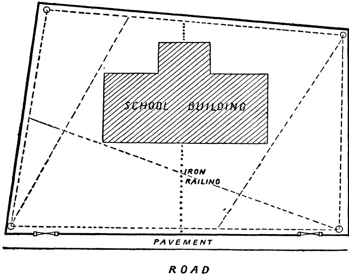
Fig. 16.—Layout of Survey Lines for a School Playground
