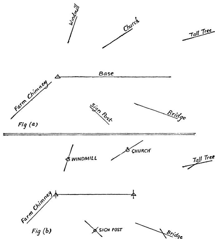
Fig. 20.—Compass Sketch
