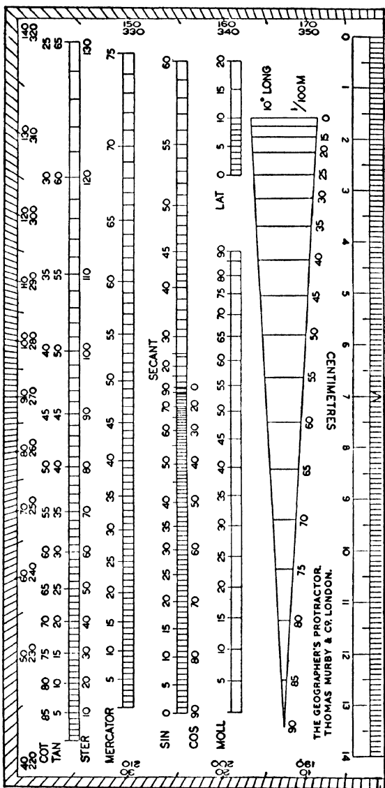
Fig. 5a—Geographer's Protractor, front
