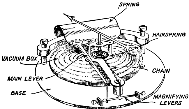
Fig. 33.—Aneroid Barometer
