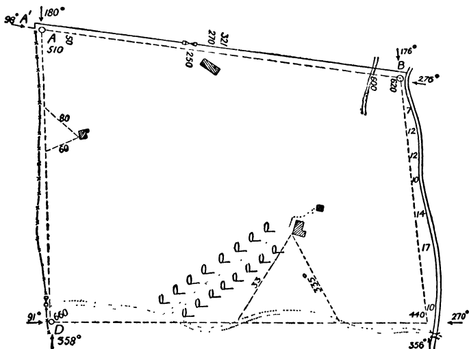
Fig. 23.—Plan of Field for Compass Traverse
