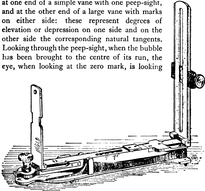
Fig. 62.—Indian Clinometer
