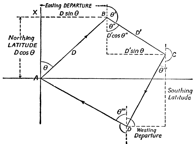
Fig. 28.—Plotting by Co-ordinates
