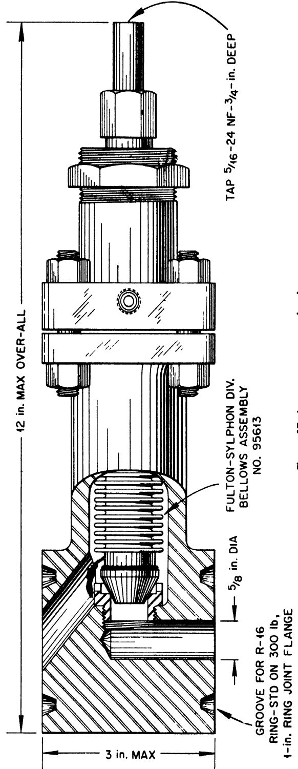
Figure 17. Low pressure control valve
