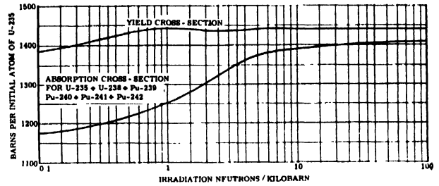
Figure 3. Conversion from natural uranium to equilibrium plutonium in thermal neutron reactor. Case 17 parameters
