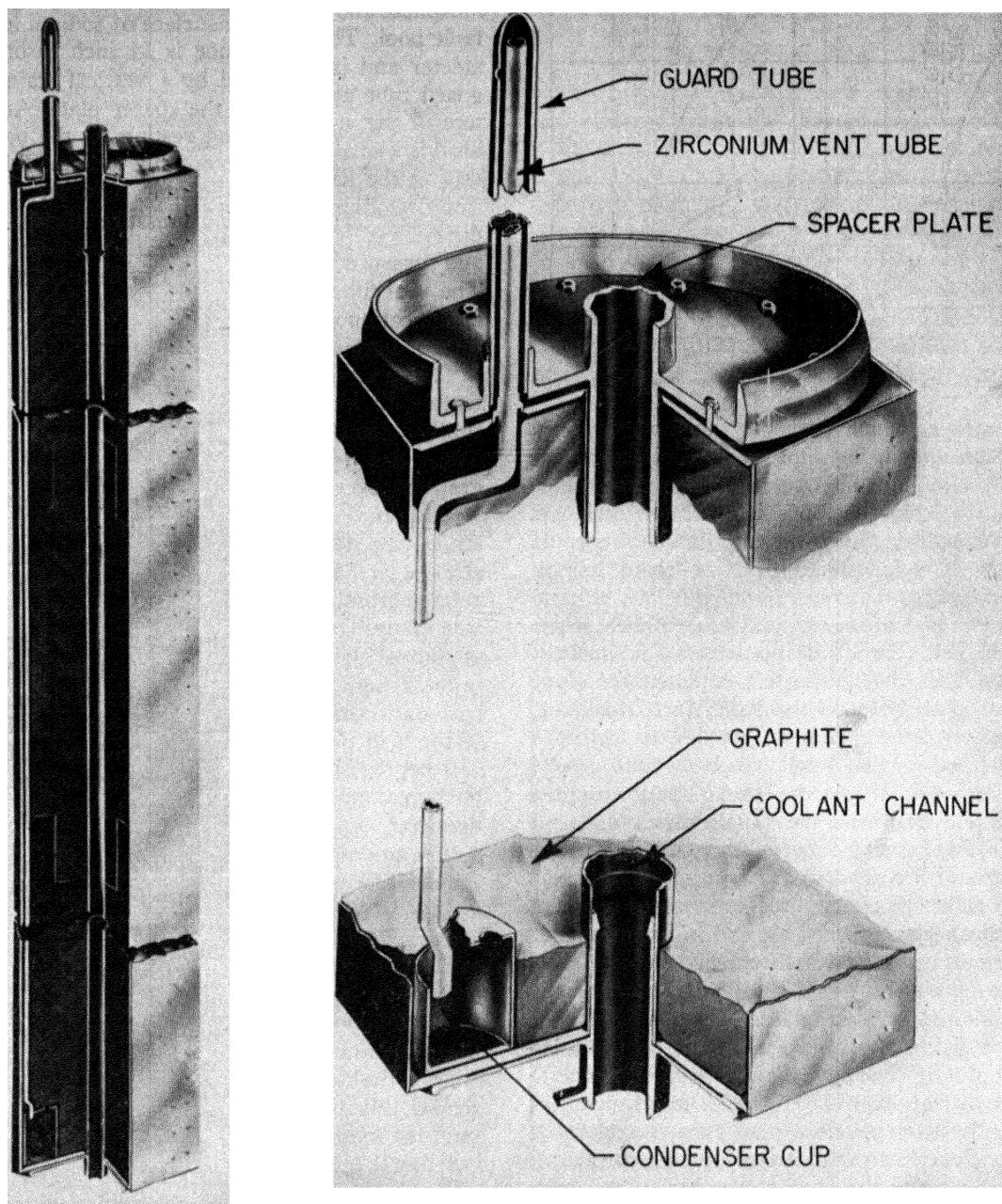
Figure 9. Zirconium-canned graphite moderator assembly
