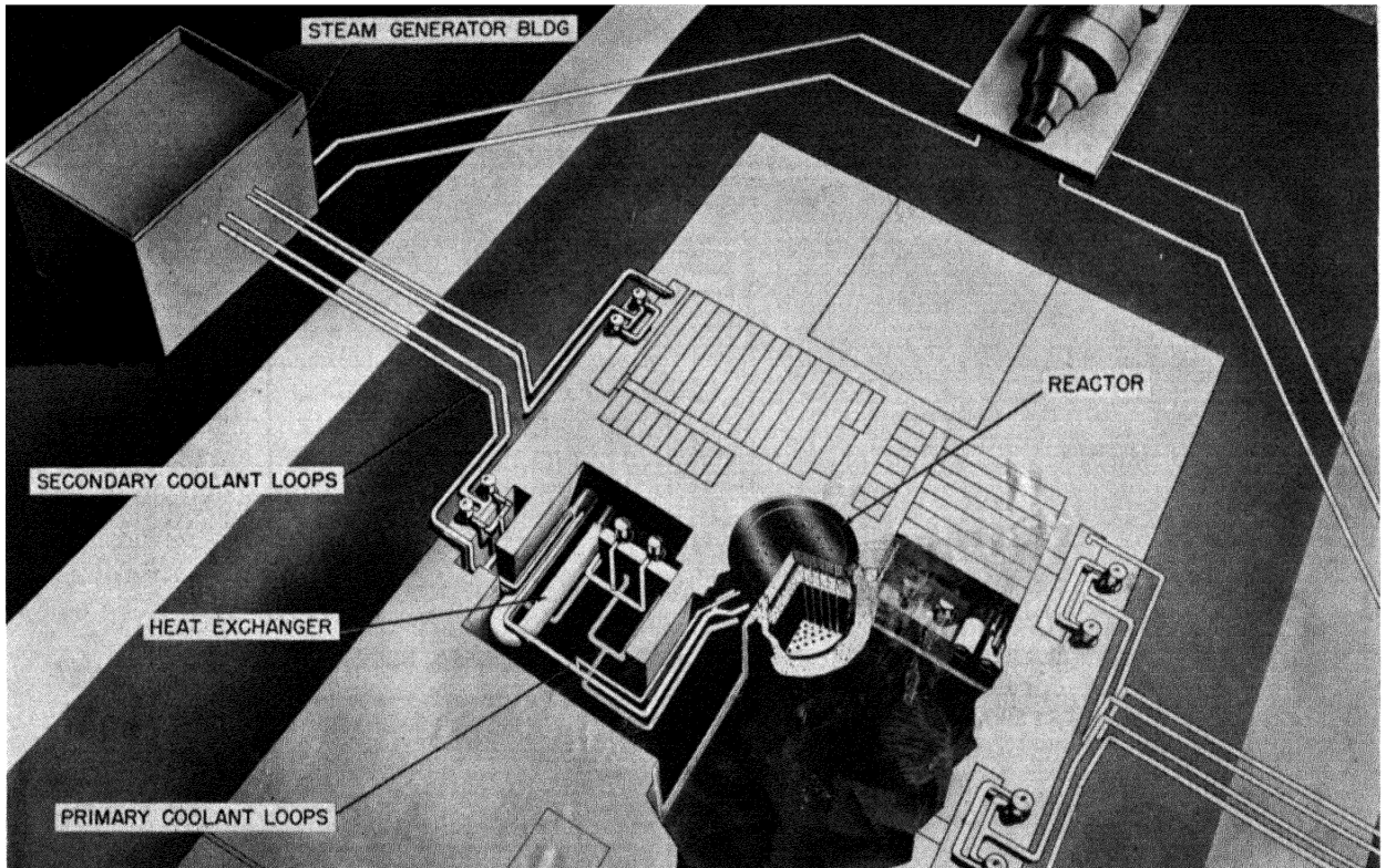
Figure 2 Aerial view of 75 megawatt reactor plant
