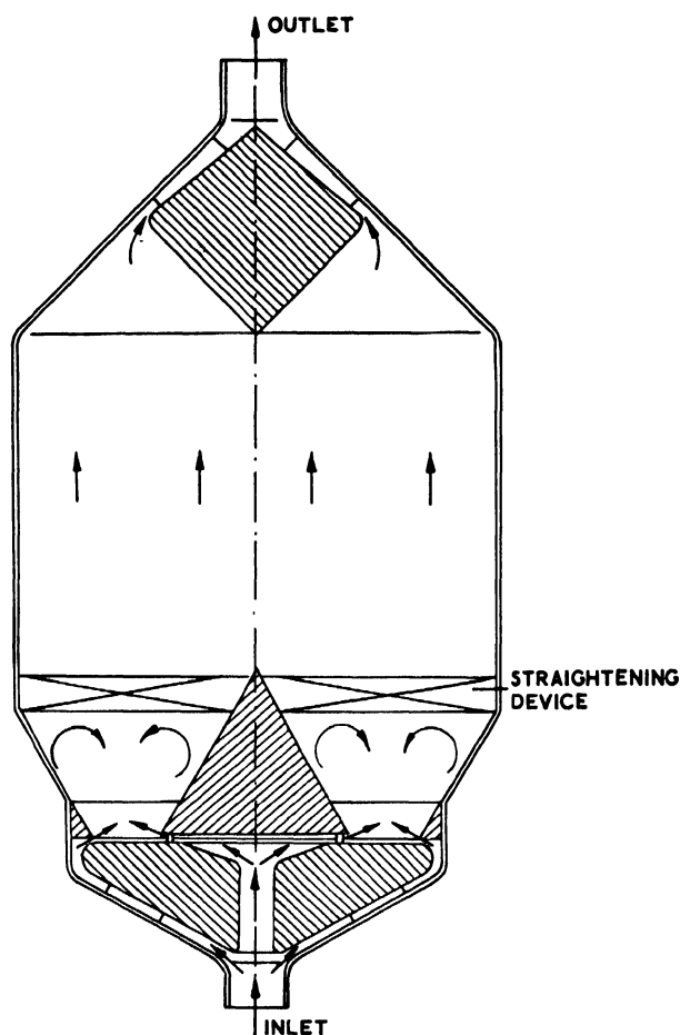
Figure 2. Drawing of the small-scale reactor vessel. Inside the cylindrical vessel, the suspension is slightly rotating
