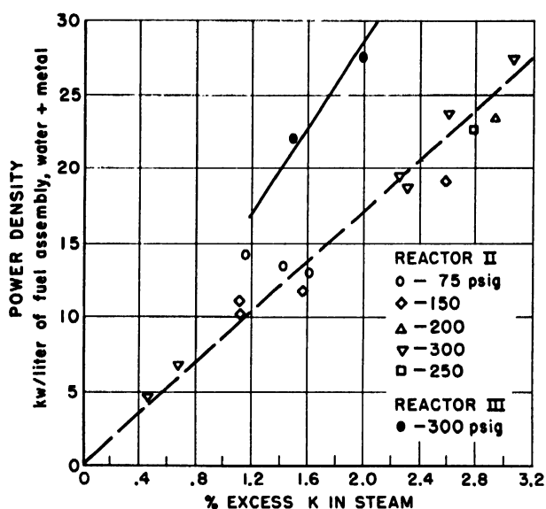
Figure 10. Effect of reactivity on power density
