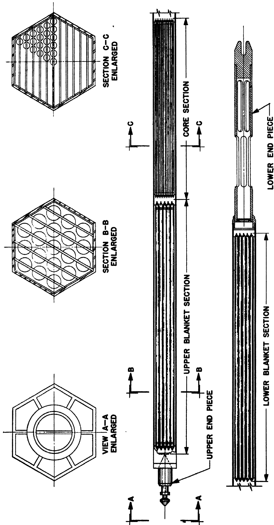
Figure 5. Core subassembly
