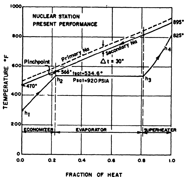
Figure 10. Temperature difference (pinchpoint) diagram. Steam conditions: 800 psig/825°F
