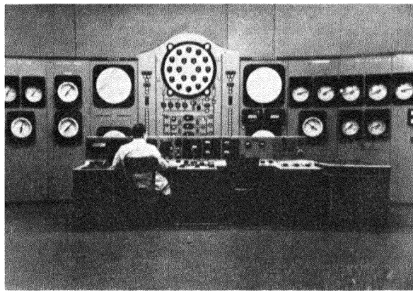
Figure 22. Central control panel. The simplified flow sheet is in the center of the panel. The switchboard is in the center of the picture
