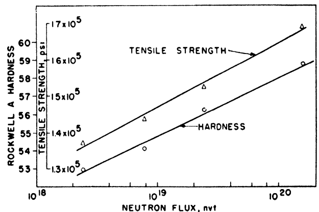
Figure 6. Hardness and tensile strength of type 347 stainless steel vs total flux
