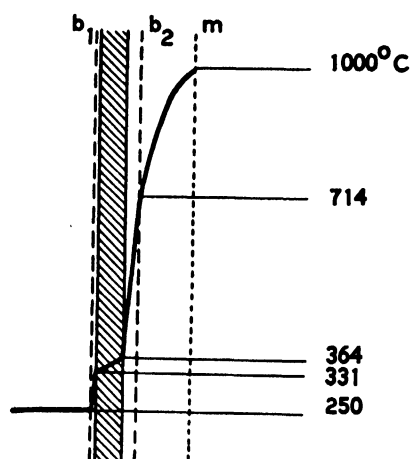
Slide 7. Temperature gradient across boundary layers; b_1 , boundary liquid film; b_2 , boundary first layer of grains; m , maximum temperature
