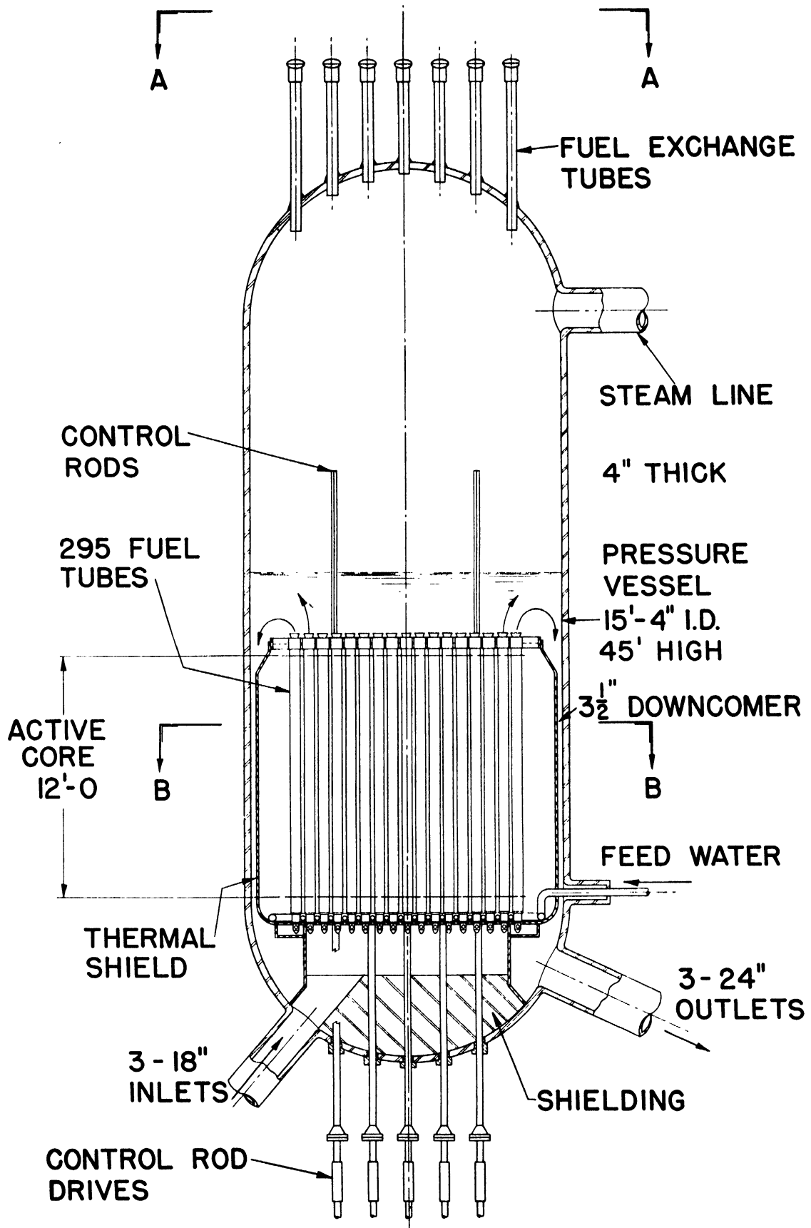
Figure 3. Vertical section through 1000-Mw D 2 O boiling reactor
