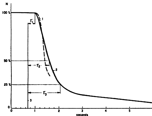
Figure 14. Decrease of reactor power after shut-down. N is power level, t time. 1. Theoretical curve. 2. Experimental curve, recorded by oscillograph. 3. Time of the emergency signal. The decrease in power to one-half takes about 0.90 seconds
