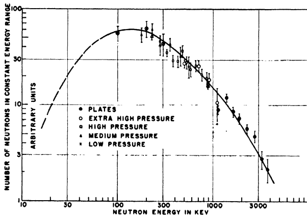
Figure 16. Neutron spectrum from hole #118 (2.6 in. from center) of the core of the EBR
