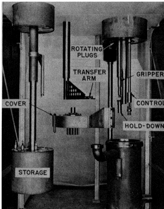
Figure 12. Mock-up of fuel handling system
