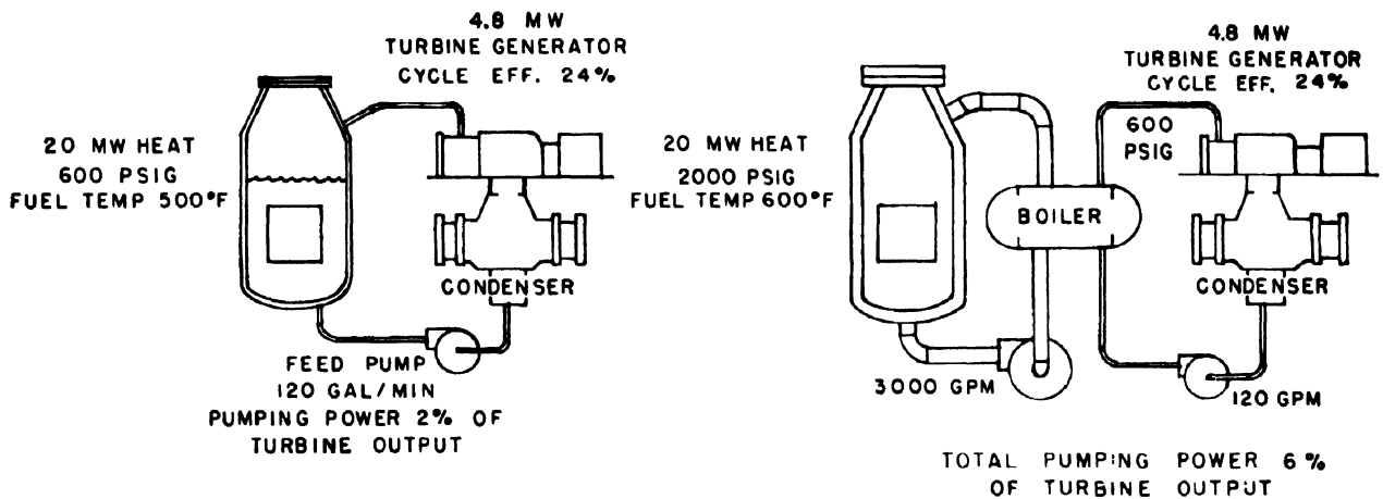
Figure 1. Comparison of the flow cycle of a boiling reactor with a pressurized water reactor
