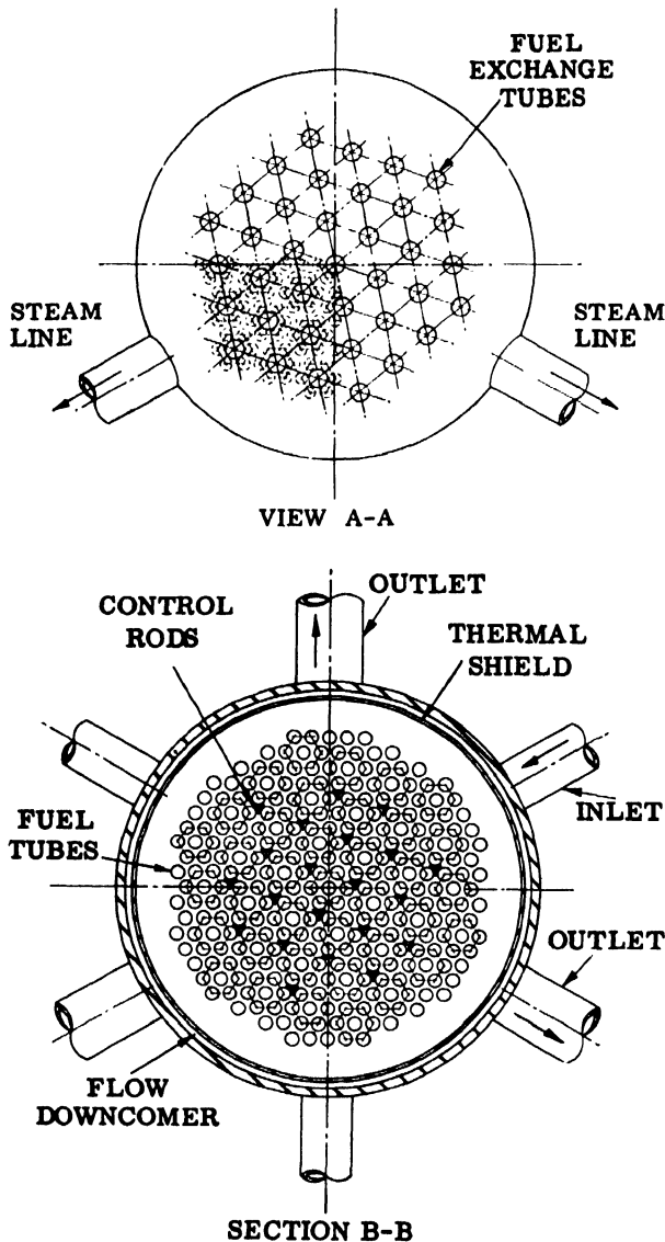
Figure 2. Plan view of 1000-Mw D 2 O boiling reactor
