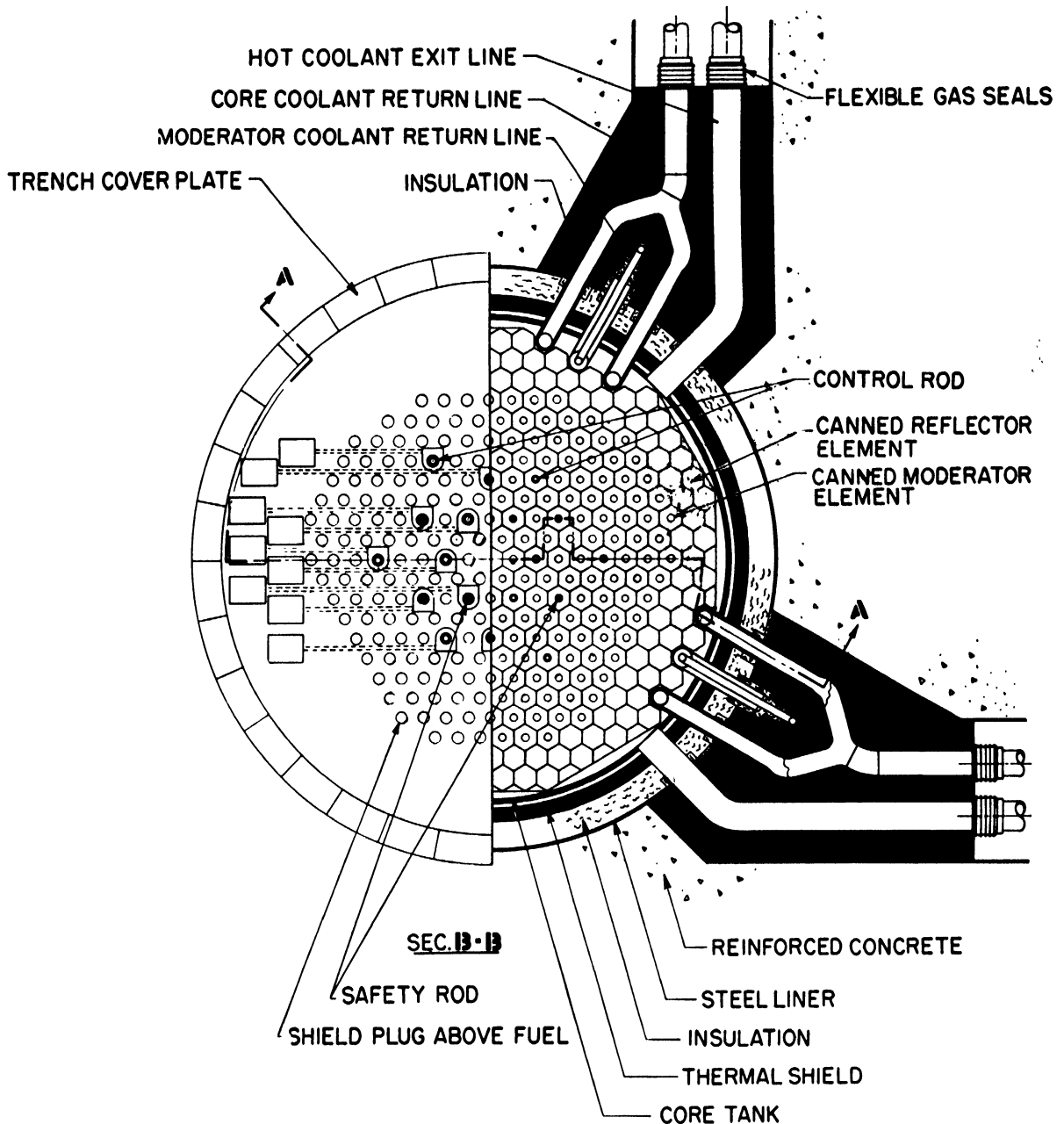
Figure 6. Reactor plan
