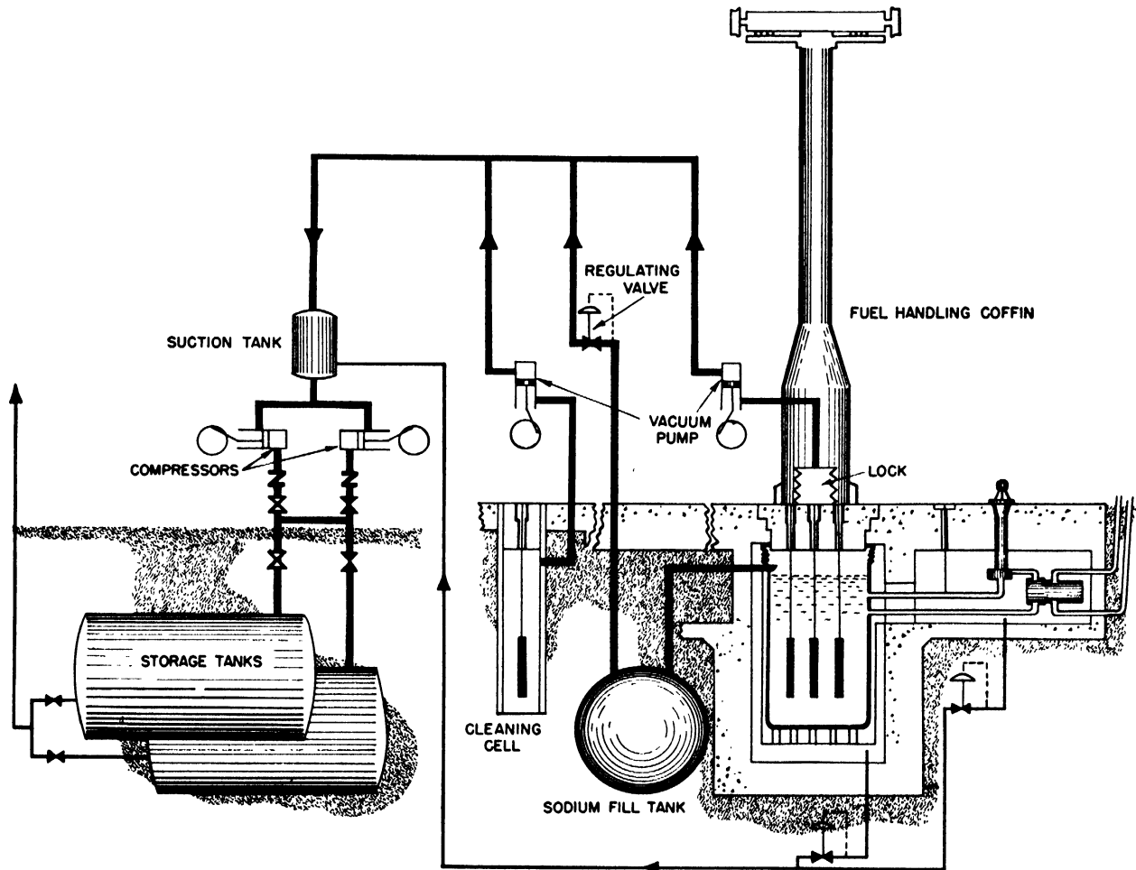
Figure 21. General arrangement for gaseous waste disposal system
