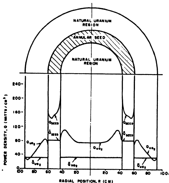
Figure 32. Radial distribution of power density for annular seed reactor with natural uranium in form of \text{UO}_2 .
