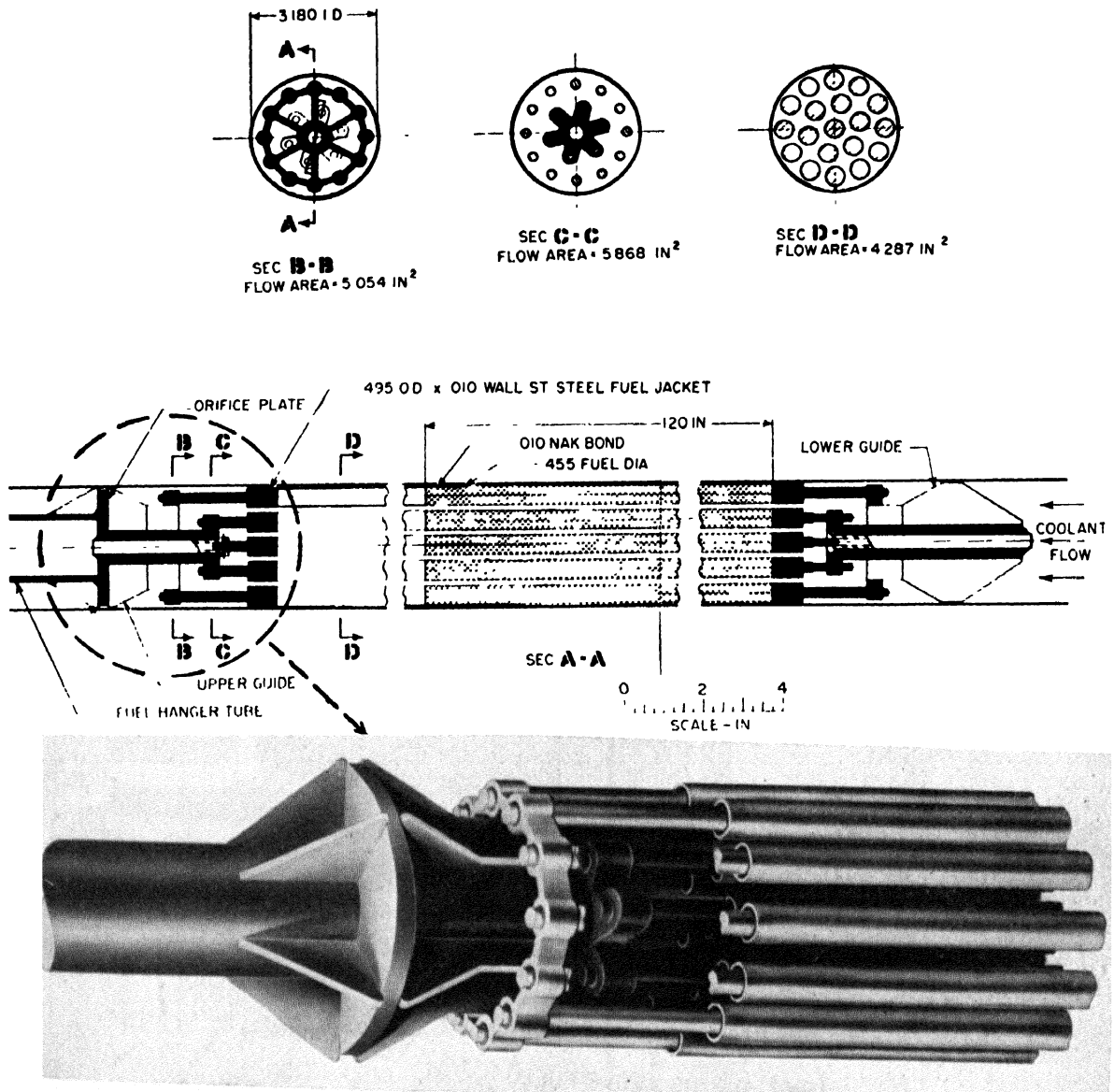
Figure 7. Nineteen-rod fuel cluster
