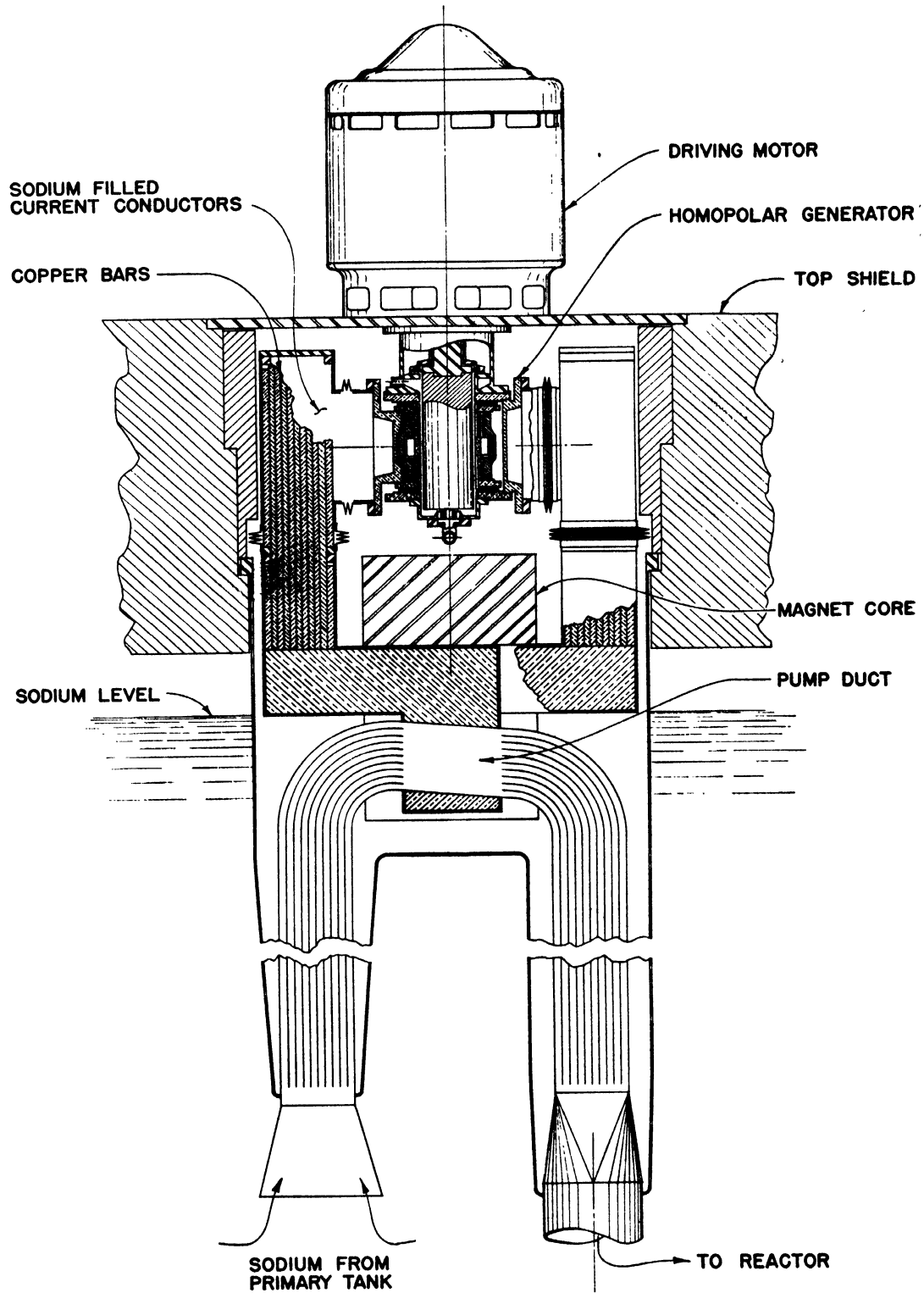
Figure 10. Primary system electromagnetic pump and generator
