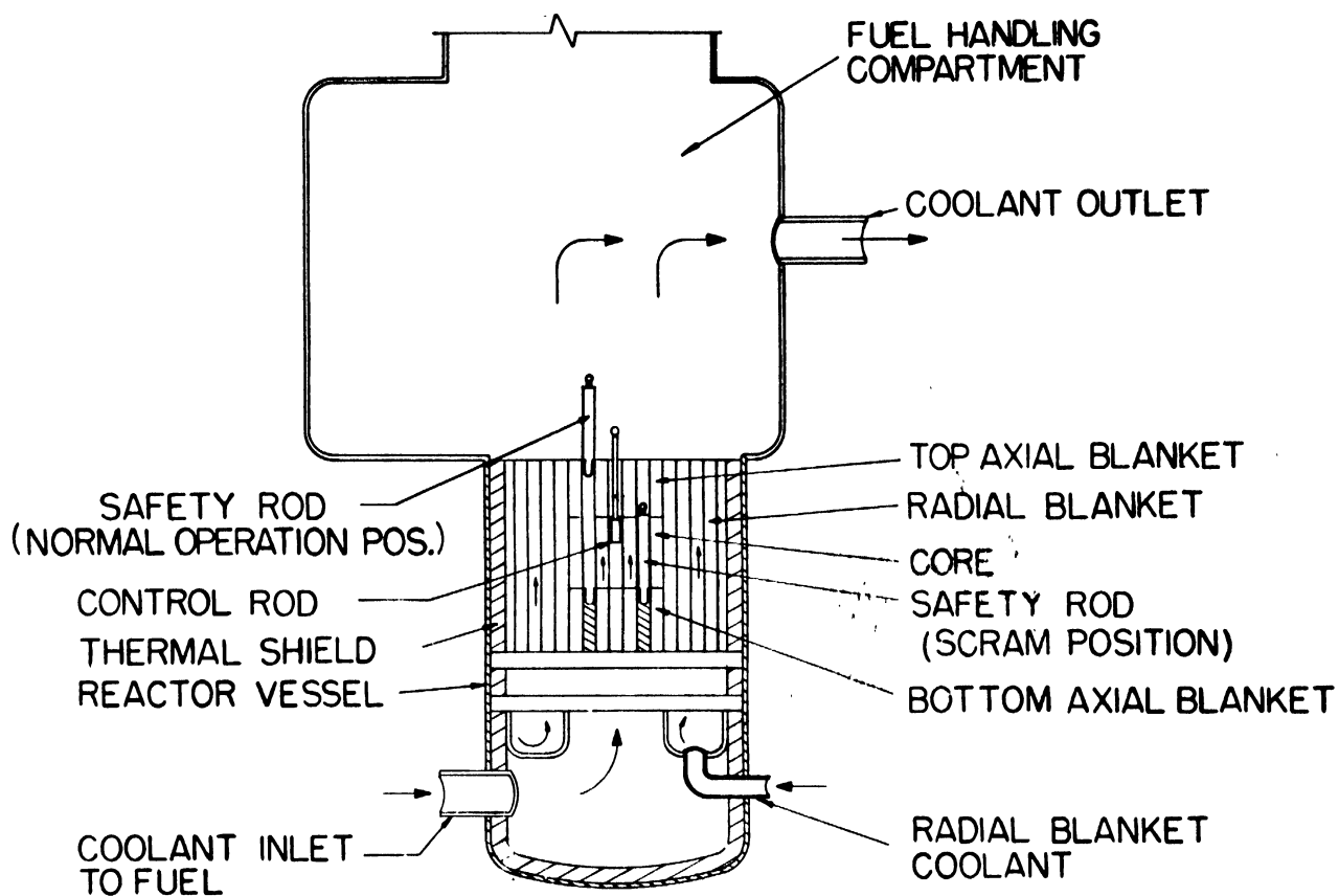
Figure 2. Reactor arrangement
