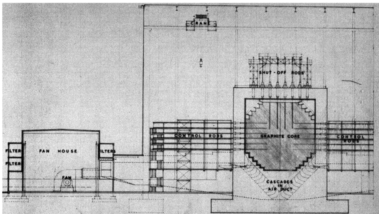
Figure 1. Longitudinal section
