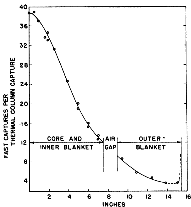
Figure 11. Radial U^{238} capture distribution along midplane of EBR
