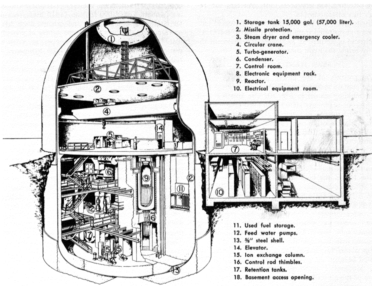
Figure 10. EBWR plant perspective
