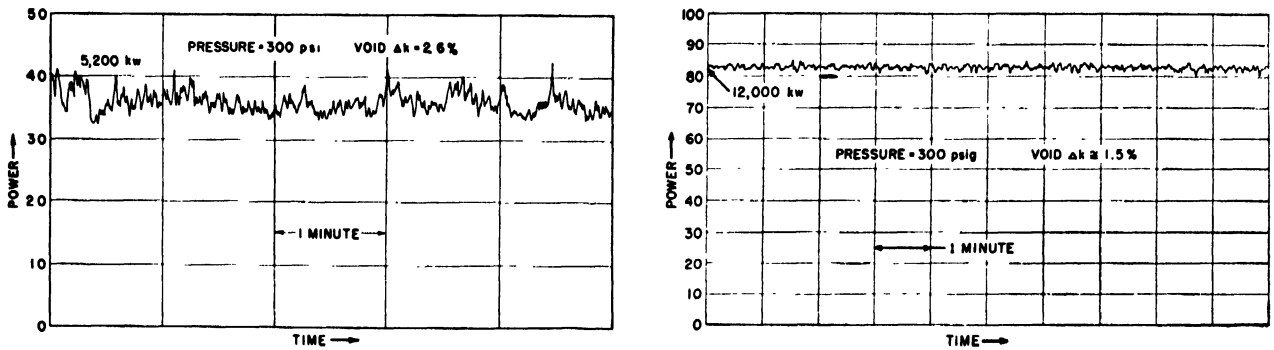
Figure 11. Reproductions of typical power records from two different boiling reactors: Figure 11a. reactor II. Figure 11b. Reactor III
