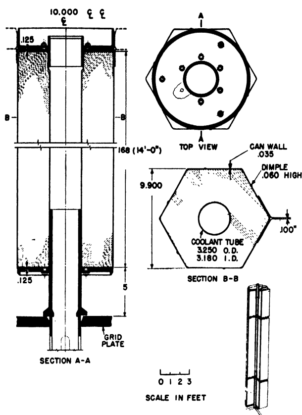
Figure 8. Moderator can
