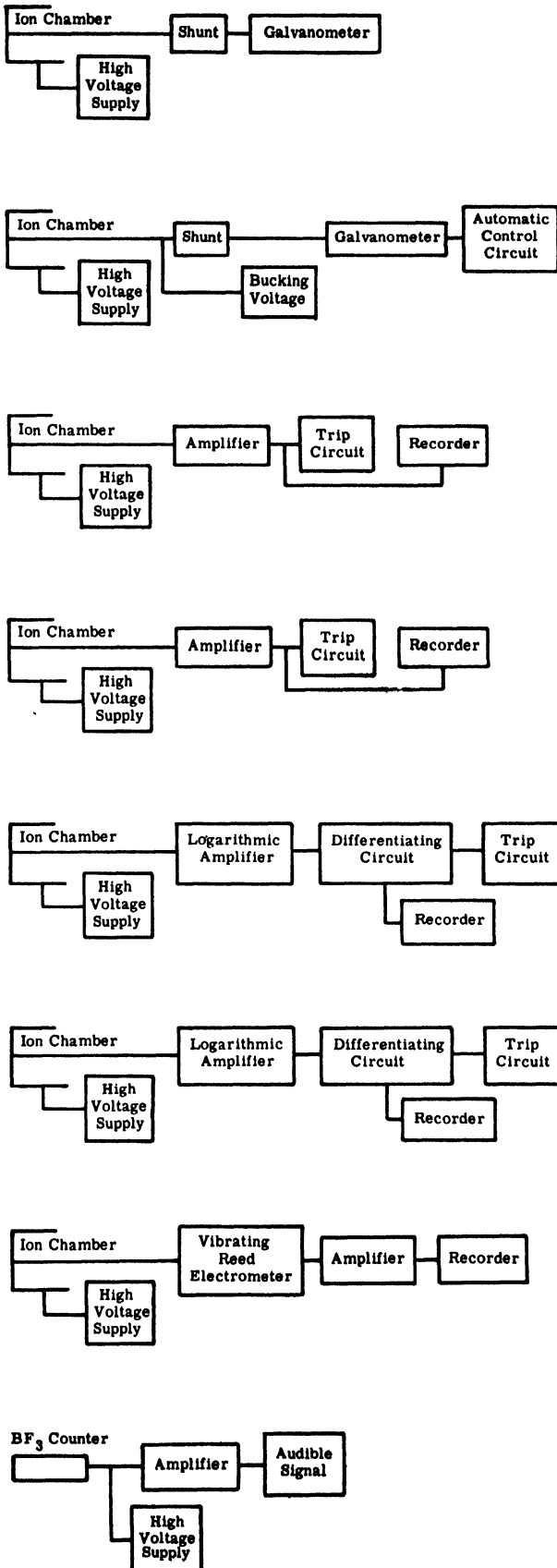
Figure 3. EBR nuclear instrumentation
