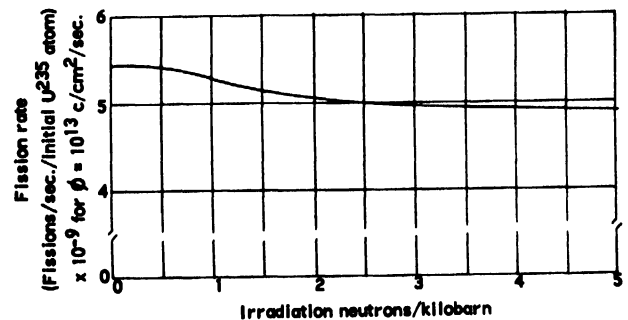
Figure 5. Long irradiation of natural uranium. Variation of heat output (fission rate) in constant flux
