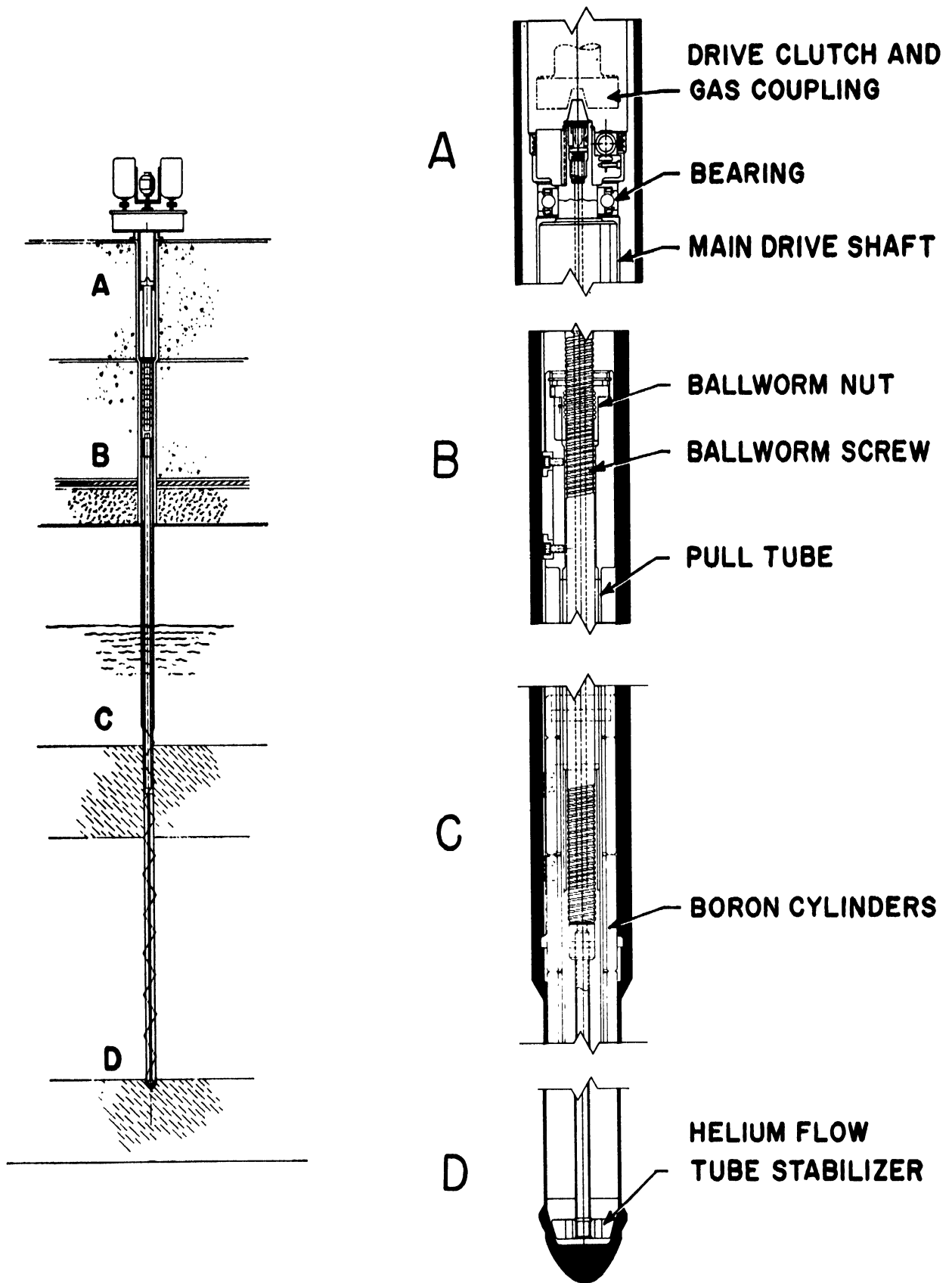
Figure 11. Control element
