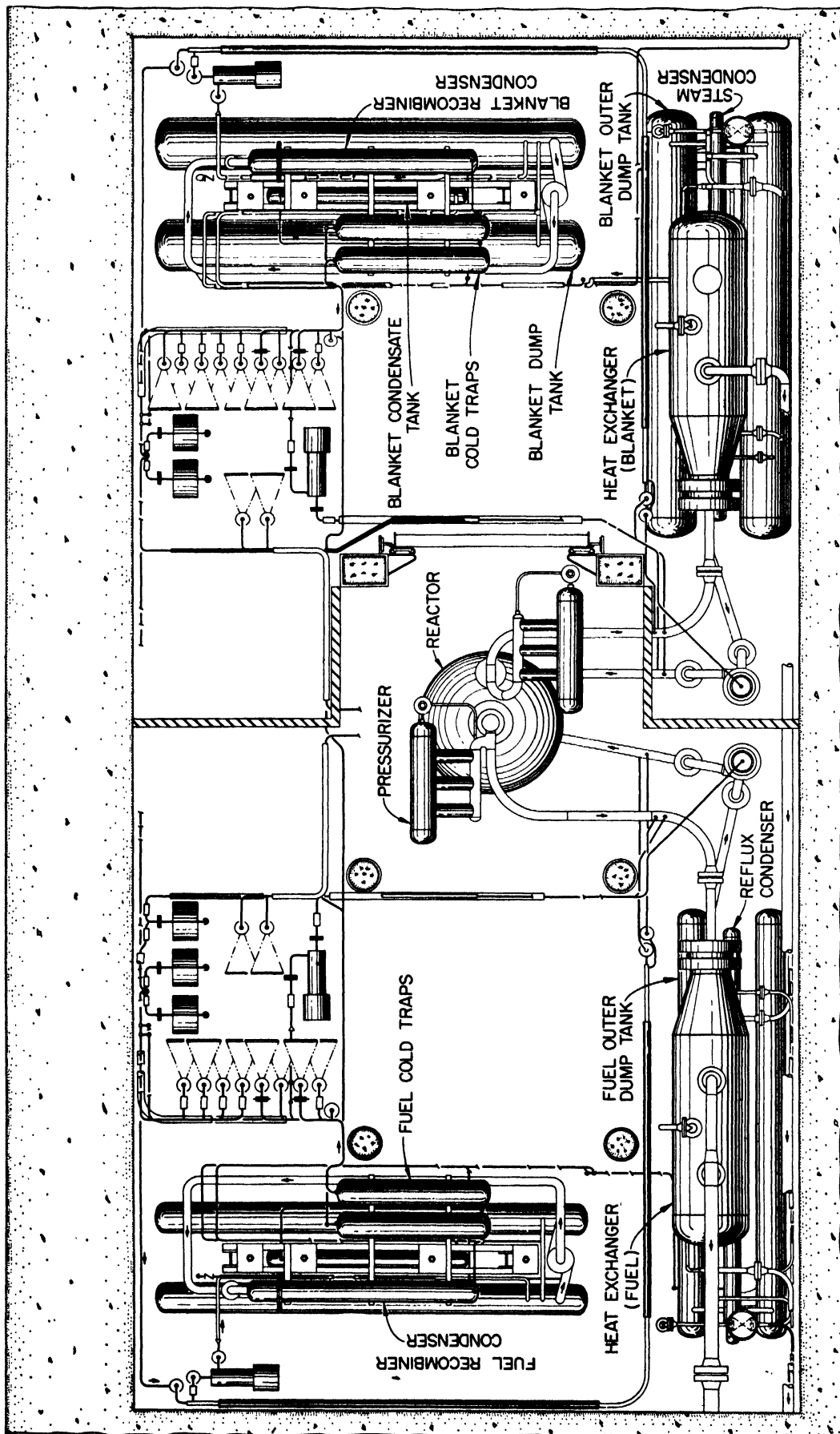
Figure 3. Reactor component arrangement—plan
