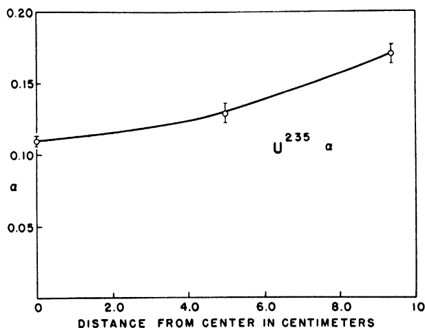
Figure 12. Radiative capture to fission ( \alpha ) of uranium-235 in EBR
