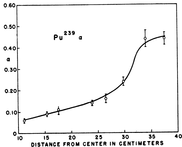
Figure 13. Radiative capture to fission ( \alpha ) of plutonium-239 in EBR
