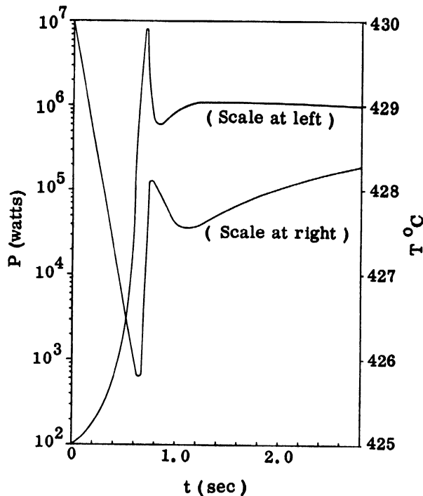
Figure 4. Instantaneous power development and temperature following an abrupt increase in heat removal rate from 10^2 to 10^6 watts
