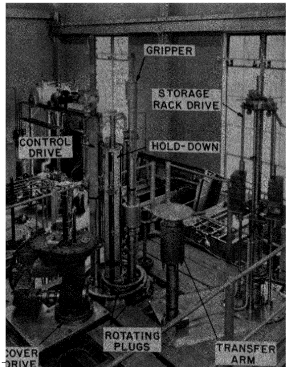
Figure 13. Mock-up of fuel handling system drives
