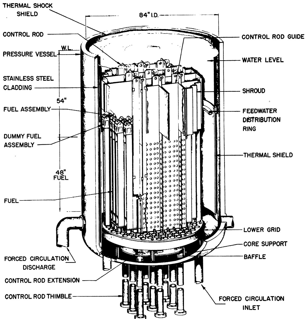
Figure 6. Perspective of EBWR
