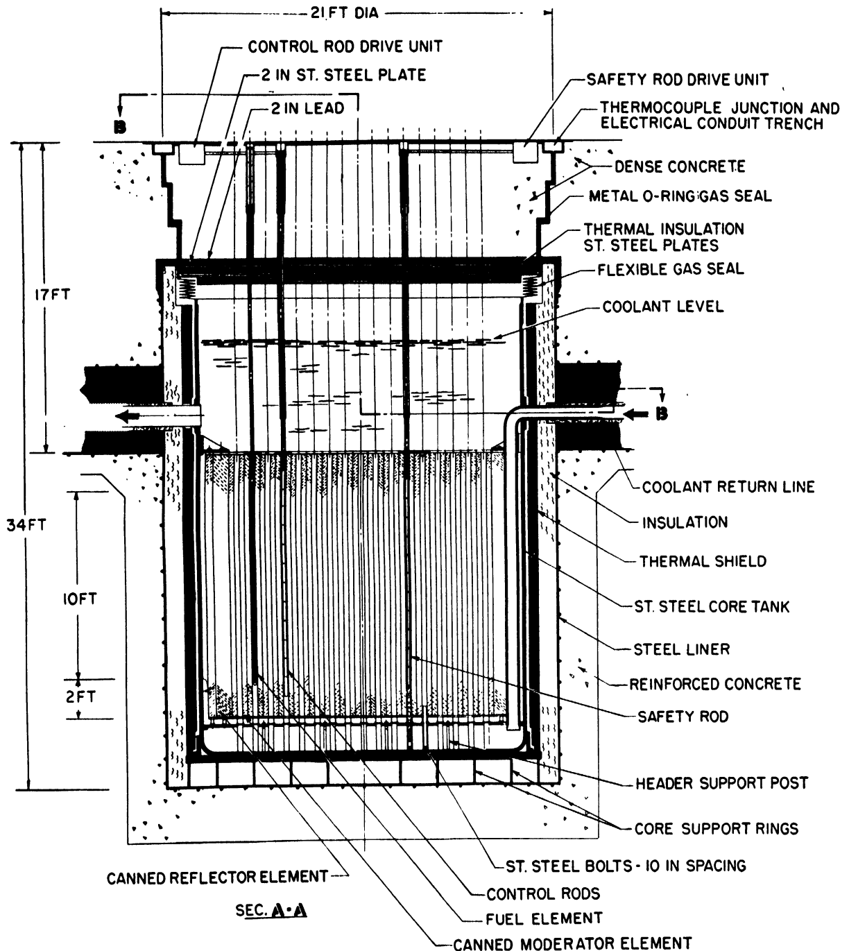
Figure 5. Reactor elevation
