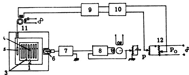
Figure 1. Error signal ( P_0 - P ) control. 1. Concrete. 2. Reflector. 3. Moderator. 4. Uranium. 5. Shim plate. 6. Ionization chamber. 7. Direct current amplifier. 8. Power recorder. 9. Magnetic amplifier. 10. Electronic amplifier. 11. Motor. 12. Comparator
