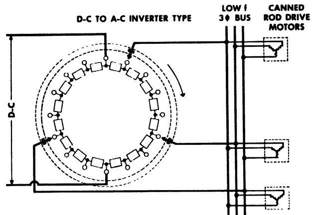
Figure 23. Control rod drive motor supply
