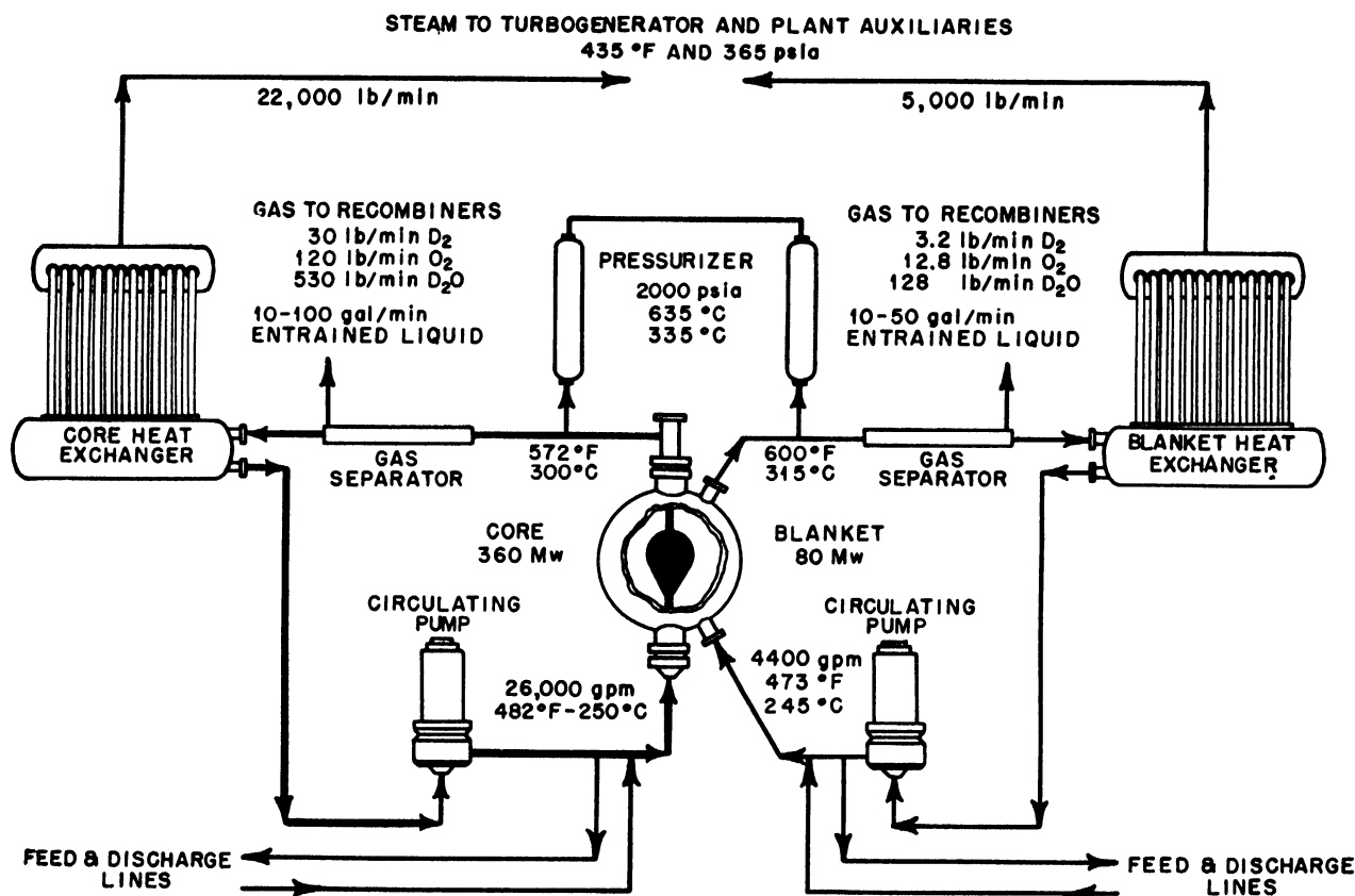
Figure 2. Flow diagram for high pressure circulating system
