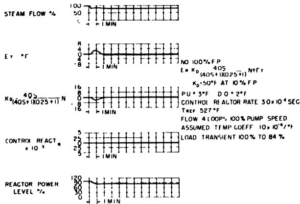
Figure 21. Simulator curves showing effect of load transient
