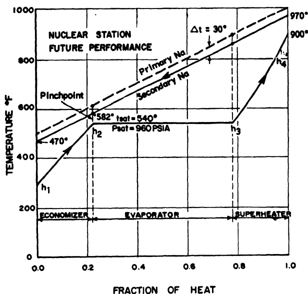
Figure 11. Temperature difference (pinchpoint) diagram. Steam conditions: 850 psig/900°F
