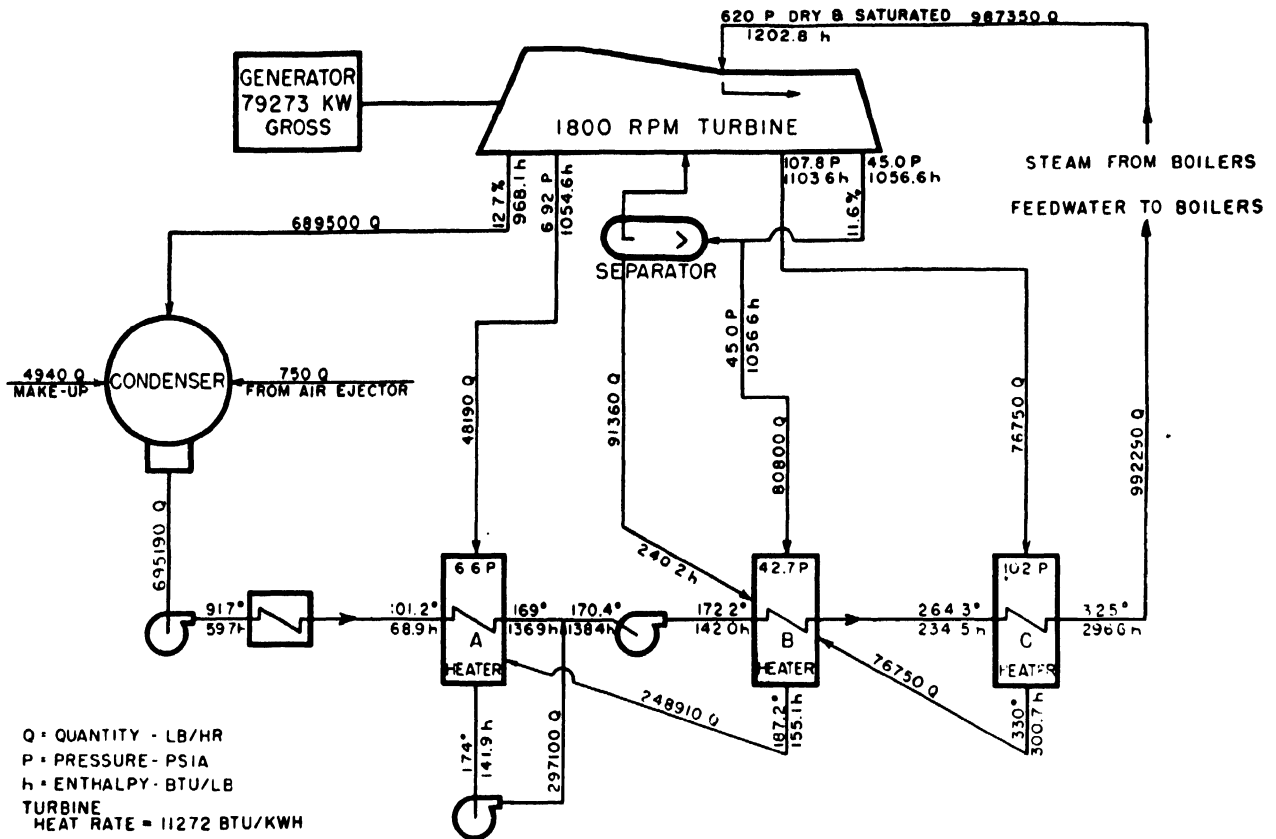
Figure 26. Heat balance diagram
