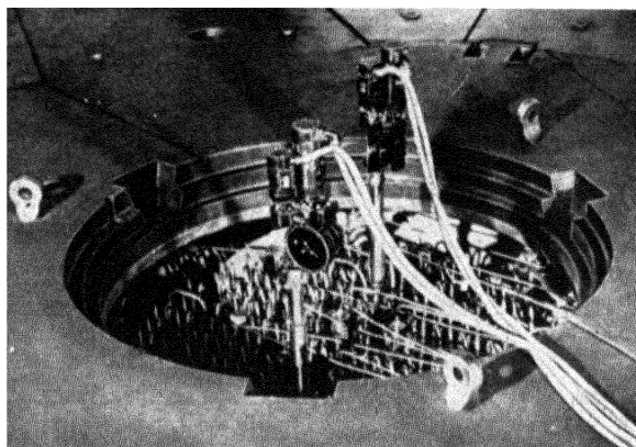
Figure 9. Upper part of reactor without cover showing the servomotors of the safety rods and their cables. The water connexions can be seen below
