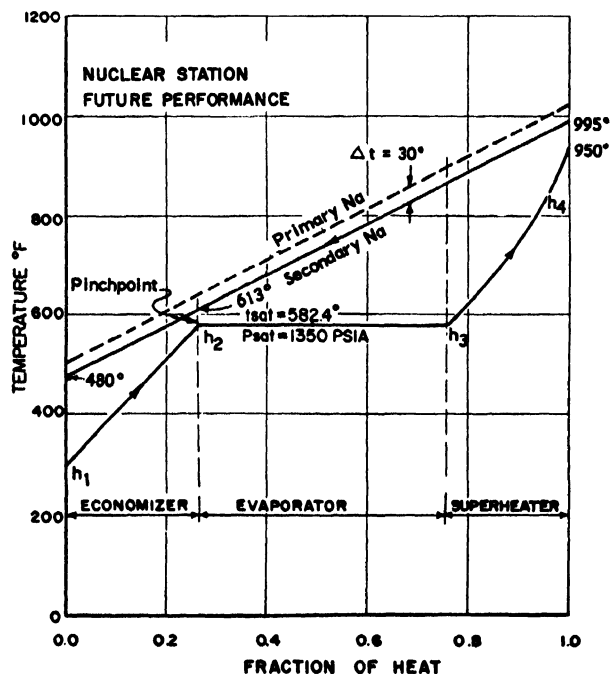
Figure 12. Temperature difference (pinchpoint) diagram. Steam conditions: 1250 psig/950°F
