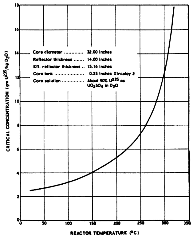
Figure 7. Critical concentration of U^{235} in core of HRT with D_2O blanket
