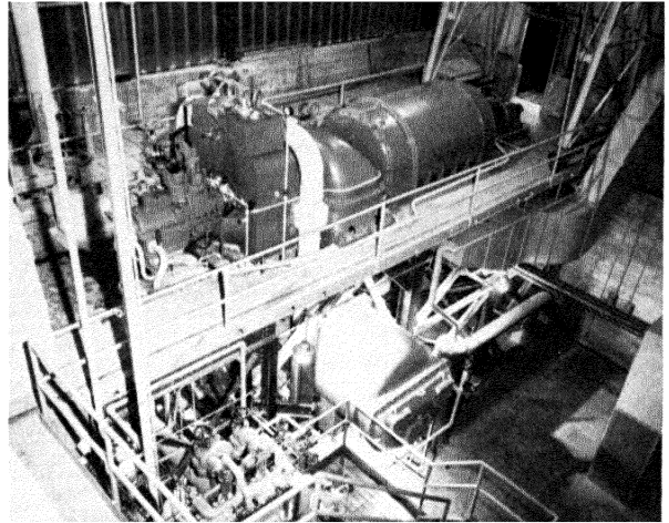
Slide 13. The turbine-generator installation
