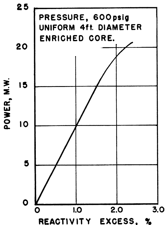
Figure 7. Thermal power vs reactivity % excess
