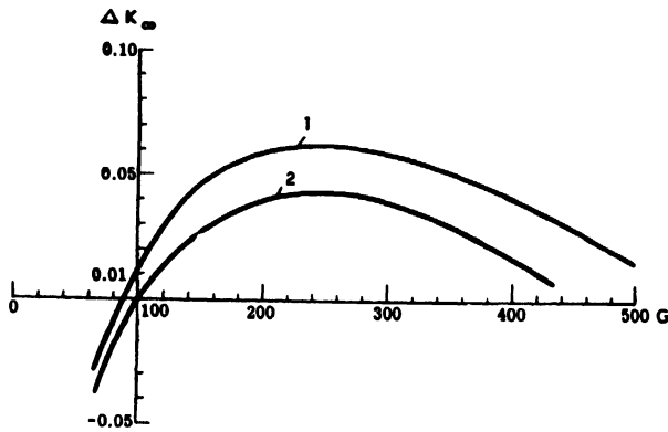
Figure 4. Variation of reactivity of the reactor in dependence on the quantity of water in the active zone ( \Delta k_{\infty} ). X-axis: quantity of water G in the active zone of the reactor. Y-axis: neutron multiplication factor increment. Curve 1 corresponds to the cold conditions (20°C). Curve 2 to the operation temperature \Delta k_{\infty} = 0 corresponds to a cold reactor with a normal content of water ( G = 100 kg)
