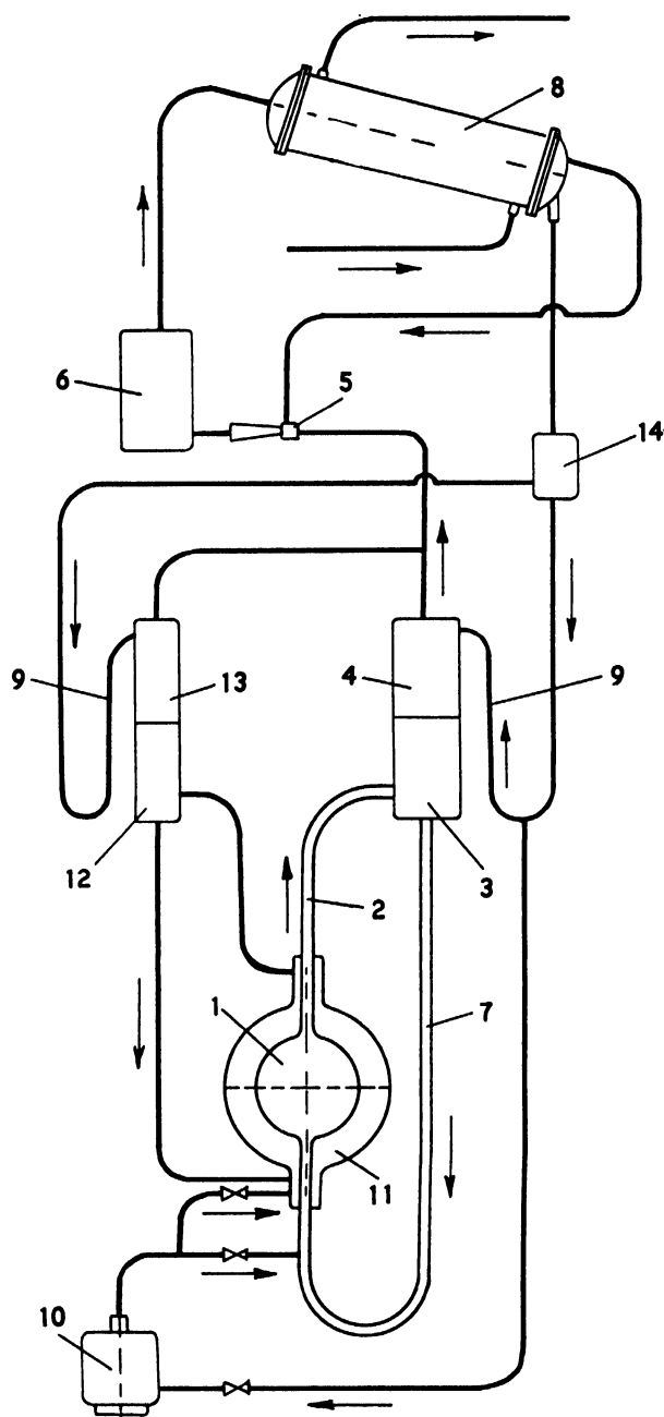
Figure 1b. Diagram of reactor with fuel regeneration: 1. Reactor. 2. Up-pipe. 3. Separator. 4. Steam purification. 5. Injector. 6. Burn chamber. 7. Down-pipe. 8. Heat exchanger. 9. Liquid seal. 10. Electric-boiler starter. 11. Reflector. 12. Reflector separator. 13. Apparatus for reflector steam purification. 14. Separator tank
