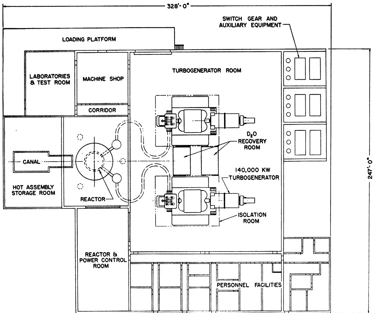
Figure 4. Plan view of central station 1000-Mw D 2 O boiling reactor
