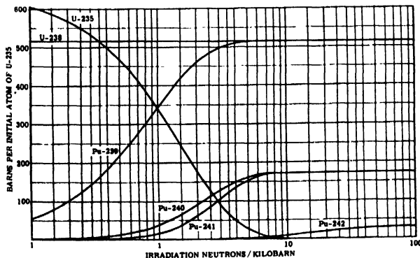
Figure 2. Long irradiation of natural uranium. Neutron changes due to growth of plutonium isotopes. Case 17 parameters
