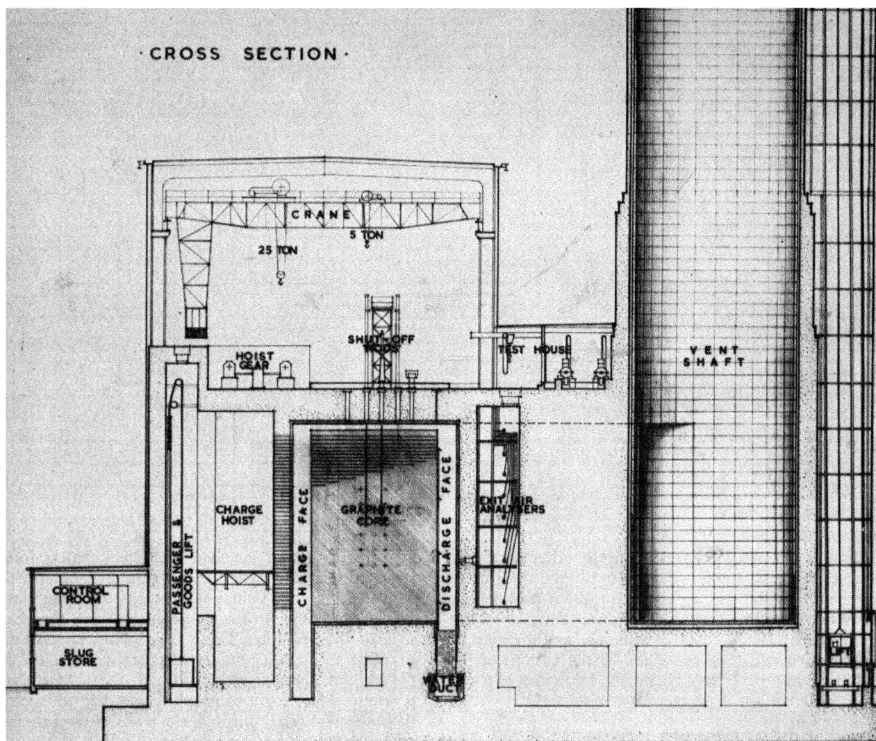
Figure 2. Cross section
