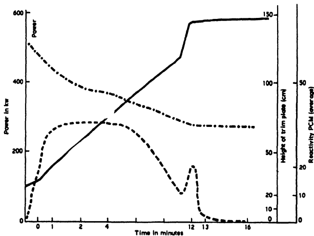
Figure 6. Power excursion for automatic passage from 100 kw to 600 kw. The corresponding reactivity excursion and height of trim plate also are shown. (Experiment carried out on P2)
