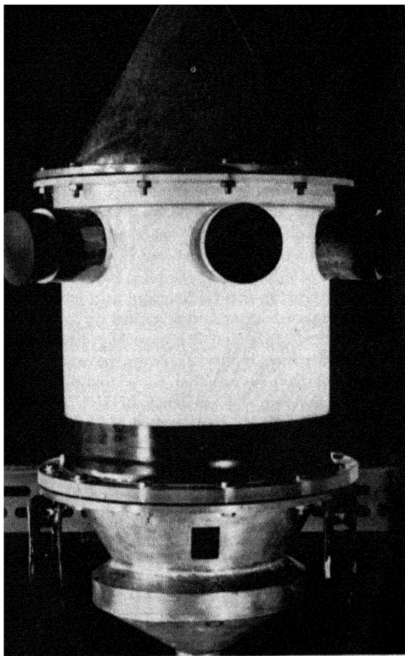
Figure 1a. Model of the small-scale reactor vessel. The side tubes are only present for experimental purposes
