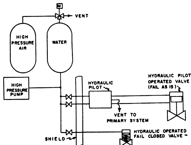
Figure 17. Valve operating system schematic
