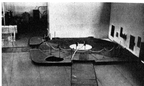
Figure 10. Upper part of reactor in operation, showing top shielding plate and safety rod servomotors
