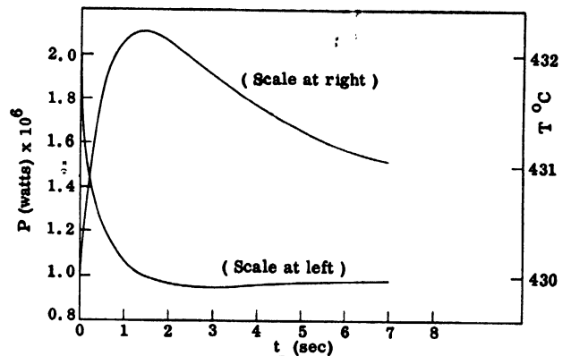
Figure 5. Instantaneous power development and temperature following an abrupt decrease in heat removal rate from 2 \times 10^6 to 1 \times 10^6 watts
