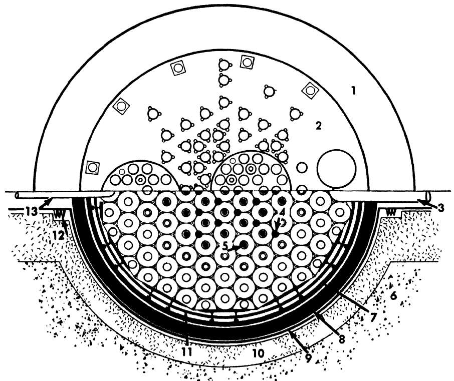
Figure 5. Reactor elevation
