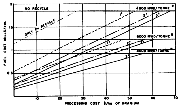
Figure 8. Fuel recycling for power reactors. Fuel costs related to uranium processing costs. Processing cost is the average for each extraction including return to reactor. Fuel cost is contribution to power cost from supply and processing of uranium at $44/kg
