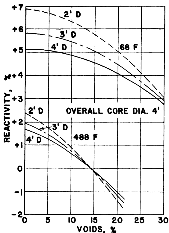
Figure 3. Reactivity vs void for various diameters of enriched zone
