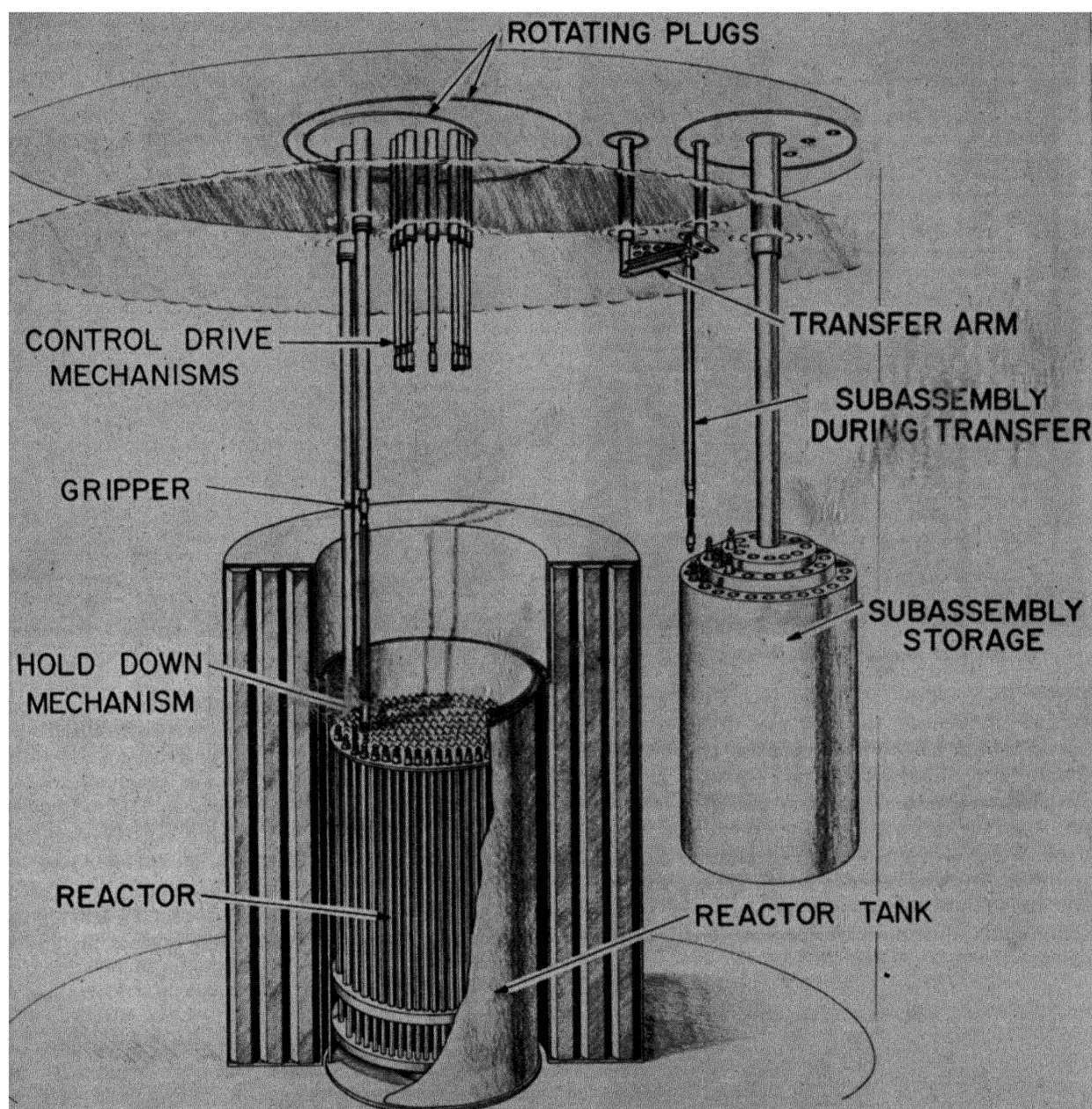
Figure 11. EBR-II fuel handling system
