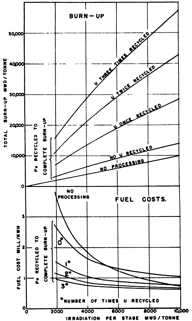
Figure 7. Burn-up and fuel costs
