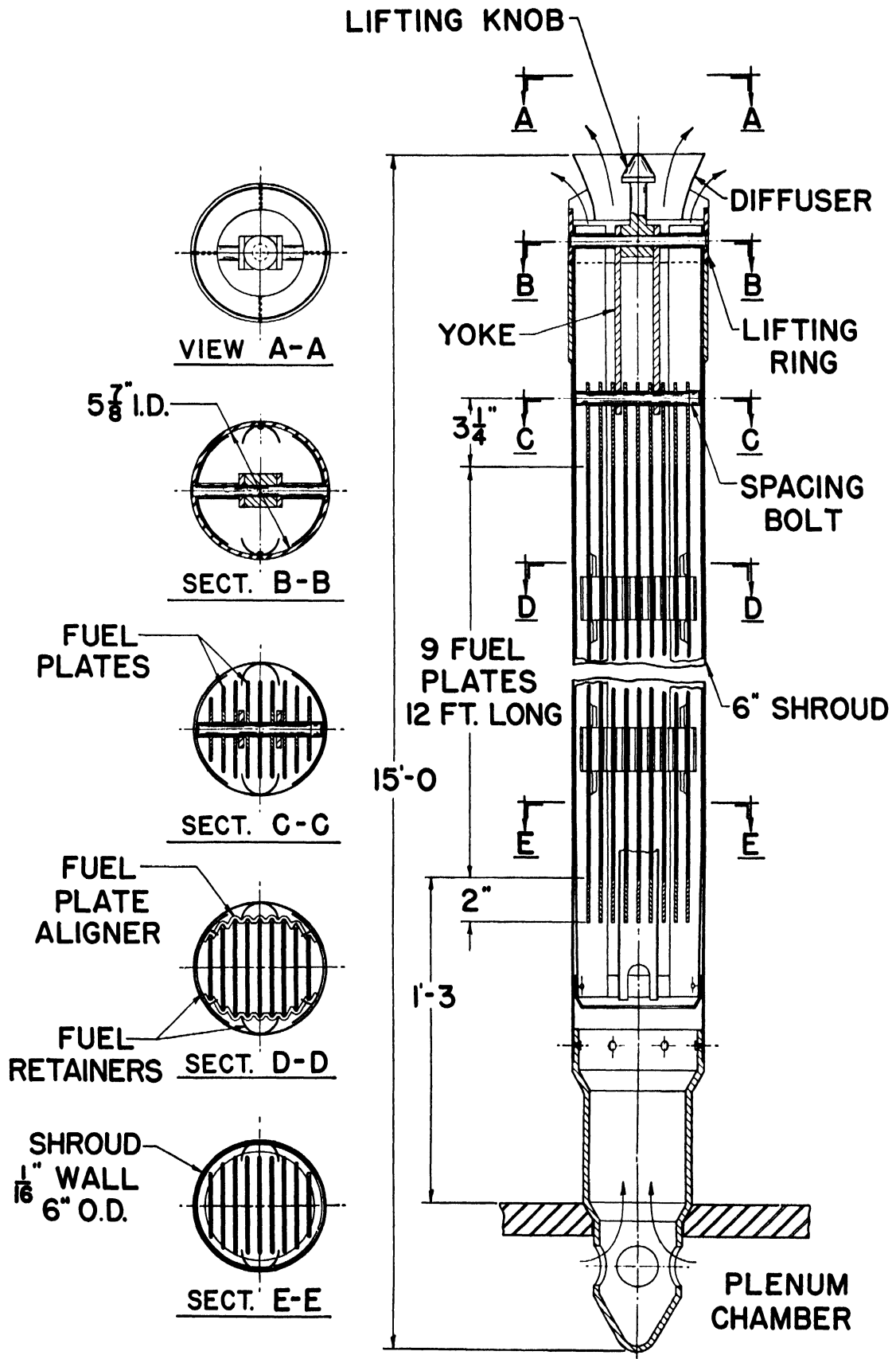
Figure 1. Fuel assembly for 1000-Mw D_2O boiling reactor
