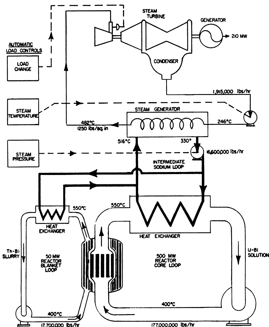
Figure 3. Heat cycle
