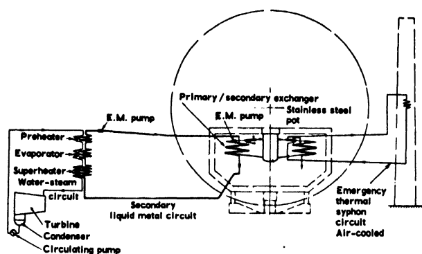
Figure 2. Diagrammatic arrangement of liquid metal and steam circuits for fast reactor
