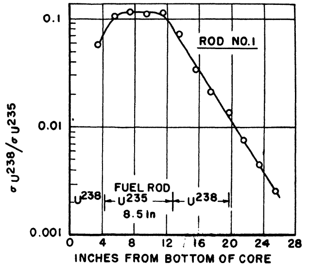
Figure 19. Vertical traverse of U^{238}/U^{235} fission ratio in center of EBR
