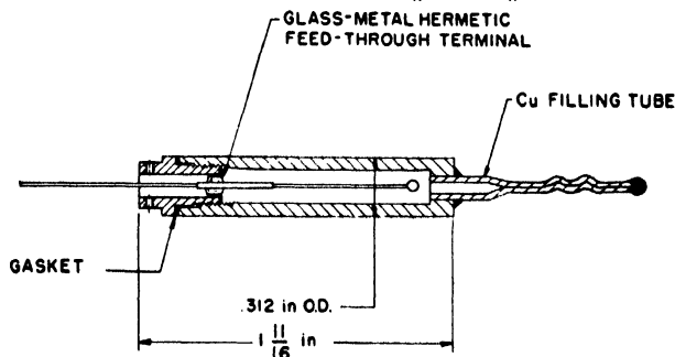
Figure 18. Fission counter used in EBR fission rate measurements
