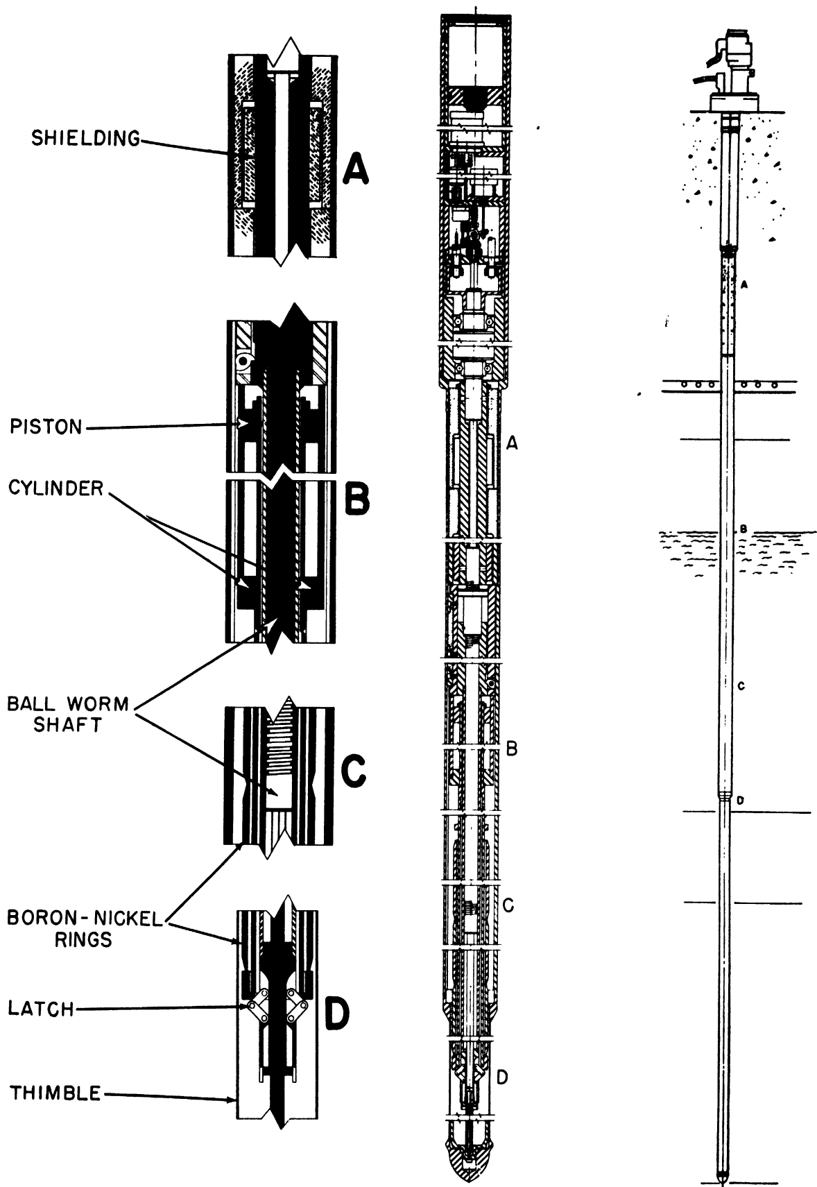
Figure 12. Safety element
