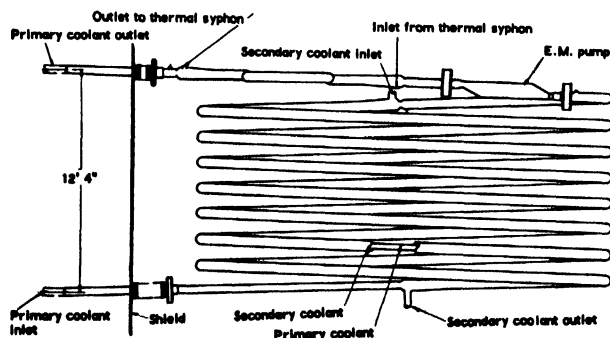
Figure 3. Primary-secondary exchanger
