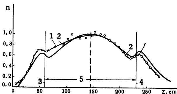
Figure 11. Axial distribution of thermal neutrons density: 1. Experimental curve, made with absorbing rods of the internal circle lowered and rods of the outer circle raised. 2. Theoretical curve, determined on the assumption that the substance of the absorbing rods is uniformly distributed in the active zone of the reactor. 3. Boundaries of the active zone and of the lower reflector. 4. Same for the upper reflector. 5. The active zone.
