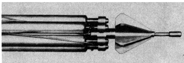
Figure 7. Seven-rod element
