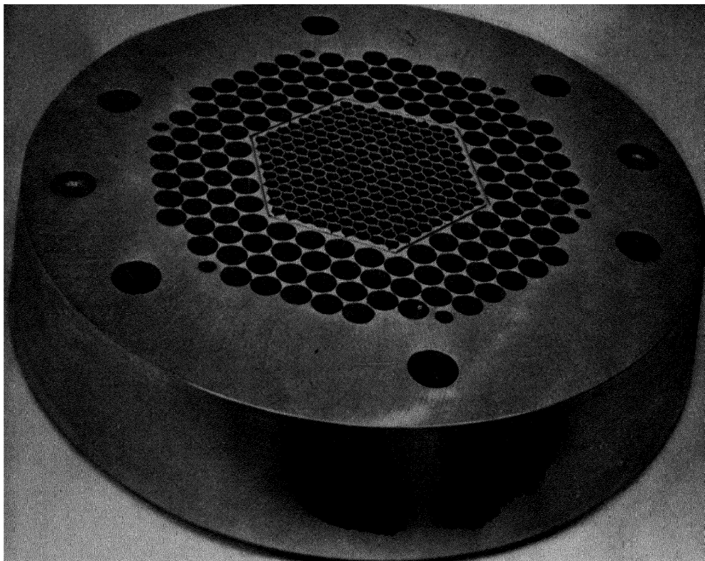
Figure 2a. Stainless steel holding plate for core fuel elements and inner blanket rods
