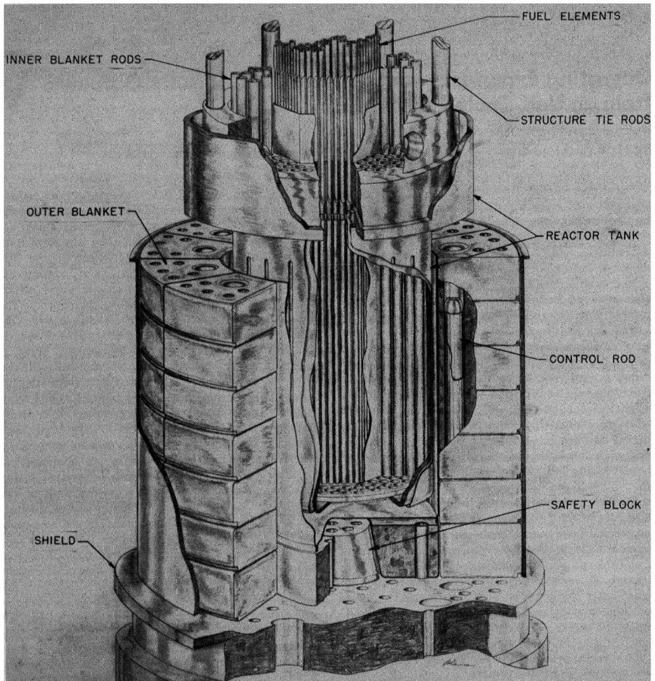
Figure 1. Cut-away showing EBR construction
