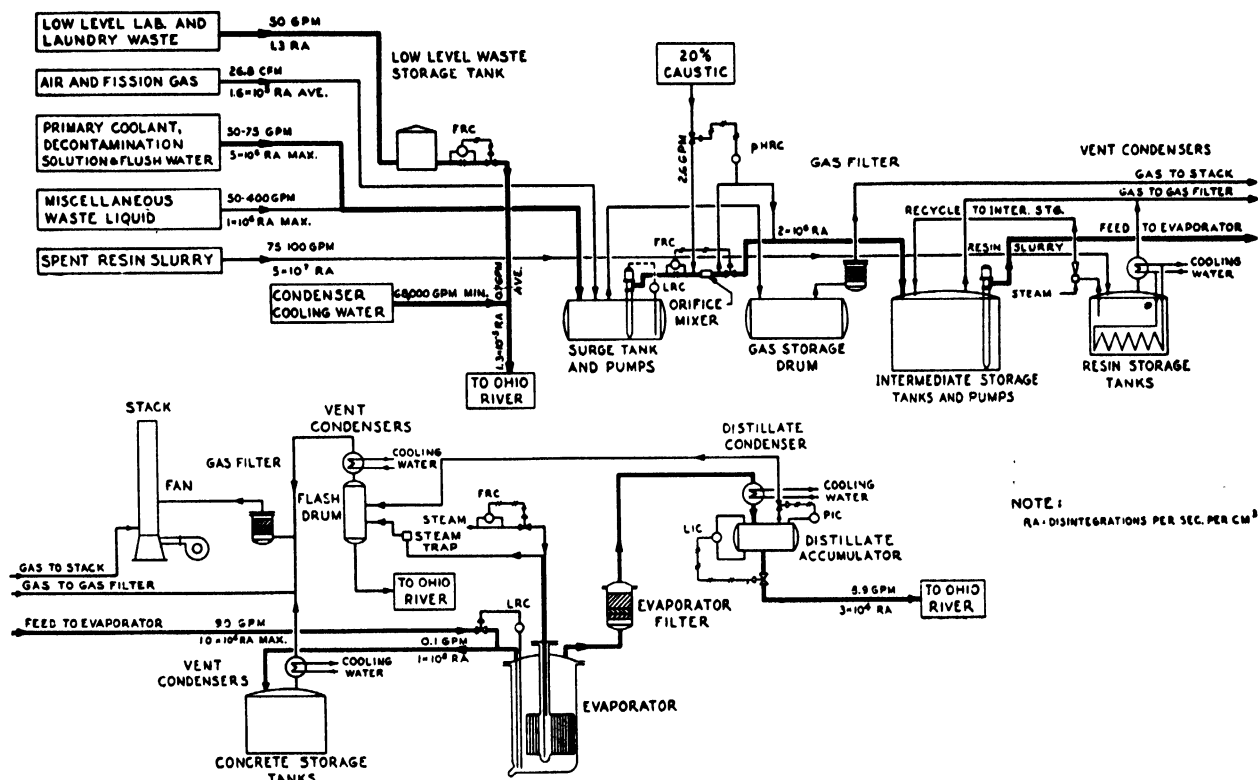
Figure 19. Waste disposal system schematic
