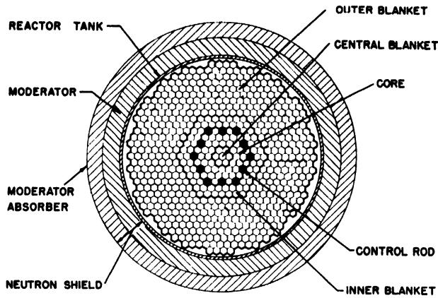
Figure 3. Schematic plan view of EBR-II reactor assembly
