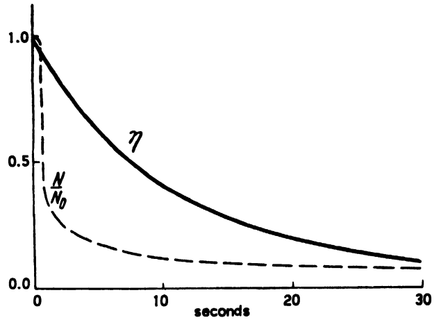
Figure 15. Changes in the water flow and reactor power after shutting off the electric supply of the circulating pump motors. X-axis: time; Y-axis: relative change in consumption of water ( \eta ) and the relative power N/N_0
