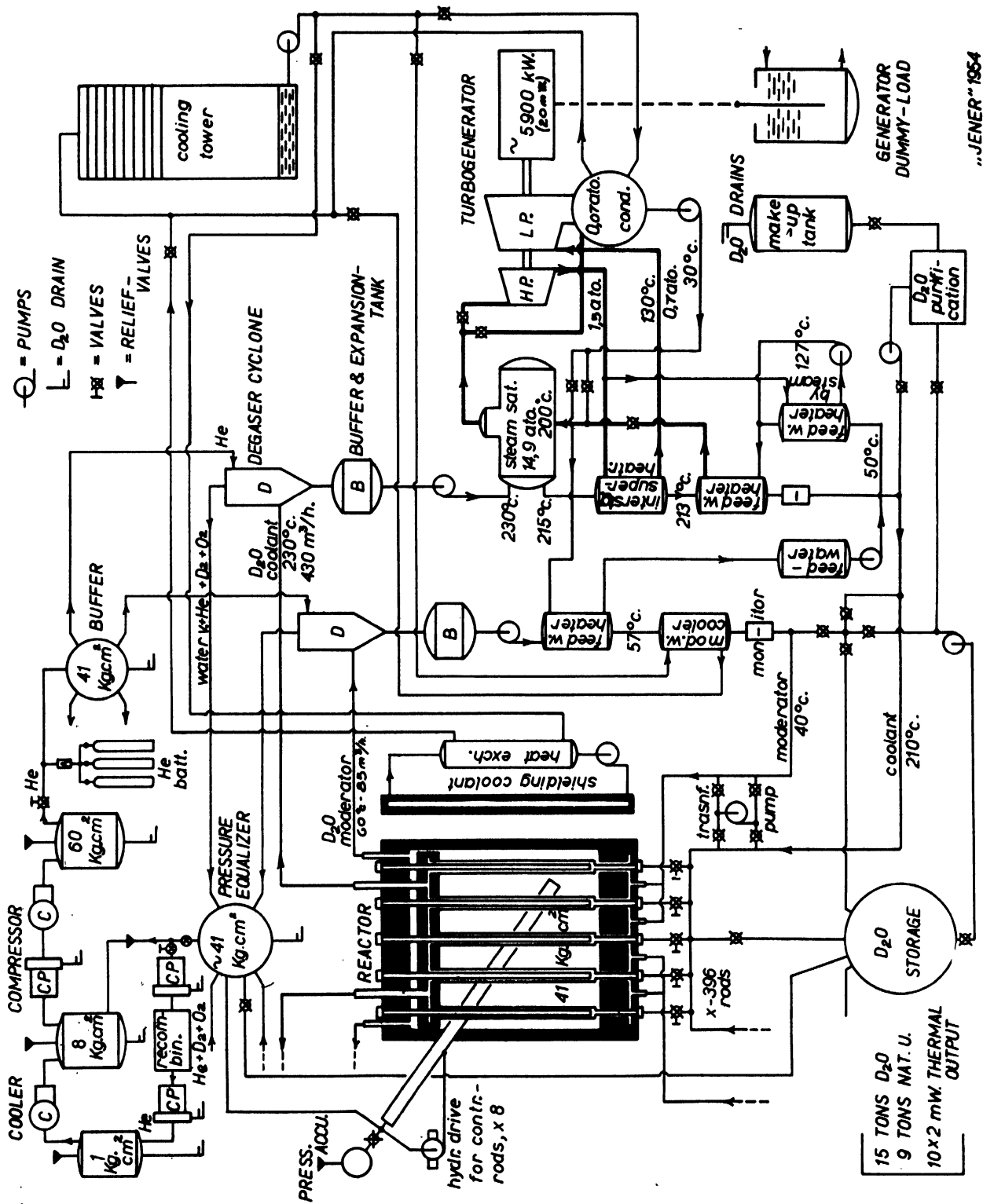
Figure 1. Flow sheet proposed for a pressurized, heavy water moderated and cooled reactor
