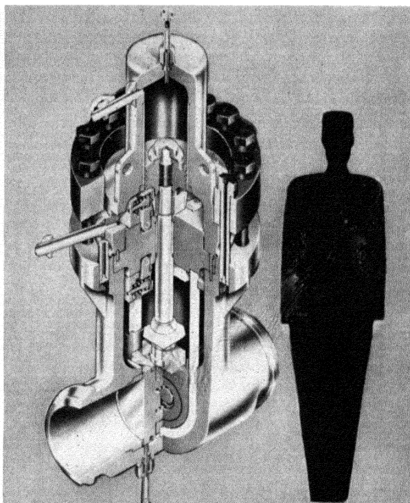
Figure 7. Main stop valve
