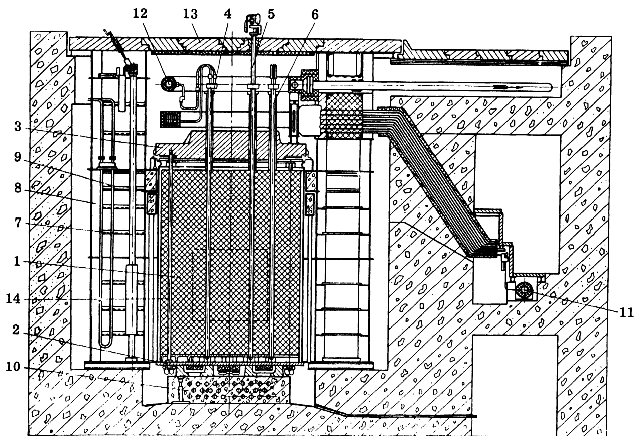
Figure 8. Atomic power station reactor: 1. Graphite brickwork. 2. Lower plate. 3. Upper plate. 4. Fuel channel. 5. Safety rod channel. 6. Automatic control rod. 7. Ionization chamber. 8. Side shield.
