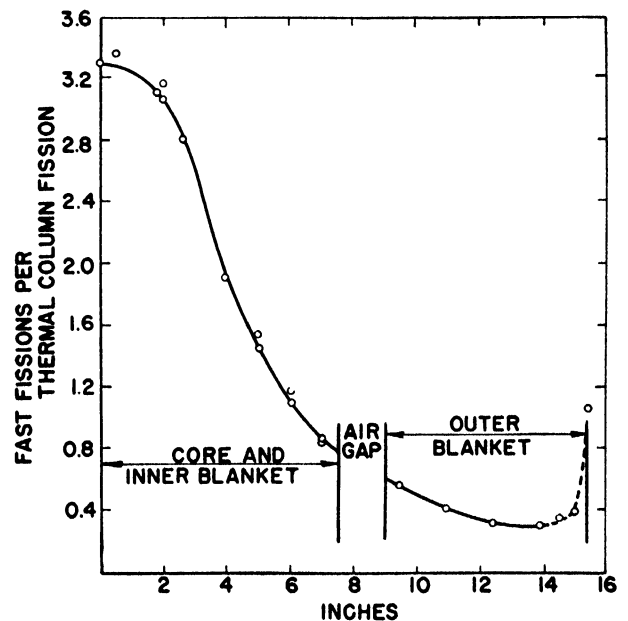
Figure 9. Radial U^{235} fission distribution along midplane of EBR
