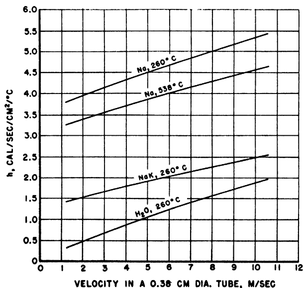
Figure 2. Comparison of heat transfer coefficients for Na and water
