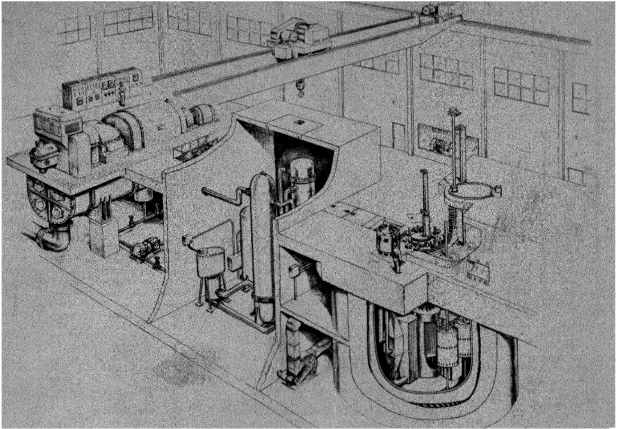
Figure 1. The EBR-II plant
