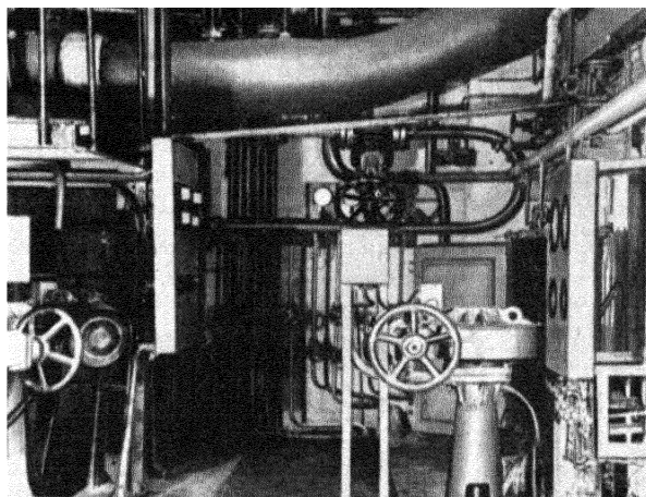
Figure 18. Part of the steam generator corridor. The open door of one of the four steam generator shielded boxes can be seen. At the top is the steam pipeline
