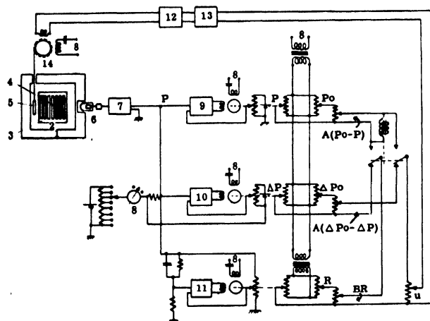
Figure 4. Schematic of automatic control device. 1. Concrete. 2. Reflector. 3. Moderator. 4. Uranium. 5. Regulating rod. 6. Ionization chamber. 7. Direct current amplifier. 8. Potentiometric switch. 9. Potentiometric power recorder. 10. "Vernier" potentiometric power recorder. 11. Potentiometric reactivity recorder. 12. Magnetic amplifier. 13. Electronic preamplifier. 14. Two phase engine
