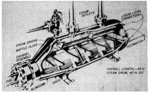
Figure 12. HRT 5 Mw steam generator
