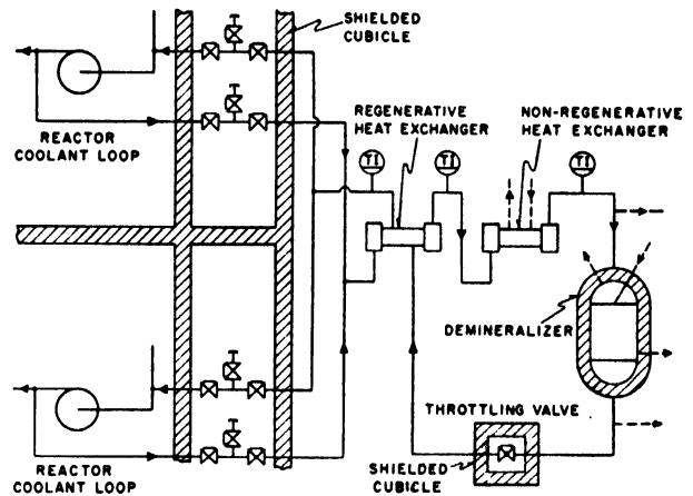
Figure 16. Purification system schematic
