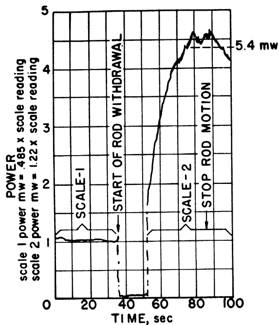
Figure 13. Power variation during reactivity addition: initial power 485 kw
