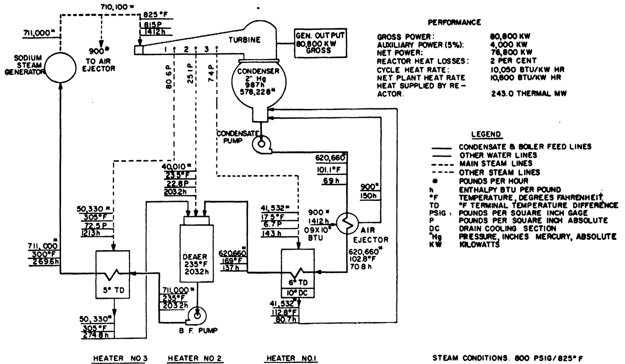
Figure 13. Preliminary heat balance
