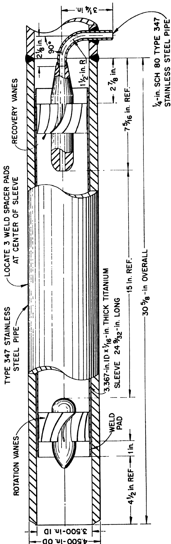
Figure 11. Gas separator
