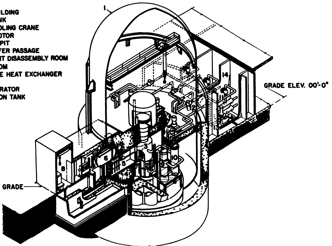
Figure 8. Perspective view of reactor building
