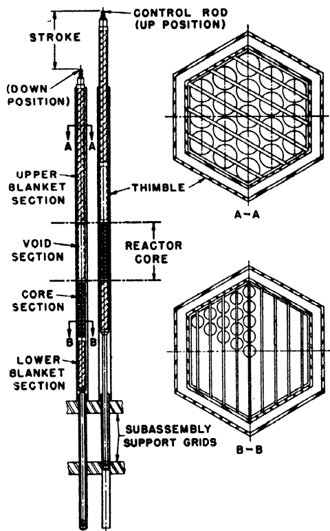
Figure 9. Control subassembly
