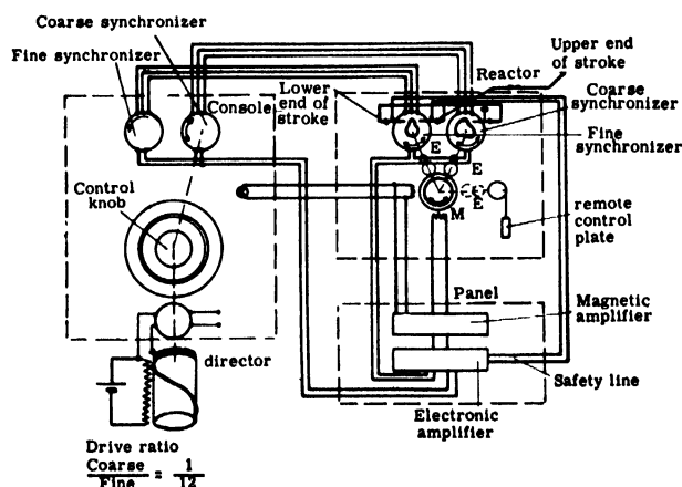
Figure 2. Director control
