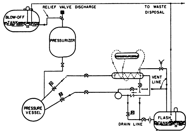
Figure 18. Coolant discharge system schematic
