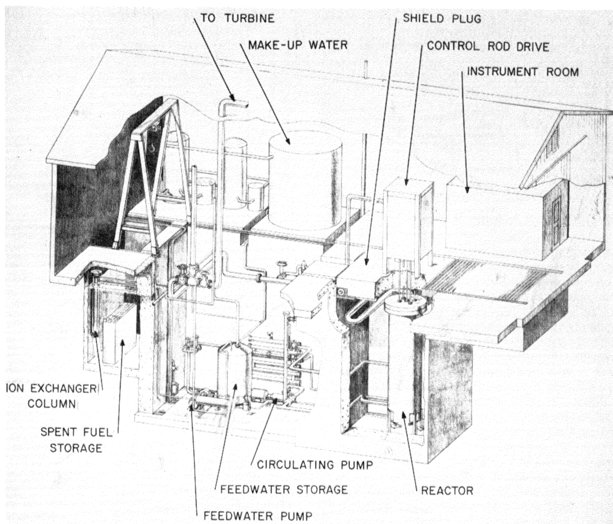
Figure 8. Reactor building
