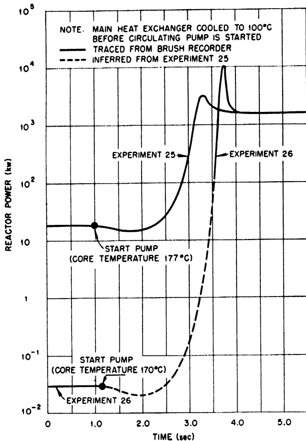
Figure 5. Power response of HRE during reactivity increase of 0.8%/sec
