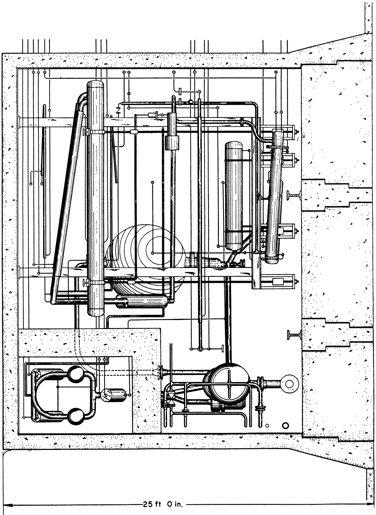
Figure 4. Reactor component arrangement—elevation
