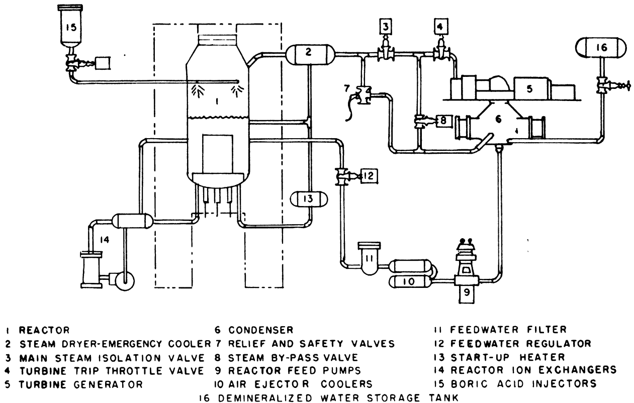
Figure 8. Schematic diagram of steam and feedwater system
