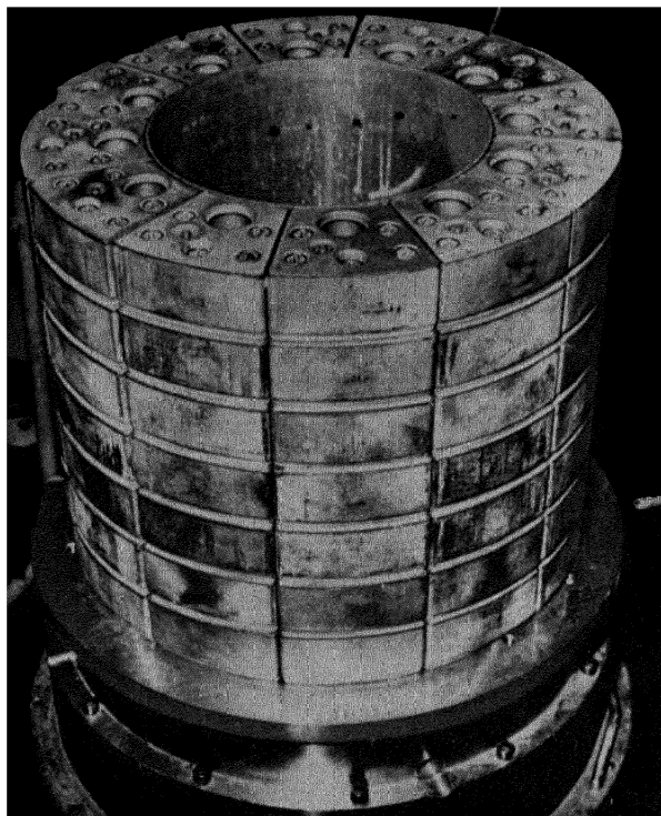
Figure 2d. Outer blanket of reactor
