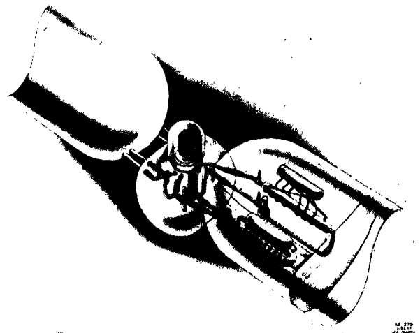
Figure 4. View of plant container showing location of equipment in two loops
