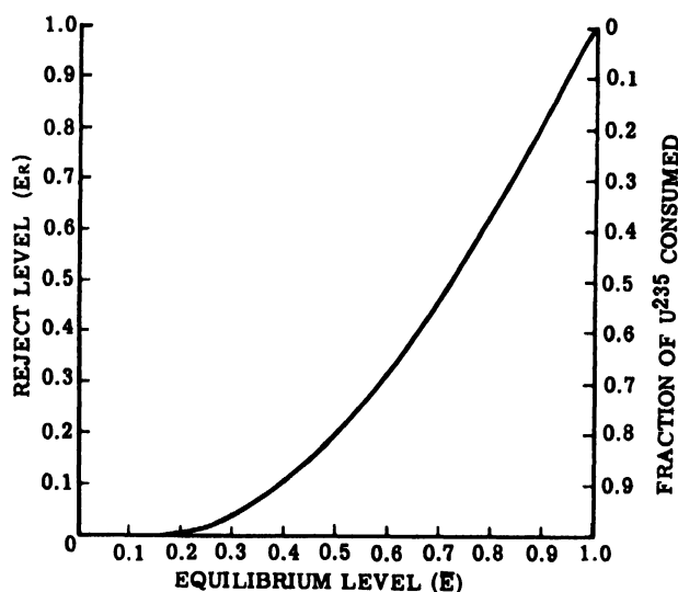
Figure 2. Reject U^{235} level E_r vs equilibrium level E
