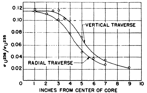
Figure 20. U^{238}/U^{235} fission ratio traverses in the EBR
