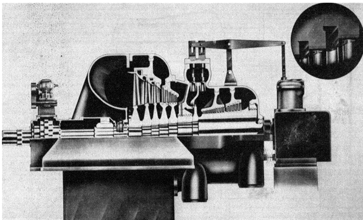
Figure 25. Turbine cross section
