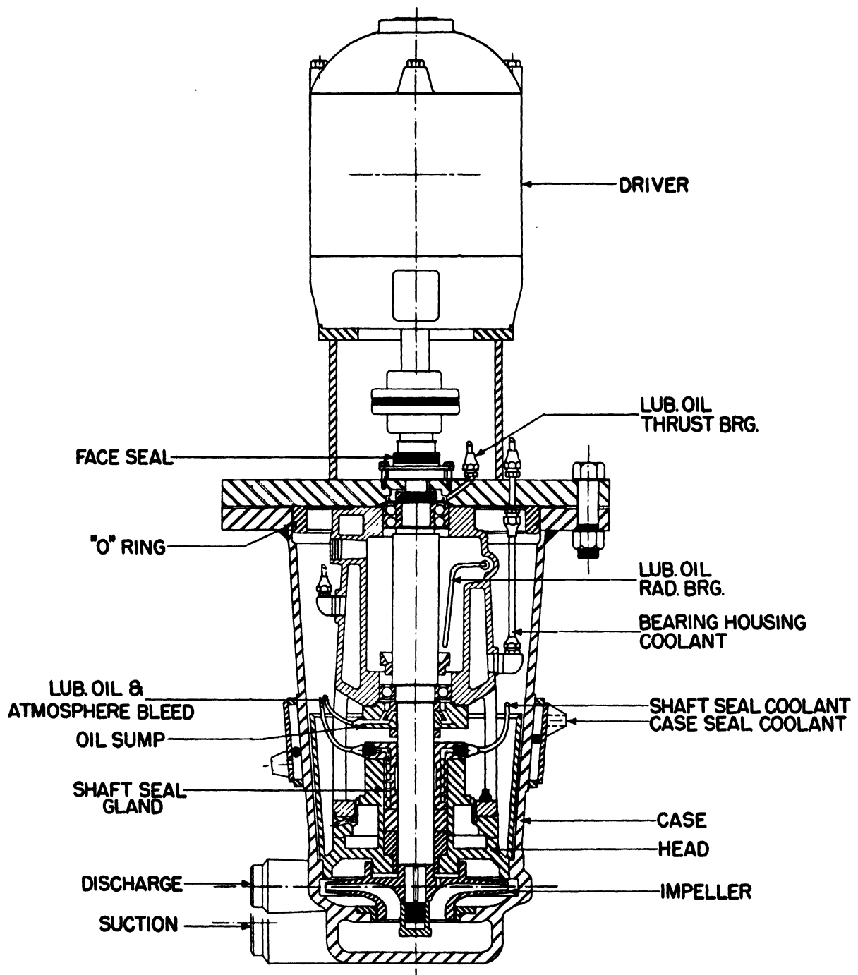
Figure 18. Cross section of main secondary sodium pump
