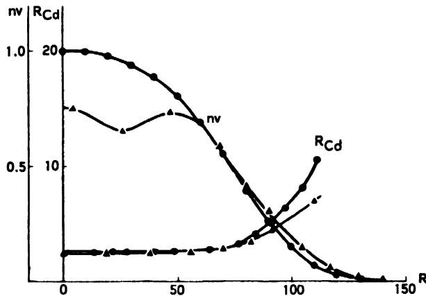
Figure 13. Distribution of resonance neutrons n\nu according to an Au indicator ( E_\gamma = 4.9 eV) and radial distribution of the cadmium ratio R_{cd} . Circular points are calculation (for uniform distribution of the substance of the absorbing rod); triangular points are experiment (with absorbing rods of the internal circle lowered)
