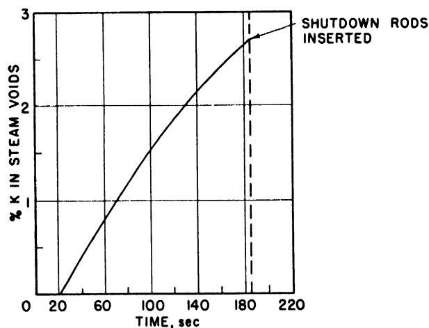
Figure 14. Reactivity addition during run of Fig. 15
