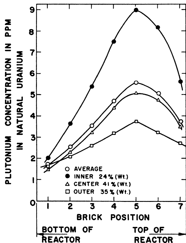
Figure 7. Plutonium distribution in the EBR outer blanket bricks
