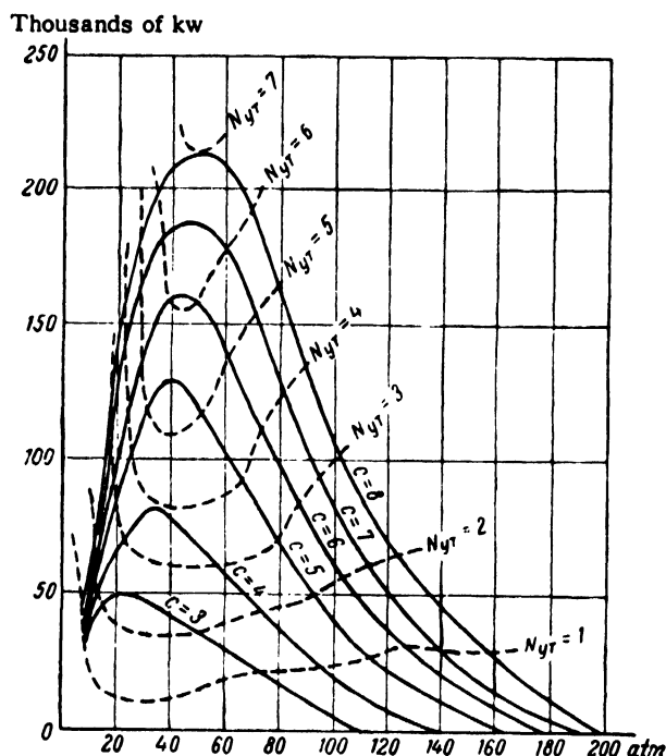
Figure 2. Dependence of heat-generating capacity of reactor on internal pressure with various concentrations of fissionable substance in working medium ( N_{sp} = N_{yr} )
