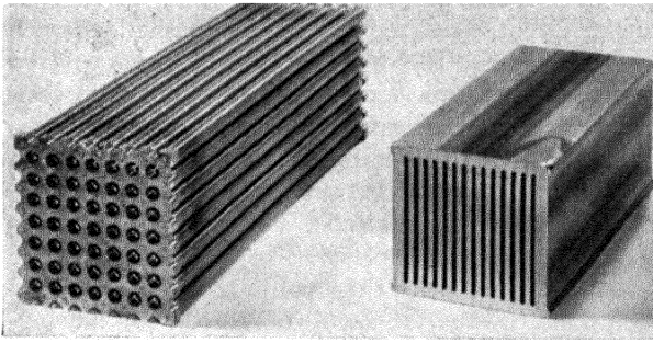
Figure 29. Failure of natural uranium fuel rod with intentionally defective cladding after testing in hot water
