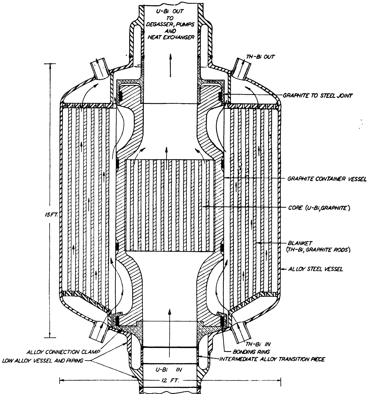
Figure 2. Reactor vessel, vertical section
