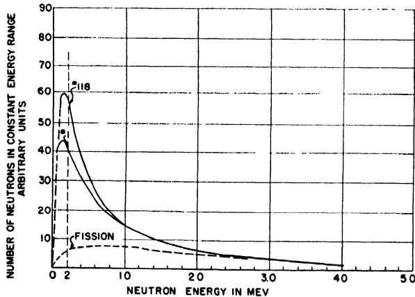
Figure 17. Neutron spectra from holes #1 and #118 of the EBR
