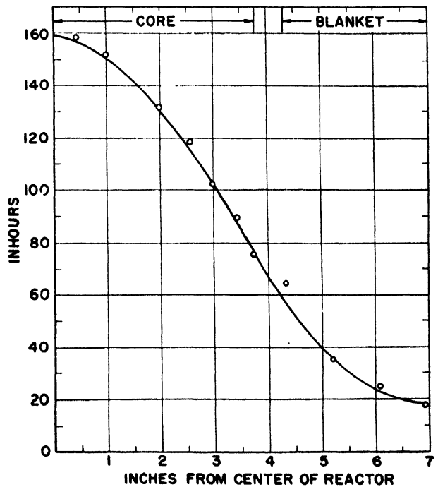
Figure 21. Inhour value of a fuel rod in EBR
