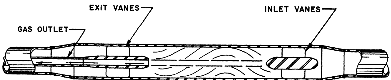
Figure 5. Axial flow gas separator
