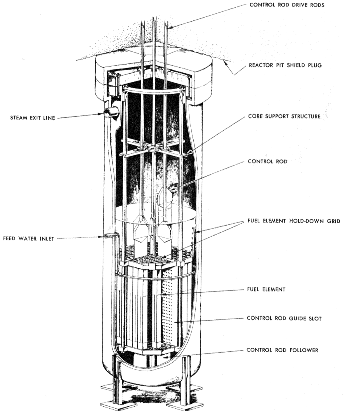
Figure 3. Core assembly in reactor vessel
