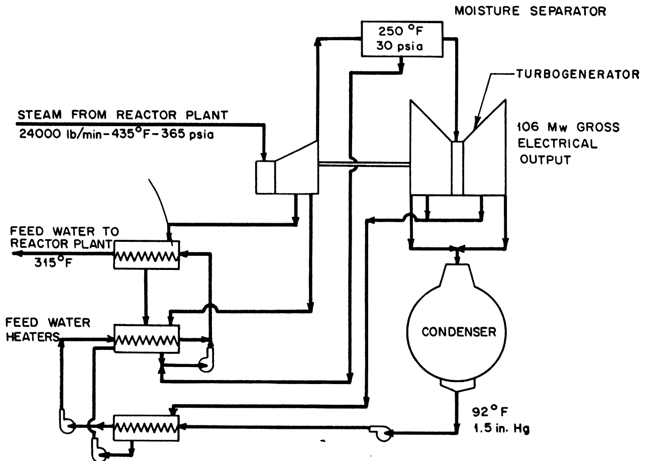
Figure 11. Flow diagram for turbogenerator
