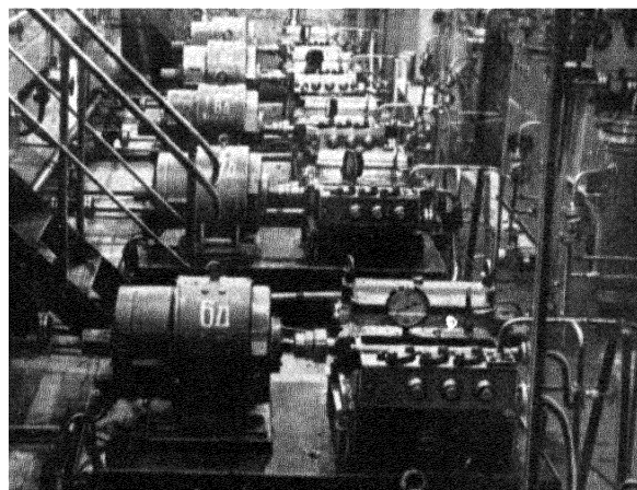
Figure 19. General view of one of the main circulating pumps
