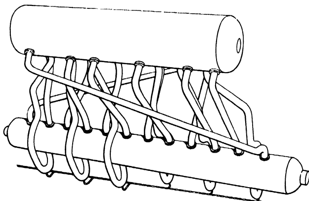
Figure 8. Steam generator with straight tube heat exchanger
