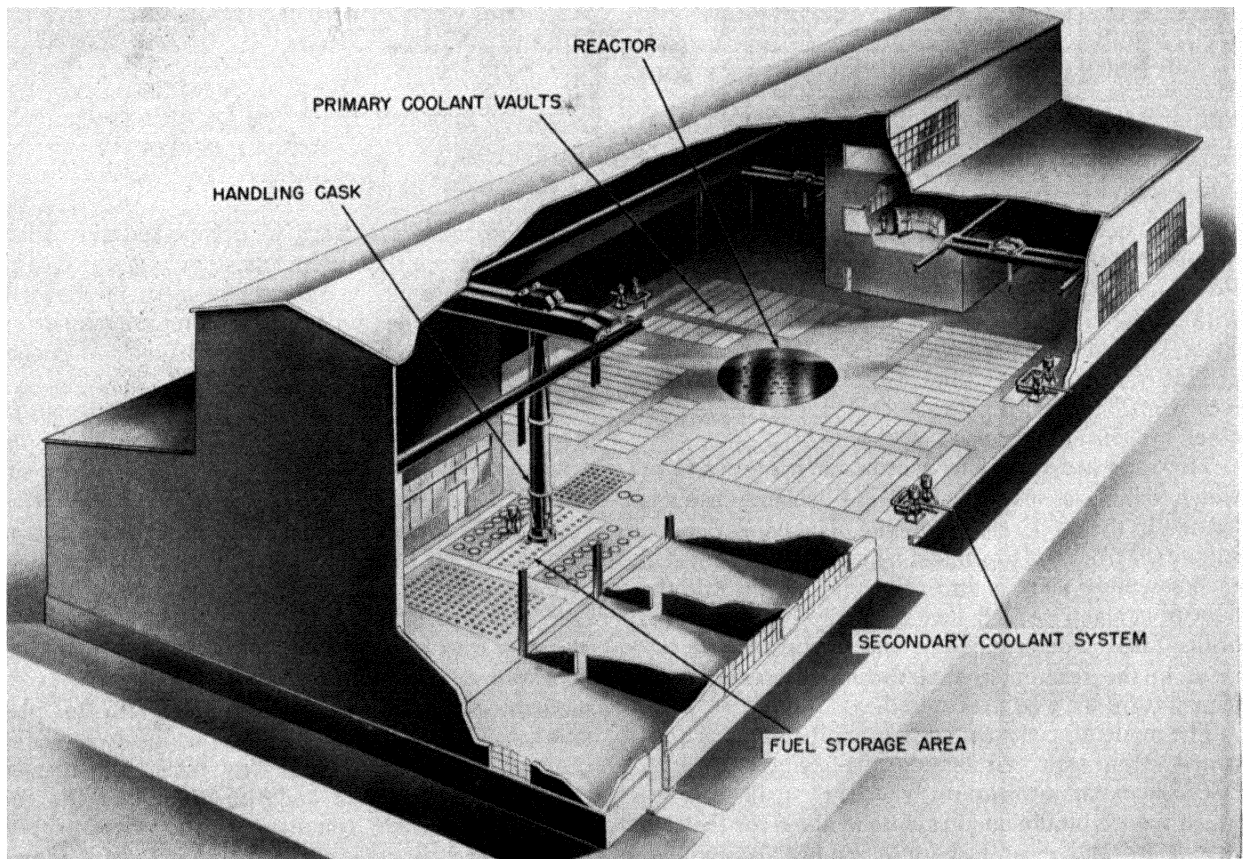
Figure 3. Aerial view of 75 megawatt reactor floor plan
