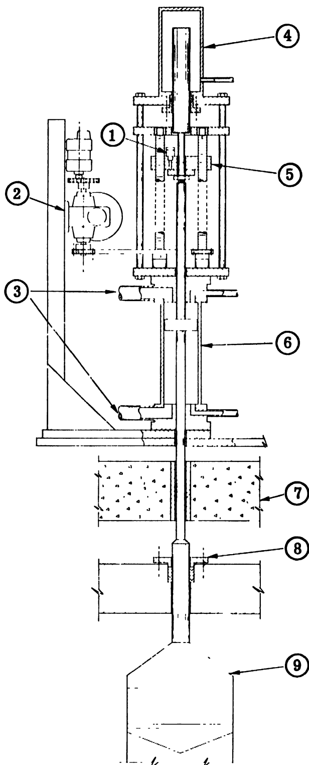
Figure 6. Diagram of control rod drive. (1) Control switch; (2) Drive motor; (3) Compressed air; (4) Balancing cylinder; (5) Travelling nut; (6) Pneumatic cylinder and piston; (7) Shield plug; (8) Packing gland; and (9) Control rod
