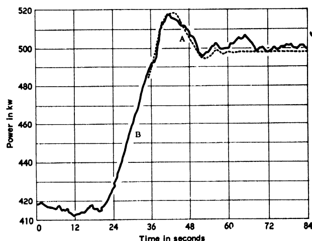
Figure 3. u = (\Delta P_0 - \Delta P) control. Change in power requirements. A: curve obtained with analog computer. B: curve obtained with the Saclay reactor
