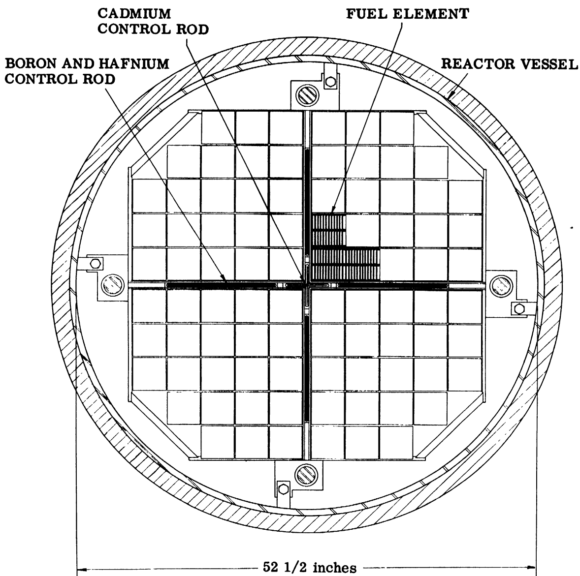
Figure 4. Cross section through reactor core
