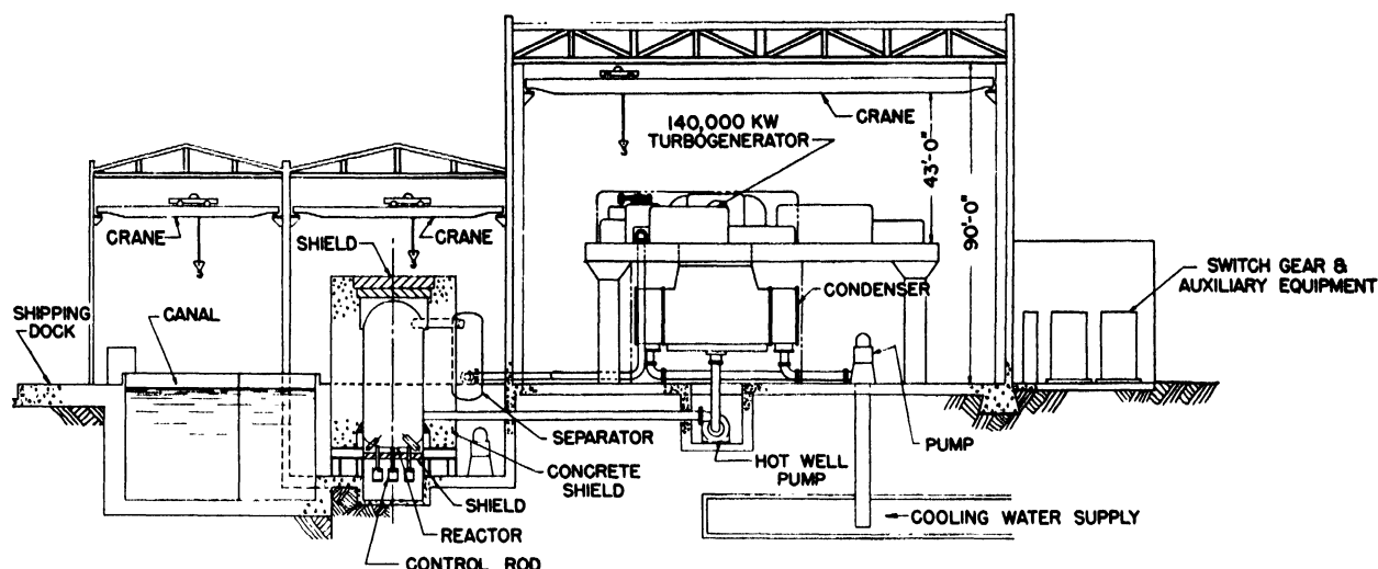
Figure 5. Elevation view of central station 1000-Mw D 2 O boiling reactor
