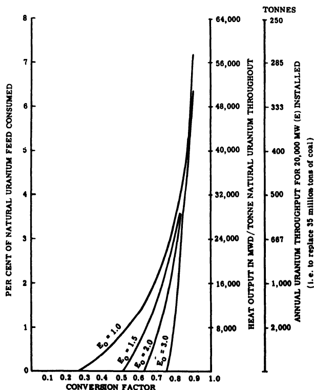
Figure 3. Natural uranium fuel requirement vs conversion factor
