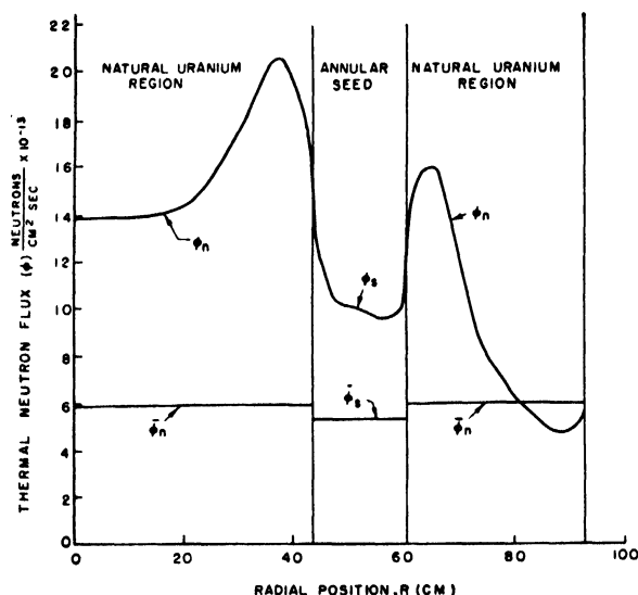
Figure 14. Radial distribution of thermal neutron flux
