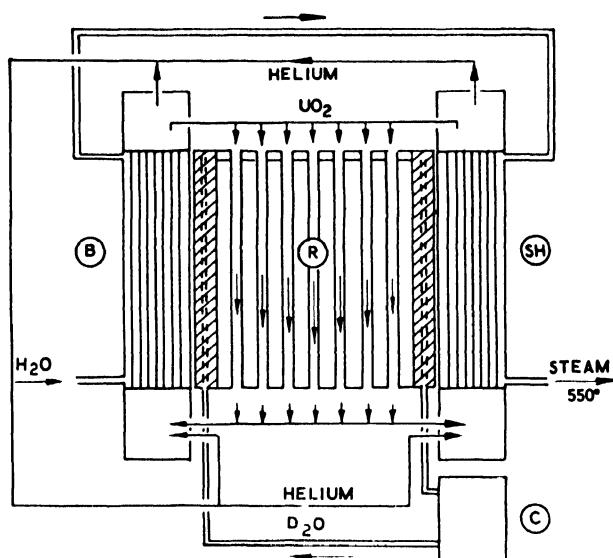
Figure 3. Flow sheet of heterogeneous reactor fuelled with a dry suspension of uranium oxide. R is reactor vessel containing graphite fuel tubes, cold heavy water as moderator and a graphite reflector; B is boilerpart of heat exchanger; SH is superheater part of heat exchanger; and C cooler of heavy water circuit
