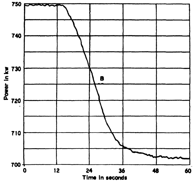
Figure 5b. u = (\Delta P_0 - \Delta P) - BR control. Negative power requirement
