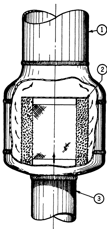
Figure 9. Catalytic recombiner. 1. 24" diameter outlet. 2. Catalyst bed, 24" diameter, 20" high, 4" thick. 3. 16" diameter inlet
