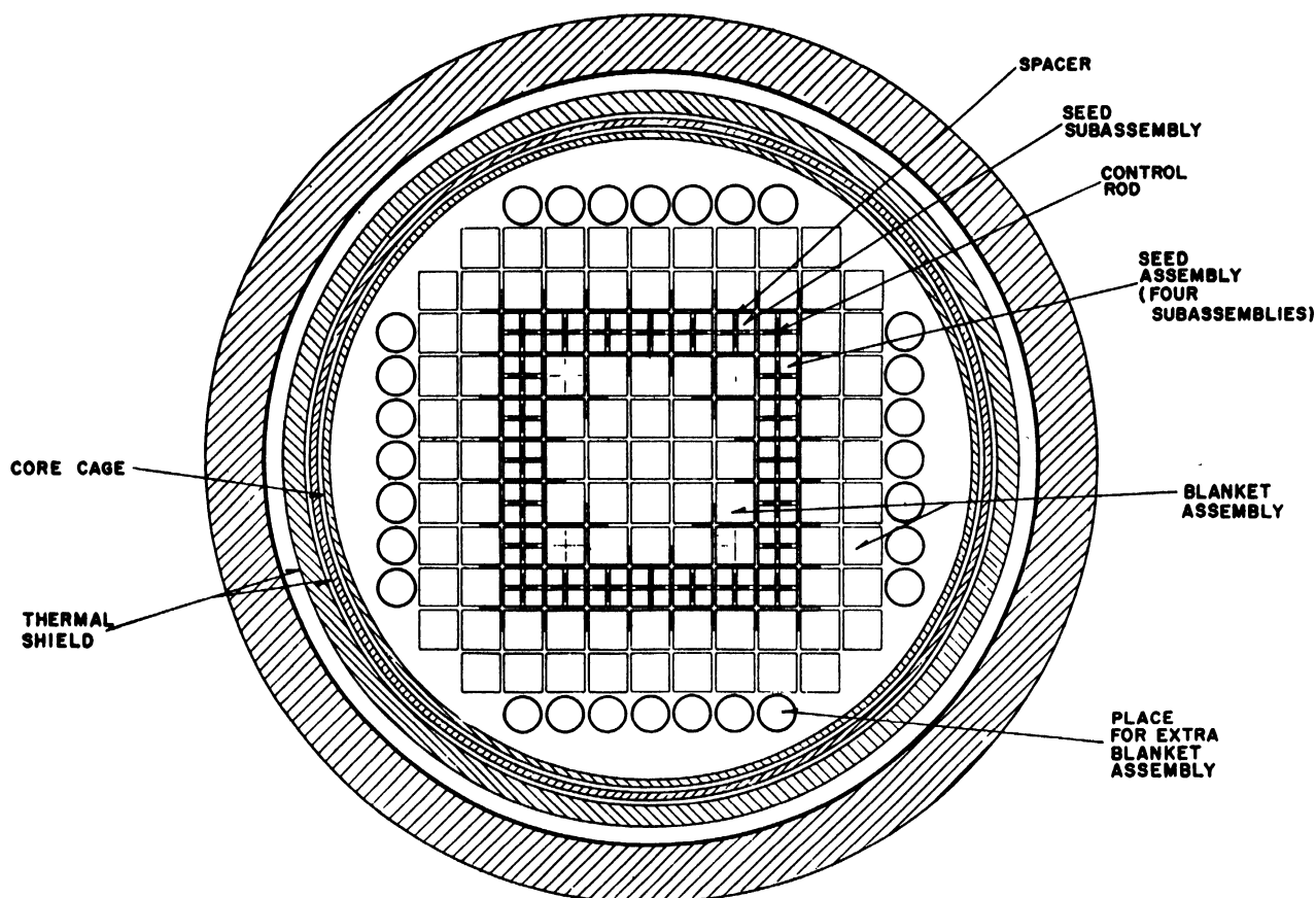
Figure 11. Cross-section view of reactor vessel and core
