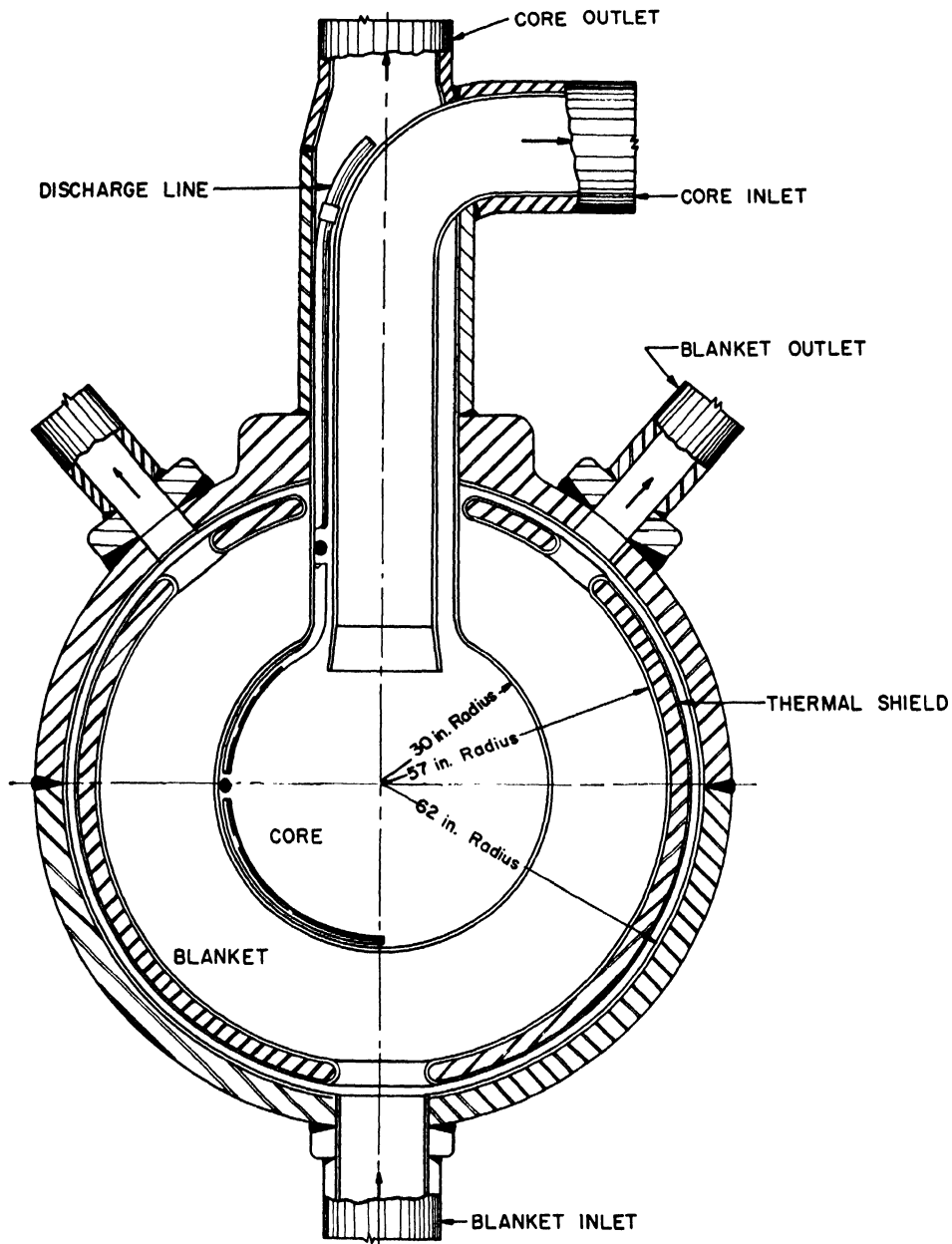
Figure 4. Two-region reactor with "concentric inlet and outlet" core
