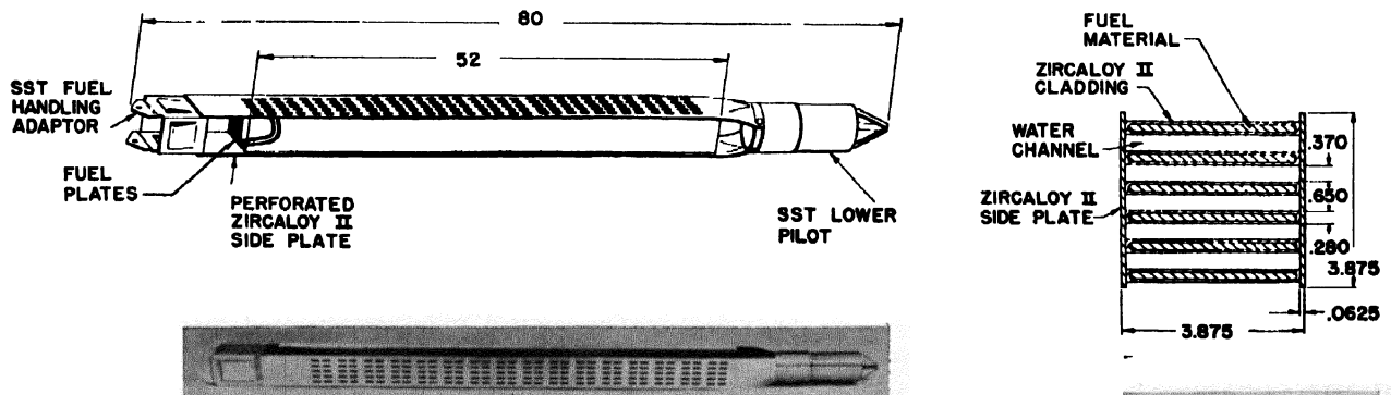
Figure 2. Above: EBWR fuel assembly. At right: End view of EBWR fuel assembly
