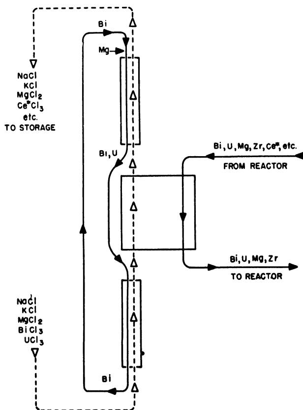
Figure 5. Fuel process
