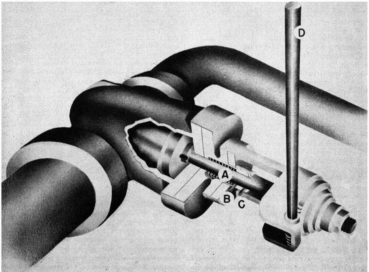
Figure 16. Arrangement for valve with frozen sodium seal
