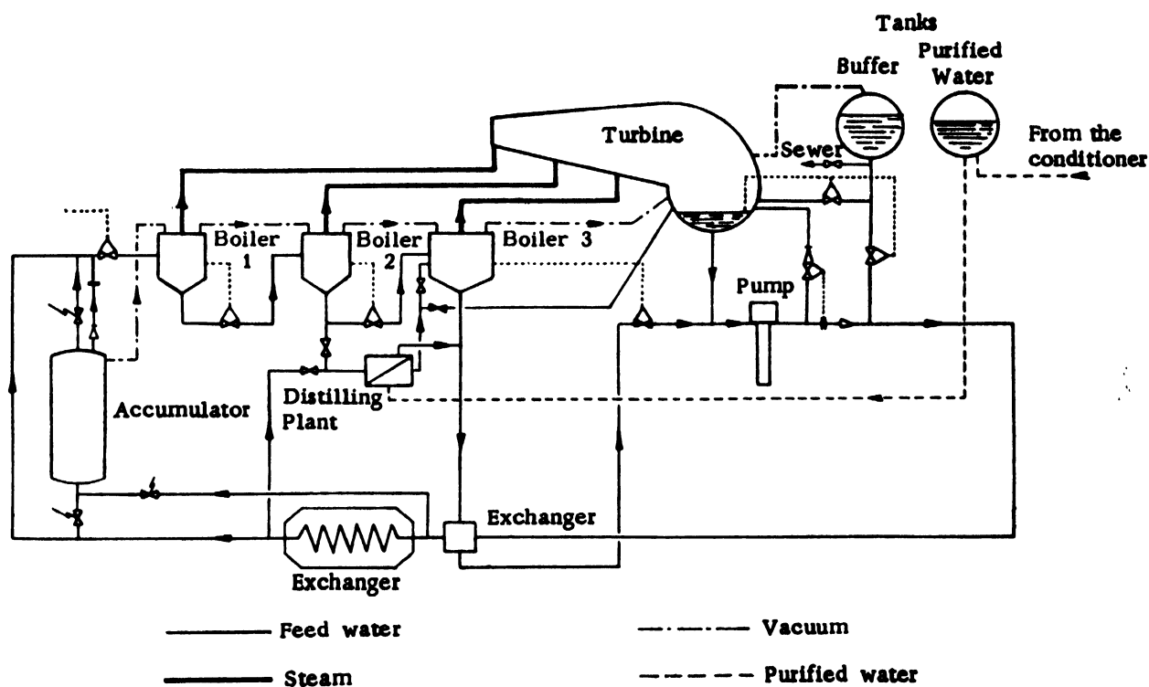
Figure 2. Schematic of the G1 arrangement
