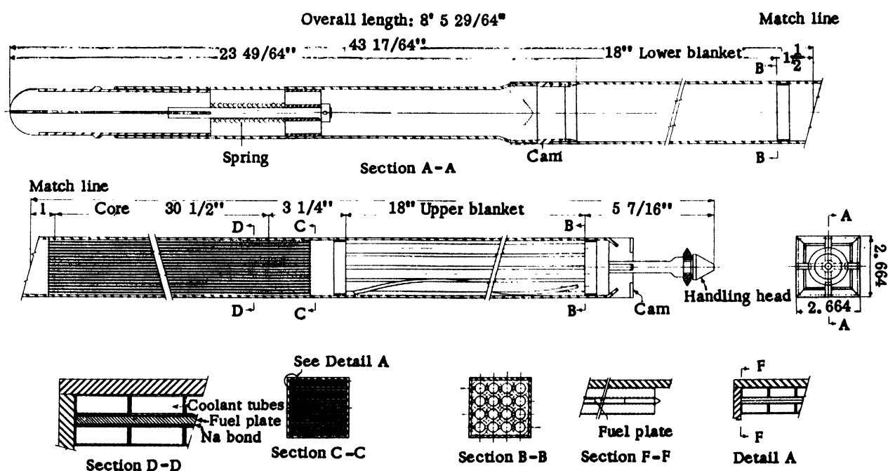
Figure 3. Flat plate sub-assembly
