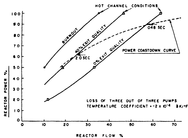
Figure 33. PWR hot channel conditions during loss-of-flow casualty
