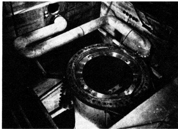
Slide 7. Photograph of top of reactor vessel
