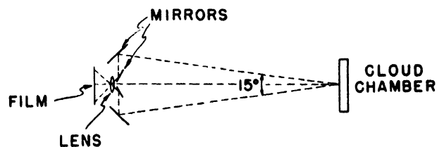
Figure 14. Stereoscopic arrangement for recording tracks
