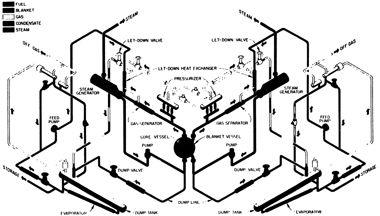
Figure 1. Reactor flow sheet—schematic
