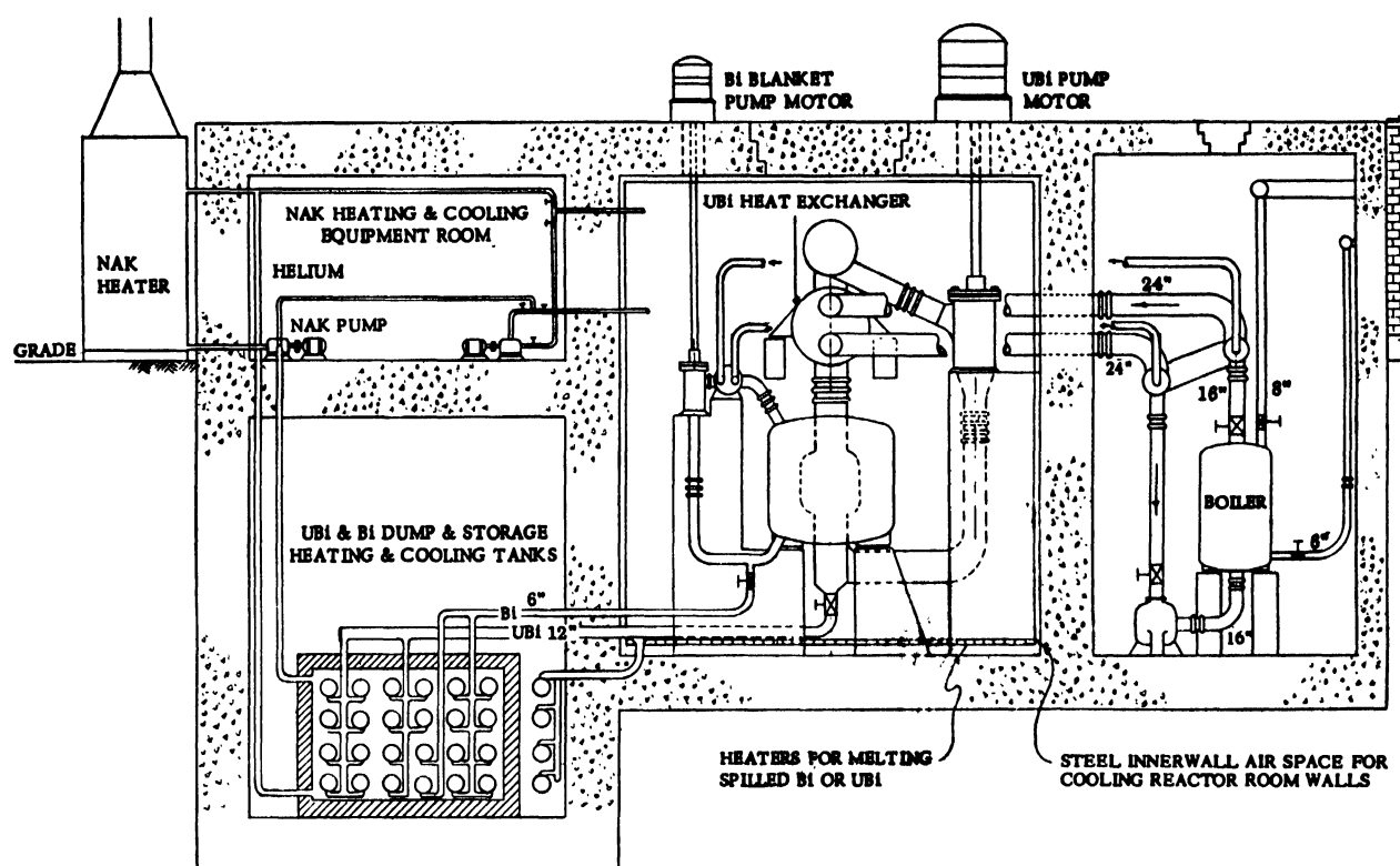
Figure 4. Liquid metal fuel reactor power plant, sectional view
