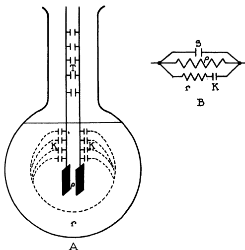
Fig. 4. Capacitance Effects in a Conductance Cell.
