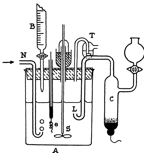
Fig. 1. Arrangement for Oxidation-Reduction Titration.
