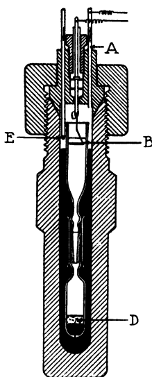
Fig. 4. Apparatus for Measuring the Potential of the Galvanic Cell
