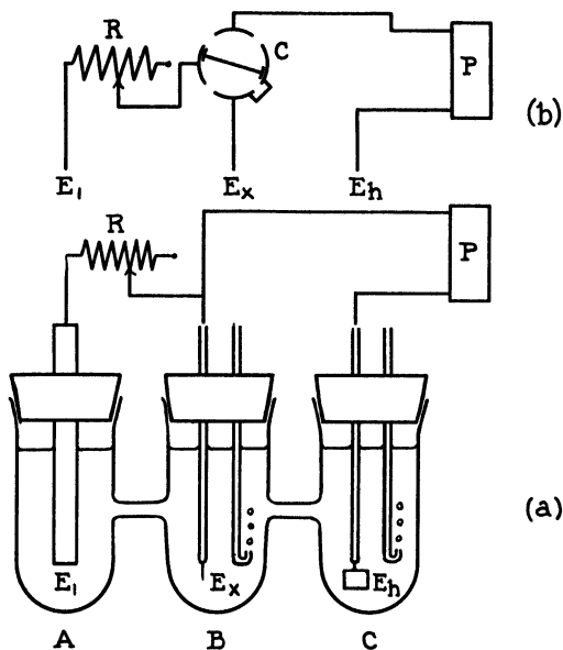
Fig. 1. An Apparatus for Measuring Overvoltage.
