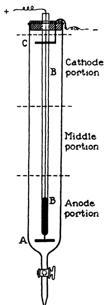
Fig. 2. Simple Hittorf Transference Apparatus.
