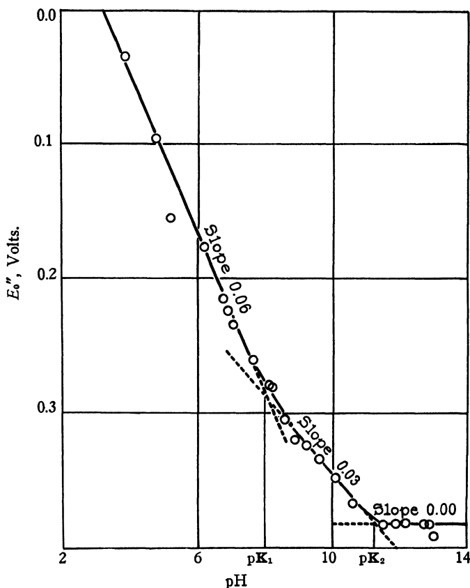
Fig. 4. The pH Dependence of E''_0 for the Oxidation-Reduction System: \beta -Sulphonate of Anthraquinone.
