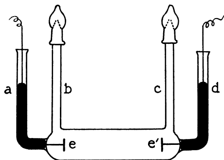
Fig. 2. A Conductance Cell.
