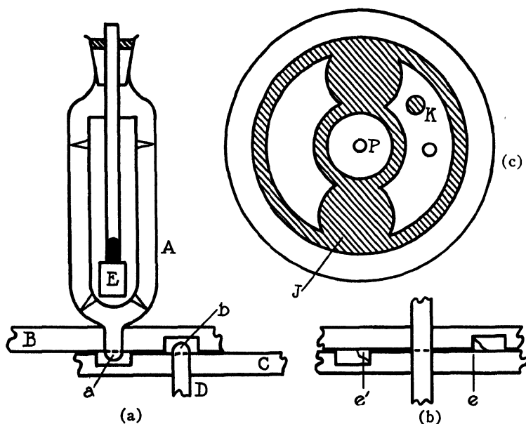
Fig. 6. Device for Forming a "Sheared Boundary."
