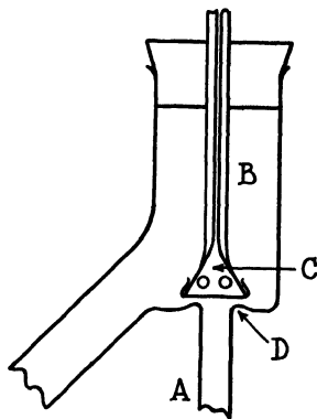
Fig. 5. Denison and Steele's Device for Forming a Moving Boundary.
