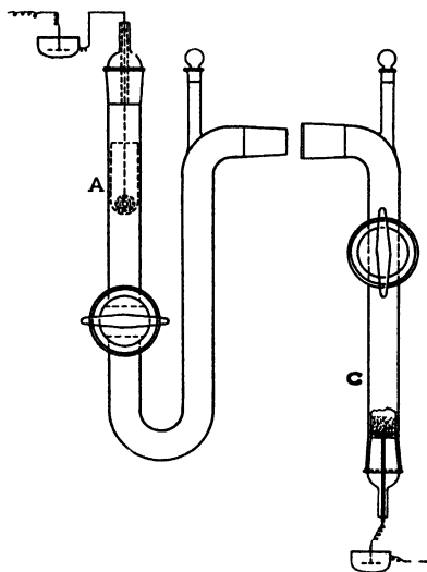
Fig. 3. Washburn's Hittorf Transference Apparatus.
