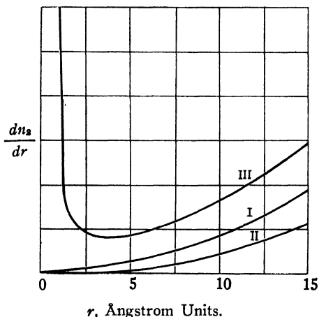
Fig. 6. The Dependence of dn_s/dr on r (after Bjerrum).
