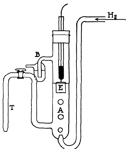
Fig. 1. Hydrogen Electrode.
