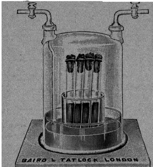
Fig. 25.—Bulloch Jar. The air inside the jar is replaced by a neutral gas (coal gas or \text{CO}_2 ) after the tubes have been placed inside. When the air has been expelled the taps are closed.
