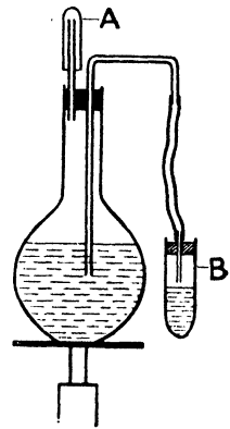
Fig. 6. — Apparatus for keeping sterilised water. Water comes out from the tube B, and the air which displaces the escaping water comes in through the tube inside A. Both ends (A and B) must therefore be protected. End B is placed in a tube containing alcohol. End A is covered by a tube containing usually cotton wool.
