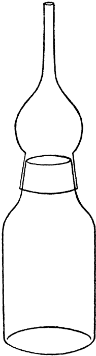
Fig. 9e — Hansen Flask. The lower part is an ordinary flask with a ground neck. The upper erection is the hollow stopper, ground in the lower part to fit the neck of the flask and plugged with cotton wool in the upper part.
