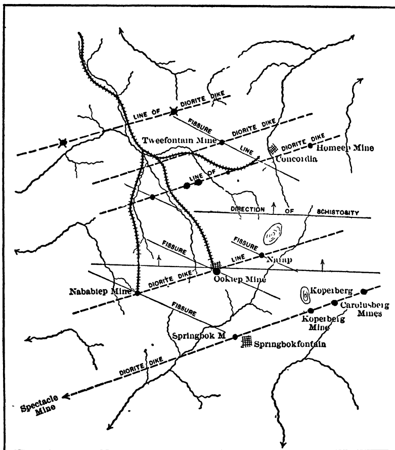
FIG 50.—MAP OF COPPER DISTRICT OF LITTLE NAMAQUALAND, CAPE COLONY. (KUNTZ)
