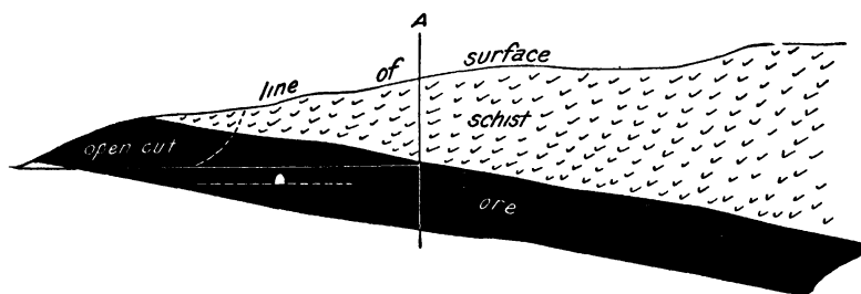
FIG 108.—CROSS-SECTION OF OREBODY, ELIZABETH MINE, SOUTH STRAFFORD, VERMONT
