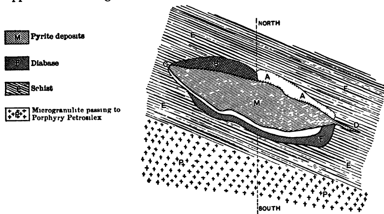
FIG. 43 — PLAN OF SAN DOMINGO PYRITE DEPOSIT, PORTUGAL (GONZALES)
