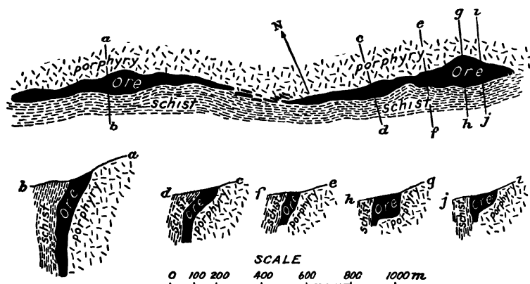
FIG 38.—CROSS-SECTION OF OREBODIES, RIO TINTO, SPAIN. (GONZALES)
