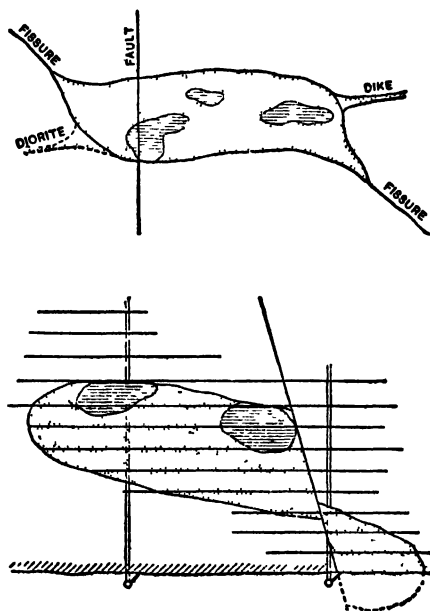
FIGS. 48 AND 49.—VERTICAL AND HORIZONTAL SECTIONS THROUGH OOKIEP MINE. (KUNTZ)
