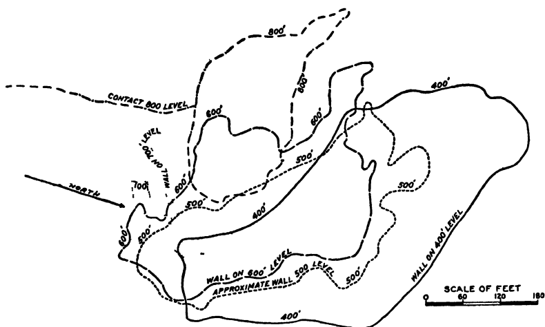
FIG 60 —LEVEL MAP OF MT LYELL, SHOWING CONTOUR OF OREBODIES AT VARIOUS LEVELS (FROM COMPANY'S MAPS)
