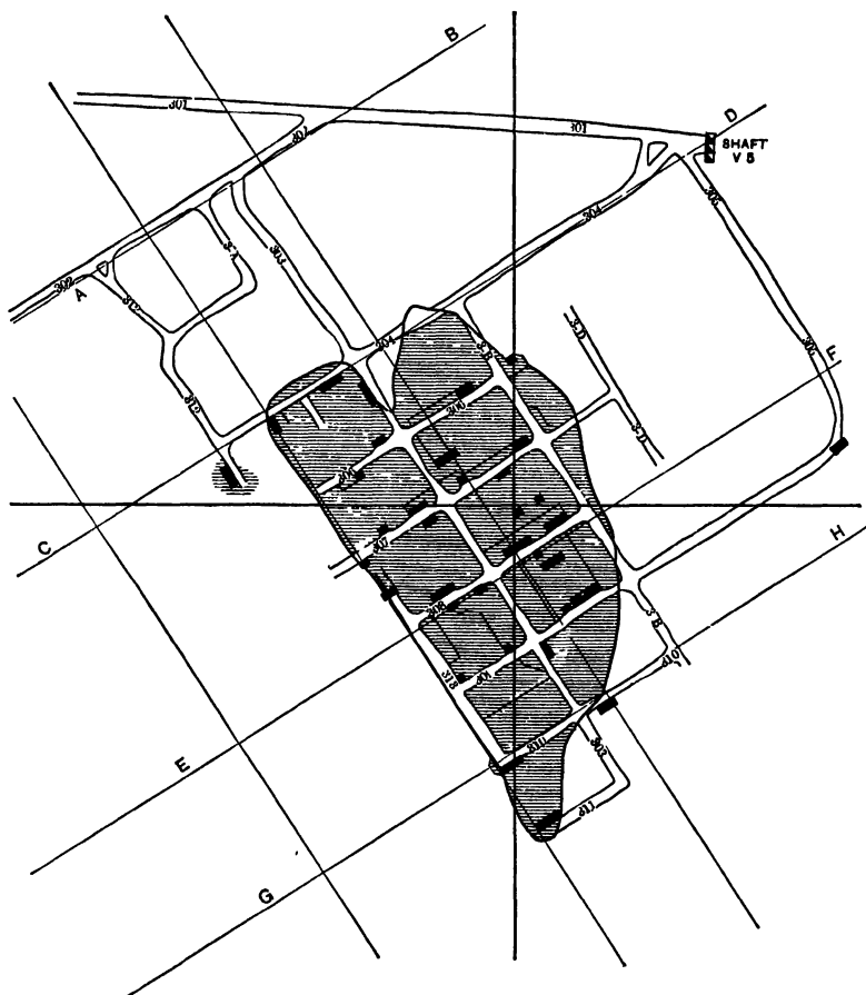
FIG 95 — MAP OF THIRD LEVEL, CAPOTE MINE, CANANEA
