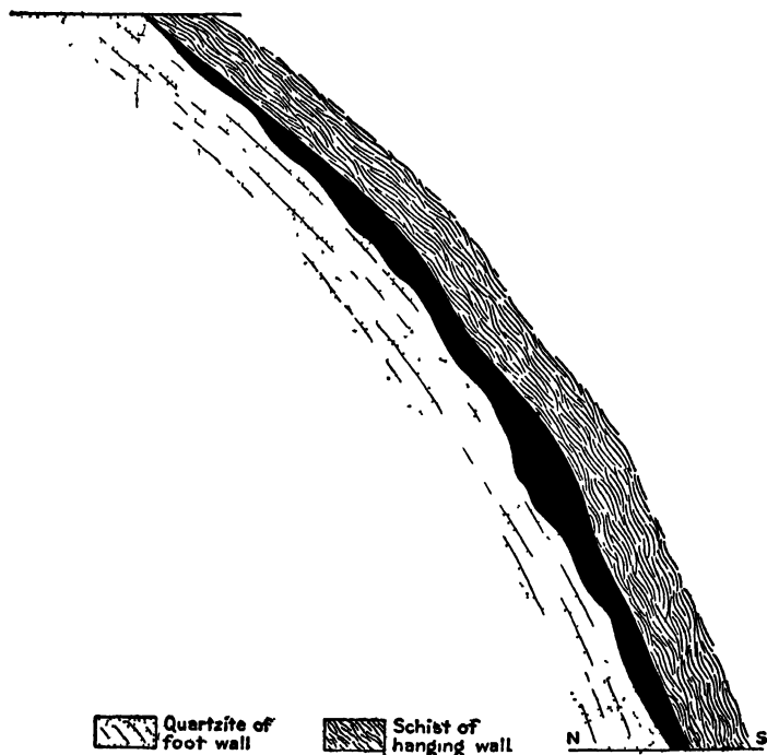
FIG. 155 — IDEALIZED VERTICAL NORTH-SOUTH SECTION, FERRIS-HAGGARTY MINE, ACROSS THE OREBODY, SHOWING CONVEXITY AND IRREGULAR DIP. (SPENCER)
