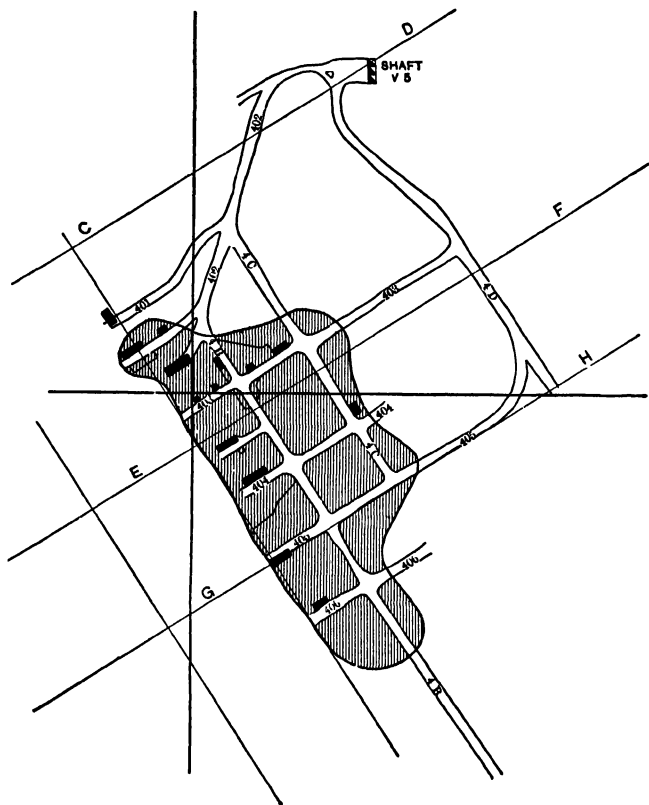
FIG 96 — MAP OF FOURTH LEVEL, CAPOTE MINE, CANANEA
