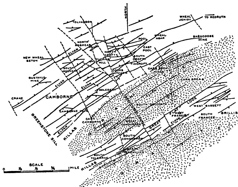
FIG. 22 — PLAN OF TIN-COPPER VEINS, CAMBORNE, CORNWALL, ENGLAND
