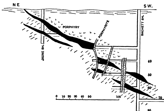
FIG. 31 — VERTICAL SECTION OF THE BOGOSLOVSK MINE. RACHETT SHAFT ON RIGHT, JAUNE ON LEFT
