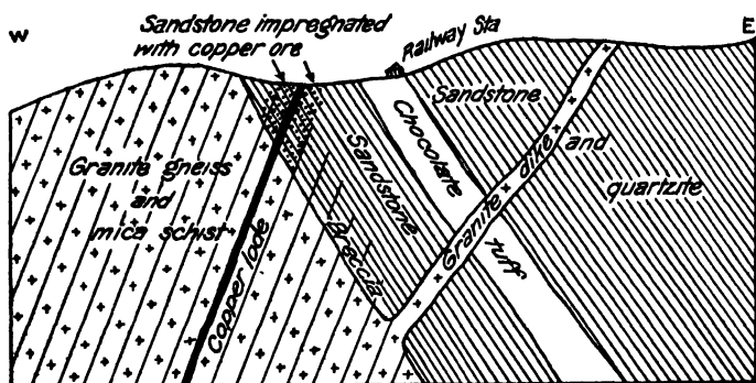
FIG 58 — SECTION ACROSS AVINO COPPER DEPOSIT, WESTERN AUSTRALIA
