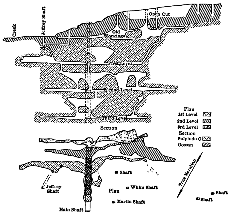
FIG. 148 — SECTION, AND MAP OF LONDON MINE, DUCKTOWN, TENN.
