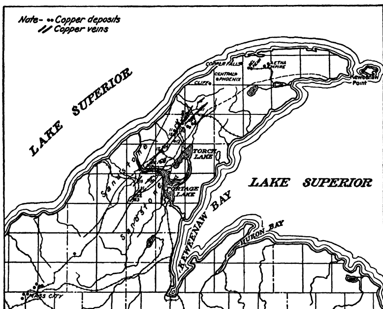
FIG. 132. — INDEX MAP OF MICHIGAN COPPER MINES
