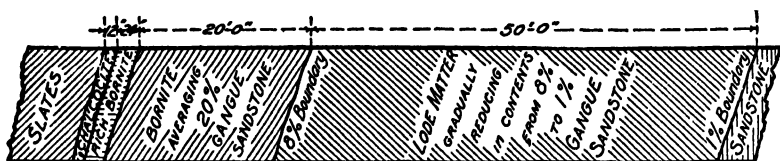
FIG 33 — CROSS-SECTION, ANNENSKY LODGE, SPASSKY MINE, SIBERIA
