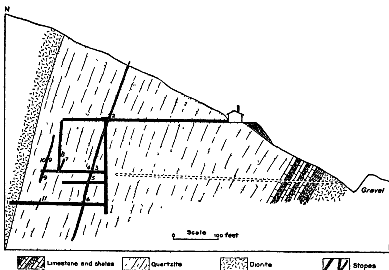
FIG. 156. — SECTION OF DOANE MINE, WYOMING (SPENCER)
