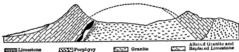
FIG. 101 — CROSS-SECTION SHOWING GEOLOGICAL RELATIONS OF JIBOSA CONTACT DEPOSIT OF COPPER, DOLORES, NEAR JIMENEZ, CHIHUAHUA, MEXICO
