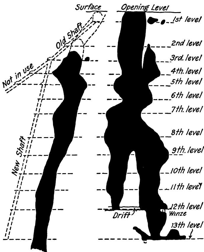
Vertical Section through Shaft
