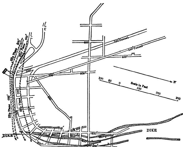
FIG 98.—LOS PILARES MINE PROJECTION OF MAIN DRIFTS IN 400-FOOT LEVEL, WITH INTERSECTIONS OF DIKE AND SLIP-PLANE (EMMONS)
