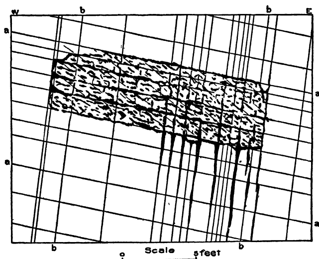
FIG 158.—DOANE MINE. HORIZONTAL SECTION OF OREBODY IN STOPE 9, ABOUT 25 FEET ABOVE 115 FEET LEVEL, SHOWING RELATION OF OREBODY TO THE LAYERS OF QUARTZITE AND THE NORTH-SOUTH FRACTURES. aa , STRATIFICATION; bb , NORTH-SOUTH CROSS FRACTURES. (SPENCER)
