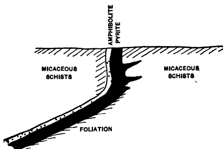
FIG 28 —VERTICAL SECTION KONGEN MINE, NORWAY (DE LAUNAY)
