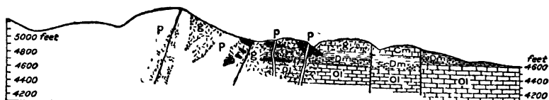
FIG 14c — IDEAL CROSS-SECTION OF MORENCI DEPOSITS
