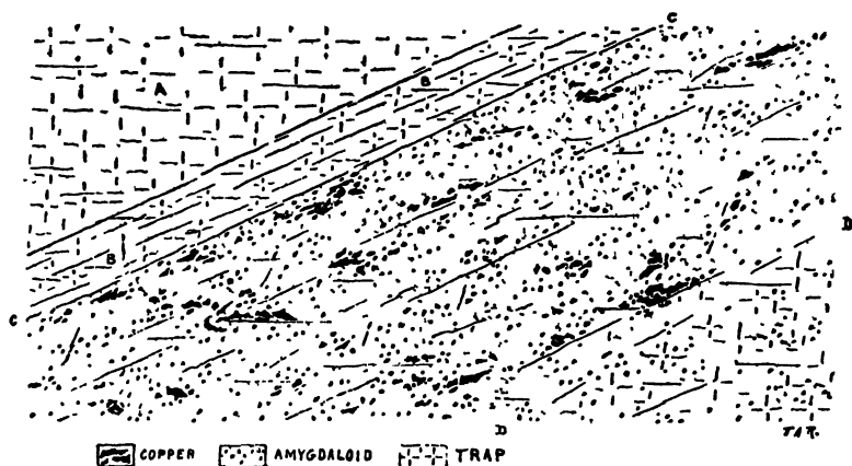
FIG 136 — SECTION OF QUINCY AMYGDALOID LODGE (RICKARD)
