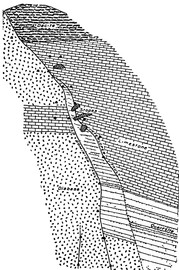
FIG 119 — VERTICAL SECTION OF THE OLD DOMINION MINE, SHOWING THE OCCURRENCE OF FAULT IN THE DIABASE OF THE FOOTWALL (RANSOME)
