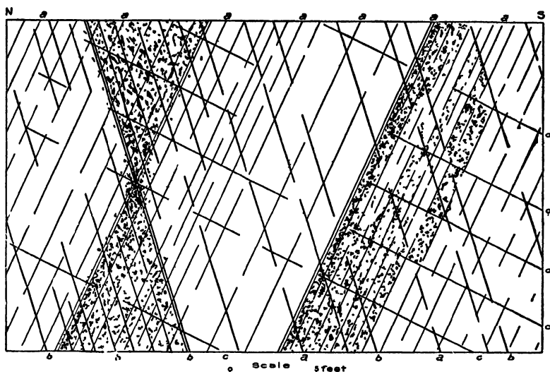
FIG 157.—DOANE MINE. DIAGRAMMATIC CROSS-SECTION IN LOWER PORTIONS OF STOPE 7 AND 8, SHOWING OCCURRENCE OF THE COPPER SULPHIDES IN BRECCIATED QUARTZITE FORMED ALONG INTERSECTING JOINT SYSTEMS aa , BEDDING PLANES AND PARALLEL JOINT FRACTURES, bb , STRONG SYSTEM OF JOINTS, cc , SUBORDINATE JOINTS, DISTRIBUTION OF SULPHIDES INDICATED BY STIPPLING (SPENCER)
