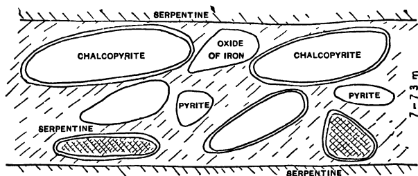
FIG 44 —CROSS-SECTION OF CORITZA OREBODIES, TURKEY
