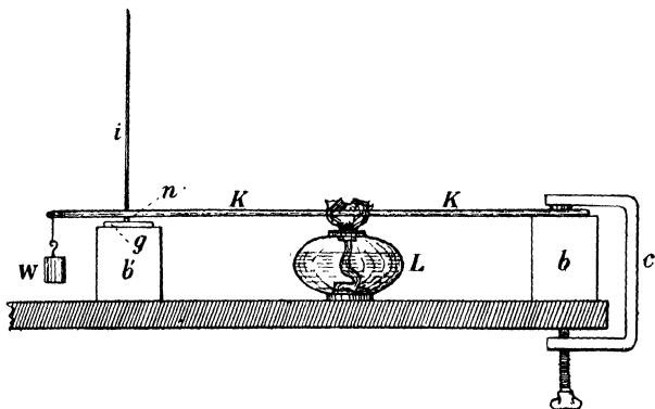
Experiment Illustrating Expansion by Heat.
