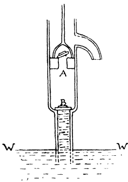
Diagram of Suction-pump.
