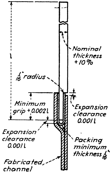
FIG. 67.—Flush channel mounting for acrylic sheet.
