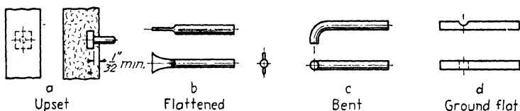
FIG. 29.—Typical rod inserts.
