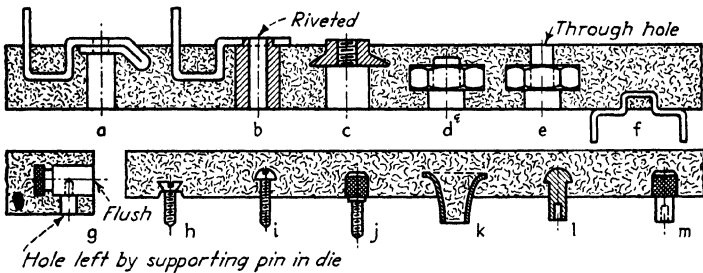
FIG. 34.—Punched, stamped, and formed inserts.
