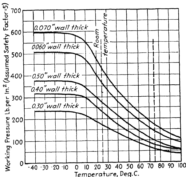
FIG. 92.—Working pressure vs. temperature, Saran tubing B-115, \frac{1}{4} in. o.d.
