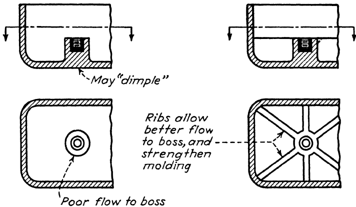
FIG. 26.—Proper design aids the molding operation.
