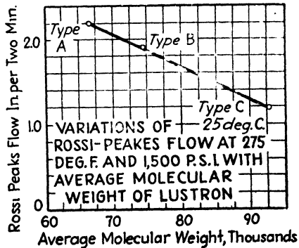
FIG. 90.—Effect of molecular weight on flow.
