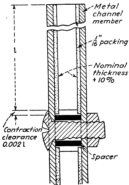
FIG. 73.—Bolt and spacer mounting.
