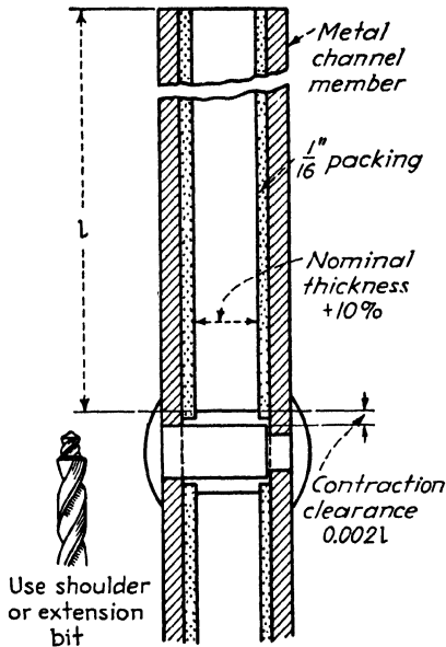
Fig. 74.—Shoulder rivet mounting requires separate drilling of metal members.
