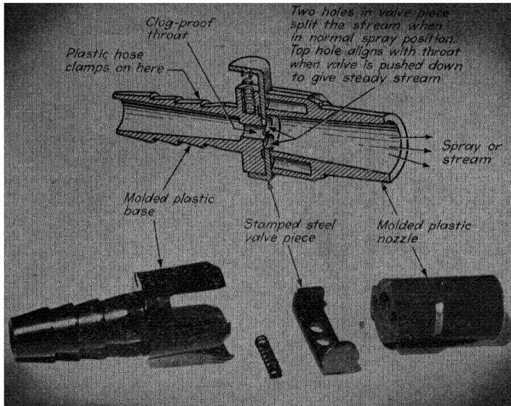
Fig. 94b.—Nozzle for stirrup pump consists of two cellulose acetate-butyrate parts cemented together with acetone.
