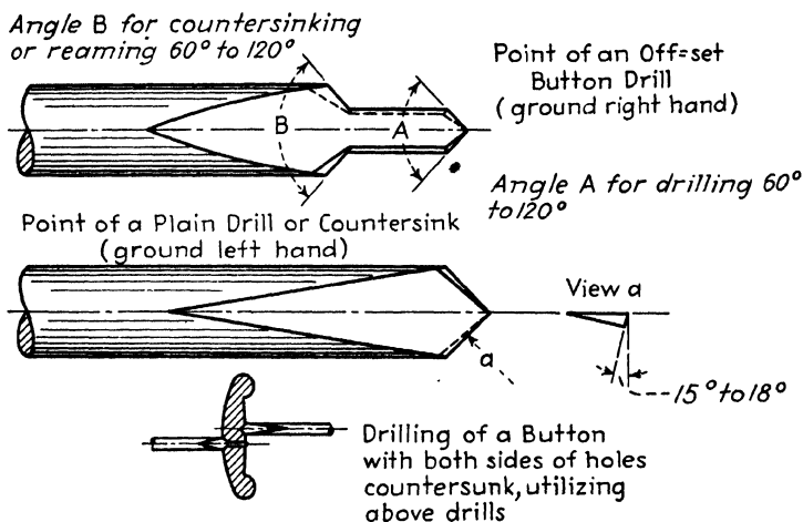
FIG. 49.—Drills used for small holes. Drills and countersinks are often used in pairs as shown.
