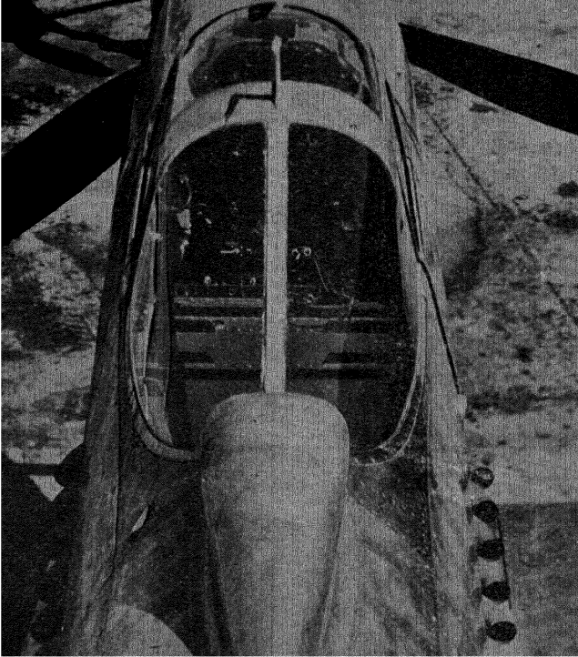
FIG. 61.—Typical acrylic plastic installation on Bell Aircraft. (Courtesy of Bell Aircraft Company.)
