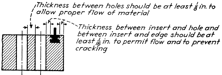
FIG. 22.—Location data for holes and inserts.
