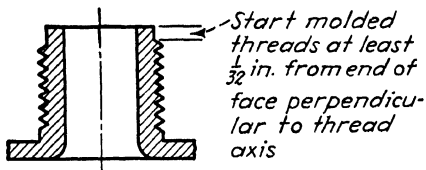
FIG. 27.—Threads can be successfully molded in.
