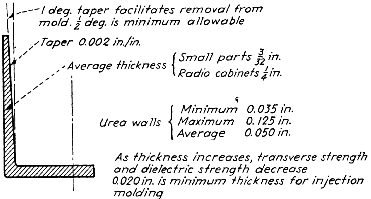
FIG. 25.—Wall taper and thickness data.
