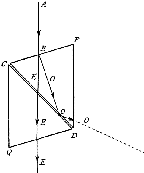
FIG. 81.—Nicol Prism.
