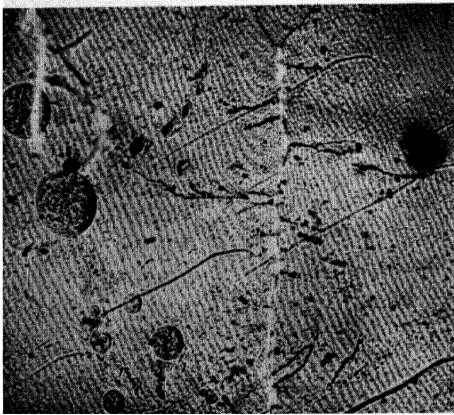
FIG. 44.—Tin Surface Crystal Boundary ( \times 80 ).
