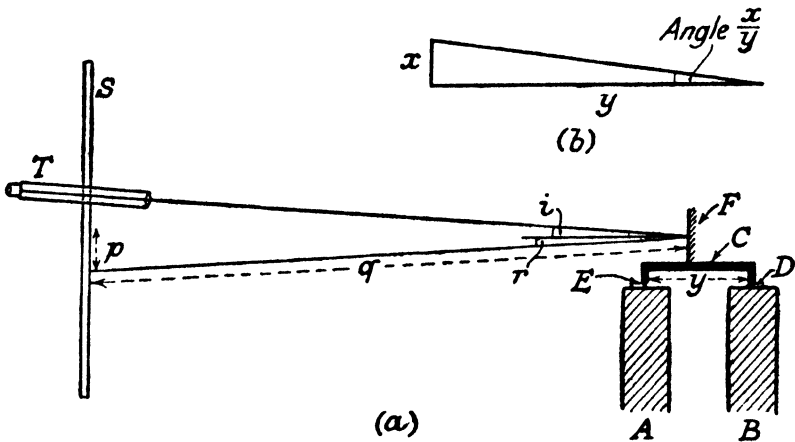
FIG. 4.—Optical Lever.
