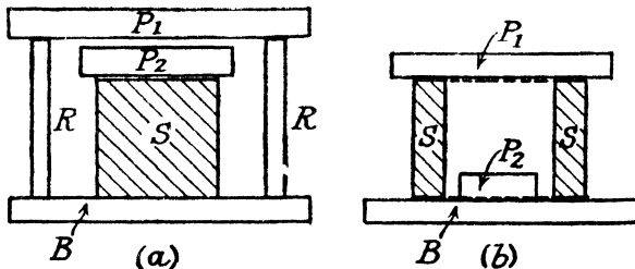
FIG. 37.—Interference Dilatometers.
