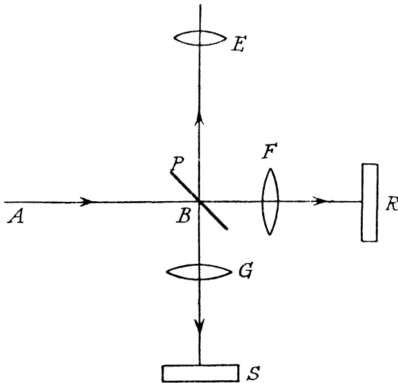
FIG. 53.—Linnik-Zeiss Micro-interferometer.
