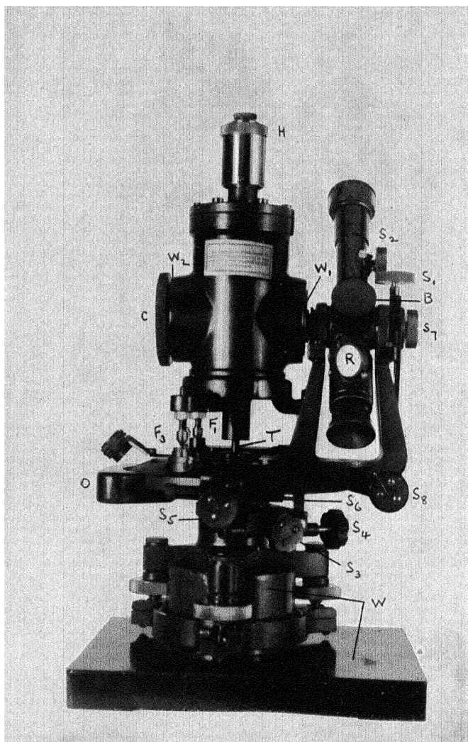
The Ordnance Survey magneto-theodolite (see Fig. 7)
