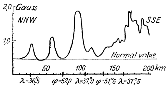
FIG. 5. Profile for the vertical intensity Z along the axial line of the Kursk anomaly (points where the profile cuts circles of latitude \phi , or meridians of longitude \lambda , are indicated below)
