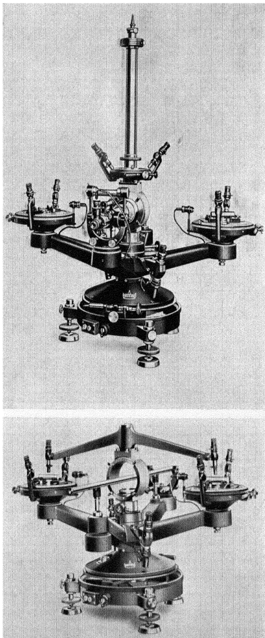
A. Schmidt's theodolite: above, in use for magnetic measurements; below, with its torsion-head replaced by a comparator device for measuring distances (Askania)
