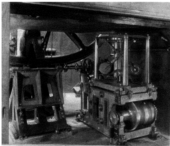
Fig. 11. The driving-clock and worm-gear that cause the 100-inch Hooker telescope to follow the stars.
