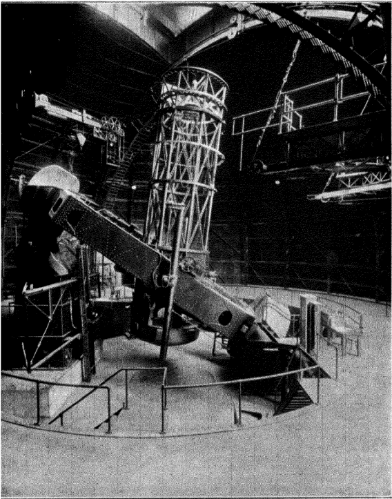
Fig. 4. The 100-inch Hooker telescope.
