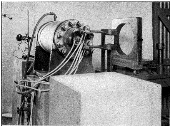
Fig. 35. Electric furnace in the Pasadena laboratory of the Mount Wilson Observatory.
