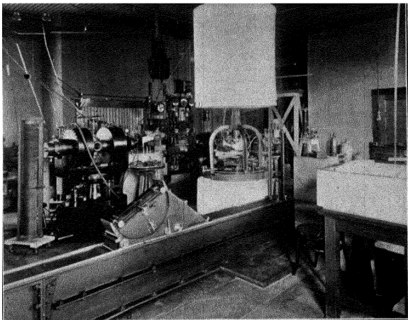
Fig. 32. Pasadena Laboratory of the Mount Wilson Observatory.
