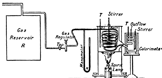
FIG. 55.—Regnault's Apparatus for the Determination of Specific Heat of Gases at Constant Pressure.
