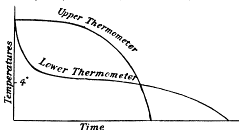
FIG. 28.—Indications of Thermometers in Hope's Apparatus.
