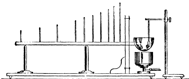
FIG. 68.—Forbes's Bar Experiment.
