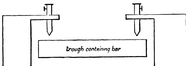
FIG. 12. —Diagram of Expansion Apparatus at the Bureau International.
