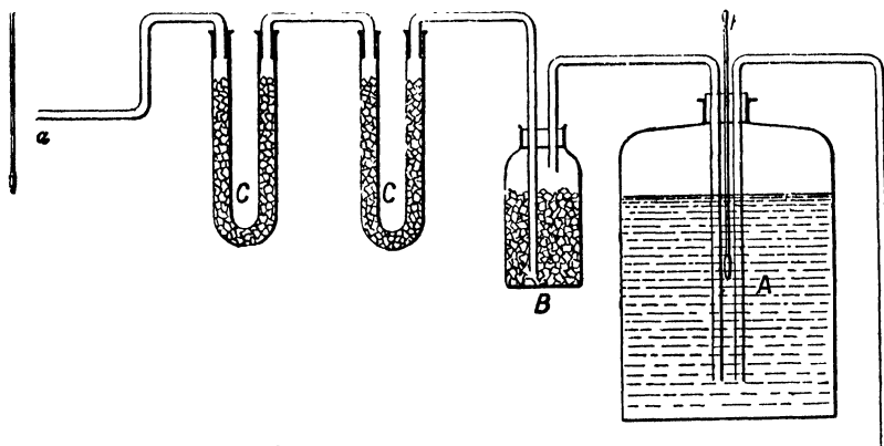
FIG. 125.—Chemical Method for Determining Dew-Point.
