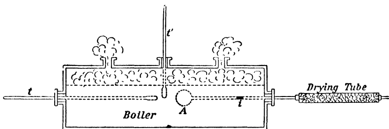
FIG. 33.—Gay-Lussac's Apparatus for Determination of Expansion of Gases at Constant Pressure.
