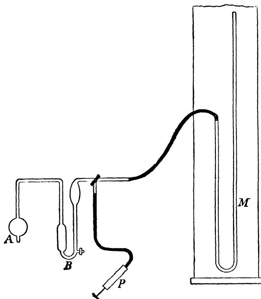
FIG. 37A.—Bottomley's Air Thermometer.—A, Air bulb; B, Sulphuric acid gauge; P, Air pump to make pressure equal on the two sides of B; M, Manometer.
