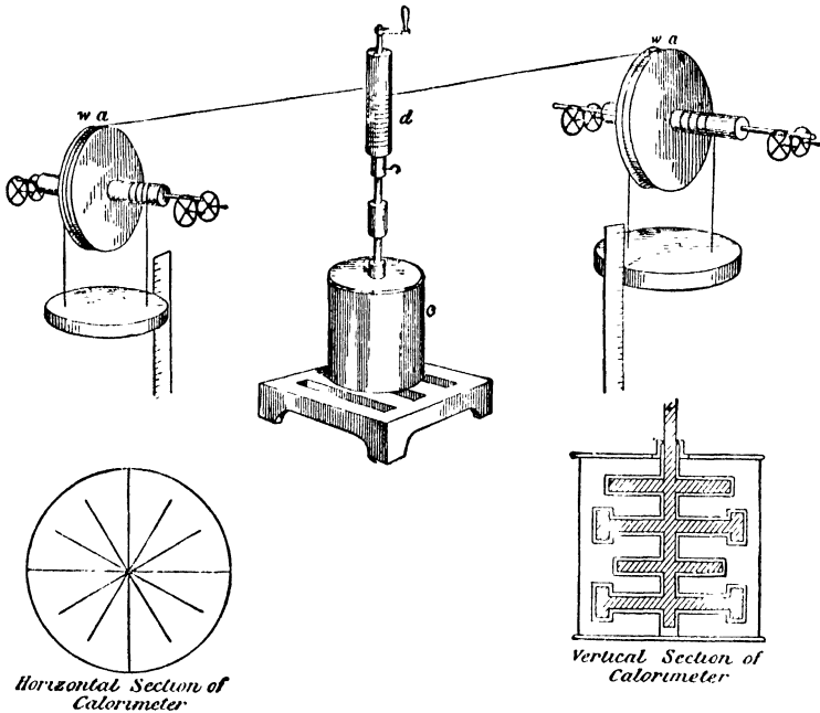
FIG. 75.—Joule's Water-Churning Apparatus for Determining the Mechanical Equivalent of Heat.
