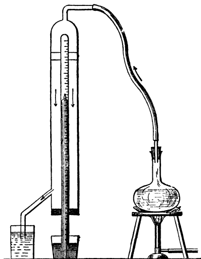
FIG. 101.—Vapour-Density Determination by Gay Lussac and Hoffmann's Method.
