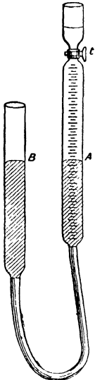
FIG. 86.—Evaporation into an Air Space.
