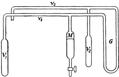
FIG. 38.—Callendar's Compensated Air Thermometer.
