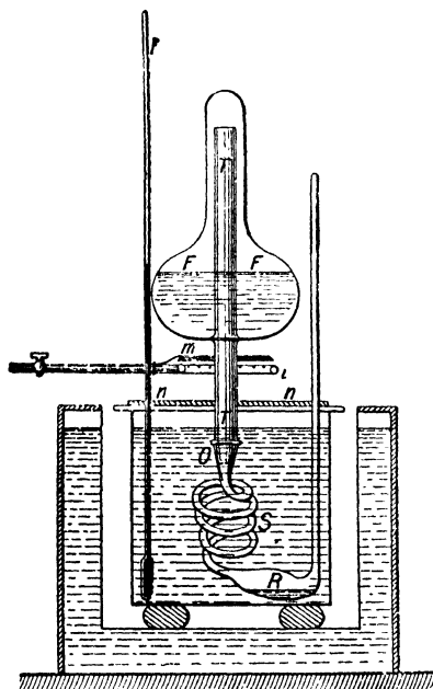
FIG. 105.—Berthelot's Apparatus for Latent Heat.
