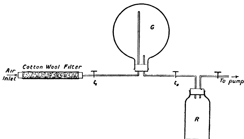
FIG. 94.—Apparatus for obtaining a Dust-Free Space.
