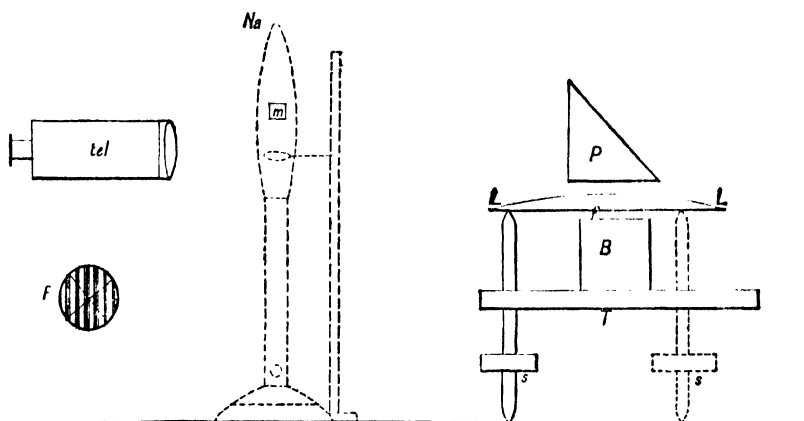
FIG. 15.—Diagram of Fizeau's Expansion Apparatus.—B, block of which expansion is to be measured placed on table T; ss , levelling screws, also supporting lens, L just above B; f , film of air-forming interference bands; P, right-angled prism throwing light down and reflecting it out again; Na, sodium flame behind the plane of the figure; m , mirror in the plane of the figure reflecting the sodium light towards P; tel , telescope directed towards P and viewing the interference bands; F represents the appearance of the bands in the telescope, which is provided with cross-wires. The expansion table is protected by a case which can be heated. This case is not represented.
