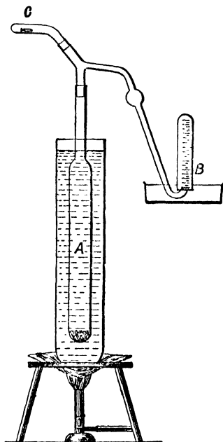
FIG. 102.—Victor Meyer's Method for Vapour-Density Determination.
