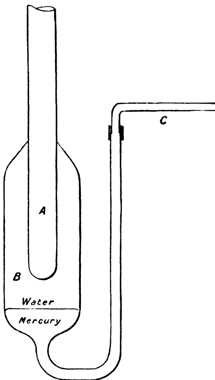
FIG. 56.—Bunsen's Ice Calorimeter.
