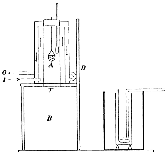
FIG. 53.—Regnault's Apparatus for Determination of Specific Heat of Solids by Method of Mixtures.
