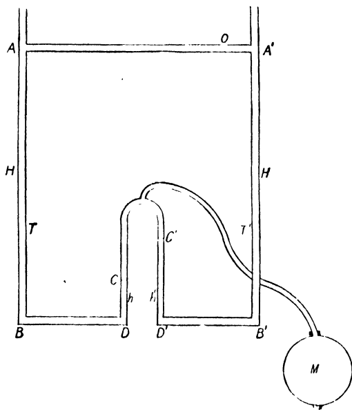
FIG. 22.—Diagram of Regnault's First Apparatus for finding the Expansion of Mercury.
