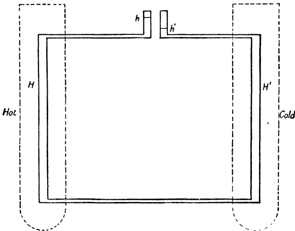
FIG. 23.—Regnault's Second Apparatus for the Expansion of Mercury.
