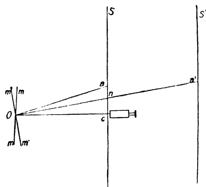
FIG. 14.—Mirror Method of Reading Deflections.
