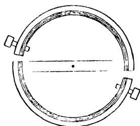
FIG. 20.—Compensating Balance for Chronometers. Outer rim brass, inner rim steel.
