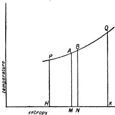
FIG. 158.—Entropy-Temperature Diagram.
