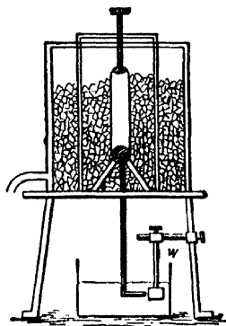
FIG. 35.—Regnault's Expansion of Gas at Constant Pressure (Rudberg's Method). Bulb opened under mercury.
