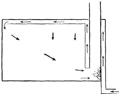
FIG. 51.—Arrangement for Warming Incoming Air.
