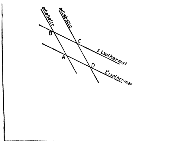
FIG. 151.—Carnot's Cycle.
