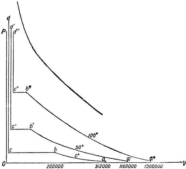
FIG. 108.—Indicator Diagram for Water-Steam.
