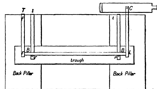
FIG. 13.—Diagram of Expansion Apparatus of Lavoisier and Laplace. Front pillars not shown. To a crosspiece T, supported horizontally across the two left-hand pillars, was attached the fixed vertical rod TFF; t were two other crosspieces to which were attached vertical rods carrying rollers rr . Another crosspiece served as the axis of the lever CL and the telescope.
