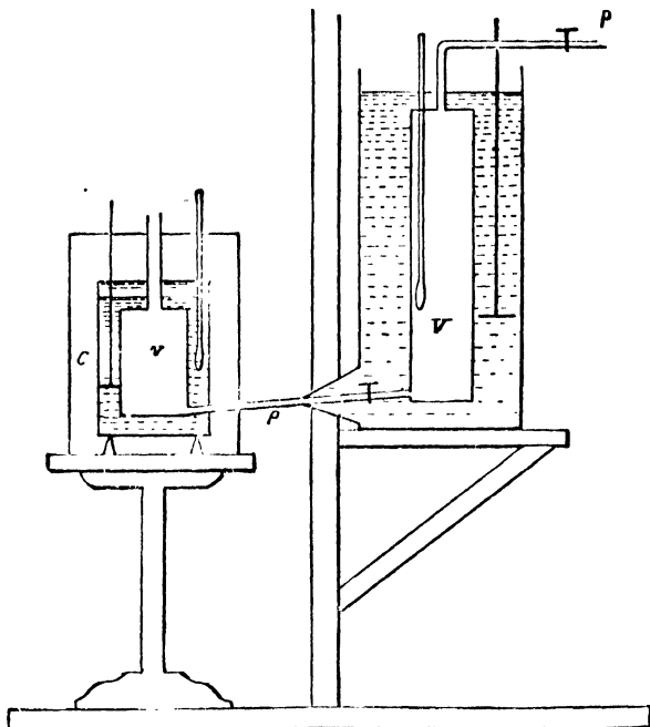
FIG. 54.—Regnault's Apparatus for Determination of Specific Heat of Liquids by Method of Mixtures.
