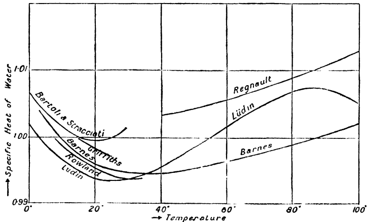
FIG. 60.—Results of Different Experiments on the Specific Heat of Water.
