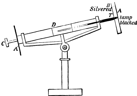
FIG. 144.—Pouillet's Pyrheliometer.
