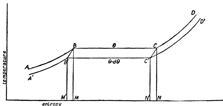
FIG. 176.—Equal Pressure Lines on the Entropy-Temperature Diagram.
