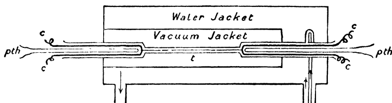
FIG. 59.—Callendar-Barnes Electric Heating Method of Determining the Specific Heat of Water.
