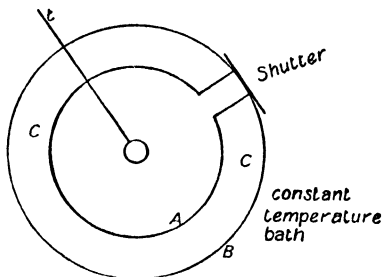
FIG. 145.—Violle's Actinometer.
