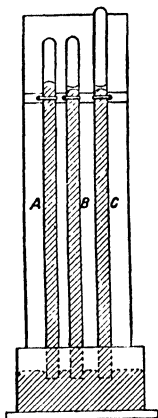
FIG. 84.—A, ordinary barometer; B and C, barometers with small quantities of water above the mercury.
