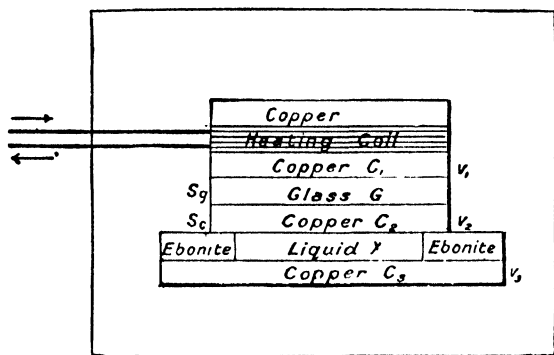
FIG. 71.—Lees's Disc Experiments on Liquids.— C_1C_2C_3 , copper discs; G, glass disc; X, liquid surrounded by ebonite ring.
