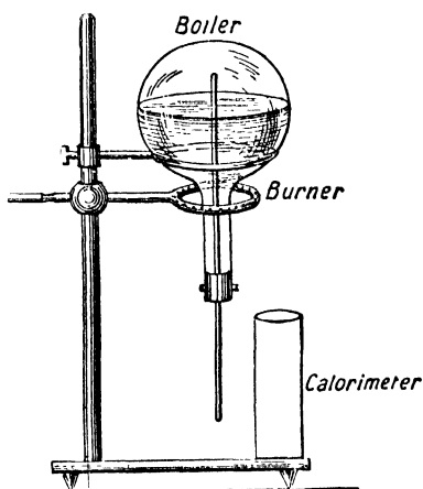
FIG. 104.—Rough Determination of Latent Heat.
