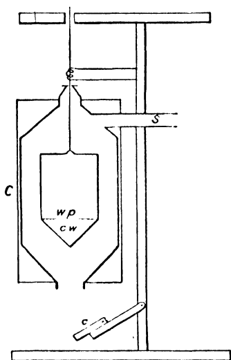
FIG. 57.—Joly's Steam Calorimeter.
