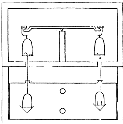
FIG. 58.—Joly's Differential Steam Calorimeter.
