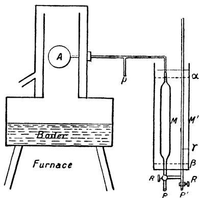
FIG. 36.—Regnault's Expansion of Gas at Constant Pressure.
