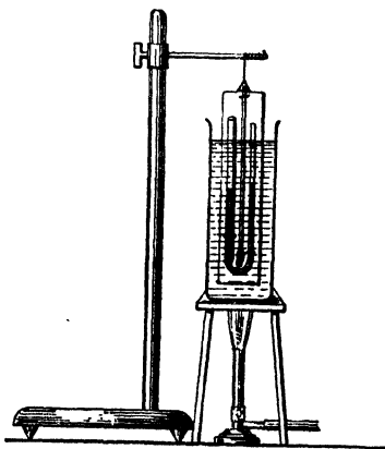
FIG. 119.—Melting-Point Apparatus.
