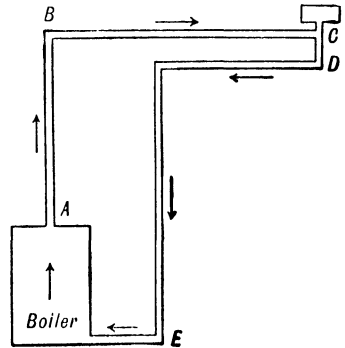
FIG. 42.—Principle of Hot-Water Heating Systems.
