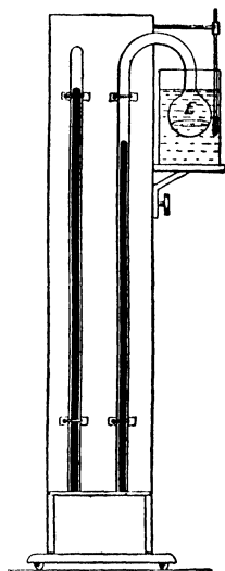
FIG. 96.—Vapour-Pressure of Ice.
