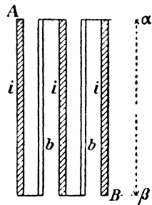
FIG. 18.—Principle of Gridiron Pendulum of Iron and Brass Bars.
