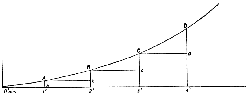
FIG. 142.—Radiation Curve broken up into Cooling Curves.
