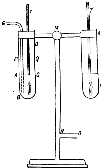
FIG. 122.—Regnault's Dew-point Hygrometer.
