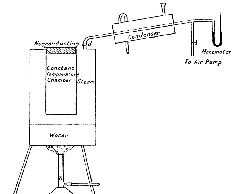
FIG. 7.—Constant-Temperature Apparatus, using the Boiling-Point Method.
