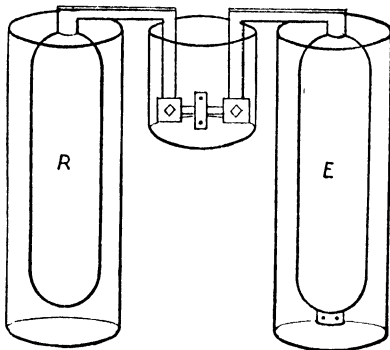
FIG. 74.—Modified Form of Joule's Apparatus.
