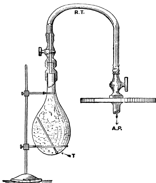
FIG. 89.—Reduction of Boiling-Point by reduction of pressure
