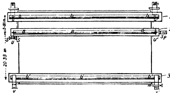
FIG. 10.—Plan of Ramsden's Expansion Apparatus.—(1) Wood trough at 0^{\circ} containing cast-iron bar bb , with cross wires in uprights uu' fixed near ends; uu' shown also in elevation; (2) copper trough with lamps underneath to raise temperature, and containing bar BB to be tested, upright U pressed against left end by adjusting screws SS , upright U' pressed against right end by spring sp . UU' carry microscope object-glasses; (3) wood trough at 0^{\circ} containing cast-iron bar b'b'' with uprights vv'' fixed near ends carrying microscope eyepieces, that on v' being provided with a micrometer m .
