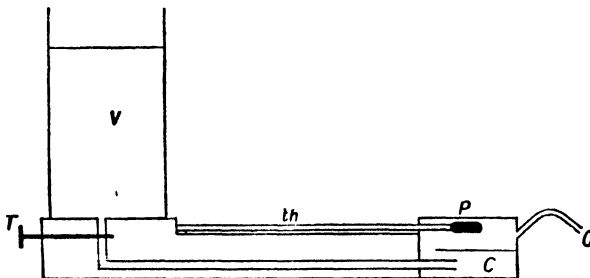
FIG. 123.—Dines's Hygrometer.
