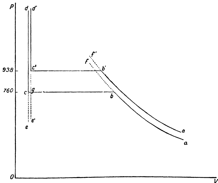
FIG. 109.—Indicator Diagram showing Prolongations of Water and of Steam beyond Normal Turning Points.
