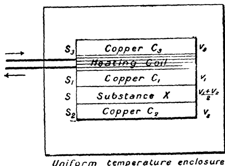
FIG. 70.—Lees's Disc Experiments on Conductivity.— C_1C_2C_3 , copper discs; X, disc to be tested; v_1v_2v_3 , temperatures above the enclosure; s, s_1s_2s_3 , emitting surfaces.
