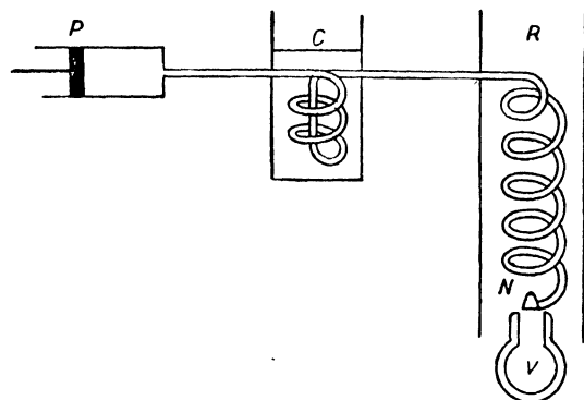
FIG. 117.—Diagram of Regenerator Process for Liquefying Gases.
