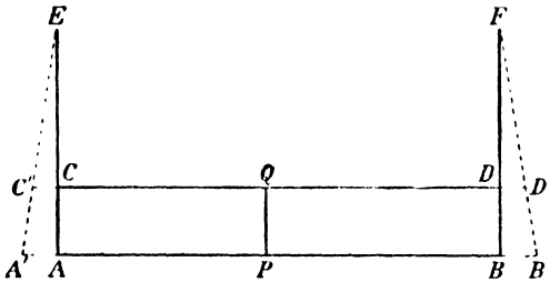
FIG. 17.—Compensation Measuring-Bar.—EF, of invariable length; AB, brass; CD, iron.
