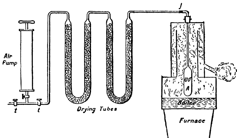
FIG. 34.—Regnault's Apparatus for Expansion of Gas at Constant Pressure (Rudberg's method). Bulb filled with gas at 100^{\circ} C. and sealed.
