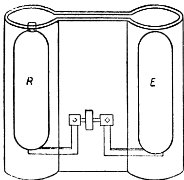
FIG. 73.—Joule's Expansion of Air Apparatus
