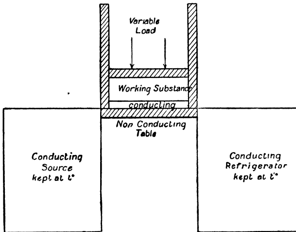
FIG. 150.—Carnot's Engine. Shaded parts non-conducting.
