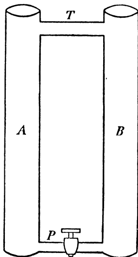
FIG. 29.—Apparatus of Joule and Playfair for Point of Maximum Density of Water.
