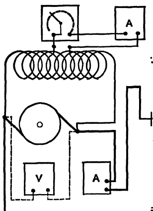
Fig. 12. — Connections for Armature Characteristic.
