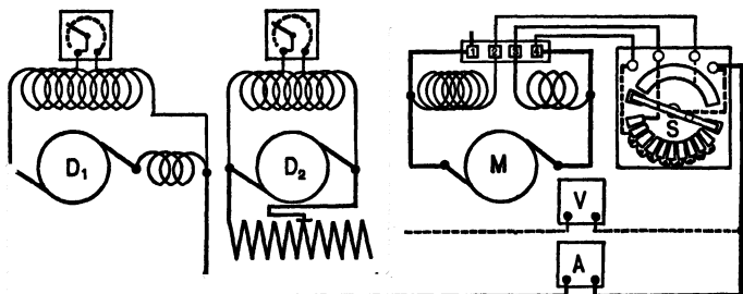
Fig. 21.—Apparatus and Connections for Efficiency Test of a Motor.
