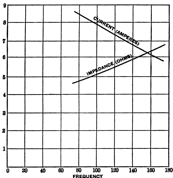
Fig. 73.—Dependence of Current and Impedance upon Frequency in a Circuit with Resistance of 4 Ohms and Self-Induction of .005 Henry.
