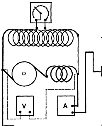
Fig. 14. — Connections for the Compound Characteristic.
