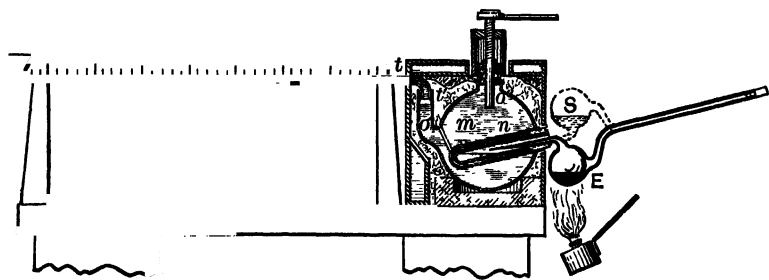
Fig. 139.— Favre and Silbermann Mercury Calorimeter.
