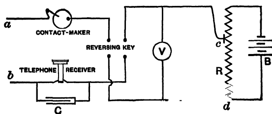
Fig. 108. — Telephone Method.
