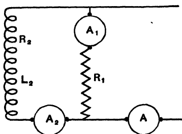
Fig. 68. Three-Ammeter Method.
