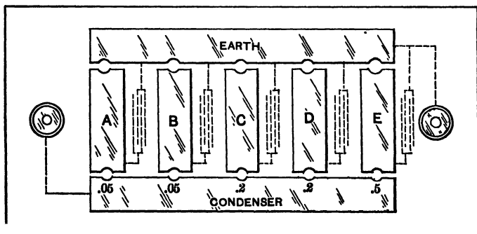
Fig. 82.—Standard Microfarad Condenser.
