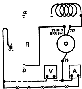
Fig. 16.—Connections for the Waterhouse Dynamo.
