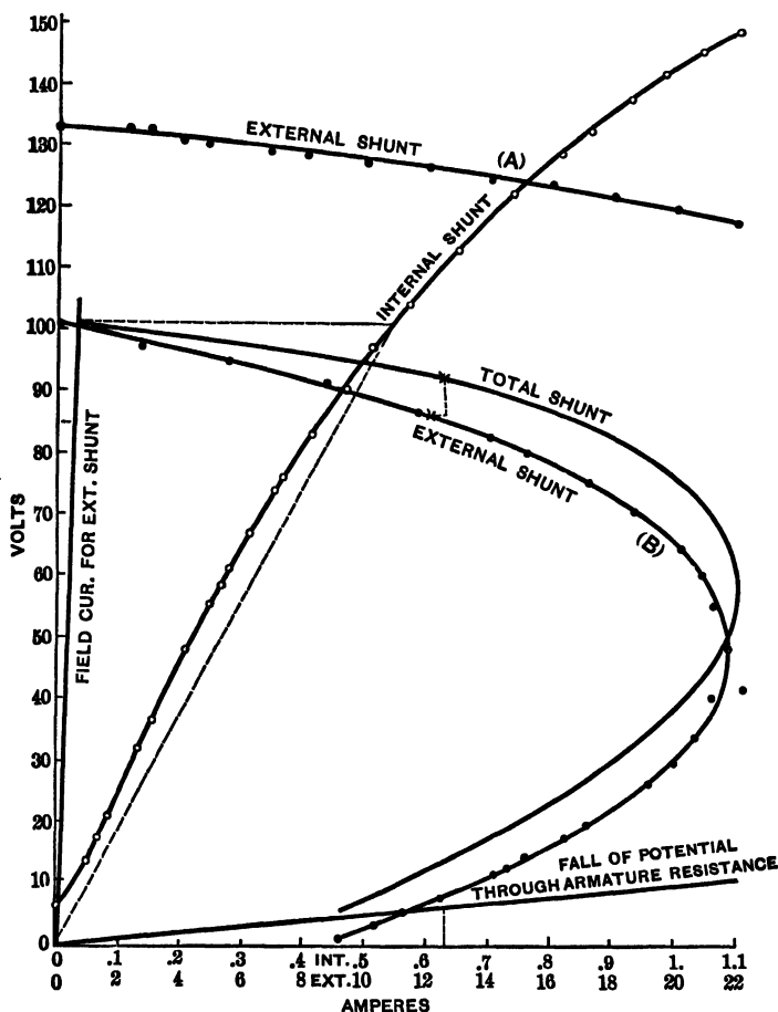
Fig. 9.—Characteristics of a Shunt Dynamo.
