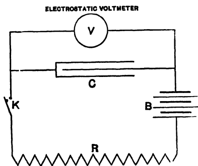
Fig. 88.—Connections for Charging Condenser through a Resistance.
