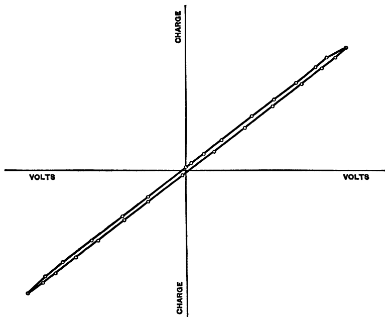
Fig. 116.—Curve for Dielectric Hysteresis.
