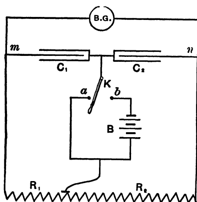
Fig. 95. — Bridge Method.
