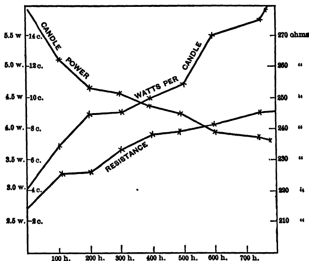
Fig. 185. — Life Curves of a Glow Lamp.
