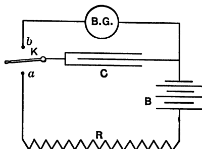
Fig. 85. — Condenser Charge. Ballistic Method.
