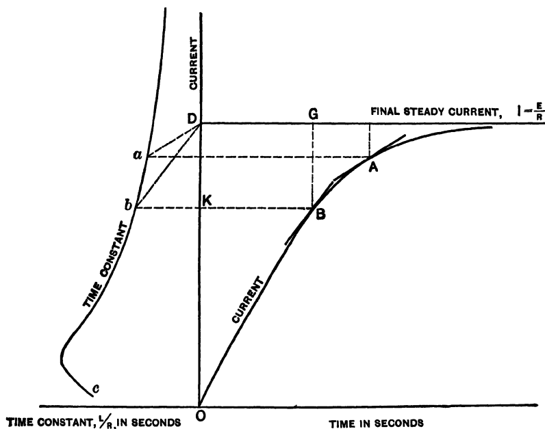
Fig. 61. — Establishment of Current in a Circuit with Variable Self-Induction.
