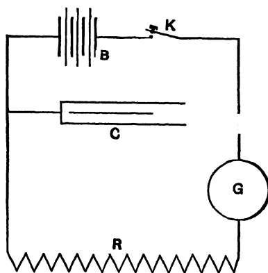
Fig. 90. — Deflection Method
