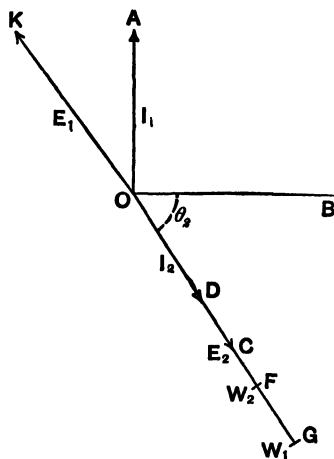
Fig. 76.—Polar Transformer Diagram.
