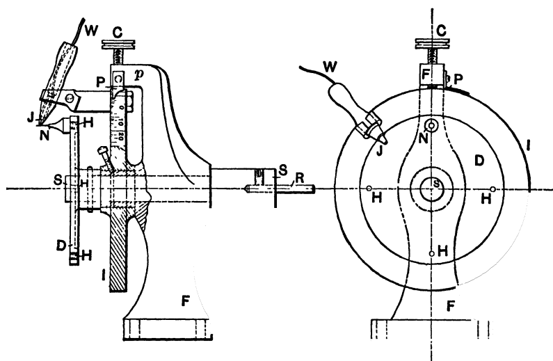
Fig. 46. — Details of Contact-Maker.
