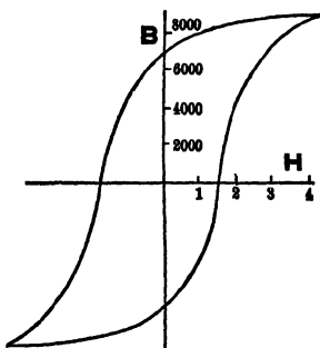
Fig. 121. — Hysteresis Loop.
