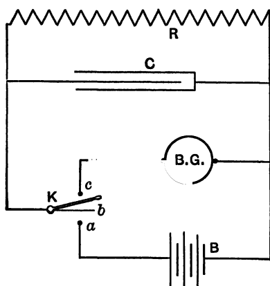
Fig. 84. — Condenser Discharge. Ballistic Method.
