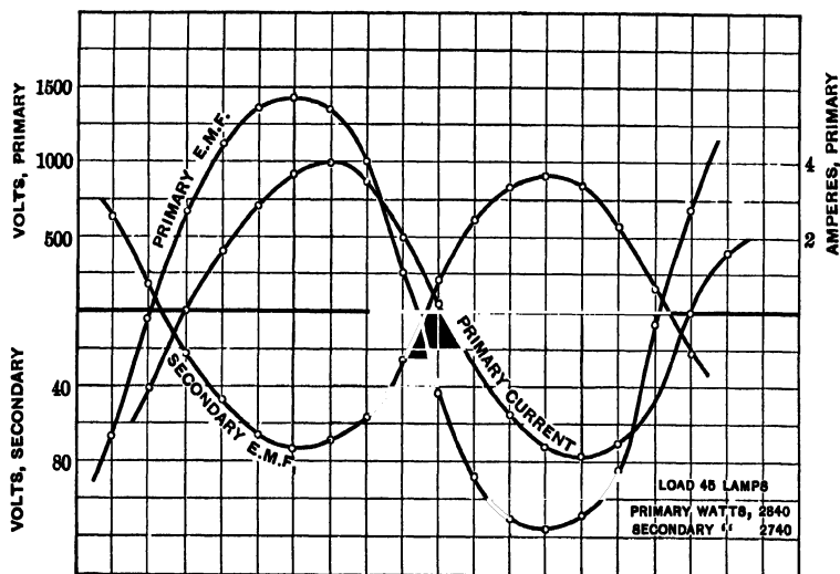
Fig. 113. — Transformer Curves.
