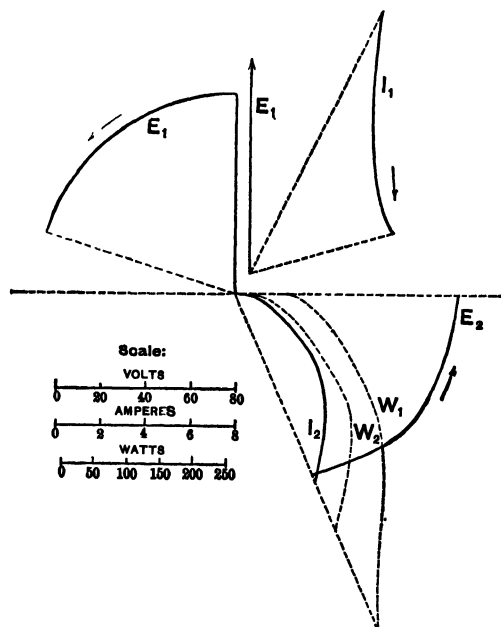
Fig. 77.—Polar Diagram for a Constant Potential Transformer at Different Loads.
