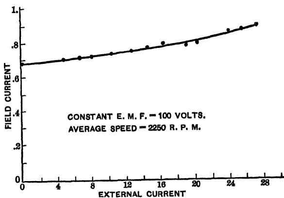
Fig. 13. — Armature Characteristic.
