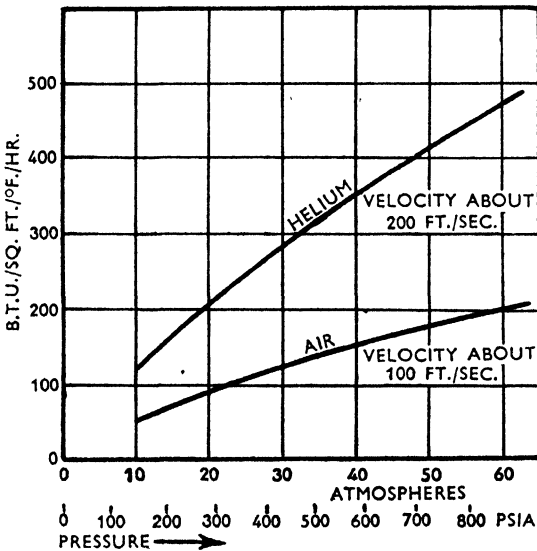
Fig. 2.—Comparison of heat transfer for air and helium in tubes of 1.2-in. diameter. Equal relative pressure drop.
