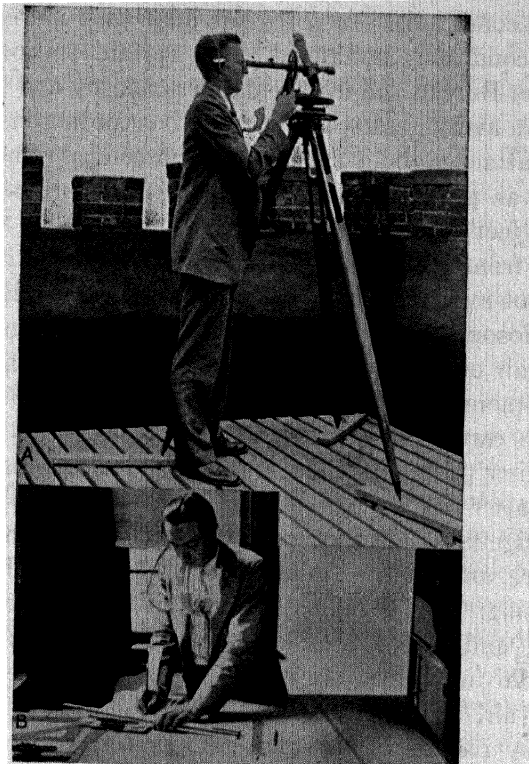
Fig. 36. Pilot Balloon Observation. A , observer following the balloon with a theodolite and telephoning its angular elevation and azimuth at one-minute intervals to B , computer at plotting board. Courtesy, U. S. Weather Bureau, Washington, D. C.
