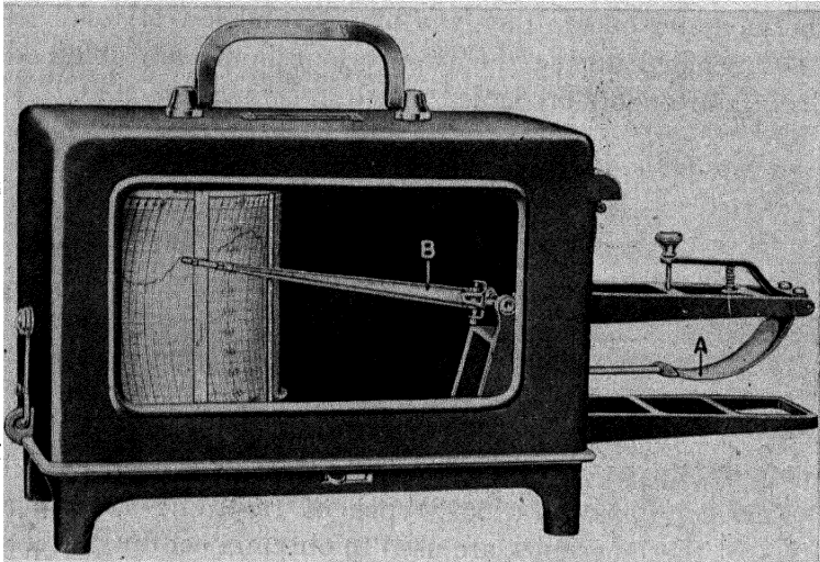
Fig. 5. Thermograph, a Recording Air Thermometer with Weekly Clock Movement Within the Cylinder. Temperature changes cause changes in the curvature of the flattened tube, A , resulting in vertical movements of the arm, B . Courtesy, J. P. Friez & Sons, Baltimore, Md.
