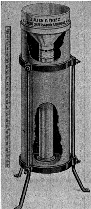
Fig. 33. Rain Gage. Standard 8-inch pattern, with measuring stick. Courtesy, J. P. Friez & Sons, Baltimore, Md.
