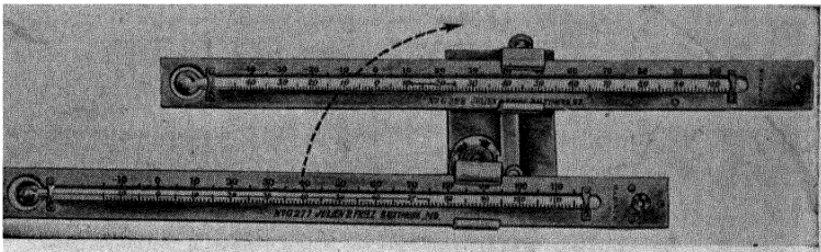
Fig. 4. Maximum and Minimum Thermometers with Townsend Support. Courtesy, J. P. Friez & Sons, Baltimore, Md.
