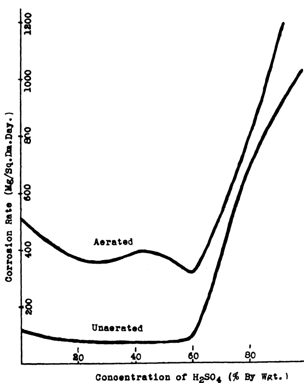
FIG. IX-5.—CORROSION OF MONEL METAL BY HOT SULPHURIC ACID (95° C. VELOCITY 16.5 FT./MIN.).
