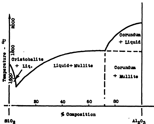
FIG. XVI-6.—LIQUID-SOLID EQUILIBRIUM, \text{SiO}_2\text{-Al}_2\text{O}_3 .
