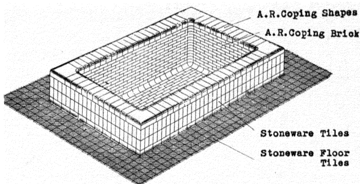
FIG. XV-5a.—ACID TANK FOR METAL TREATMENT.
