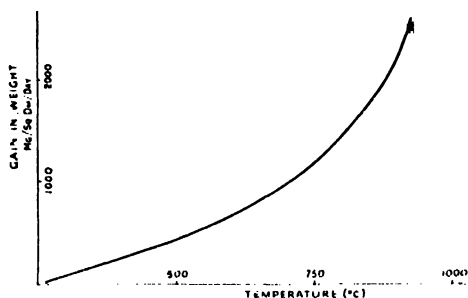
FIG. III-17. HIGH TEMPERATURE OXIDATION OF CAST IRON.
