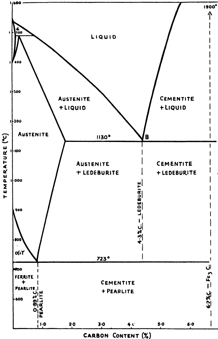
FIG. III-3.—THE IRON-CARBON DIAGRAM.
