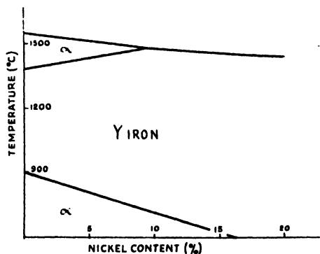
FIG. III-2.—IRON-NICKEL DIAGRAM.
