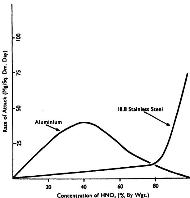
FIG. VII-6.—ATTACK OF COLD NITRIC ACID ON STAINLESS STEEL AND ALUMINIUM.
