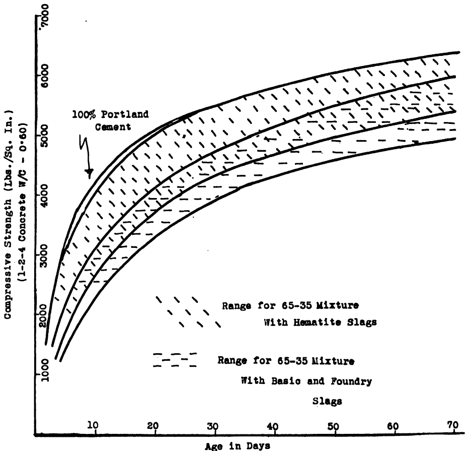
FIG. XIII-3.—SETTING OF PORTLAND CEMENT, PORTLAND—BLAST-FURNACE CEMENT.
