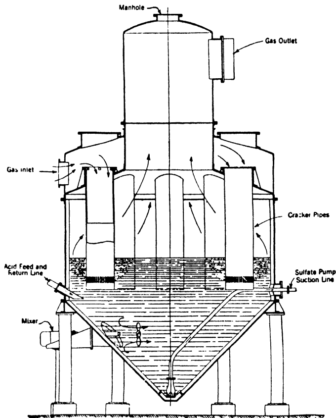
FIG. VI-6.—LEAD-LINED AMMONIUM SULPHATE CRYSTALLISER.
