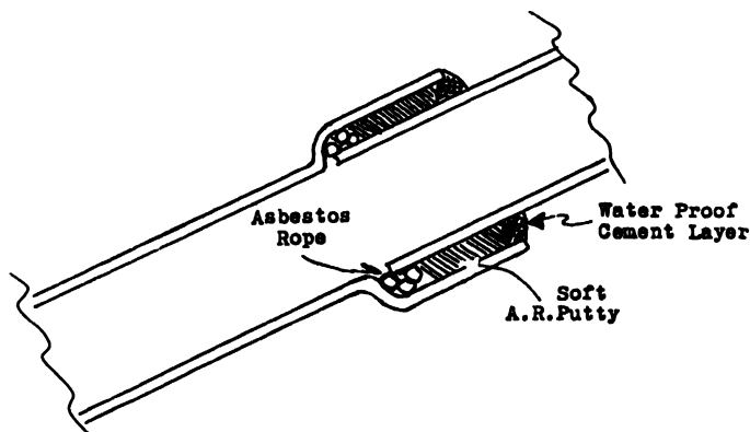
FIG. XIV-3.—SPIGOT-FAUCET JOINT IN A.R. STONEWARE PIPE.
