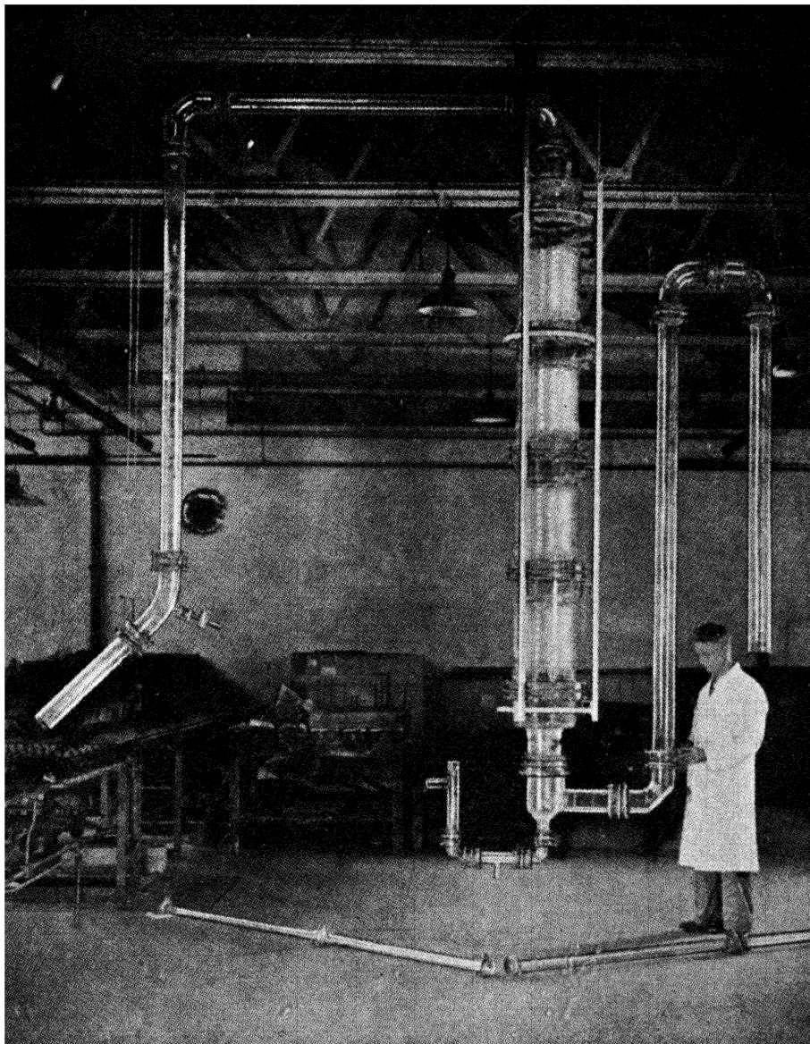
FIG. XVII-6.—GLASS SCRUBBING TOWER WITH INTERNAL COOLING.
