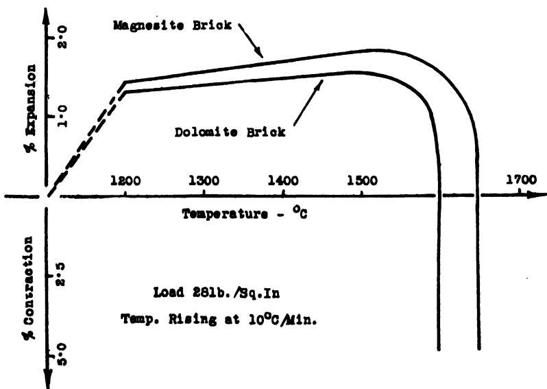
FIG. XVI-10.—REFRACTORINESS UNDER LOAD (ALKALINE REFRACTORIES).
