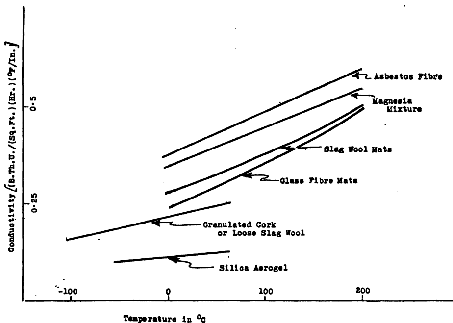
FIG. XVI-13.—CONDUCTIVITY OF INSULATING MATERIALS (Low Temperatures).
