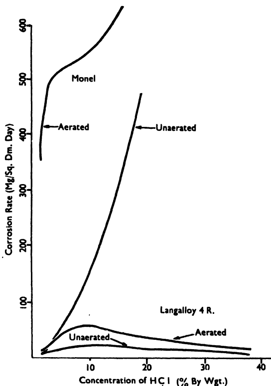
FIG. IX-8.—ATTACK OF COLD HYDROCHLORIC ACID ON MONEL AND LUNGALLOY. (After Richardson, Metallurgia , 1949)
