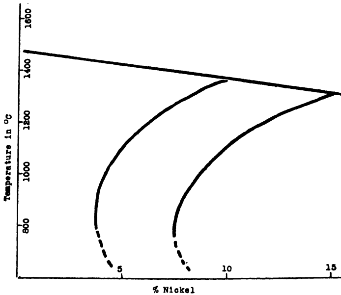
FIG. V-3.—EFFECT OF NICKEL IN AUSTENITE STABILITY IN IRON + 18% CHROMIUM.
