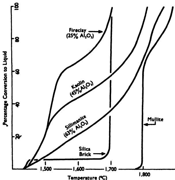
FIG. XVI-7.—MELTING CHARACTERISTICS OF REFRACTORIES.
