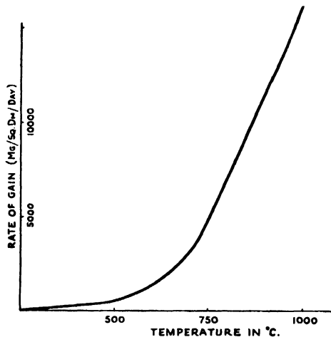
FIG. IV-16.—OXIDATION OF MILD STEEL.
