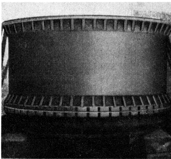
FIG. X-2.—LOWER SECTION OF HCN GENERATOR IN HIGH-SILICON IRON. WEIGHT 2 TONS.
