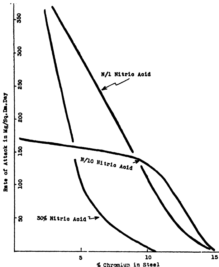
FIG. V-1.—EFFECT OF CHROMIUM CORROSION ON RESISTANCE.
