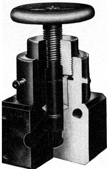
FIG. XIX-6a.—VALVE IN KARBATE.
