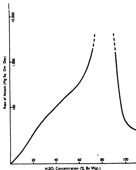
FIG. VII-5.—ACTION OF SULPHURIC ACID ON ALUMINIUM (99.9 Al).
