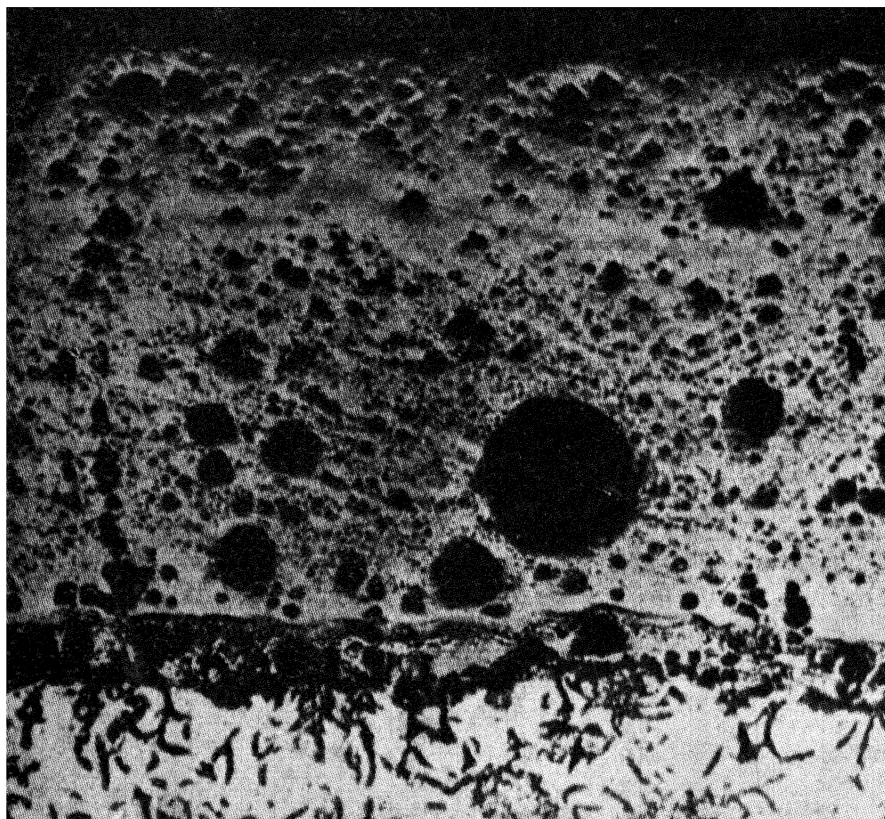
FIG. XII-6.—HOT DUST ENAMEL ON CAST IRON ( \times 75 ).
