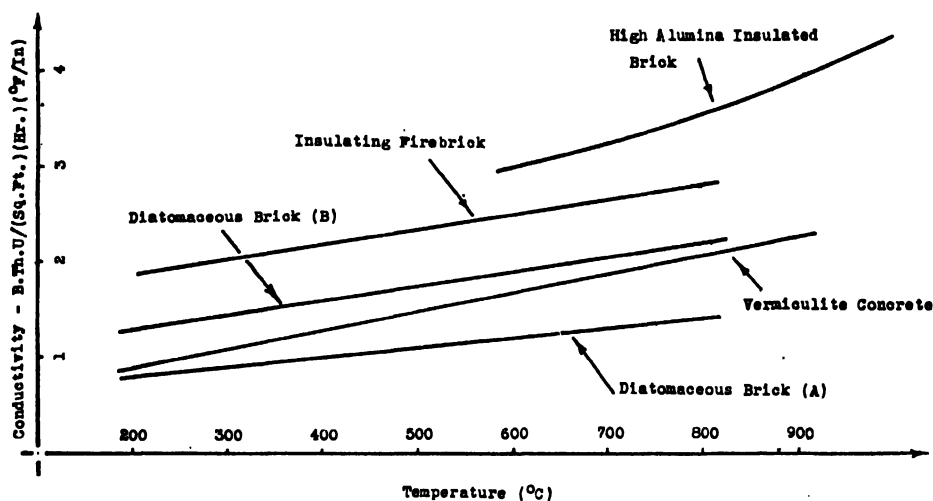
FIG. XVI-12.—CONDUCTIVITY OF INSULATING MATERIALS (High Temperatures).
