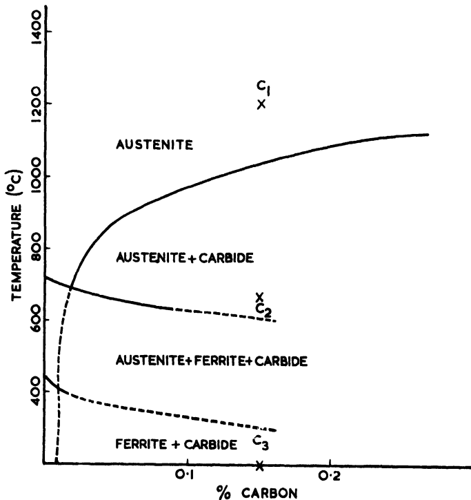
FIG. V-4.—PHASE DIAGRAM FOR 18Cr 8Ni STEEL.
