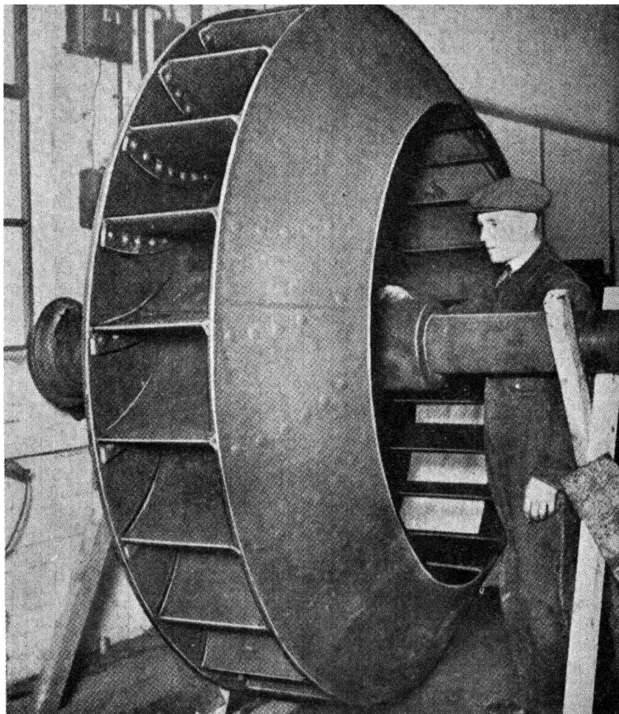
FIG. XIX-13.—RUBBER-LINED FAN—7 FT. DIAMETER.
