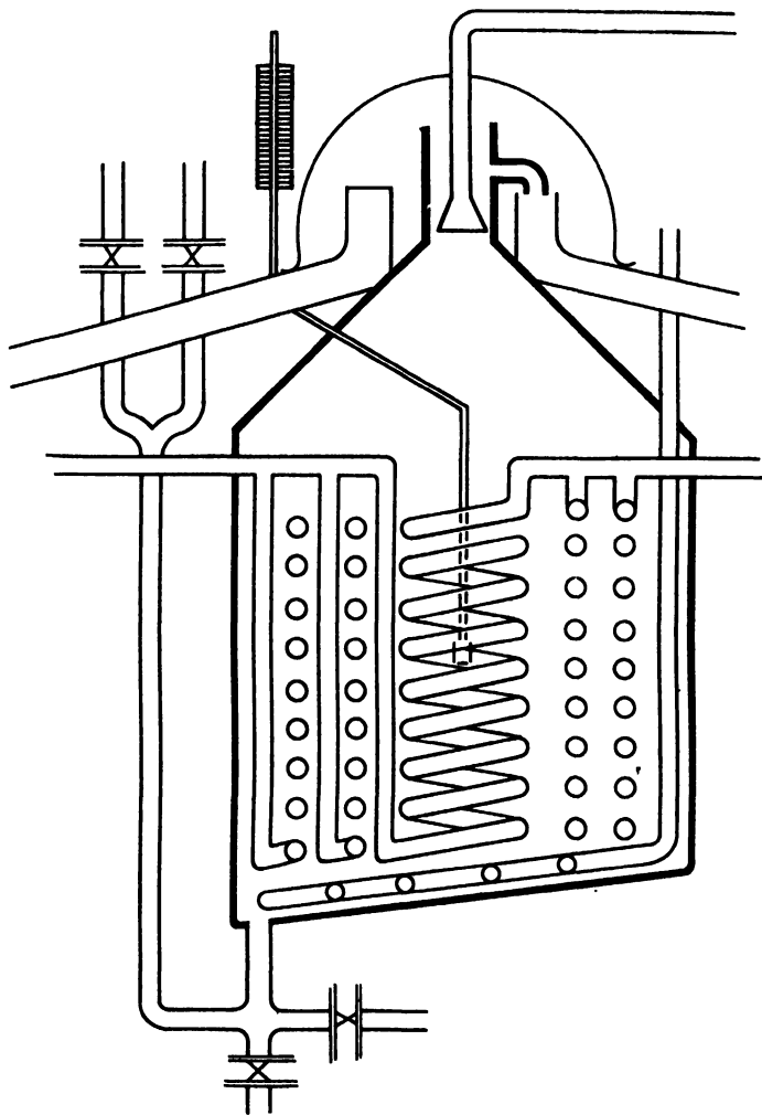
FIG. VI-5.—HEAVY LEAD CONSTRUCTION—GLYCERINE NITRATOR.
