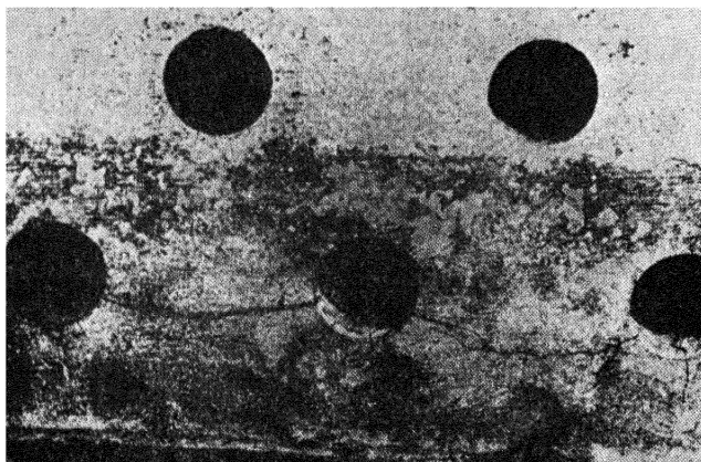
FIG. IV-12.—CAUSTIC EMBRITTLEMENT OF BOILER STEEL.
