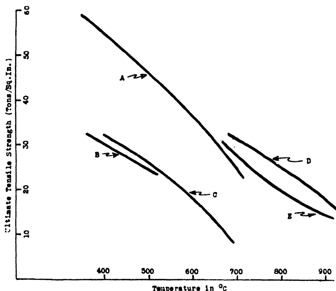
FIG. V-10a.—STRENGTHS OF HEAT RESISTING ALLOYS.
