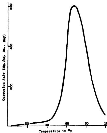
FIG. XII-2.—CORROSION OF ZINC BY DISTILLED WATER.
