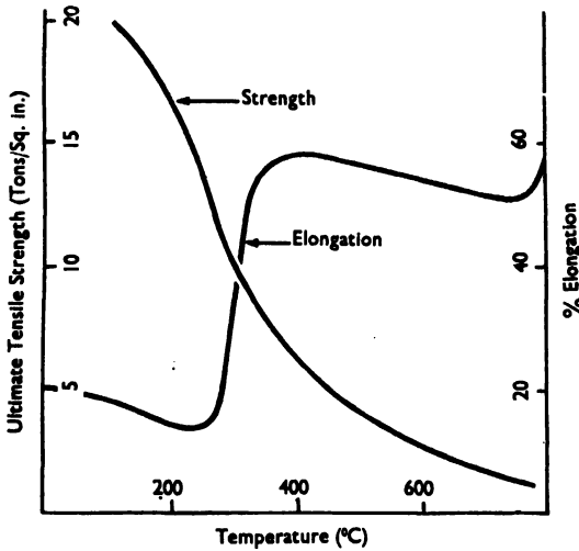
FIG. VIII-2b.—HARDENED HIGH CONDUCTIVITY COPPER—TENSILE STRENGTH AND DUCTILITY v. TEMPERATURE.
