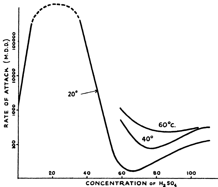
FIG. IV-14.—ATTACK OF SULPHURIC ACID ON STEEL.
