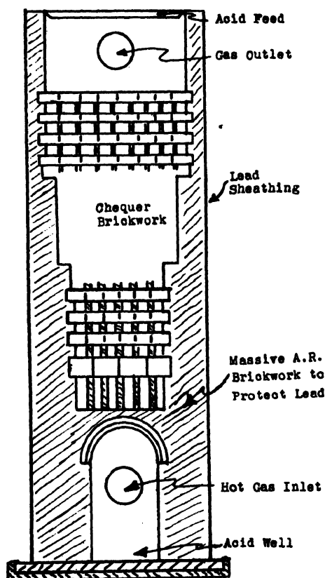
FIG. XV-4.—ACID RESISTING BRICKWORK FOR GLOVER TOWER. (30 ft. high, 9 ft. sq.)
