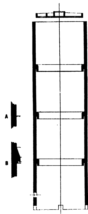
FIG. XV-8.—JOINTS IN STONEWARE TOWER (A) BUTT JOINT (B) DRIP RING (C) INTERNAL FLANGE.
