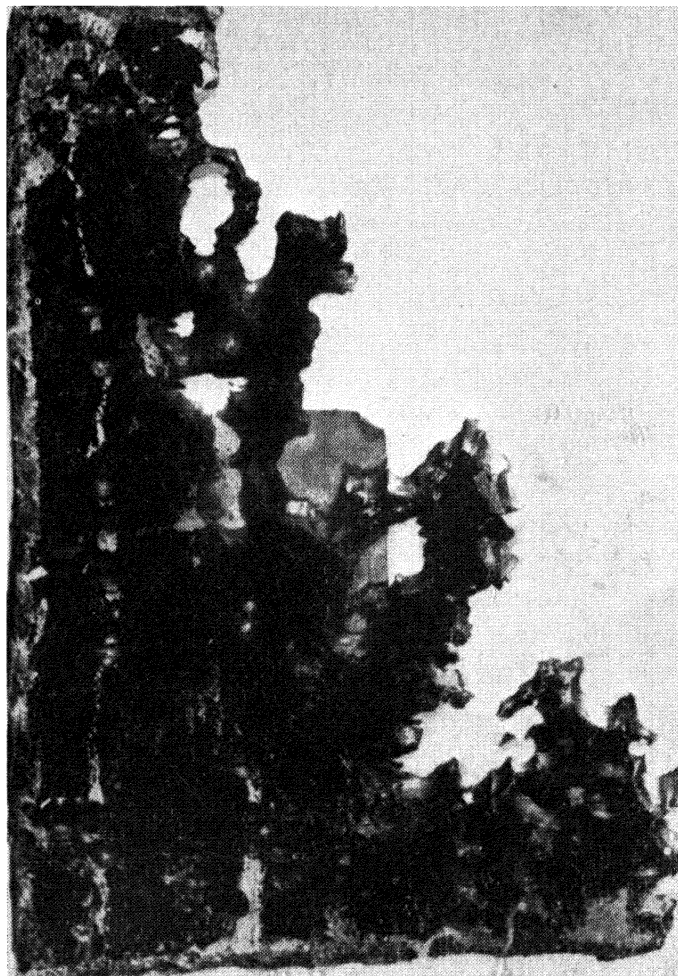
FIG. VII-7.—EFFECT OF ANHYDROUS PROPIONIC ACID ON ALUMINIUM.
