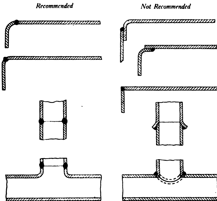
FIG. VII-4.—THE DESIGN AND POSITION OF GAS-WELDED JOINTS IN ALUMINIUM.
