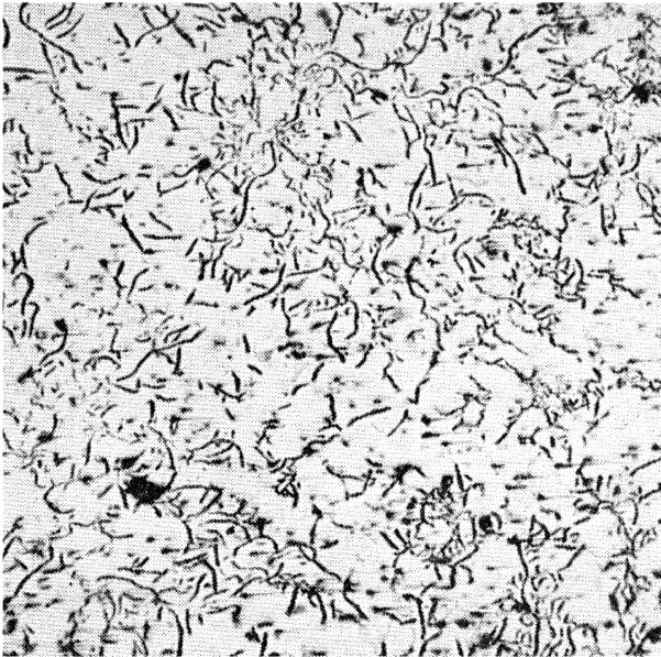
FIG. III-8.—GREY CAST IRON, SHOWING FINE GRAPHITE.
