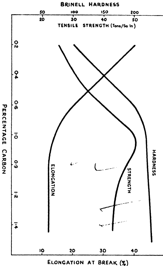
FIG. IV-3.—CHARACTERISTICS OF CARBON STEELS.
