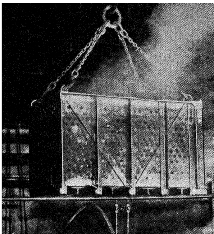
FIG. IX-4.—MONEL METAL PICKLING BASKET (AFTER 10 YEARS' SERVICE).
