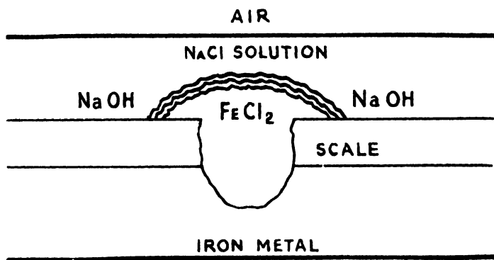
FIG. III-13.—CORROSION PITTING.
