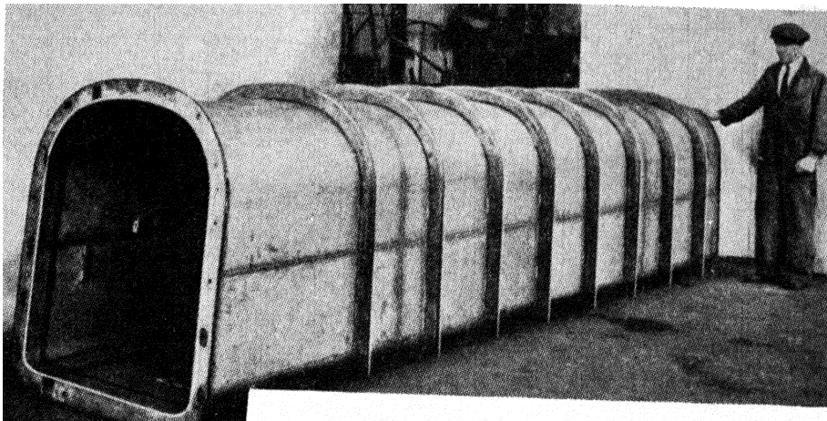
FIG. IX-6.—GAS-TIGHT WELDED INCONEL MUFFLE FOR WORKING AT 900° C.
