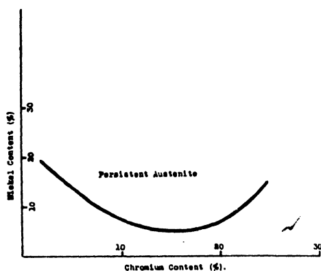
FIG. V-6.—PERSISTENT AUSTENITE IN Fe-Cr-Ni ALLOYS.
