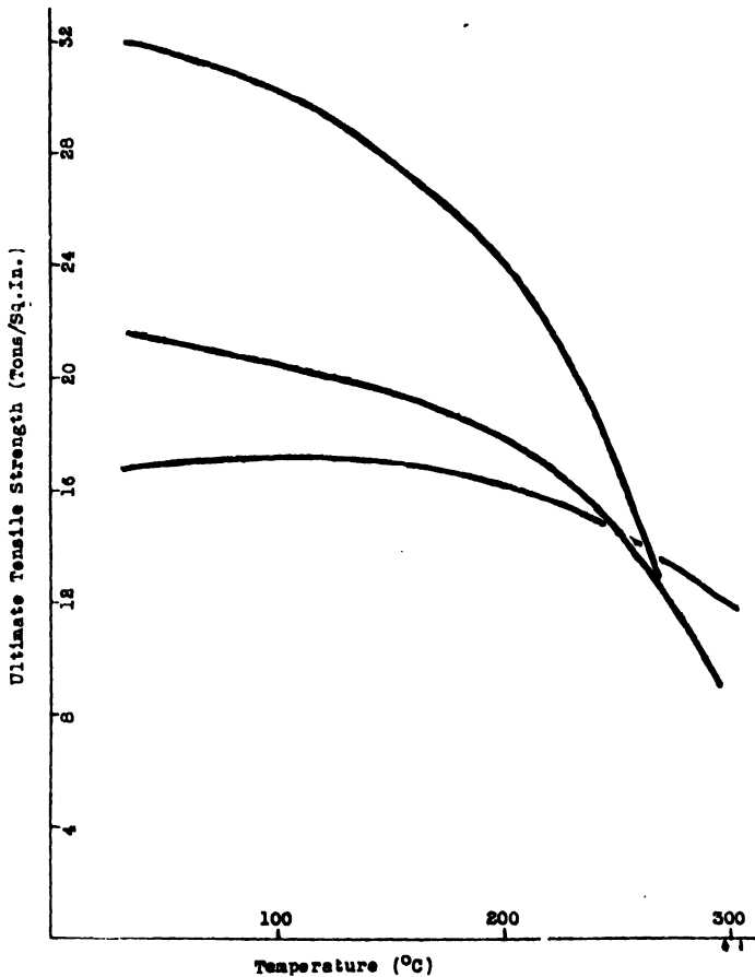
FIG. VII-2.—TEMPERATURE-STRENGTH CURVES FOR ALUMINIUM ALLOYS.
