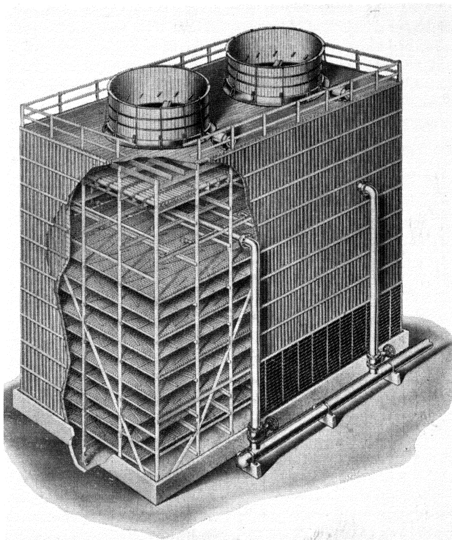
FIG. XVIII-5.—INTERNAL CONSTRUCTION OF WOODEN WATER COOLING TOWER.
