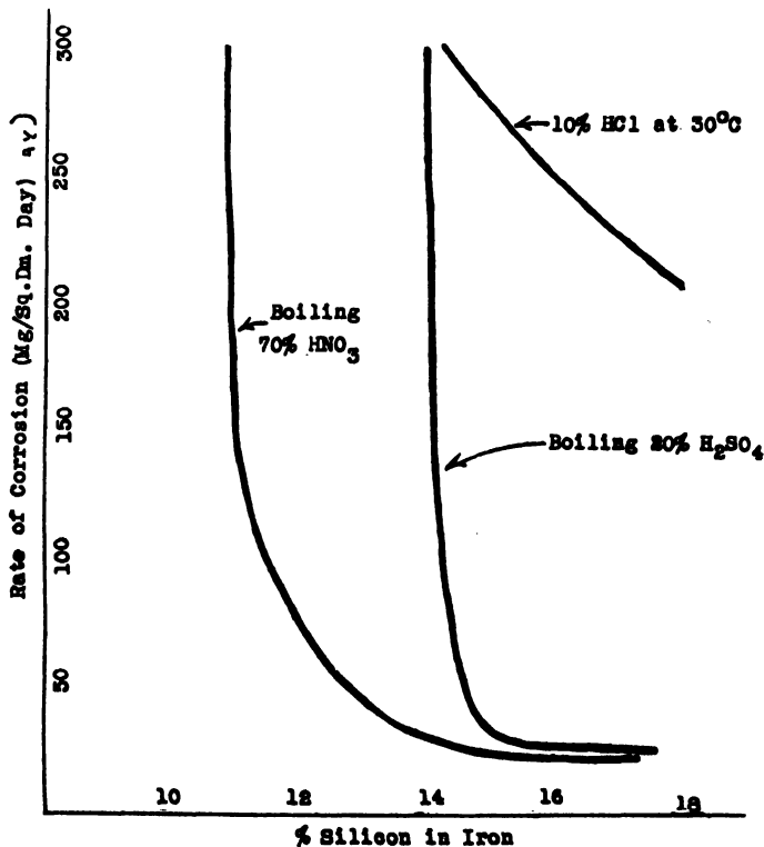
FIG. X-1.—ATTACK OF ACIDS ON SILICON-IRON ALLOYS.
