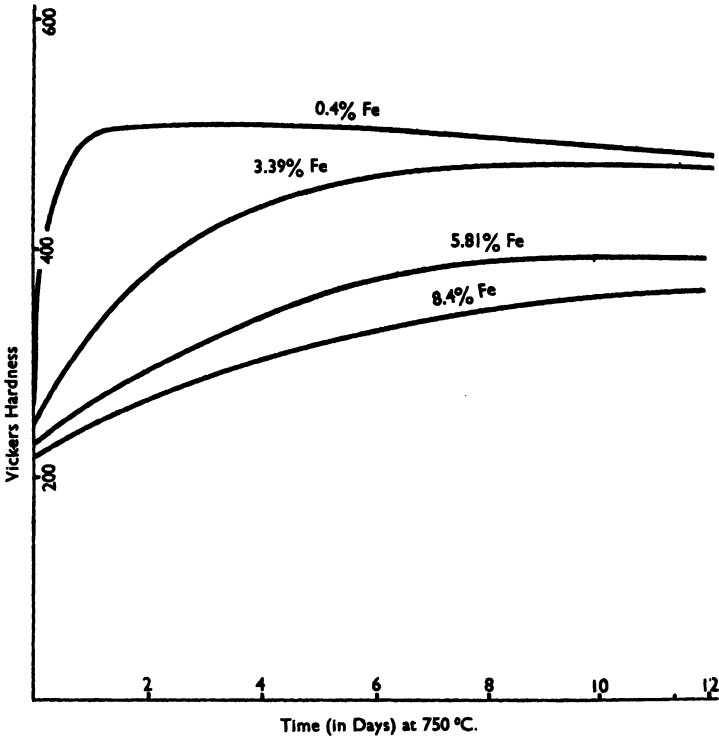
FIG. IX-7.—EFFECT OF IRON CONTENT ON CORROSIST HARDENING. (After Hallett, Proc. Chem. Eng. Grp. , 1950)
