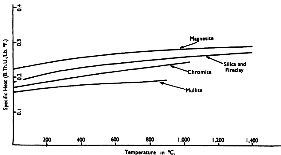
FIG. XVI-8.—SPECIFIC HEATS OF REFRACTORIES.
