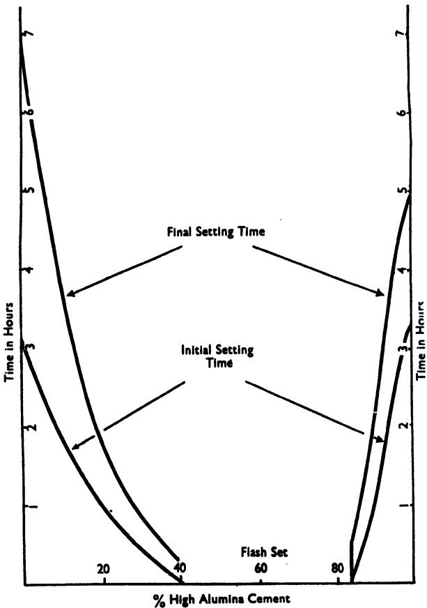
FIG. XIII-5.—SETTING TIMES FOR MIXTURES OF ALUMINA AND PORTLAND CEMENT.
