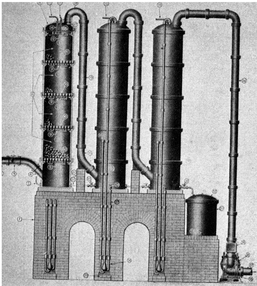
FIG. XV-6.—STONEWARE ABSORPTION TOWERS.
