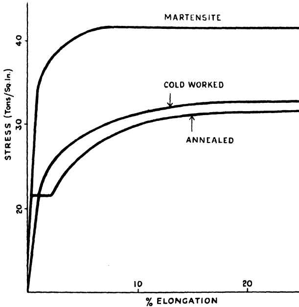
FIG. IV-5.—EFFECTS OF COLD WORKING OR QUENCHING.
