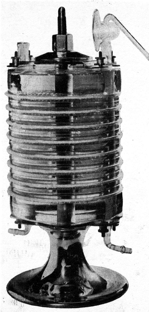
FIG. XVII-7.—ALL-GLASS FILTER PRESS.
