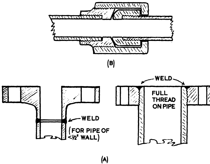
FIG. IV-9.—PIPE JOINTS.
