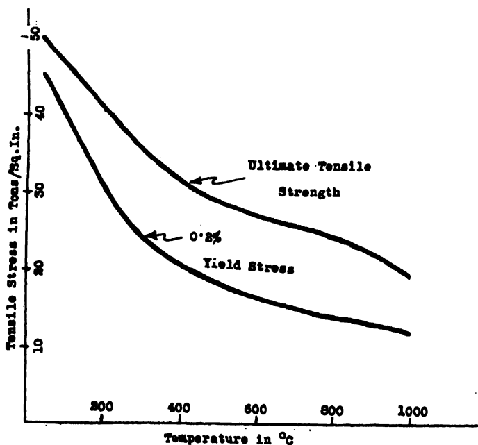
FIG. XI-3.—STRENGTH OF TITANIUM METAL.
