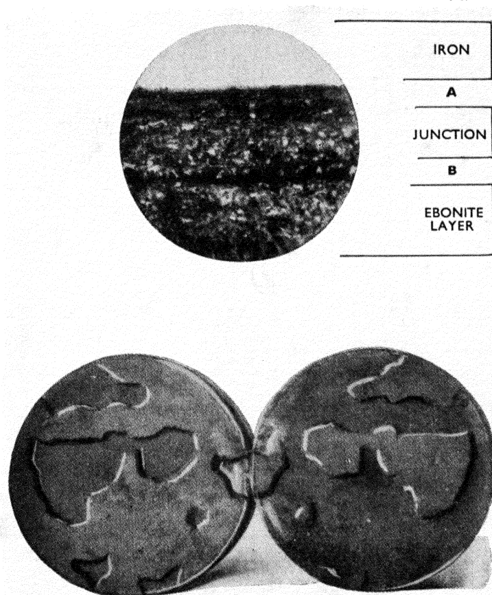
FIG. XIX-8.—ADHESION OF EBONITE TO IRON.
