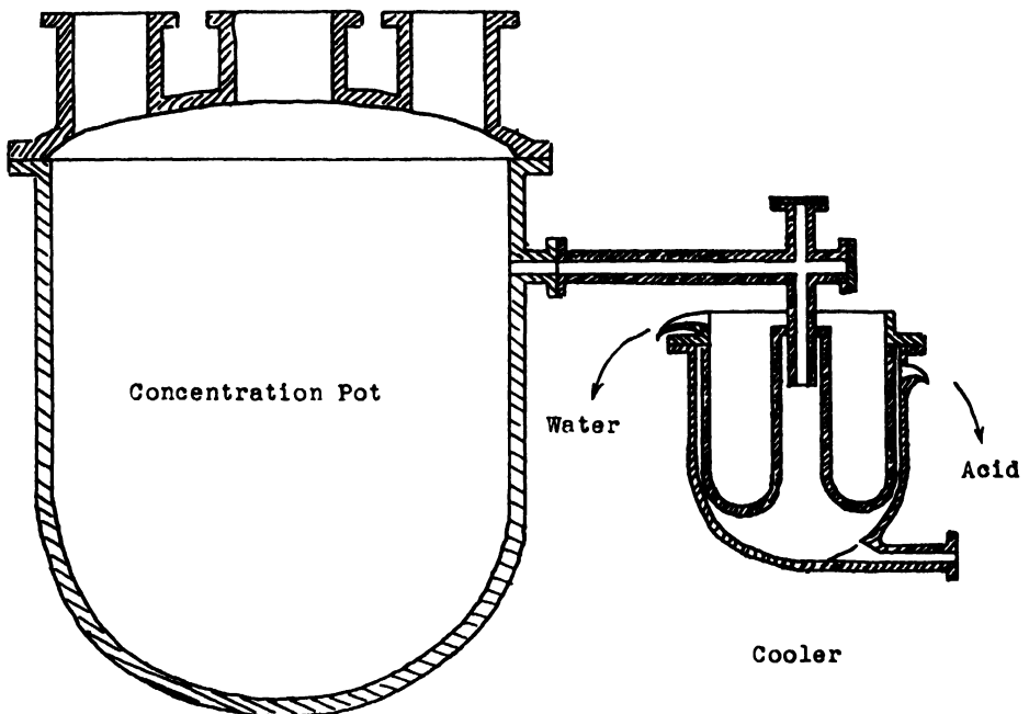
FIG. III-11.—CAST IRON CONSTRUCTION.
