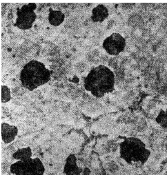
FIG. III-9.—GREY CAST IRON, AS FIG. III-7 AFTER NODULISING TREATMENT.
