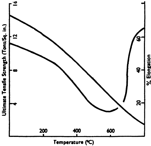
FIG. VIII-2a.—TOUGH PITCH ARSENICAL COPPER STRENGTH AND DUCTILITY v. TEMPERATURE.
