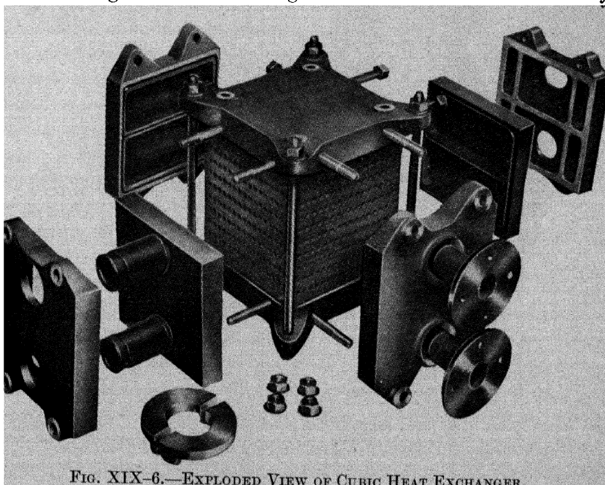
FIG. XIX-6.—EXPLODED VIEW OF CUBIC HEAT EXCHANGER.
