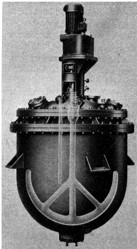
FIG. XII-7.—JACKETED ENAMELLED IRON REACTION VESSEL.
