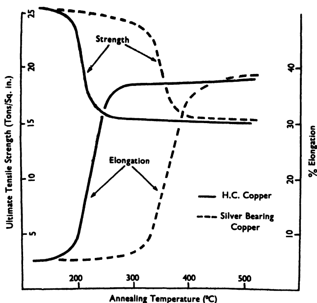
FIG. VIII-1.—EFFECT OF ANNEALING ON STRENGTH AND DUCTILITY.
