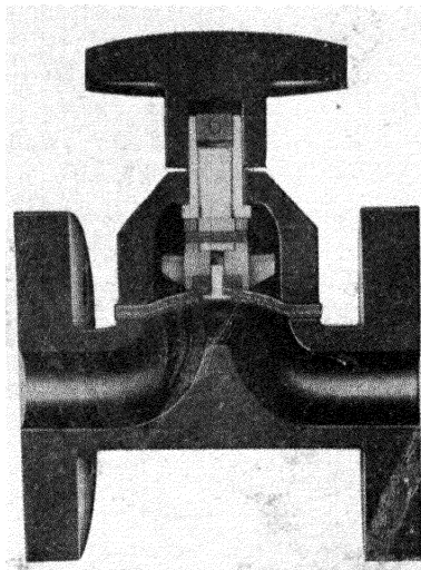
FIG. XIX-15.—VALVE IN EBONITE (with Soft Rubber Diaphragm).
