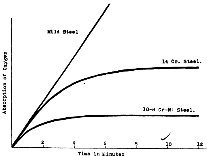
FIG. V-9.—INITIAL CORROSION RATES OF ALLOY STEELS.
