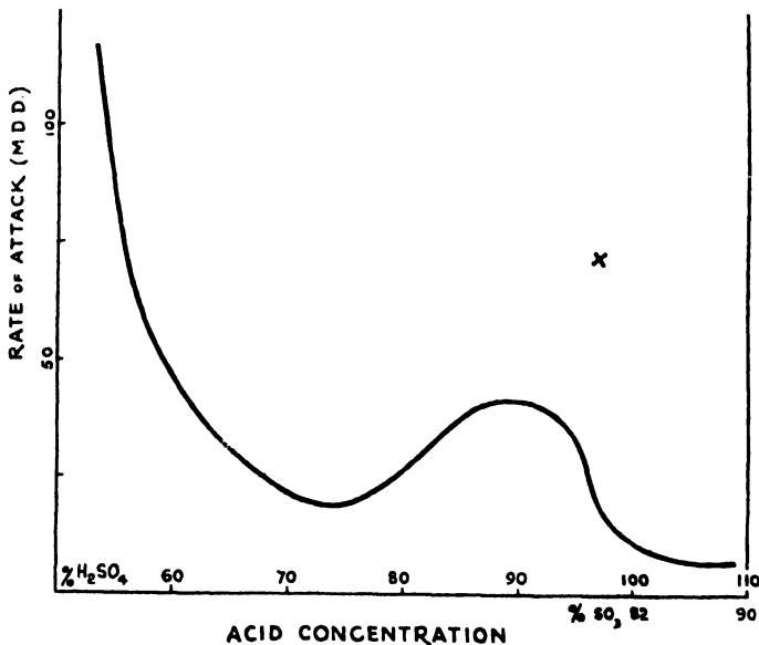
FIG. III-16.—ACTION OF COLD H 2 SO 4 ON CAST IRON.
