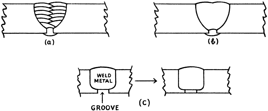
FIG. IV-8.—FUSION WELDS IN HEAVY PLATE.
