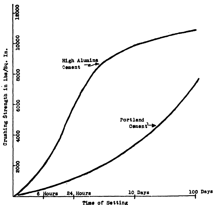
FIG. XIII-4.—SETTING OF ALUMINA AND PORTLAND CEMENTS.
