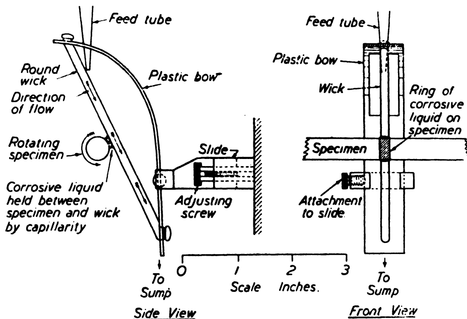
FIG. II-13.—CORROSION FATIGUE TEST.
