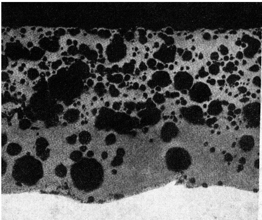
FIG. XII-5.—WET SPRAY ENAMEL ON MILD STEEL.
