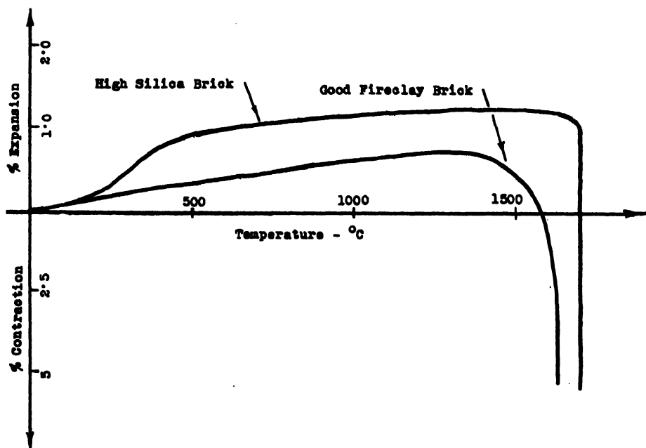
FIG. XVI-5.—REFRACTORINESS UNDER LOAD. (Rate of Heating—10° C./Min.)
