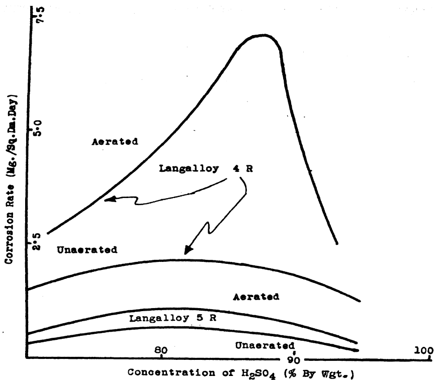
FIG. IX-9a.—RESISTANCE OF LANGALLOYS TO COLD SULPHURIC ACID. (After Richardson, Metallurgia , 1949)
