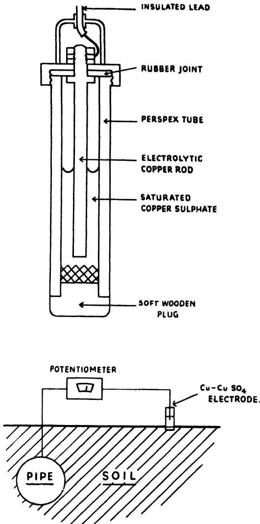
FIG. III-14.—Cu-CuSO 4 ELECTRODE FOR SOIL CORROSION TESTS.
