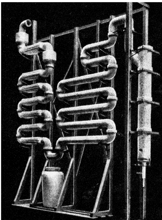
FIG. XVII-1.—HYDROCHLORIC ACID FROM H_2 AND Cl_2 PLANT IN VITREOSIL.
