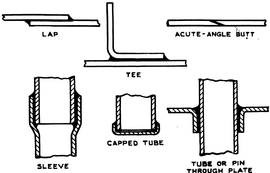
FIG. VIII-4.—EXAMPLES OF COPPER BRAZING.
