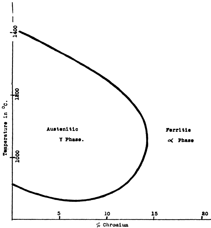
FIG. V-2.—EFFECT OF CHROMIUM ON AUSTENITE STABILITY.
