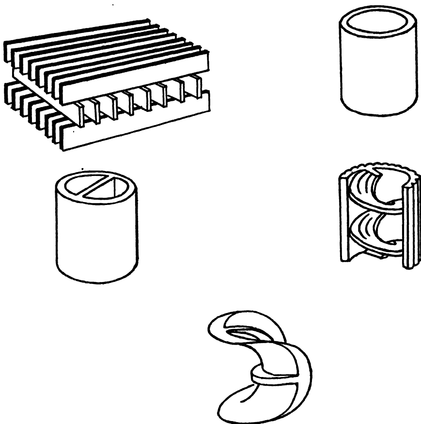
FIG. XV-7.—STONEWARE SHAPES FOR ABSORPTION TOWER PACKINGS.
