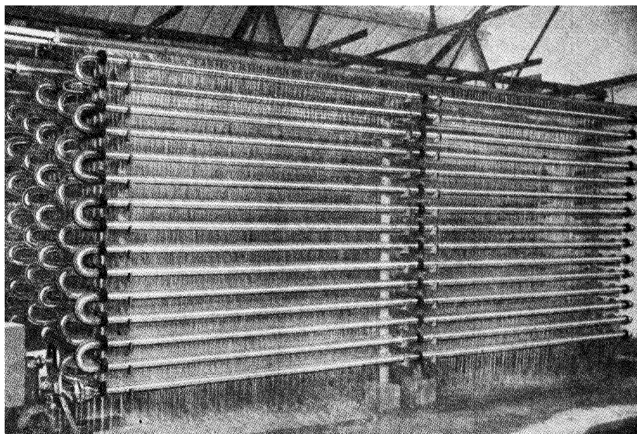
FIG. XVII-4.—SPRAY COOLERS IN GLASS PIPE.
