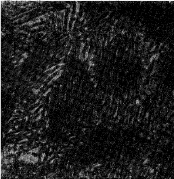
FIG. IV-2.—LAMELLAR PEARLITE.
