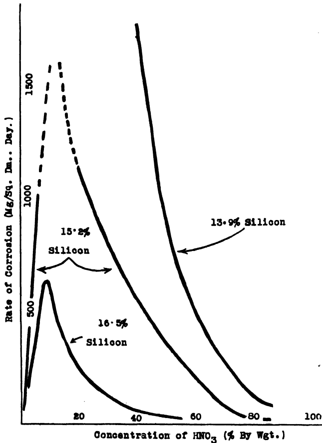
FIG. X-5.—CORROSION OF SILICON IRON BY BOILING NITRIC ACID.
