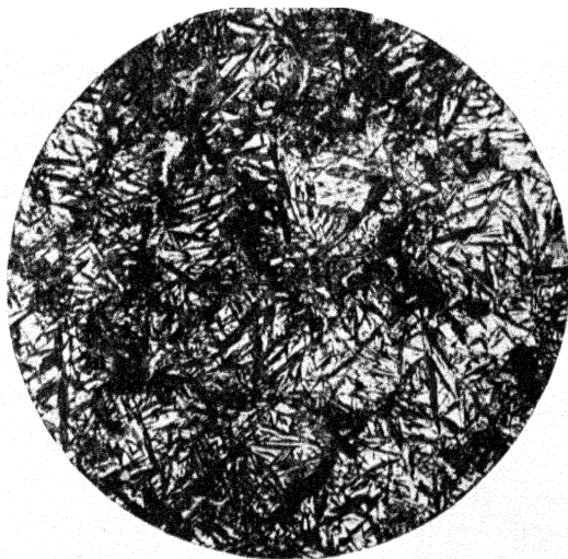
FIG. III-10.—MARTENSITIC CAST IRON. (From "Metallurgical Materials". Courtesy of V. N. Wood and Messrs. Chapman & Hall, Ltd.)
