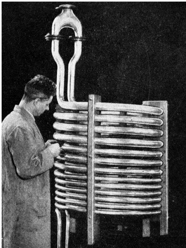
FIG. XI-1.—LARGE COOLING COIL IN PURE SILVER.
