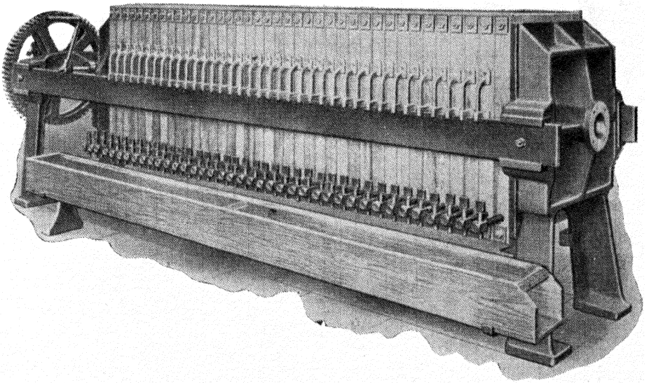
FIG. XVIII-3b.—WOODEN FILTER PRESS.
