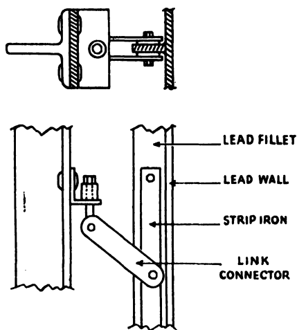
FIG. VI-3.—SUPPORT FOR LEAD CHAMBER WALL.
