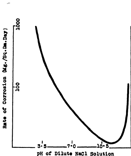
FIG. XII-1.—CORROSION OF ZINC BY AQUEOUS SOLUTION. EFFECT OF pH .
