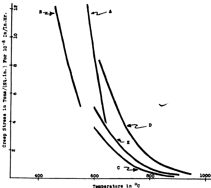
FIG. V-10b.—STRENGTHS OF HEAT RESISTING ALLOYS.
