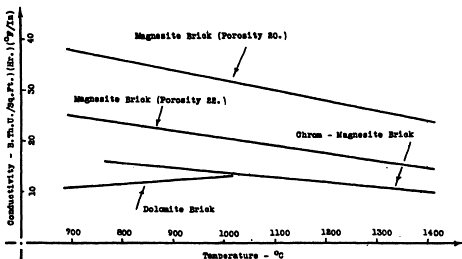
FIG. XVI-11.—CONDUCTIVITY OF ALKALINE REFRACTORIES.
