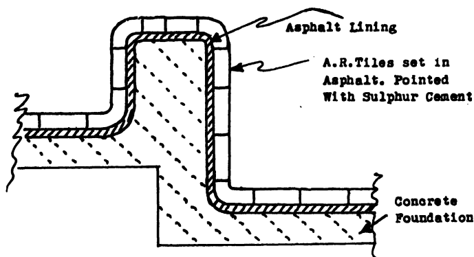
FIG. XIV-2.—SECTION THROUGH ACID PICKLING BATH WALL.
