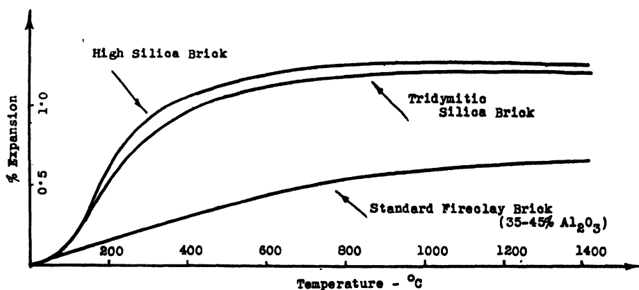
FIG. XVI-4.—THERMAL EXPANSION OF REFRACTORY BRICKS.
