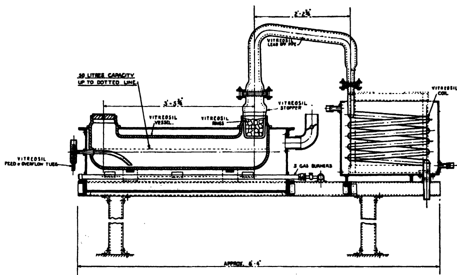
FIG. XVII-2.—VITREOSIL PLANT FOR PURE DISTILLED WATER.
