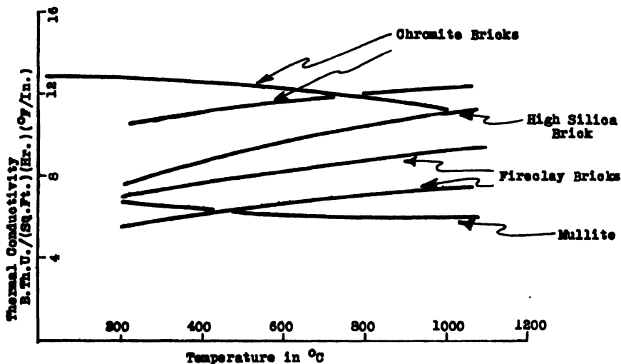
FIG. XVI-9.—THERMAL CONDUCTIVITIES OF TYPICAL REFRACTORIES.
