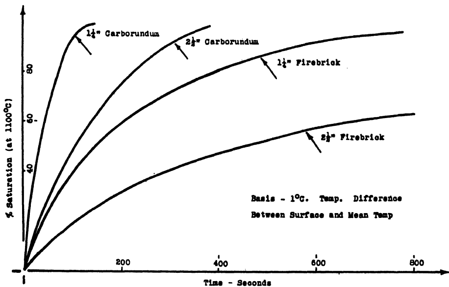
FIG. XVI-2.—HEAT SATURATION CURVES.
