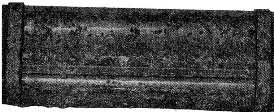
FIG. XII-3.—PAINT FAILURE AFTER 18 MONTHS. WIRE-BRUSHING FOLLOWED BY ONE COAT RED LEAD AND TWO COATS A.R. PAINT. INDUSTRIAL ATMOSPHERIC CONDITIONS.
