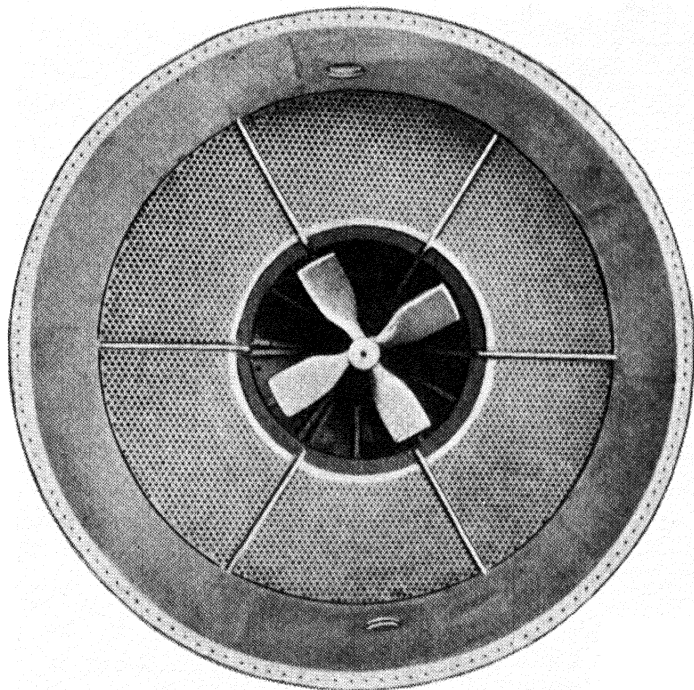
FIG. IX-3.—SECTION OF 24 FT. DIAM. NICKEL EVAPORATOR.
