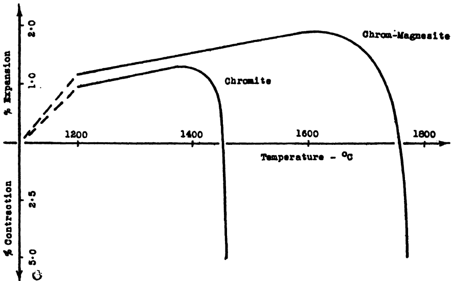
FIG. XVI-1.—REFRACTORINESS UNDER LOAD. Temperature Rising at 10^{\circ}/\text{Min} .
