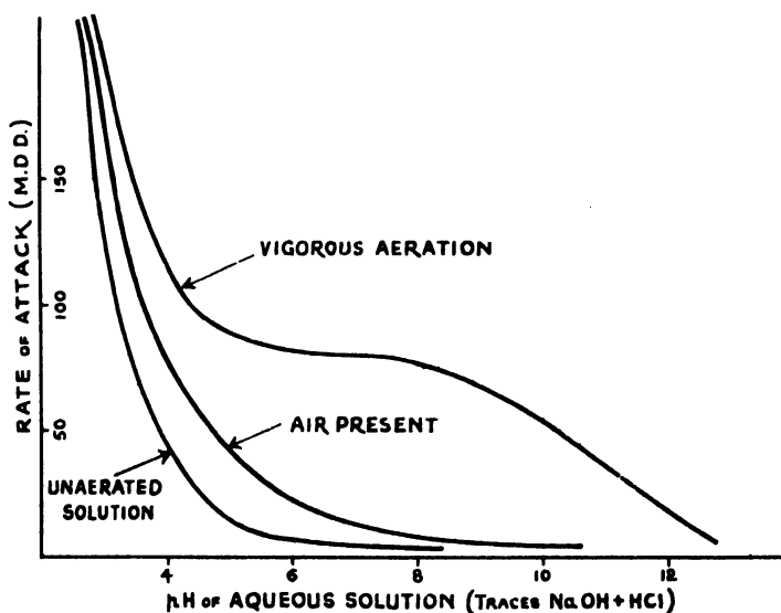
FIG. III-15.—CORROSION OF CAST IRON.
