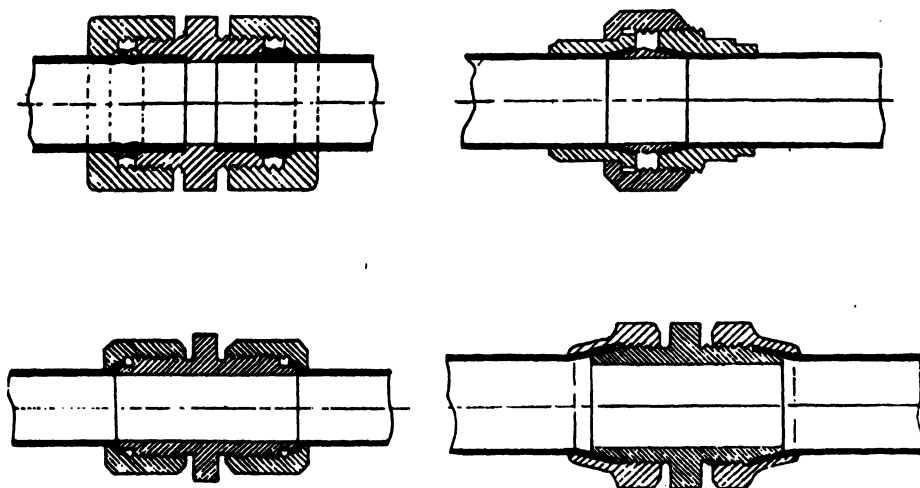
FIG. VIII-5.—SELF-SEALING PIPE JOINTS.
