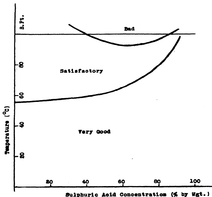
FIG. IX-9b.—RESISTANCE OF CORROSIST B TO SULPHURIC ACID. (After Hallett, Proc. Chem. Eng. Group , 1950)
