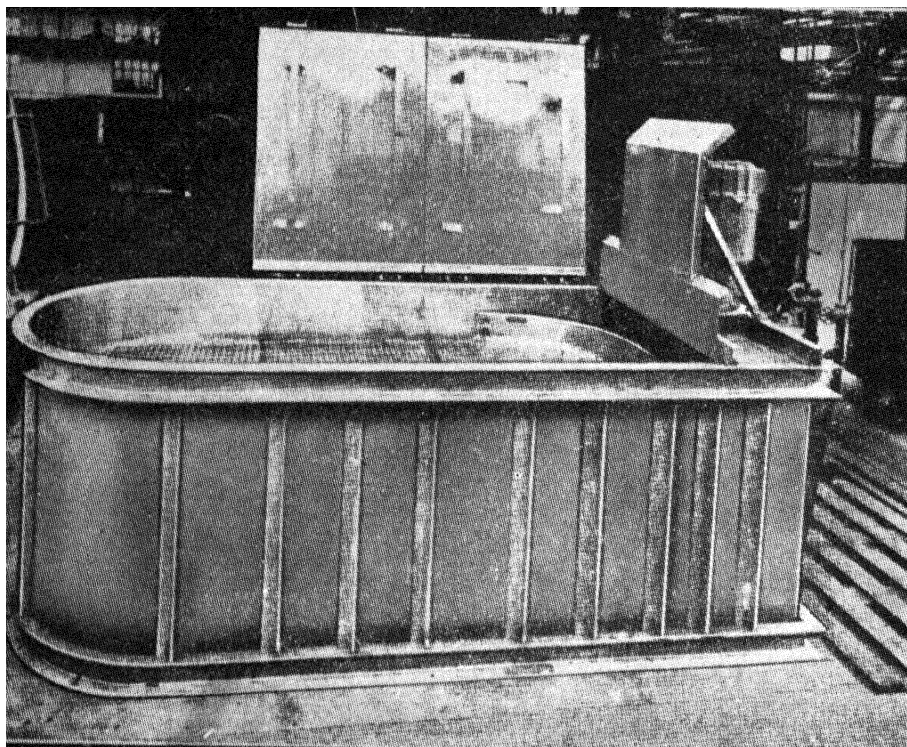
FIG. V-7.—STAINLESS-STEEL VESSEL WITH MILD-STEEL REINFORCEMENT.
