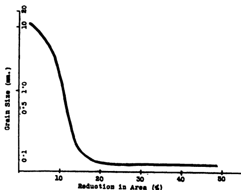
FIG. VII-1.—REDUCTION IN ALUMINIUM GRAIN SIZE BY COLD WORKING.
