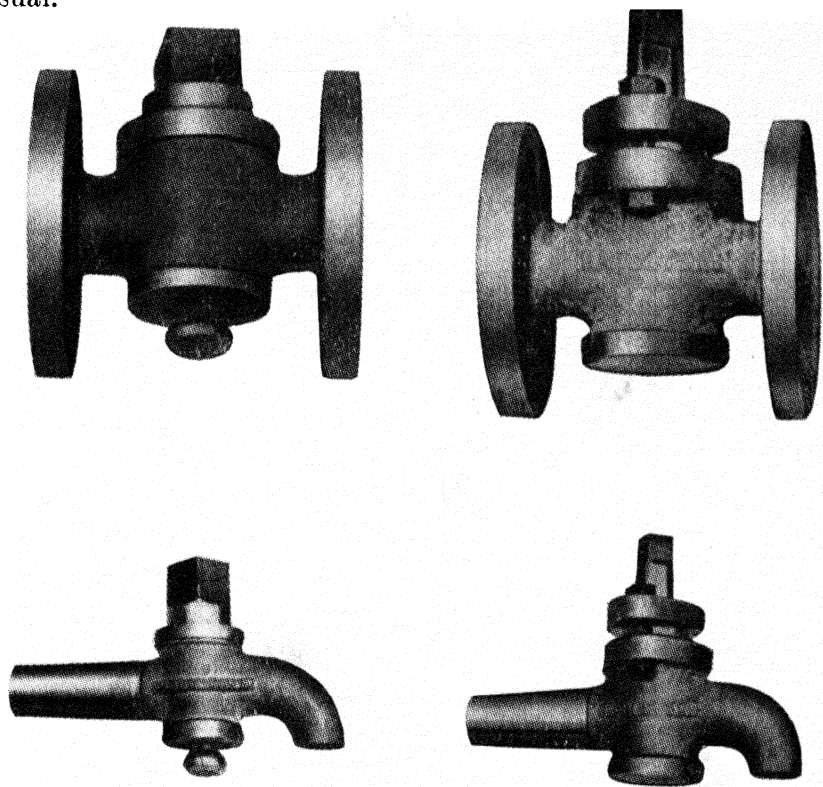
FIG. VI-9.—TAPS IN HARD LEAD AND SILICON IRON.
