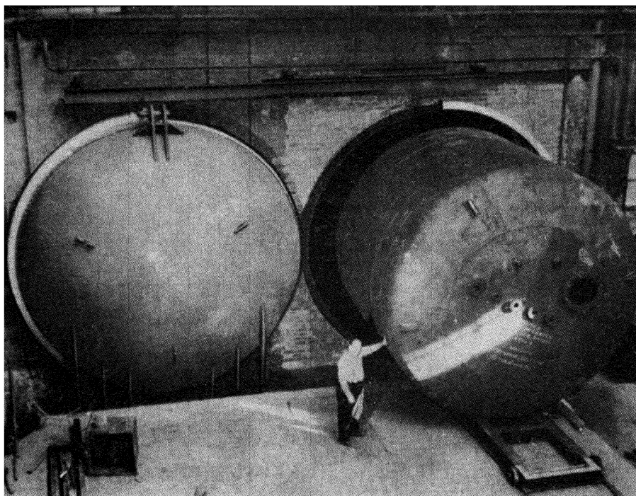
FIG. XIX-9.—LINED TANK ENTERING VULCANISING PAN. Pan size 15 ft. dia. \times 20 ft. long.
