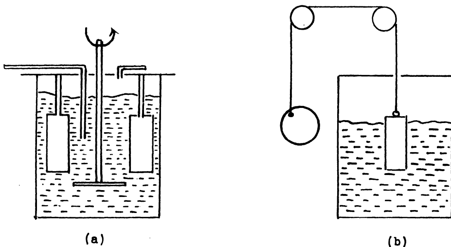
FIG. II-8.—CORROSION TESTING.
