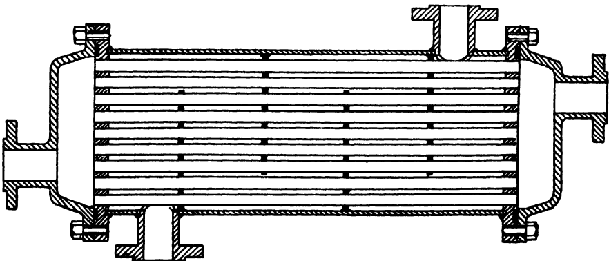
FIG. IV-10.—TUBE AND SHELL CONSTRUCTION.
