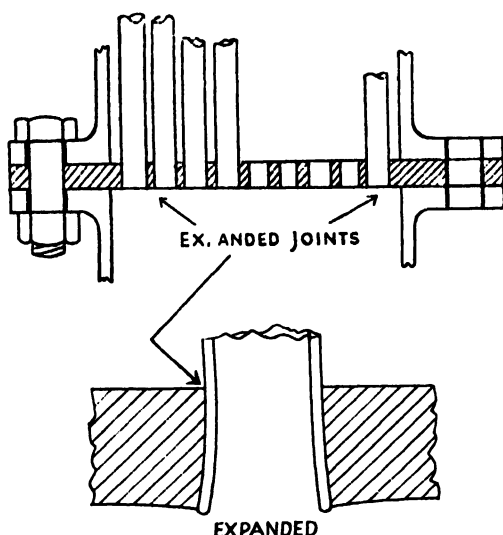
FIG. IV-11.—"EXPANDED" JOINTS.
