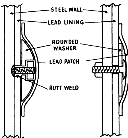
FIG. VI-4.—ATTACHMENT OF LEAD LINING.
