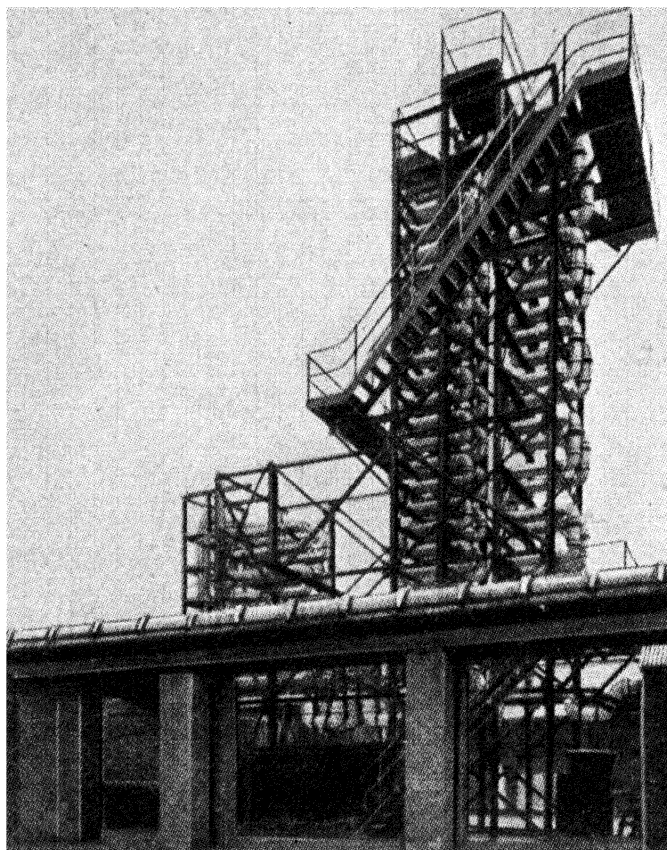
FIG. XVII-3.—LARGE VITREOSIL CONDENSERS AND GAS SCRUBBERS
