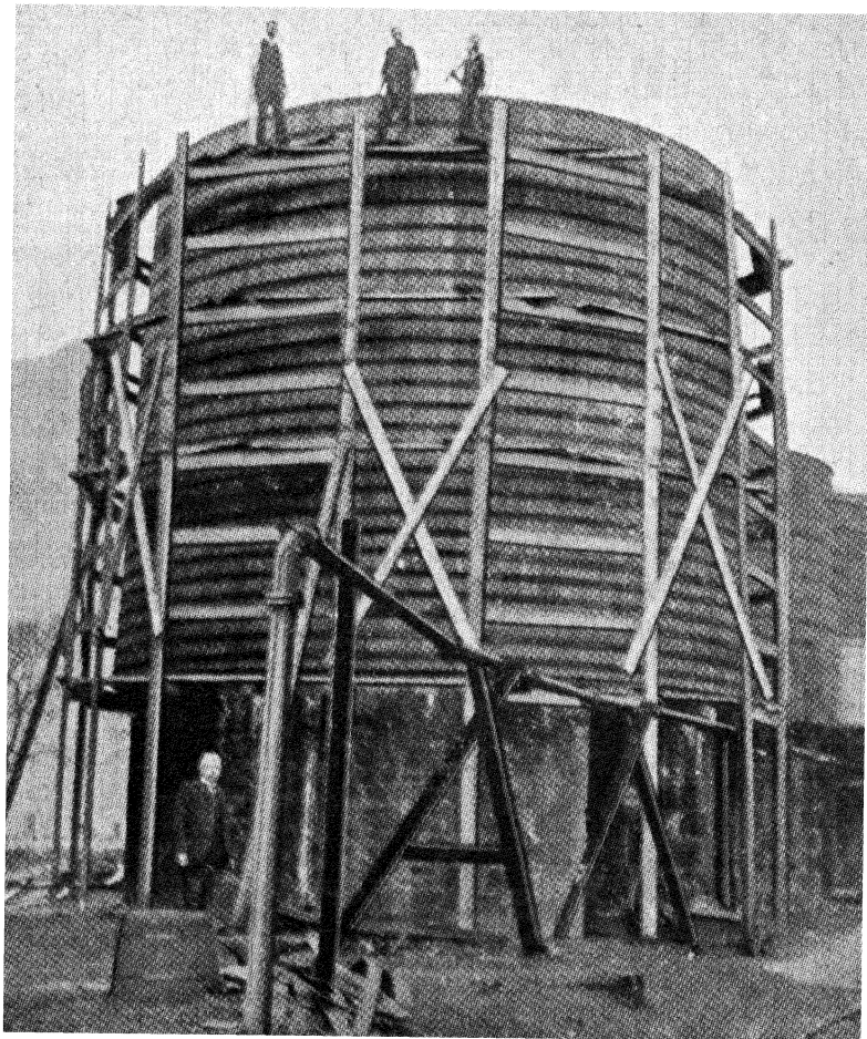
FIG. XVIII-2.—WOODEN VAT OF 115,000 GALLONS CAPACITY.
