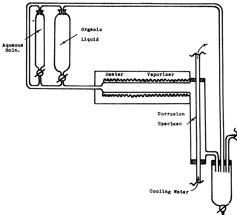
FIG. II-10.—CORROSION UNDER CONDENSATION CONDITIONS.
