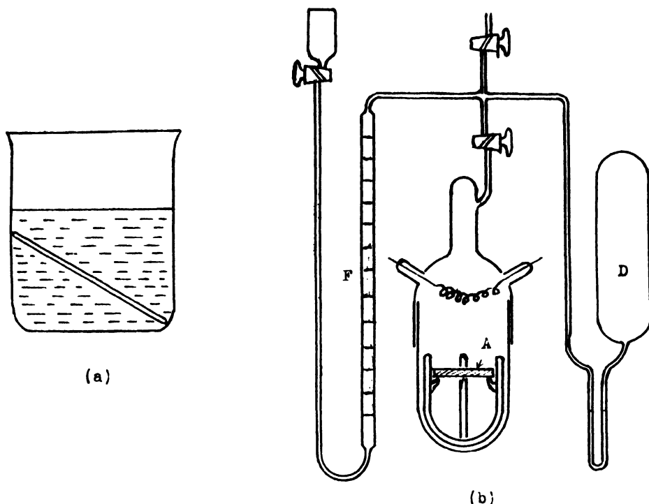
FIG. 11-7.—CORROSION TESTING.
