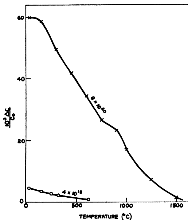
Figure 7. Recovery of c -spacing changes: eight hour anneals
