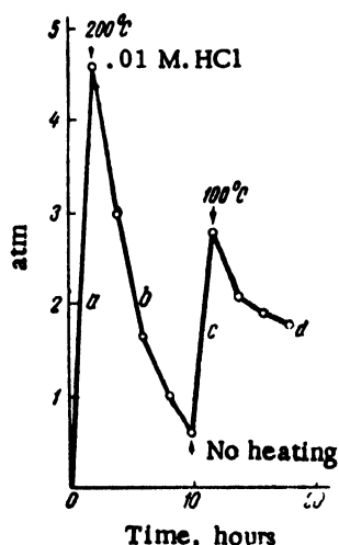
Figure 7. Influence of temperature on radiolysis of hydrochloric acid solution
