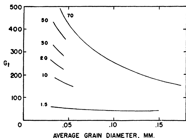
Figure 2. Combined effect of grain size and cold work upon growth rate ( G_t ) of uranium under thermal cycling: (curve numbers denote per cent reduction in area by rolling after which the specimens were recrystallized at 575°C, G_t = micro-in./in./cycle)
