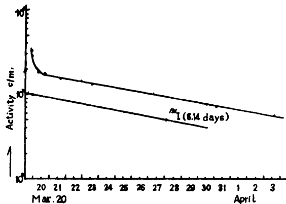
Figure 6A. Decay curve of iodine fraction
