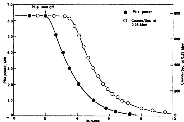
Figure 7. Active gas evolved after pile shut-off (He flow 6000 \text{cm}^3/\text{min} )
