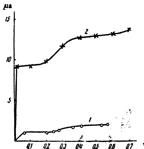
Figure 3. Dependence of the strength of the polarizing current on the potential during the action of gamma radiations: (1) stationary electrode; (2) rotating electrode
