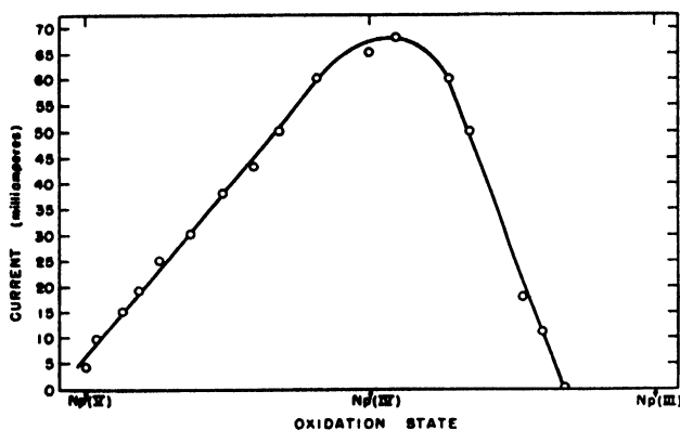
Figure 7. Current-time behavior in reduction of Np(V) at a cathode potential of approximately -0.15 volt.
