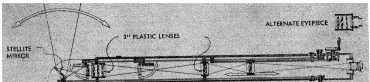
Figure 1. Through-wall periscope showing arrangements of mirror control, lens interchange and light path
