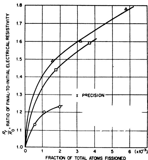
Figure 1. Effect of fission in Al-U alloys: Wt.% U: circles, 5.7; squares, 17.2; triangles, 15
