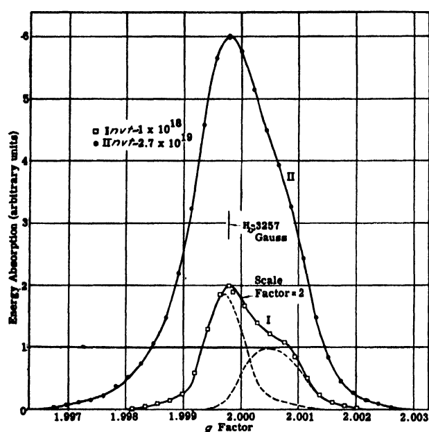
Figure 17. Paramagnetic resonance at 9121 megacycles in Corning silica glass
