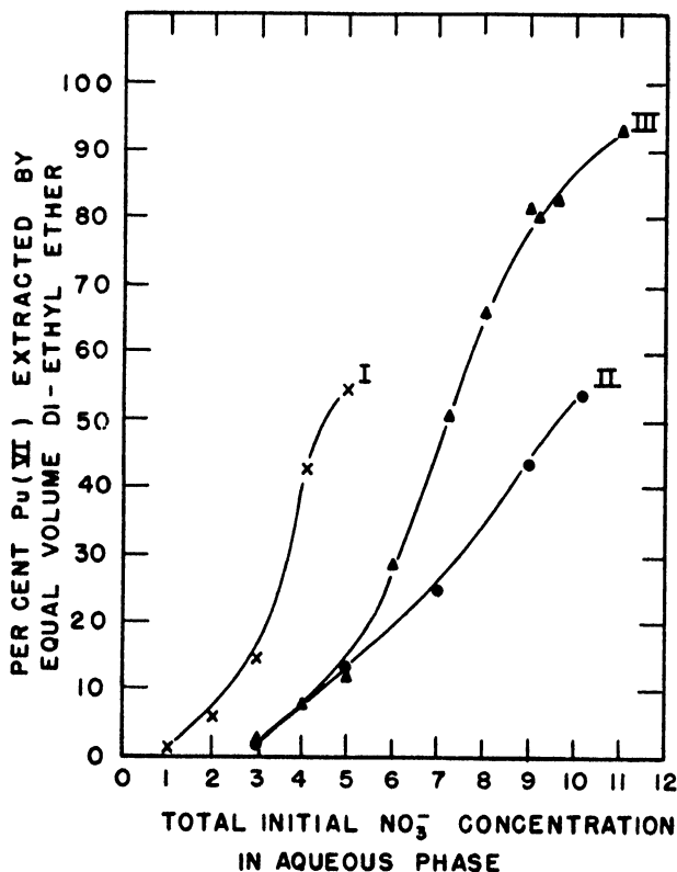
Figure 6. Effect of total nitrate ion concentration on the extraction of plutonium(VI) by diethyl ether: (curve I) \text{HNO}_3 only; (curve II) 1 M \text{HNO}_3 + \text{NH}_4\text{NO}_3 ; (curve III) 1 M \text{HNO}_3 + \text{Ca}(\text{NO}_3)_2 . (Brody, Orlemann, Jensen, and Dixon, unpublished information, 1944)
