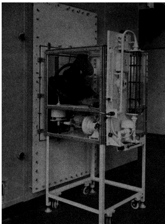
Figure 5. Glove box attached to one of the panels of the decontamination room showing worker in pressurized suit
