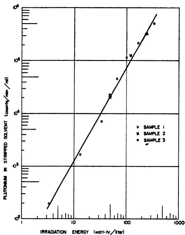
Figure 5. Plutonium retention in irradiated 30% tributyl phosphate in naphtha solvent
