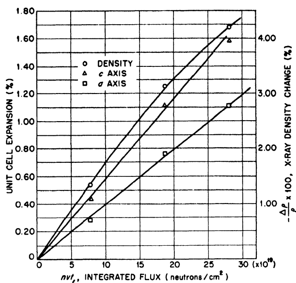
Figure 3. Effect of radiation on density and unit cell expansion for a zircon single crystal
