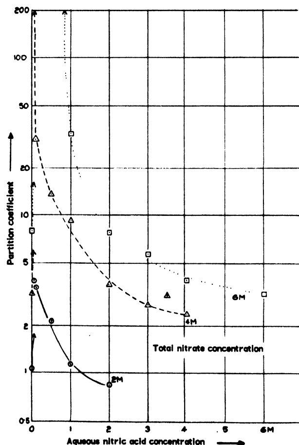
Figure 3. Salting-out of thorium by sodium nitrate into 19% TBP/kerosene
