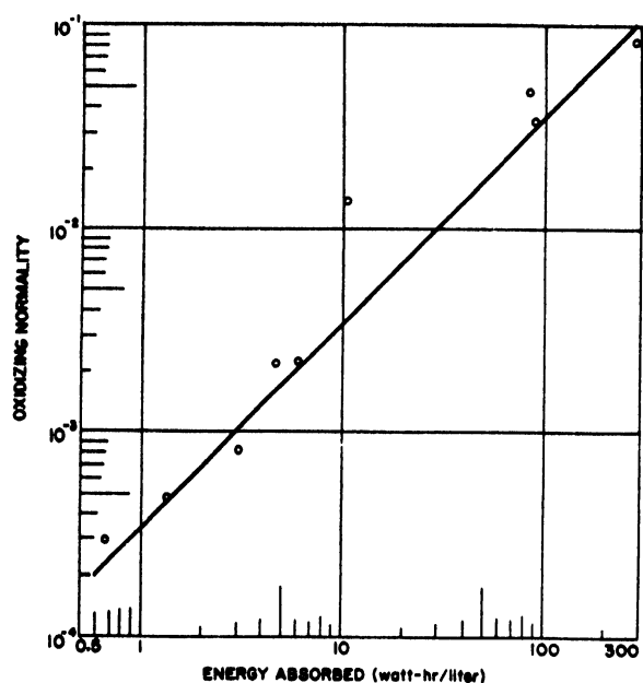
Figure 7. Oxidizing power of irradiated 40% tributyl phosphate in naphtha solvent
