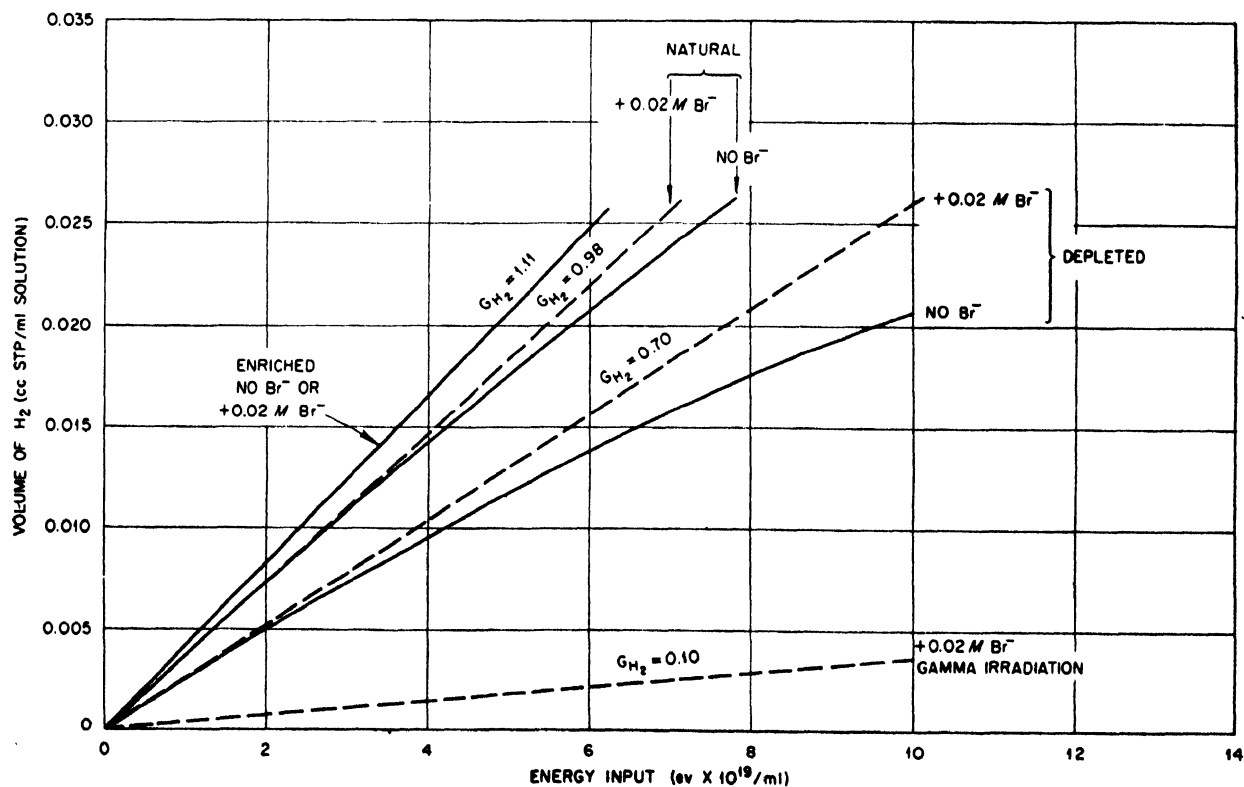
Figure 3. Effect of type of radiation on hydrogen yield from irradiated UO_2SO_4 solutions (concentration \sim 200 gm U/liter)
