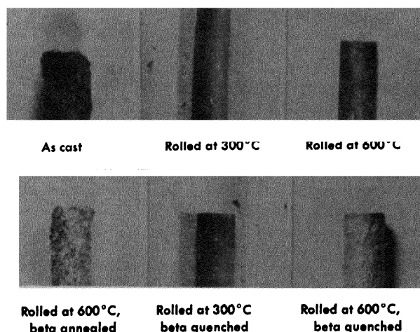
Figure 10. Relative appearance of various uranium specimens after irradiation to 0.1% atom burn-up
