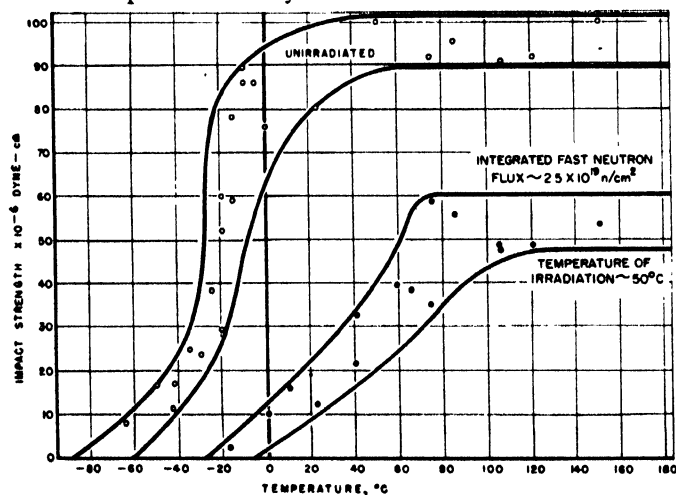
Figure 5. The effect of reactor irradiation on the impact strength of SA-70 pressure vessel steel
