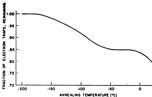
Figure 10. Annealing of electron traps measured by susceptibility
