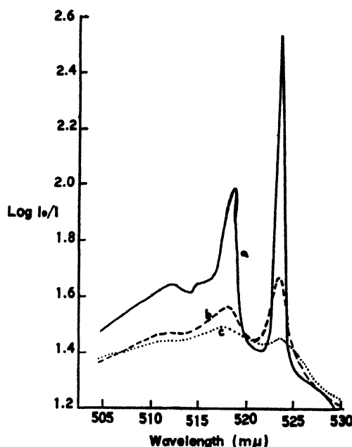
Figure 4. Absorption bands of LiF after ten minute neutron irradiation and nine hours Mineralight at room temperature. Measured at (a) — 190°C, (b) — 120°C and (c) — 75°C
