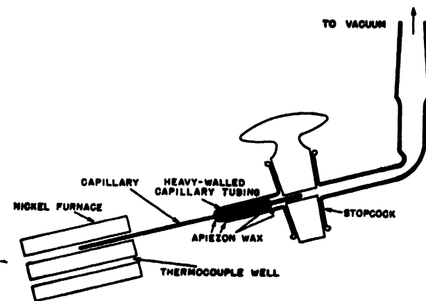
Figure 2. Apparatus for opening capillaries
