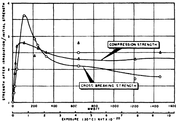
Figure 1. Changes in mechanical strength as function of exposure for parallel cut KC graphite
