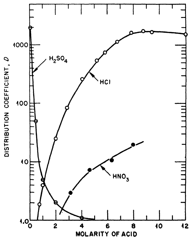
Figure 2. Adsorption of U(VI) from various mineral acids
