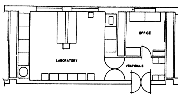
Figure 1. Self-contained standard suit comprising vestibule, office and laboratory
