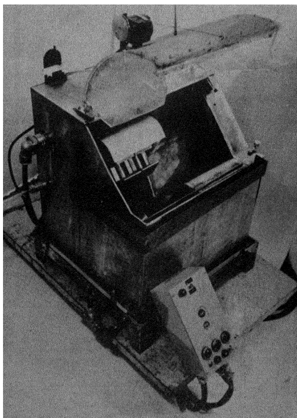
Figure 22. Remotely operated cut-off machine and its controls
