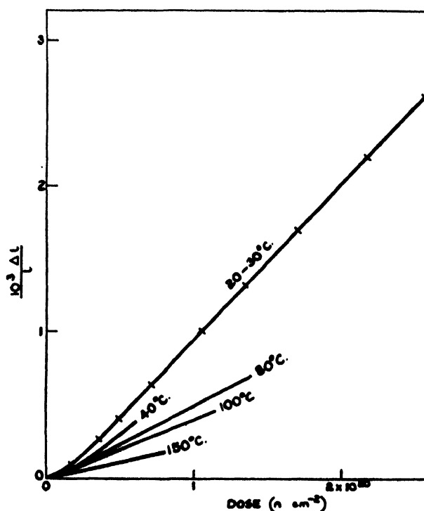
Figure 6. Growth perpendicular to extrusion direction at different irradiation temperatures
