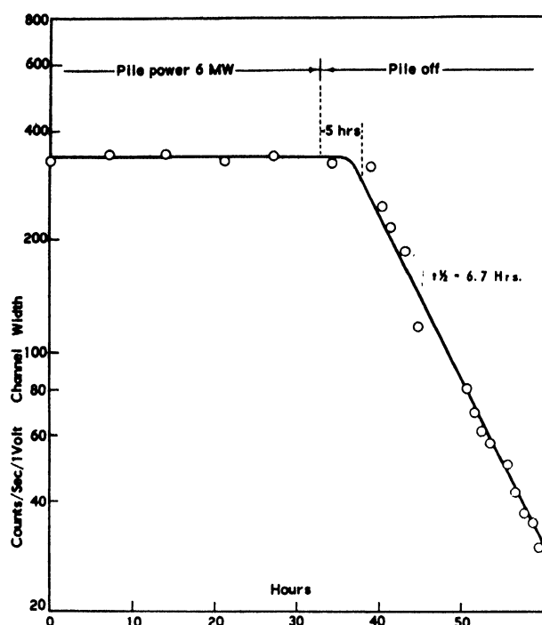
Figure 6. \text{Xe}^{135} evolved after pile shut-off (He flow 1 cc/min)
