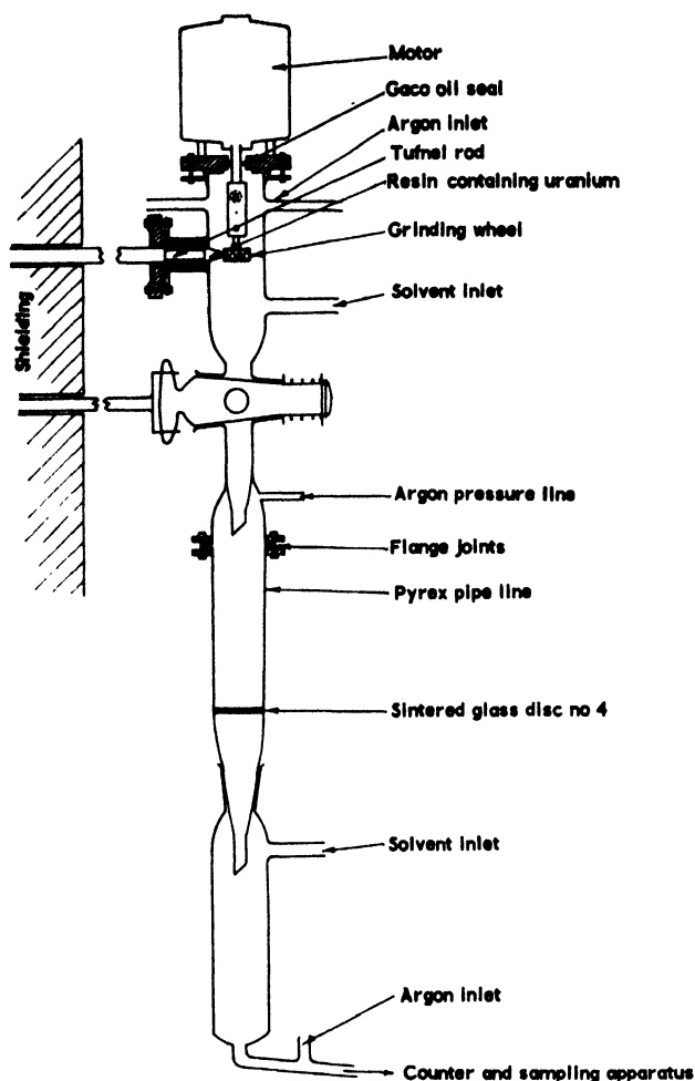
Figure 1. Grinding apparatus (half size)
