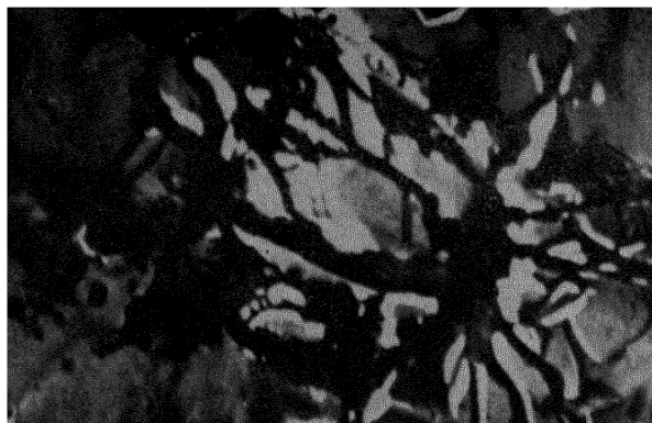
Figure 7. Uranium carbide grain after irradiation ( \times 15,000 )
