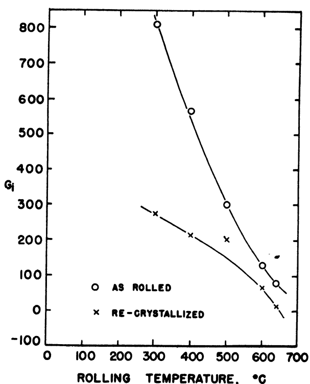
Figure 8. Effect of rolling temperature on the irradiation growth rate of oval-rolled uranium
