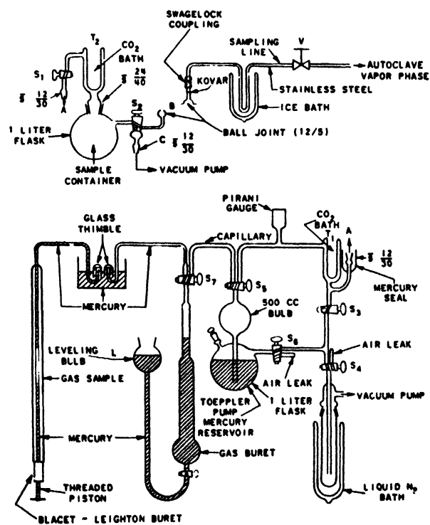
Figure 4. Gas sampling, transfer and analysis apparatus
