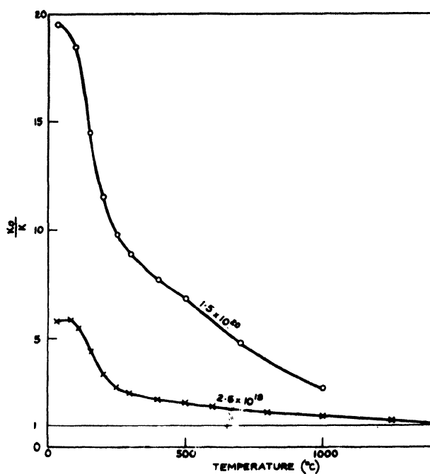
Figure 5. Recovery of thermal resistivity changes; two hour anneals
