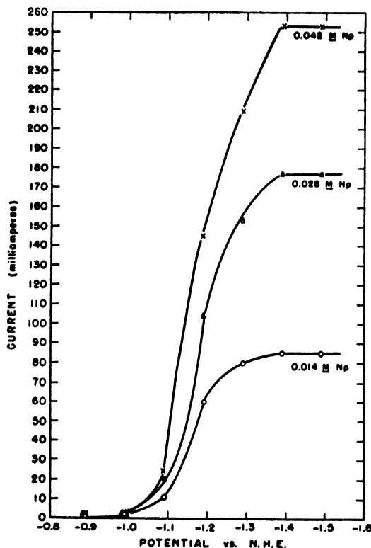
Figure 6. Current-voltage curve obtained in the oxidation of Np(V) to Np(VI)
