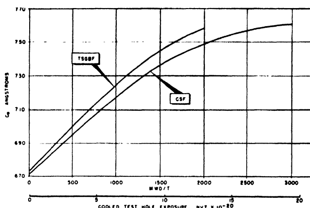
Figure 13. C_0 displacement in irradiated graphite
