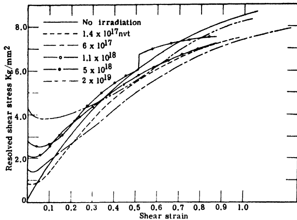
Slide 1. Stress-strain curves of neutron-irradiated copper single crystals
