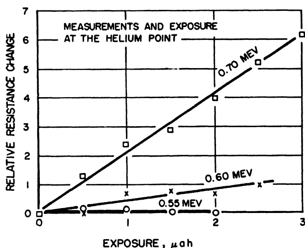
Figure 1. The change in the electrical resistance of a 0.0001 cm thick nickel foil as a function of exposure for various electron energies
