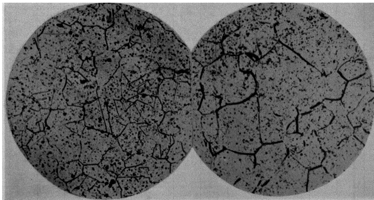
Figure 3. Microstructure of nickel: (left) before irradiation; (right) after irradiation
