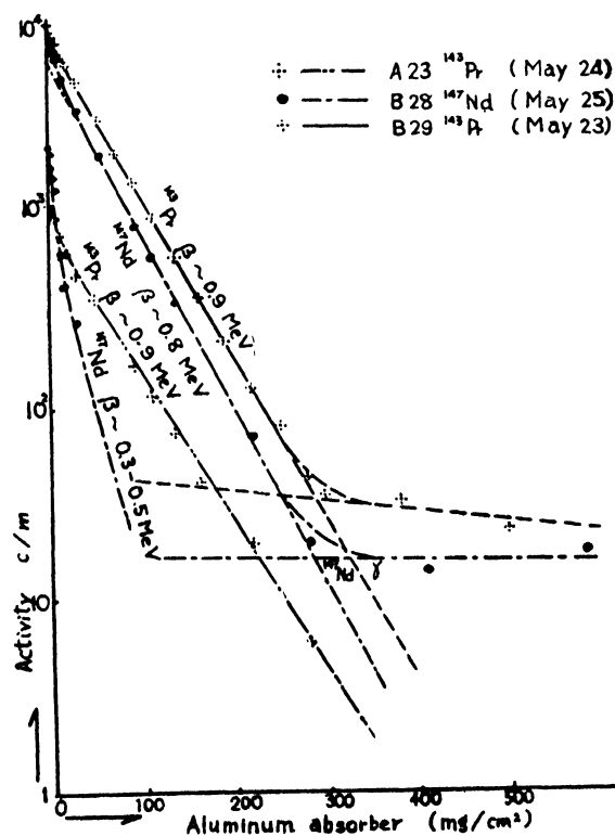
Figure 13. Aluminum absorption curves of Pr and Nd fractions
