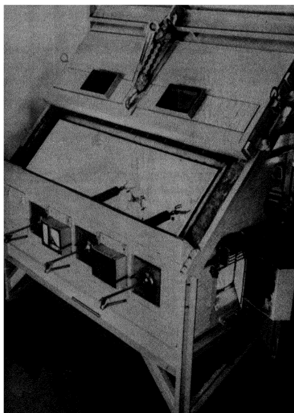
Figure 11. Atmosphere box for gamma radiation
