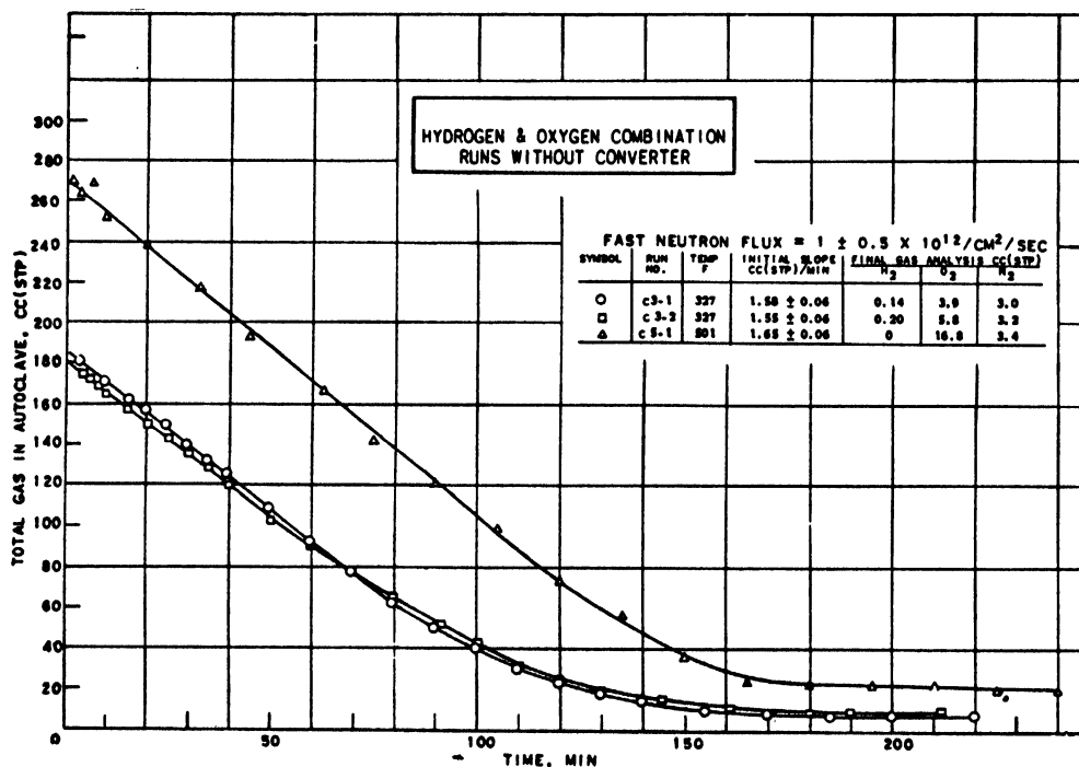
Figure 5. Hydrogen and oxygen combination runs without converter
