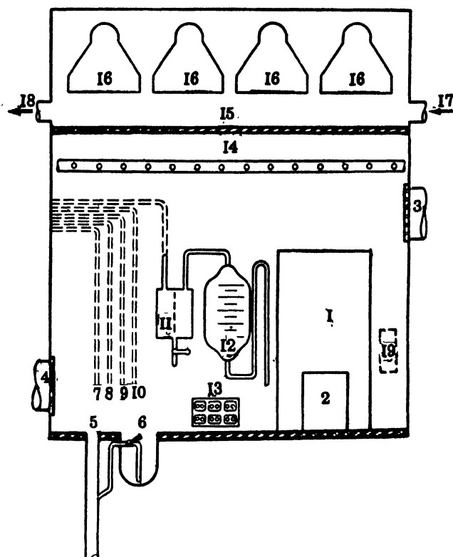
Figure 5. Equipment of a hot cell: (1) access door for entrance of personnel and delivery of equipment into the cell; (2) small door which closes the channel, connecting the cell with conveyor; (3) indraft ventilation duct with prefilter; (4) exhaust ventilation duct with prefilter; (5) drain; (6) collection bottle; (7) hot water; (8) cold water; (9) portable shower; (10) duplicate line of the air-vacuum system; (11) trap, filled with alkali solution; (12) intermediate buffer vessel; (13) electrical inlet; (14) wall shower; (15) glass, separating the illuminating lamps from the cell; (16) illuminating lamps; (17) indraft ventilation duct for cooling the illuminating lamps; (18) exhaust ventilation duct for cooling the illuminating lamps; (19) dosimeter
