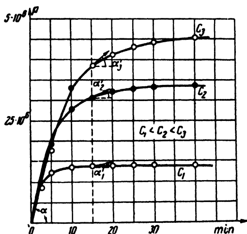
Figure 5. Dependence of electrodeposition on initial element concentration C in the electrolyte
