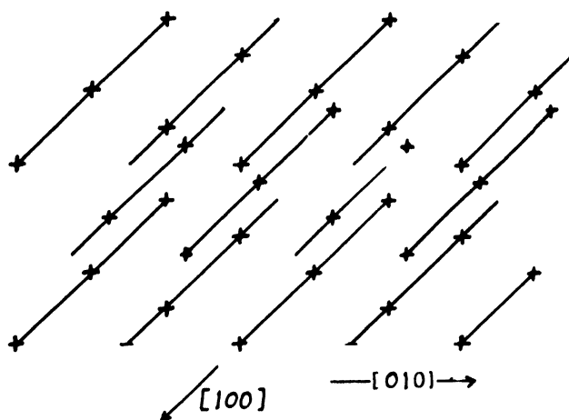
Slide 23. Growth of uranium by a diffusion mechanism: (slip plane is [010] and direction [100] )
