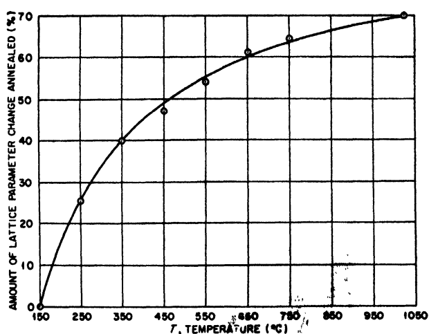
Figure 8. Lattice expansion annealing in diamond
