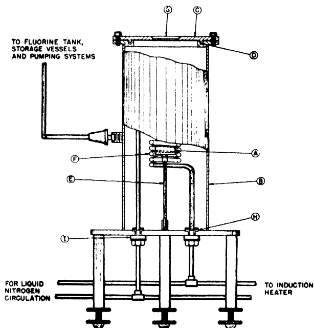
Figure 1. Reactor for plutonium hexafluoride: (A) nickel dish filled with \text{PuF}_4 ; (B) brass reactor can; (C) removable cover for loading reactor; (D) tongue and groove, teflon gasket for closure; (E) nickel supporting rod for nickel dish; (F) coil of \frac{3}{16} -in. copper tubing; (G) fluorothene window; (H) teflon seal and insulator; (I) micalox insulator
