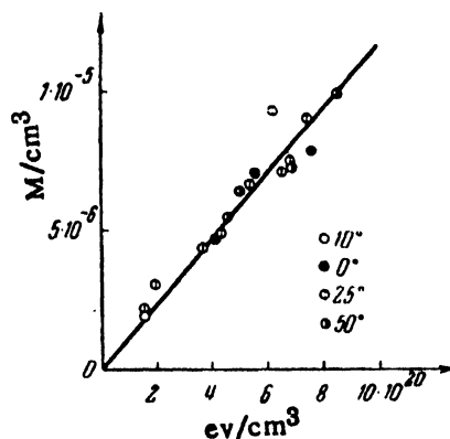
Figure 4. Formation of aldehyde upon irradiation of oxygen-free ethyl alcohol at various temperatures
