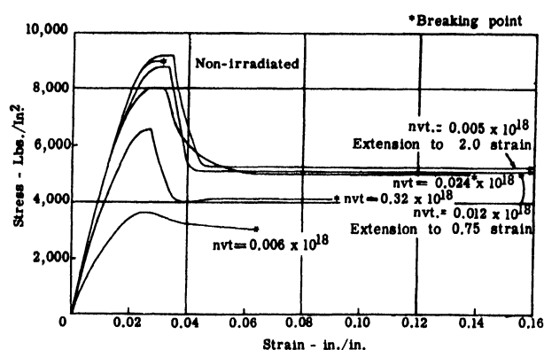
Slide 16. Stress-strain curves for pile irradiated vinyl chloride acetate
