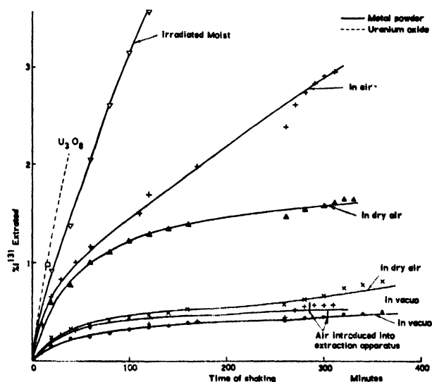
Figure 3. Extraction of I 131 from uranium powder irradiated under various conditions
