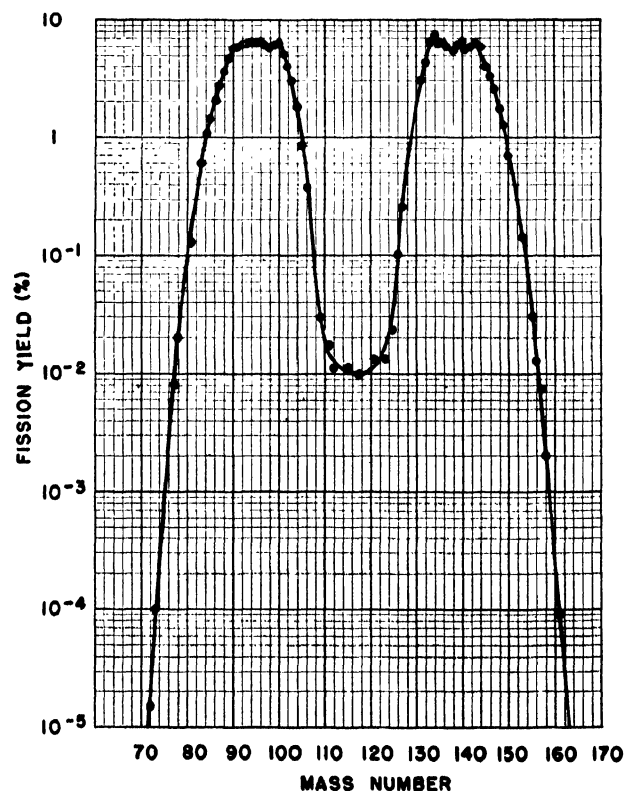
Figure 5. Yield-mass curve for slow neutron-induced fission of U 235
