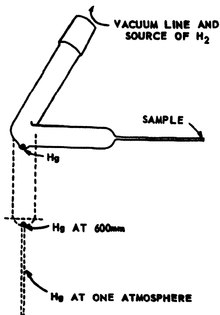
Figure 4. Hydride apparatus
