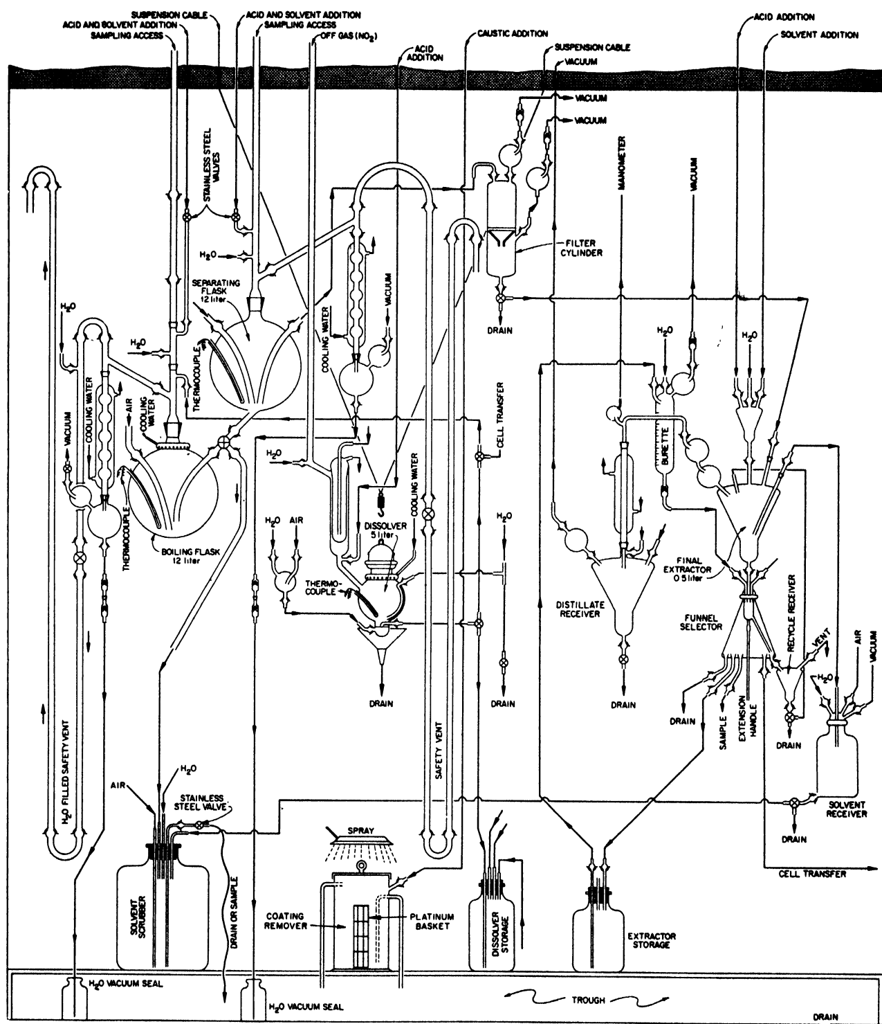
Figure 12. Laboratory-scale solvent extraction equipment for remote operation
