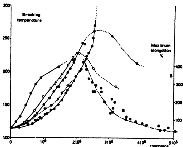
Figure 7. Variation in melting point (curves I to IV) and of maximum elongation of samples (curve B) as a function of the irradiation dose in the presence of air. Curve I, intensity 432 r/min; curve II, intensity 113 r/min; curve III, intensity 42.3 r/min; curve IV, intensity 7.3 r/min
