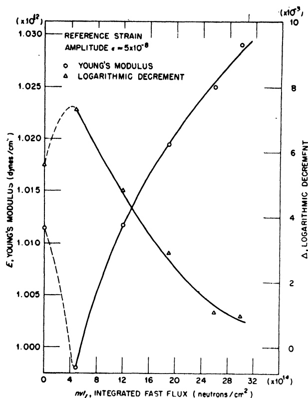
Slide 4. Young's modulus and logarithmic decrement vs integrated flux for copper single crystals
