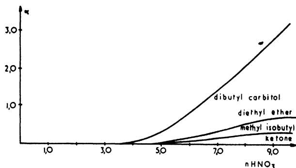
Figure 5. The partition of thorium between nitric acid and diethyl ether, dibutyl carbitol and methyl isobutyl ketone
