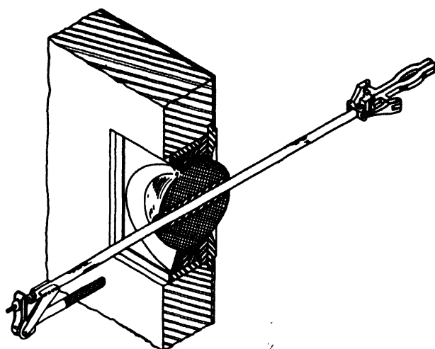
Figure 3. Section through shielding wall showing ball socket manipulator
