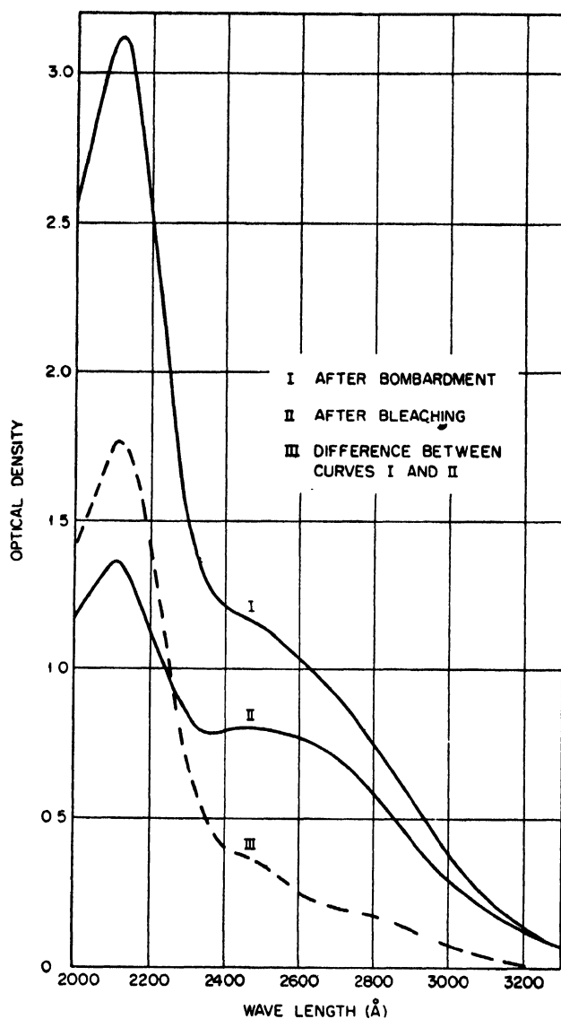
Figure 14. Optical density vs wave length for fast neutron bombarded Corning silica glass
