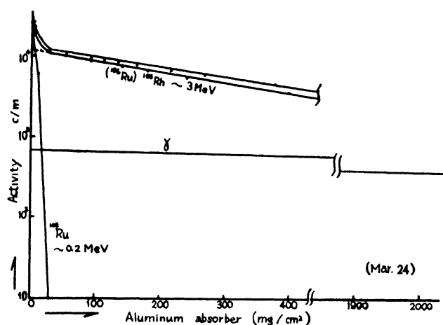
Figure 8. Absorption curve of Ru (Rh) fraction
