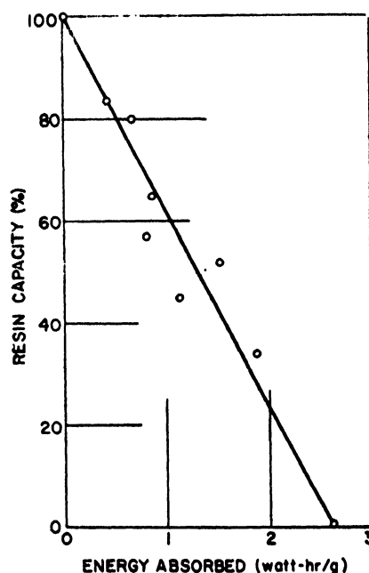
Figure 3. Capacity loss of Dowex A-1 anion-exchange resin (quaternary amine polystyrene) as a result of \text{Co}^{60} gamma irradiation
