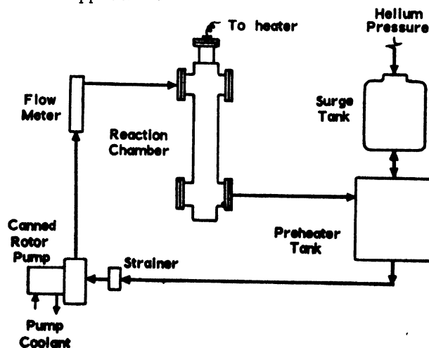
Figure 1. Flow diagram of thermal test loop
