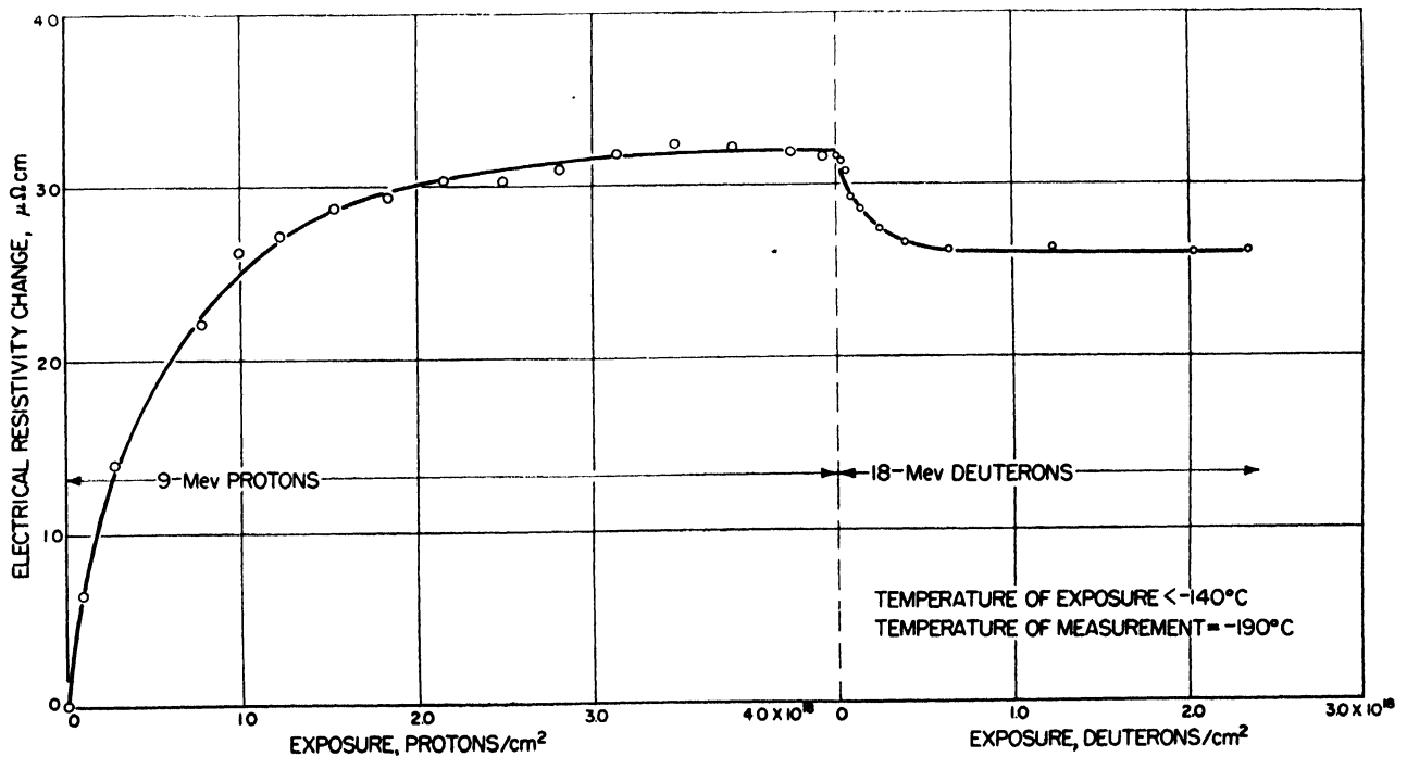
Figure 2. The change in the electrical resistivity of 0.0005 cm thick thorium foil as a function of exposure to protons and deuterons
