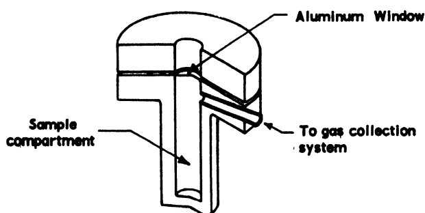
Figure 6. Steel exposure cell for electron irradiations
