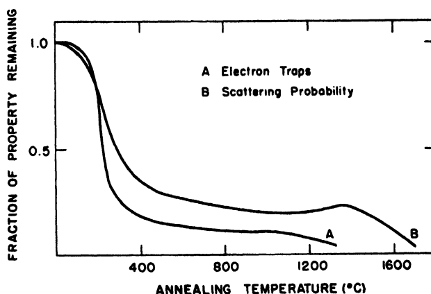
Figure 7. Annealing of electron traps and scattering centers
