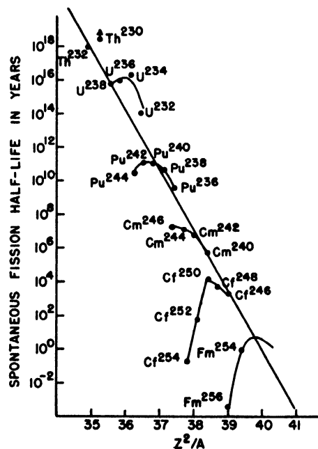
Figure 2. Spontaneous fission half-life versus Z^2/A
