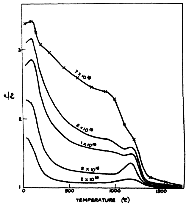
Figure 2. Recovery of resistivity changes: one hour anneals
