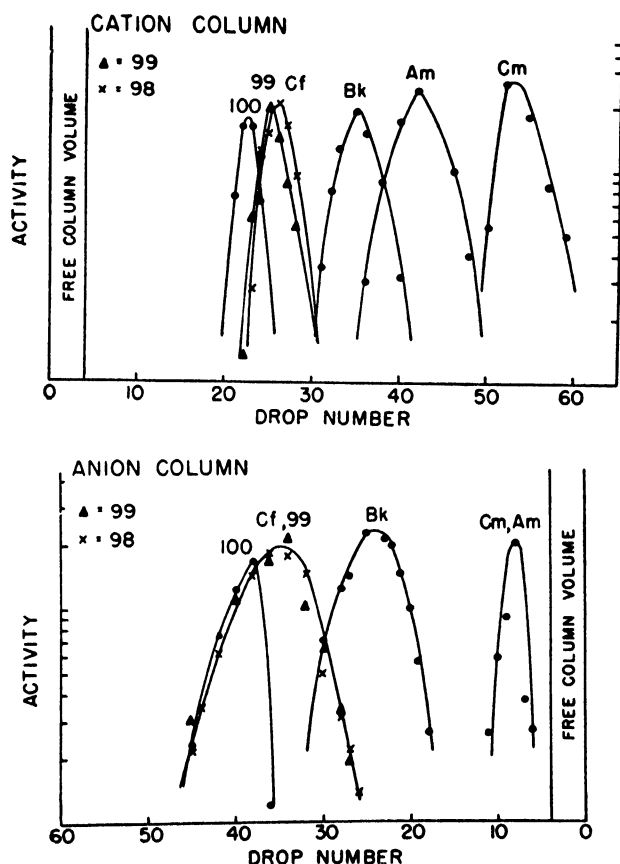
Figure 10. (top) Elution of actinides from Dowex-50 resin with 20 per cent alcohol-12.5 M HCl; (bottom) elution of actinides from Dowex-1 resin with 13 M HCl. Figure reprinted from reference 88
