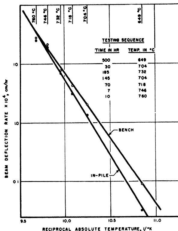
Figure 4. The effect of reactor exposure on the creep rate of type 347 stainless steel beams
