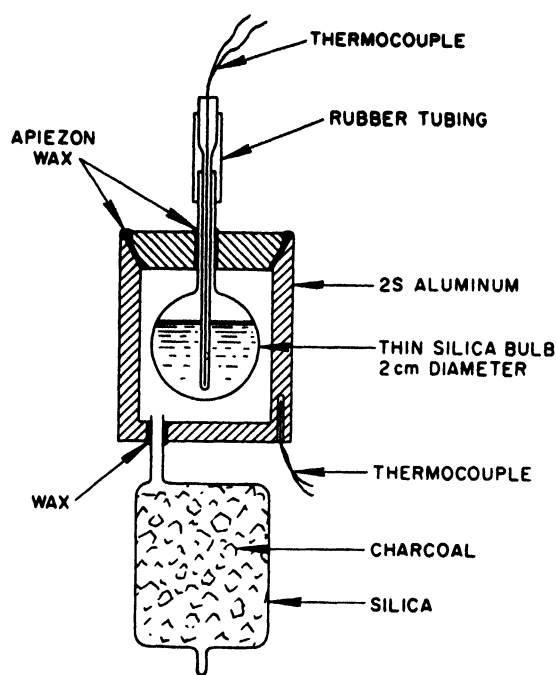
Figure 1. Calorimeter for measuring reactor radiation absorbed in water and uranium solutions
