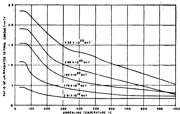
Figure 37. Effect of annealing temperature on thermal conductivity: all exposures 30^\circ\text{C}
