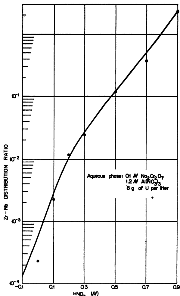
Figure 2. Effect of nitric acid concentration on distribution ratio of zirconium and niobium in methylisobutyl ketone extraction
