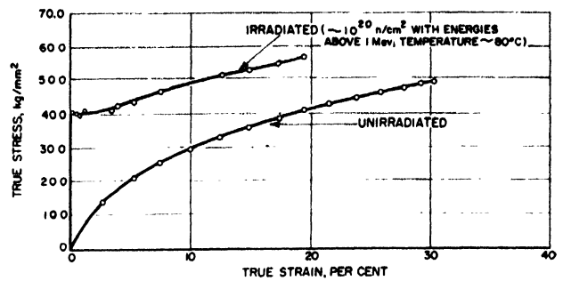
Figure 3. The effect of reactor exposure on the stress-strain curve of nickel
