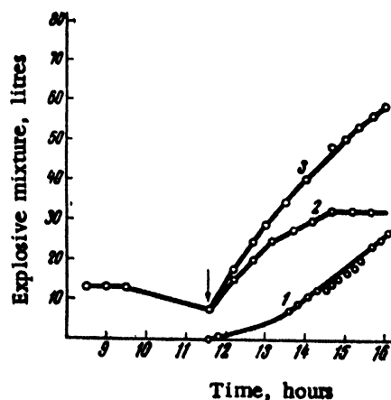
Figure 2. Accumulation of explosive mixture in liquid and gas at 42 kw: (curve 1) accumulation in gas; (2) in liquid; (3) total accumulation
