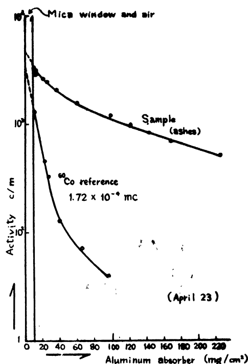
Figure 2. Aluminum absorption curves of ashes and Co 60 reference sample
