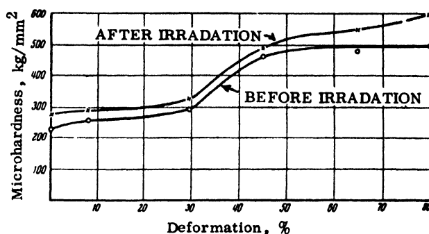
Figure 6. Change in hardness of type X18H9T stainless steel specimens as a function of degree of preliminary deformation: O, before irradiation; X, after irradiation
