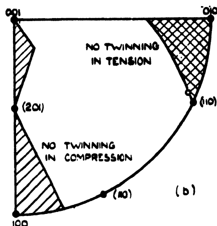
Slide 21. Restrictions on twinning in uranium (after Cahn)
