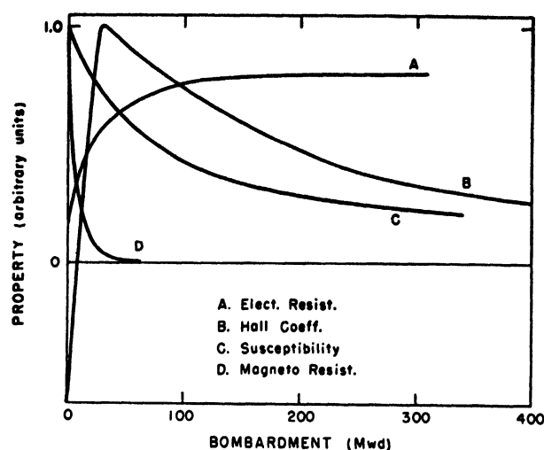
Figure 5. Electrical properties after bombardment
