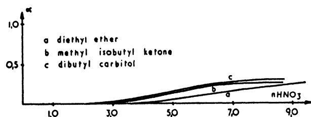
Figure 3. The partition of neptunium(IV) between nitric acid and diethyl ether, dibutyl carbitol and methyl isobutyl ketone
