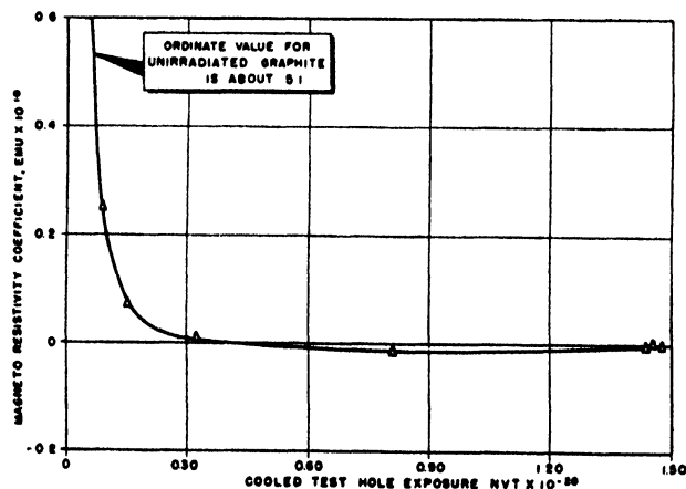
Figure 26. Magneto-resistivity coefficients of KC graphite
