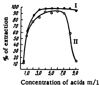
Figure 6. Effect of the concentration and nature of the acid on the extraction of the diethyldithiocarbamate compound of technetium by chloroform: (I) sulphuric acid medium, (II) hydrochloric acid medium
