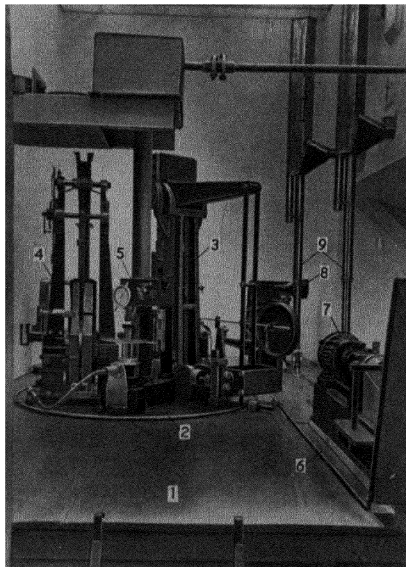
Figure 9. General view of mechanical test cell: (1) stainless steel working platform; (2) revolving stand with equipment on it; (3) combined testing machine (up to 5 tons); (4) 10 kg pendulum impact testing machine; (5) "Rockwell" hardness tester; (6-7) one of the lateral trolleys with a fatigue machine; (8) trolley with the remote microhardness tester; (9) manipulators
