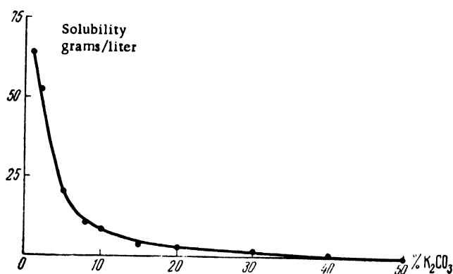
Figure 1. The solubility of potassium uranyltricarbonate in solutions of K_2CO_3 at 22°–23°C
