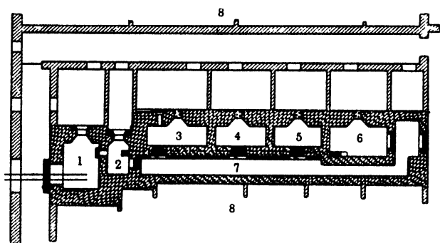
Figure 1. Layout of cells of metal-research "hot laboratory"; (I) cell of "hot" machine shop, (II) distribution cell and storage, (III) metallographic cell, (IV)-(V) physical measurements cell, (VI) mechanical tests cell, (VII) transportation corridor, (VIII) "semi-hot" laboratories
