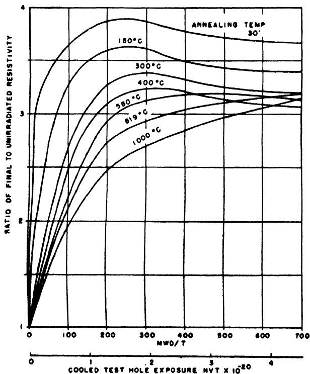
Figure 39. Annealing electrical resistivity: transverse cut CSF graphite
