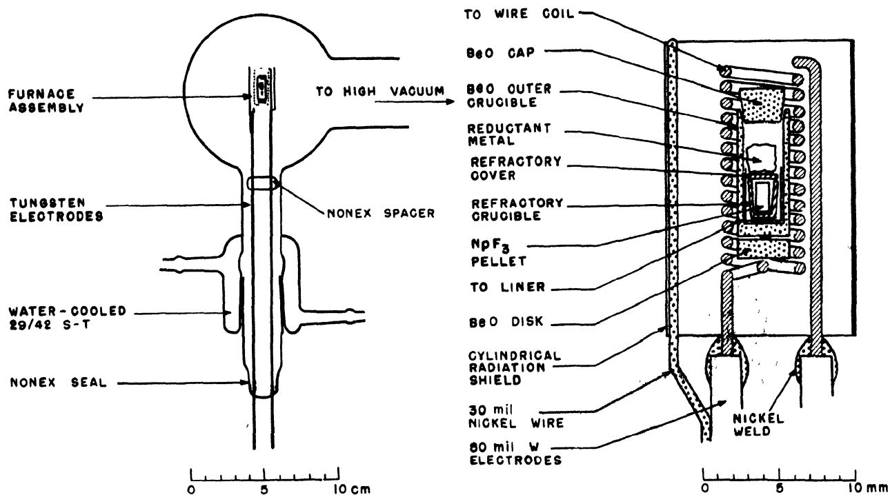
Figure 3. Furnace assembly
