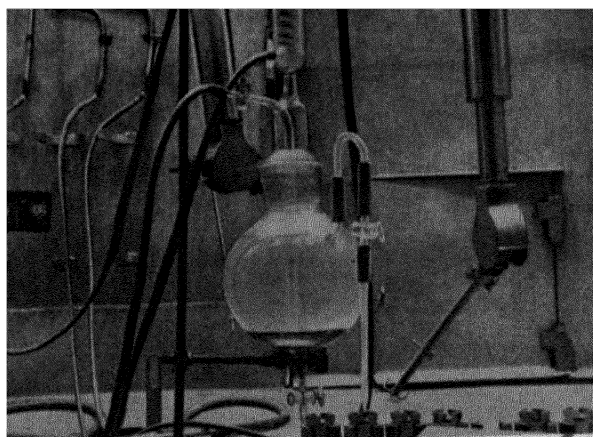
Figure 11. Extractor in the hot cell
