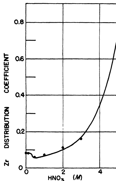
Figure 12. Effect of nitric acid concentration on extraction of zirconium by 15% tributyl phosphate in Varsol
