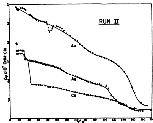
Figure 7. The decrease of bombardment-induced resistivity of copper, silver and gold as the specimens are warmed slowly from liquid helium temperatures (After Cooper). The decrease is irreversible. Sharp drops are found in silver and copper near 30°K and 40°K, respectively. The experiments indicate that no drop occurs in these two materials at lower temperatures. Gold does not appear to show a similar abrupt drop; however, there is reason to believe that the gold specimen was not in as good thermal contact with the cryostat as the other specimens.
