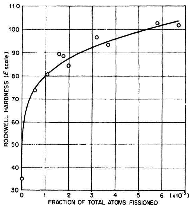
Figure 3. Effect of fission in aluminum-uranium alloys upon hardness
