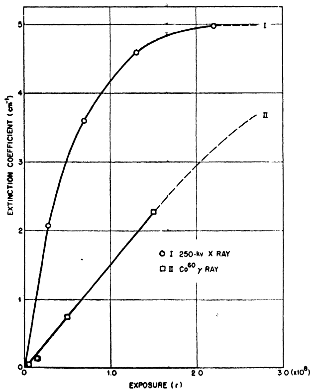
Figure 15. Absorption at 2150 Å in irradiated Corning silica glass
