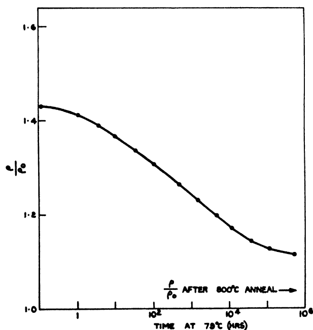
Figure 3. Recovery of resistivity changes: composite curve from data at temperatures up to 200°C; constant activation energy of 1.2 ev
