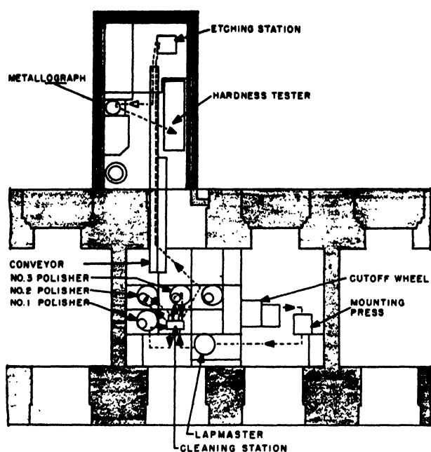
Figure 21. Schematic of metallographic processes
