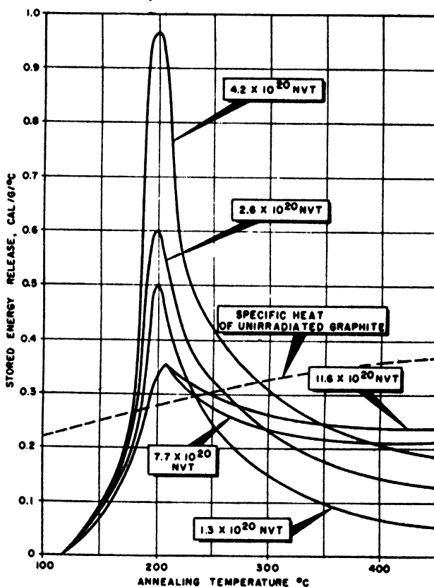
Figure 30. Stored energy annealing spectra in irradiated graphite
