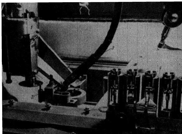
Figure 7. Cutting cell interior with milling machine: (1) head of the machine and mill; (2) cut-off rest of the machine with sample; (3) flexible shaft to the mechanism for clamping the samples; (4) instruments for manipulator
