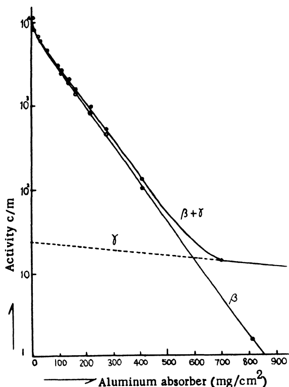
Figure 5. Aluminum absorption curve of Te fraction
