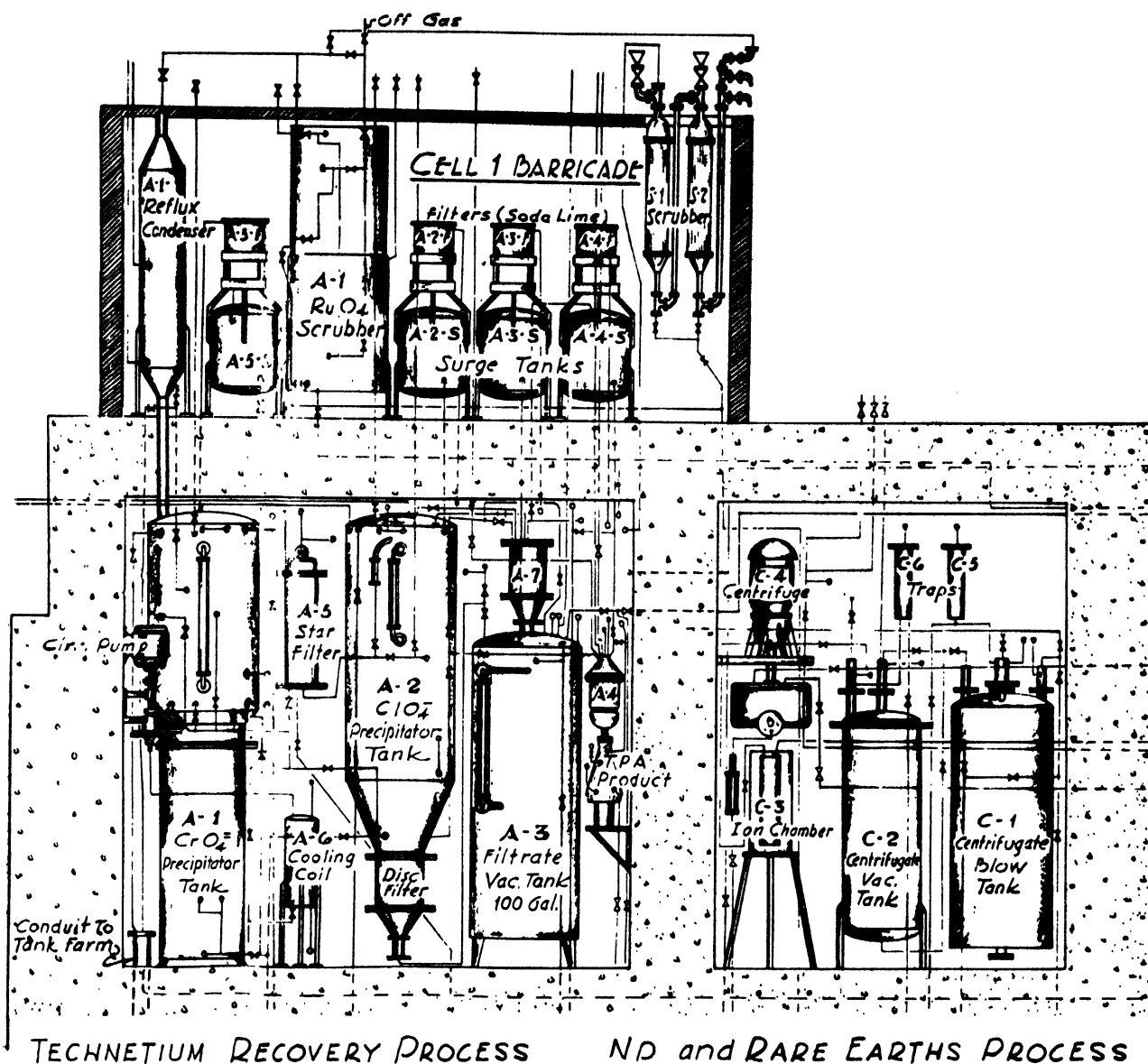
Figure 14. Typical radiochemical pilot plant scale equipment
