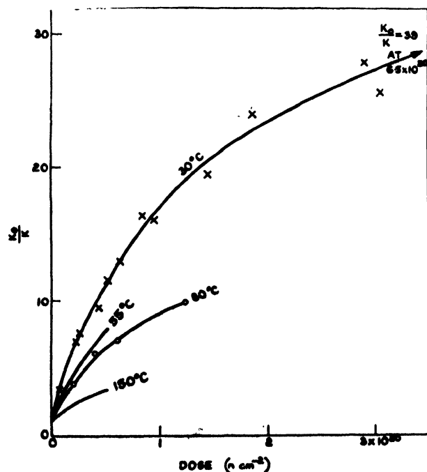
Figure 4. Changes of thermal resistivity at different irradiation temperatures
