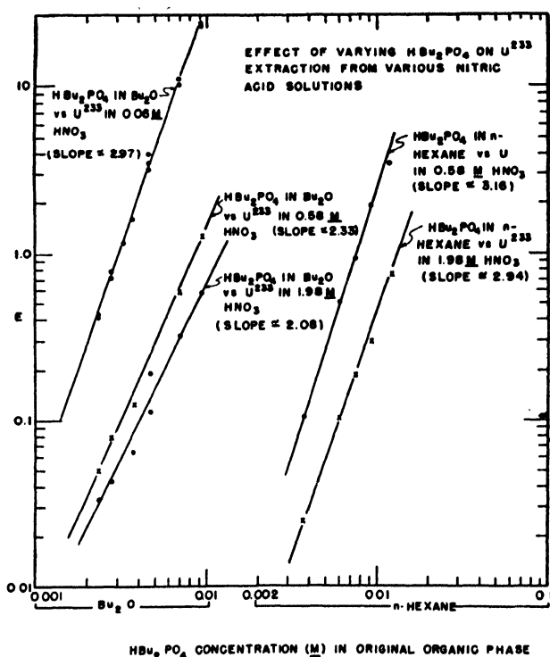
Figure 4. Extraction of uranium into a dilute solution of dibutyl phosphate in butyl ether or n-hexane. Effect of nitric acid concentration and of concentration of dibutylphosphate is shown. (Stewart, D. C. and Hicks, T. E., University of California Radiation Laboratory Report UCRL-861, August 1950)
