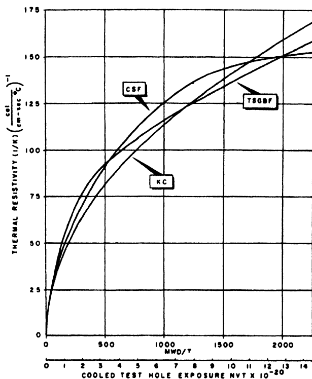
Figure 5. Radiation damage to thermal conductivity of transverse cut graphites
