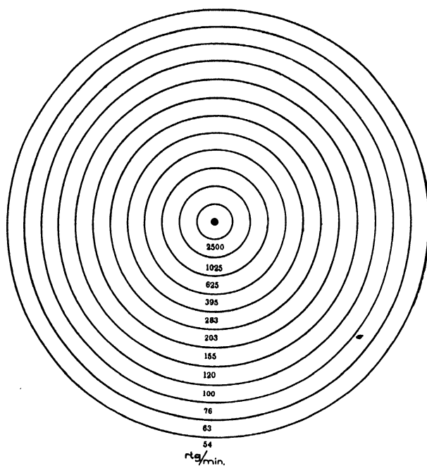
Figure 4. Iso-intensity circles ( r/\text{min} ) for a linear 100 curie source of \text{Co}^{60} , 20 cm high, immersed in methyl methacrylate. The values correspond to an average for variations with height of the point considered
