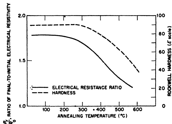
Figure 4. Annealing of radiation-produced changes of aluminum-uranium alloys
