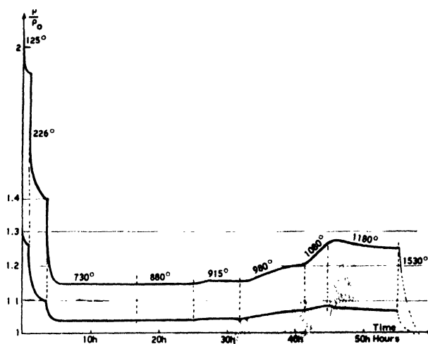
Figure 3. Curve A: sample irradiated with flux of 6 \times 10^{18} n/cm 2 in central channel. Curve B: sample irradiated with flux of 3-4 \times 10^{19} n/cm 2 in vertical converter
