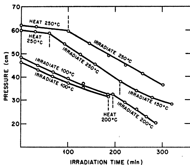
Figure 5. Changes in pressure of hydrogen and oxygen over water irradiated with cobalt gamma rays at high temperatures. Dose rate 1.4 \times 10^{17} \text{ev}\cdot\text{gm}^{-1}\cdot\text{min}^{-1}
