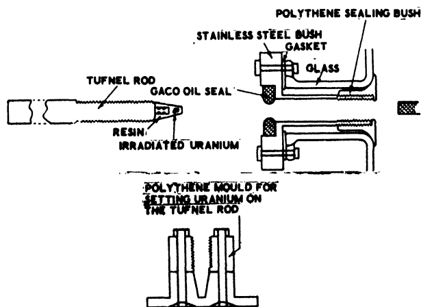
Figure 2. Details of grinding bush and mould
