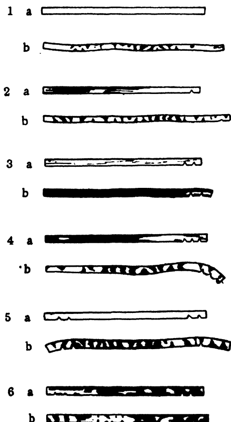
Figure 12. The appearance of foil strips of uranium alloy containing 0.61% molybdenum before (a) and after (b) irradiation: (1) cold-rolled; (2) annealed at 120°; (3) at 215°; (4) at 300°; (5) 412°; (6) 500°
