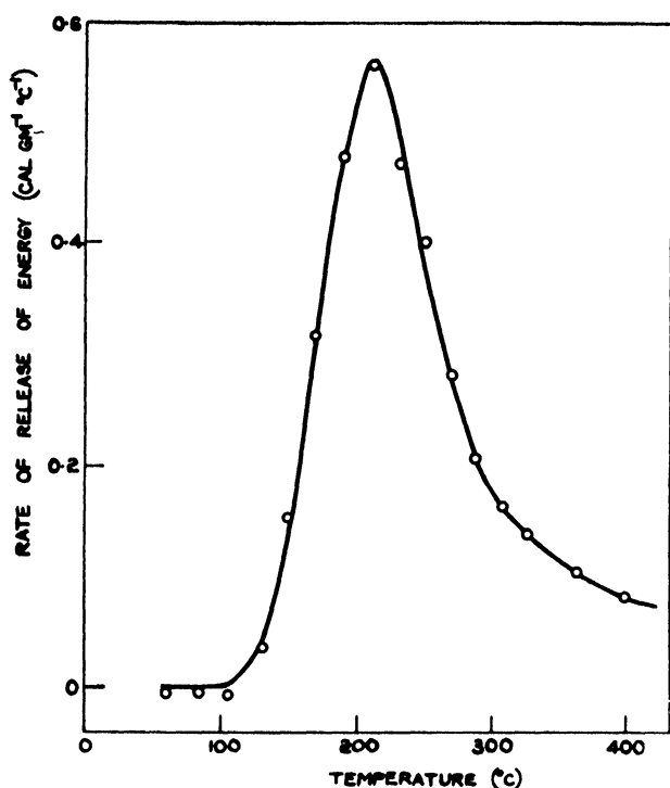
Figure 9. Rate of release of energy: linear rise of temperature ( 20^{\circ}\text{C min}^{-1} ); irradiation \sim 2 \times 10^{20} at 50^{\circ}\text{C}
