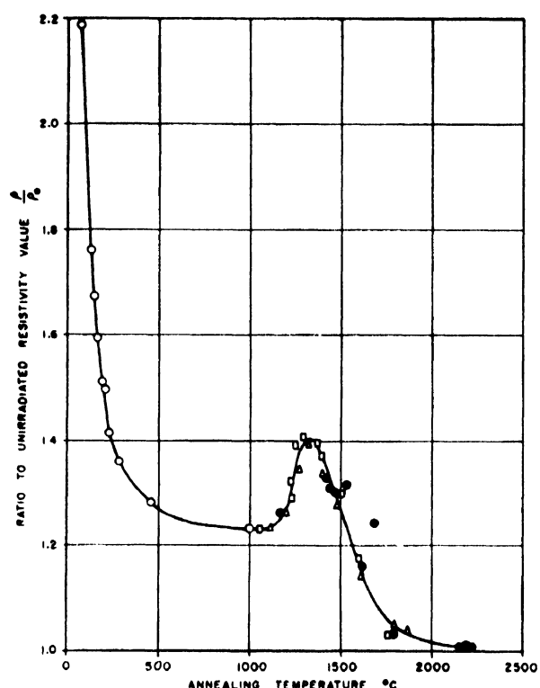
Figure 40. High temperature annealing effects on electrical resistivity: exposure 9.61 \times 10^{18} nvt
