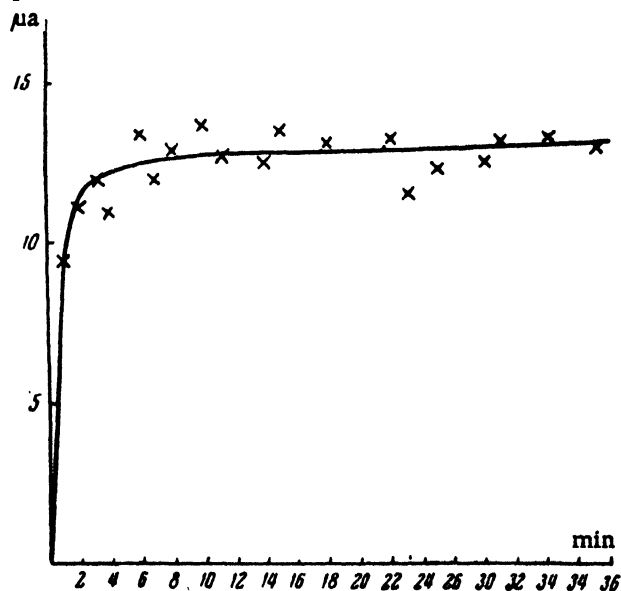
Figure 4. Dependence of the strength of the polarizing current on the time of gamma radiation action, when the constant potential of the electrode is V = 0.4 \text{ V}
