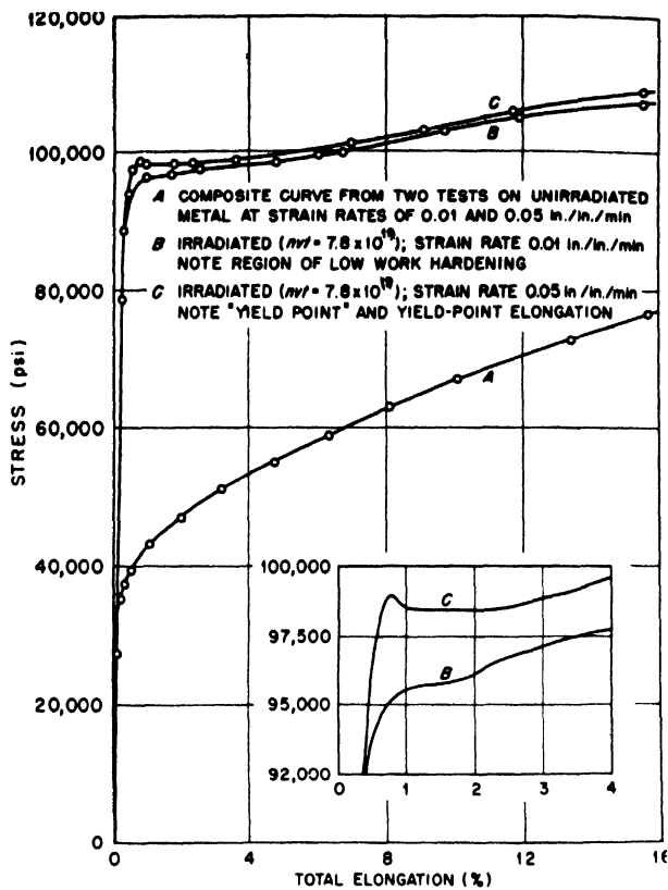
Slide 6. Conventional tension stress-strain curves for annealed austenitic stainless steel type 347
