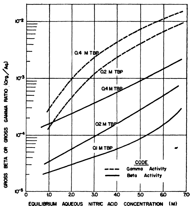
Figure 11. Distribution of fission product activity between aqueous nitric acid and diluted tributyl phosphate systems: 60% U saturation
