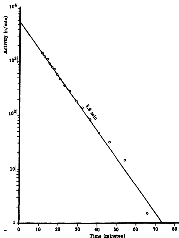
Figure 5. Disintegration curve of Fe obtained by (n,\alpha) reaction and measured in a scintillation counter
