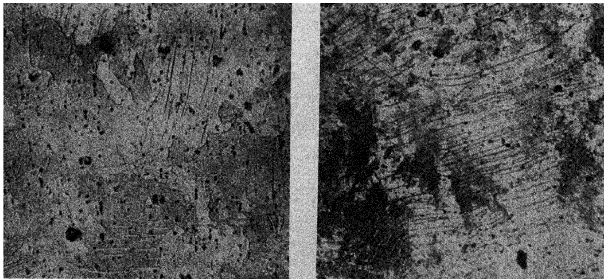
Figure 2. (a) Uranium microstructure before irradiation, obtained from a replica ( \times 240 ); (b) uranium microstructure after irradiation, obtained from a replica ( \times 240 )
