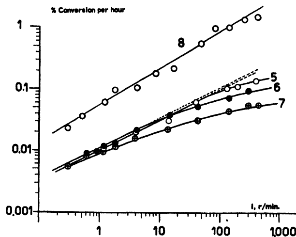
Figure 3. Rate of polymerization of styrolene in solution as a function of \gamma -ray intensity: curve 5, 40% styrolene (in moles) in toluene; curve 6, 20% styrolene (in moles) in toluene; curve 7, 10% styrolene (in moles) in toluene; curve 8, 10% styrolene (in moles) in propanol
