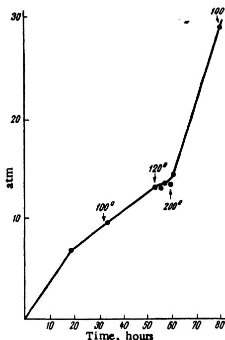
Figure 11. Radiolysis of 0.1 M solution of uranyl sulfate in the experimental hole (outside the converter).
