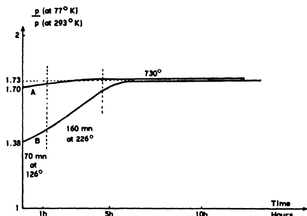
Figure 4. Curve A: sample irradiated with flux of 6 \times 10^{18} n/cm 2 in central channel. Curve B: sample irradiated with flux of 3-4 \times 10^{19} n/cm 2 in vertical converter
