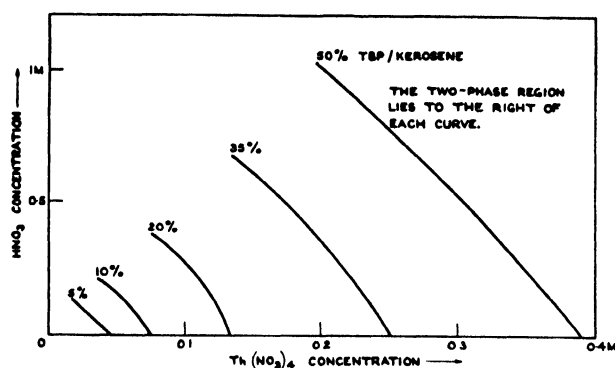
Figure 5. Limits of solubility of \text{Th}(\text{NO}_3)_4 in TBP/kerosene
