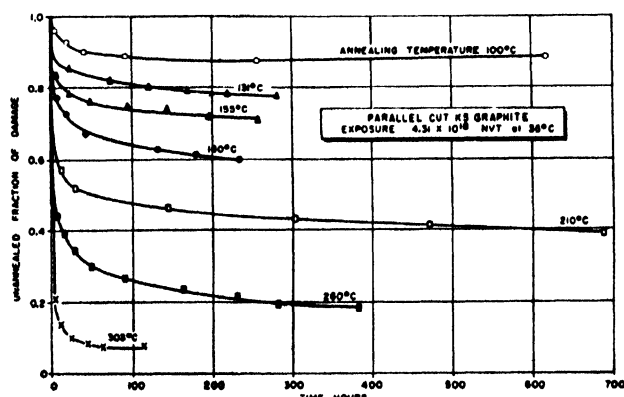
Figure 33. Isothermal annealing of Young's modulus changes
