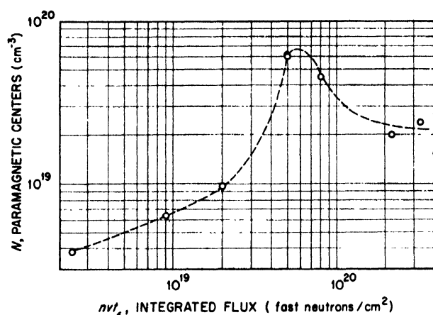
Figure 12. Bombardment introduced paramagnetic centers in quartz vs irradiation
