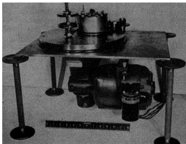
Figure 24. Remotely operated polishing wheel
