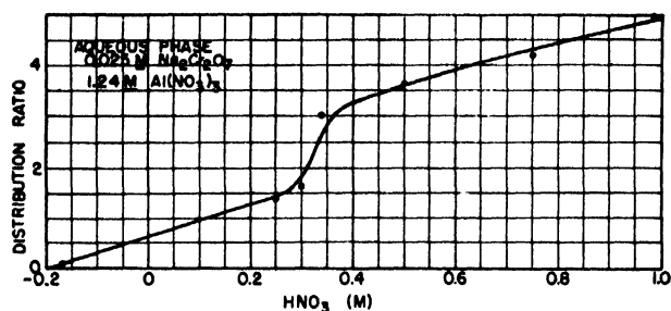
Figure 7. Effect of nitric acid concentration on the methylisobutyl ketone extraction of cerium
