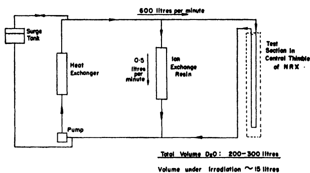
Figure 2. Loop circuit
