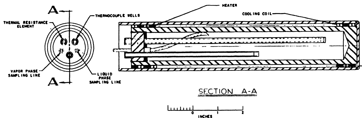
Figure 1. Cutaway of autoclave
