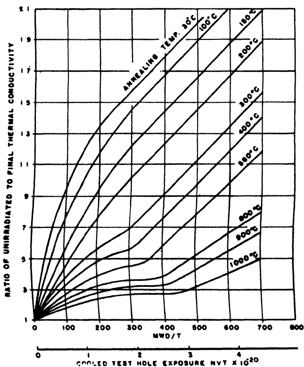
Figure 38. Annealing isotherms for transverse cut CSF graphite
