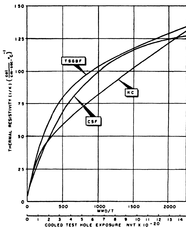
Figure 4. Radiation damage to thermal conductivity of parallel cut graphites
