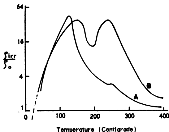
Figure 1. Ratio of electrical resistivities of irradiated and normal NaCl as a function of temperature rising at the rate of 2^\circ\text{C} per minute. Total flux of 350 Mev protons 5.3 \times 10^{13} (curve A) and 9 \times 10^{15} (curve B) per \text{cm}^2
