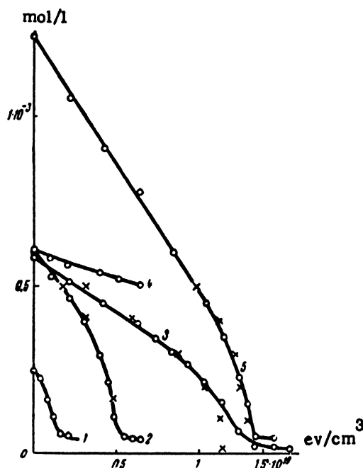
Figure 20. Dependence of concentration of H 2 O 2 on the dose: (1, 2 and 5) concentration of H 2 = 0.84 \times 10^{-3} M; (3) 0.42 \times 10^{-3} M; (4) solution saturated with air. Circles designate experimental results, crosses designate calculated results
