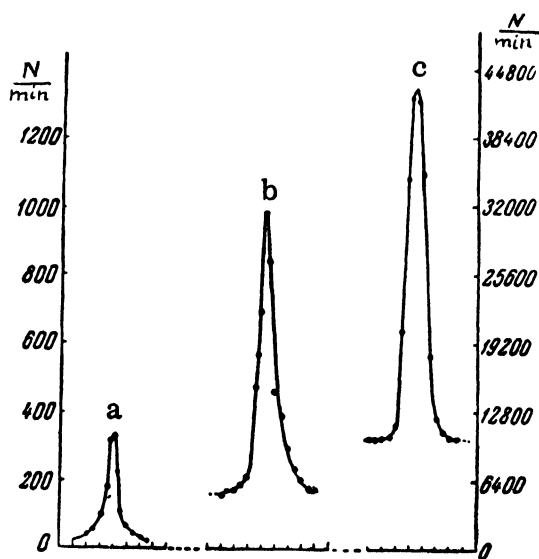
Figure 11. Roentgenogram of line (III) aluminium
