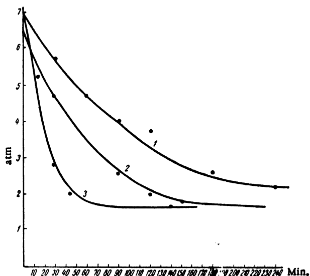
Figure 12. Recombination of explosive mixture during irradiation of ampoules with solutions of uranyl fluoride wrapped in cadmium foil: (curve 1) 1 M uranyl fluoride; (2) 0.01 M uranyl fluoride; (3) water
