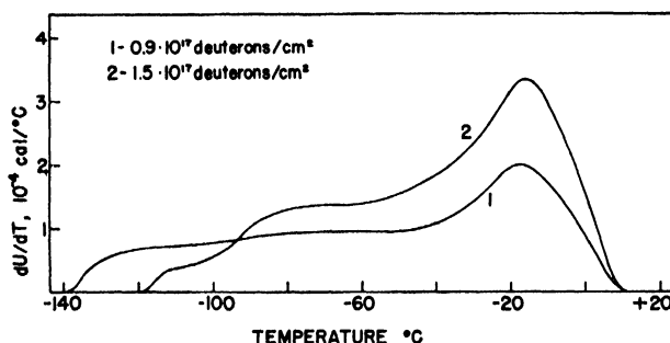
Figure 10. Stored energy release during the annealing of two irradiated specimens of copper. (after Overhauser)
