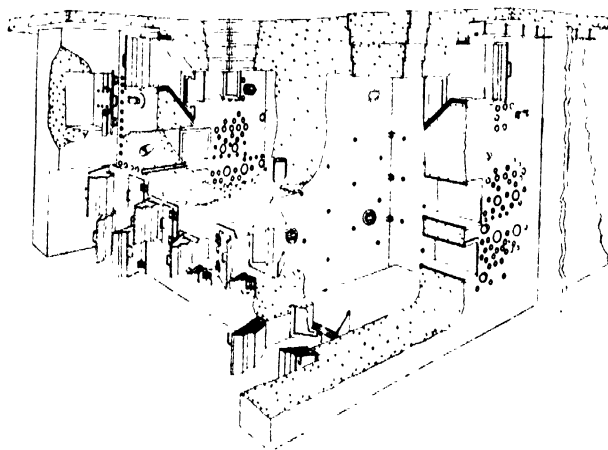
Figure 7. Perspective of typical radiochemical hot cells
