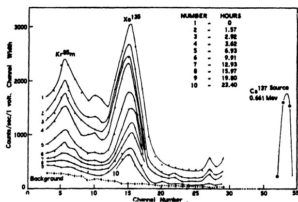
Figure 4. \gamma -spectrum on multi-channel pulse analyser
