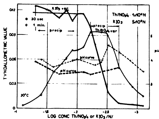
Figure 5. Typical precipitation curves (30 sec and 1 min tyndallograms and pH curves) for the systems: (1) (thick lines) 1 \times 10^{-2} N thorium nitrate and 5 \times 10^{-2} – 8 \times 10^{-4} N potassium iodate; (2) (thin lines) 5 \times 10^{-3} N potassium iodate and 8 \times 10^{-2} – 8 \times 10^{-4} N thorium nitrate
