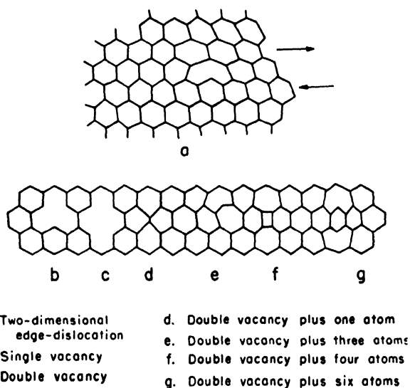
Figure 2. Probable configurations of 2-dimensional dislocations
