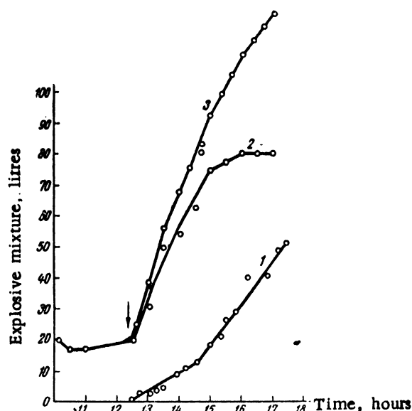
Figure 4. Accumulation of explosive mixture in liquid and gas at 105 kw: (curve 1) accumulation in gas; (2) in liquid; (3) total accumulation
