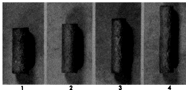
Figure 6. Effect of 0.1% atom burnup on 600°C rolled and beta quenched uranium after further cold work at 300°C: (1) no cold work; (2) 5% red. at 300°C; (3) 10% red. at 300°C; (4) 25% red. at 300°C
