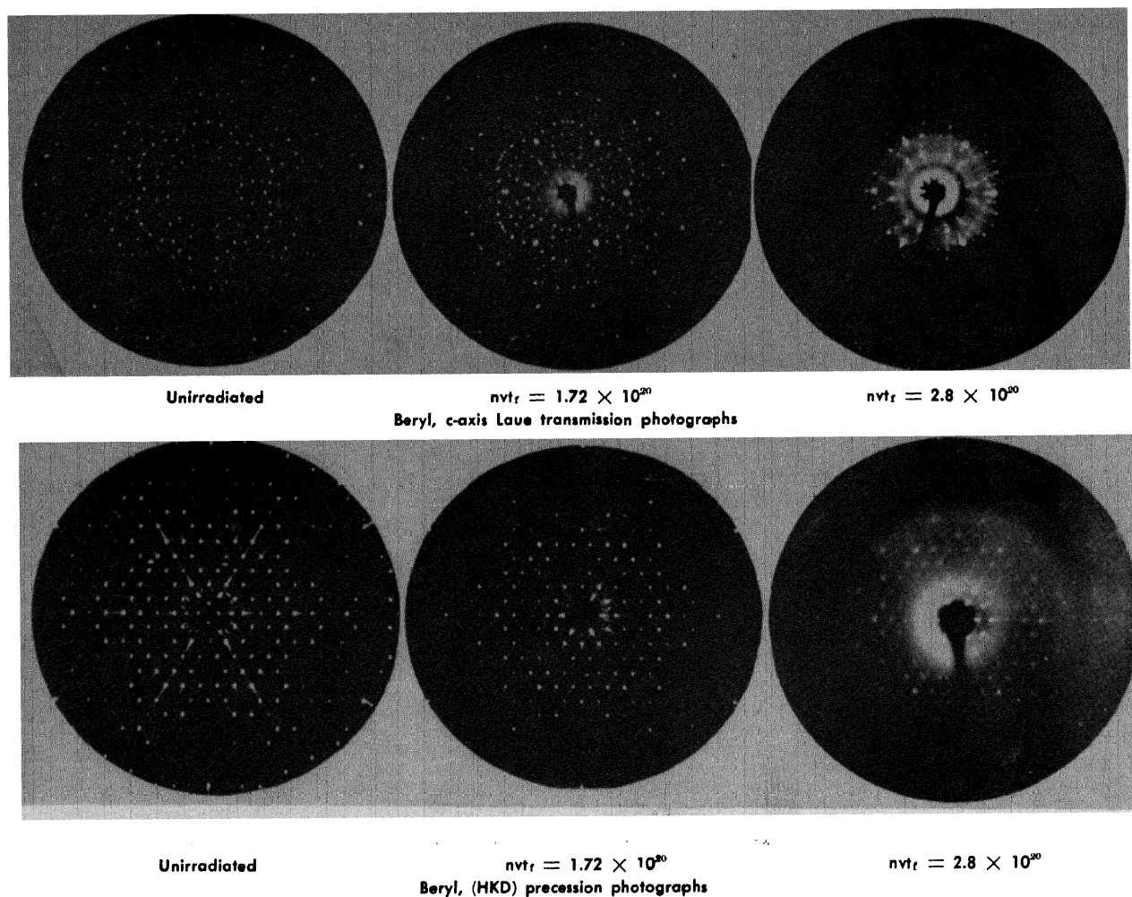
Figure 5. Transmission patterns of fast neutron bombarded beryl
