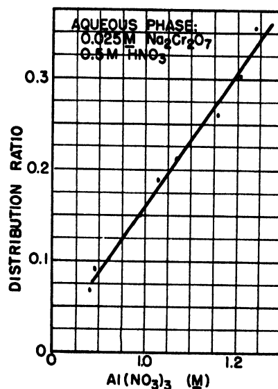
Figure 6. Effect of aluminum nitrate concentration on extraction of cerium by methylisobutyl ketone containing 0.3 M \text{HNO}_3
