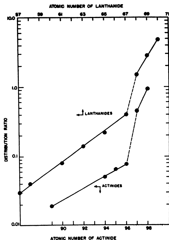
Figure 12. Solvent extraction behavior of trivalent lanthanide and actinide elements into tributyl phosphate from 12.0 N HCl
