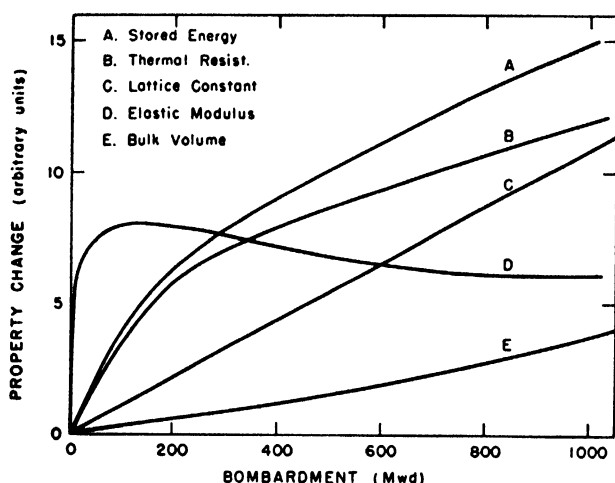
Figure 3. Property changes during bombardment at room temperature
