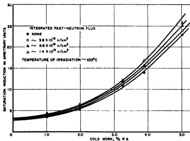
Figure 6. The effect of reactor irradiation on the saturation value of the magnetic induction of type 347 stainless steel
