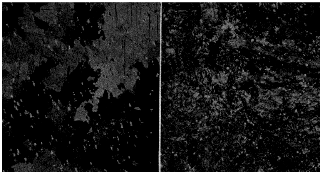
Figure 12. Effect of irradiation on the metallographic structure of uranium, (100 diameters, polarized light): (left) beta quenched uranium before irradiation; (right) beta quenched uranium after irradiation
