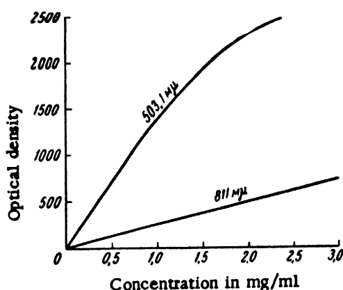
Figure 3. Applicability of Beer's law to 503.1 m\mu and 811 m\mu peaks: cell thickness, 1.0046 cm
