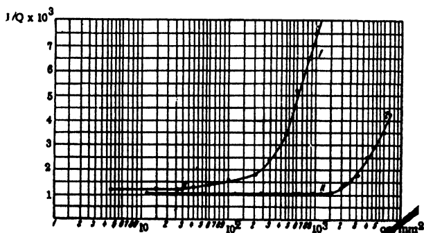
Figure 14. Curve of internal friction versus tension caused by amplitude of vibration before (1) and after (2) irradiation
