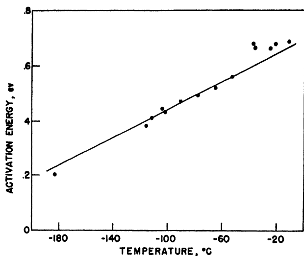
Figure 8. Plot of the principal activation energy effective in the annealing of copper, bombarded at liquid nitrogen temperature, as a function of the annealing temperature (after Overhauser). The value near 0.69 eV appears prominently above -60^{\circ}\text{C}
