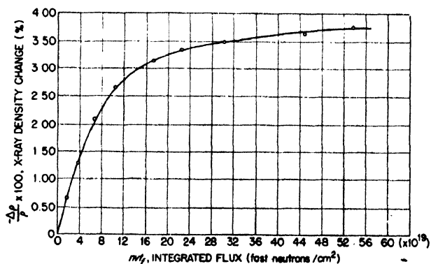
Figure 6. Effect of neutron irradiation on the density of diamond
