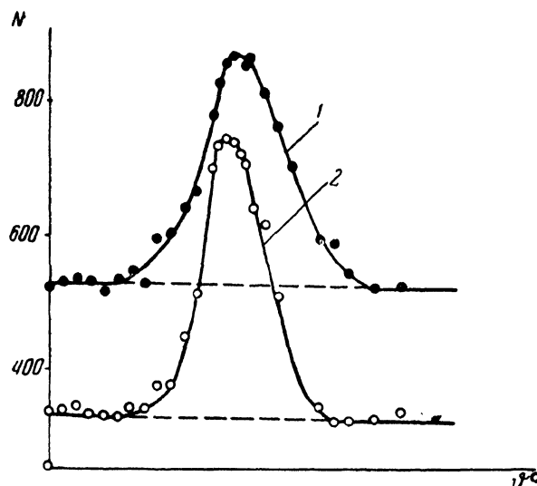
Figure 13. Lines (114) of a uranium X-ray diffraction pattern: (1) before irradiation; (2) after irradiation
