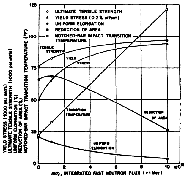
Slide 5. Integrated fast-neutron flux dependence of several mechanical properties of A-212B carbon-silicon steel
