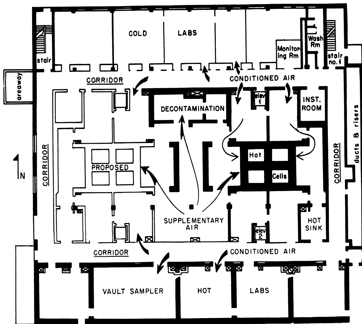
Figure 5. Floor plan of a radiochemical laboratory building with radiation zoning and air flow planning
