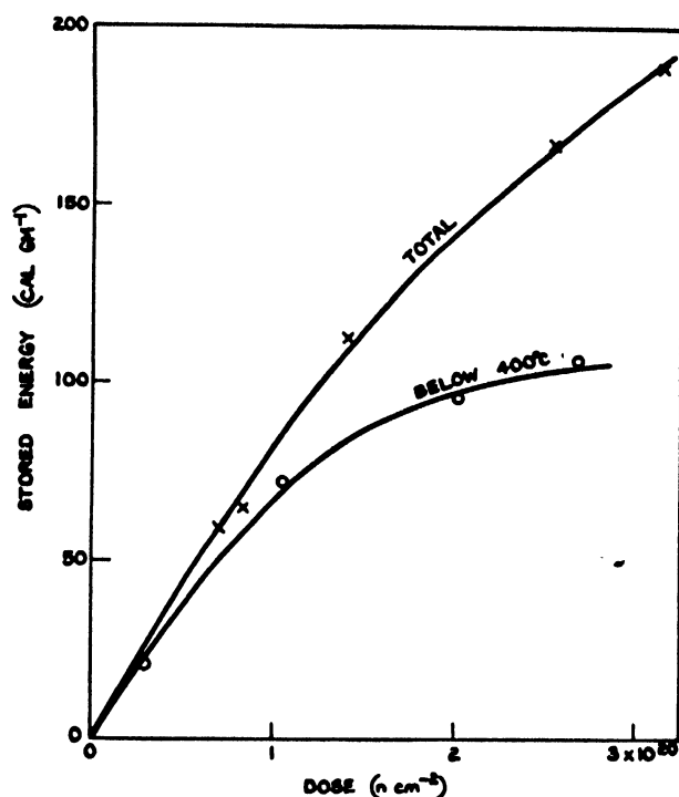
Figure 8. Total stored energy and energy released below about 400°C: irradiation temperature 30°C
