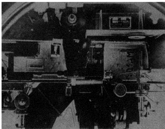
Slide 33. The machine for testing irradiated specimens for fatigue
