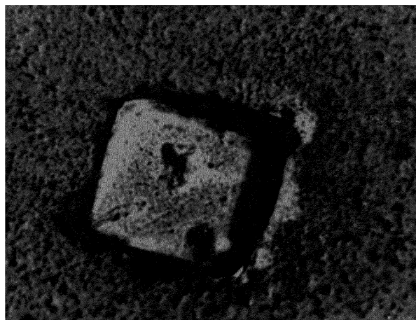
Figure 5. Uranium carbide grain before irradiation ( \times 4500 )
