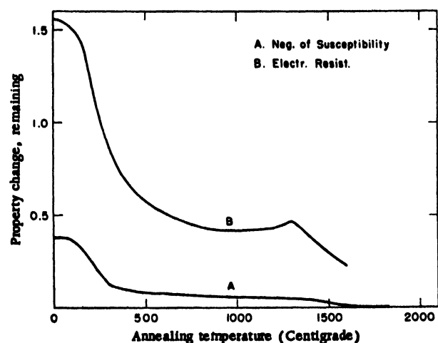
Figure 6. Annealing of electrical properties above room temperature
