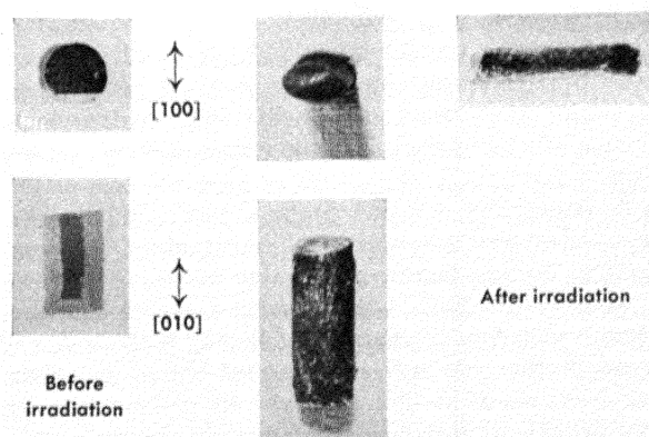
Figure 1. Aspects of a cylindrical single crystal of alpha uranium before and after irradiation in a reactor (0.1% atom burn-up)
