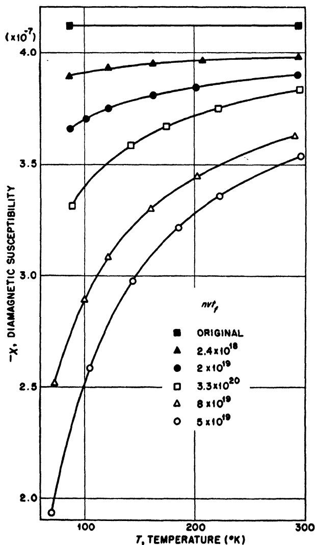
Figure 10. Diamagnetic susceptibility of irradiated quartz
