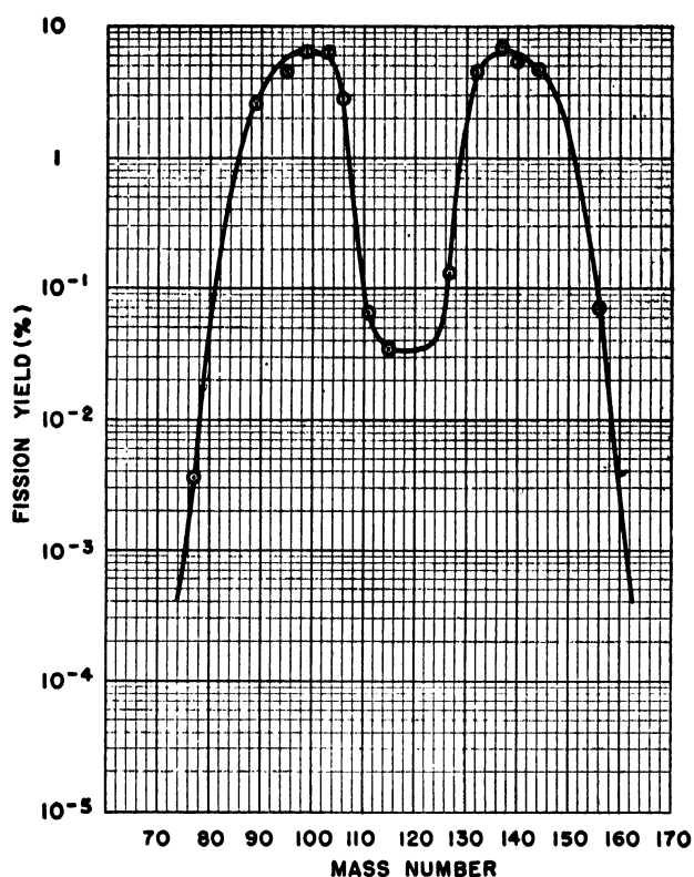
Figure 2. Yield-mass curve for fast neutron-induced fission of U 238
