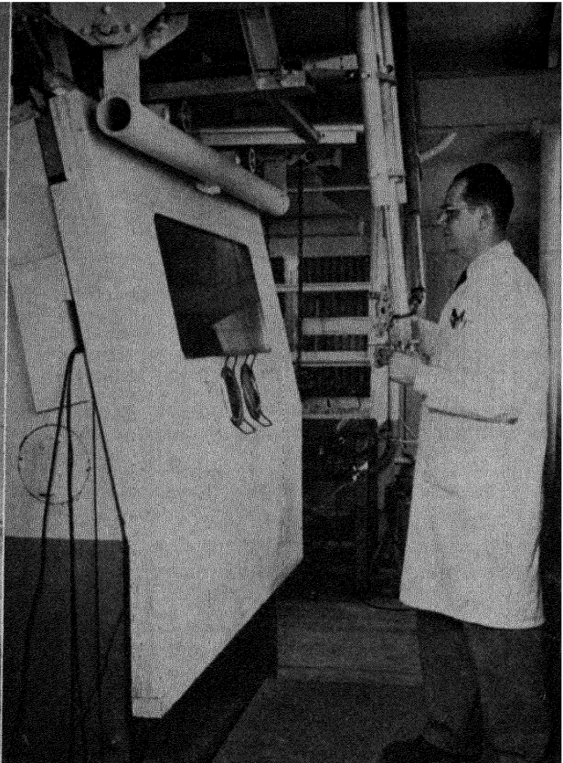
Figure 6. Operating manipulators of a junior cave
