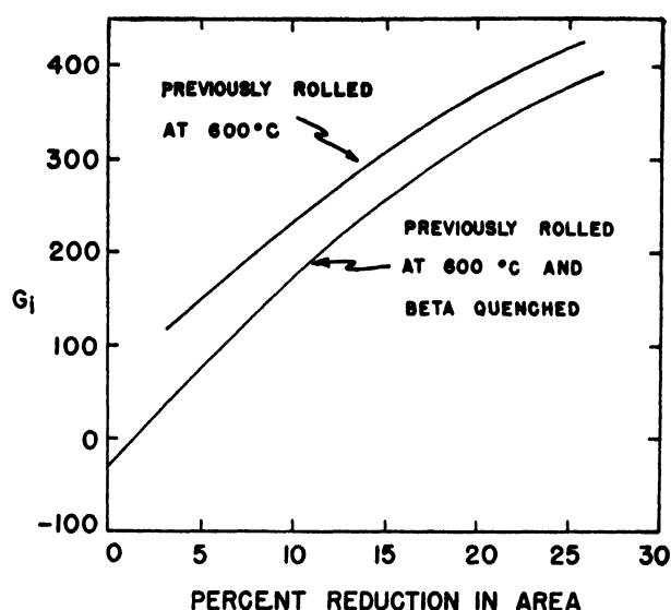
Figure 5. Effect of additional cold work (at 300°C) on the irradiation growth rate of uranium (previously rolled at 600°C)
