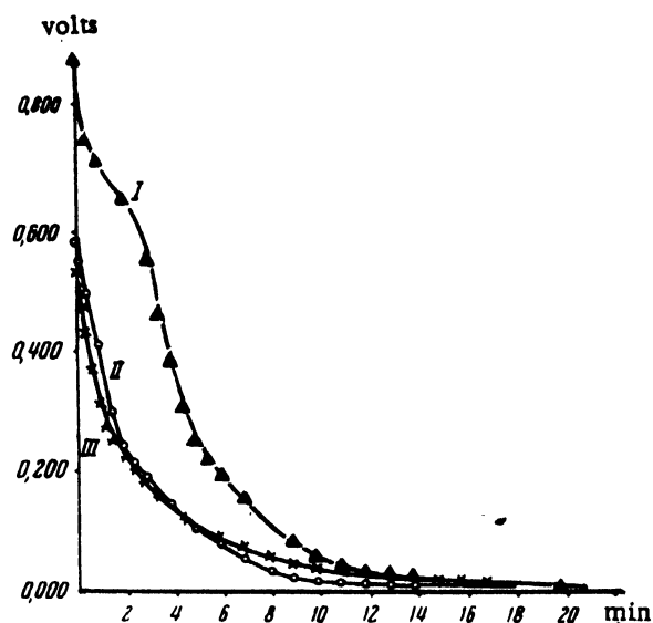
Figure 1. Dependence of Pt electrode potential on the time of gamma radiation action (curves I and II) and on the time of charging the electrode with 10 \mu\text{A} current (curve III)
