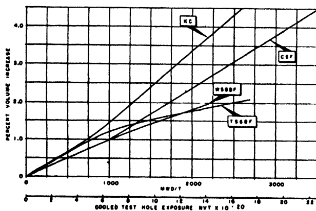
Figure 21. Volume expansion of graphite with irradiation
