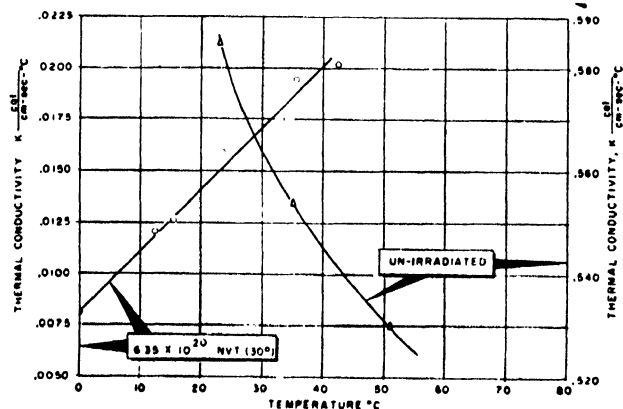
Figure 7. Variation of thermal conductivity with temperature parallel cut KC
