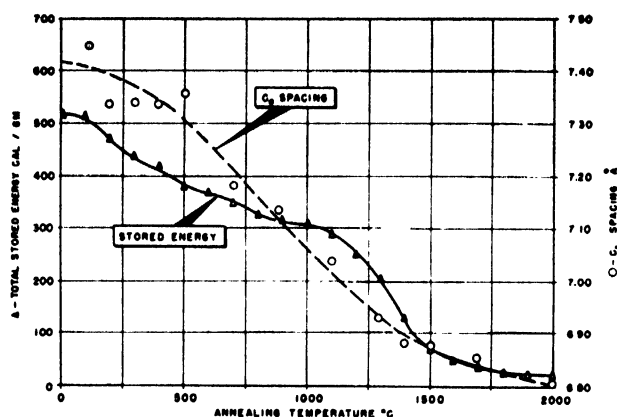
Figure 29. Annealing of total stored energy
