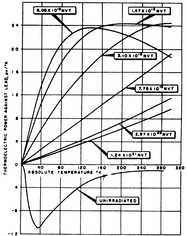
Figure 24. Thermoelectric power of parallel cut KC graphite irradiations at 30°C
