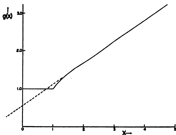
Figure 3. The number of atoms displaced per primary, g(x) , as a function of the energy of the primary in units of E_d . The dotted line represents the extrapolation of the essentially linear portion of the curve above x = 3 to negative values of x . (See text)
