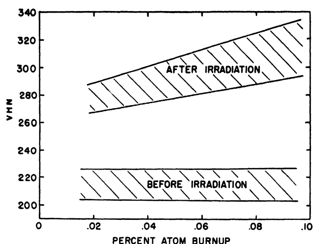
Figure 13. Change in Vickers hardness of uranium as a function of burnup (recrystallized before irradiation)
