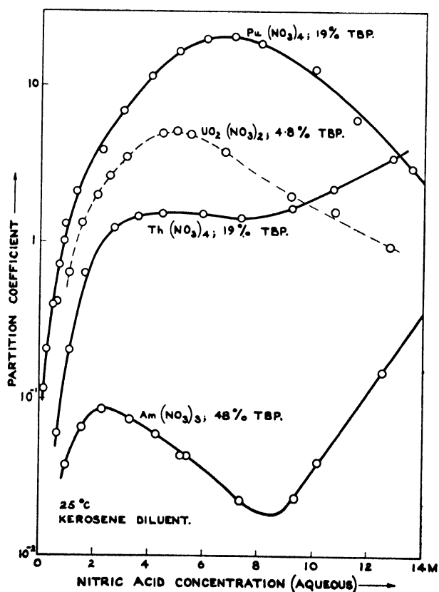
Figure 2. 25°C kerosene diluent
