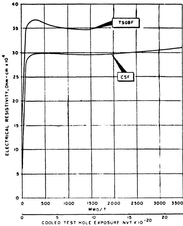
Figure 8. Radiation damage to electrical resistivity of parallel cut graphite
