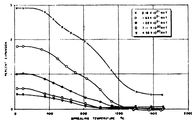
Figure 42. Annealing physical expansion: transverse cut CSF
