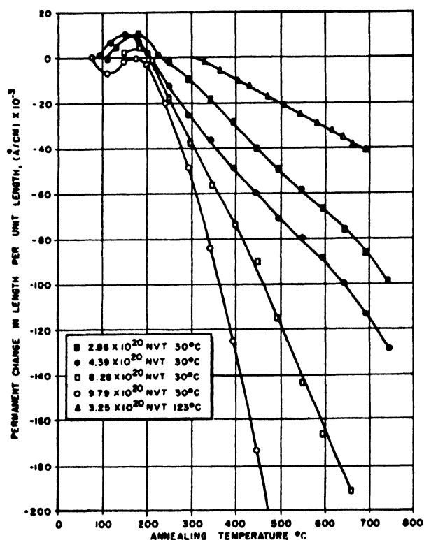
Figure 43. Physical expansion annealing: interferometer measurements
