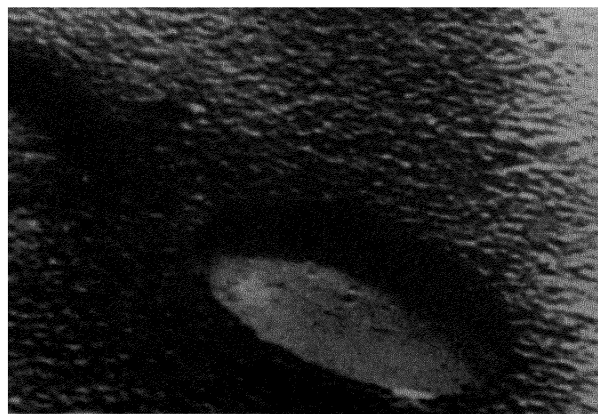
Figure 4a. Uranium microstructure before irradiation ( \times 15,000 )
