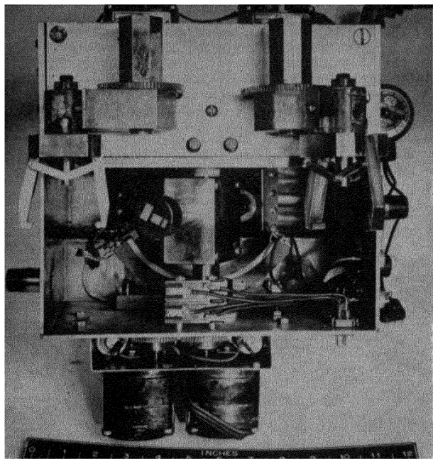
Figure 23. In-cell portion of ultrasonic specimen cleaner
