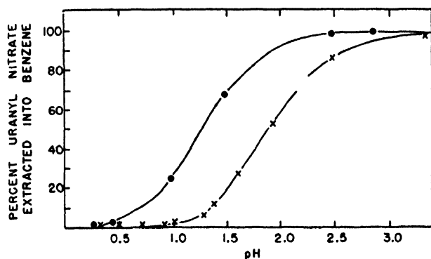
Figure 5. Extraction of trace amounts of uranyl nitrate by an equal volume of 0.2 M benzene solution of TTA from aqueous solutions of varying acidity: (x) dilute nitric acid; (o) dilute nitric acid plus 2.5 M Ca(NO 3 ) 2 .
