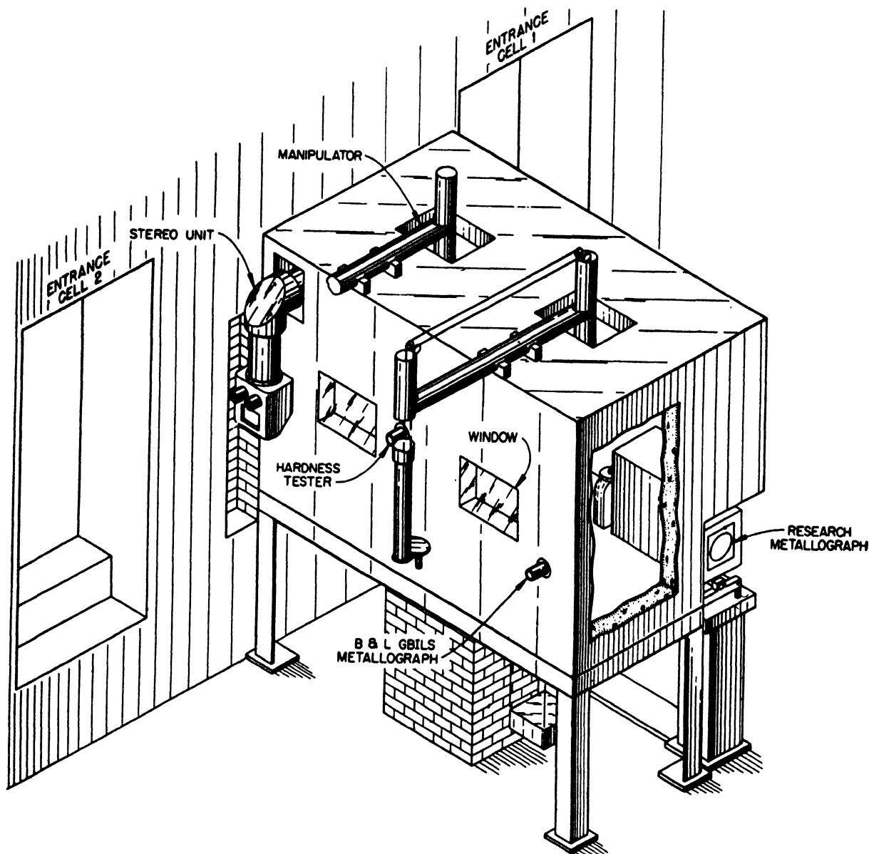
Figure 25. Schematic of cell 2A showing metallographic installation
