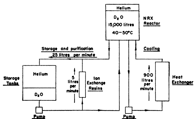
Figure 1. D_2O system in the NRX reactor
