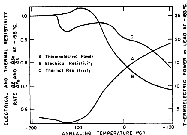
Figure 8. Annealing of electrical properties at low temperatures
