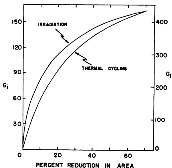
Figure 4. Effect of cold work upon the irradiation growth rate ( G_i ) and thermal cycling growth rate ( G_t ) of uranium: (specimens were recrystallized at 575°C before testing; G_i = micro-in./in./ppm° burn-up, G_t = micro-in./in./cycle)
