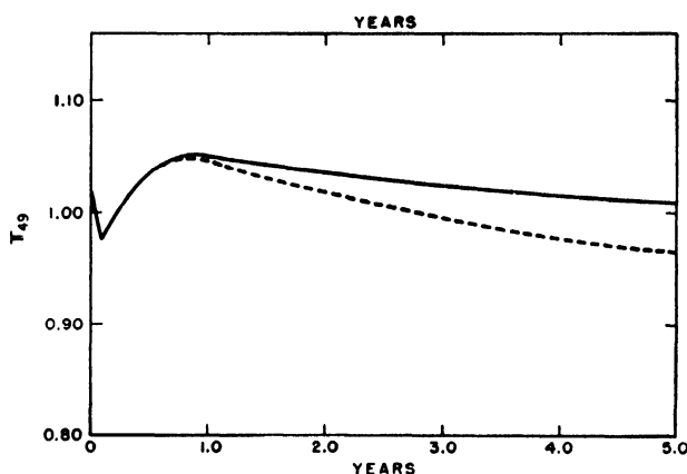
Figure 3b. Variation in \pi_{49} , the productivity, or breeding ratio for \text{Pu}^{239} , as a function of time (for definition of \pi_{49} , see text). \pi_{49} = 1 corresponds to the case where \text{Pu}^{239} is formed as rapidly from \text{U}^{238} as it is destroyed by neutron absorption, neglecting other sources of neutron loss (as neutron escape or parasitic absorption). The dashed curve includes the effect of \text{Am}^{243} , \text{Cm}^{244} , and \text{Cm}^{245} , while the solid curve represents only the plutonium isotopes
