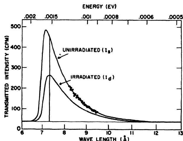
Figure 1. Slow neutron intensity transmitted by an irradiated and unirradiated graphite specimen. For clarity, only a typical group of experimental points had been reproduced along one curve to indicate their number and spread. Only intensities to the right of the vertical line at 7.30 Å were considered in computing I_s and I_d .
