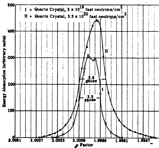
Figure 13. Paramagnetic resonance in irradiated piezo quartz
