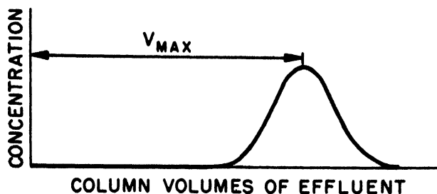
Slide 12. Column method: V_{max} = i + D_v , where i is fractional interstitial volume, D_v is volume distribution coefficient (amount per liter bed/amount per liter solution)
