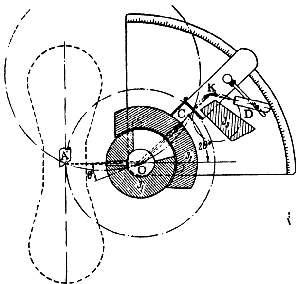
Figure 10. Drawing of instrument for X-ray analysis
