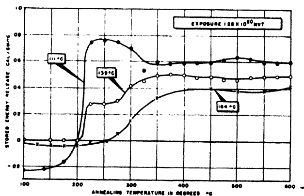
Figure 31. Effect of exposure temperature on stored energy
