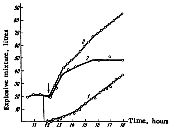
Figure 3. Accumulation of explosive mixture in liquid and gas at 50 kw: (curve 1) accumulation in gas; (2) in liquid; (3) total accumulation
