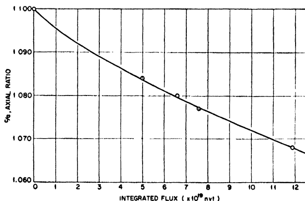
Figure 1. Change in axial ratio of quartz with fast neutron bombardment
