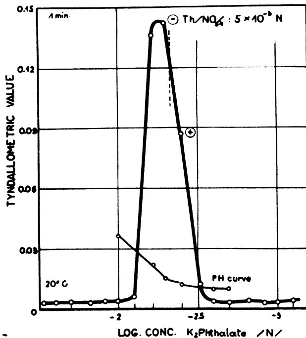
Figure 4. Typical precipitation curve (1 min tyndallogram and pH curve) for the systems: 5 \times 10^{-3} \text{ N} thorium nitrate and 3 \times 10^{-2} – 8 \times 10^{-4} \text{ N} potassium phthalate
