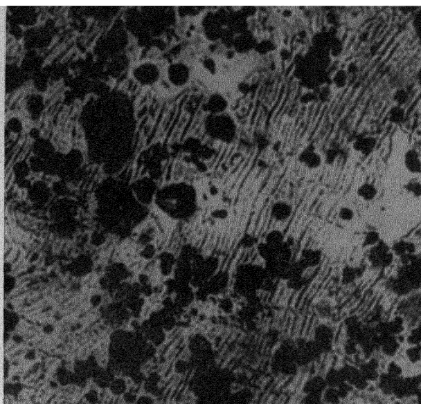
Figure 3b. Uranium microstructure after irradiation ( \times 200 )
