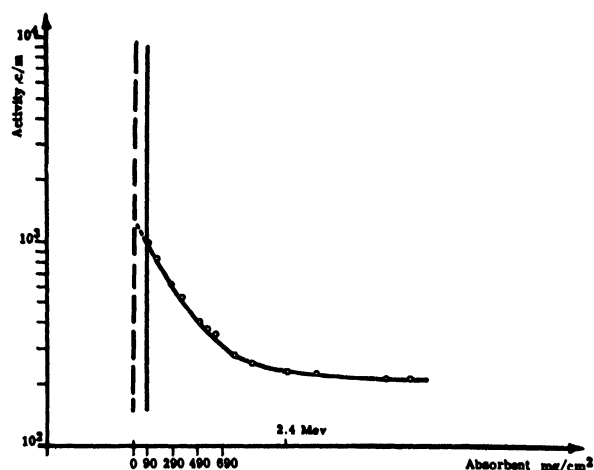
Figure 6. \text{Xe}^{138} absorption curve
