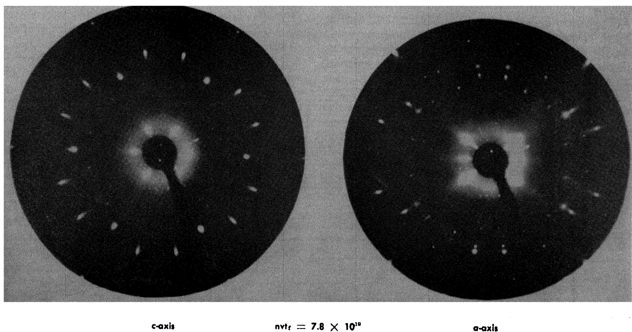
Figure 4. Irradiated quartz Laue transmission photographs
