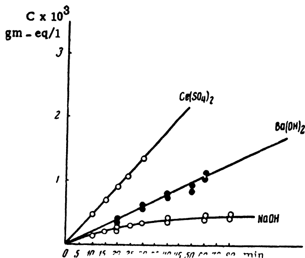
Figure 6. The kinetics of the precipitation of BaO \cdot 2H_2O_2 in Ba(OH)_2 solution of hydrogen peroxide formation in 0.3N NaOH solution and of Ce(SO_4)_2 reduction by an electron beam
