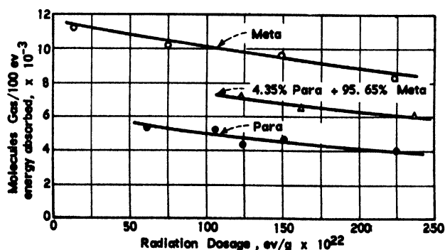
Figure 10. Improved radiation stability of terphenyl mixtures at 350°C
