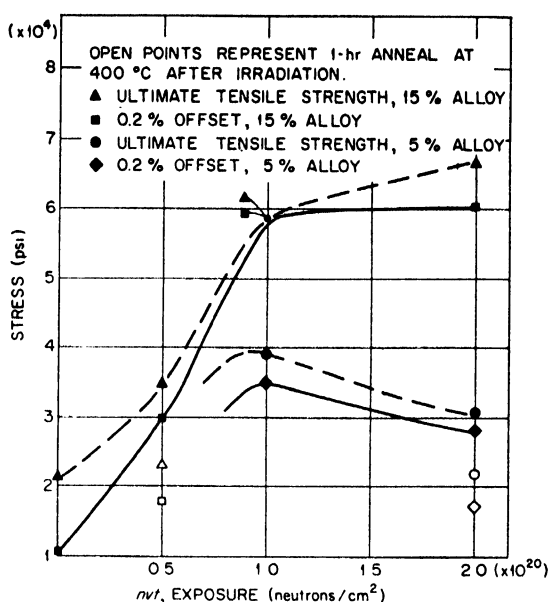
Figure 5. Effect of fission in aluminum-uranium alloys upon the tensile strength at 30°C
