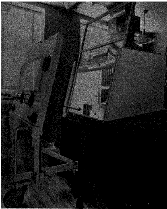
Figure 7. Shielded hood with ball joint manipulators
