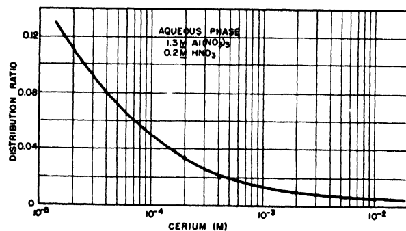
Figure 9. Effect of inert cerium on the scrubbing of tracer cerium from methylisobutyl ketone containing tracer cerium
