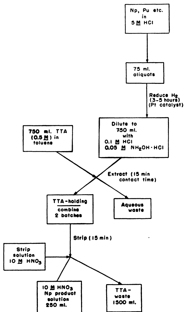
Figure 4. Cycle IV: flowsheet III
