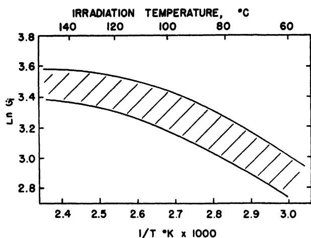
Figure 9. Effect of irradiation temperature on growth rate ( G_i ) of 300°C-rolled and beta quenched uranium
