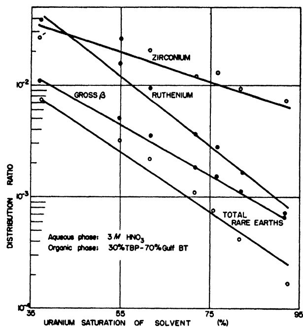
Figure 10. Effect of uranium saturation of tributyl phosphate on fission product extraction
