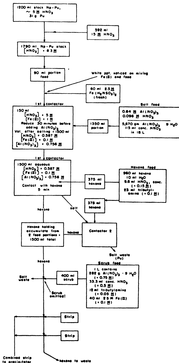
Figure 3. Cycle II: flowsheet II, Np-Pu separation
