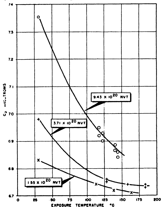
Figure 14. Variations in C_0 displacement of CSF graphite with exposure temperature
