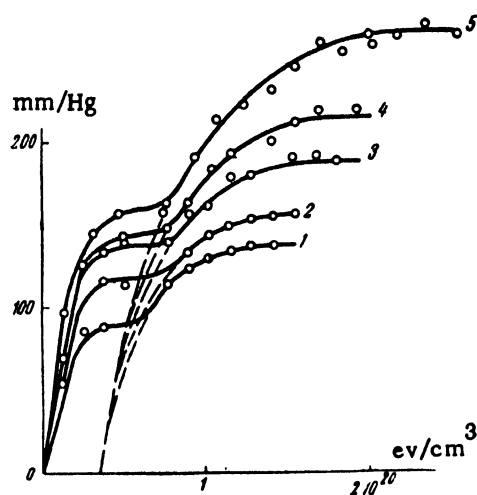
Figure 15. The dependence of the pressure of the evolved hydrogen upon the dose at concentrations of oxygen given in the preceding figure
