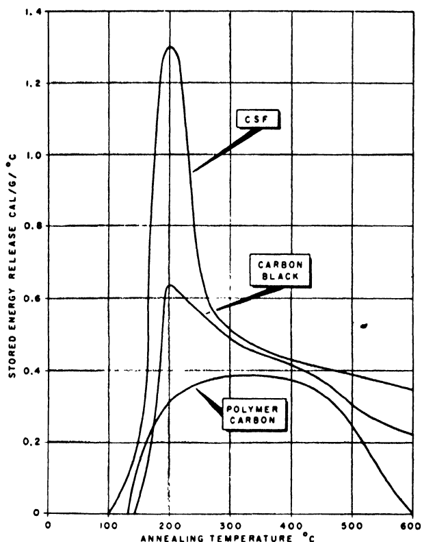
Figure 32. Stored energy in special carbons: exposure 3.42 \times 10^{20} nvt ( 30^{\circ} )
