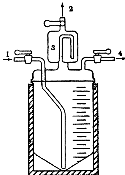
Figure 8. Diagram of dissolver: (1) inlet and outlet of solutions; (2) to ventilation; (3) trap; (4) to air-vacuum system
