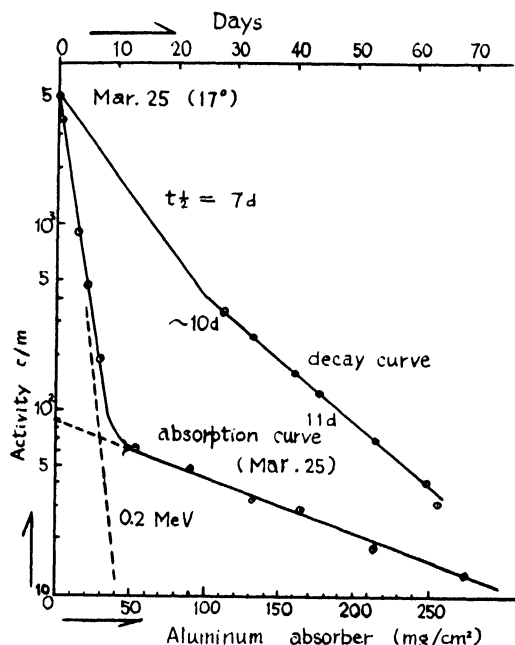
Figure 10. Decay curve and aluminum absorption curve of uranium fraction
