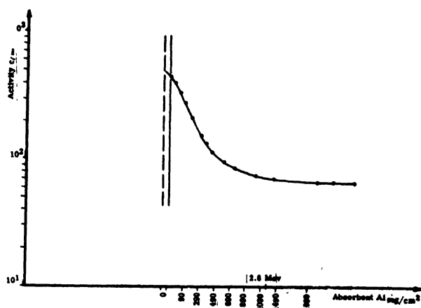
Figure 7. \text{Cs}^{138} absorption curve
