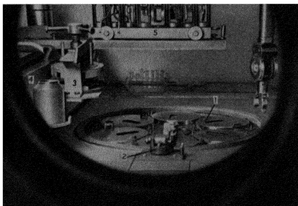
Figure 5. Inside view of metallographic cell. Grinding machine in foreground
