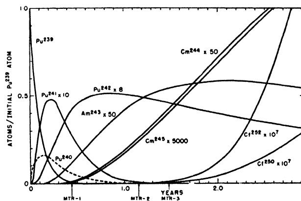
Figure 4. Production of heavier nuclides when \text{Pu}^{239} is irradiated at a flux of 3 \times 10^{14} neutrons/cm 2 for long time periods. The case treated represents one in which an individual \text{Pu}^{239} sample is placed in a reactor and the composition calculated for various alternative times of withdrawal. This case corresponds to that of the MTR bombardments, and the arrows indicate the approximate withdrawal times for the MTR samples described in Table 3. It may be noted that within the period shown, only the nuclides through \text{Am}^{243} have reached saturation. Further irradiation would increase the amounts of the higher nuclides
