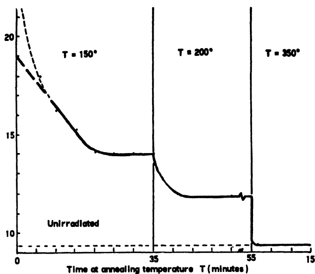
Figure 5. Diamond point hardness as a function of annealing time of KCl irradiated with 2 \mu\text{-hr} of 1 Mev electrons at 20^\circ\text{C}
