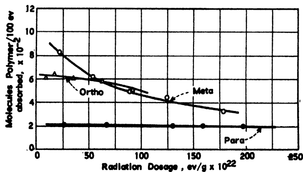
Figure 7. Relative radiation resistance of terphenyl isomers at 400°C
