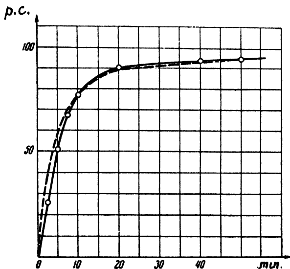
Figure 4. Dependence of deposited substance on electrolysis time
