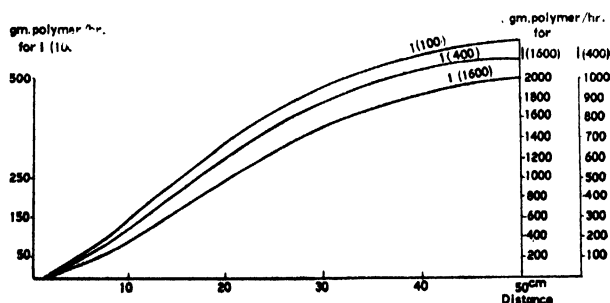
Figure 5. Hourly production in grams of polymethyl methacrylate as a function of the reactor radius, at 19^\circ\text{C} , for a linear source 20 cm high, placed on the axis of a cylindrical reactor. The curves have reference to sources of 100, 400 and 1600 curies respectively
