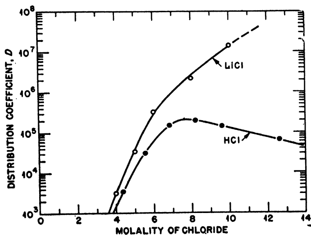
Slide 23. Adsorption of Ga(III) from HCl and LiCl solutions
