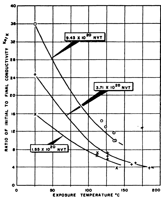
Figure 6. Variations in thermal conductivity of transverse cut CSF graphite with exposure temperature
