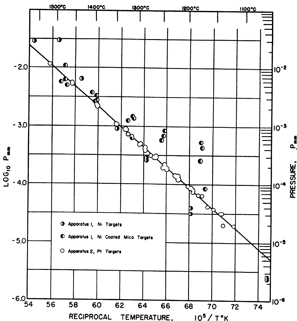
Figure 1. The vapor pressure of liquid plutonium
