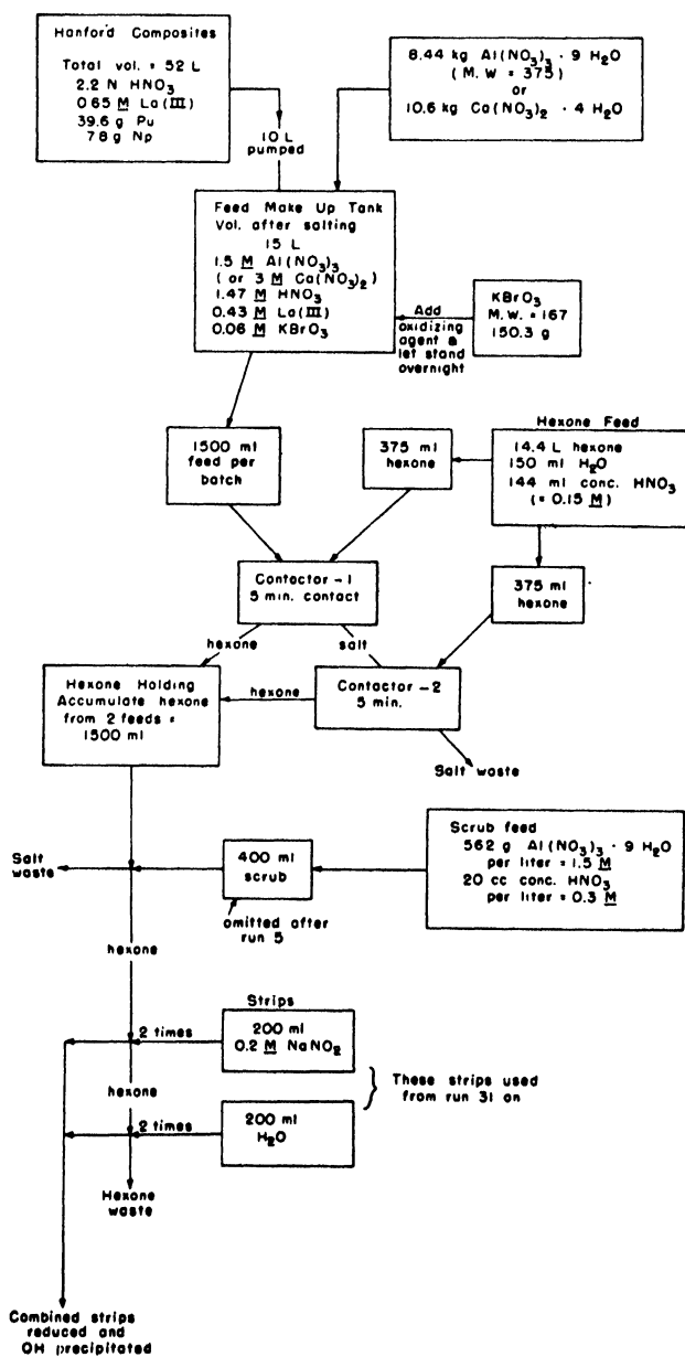
Figure 2. Cycle I: flowsheet IB; (used for runs 4-57)
