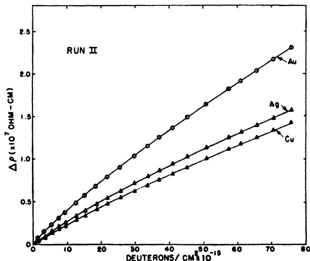
Figure 5. The changes of resistivity \Delta\rho of copper, silver and gold as functions of flux \Phi . The curves may be fitted accurately with a function of the form (36). (After Cooper)
