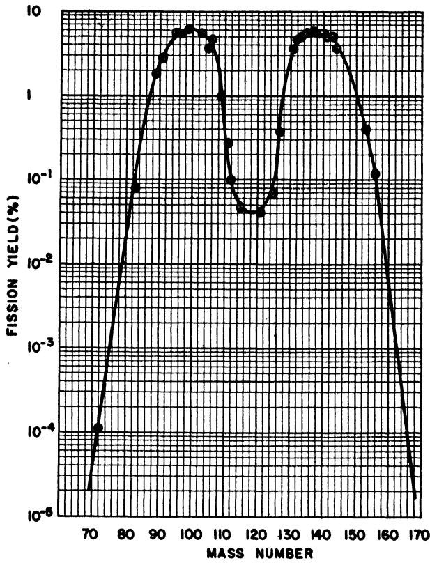
Figure 3. Yield-mass curve for slow neutron-induced fission of \text{Pu}^{239}
