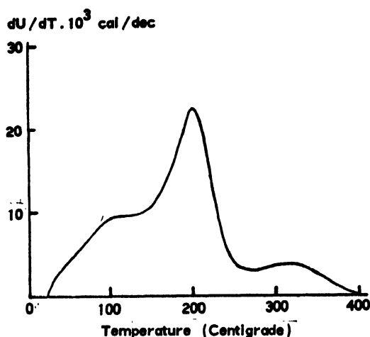
Figure 3. Excess heat evolution by NaCl irradiated with 350 Mev protons as a function of temperature rising at the rate of 2^\circ\text{C} per minute. Total flux 9.3 \times 10^{15} protons per \text{cm}^2 . Sample size 1.218 gm
