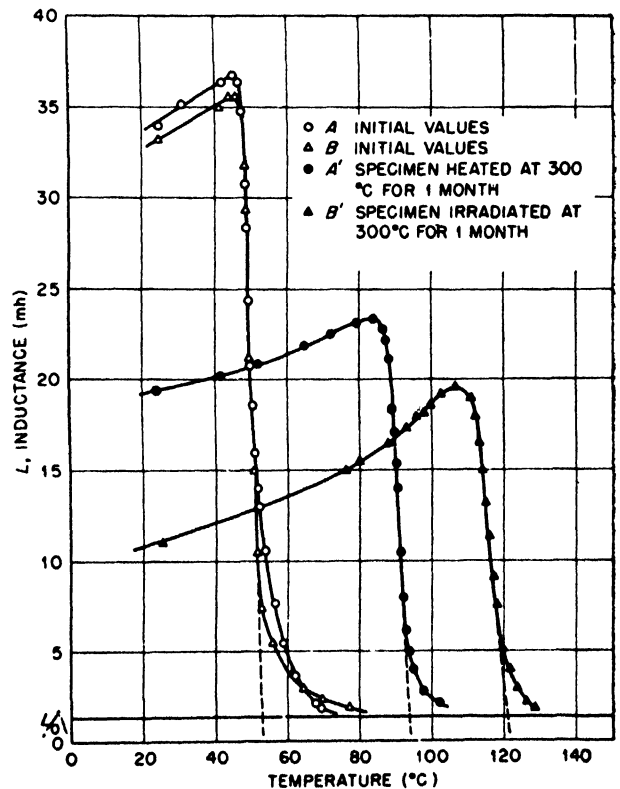
Slide 8. Inductance vs temperature curves for nickel-beryllium
