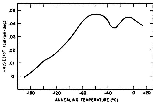
Figure 9. Annealing of stored energy at low temperatures
