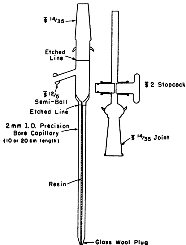
Figure 1. Unjacketed column and cap
