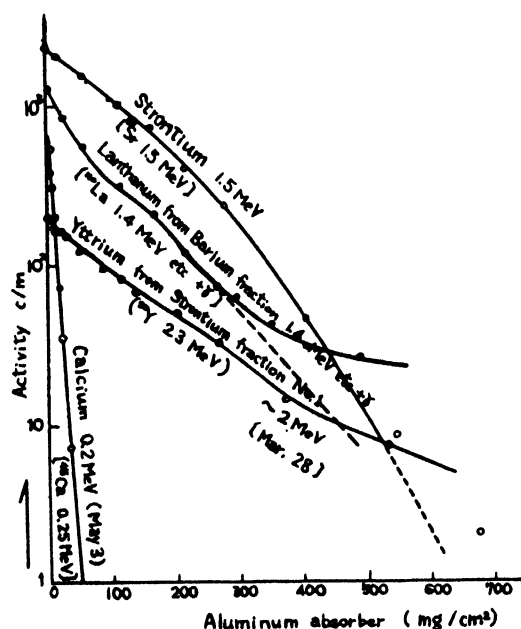
Figure 17. Aluminum absorption curves of \text{Sr}^{85} , \text{La}^{140} , \text{Y}^{90} and \text{Ca}^{45} fractions
