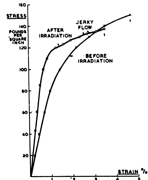
Slide 27. Effects of a short irradiation on the stress-strain characteristics of uranium
