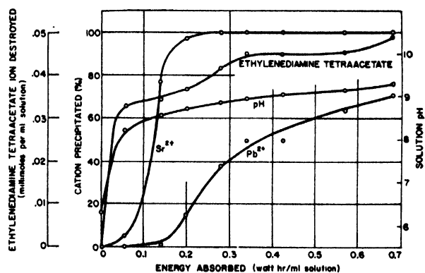
Figure 8. Radiation stability of ethylenediamine tetraacetate solution
