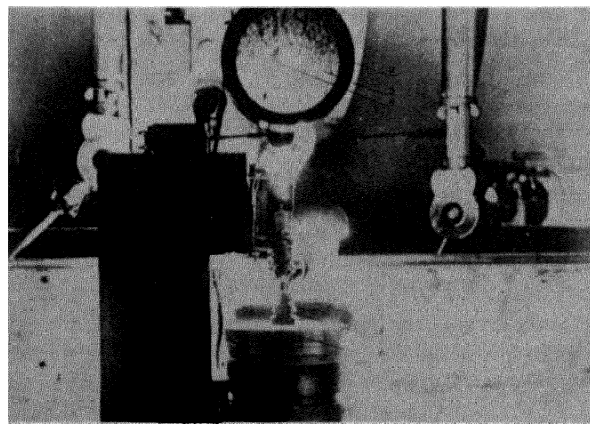
Slide 34. The remote-controlled instrument for measuring the microhardness of radioactive specimens, in operation
