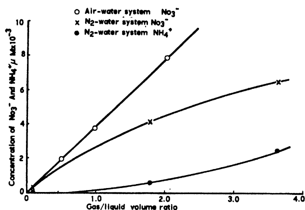
Figure 3. Variation of gas/liquid volume ratio at constant thermal neutron dose of 2.92 \times 10^{18} n-cm ^{-2}
