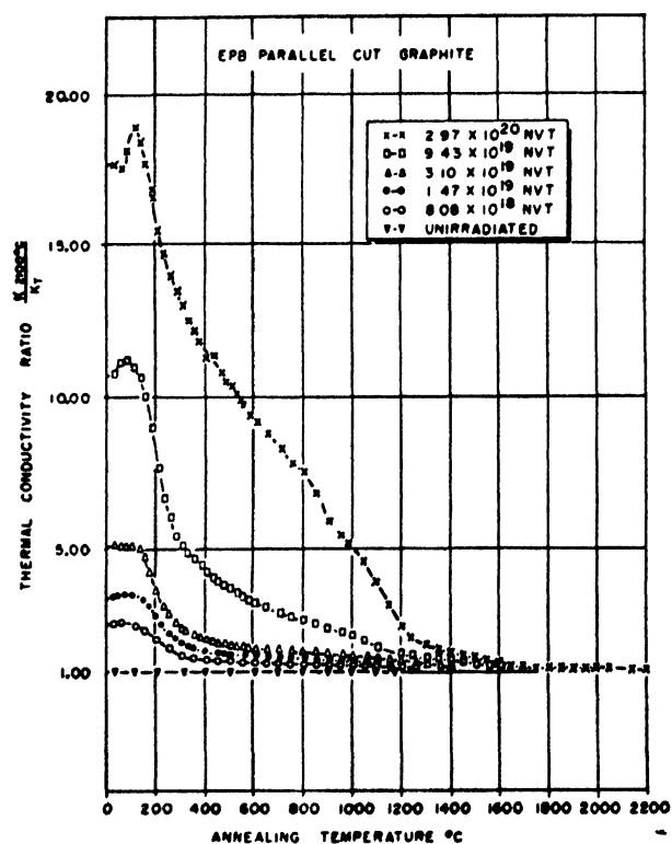
Figure 44. Pulse annealing of thermal conductivity damage
