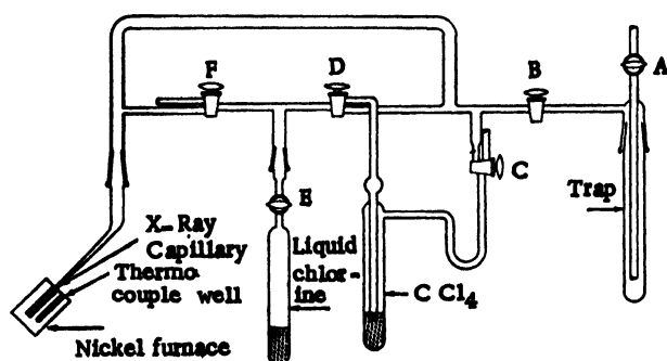
Figure 1. Apparatus for the preparation of chlorides
