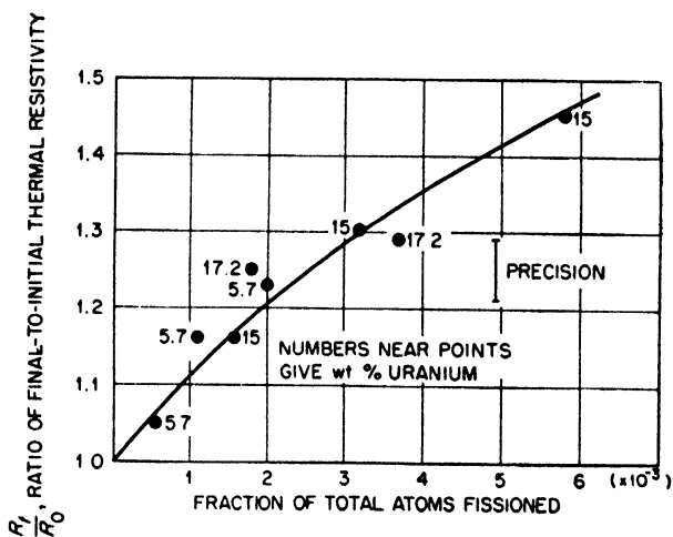
Figure 2. Effect of fission in aluminum-uranium alloys upon ratio of final-to-initial thermal resistivity
