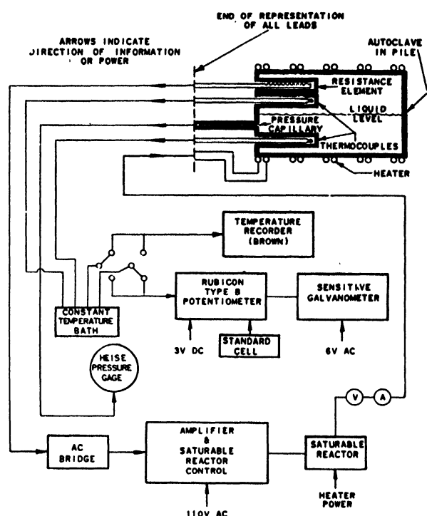
Figure 3. Schematic diagram of instrumentation and control
