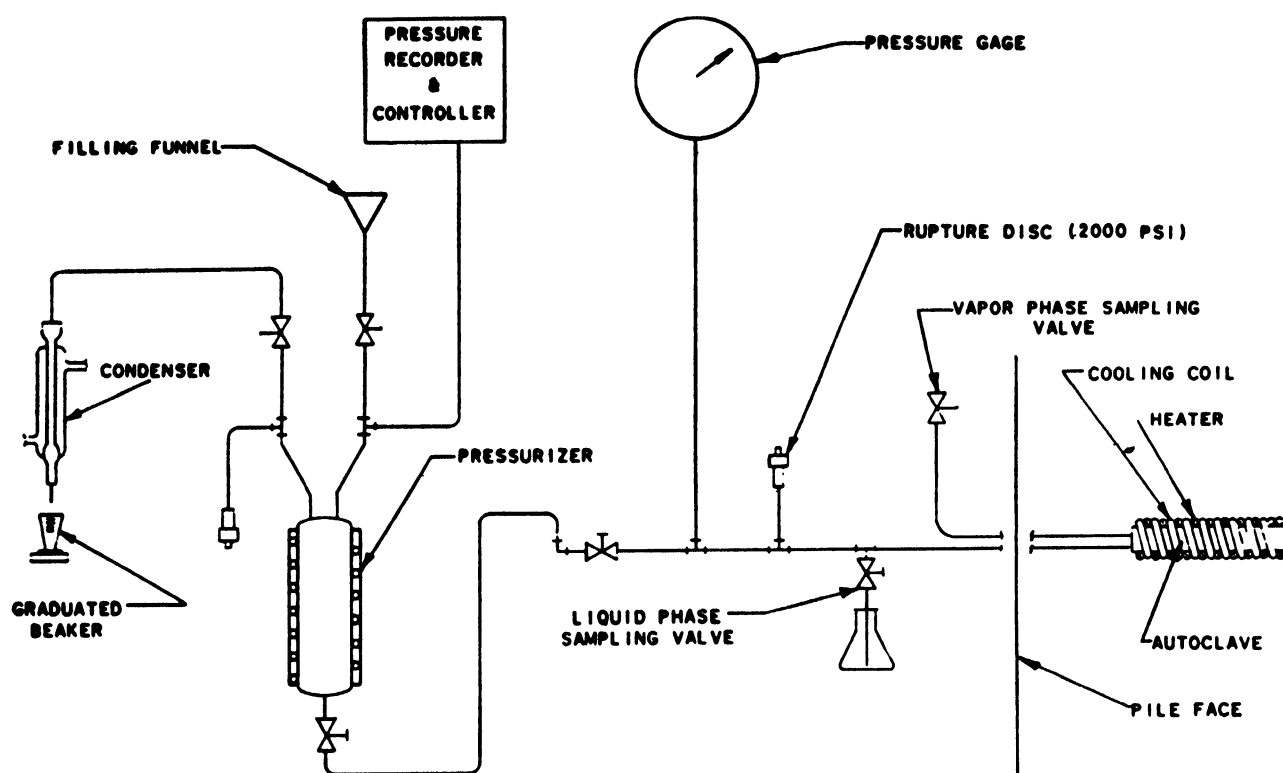
Figure 2. Pressure system
