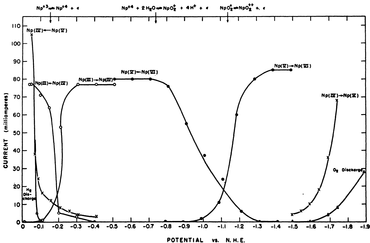
Figure 5. Current-voltage curves for oxidation-reduction reactions of neptunium
