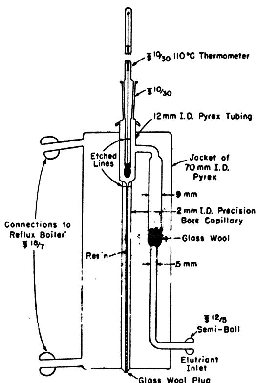
Figure 2. Jacketed column for non-room temperature experiments
