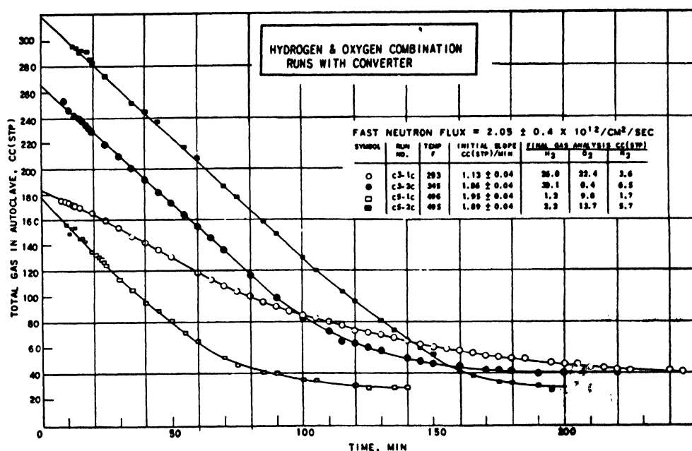
Figure 6. Hydrogen and oxygen combination runs with converter
