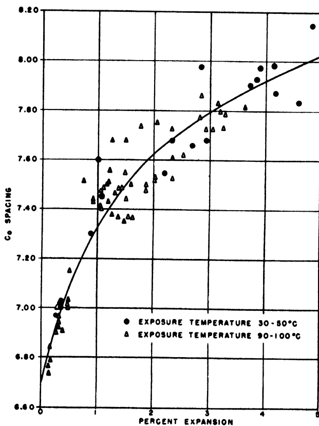
Figure 23. Expansion correlations for materials testing reactor irradiation; transverse cut CSF
