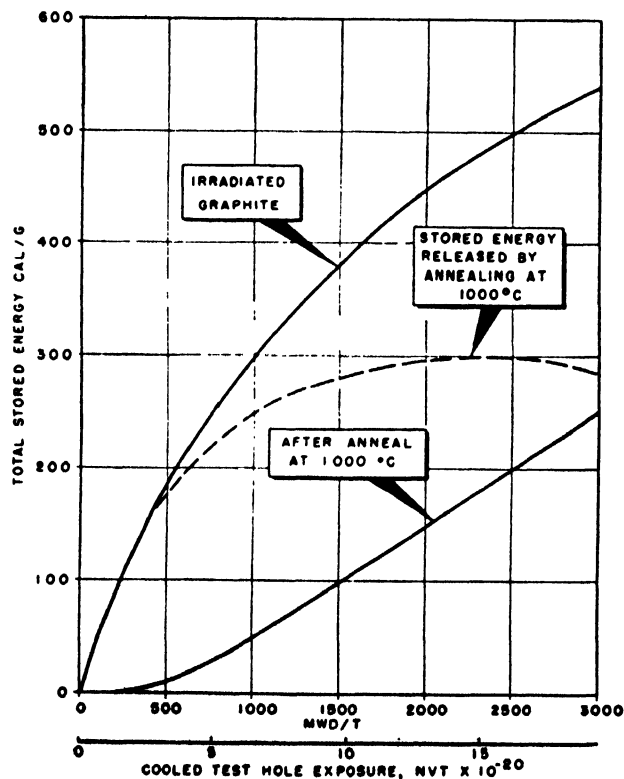
Figure 28. Build-up of total stored energy in irradiated graphite
