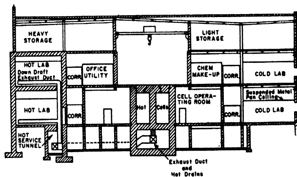
Figure 6. Isotope research building: section in elevation of a radiochemical laboratory building with hot down-draft exhaust in a basement service tunnel
