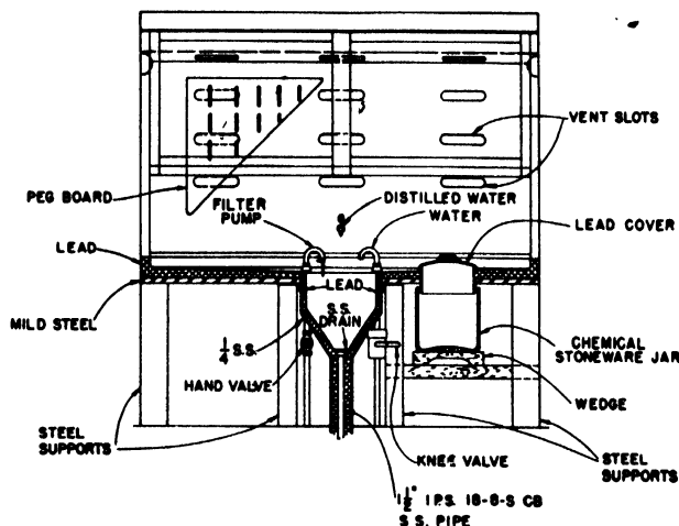
Figure 10. Hot waste and decontamination sink
