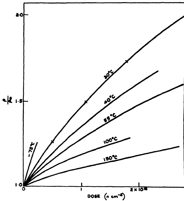
Figure 1. Changes of electrical resistivity at different irradiation temperatures
