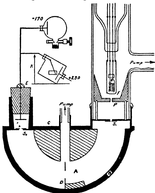
Fig. 7. Dempster's apparatus for detection of isotopes.
