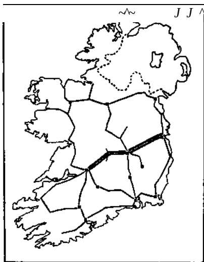
FIG. 103. SHANNON HYDRO-ELECTRIC POWER DISTRIBUTION SCHEME
