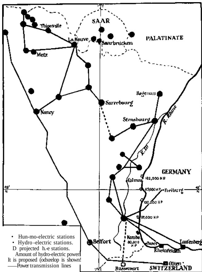
FIG. 15. MAP OF ELECTRICAL POWER DISTRIBUTION IN ALSACE-LORRAINE
