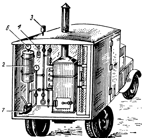
Fig. 28. General view of a portable steam-formalin disinfection chamber "AIHK" (after V.I. Vashkov)
