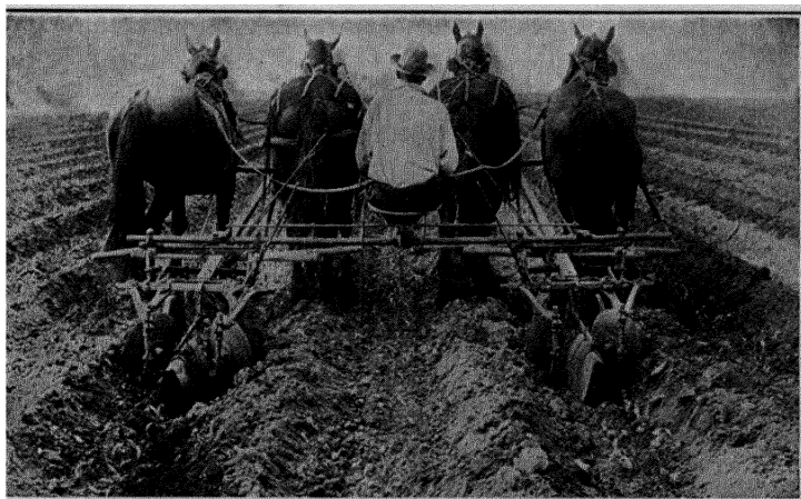
FIG. 40.—Lister two-row cultivator, illustrating method of throwing dirt away from the plants in the furrow the first time over. When the plants are larger the dirt will be thrown toward them.
