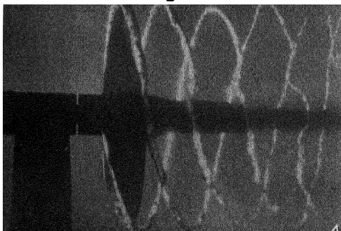
Photograph of the cavitations formed by a propeller in the experimental tank of the Parsons Marine Steam Turbine Co. The propeller is the disc-shaped object at the left centre of the photograph. There are three blades on it, and each is leaving a cork-screw line of bubbles in the water which goes past the blade. We can see where the spirals begin at the screw.
