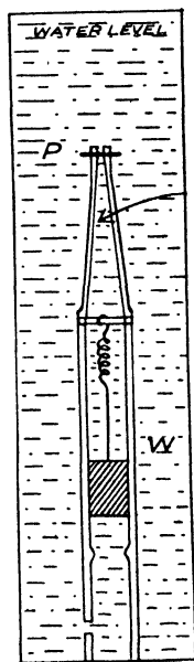
FIG. 15.—Parsons' water hammer.
