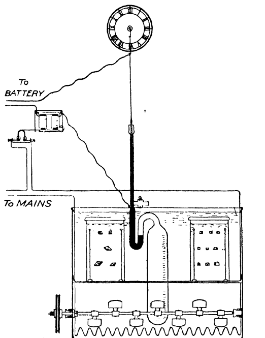
FIG. 28.—The thermostat.
