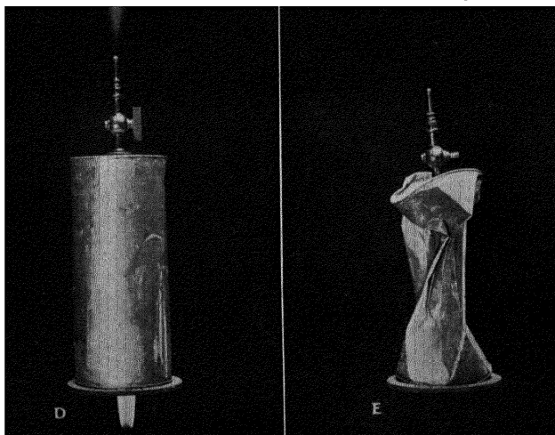
The water in the tin was boiling vigorously when the Bunsen burner was removed and the stop-cock closed. When cold water was poured over it, it collapsed.
