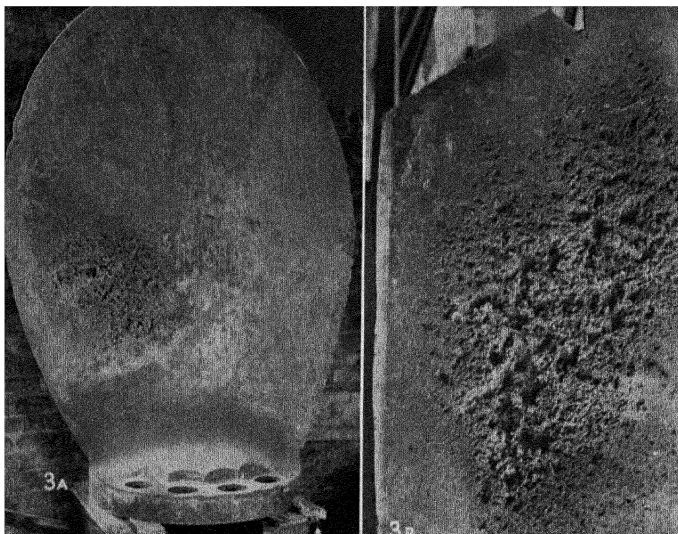
The right-hand figure shows erosion in a portion of an early propeller blade of the "Mauretania" Notice the small bite in the edge of the blade shown in full in the left-hand figure.
