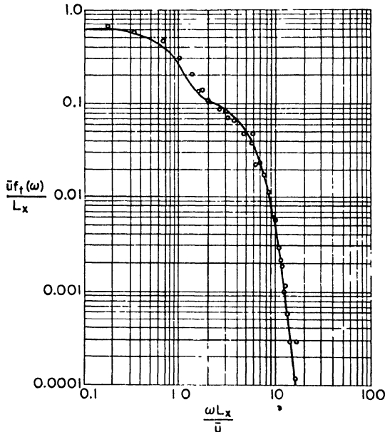
FIG. 9. Typical spectrum of turbulence at a fixed point in a wind tunnel stream 40 mesh lengths downstream of a grid.
