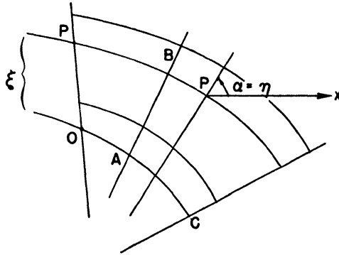
FIG. 14. Characteristic coordinates in simple wave.
