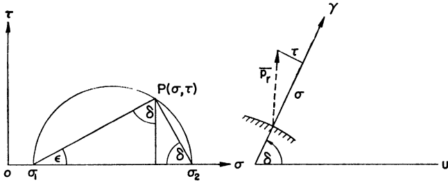
FIG. 4. Mohr's circle.
