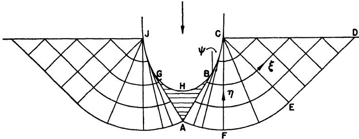
FIG. 28. Curved indenter.
