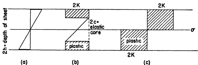
FIG. 15. Stresses in bent slab.
