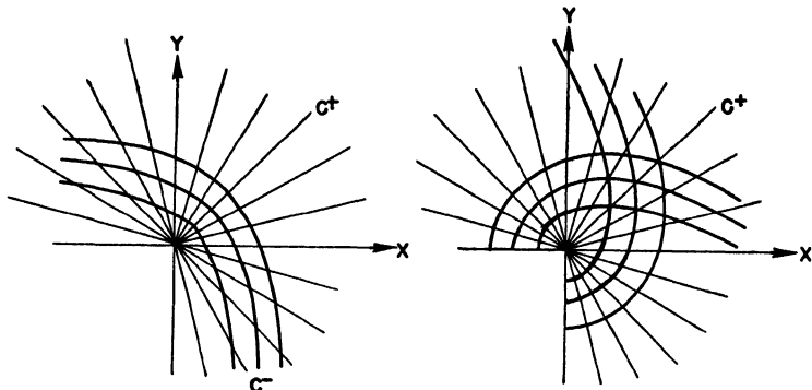
FIG. 13. (a) Parabola limit; straight characteristics and cross characteristics. (b) Parabola limit; lines of principal stress.
