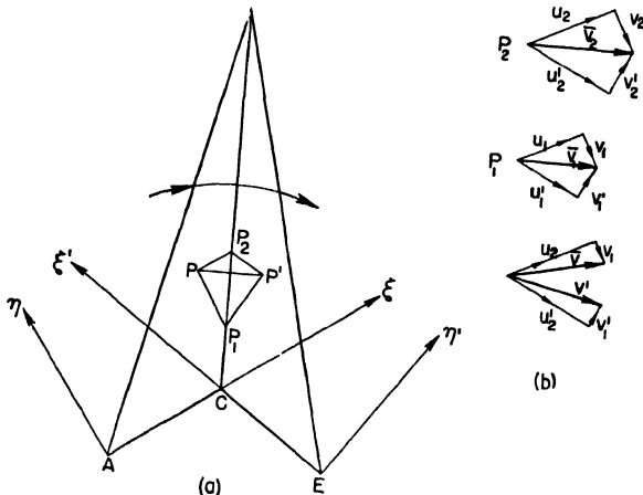
FIG. 23. Velocity solution for wedge (Fig. 20).
