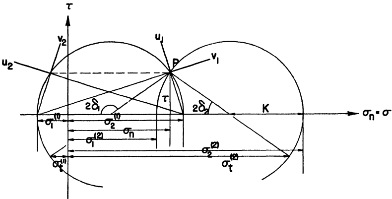
FIG. 18. Mohr circles of two stress tensors having one stress vector in common (stress discontinuity).
