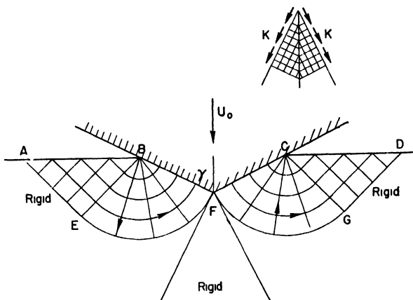
FIG. 26. Straight sided indenter.
