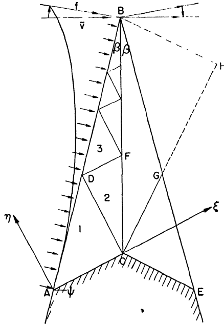
FIG. 20. Wedge under one-sided pressure.
