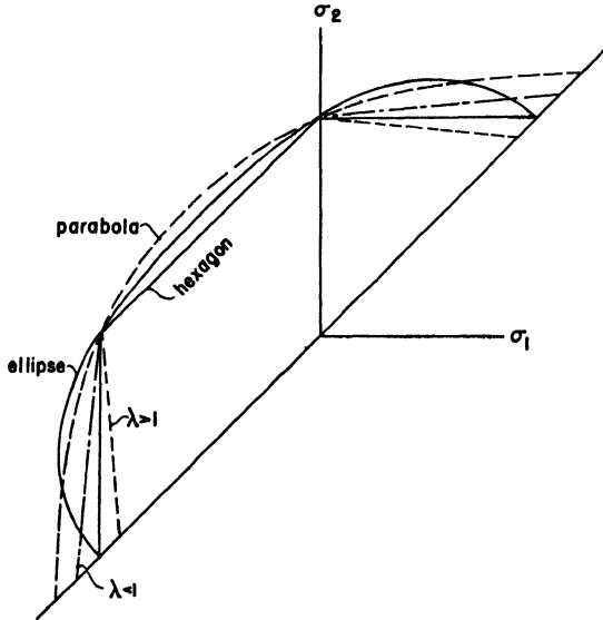
FIG. 2. Generalized Saint Venant conditions.
