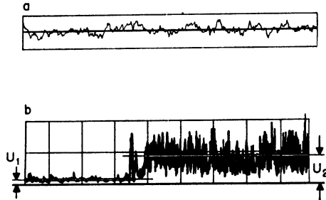
FIG. 4. Two typical turbulent velocity recordings: (a) in a wind tunnel stream, (b) in the natural wind.
