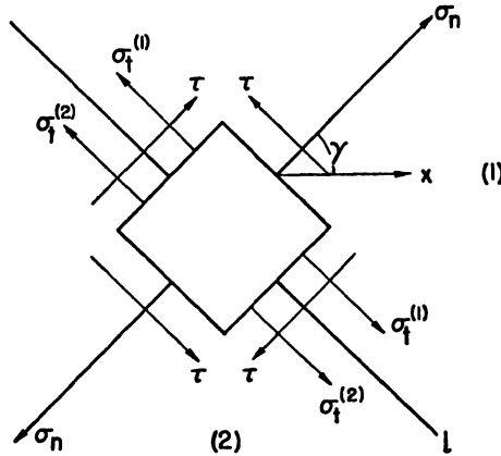
FIG. 16. Discontinuous stresses in plane strain.
