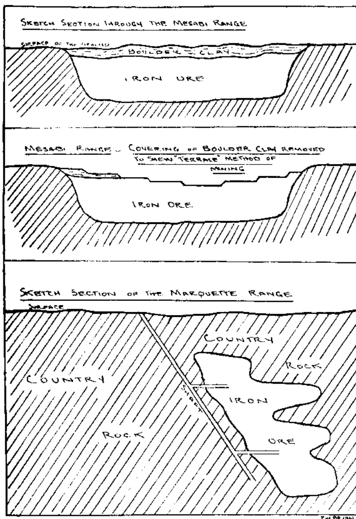
FIG. 67.—Diagrams to show Mining Conditions in the Lake Superior Country.
